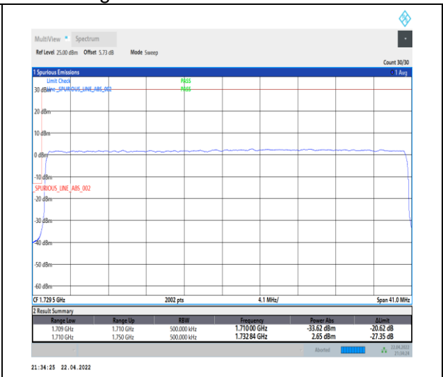
1-N66-PC3-15-40-L-3-DFT-PI2BPSK-Outer_Full-216@0-Ant0-seegraph-PASS-see graph
