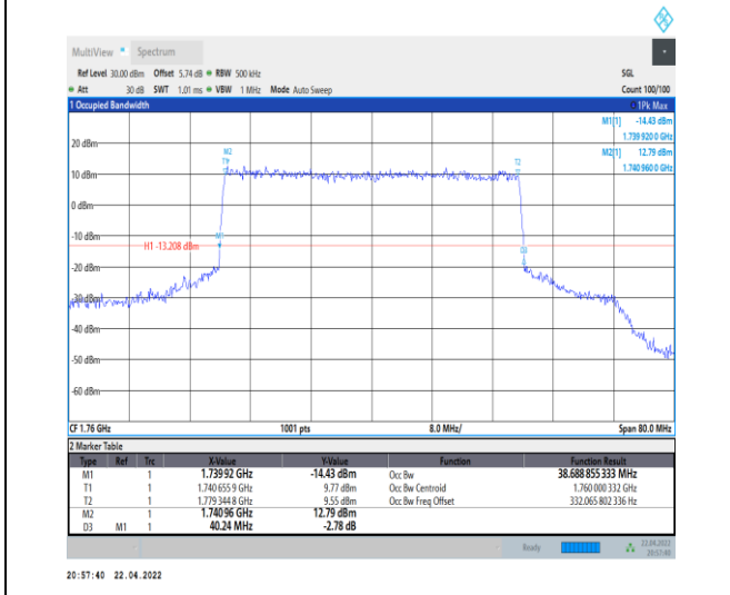
1-N66-PC3-15-40-H-6-CP-QPSK-Outer_Full-216 @ 0-Ant0-38.689-40.240-≤40-PASS
