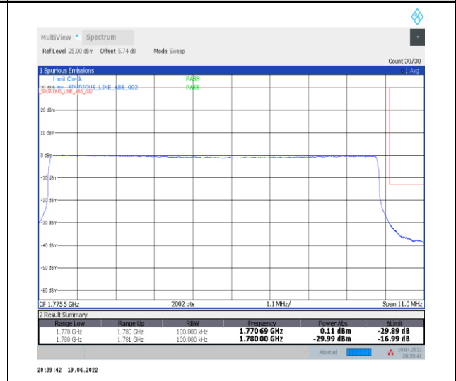
1-N66-PC3-15-10-H-6-CP-QPSK-Outer_Full-52@0-Ant0-seegraph-PASS-see graph
