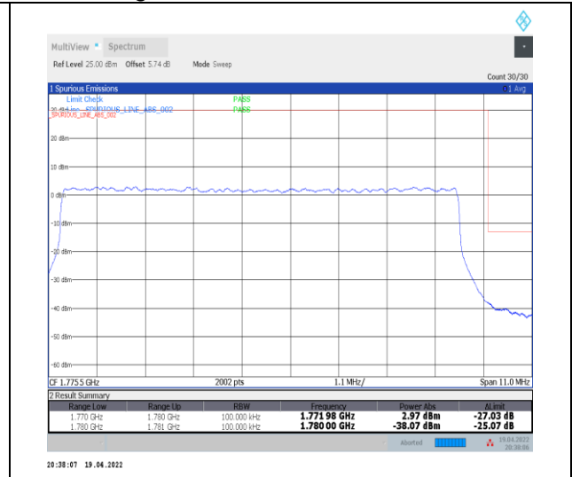
1-N66-PC3-15-10-H-3-DFT-PI2BPSK-Outer_Full-50@0-Ant0-seegraph-PASS-see graph
