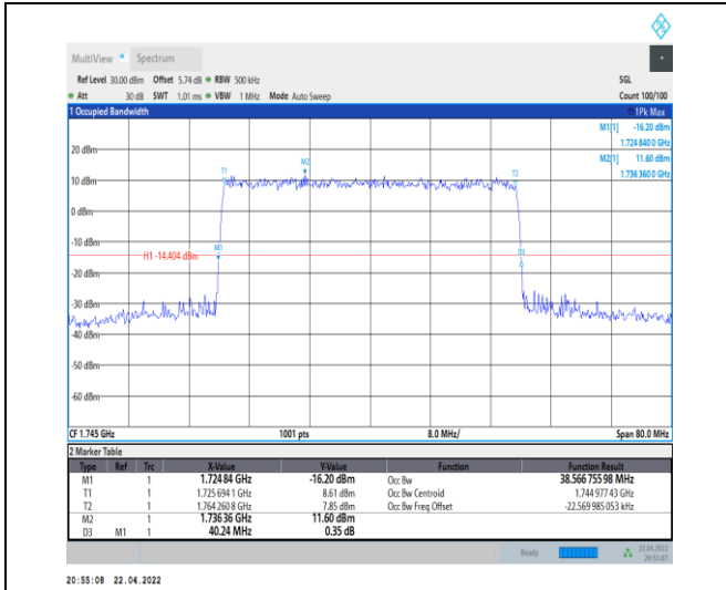
1-N66-PC3-15-40-M-5-DFT-256QAM-Outer_Full-216 @ 0-Ant0-38.567-40.240-≤40-PASS
