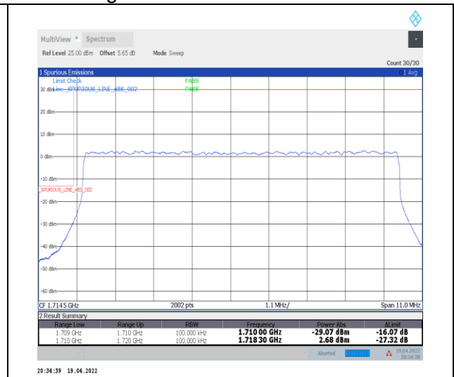
1-N66-PC3-15-10-L-3-DFT-PI2BPSK-Outer_Full-50@0-Ant0-seegraph-PASS-see graph
