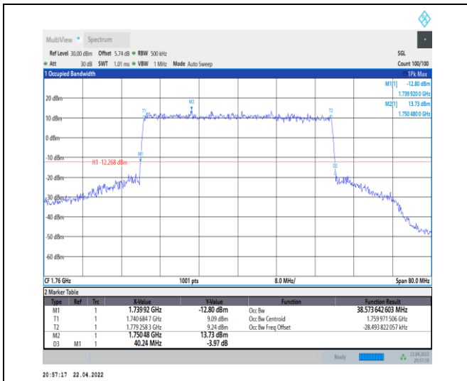
1-N66-PC3-15-40-H-4-DFT-64QAM-Outer_Full-216 @ 0-Ant0-38.574-40.240-≤40-PASS
