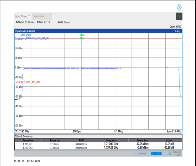
1-N66-PC3-15-30-L-6-CP-QPSK-Outer_Full-160@0-Ant0-seegraph-PASS-see graph
