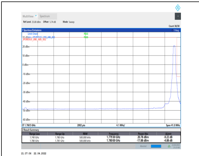
1-N66-PC3-15-40-H-2-DFT-PI2BPSK-Edge_1RB_Right-t-1@215-Ant0-seegraph-PASS-see graph
