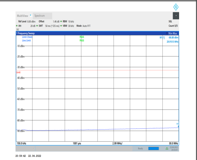
1-N66-PC3-15-40-M-1-DFT-PI2BPSK-Inner_1RB_Le ft-1@1-0.15-30-Ant0--86.88--33-PASS
