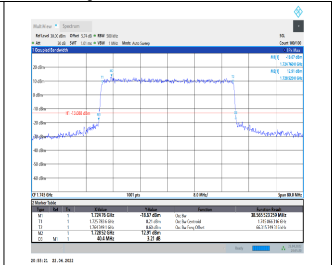
1-N66-PC3-15-40-M-6-CP-QPSK-Outer_Full-216 @ 0-Ant0-38.566-40.400-≤40-PASS
