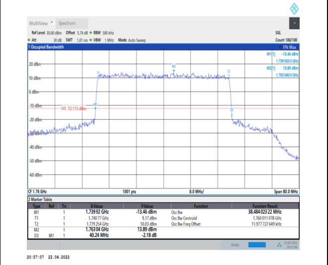
1-N66-PC3-15-40-H-3-DFT-16QAM-Outer_Full-216 @ 0-Ant0-38.484-40.240-≤40-PASS
