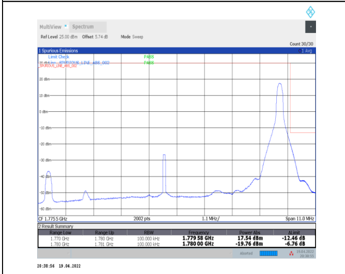
1-N66-PC3-15-10-H-5-CP-QPSK-Edge_1RB_Right-1@51-Ant0-seegraph-PASS-see graph
