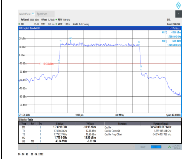
1-N66-PC3-15-40-H-2-DFT-PI2BPSK-Outer_Full-216 @ 0-Ant0-38.563-40.240-≤40-PASS
