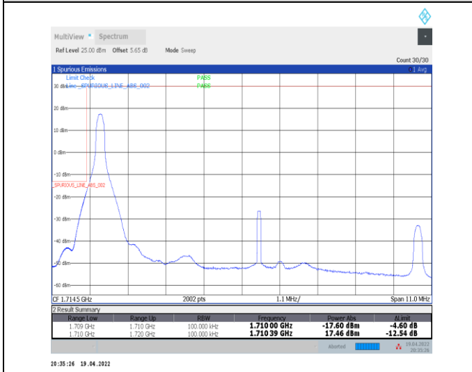
1-N66-PC3-15-10-L-4-CP-QPSK-Edge_1RB_Left-1@0-Ant0-seegraph-PASS-see graph
