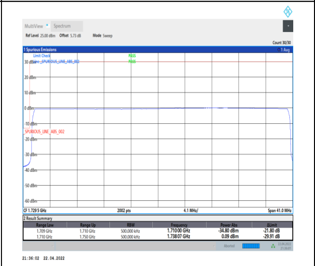
1-N66-PC3-15-40-L-6-CP-QPSK-Outer_Full-216@0-Ant0-seegraph-PASS-see graph
