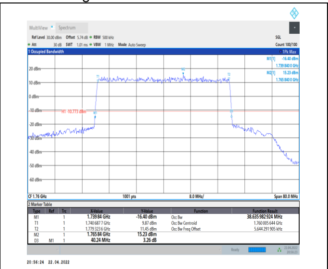
1-N66-PC3-15-40-H-1-DFT-QPSK-Outer_Full-216 @ 0-Ant0-38.636-40.240-≤40-PASS
