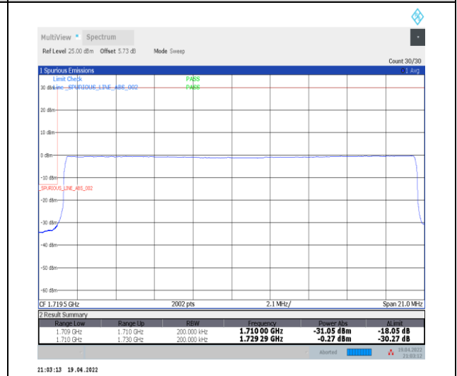
1-N66-PC3-15-20-L-6-CP-QPSK-Outer_Full-106@0-Ant0-seegraph-PASS-see graph
