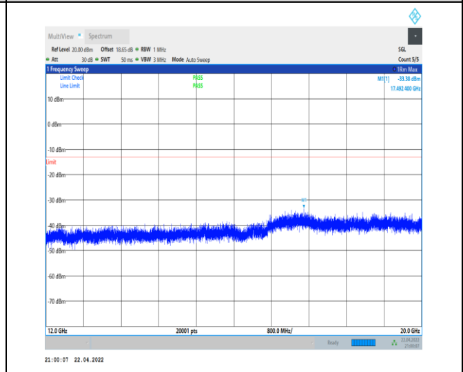
1-N66-PC3-15-40-M-1-DFT-PI2BPSK-Inner_1RB_Le ft-1@1-12000-20000-Ant0--33.38--13-PASS
