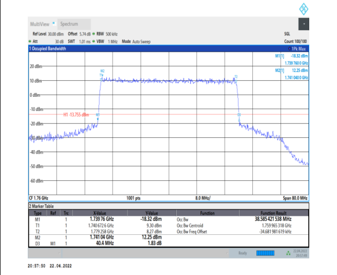
1-N66-PC3-15-40-H-7-CP-16QAM-Outer_Full-216 @ 0-Ant0-38.585-40.400-≤40-PASS
