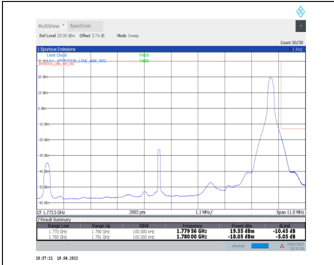
1-N66-PC3-15-10-H-2-DFT-PI2BPSK-Edge_1RB_Right-t-1@51-Ant0-seegraph-PASS-see graph
