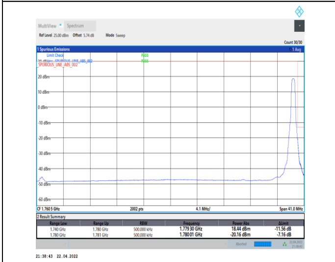
1-N66-PC3-15-40-H-5-CP-QPSK-Edge_1RB_Right-1@215-Ant0-seegraph-PASS-see graph
