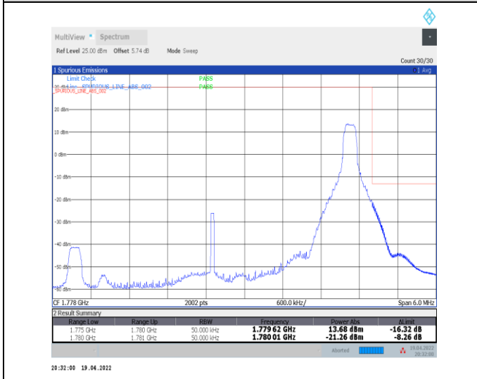
1-N66-PC3-15-5-H-5-CP-QPSK-Edge_1RB_Right-1@24-Ant0-seegraph-PASS-see graph
