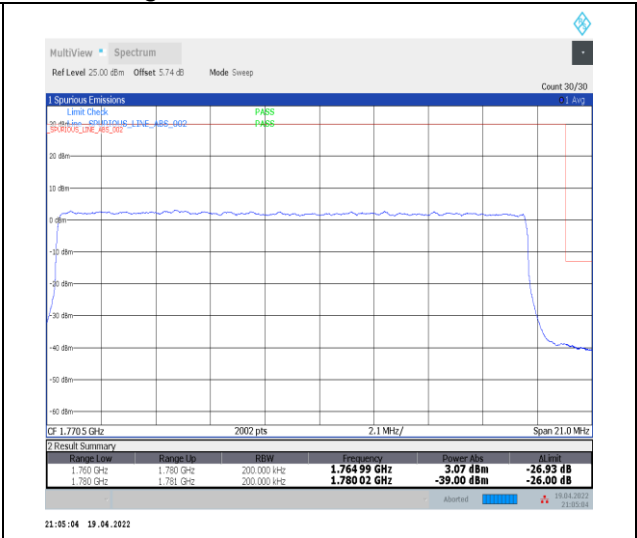
1-N66-PC3-15-20-H-3-DFT-PI2BPSK-Outer_Full-100@0-Ant0-seegraph-PASS-see graph
