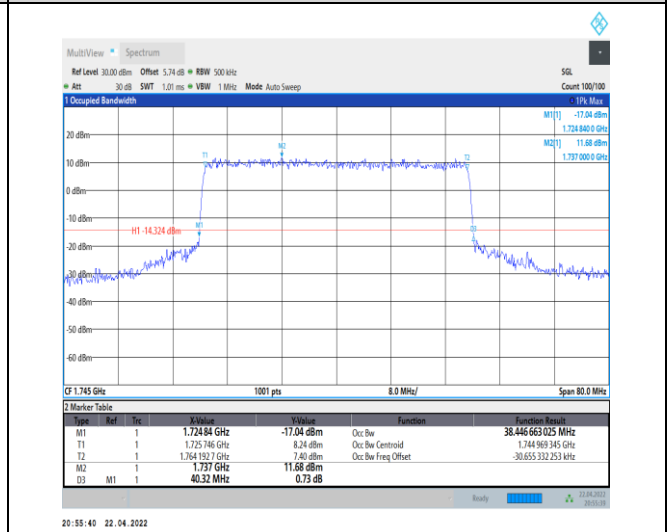
1-N66-PC3-15-40-M-8-CP-64QAM-Outer_Full-216 @ 0-Ant0-38.447-40.320-≤40-PASS
