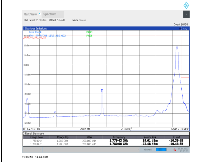
1-N66-PC3-15-20-H-5-CP-QPSK-Edge_1RB_Right-1@105-Ant0-seegraph-PASS-see graph
