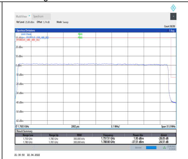
1-N66-PC3-15-30-H-3-DFT-PI2BPSK-Outer_Full-160@0-Ant0-seegraph-PASS-see graph
