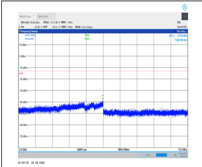
1-N66-PC3-15-40-L-1-DFT-PI2BPSK-Inner_1RB_Le ft-1@1-3000-12000-Ant0--37.90--13-PASS
