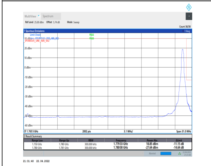
1-N66-PC3-15-30-H-5-CP-QPSK-Edge_1RB_Right-1@159-Ant0-seegraph-PASS-see graph
