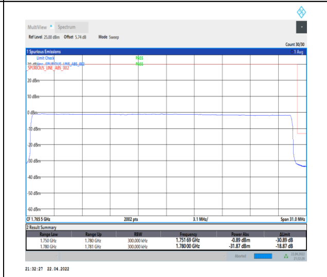
1-N66-PC3-15-30-H-6-CP-QPSK-Outer_Full-160@0-Ant0-seegraph-PASS-see graph
