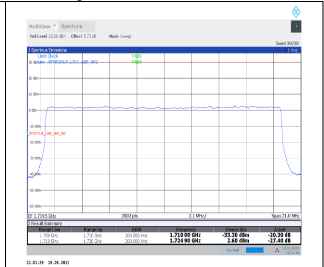
1-N66-PC3-15-20-L-3-DFT-PI2BPSK-Outer_Full-100@0-Ant0-seegraph-PASS-see graph
