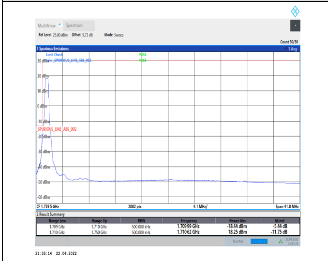
1-N66-PC3-15-40-L-4-CP-QPSK-Edge_1RB_Left-1@0-Ant0-seegraph-PASS-see graph
