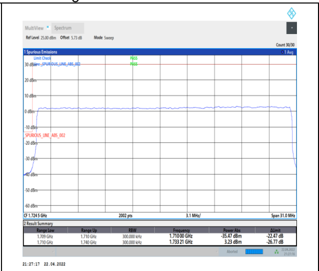
1-N66-PC3-15-30-L-3-DFT-PI2BPSK-Outer_Full-160@0-Ant0-seegraph-PASS-see graph
