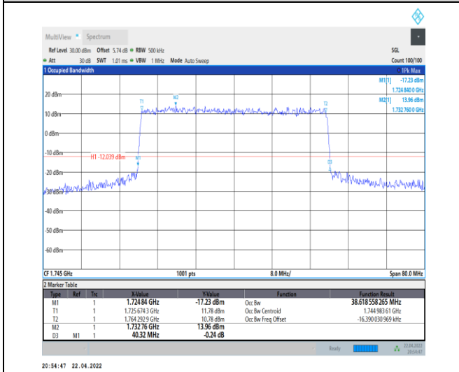
1-N66-PC3-15-40-M-3-DFT-16QAM-Outer_Full-216 @0-Ant0-38.619-40.320-≤40-PASS
