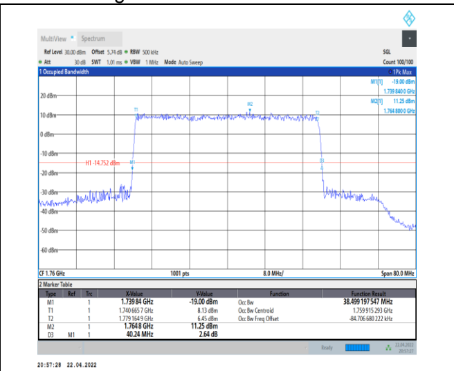
1-N66-PC3-15-40-H-5-DFT-256QAM-Outer_Full-216 @ 0-Ant0-38.499-40.240-≤40-PASS
