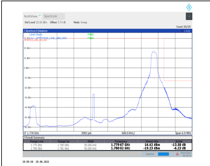
1-N66-PC3-15-5-H-2-DFT-PI2BPSK-Edge_1RB_Right-1@24-Ant0-seegraph-PASS-see graph
