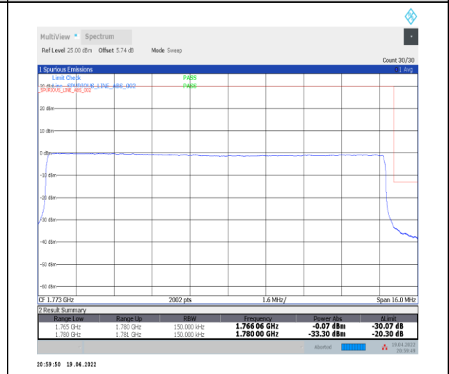
1-N66-PC3-15-15-H-6-CP-QPSK-Outer_Full-79@0-Ant0-seegraph-PASS-see graph
