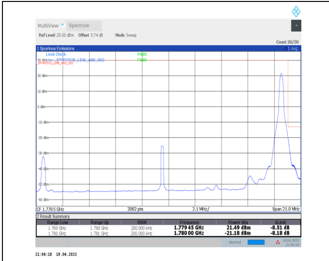
1-N66-PC3-15-20-H-2-DFT-PI2BPSK-Edge_1RB_Right-t-1@105-Ant0-seegraph-PASS-see graph
