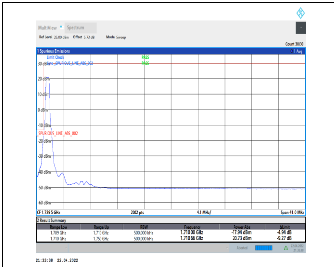
1-N66-PC3-15-40-L-1-DFT-PI2BPSK-Edge_1RB_Left-1@0-Ant0-seegraph-PASS-see graph
