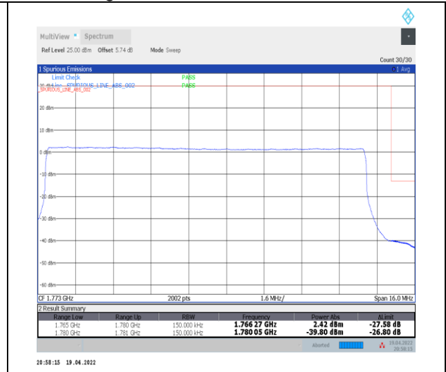
1-N66-PC3-15-15-H-3-DFT-PI2BPSK-Outer_Full-75@0-Ant0-seegraph-PASS-see graph
