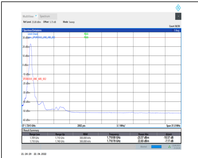
1-N66-PC3-15-30-L-1-DFT-PI2BPSK-Edge_1RB_Left-1@0-Ant0-seegraph-PASS-see graph
