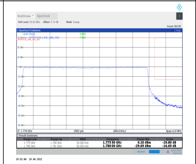
1-N66-PC3-15-5-H-6-CP-QPSK-Outer_Full-25@0-Ant0-seegraph-PASS-see graph
