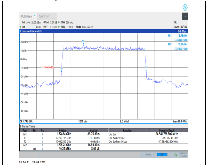
1-N66-PC3-15-40-M-2-DFT-PI2BPSK-Outer_Full-216@ 0-Ant0-38.542-40.240-≤40-PASS
