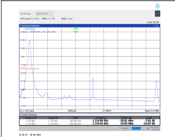
1-N66-PC3-15-20-L-4-CP-QPSK-Edge_1RB_Left-1@0-Ant0-seegraph-PASS-see graph
