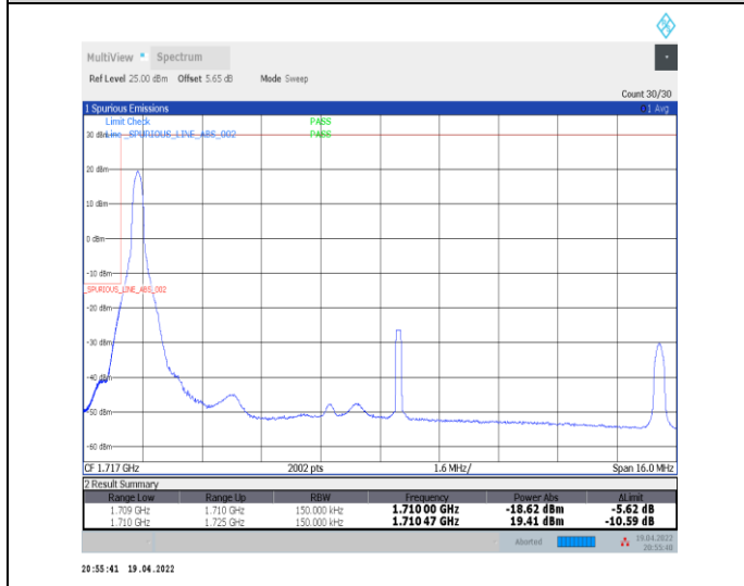
1-N66-PC3-15-15-L-4-CP-QPSK-Edge_1RB_Left-1@0-Ant0-seegraph-PASS-see graph
