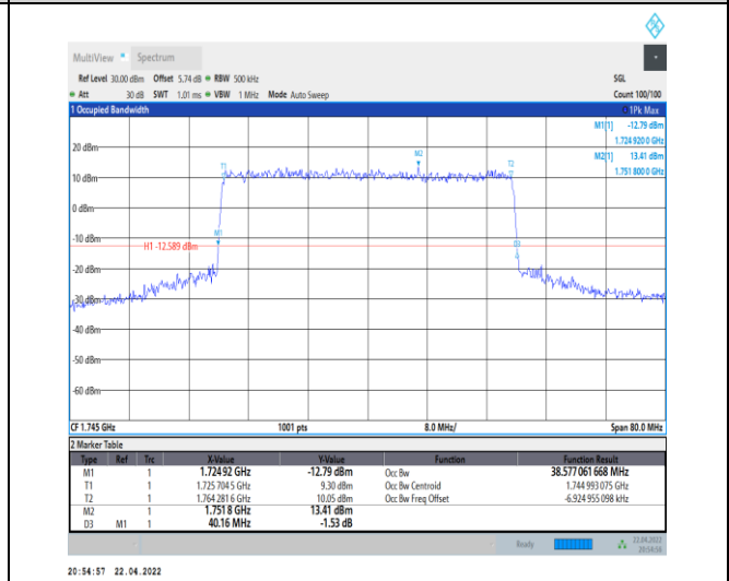
1-N66-PC3-15-40-M-4-DFT-64QAM-Outer_Full-216 @0-Ant0-38.577-40.160-≤40-PASS
