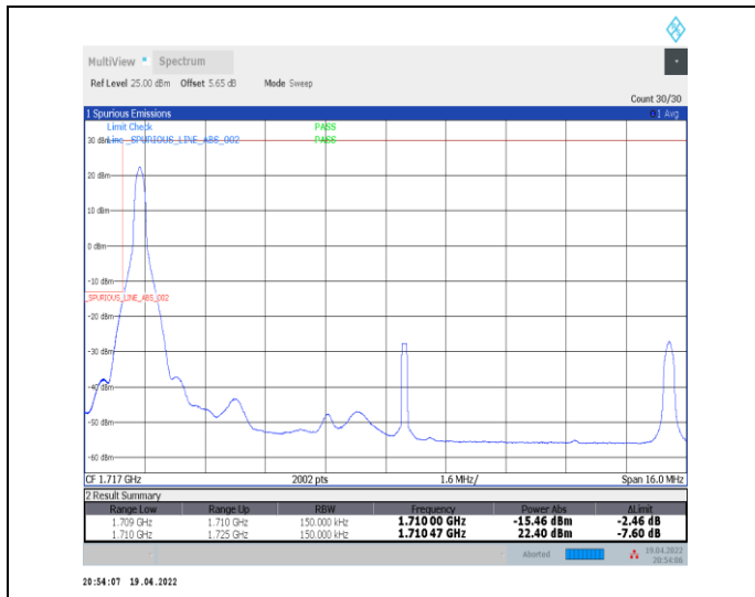
1-N66-PC3-15-15-L-1-DFT-PI2BPSK-Edge_1RB_Left-1@0-Ant0-seegraph-PASS-see graph
