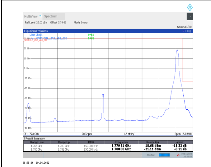
1-N66-PC3-15-15-H-5-CP-QPSK-Edge_1RB_Right-1@78-Ant0-seegraph-PASS-see graph
