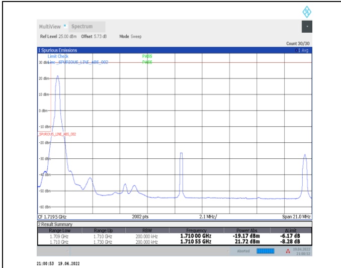
1-N66-PC3-15-20-L-1-DFT-PI2BPSK-Edge_1RB_Left-1@0-Ant0-seegraph-PASS-see graph
