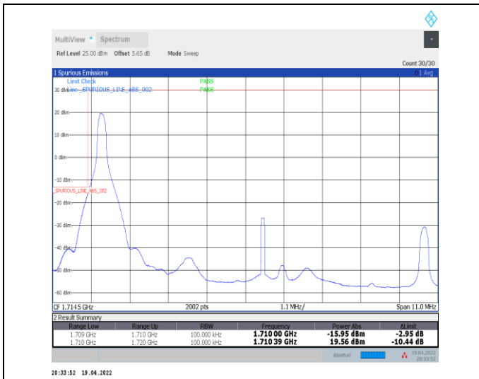
1-N66-PC3-15-10-L-1-DFT-PI2BPSK-Edge_1RB_Left-1@0-Ant0-seegraph-PASS-see graph
