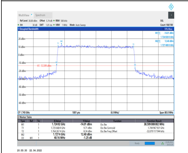
1-N66-PC3-15-40-M-7-CP-16QAM-Outer_Full-216 @ 0-Ant0-38.599-40.160-≤40-PASS
