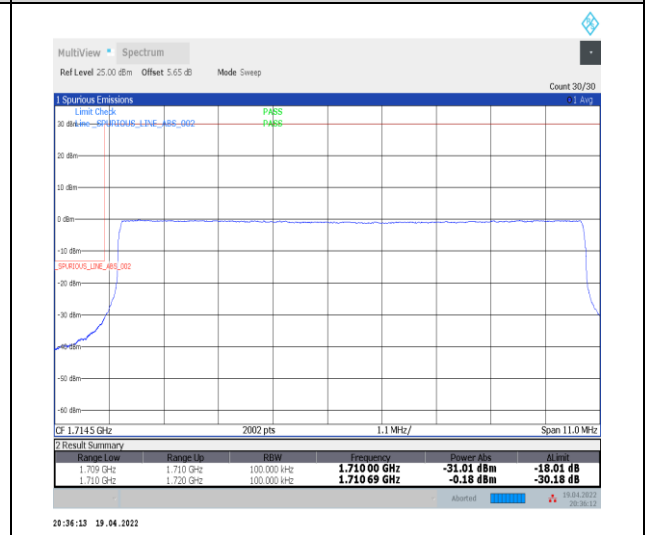
1-N66-PC3-15-10-L-6-CP-QPSK-Outer_Full-52@0-Ant0-seegraph-PASS-see graph
