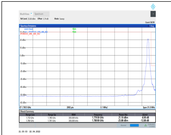
1-N66-PC3-15-30-H-2-DFT-PI2BPSK-Edge_1RB_Right-t-1@159-Ant0-seegraph-PASS-see graph
