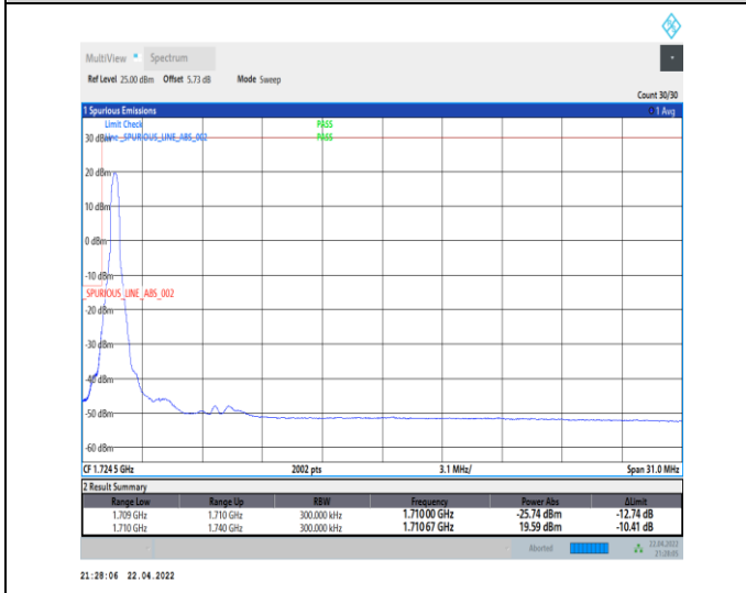
1-N66-PC3-15-30-L-4-CP-QPSK-Edge_1RB_Left-1@0-Ant0-seegraph-PASS-see graph
