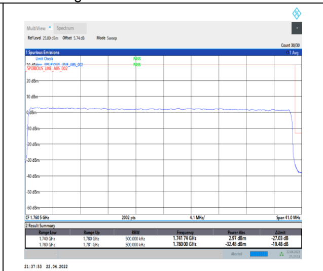
1-N66-PC3-15-40-H-3-DFT-PI2BPSK-Outer_Full-216@0-Ant0-seegraph-PASS-see graph
