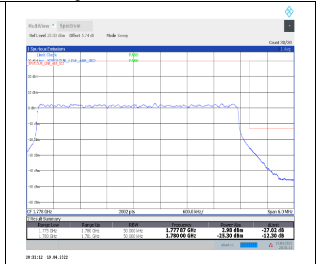
1-N66-PC3-15-5-H-3-DFT-PI2BPSK-Outer_Full-25@0-Ant0-seegraph-PASS-see graph
