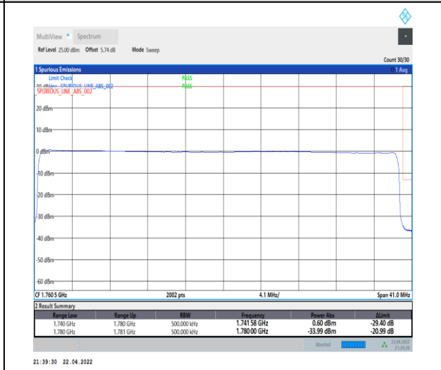
1-N66-PC3-15-40-H-6-CP-QPSK-Outer_Full-216@0-Ant0-seegraph-PASS-see graph
