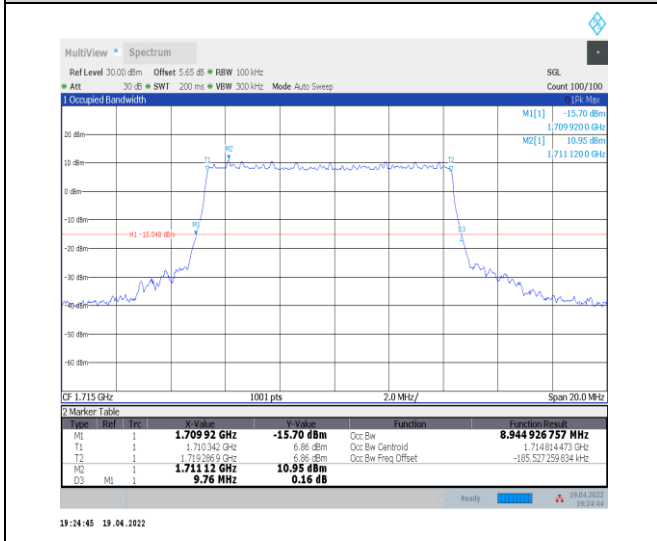
1-N66-PC3-15-10-L-4-DFT-64QAM-Outer_Full-50 @ 0-Ant0-8.945-9.760-≤10-PASS
