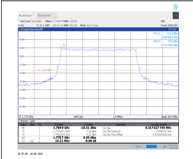
1-N66-PC3-15-10-H-6-CP-QPSK-Outer_Full-52@0- Ant0-9.318-10.220-≤10-PASS
