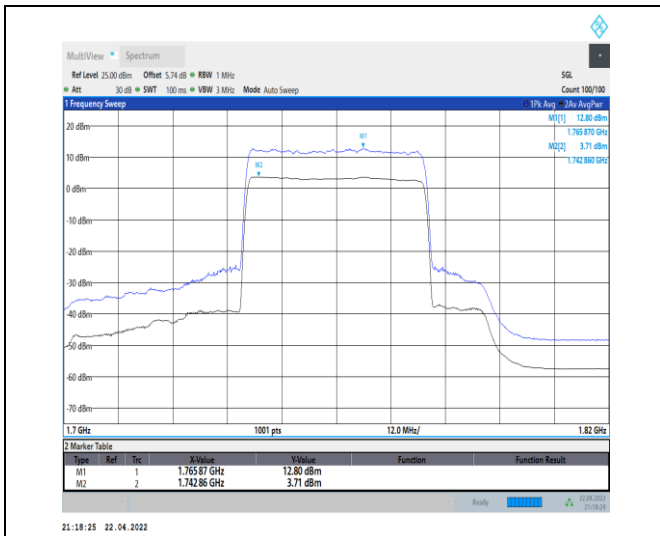
1-N66-PC3-15-40-H-1-DFT-256QAM-Outer_Full-216 @0-Ant0-9.09-100%-0.00-9.09-PASS-≤13
