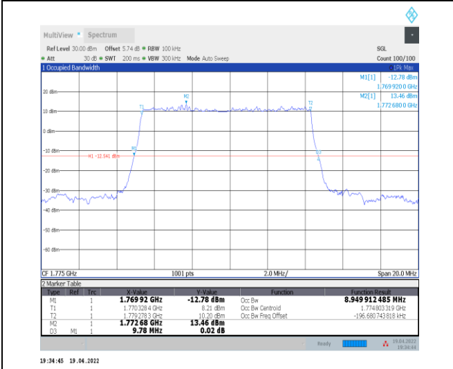
1-N66-PC3-15-10-H-2-DFT-PI2BPSK-Outer_Full-50 @0-Ant0-8.95-9.780-≤10-PASS
