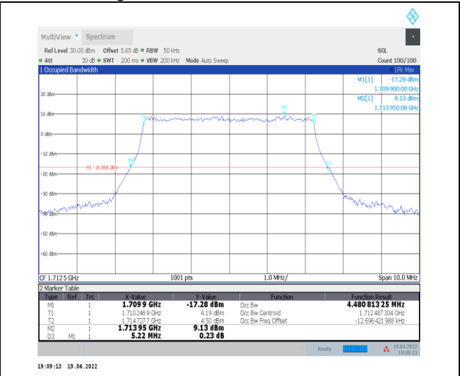
1-N66-PC3-15-5-L-6-CP-QPSK-Outer_Full-25@0-An t0-4.481-5.220-≤5-PASS
