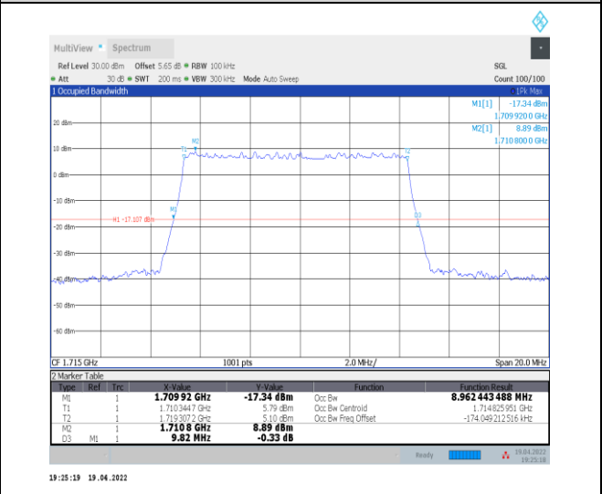
1-N66-PC3-15-10-L-5-DFT-256QAM-Outer_Full-50 @ 0-Ant0-8.962-9.820-≤10-PASS
