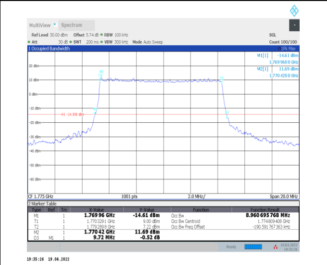
1-N66-PC3-15-10-H-3-DFT-16QAM-Outer_Full-50@ 0-Ant0-8.961-9.720-≤10-PASS
