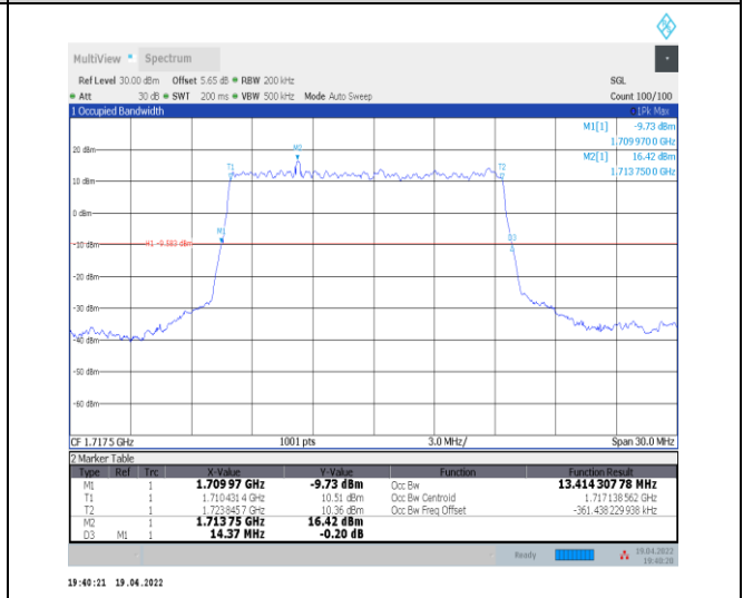
1-N66-PC3-15-15-L-2-DFT-PI2BPSK-Outer_Full-75@0 @0-Ant0-13.414-14.370-<=15-PASS
