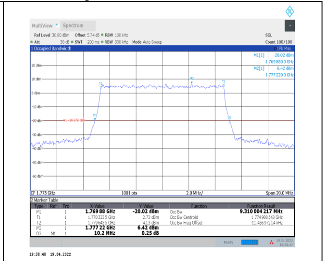
1-N66-PC3-15-10-H-9-CP-256QAM-Outer_Full-52@0 0-Ant0-9.31-10.200-<=10-PASS
