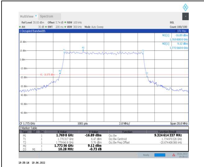
1-N66-PC3-15-10-H-8-CP-64QAM-Outer_Full-52@0 -Ant0-9.325-10.280-<=10-PASS
