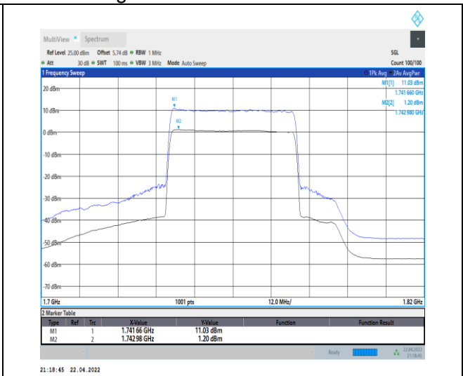
1-N66-PC3-15-40-H-2-CP-256QAM-Outer_Full-216 @0-Ant0-9.83-100%-0.00-9.83-PASS-≤13
