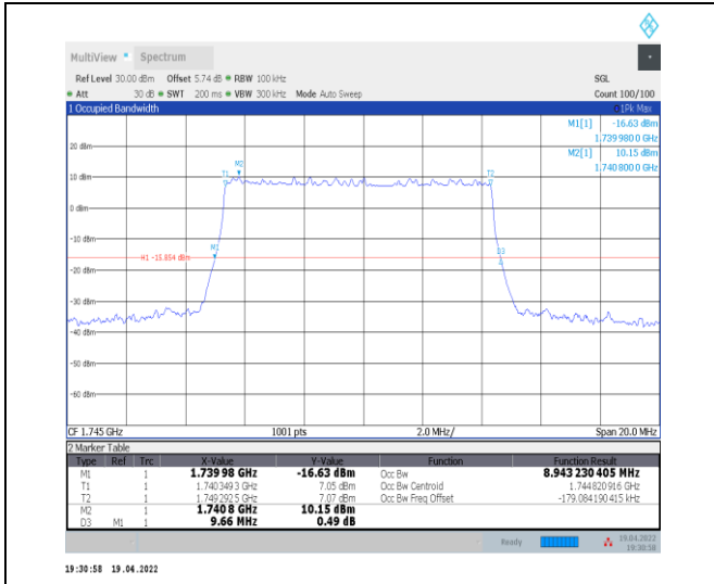
1-N66-PC3-15-10-M-5-DFT-256QAM-Outer_Full-50 @ 0-Ant0-8.943-9.660-≤10-PASS
