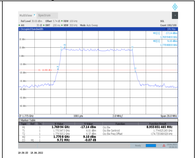
1-N66-PC3-15-10-H-5-DFT-256QAM-Outer_Full-50@ 0-Ant0-8.956-9.720-≤10-PASS
