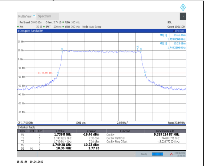
1-N66-PC3-15-10-M-6-CP-QPSK-Outer_Full-52 @ 0-Ant0-9.319-10.360-≤10-PASS
