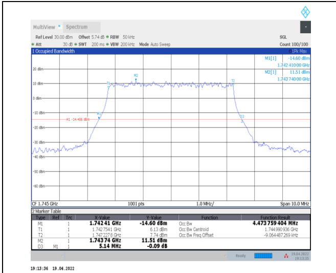
1-N66-PC3-15-5-M-4-DFT-64QAM-Outer_Full-25@0 -Ant0-4.474-5.140-≤5-PASS
