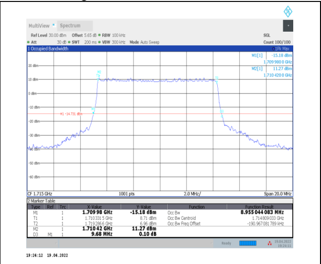
1-N66-PC3-15-10-L-3-DFT-16QAM-Outer_Full-50 @ 0-Ant0-8.955-9.680-≤10-PASS
