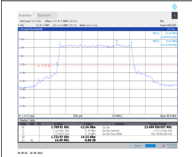
1-N66-PC3-15-15-L-1-DFT-QPSK-Outer_Full-75@0- Ant0-13.5-14.490-<=15-PASS
