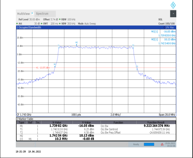
1-N66-PC3-15-10-M-8-CP-64QAM-Outer_Full-52 @ 0-Ant0-9.323-10.300-≤10-PASS
