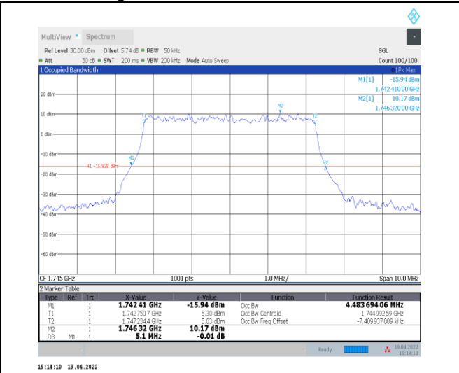
1-N66-PC3-15-5-M-5-DFT-256QAM-Outer_Full-25@0 0-Ant0-4.484-5.100-≤5-PASS
