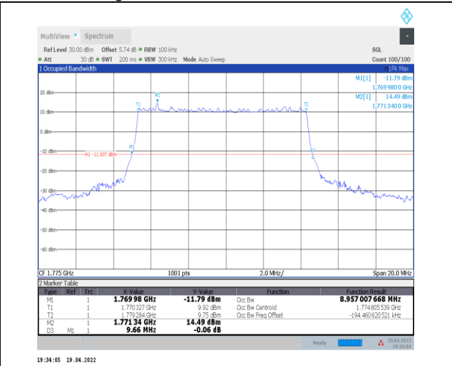
1-N66-PC3-15-10-H-1-DFT-QPSK-Outer_Full-50@0- Ant0-8.957-9.660-≤10-PASS
