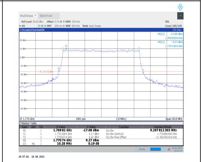
1-N66-PC3-15-10-H-7-CP-16QAM-Outer_Full-52@0- Ant0-9.298-10.280-≤10-PASS
