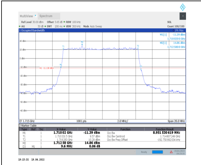
1-N66-PC3-15-10-L-2-DFT-PI2BPSK-Outer_Full-50 @ 0-Ant0-8.952-9.600-≤10-PASS
