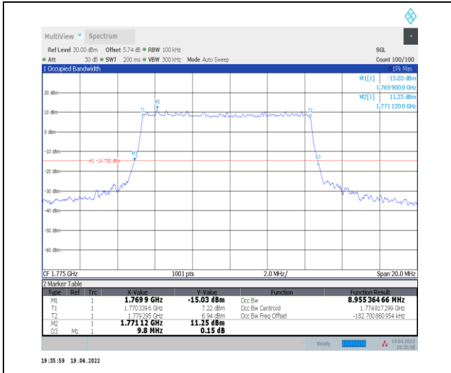
1-N66-PC3-15-10-H-4-DFT-64QAM-Outer_Full-50@ 0-Ant0-8.955-9.800-≤10-PASS
