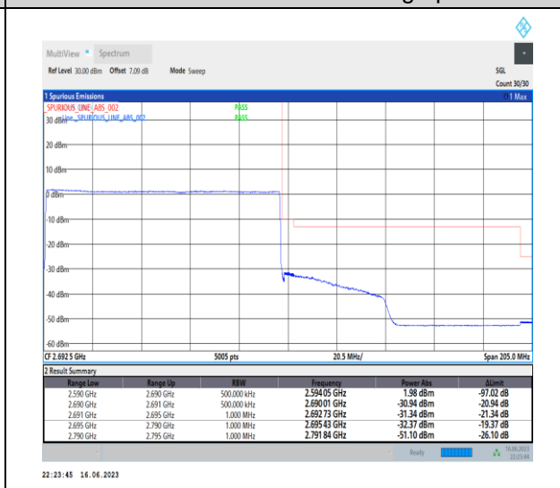
1-N41-PC1-30-100-H-6-CP-QPSK-Outer_Full-273 @0-Ant0-1--PASS-see graph
