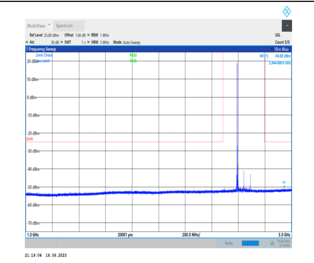
1-N41-PC1-30-100-H-1-DFT-QPSK-Edge_1RB_Left -1@0-1000-3000-Ant0-2944.60--50.83--25-PASS
