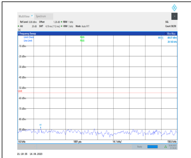
1-N41-PC1-30-100-H-1-DFT-QPSK-Edge_1RB_Left -1@0-0.009-0.15-Ant0-0.03--89.07--55-PASS
