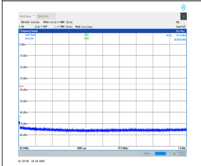
1-N41-PC1-30-100-H-1-DFT-QPSK-Edge_1RB_Left -1@0-30-1000-Ant0-30.97--67.18--35-PASS
