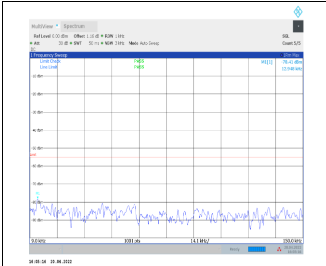
1-N41--30-100-H-1-DFT-PI2BPSK-Inner_1RB_Left-1 @ 1-0.009-0.15-Ant0--78.41--55-PASS
