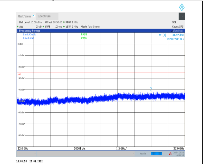
1-N41--30-100-H-1-DFT-PI2BPSK-Inner_1RB_Left-1 @ 1-12000-27000-Ant0--41.62--25-PASS
