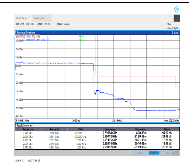
1-N41-PC1-30-100-H-3-DFT-PI2BPSK-Outer_Full-270@0-Ant0-1--PASS-see graph
