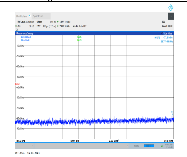
1-N41-PC1-30-100-H-1-DFT-QPSK-Edge_1RB_Left -1@0-0.15-30-Ant0-29.78--77.21--45-PASS
