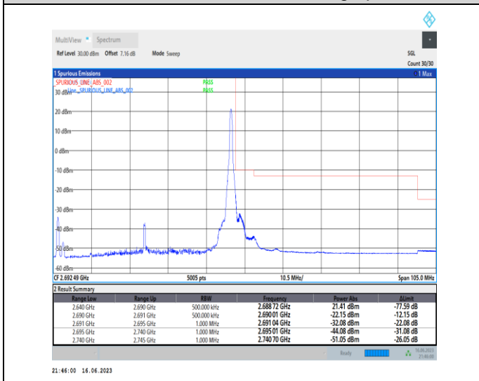
1-N41-PC1-30-50-H-5-CP-QPSK-Edge_1RB_Right-1 @132-Ant0-1--PASS-see graph
