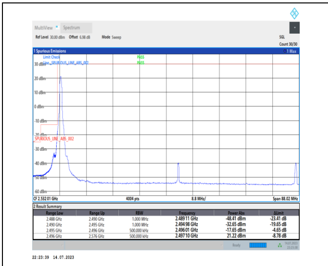
1-N41-PC1-30-80-L-1-DFT-PI2BPSK-Edge_1RB_Left -1@0-Ant0-1--PASS-see graph
