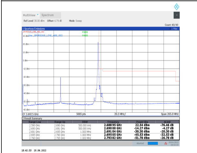
1-N41--30-100-H-5-CP-QPSK-Edge_1RB_Right-1 @27 2-Ant0-PASS-see graph
