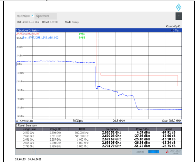
1-N41--30-100-H-3-DFT-PI2BPSK-Outer_Full-270 @0-Ant0-PASS-see graph
