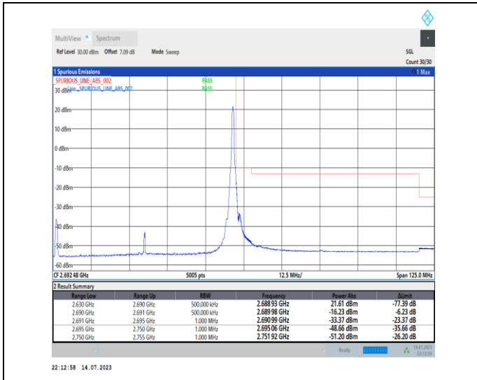
1-N41-PC1-30-60-H-2-DFT-PI2BPSK-Edge_1RB_Right t-1 @ 161-Ant0-1--PASS-see graph
