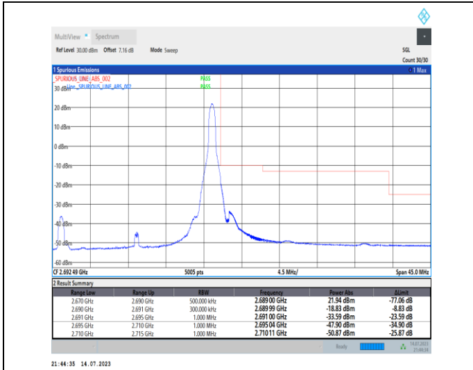
1-N41-PC1-30-20-H-2-DFT-PI2BPSK-Edge_1RB_Righ t-1@50-Ant0-1--PASS-see graph
