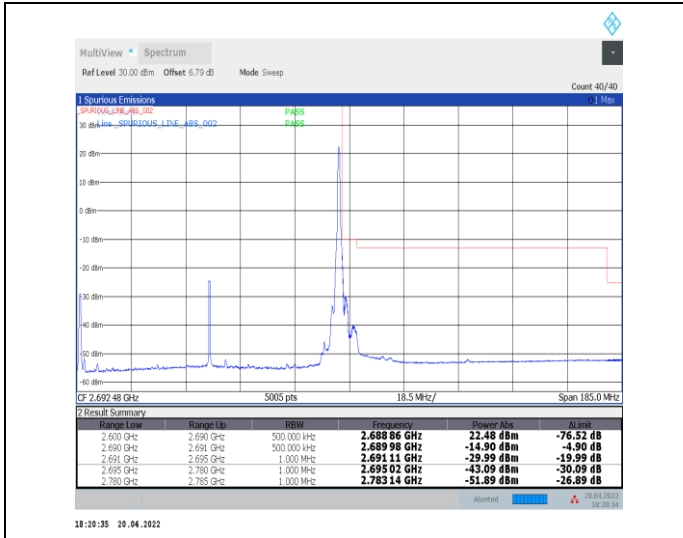
1-N41--30-90-H-2-DFT-PI2BPSK-Edge_1RB_Right-1@ 244-Ant0-PASS-see graph
