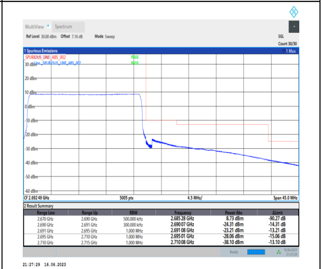
1-N41-PC1-30-20-H-6-CP-QPSK-Outer_Full-51 @ 0-Ant0-1--PASS-see graph
