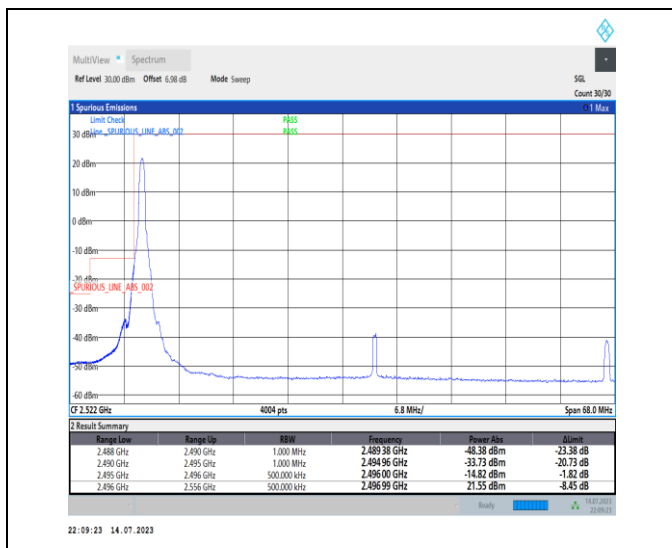
1-N41-PC1-30-60-L-1-DFT-PI2BPSK-Edge_1RB_Left -1@0-Ant0-1--PASS-see graph
