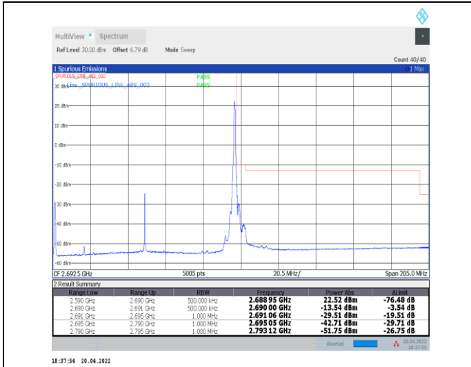
1-N41--30-100-H-2-DFT-PI2BPSK-Edge_1RB_Right-1 @272-Ant0-PASS-see graph
