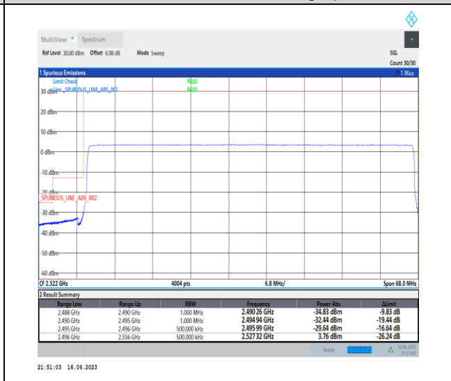
1-N41-PC1-30-60-L-6-CP-QPSK-Outer_Full-162@0 -Ant0-1--PASS-see graph
