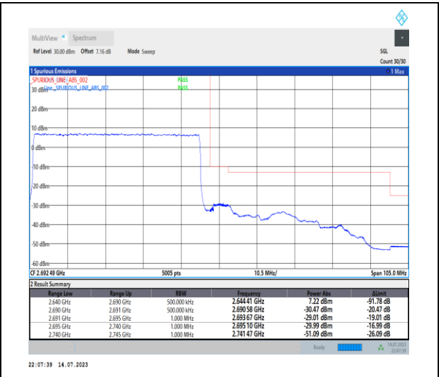
1-N41-PC1-30-50-H-3-DFT-PI2BPSK-Outer_Full-1 28@0-Ant0-1--PASS-see graph
