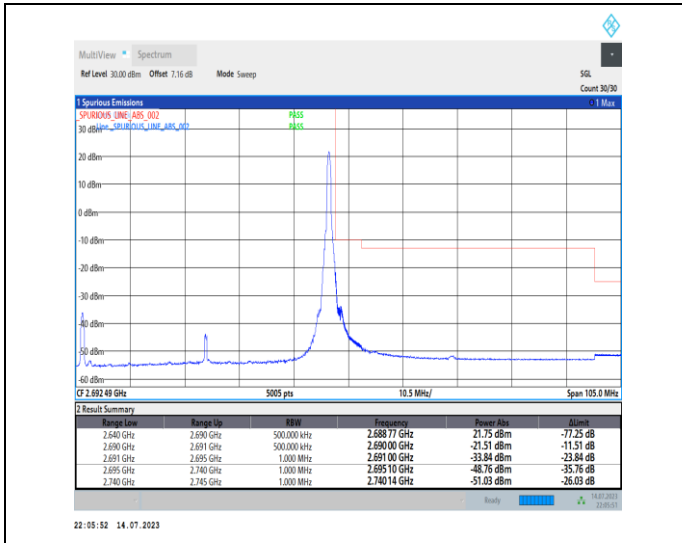
1-N41-PC1-30-50-H-2-DFT-PI2BPSK-Edge_1RB_Right t-1@132-Ant0-1--PASS-see graph
