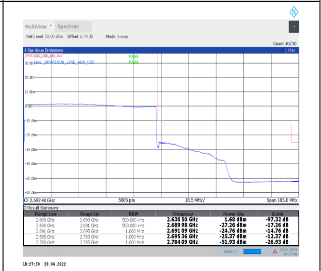
1-N41--30-90-H-6-CP-QPSK-Outer_Full-245@0-A nt0-PASS-see graph
