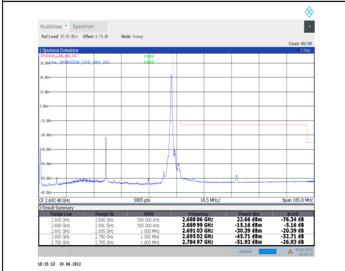
1-N41--30-90-H-5-CP-QPSK-Edge_1RB_Right-1@244 -Ant0-PASS-see graph
