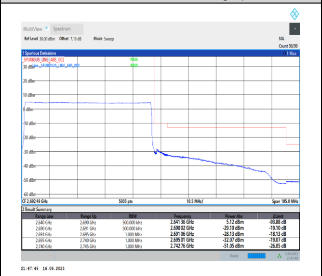
1-N41-PC1-30-50-H-6-CP-QPSK-Outer_Full-133 @0-Ant0-1--PASS-see graph
