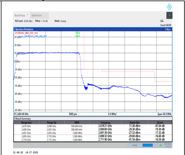
1-N41-PC1-30-20-H-3-DFT-PI2BPSK-Outer_Full-5 0@0-Ant0-1--PASS-see graph
