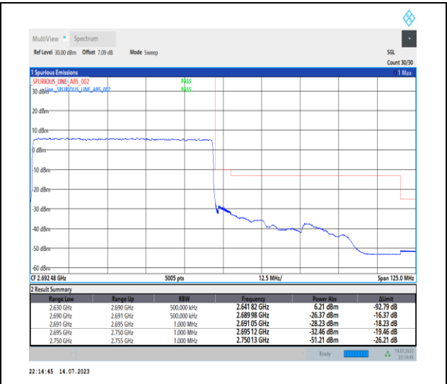
1-N41-PC1-30-60-H-3-DFT-PI2BPSK-Outer_Full-1 62 @ 0-Ant0-1--PASS-see graph
