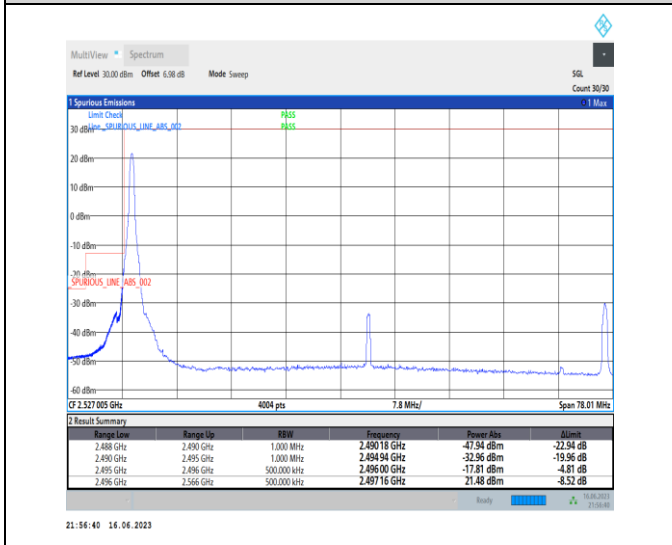
1-N41-PC1-30-70-L-4-CP-QPSK-Edge_1RB_Left-1@ 0-Ant0-1--PASS-see graph
