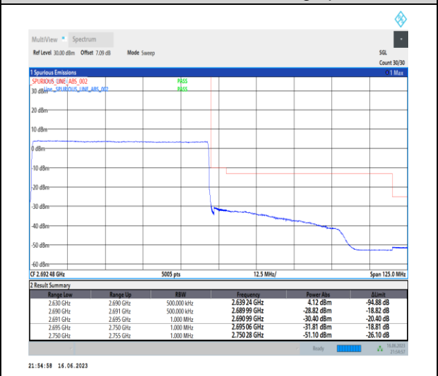
1-N41-PC1-30-60-H-6-CP-QPSK-Outer_Full-162 @ 0-Ant0-1--PASS-see graph
