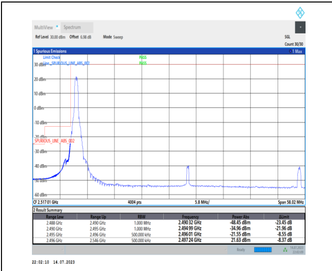
1-N41-PC1-30-50-L-1-DFT-PI2BPSK-Edge_1RB_Left -1@0-Ant0-1--PASS-see graph
