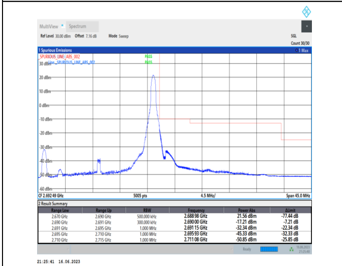
1-N41-PC1-30-20-H-5-CP-QPSK-Edge_1RB_Right-1 @50-Ant0-1--PASS-see graph
