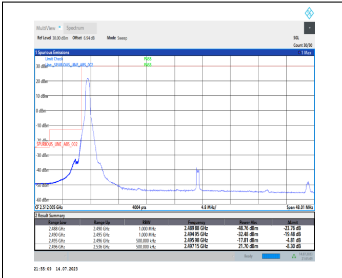
1-N41-PC1-30-40-L-1-DFT-PI2BPSK-Edge_1RB_Left -1@0-Ant0-1--PASS-see graph
