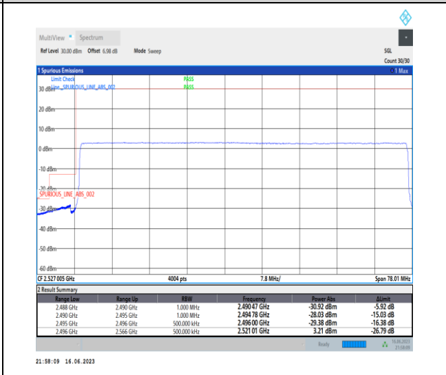
1-N41-PC1-30-70-L-6-CP-QPSK-Outer_Full-189@0 -Ant0-1--PASS-see graph
