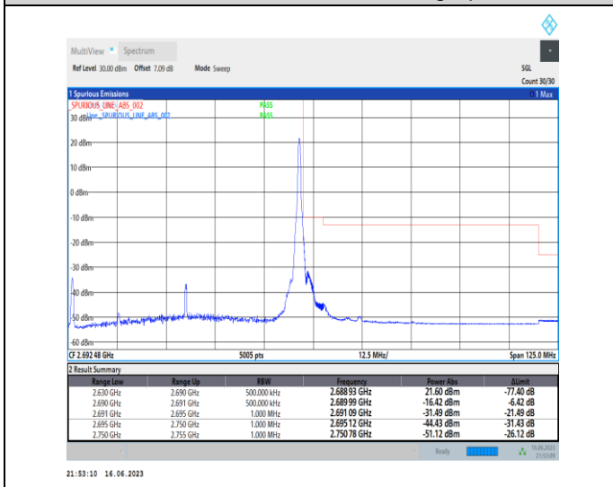
1-N41-PC1-30-60-H-5-CP-QPSK-Edge_1RB_Right-1 @ 161-Ant0-1--PASS-see graph
