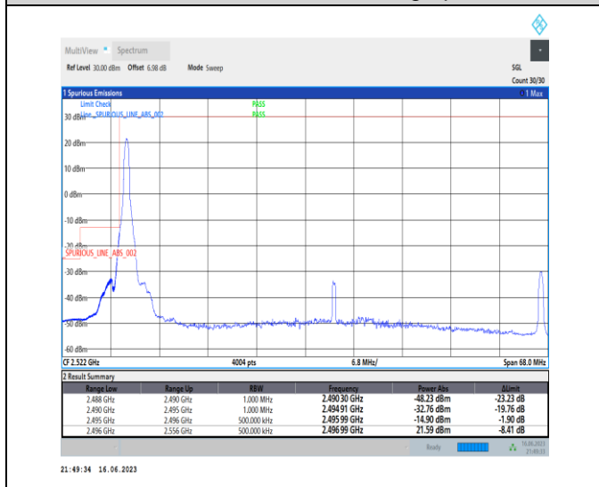
1-N41-PC1-30-60-L-4-CP-QPSK-Edge_1RB_Left-1@ 0-Ant0-1--PASS-see graph
