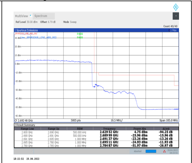
1-N41--30-90-H-3-DFT-PI2BPSK-Outer_Full-240 @0-Ant0-PASS-see graph
