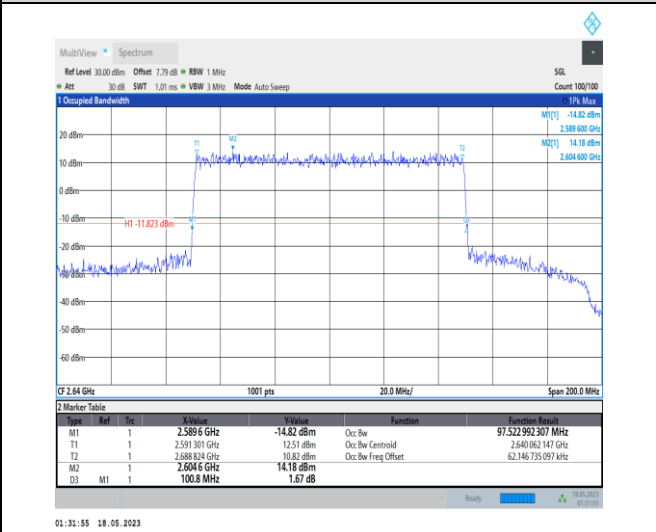
1-N41-PC1-30-100-H-6-CP-QPSK-Outer_Full-273 @0-Ant0-97.523-100.800-≤100-PASS
