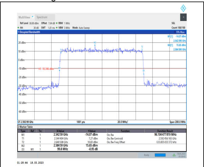
1-N41-PC1-30-100-M-1-DFT-QPSK-Outer_Full-270 @ 0-Ant0-96.104-99.800-≤100-PASS
