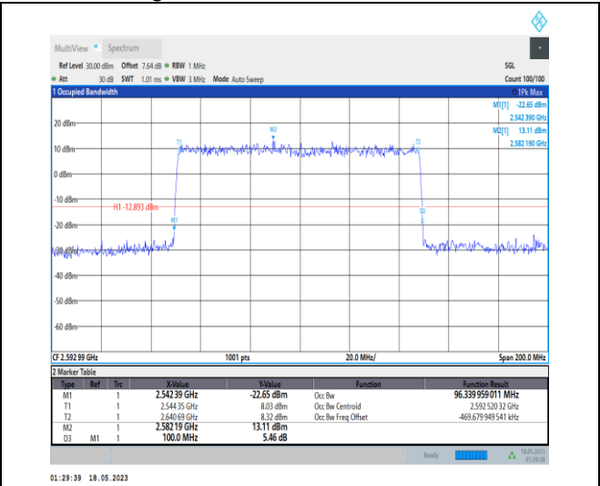
1-N41-PC1-30-100-M-5-DFT-256QAM-Outer_Full-270 @0-Ant0-96.34-100.000-≤100-PASS
