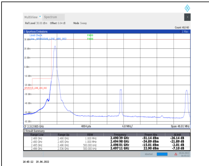
1-N41--30-40-L-1-DFT-PI2BPSK-Edge_1RB_Left-1@0-Ant0-PASS-see graph
