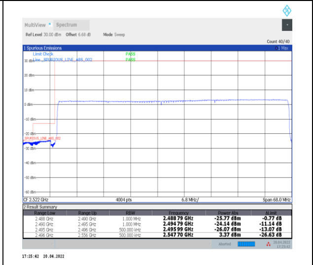
1-N41--30-60-L-6-CP-QPSK-Outer_Full-162@0-Ant0-PASS-see graph
