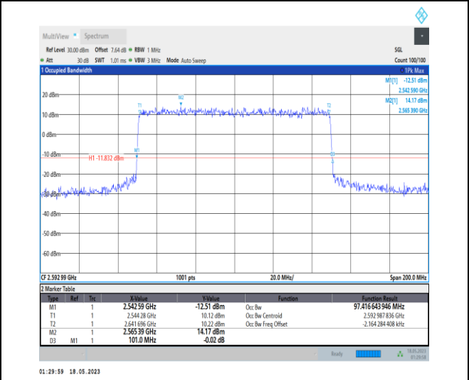
1-N41-PC1-30-100-M-7-CP-16QAM-Outer_Full-273 @0-Ant0-97.417-101.000-≤100-PASS
