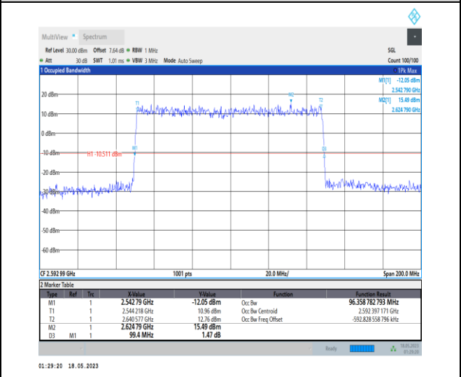
1-N41-PC1-30-100-M-3-DFT-16QAM-Outer_Full-270 @ 0-Ant0-96.359-99.400-≤100-PASS
