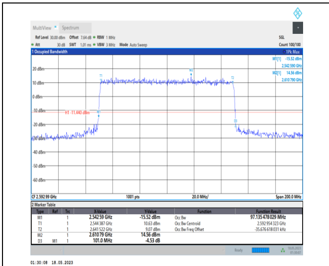
1-N41-PC1-30-100-M-8-CP-64QAM-Outer_Full-273 @0-Ant0-97.135-101.000-≤100-PASS
