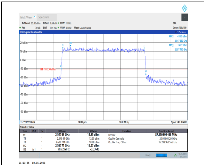
1-N41-PC1-30-90-M-7-CP-16QAM-Outer_Full-245@ 0-Ant0-87.391-90.720-≤90-PASS
