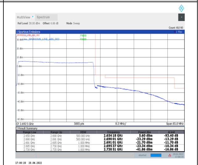
1-N41--30-40-H-6-CP-QPSK-Outer_Full-106@0-Ant0-PASS-see graph
