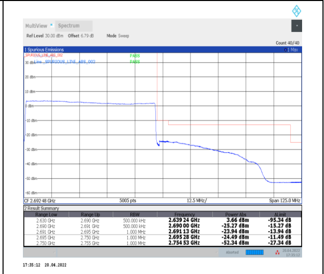
1-N41--30-60-H-6-CP-QPSK-Outer_Full-162@0-Ant0-PASS-see graph
