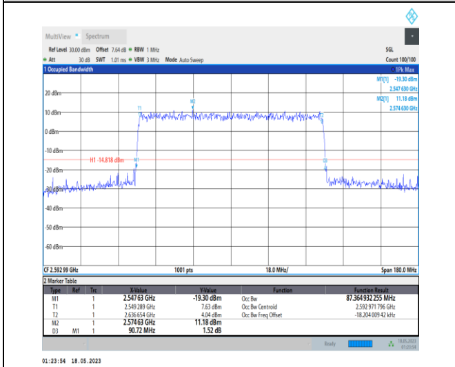
1-N41-PC1-30-90-M-9-CP-256QAM-Outer_Full-245 @0-Ant0-87.365-90.720-≤90-PASS
