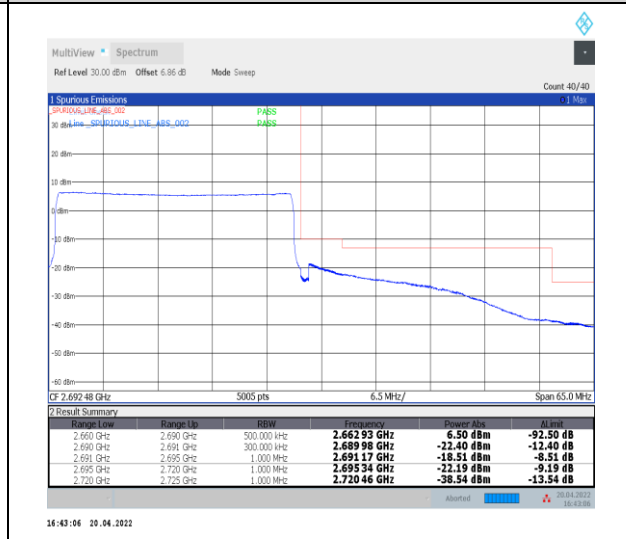
1-N41--30-30-H-6-CP-QPSK-Outer_Full-78@0-Ant0-PASS-see graph
