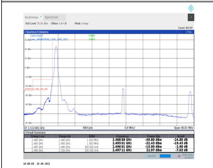
1-N41--30-40-L-4-CP-QPSK-Edge_1RB_Left-1@0-Ant0-PASS-see graph
