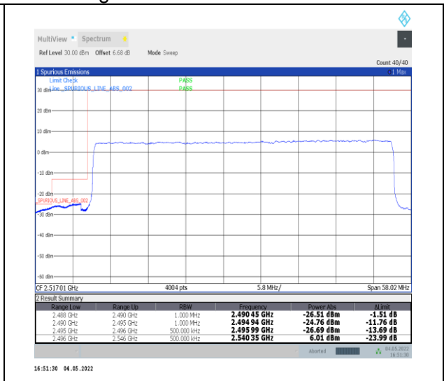
1-N41--30-50-L-3-DFT-PI2BPSK-Outer_Full-128@0-Ant0-PASS-see graph
