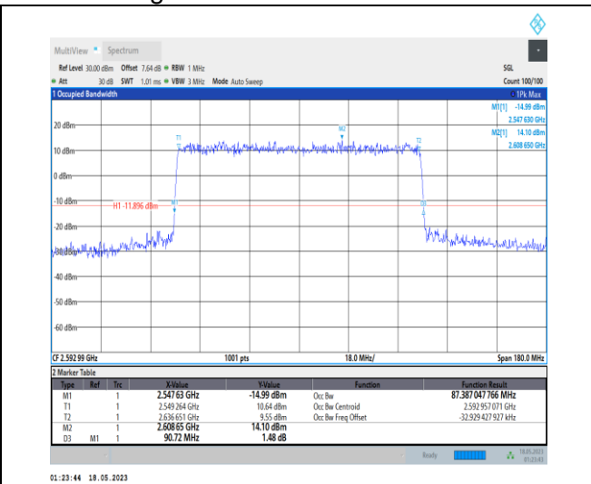
1-N41-PC1-30-90-M-8-CP-64QAM-Outer_Full-245@ 0-Ant0-87.387-90.720-≤90-PASS
