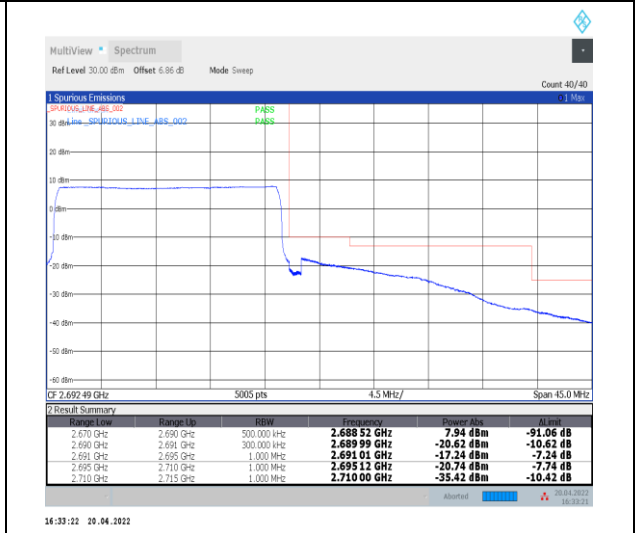
1-N41--30-20-H-6-CP-QPSK-Outer_Full-51@0-Ant0-PASS-see graph
