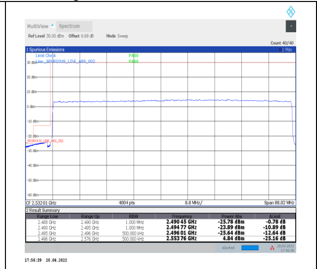
1-N41--30-80-L-3-DFT-PI2BPSK-Outer_Full-216@0-Ant0-PASS-see graph
