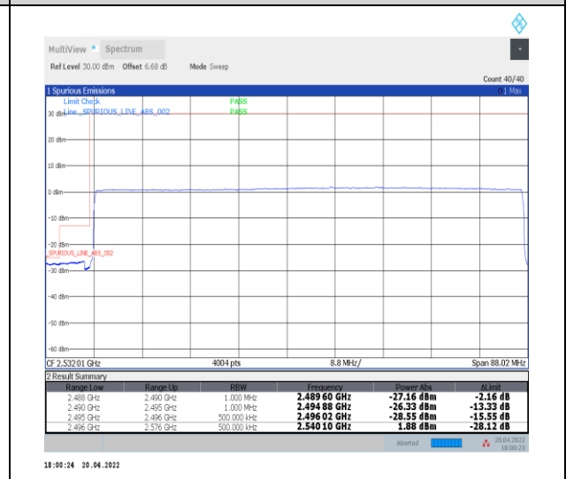
1-N41--30-80-L-6-CP-QPSK-Outer_Full-217@0-Ant0-PASS-see graph
