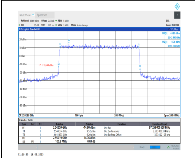
1-N41-PC1-30-100-M-6-CP-QPSK-Outer_Full-273 @0-Ant0-97.259-100.800-≤100-PASS
