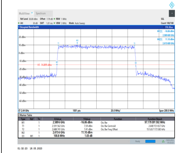
1-N41-PC1-30-100-H-9-CP-256QAM-Outer_Full-273 @0-Ant0-97.179-100.800-≤100-PASS
