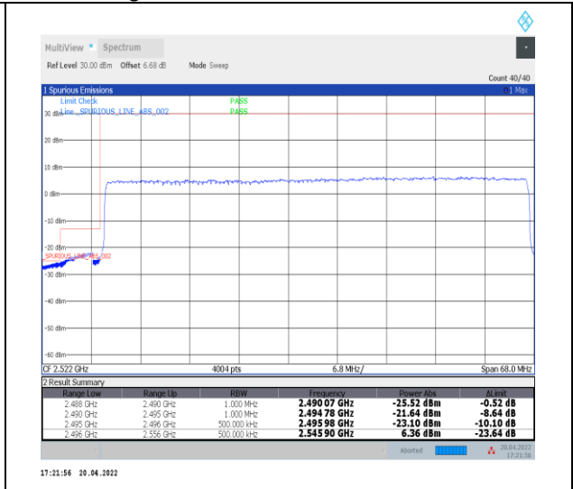
1-N41--30-60-L-3-DFT-PI2BPSK-Outer_Full-162@0-Ant0-PASS-see graph
