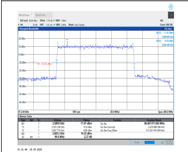
1-N41-PC1-30-100-H-5-DFT-256QAM-Outer_Full-27 @0-Ant0-96.461-99.400-≤100-PASS
