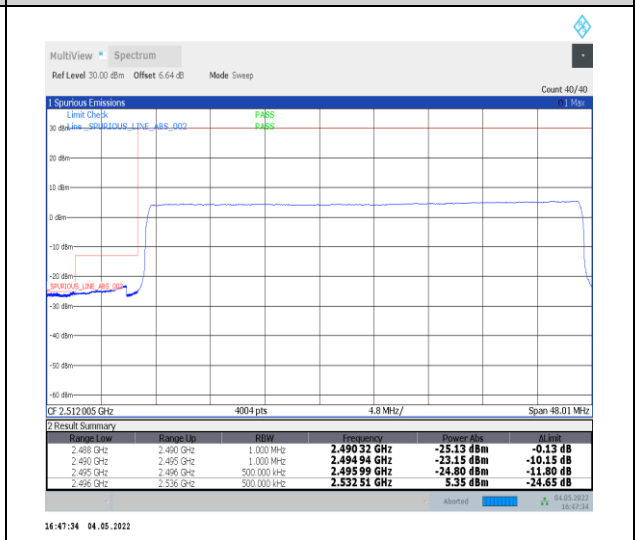
1-N41--30-40-L-6-CP-QPSK-Outer_Full-106@0-Ant0-PASS-see graph
