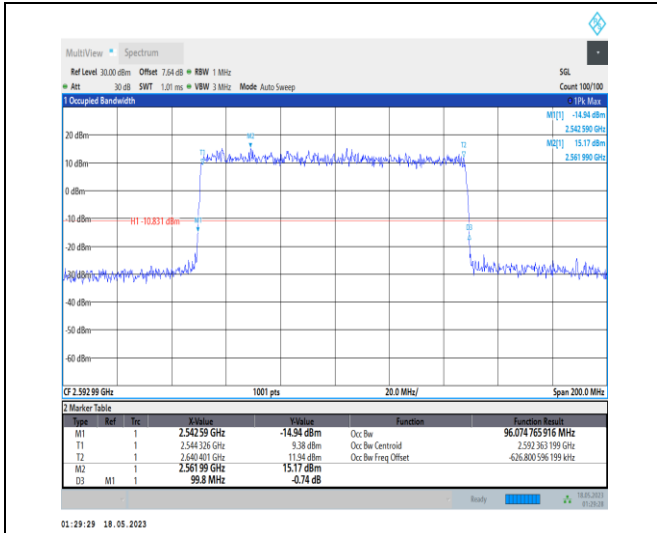
1-N41-PC1-30-100-M-4-DFT-64QAM-Outer_Full-270 @0-Ant0-96.075-99.800-≤100-PASS
