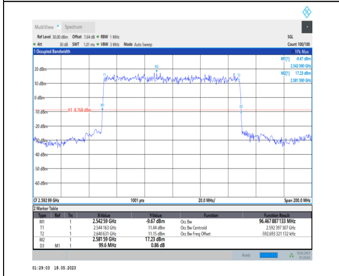
1-N41-PC1-30-100-M-2-DFT-PI2BPSK-Outer_Full-270 @ 0-Ant0-96.468-99.600-≤100-PASS
