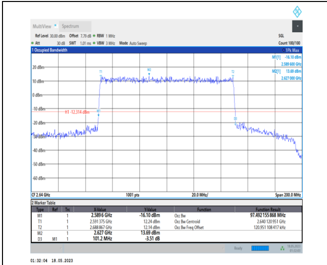
1-N41-PC1-30-100-H-7-CP-16QAM-Outer_Full-273 @0-Ant0-97.492-101.200-≤100-PASS
