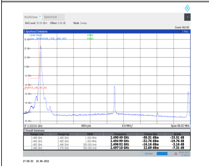
1-N41--30-80-L-4-CP-QPSK-Edge_1RB_Left-1@0-Ant0-PASS-see graph
