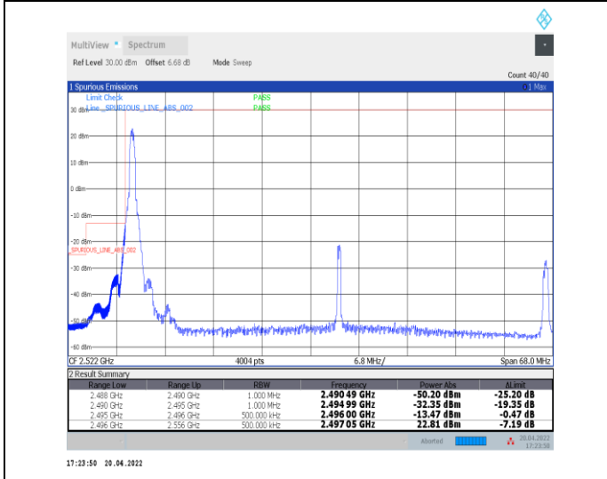
1-N41--30-60-L-4-CP-QPSK-Edge_1RB_Left-1@0-Ant0-PASS-see graph
