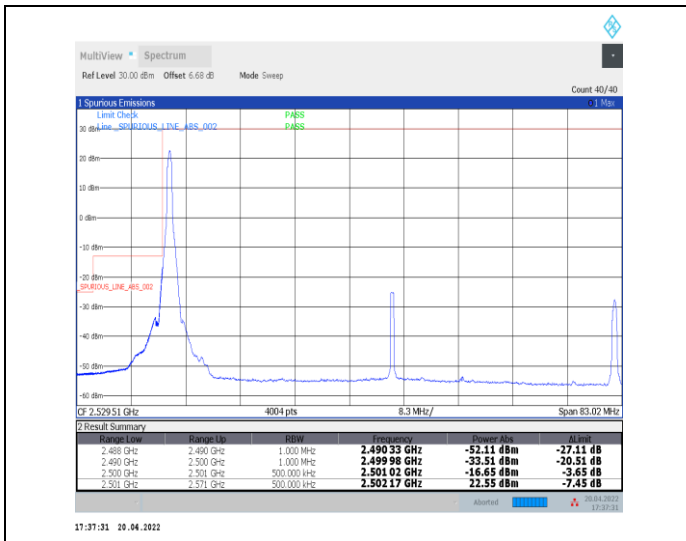
1-N41--30-70-L-1-DFT-PI2BPSK-Edge_1RB_Left-1@0-Ant0-PASS-see graph
