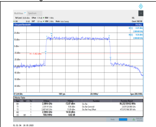
1-N41-PC1-30-100-H-4-DFT-64QAM-Outer_Full-270 @0-Ant0-96.233-100.000-≤100-PASS
