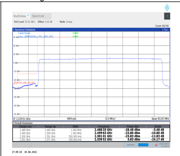
1-N41--30-70-L-3-DFT-PI2BPSK-Outer_Full-180@0-Ant0-PASS-see graph
