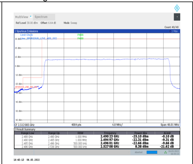
1-N41--30-40-L-3-DFT-PI2BPSK-Outer_Full-100@0-Ant0-PASS-see graph
