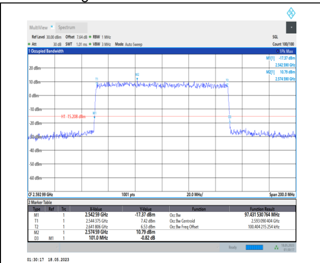
1-N41-PC1-30-100-M-9-CP-256QAM-Outer_Full-273 @0-Ant0-97.432-101.000-≤100-PASS
