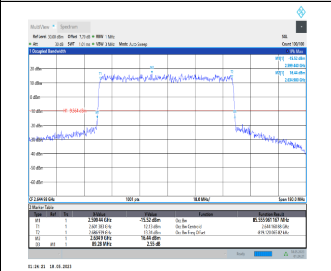
1-N41-PC1-30-90-H-1-DFT-QPSK-Outer_Full-240@ 0-Ant0-85.556-89.280-≤90-PASS
