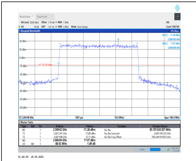
1-N41-PC1-30-90-H-2-DFT-PI2BPSK-Outer_Full-240 @ 0-Ant0-85.708-88.920-≤90-PASS
