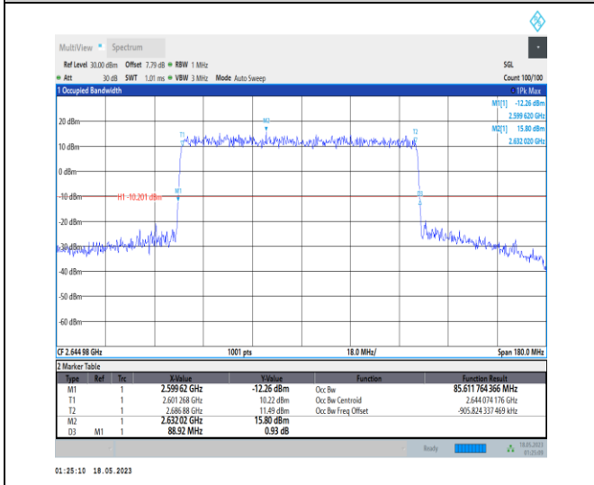
1-N41-PC1-30-90-H-4-DFT-64QAM-Outer_Full-240 @ 0-Ant0-85.612-88.920-≤90-PASS
