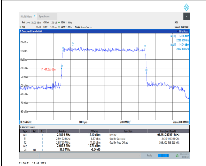
1-N41-PC1-30-100-H-1-DFT-QPSK-Outer_Full-270 @0-Ant0-96.233-99.800-≤100-PASS
