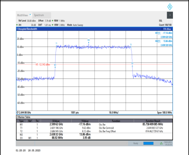
1-N41-PC1-30-90-H-5-DFT-256QAM-Outer_Full-240 @ 0-Ant0-85.758-88.920-≤90-PASS
