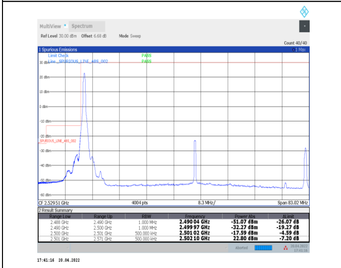
1-N41--30-70-L-4-CP-QPSK-Edge_1RB_Left-1@0-Ant0-PASS-see graph
