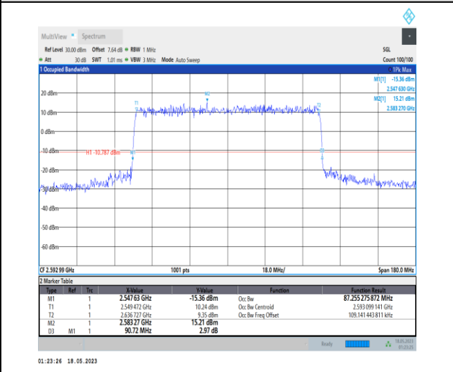
1-N41-PC1-30-90-M-6-CP-QPSK-Outer_Full-245 @ 0-Ant0-87.255-90.720-≤90-PASS
