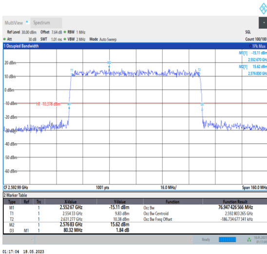
1-N41-PC1-30-80-M-4-DFT-64QAM-Outer_Full-216 @0-Ant0-76.947-80.320-≤80-PASS
