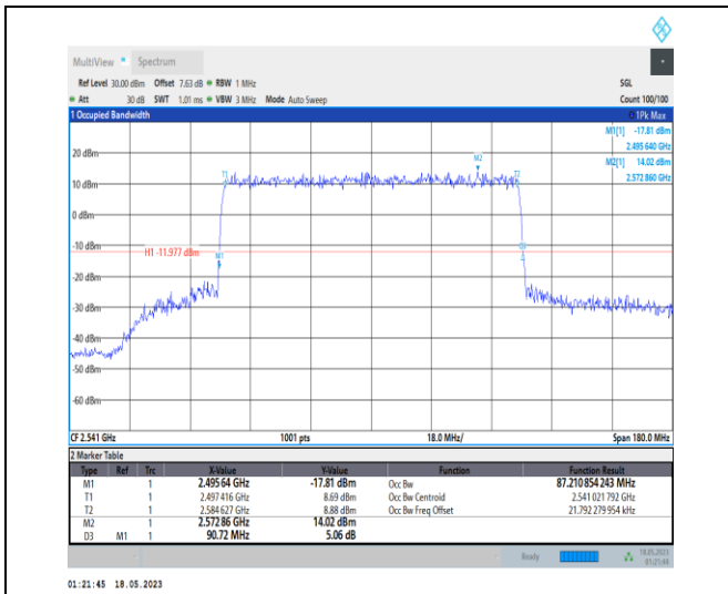
1-N41-PC1-30-90-L-8-CP-64QAM-Outer_Full-245@ 0-Ant0-87.211-90.720-≤90-PASS
