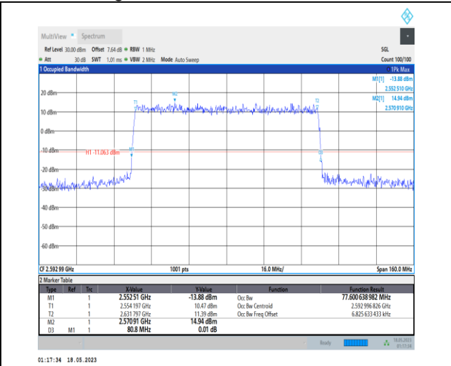
1-N41-PC1-30-80-M-7-CP-16QAM-Outer_Full-217@0 0-Ant0-77.601-80.800-≤80-PASS
