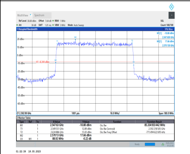
1-N41-PC1-30-90-M-2-DFT-PI2BPSK-Outer_Full-24 0@0-Ant0-85.335-88.920-≤90-PASS
