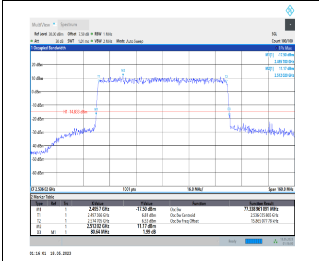
1-N41-PC1-30-80-L-9-CP-256QAM-Outer_Full-217 @0-Ant0-77.339-80.640-≤80-PASS
