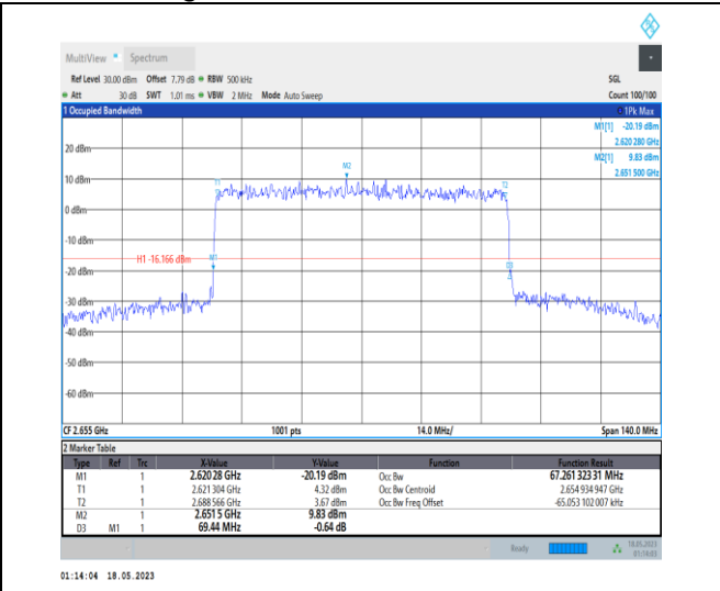
1-N41-PC1-30-70-H-9-CP-256QAM-Outer_Full-189@0-Ant0-67.261-69.440-<=70-PASS
