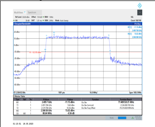
1-N41-PC1-30-80-L-8-CP-64QAM-Outer_Full-217@ 0-Ant0-77.41-80.640-≤80-PASS
