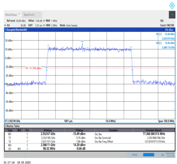
1-N41-PC1-30-80-M-5-DFT-256QAM-Outer_Full-216 @0-Ant0-77.367-80.320-≤80-PASS
