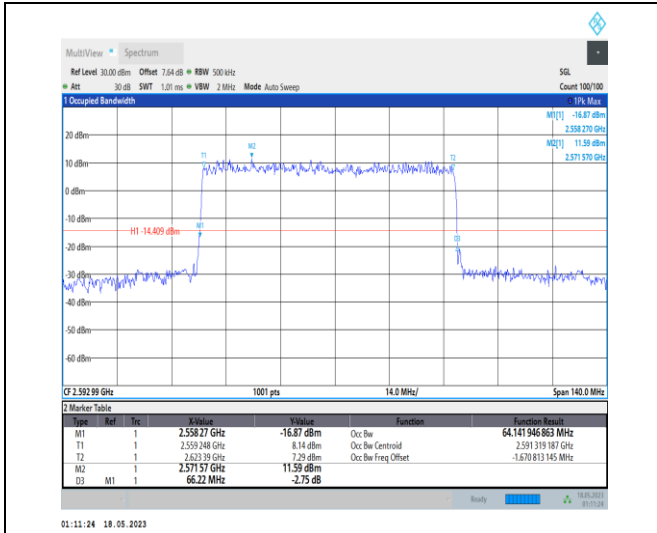
1-N41-PC1-30-70-M-5-DFT-256QAM-Outer_Full-180 @ 0-Ant0-64.142-66.220-<=70-PASS
