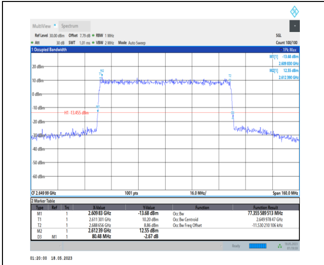
1-N41-PC1-30-80-H-9-CP-256QAM-Outer_Full-217 @ 0-Ant0-77.356-80.480-≤80-PASS
