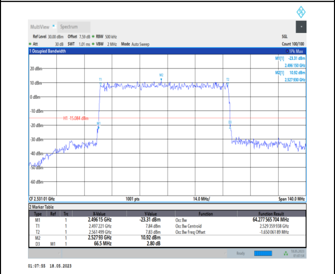
1-N41-PC1-30-70-L-5-DFT-256QAM-Outer_Full-180 @ 0-Ant0-64.278-66.500-≤70-PASS
