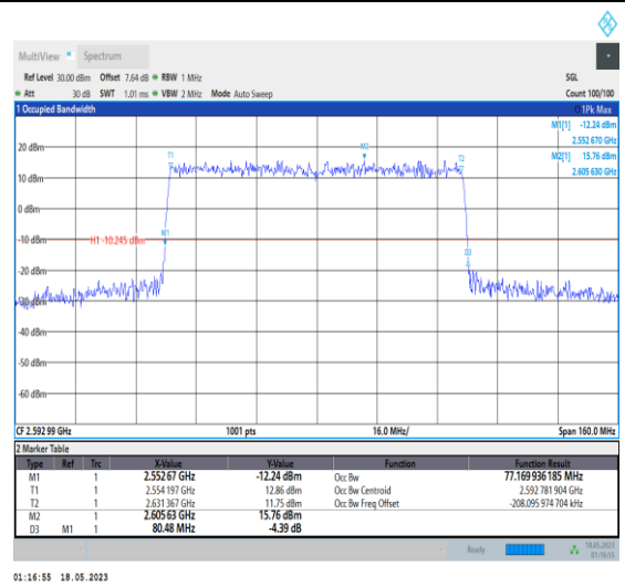
1-N41-PC1-30-80-M-3-DFT-16QAM-Outer_Full-216 @0-Ant0-77.17-80.480-≤80-PASS
