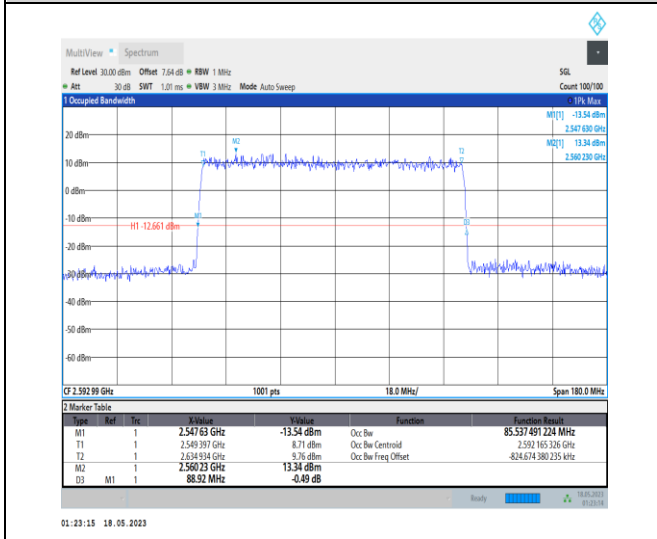
1-N41-PC1-30-90-M-5-DFT-256QAM-Outer_Full-240 @ 0-Ant0-85.537-88.920-≤90-PASS
