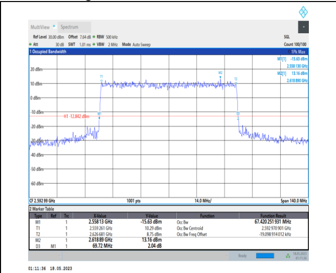
1-N41-PC1-30-70-M-6-CP-QPSK-Outer_Full-189 @ 0-Ant0-67.42-69.720-<=70-PASS
