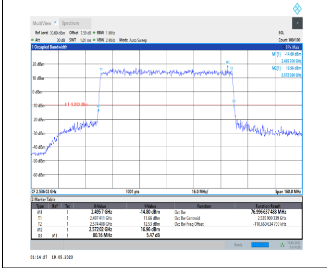
1-N41-PC1-30-80-L-1-DFT-QPSK-Outer_Full-216@0-Ant0-76.997-80.160-<=80-PASS
