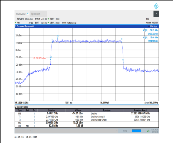
1-N41-PC1-30-80-L-6-CP-QPSK-Outer_Full-217 @ 0-Ant0-77.294-80.800-≤80-PASS
