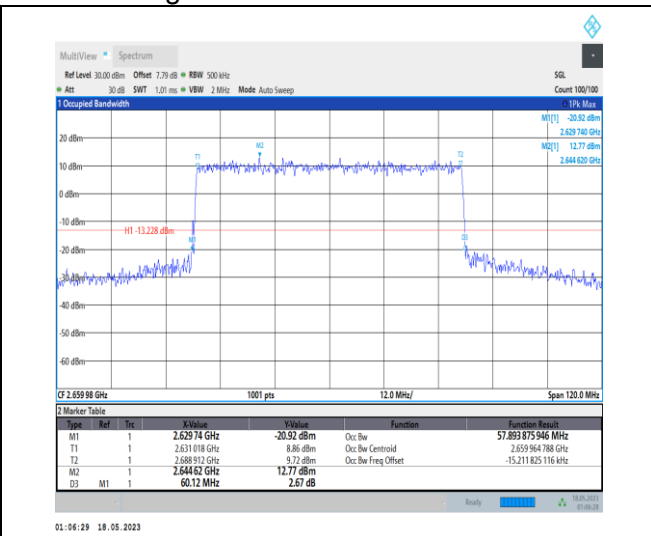
1-N41-PC1-30-60-H-8-CP-64QAM-Outer_Full-162@ 0-Ant0-57.894-60.120-≤60-PASS
