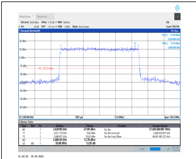
1-N41-PC1-30-60-H-7-CP-16QAM-Outer_Full-162@ 0-Ant0-57.696-59.880-≤60-PASS
