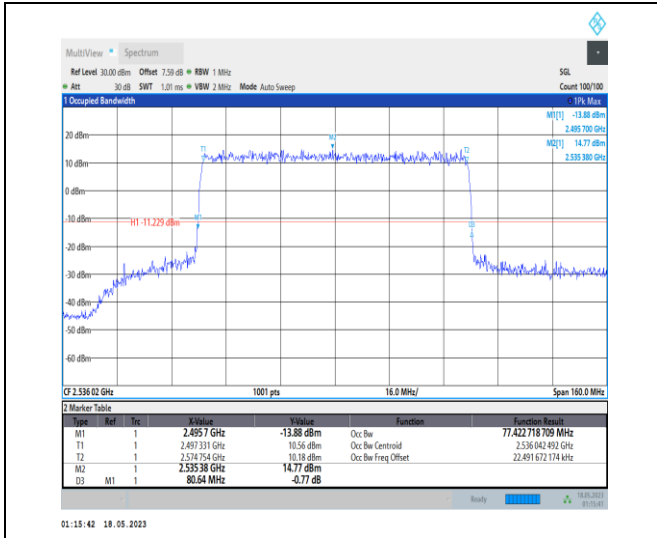
1-N41-PC1-30-80-L-7-CP-16QAM-Outer_Full-217@ 0-Ant0-77.423-80.640-≤80-PASS
