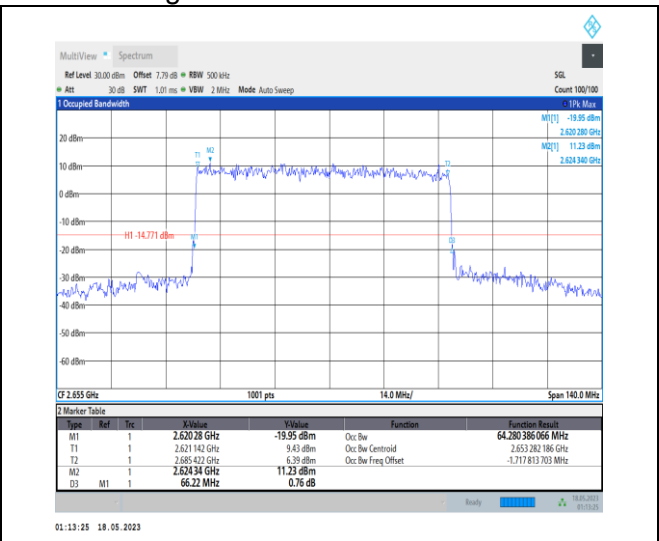
1-N41-PC1-30-70-H-5-DFT-256QAM-Outer_Full-180 @ 0-Ant0-64.28-66.220-≤70-PASS
