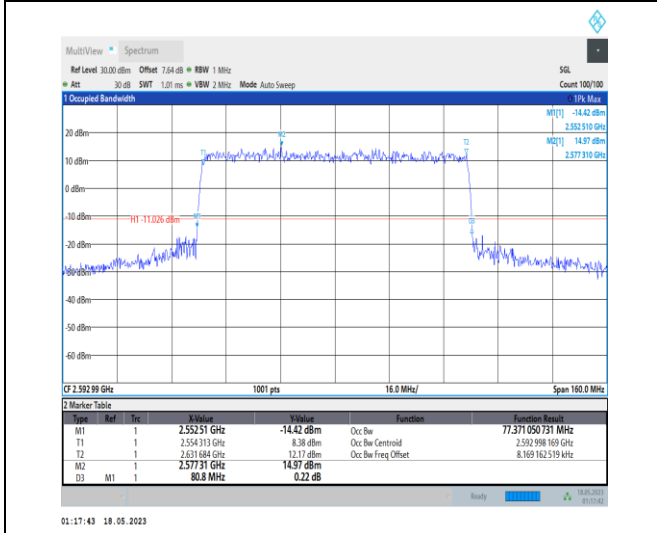
1-N41-PC1-30-80-M-8-CP-64QAM-Outer_Full-217@0 0-Ant0-77.371-80.800-≤80-PASS
