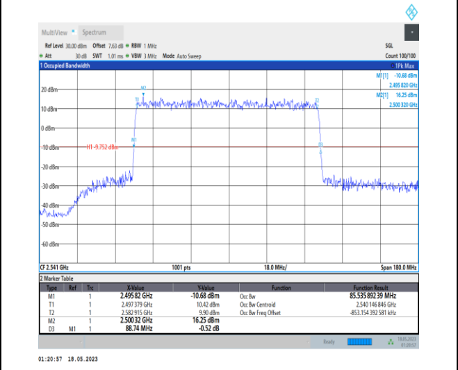
1-N41-PC1-30-90-L-3-DFT-16QAM-Outer_Full-240 @ 0-Ant0-85.536-88.740-≤90-PASS
