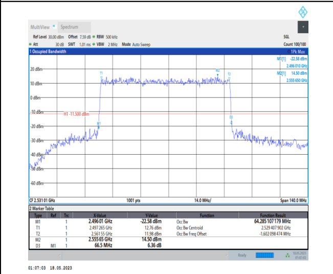
1-N41-PC1-30-70-L-1-DFT-QPSK-Outer_Full-180@ 0-Ant0-64.285-66.500-≤70-PASS
