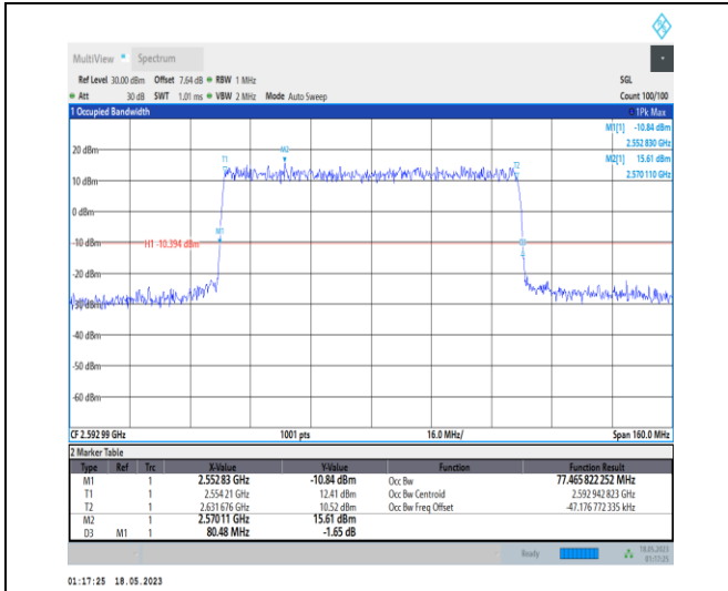
1-N41-PC1-30-80-M-6-CP-QPSK-Outer_Full-217@0 -Ant0-77.466-80.480-≤80-PASS
