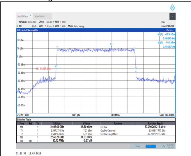
1-N41-PC1-30-90-L-9-CP-256QAM-Outer_Full-245 @0-Ant0-87.29-90.720-≤90-PASS
