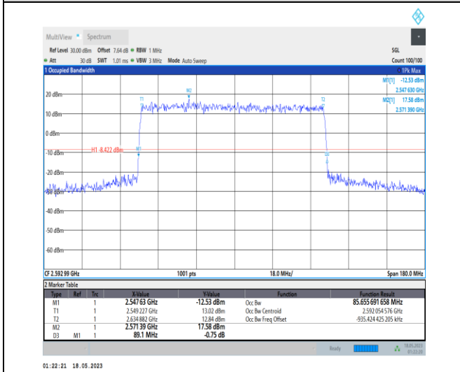
1-N41-PC1-30-90-M-1-DFT-QPSK-Outer_Full-240@ 0-Ant0-85.656-89.100-≤90-PASS
