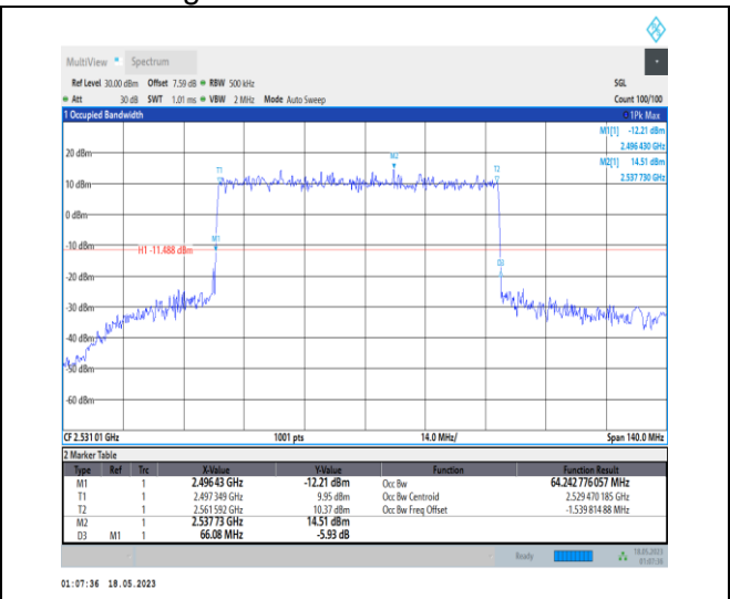
1-N41-PC1-30-70-L-3-DFT-16QAM-Outer_Full-180 @ 0-Ant0-64.243-66.080-≤70-PASS
