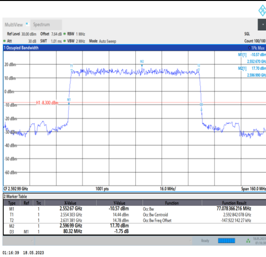
1-N41-PC1-30-80-M-2-DFT-PI2BPSK-Outer_Full-21 @0-Ant0-77.078-80.320-≤80-PASS
