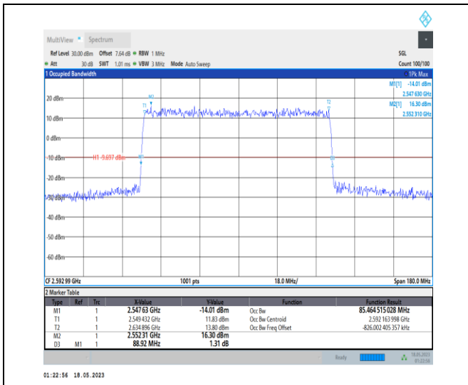
1-N41-PC1-30-90-M-3-DFT-16QAM-Outer_Full-240 @ 0-Ant0-85.465-88.920-≤90-PASS
