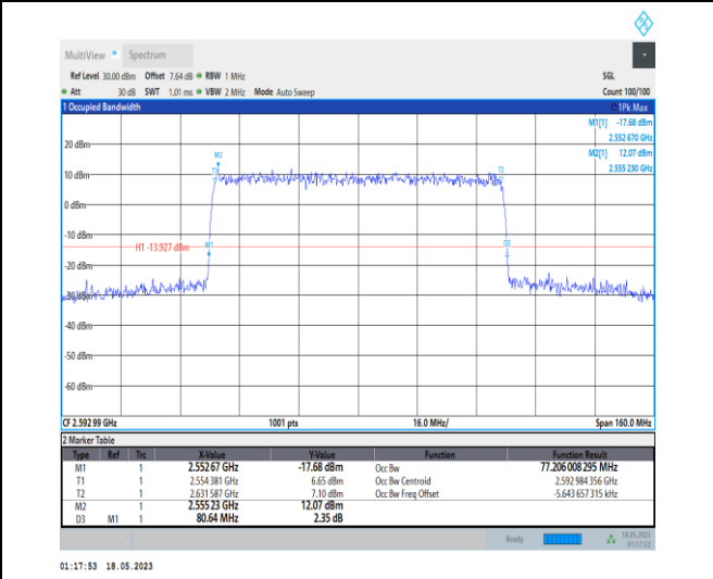
1-N41-PC1-30-80-M-9-CP-256QAM-Outer_Full-217@0 @0-Ant0-77.206-80.640-≤80-PASS
