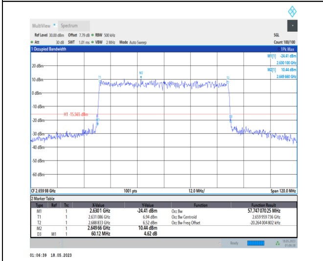
1-N41-PC1-30-60-H-9-CP-256QAM-Outer_Full-162 @0-Ant0-57.747-60.120-≤60-PASS
