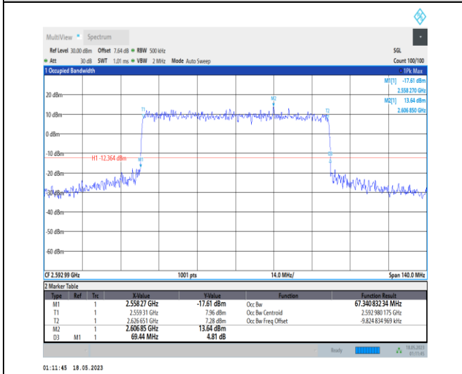
1-N41-PC1-30-70-M-7-CP-16QAM-Outer_Full-189 @ 0-Ant0-67.341-69.440-<=70-PASS
