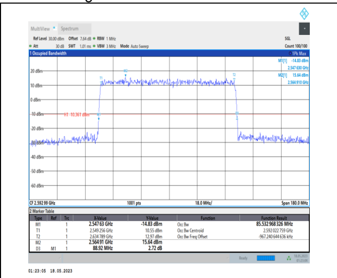
1-N41-PC1-30-90-M-4-DFT-64QAM-Outer_Full-240 @ 0-Ant0-85.533-88.920-≤90-PASS
