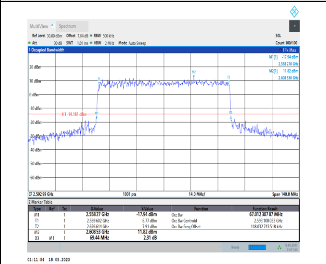
1-N41-PC1-30-70-M-8-CP-64QAM-Outer_Full-189 @ 0-Ant0-67.012-69.440-<=70-PASS
