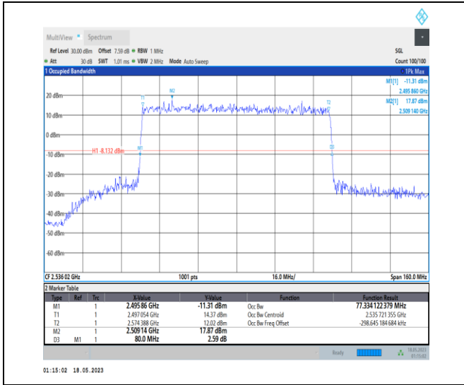
1-N41-PC1-30-80-L-3-DFT-16QAM-Outer_Full-216 @ 0-Ant0-77.334-80.000-≤80-PASS
