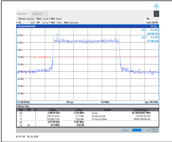
1-N41-PC1-30-50-M-3-DFT-16QAM-Outer_Full-128 @ 0-Ant0-45.741-47.400-≤50-PASS
