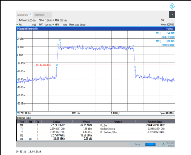
1-N41-PC1-30-40-M-9-CP-256QAM-Outer_Full-106@0 -Ant0-37.865-39.440-≤40-PASS
