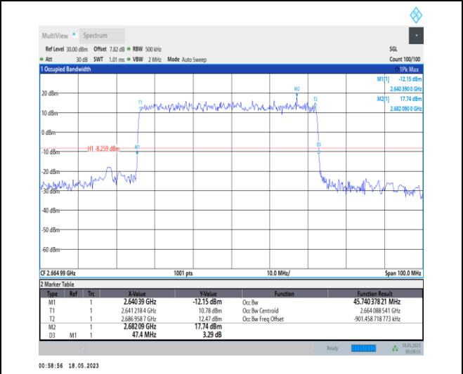
1-N41-PC1-30-50-H-1-DFT-QPSK-Outer_Full-128@ 0-Ant0-45.74-47.400-≤50-PASS
