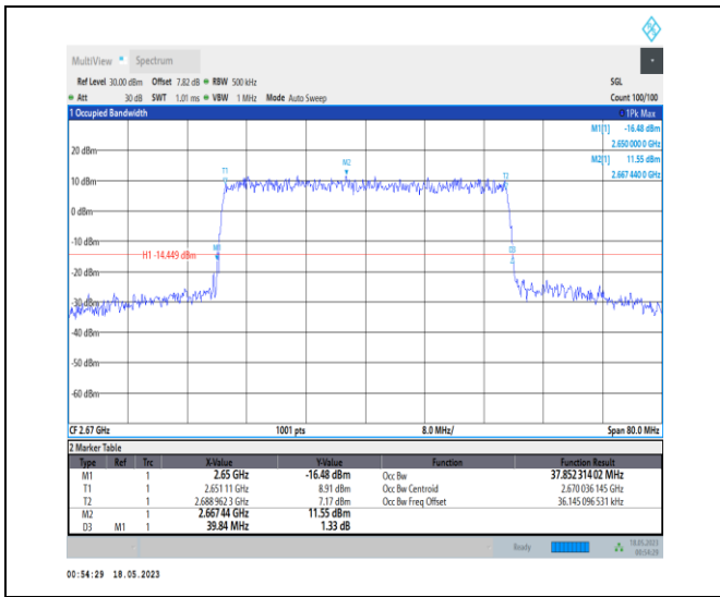
1-N41-PC1-30-40-H-9-CP-256QAM-Outer_Full-106 @ 0-Ant0-37.852-39.840-≤40-PASS
