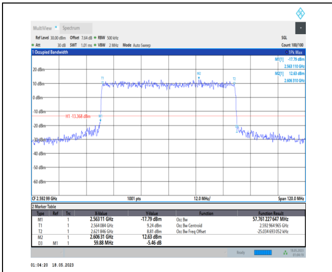
1-N41-PC1-30-60-M-8-CP-64QAM-Outer_Full-162@ 0-Ant0-57.761-59.880-≤60-PASS
