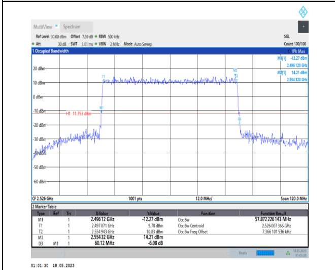
1-N41-PC1-30-60-L-3-DFT-16QAM-Outer_Full-162 @0-Ant0-57.872-60.120-≤60-PASS
