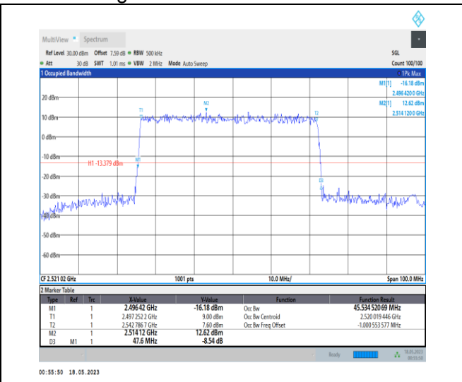
1-N41-PC1-30-50-L-5-DFT-256QAM-Outer_Full-128 @ 0-Ant0-45.535-47.600-≤50-PASS
