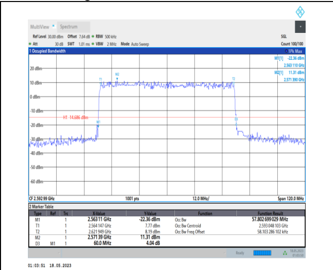
1-N41-PC1-30-60-M-5-DFT-256QAM-Outer_Full-162 @ 0-Ant0-57.803-60.000-≤60-PASS
