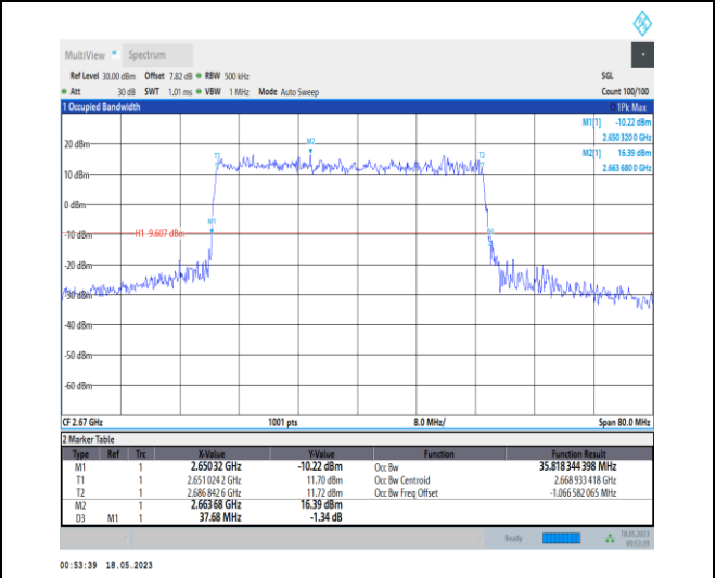
1-N41-PC1-30-40-H-4-DFT-64QAM-Outer_Full-100@0-Ant0-35.818-37.680-≤40-PASS
