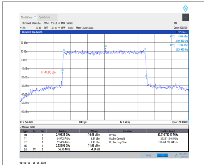
1-N41-PC1-30-60-L-5-DFT-256QAM-Outer_Full-162 @ 0-Ant0-57.711-59.760-≤60-PASS
