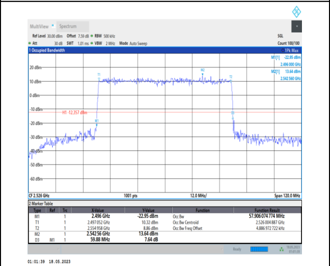
1-N41-PC1-30-60-L-4-DFT-64QAM-Outer_Full-162 @0-Ant0-57.906-59.880-≤60-PASS
