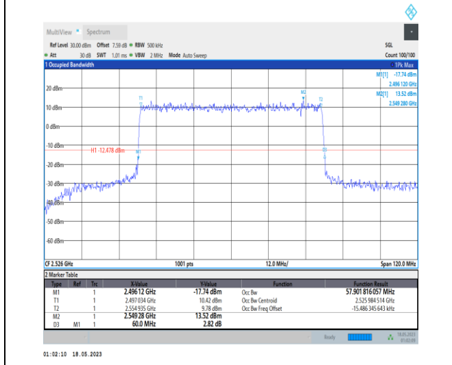
1-N41-PC1-30-60-L-7-CP-16QAM-Outer_Full-162 @ 0-Ant0-57.902-60.000-≤60-PASS
