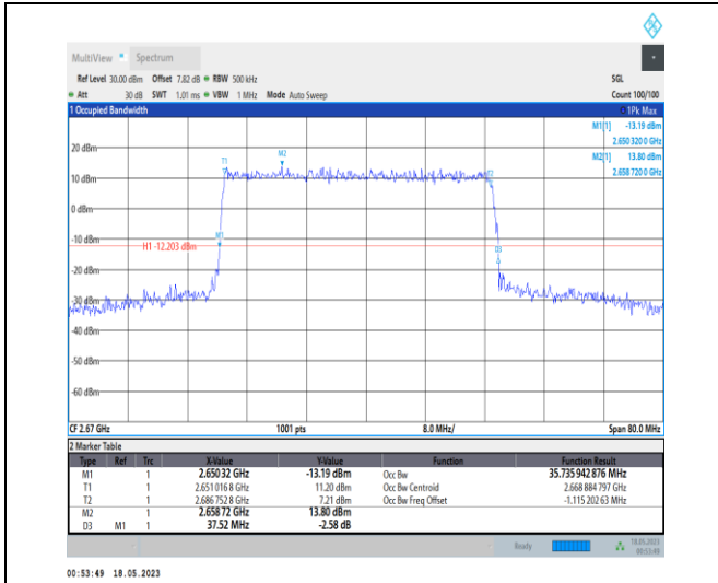
1-N41-PC1-30-40-H-5-DFT-256QAM-Outer_Full-100 @ 0-Ant0-35.736-37.520-≤40-PASS
