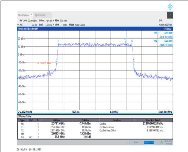
1-N41-PC1-30-40-M-6-CP-QPSK-Outer_Full-106@0 -Ant0-37.886-39.600-≤40-PASS
