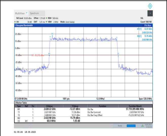
1-N41-PC1-30-60-H-2-DFT-PI2BPSK-Outer_Full-16 2@0-Ant0-57.755-60.000-≤60-PASS
