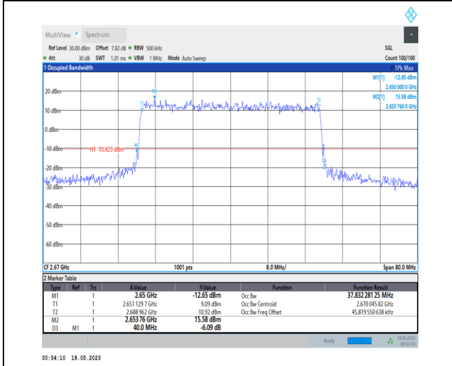
1-N41-PC1-30-40-H-7-CP-16QAM-Outer_Full-106 @ 0-Ant0-37.832-40.000-≤40-PASS
