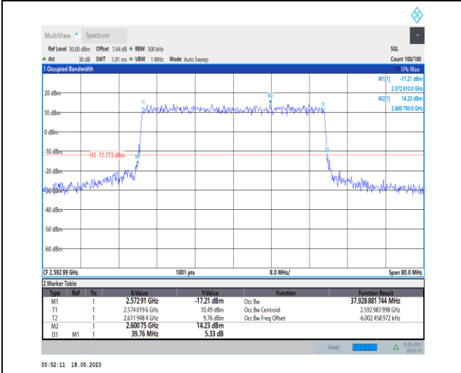
1-N41-PC1-30-40-M-8-CP-64QAM-Outer_Full-106@0 -Ant0-37.929-39.760-≤40-PASS
