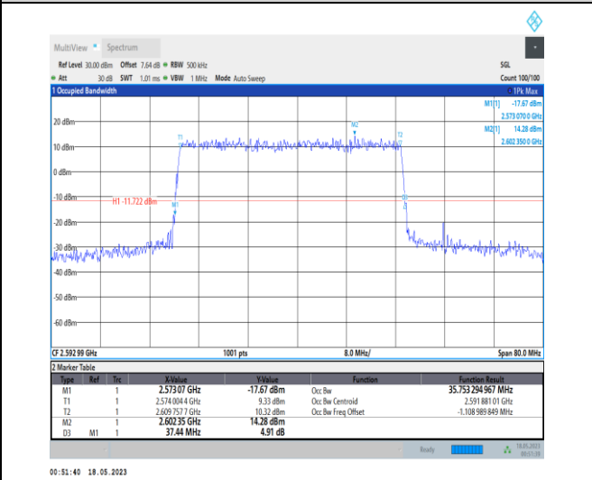
1-N41-PC1-30-40-M-5-DFT-256QAM-Outer_Full-100@0-Ant0-35.753-37.440-≤40-PASS
