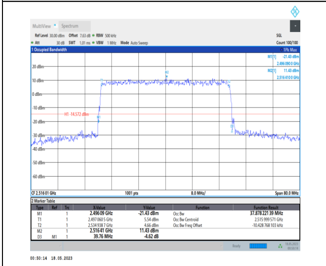
1-N41-PC1-30-40-L-9-CP-256QAM-Outer_Full-106 @0-Ant0-37.878-39.760-≤40-PASS
