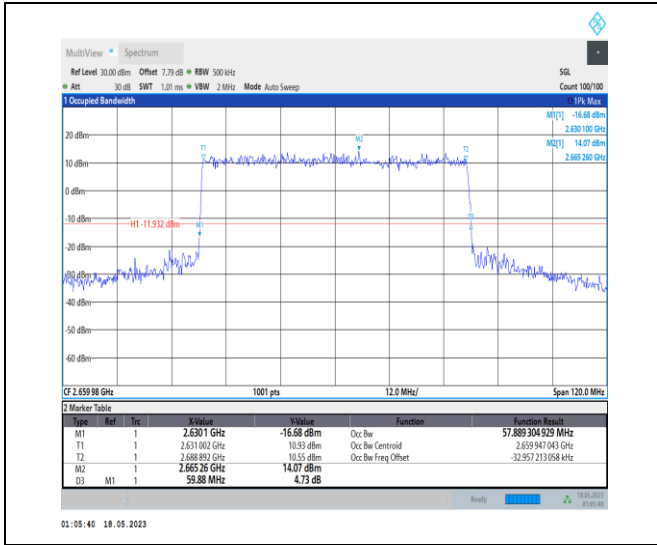
1-N41-PC1-30-60-H-3-DFT-16QAM-Outer_Full-162 @ 0-Ant0-57.889-59.880-≤60-PASS
