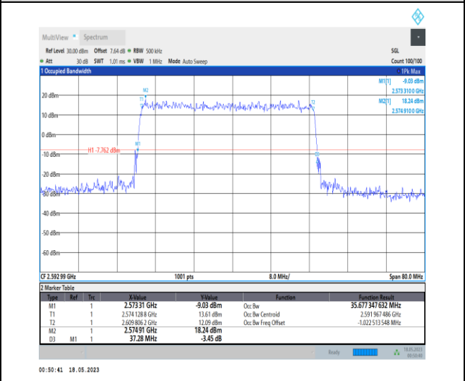
1-N41-PC1-30-40-M-1-DFT-QPSK-Outer_Full-100@ 0-Ant0-35.677-37.280-≤40-PASS
