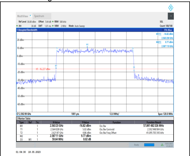
1-N41-PC1-30-60-M-9-CP-256QAM-Outer_Full-162 @0-Ant0-57.841-59.640-≤60-PASS
