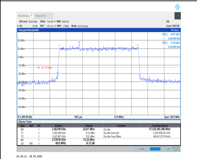
1-N41-PC1-30-60-M-7-CP-16QAM-Outer_Full-162 @ 0-Ant0-57.525-60.000-≤60-PASS
