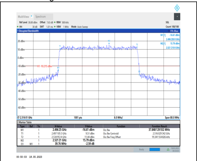
1-N41-PC1-30-40-L-8-CP-64QAM-Outer_Full-106@ 0-Ant0-37.848-39.760-≤40-PASS
