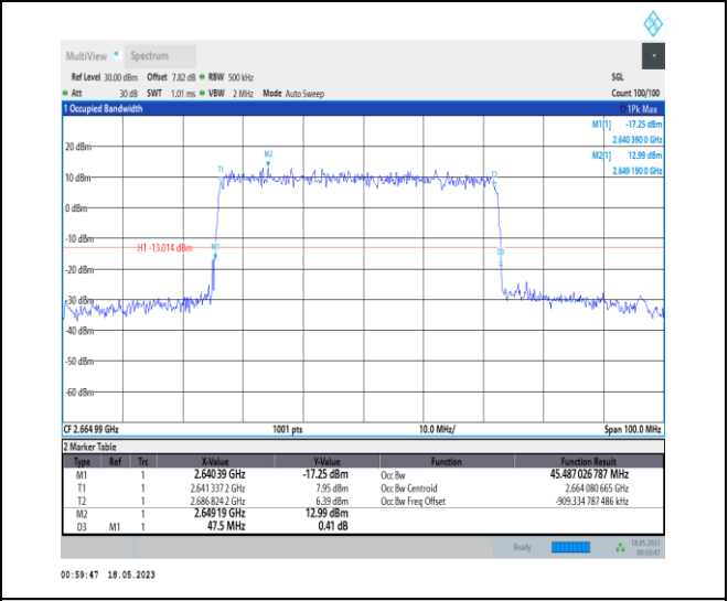
1-N41-PC1-30-50-H-5-DFT-256QAM-Outer_Full-128 @0-Ant0-45.487-47.500-≤50-PASS
