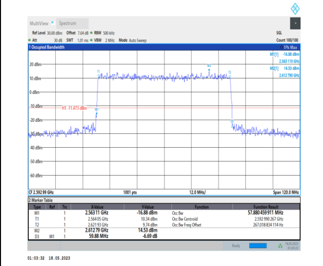
1-N41-PC1-30-60-M-3-DFT-16QAM-Outer_Full-162 @ 0-Ant0-57.88-59.880-≤60-PASS
