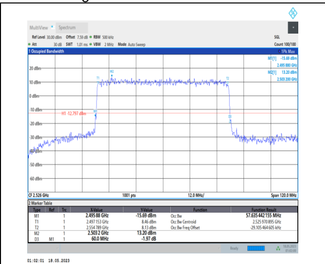
1-N41-PC1-30-60-L-6-CP-QPSK-Outer_Full-162 @ 0-Ant0-57.635-60.000-≤60-PASS
