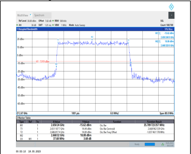
1-N41-PC1-30-40-H-2-DFT-PI2BPSK-Outer_Full-100@0-Ant0-35.71-37.680-≤40-PASS
