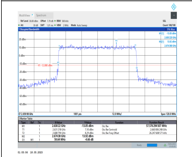
1-N41-PC1-30-60-H-1-DFT-QPSK-Outer_Full-162@ 0-Ant0-57.576-59.640-≤60-PASS
