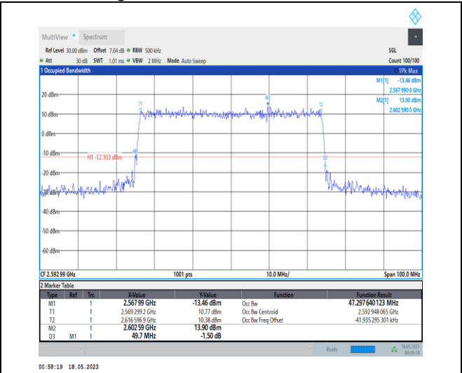
1-N41-PC1-30-50-M-8-CP-64QAM-Outer_Full-133@ 0-Ant0-47.298-49.700-≤50-PASS
