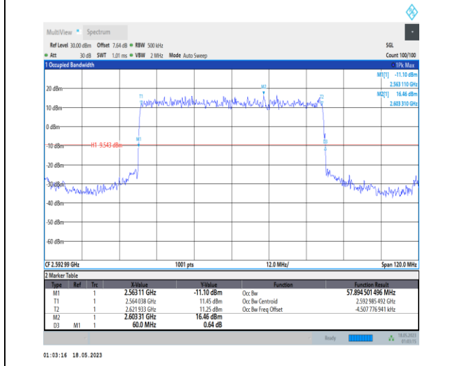
1-N41-PC1-30-60-M-2-DFT-PI2BPSK-Outer_Full-162 @ 0-Ant0-57.895-60.000-≤60-PASS
