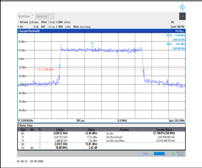
1-N41-PC1-30-60-H-6-CP-QPSK-Outer_Full-162 @ 0-Ant0-57.748-59.880-≤60-PASS
