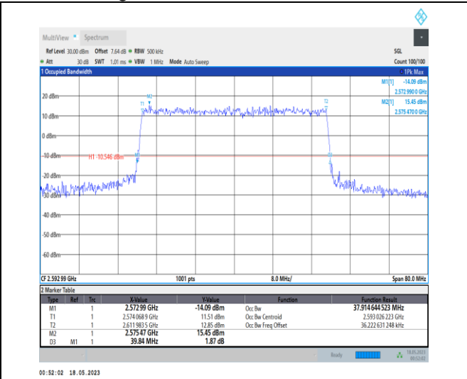
1-N41-PC1-30-40-M-7-CP-16QAM-Outer_Full-106@0 -Ant0-37.915-39.840-≤40-PASS
