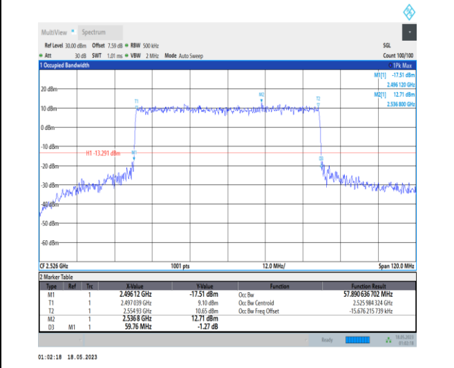
1-N41-PC1-30-60-L-8-CP-64QAM-Outer_Full-162 @ 0-Ant0-57.891-59.760-≤60-PASS
