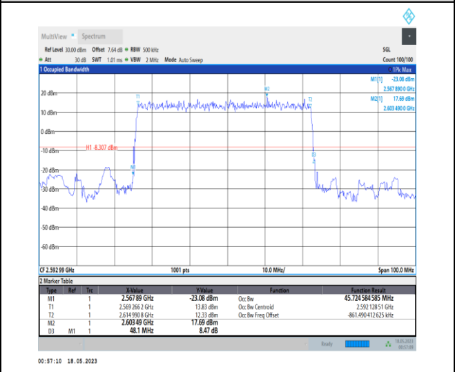
1-N41-PC1-30-50-M-2-DFT-PI2BPSK-Outer_Full-12 8@0-Ant0-45.725-48.100-≤50-PASS
