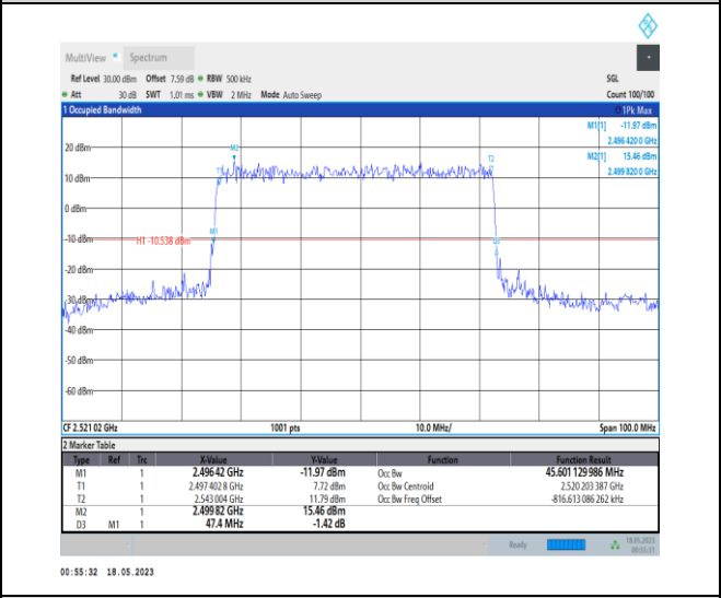
1-N41-PC1-30-50-L-3-DFT-16QAM-Outer_Full-128 @ 0-Ant0-45.601-47.400-≤50-PASS
