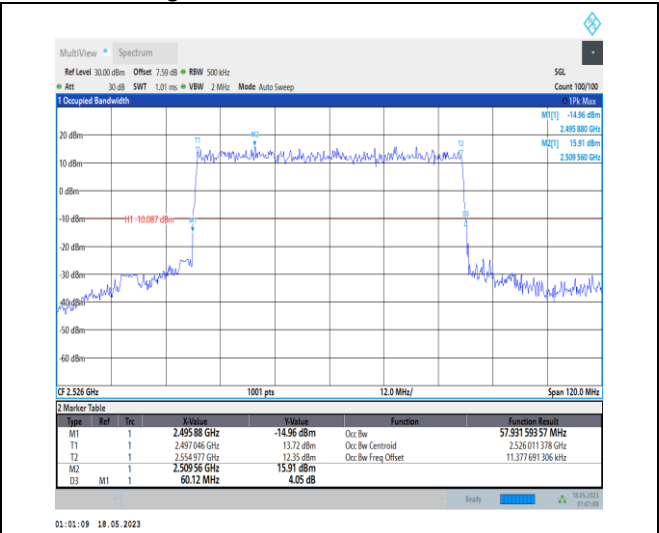
1-N41-PC1-30-60-L-2-DFT-PI2BPSK-Outer_Full-162 @0-Ant0-57.932-60.120-≤60-PASS
