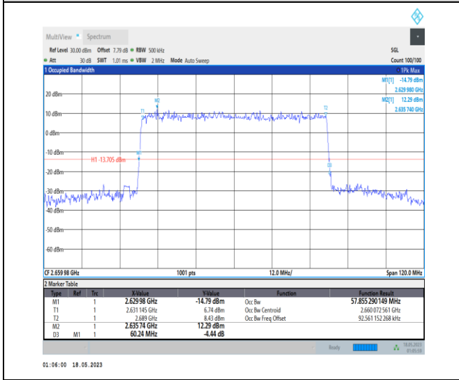
1-N41-PC1-30-60-H-5-DFT-256QAM-Outer_Full-162 @ 0-Ant0-57.855-60.240-≤60-PASS
