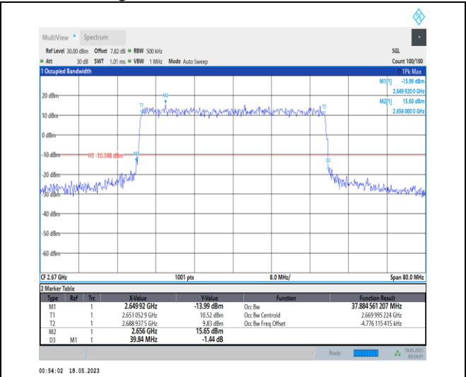
1-N41-PC1-30-40-H-6-CP-QPSK-Outer_Full-106 @ 0-Ant0-37.885-39.840-≤40-PASS
