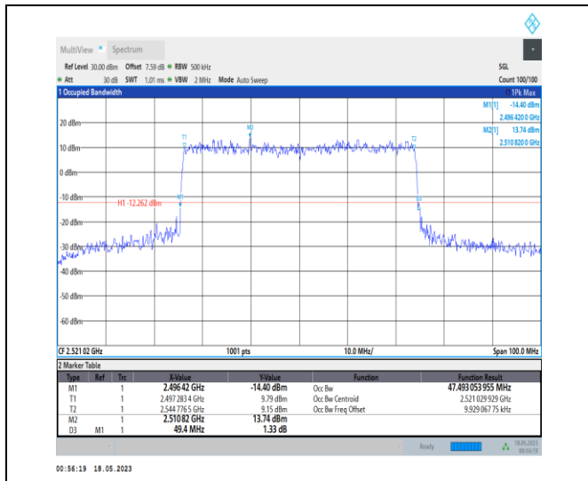
1-N41-PC1-30-50-L-8-CP-64QAM-Outer_Full-133@ 0-Ant0-47.493-49.400-≤50-PASS
