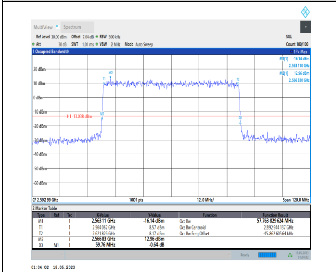
1-N41-PC1-30-60-M-6-CP-QPSK-Outer_Full-162 @ 0-Ant0-57.764-59.760-≤60-PASS
