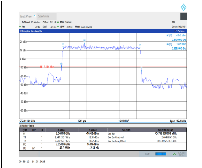
1-N41-PC1-30-50-H-2-DFT-PI2BPSK-Outer_Full-128 @0-Ant0-45.75-47.900-≤50-PASS
