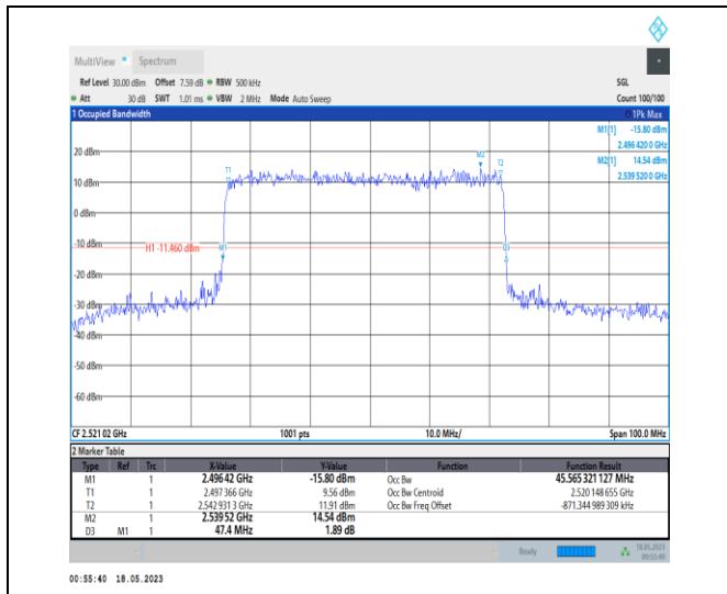
1-N41-PC1-30-50-L-4-DFT-64QAM-Outer_Full-128 @ 0-Ant0-45.565-47.400-≤50-PASS
