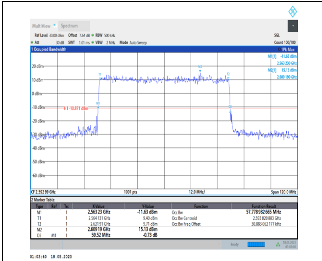
1-N41-PC1-30-60-M-4-DFT-64QAM-Outer_Full-162 @ 0-Ant0-57.779-59.520-≤60-PASS
