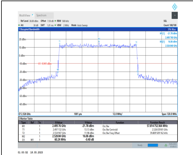
1-N41-PC1-30-60-L-1-DFT-QPSK-Outer_Full-162@0 -Ant0-57.815-60.240-≤60-PASS
