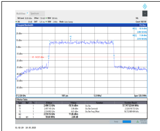
1-N41-PC1-30-60-L-9-CP-256QAM-Outer_Full-162 @ 0-Ant0-57.748-59.640-≤60-PASS
