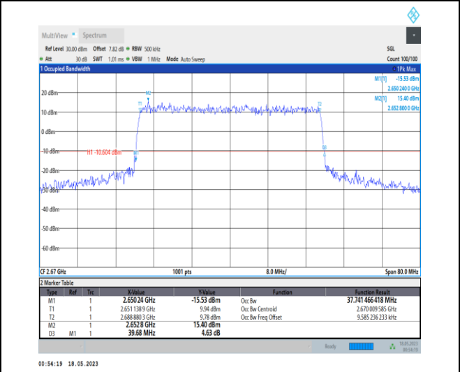
1-N41-PC1-30-40-H-8-CP-64QAM-Outer_Full-106 @ 0-Ant0-37.741-39.680-≤40-PASS
