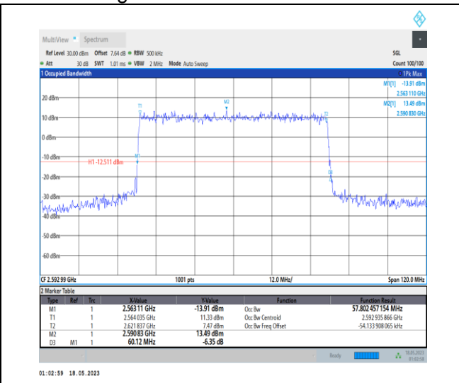
1-N41-PC1-30-60-M-1-DFT-QPSK-Outer_Full-162 @ 0-Ant0-57.802-60.120-≤60-PASS
