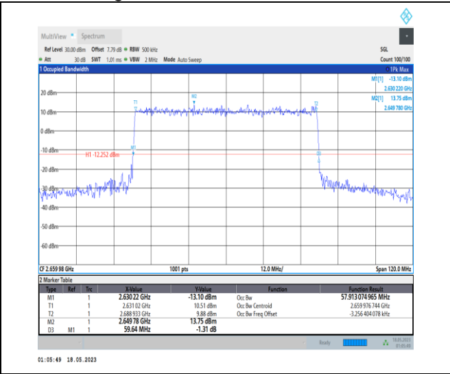
1-N41-PC1-30-60-H-4-DFT-64QAM-Outer_Full-162 @ 0-Ant0-57.913-59.640-≤60-PASS
