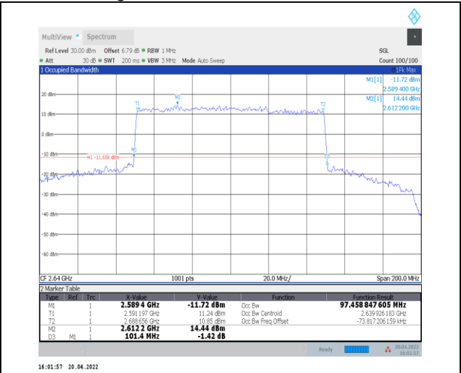
1-N41--30-100-H-8-CP-64QAM-Outer_Full-273@0-A nt0-97.459-101.400-≤100-PASS
