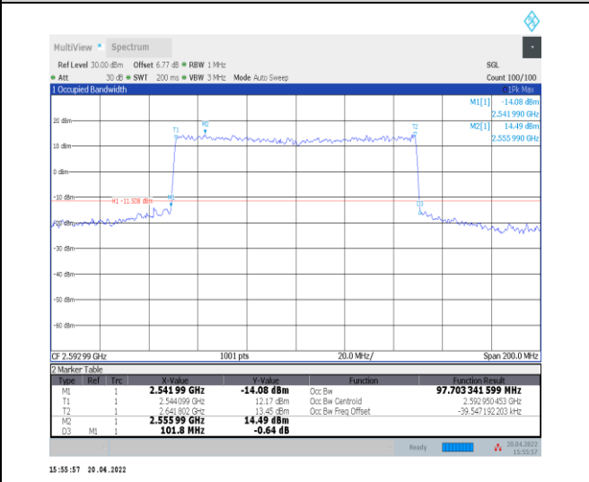
1-N41--30-100-M-7-CP-16QAM-Outer_Full-273@0-Ant0-97.703-101.800-≤100-PASS
