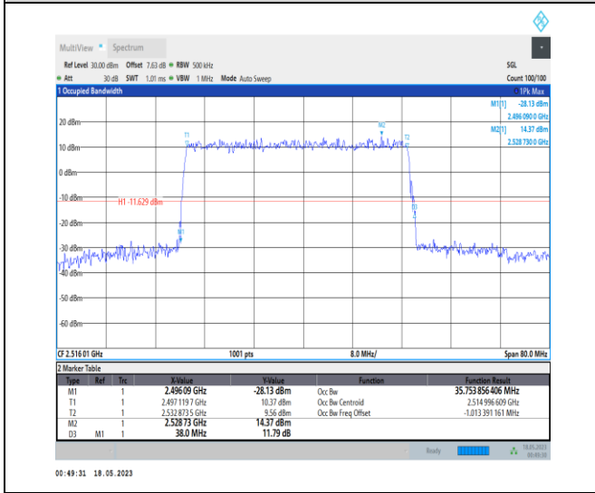
1-N41-PC1-30-40-L-5-DFT-256QAM-Outer_Full-100 @ 0-Ant0-35.754-38.000-≤40-PASS
