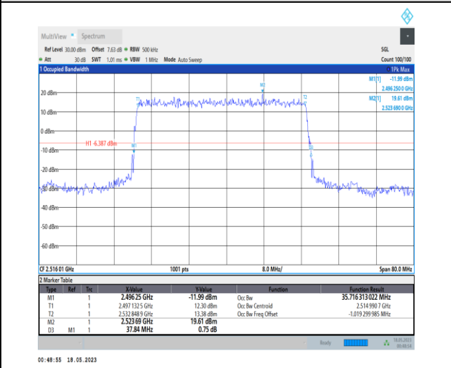
1-N41-PC1-30-40-L-2-DFT-PI2BPSK-Outer_Full-100@0 -Ant0-35.716-37.840-<=40-PASS
