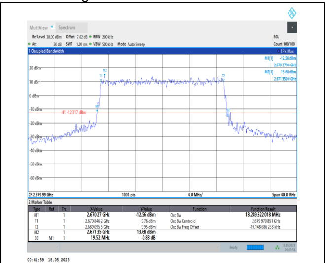
1-N41-PC1-30-20-H-8-CP-64QAM-Outer_Full-51@0 -Ant0-18.249-19.520-≤20-PASS
