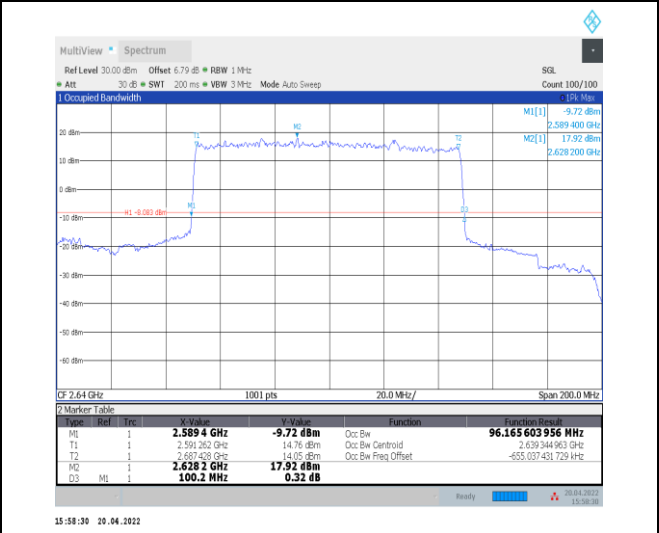
1-N41--30-100-H-2-DFT-Pl2BPSK-Outer_Full-270@ 0-Ant0-96.166-100.200-≤100-PASS
