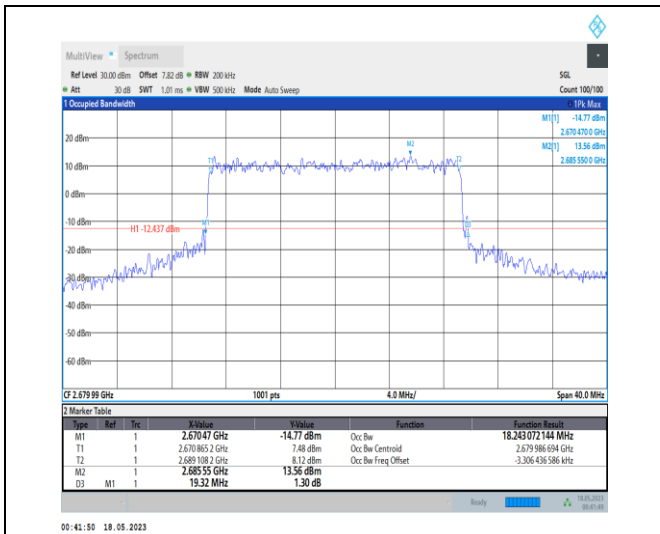
1-N41-PC1-30-20-H-7-CP-16QAM-Outer_Full-51@0 -Ant0-18.243-19.320-≤20-PASS
