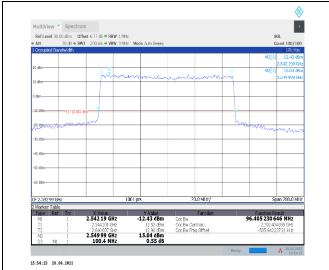
1-N41--30-100-M-4-DFT-64QAM-Outer_Full-270@0-Ant0-96.405-100.400-≤100-PASS
