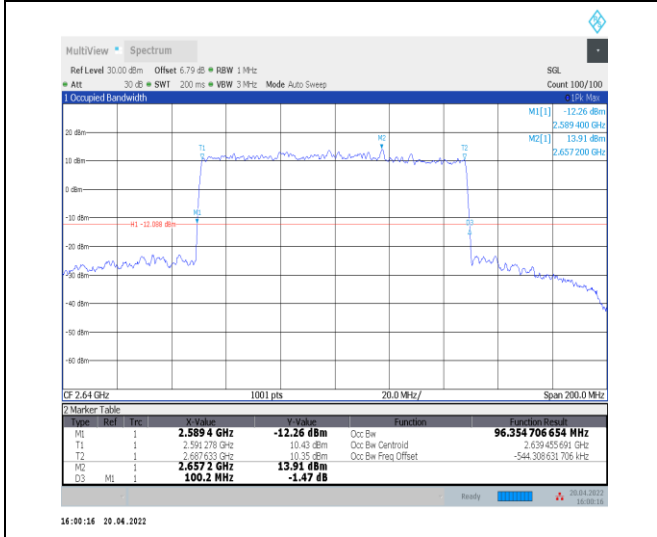
1-N41--30-100-H-5-DFT-256QAM-Outer_Full-270@0-Ant0-96.355-100.200-<=100-PASS
