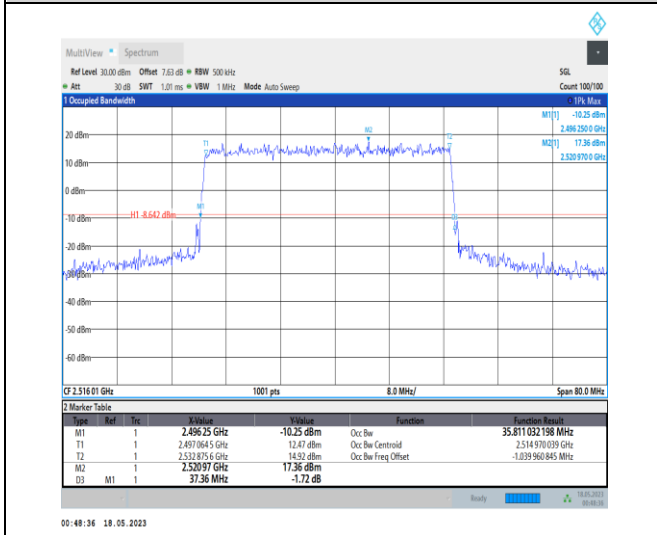
1-N41-PC1-30-40-L-1-DFT-QPSK-Outer_Full-100@0 -Ant0-35.811-37.360-<=40-PASS
