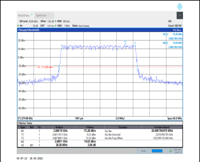
1-N41-PC1-30-30-H-3-DFT-16QAM-Outer_Full-75@ 0-Ant0-26.699-28.380-≤30-PASS
