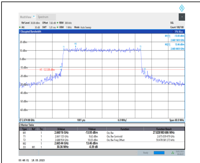
1-N41-PC1-30-30-H-8-CP-64QAM-Outer_Full-78@0 -Ant0-27.829-30.360-<=30-PASS
