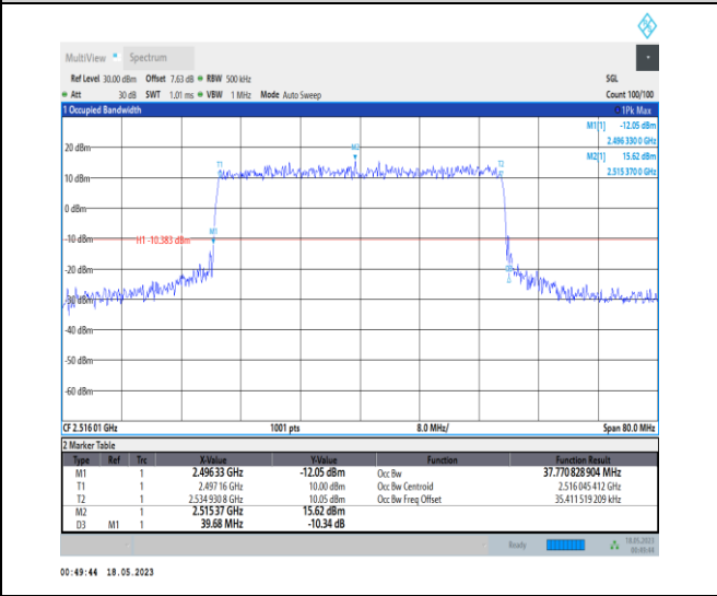
1-N41-PC1-30-40-L-6-CP-QPSK-Outer_Full-106 @ 0-Ant0-37.771-39.680-≤40-PASS
