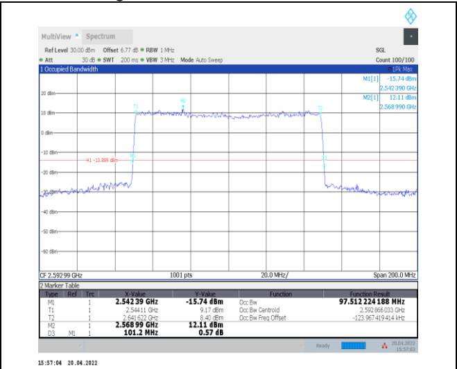
1-N41--30-100-M-9-CP-256QAM-Outer_Full-273@0- Ant0-97.512-101.200-≤100-PASS
