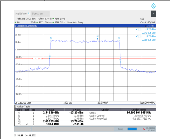
1-N41--30-100-M-5-DFT-256QAM-Outer_Full-270@0-Ant0-96.592-100.400-≤100-PASS
