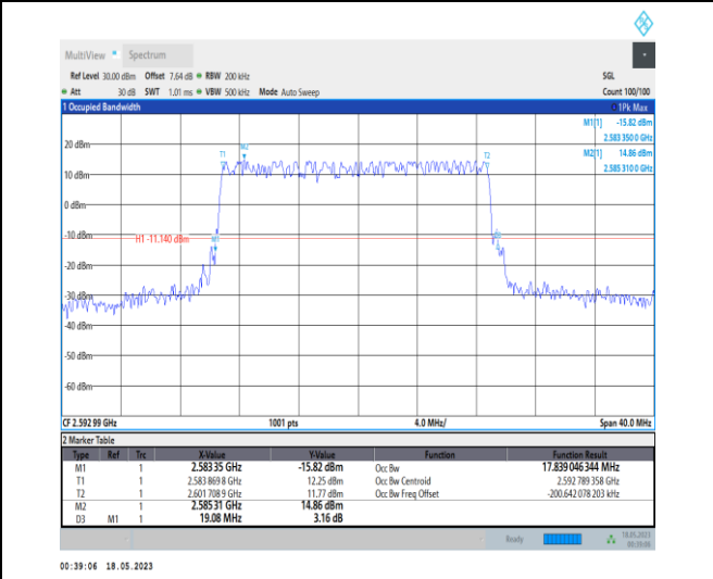
1-N41-PC1-30-20-M-3-DFT-16QAM-Outer_Full-50@ 0-Ant0-17.839-19.080-≤20-PASS
