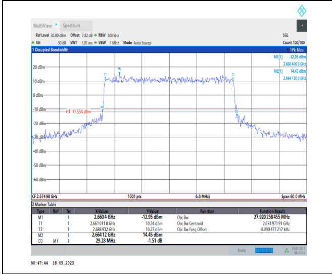
1-N41-PC1-30-30-H-6-CP-QPSK-Outer_Full-78@0- Ant0-27.92-29.280-≤30-PASS
