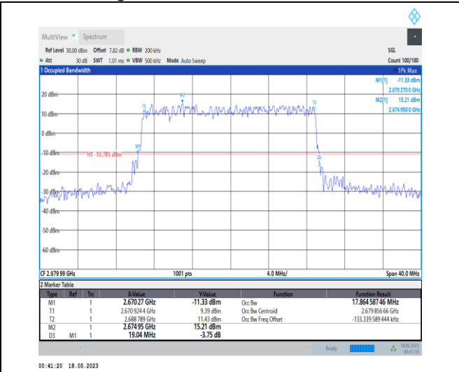
1-N41-PC1-30-20-H-4-DFT-64QAM-Outer_Full-50@ 0-Ant0-17.865-19.040-≤20-PASS
