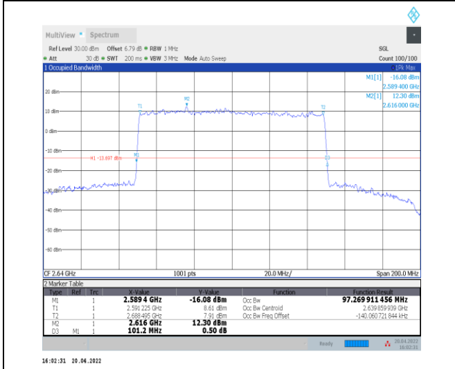
1-N41--30-100-H-9-CP-256QAM-Outer_Full-273@0-A Ant0-97.27-101.200-≤100-PASS
