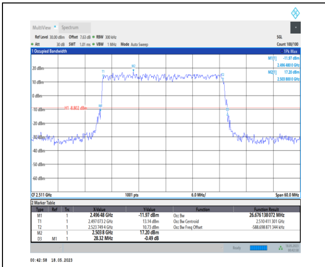
1-N41-PC1-30-30-L-2-DFT-PI2BPSK-Outer_Full-75 @ 0-Ant0-26.676-28.320-≤30-PASS
