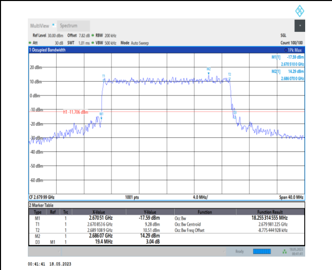
1-N41-PC1-30-20-H-6-CP-QPSK-Outer_Full-51@0- Ant0-18.255-19.400-≤20-PASS
