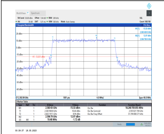
1-N41-PC1-30-20-M-6-CP-QPSK-Outer_Full-51@0- Ant0-18.241-19.480-<=20-PASS
