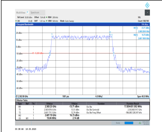
1-N41-PC1-30-20-M-2-DFT-PI2BPSK-Outer_Full-50@ 0-Ant0-17.855-19.040-≤20-PASS
