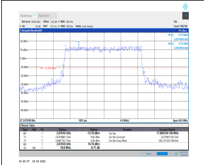
1-N41-PC1-30-20-H-1-DFT-QPSK-Outer_Full-50 @ 0-Ant0-17.839-18.800-<math>\leq 20</math>-PASS
