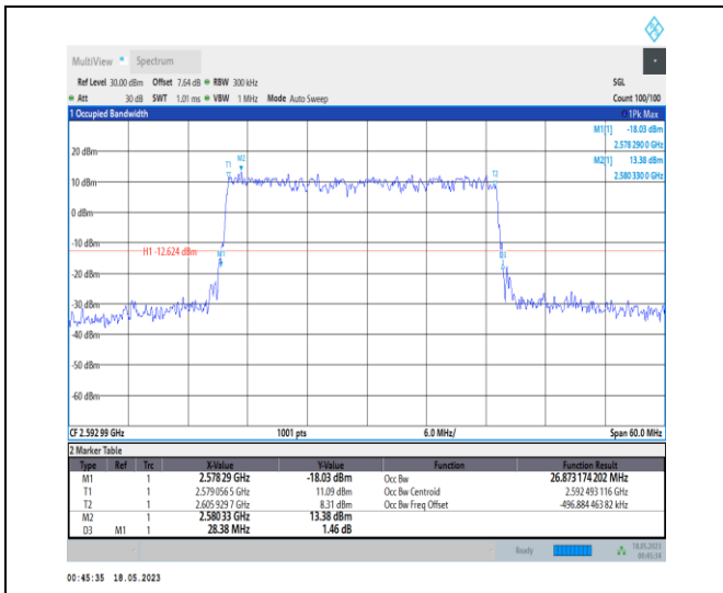
1-N41-PC1-30-30-M-5-DFT-256QAM-Outer_Full-75 @ 0-Ant0-26.873-28.380-≤30-PASS
