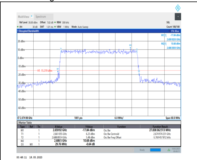
1-N41-PC1-30-30-H-9-CP-256QAM-Outer_Full-78@0 -Ant0-27.838-29.760-<=30-PASS
