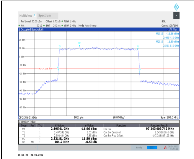
1-N41--30-100-L-9-CP-256QAM-Outer_Full-273@0-Ant0-97.243-101.200-≤100-PASS
