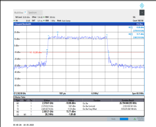
1-N41-PC1-30-30-M-4-DFT-64QAM-Outer_Full-75@0 -Ant0-26.795-28.200-≤30-PASS
