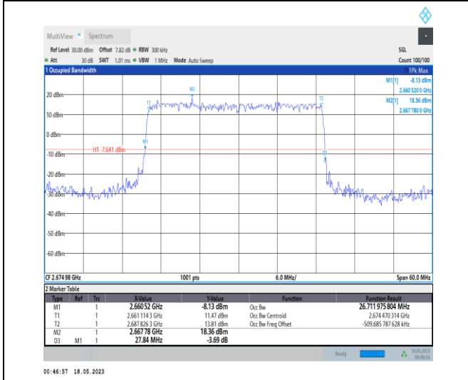
1-N41-PC1-30-30-H-2-DFT-PI2BPSK-Outer_Full-75 @0-Ant0-26.712-27.840-≤30-PASS
