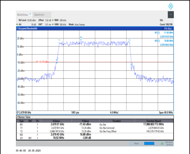
1-N41-PC1-30-20-H-2-DFT-PI2BPSK-Outer_Full-50 @ 0-Ant0-17.887-18.920-<math>\leq 20</math>-PASS
