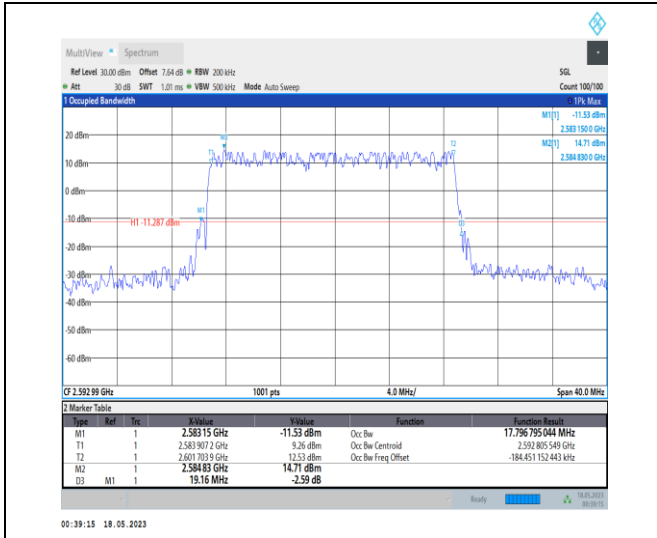
1-N41-PC1-30-20-M-4-DFT-64QAM-Outer_Full-50@ 0-Ant0-17.797-19.160-<=20-PASS
