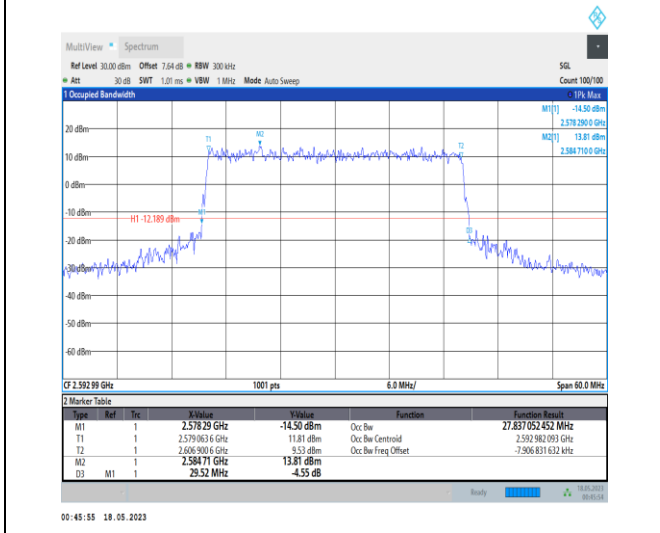
1-N41-PC1-30-30-M-7-CP-16QAM-Outer_Full-78 @ 0-Ant0-27.837-29.520-≤30-PASS
