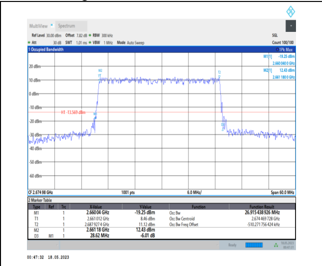
1-N41-PC1-30-30-H-5-DFT-256QAM-Outer_Full-75@ 0-Ant0-26.915-28.620-≤30-PASS
