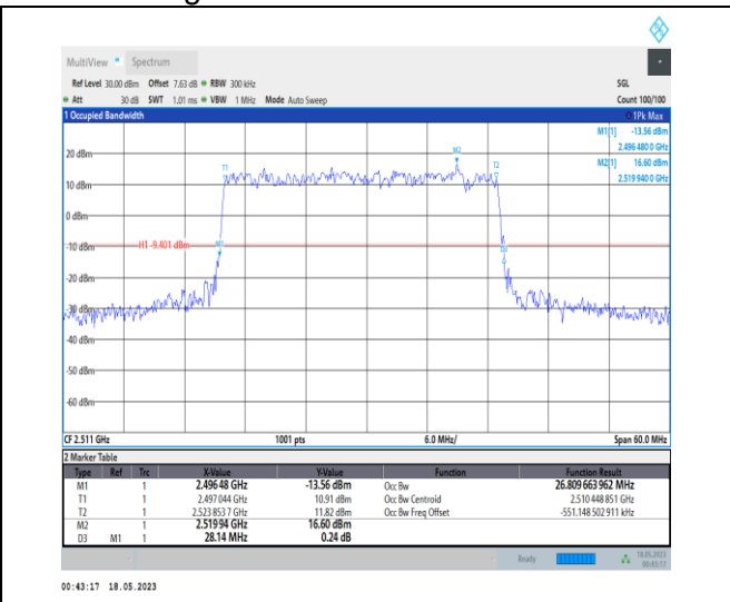
1-N41-PC1-30-30-L-3-DFT-16QAM-Outer_Full-75 @ 0-Ant0-26.81-28.140-≤30-PASS
