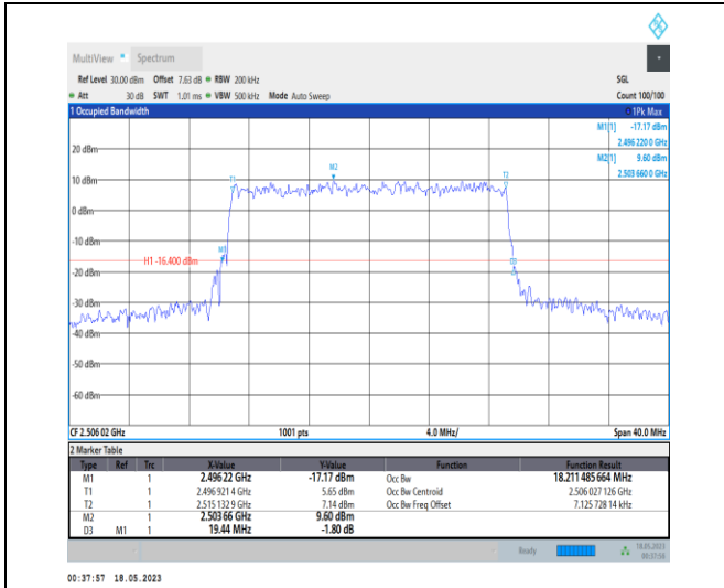
1-N41-PC1-30-20-L-9-CP-256QAM-Outer_Full-51@ 0-Ant0-18.211-19.440-≤20-PASS
