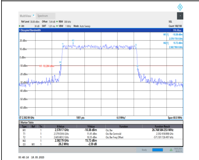
1-N41-PC1-30-30-M-3-DFT-16QAM-Outer_Full-75@0 -Ant0-26.769-28.200-≤30-PASS
