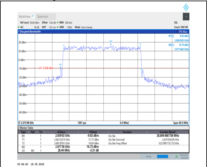
1-N41-PC1-30-30-H-1-DFT-QPSK-Outer_Full-75@0- Ant0-26.844-28.440-≤30-PASS
