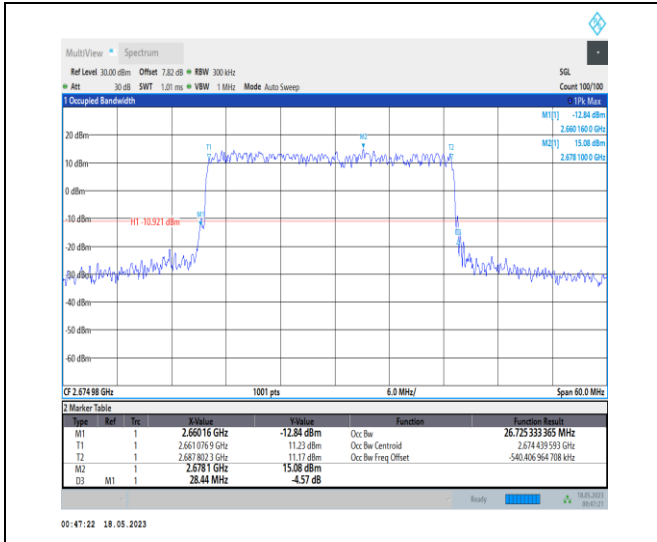
1-N41-PC1-30-30-H-4-DFT-64QAM-Outer_Full-75@ 0-Ant0-26.725-28.440-≤30-PASS
