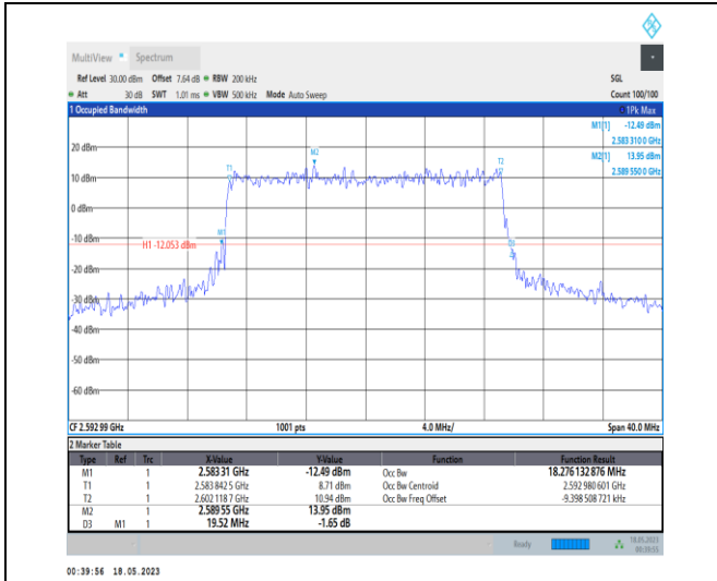
1-N41-PC1-30-20-M-8-CP-64QAM-Outer_Full-51 @ 0 -Ant0-18.276-19.520-<math>\leq 20</math>-PASS
