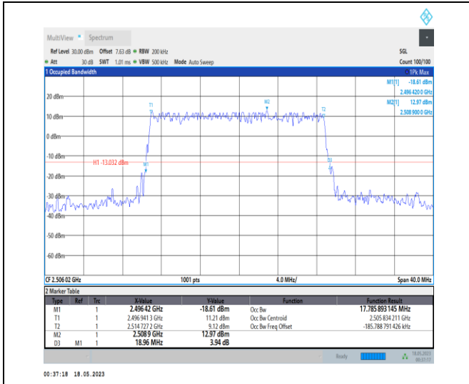
1-N41-PC1-30-20-L-5-DFT-256QAM-Outer_Full-50 @0-Ant0-17.786-18.960-≤20-PASS
