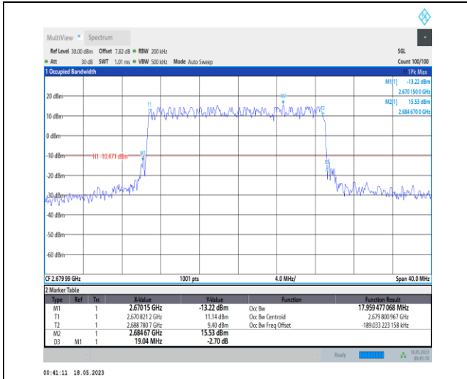
1-N41-PC1-30-20-H-3-DFT-16QAM-Outer_Full-50@ 0-Ant0-17.959-19.040-≤20-PASS
