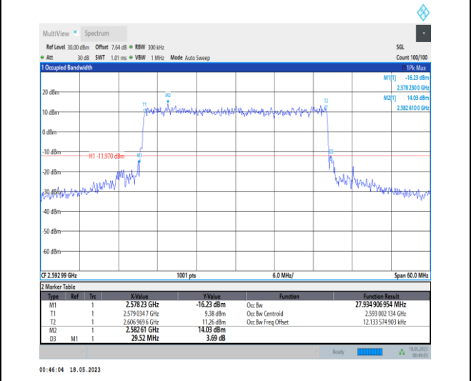
1-N41-PC1-30-30-M-8-CP-64QAM-Outer_Full-78 @ 0-Ant0-27.935-29.520-≤30-PASS
