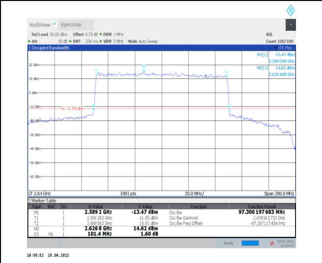
1-N41--30-100-H-6-CP-QPSK-Outer_Full-273@0-Ant0-97.3-101.400-<=100-PASS
