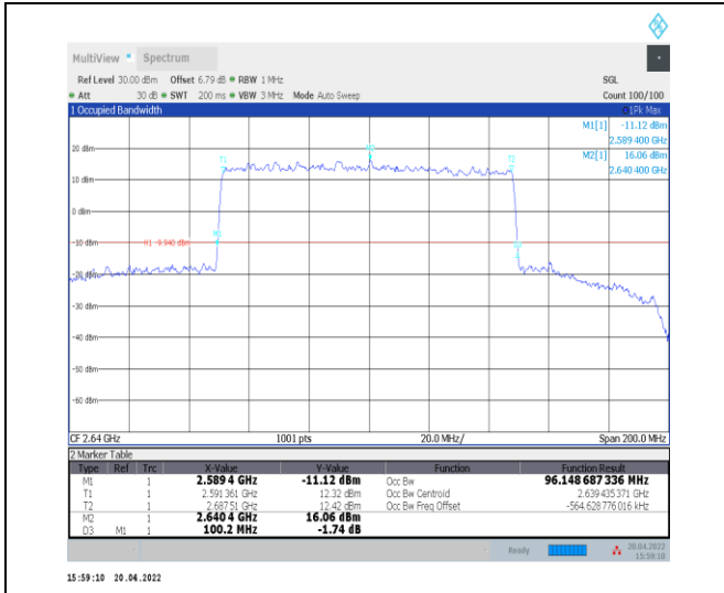
1-N41--30-100-H-3-DFT-16QAM-Outer_Full-270@0-Ant0-96.149-100.200-<=100-PASS
