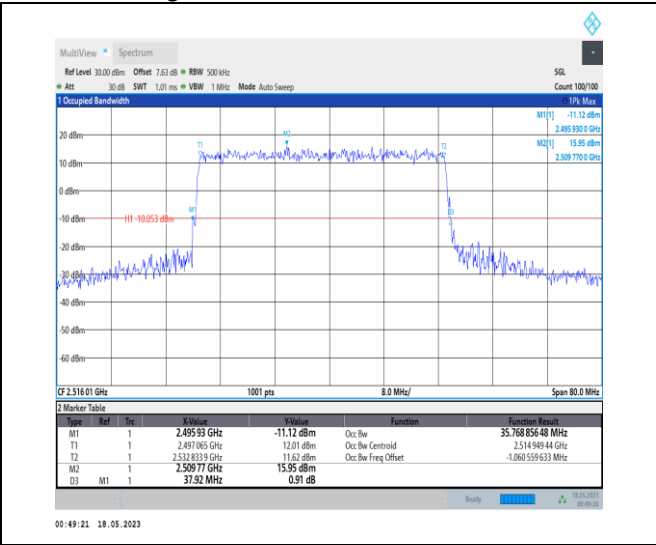
1-N41-PC1-30-40-L-4-DFT-64QAM-Outer_Full-100 @ 0-Ant0-35.769-37.920-≤40-PASS
