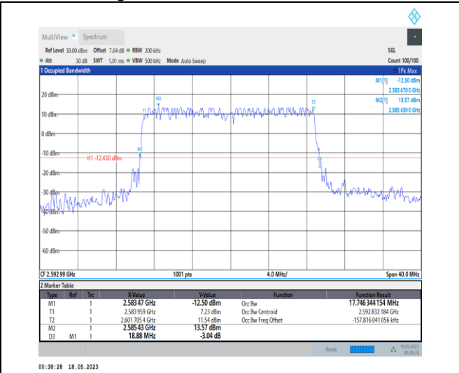
1-N41-PC1-30-20-M-1-DFT-QPSK-Outer_Full-50@0 -Ant0-17.746-18.880-≤20-PASS
