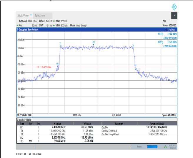
1-N41-PC1-30-20-L-6-CP-QPSK-Outer_Full-51 @0-Ant0-18.145-19.440-≤20-PASS
