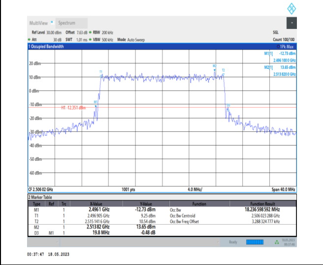
1-N41-PC1-30-20-L-8-CP-64QAM-Outer_Full-51 @0-Ant0-18.237-19.800-≤20-PASS
