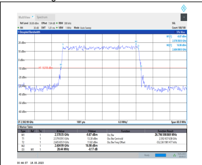
1-N41-PC1-30-30-M-2-DFT-PI2BPSK-Outer_Full-75@0 -Ant0-26.797-28.440-≤30-PASS
