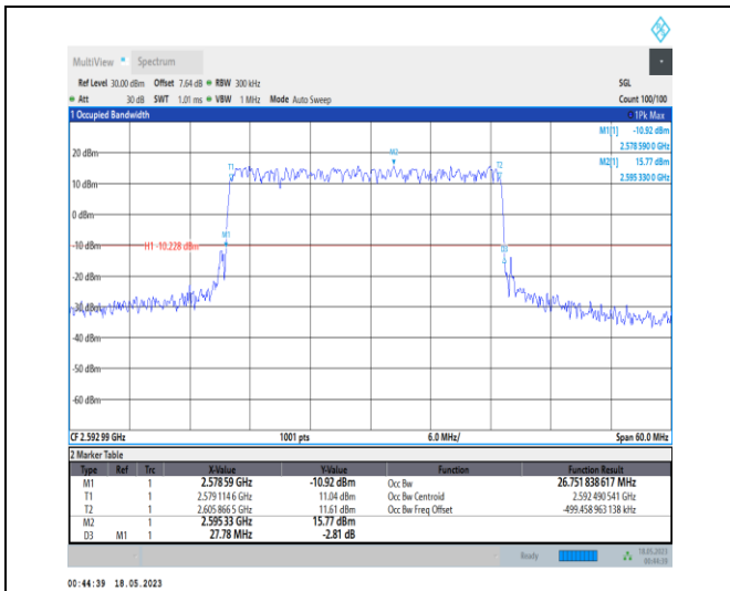
1-N41-PC1-30-30-M-1-DFT-QPSK-Outer_Full-75@0 -Ant0-26.752-27.780-≤30-PASS
