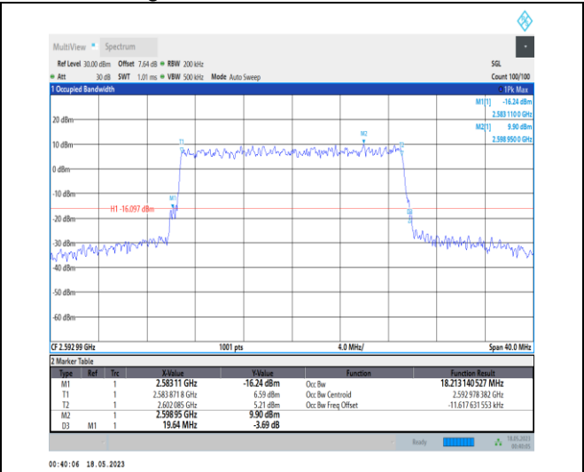
1-N41-PC1-30-20-M-9-CP-256QAM-Outer_Full-51 @ 0-Ant0-18.213-19.640-<math>\leq 20</math>-PASS
