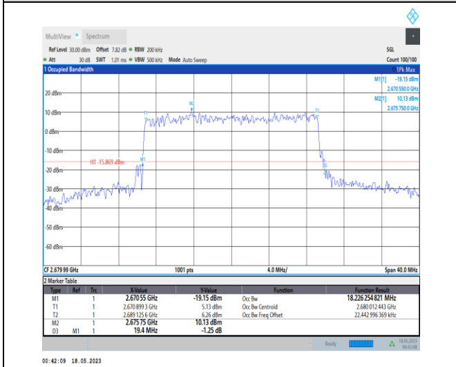
1-N41-PC1-30-20-H-9-CP-256QAM-Outer_Full-51@0 0-Ant0-18.226-19.400-≤20-PASS
