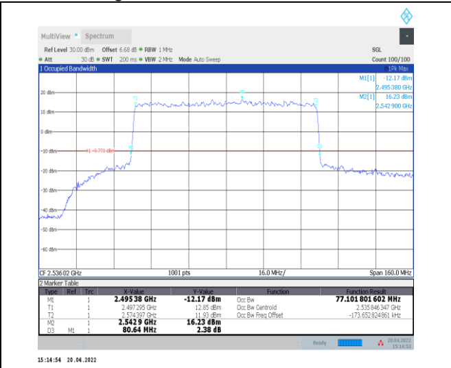
1-N41--30-80-L-4-DFT-64QAM-Outer_Full-216@0-A nt0-77.102-80.640-<math>\leq 80</math>-PASS
