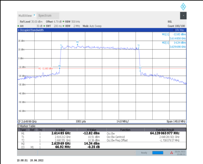
1-N41--30-70-H-3-DFT-16QAM-Outer_Full-180@0-A nt0-64.139-66.920-≤70-PASS
