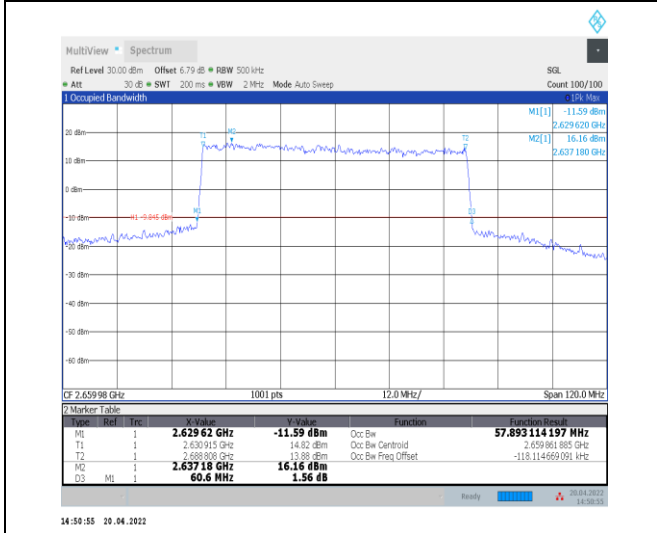
1-N41--30-60-H-1-DFT-QPSK-Outer_Full-162@0-An t0-57.893-60.600-≤60-PASS
