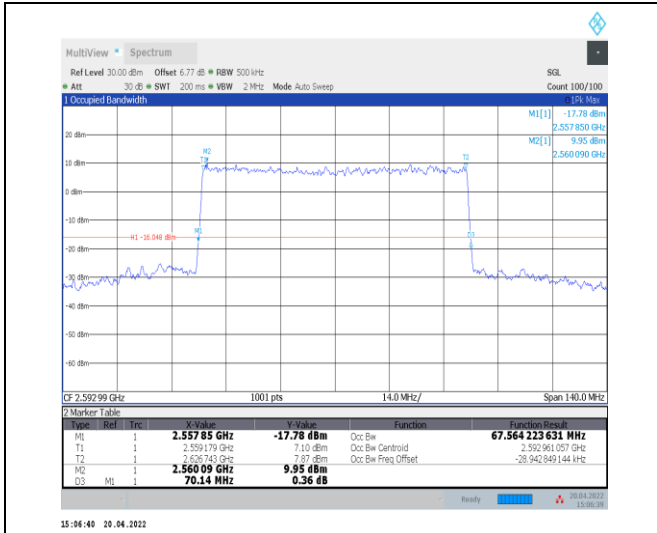
1-N41--30-70-M-9-CP-256QAM-Outer_Full-189@0-A nt0-67.564-70.140-≤70-PASS
