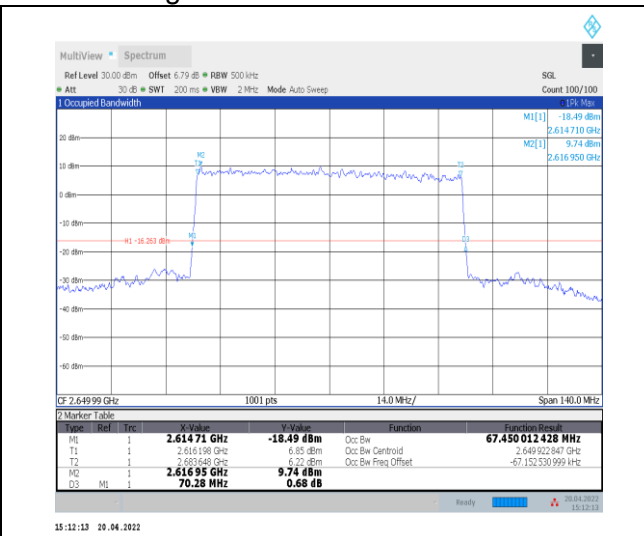
1-N41--30-70-H-9-CP-256QAM-Outer_Full-189@0-A nt0-67.45-70.280-≤70-PASS
