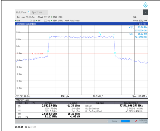
1-N41--30-80-M-8-CP-64QAM-Outer_Full-217@0-Ant t0-77.541-81.120-<80-PASS
