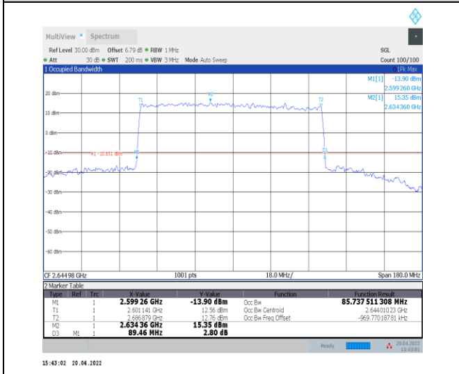
1-N41--30-90-H-4-DFT-64QAM-Outer_Full-240@0-A Ant0-85.738-89.460-≤90-PASS
