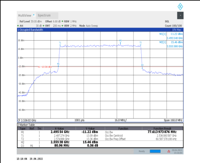
1-N41--30-80-L-6-CP-QPSK-Outer_Full-217@0-Ant 0-77.614-80.960-<math>\leq 80</math>-PASS
