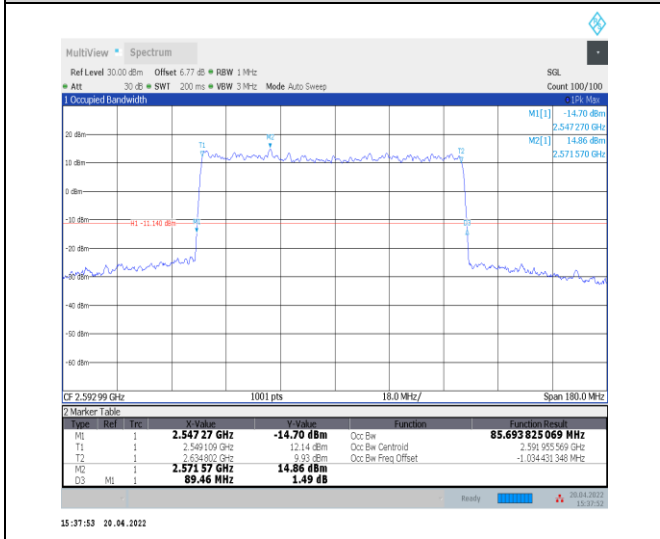
1-N41--30-90-M-5-DFT-256QAM-Outer_Full-240@0-O Ant0-85.694-89.460-≤90-PASS
