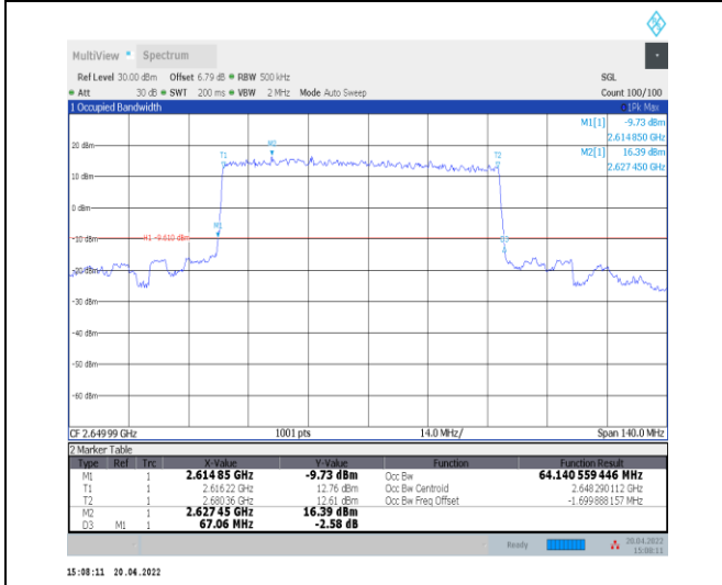
1-N41--30-70-H-2-DFT-PI2BPSK-Outer_Full-180@0-A Ant0-64.141-67.060-≤70-PASS
