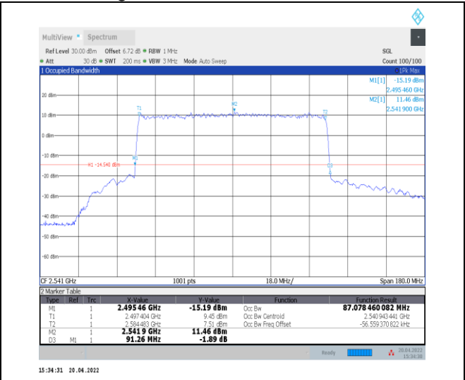
1-N41--30-90-L-9-CP-256QAM-Outer_Full-245@0-Ant 0-87.078-91.260-≤90-PASS
