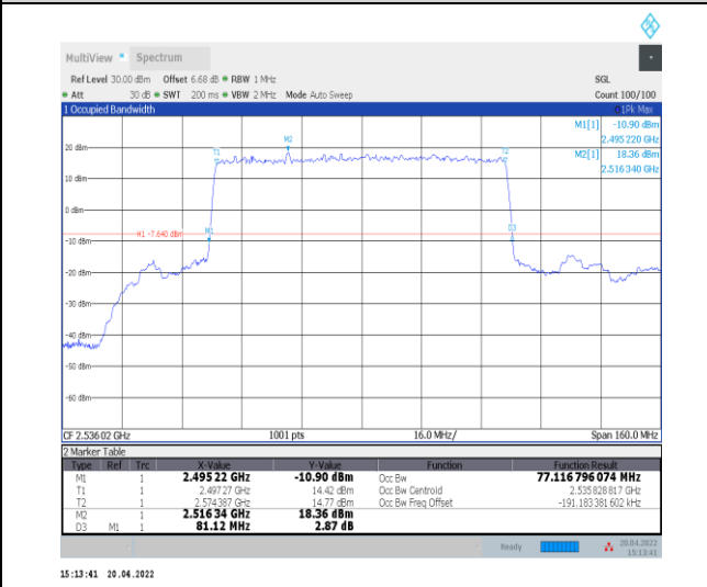
1-N41--30-80-L-2-DFT-PI2BPSK-Outer_Full-216@0-Ant 0-77.117-81.120-≤80-PASS
