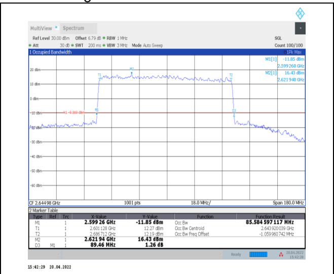
1-N41--30-90-H-3-DFT-16QAM-Outer_Full-240@0-A Ant0-85.585-89.460-≤90-PASS
