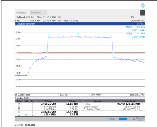
1-N41--30-100-L-7-CP-16QAM-Outer_Full-273@0-A nt0-97.464-101.400-≤100-PASS
