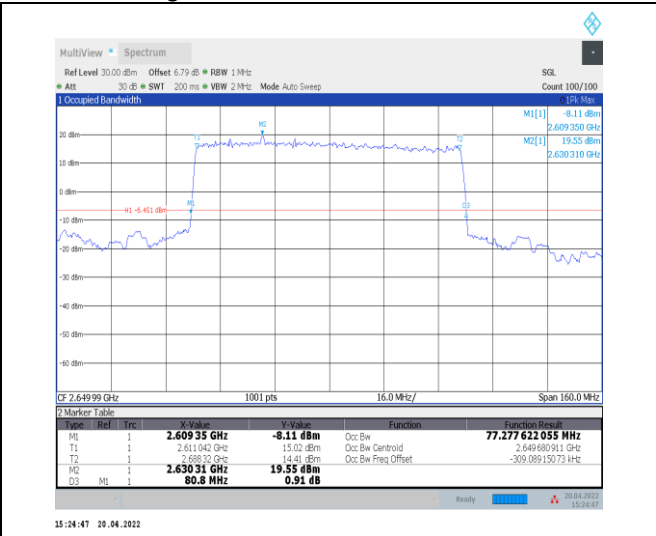
1-N41--30-80-H-2-DFT-PI2BPSK-Outer_Full-216@0 -Ant0-77.278-80.800-<math>\leq 80</math>-PASS
