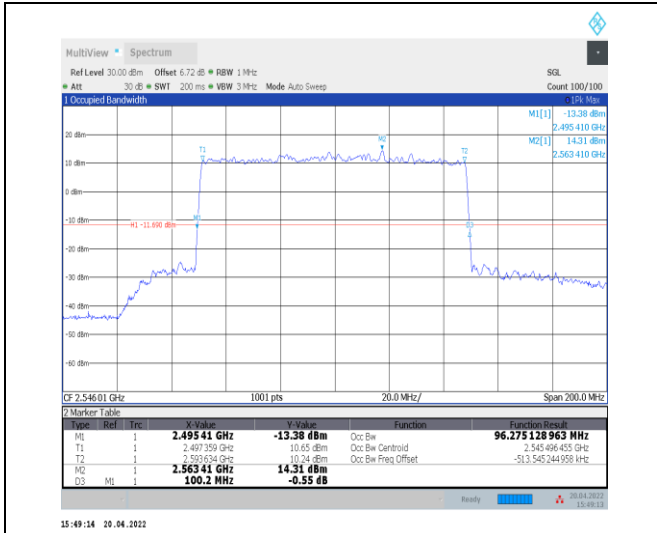
1-N41--30-100-L-5-DFT-256QAM-Outer_Full-270@0 -Ant0-96.275-100.200-≤100-PASS
