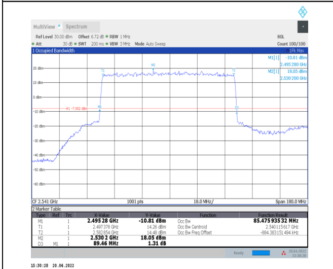
1-N41--30-90-L-2-DFT-PI2BPSK-Outer_Full-240@0-Ant0 0-85.476-89.460-≤90-PASS
