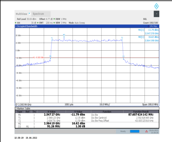
1-N41--30-90-M-6-CP-QPSK-Outer_Full-245@0-Ant 0-87.608-91.260-≤90-PASS
