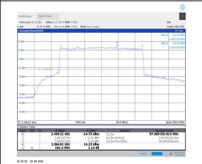
1-N41--30-100-L-8-CP-64QAM-Outer_Full-273@0-A nt0-97.37-101.400-≤100-PASS
