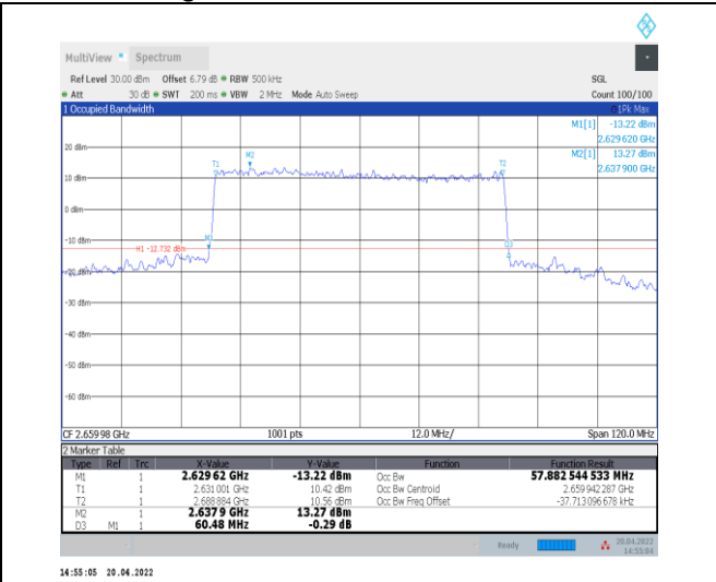
1-N41--30-60-H-8-CP-64QAM-Outer_Full-162@0-An t0-57.883-60.480-<=60-PASS
