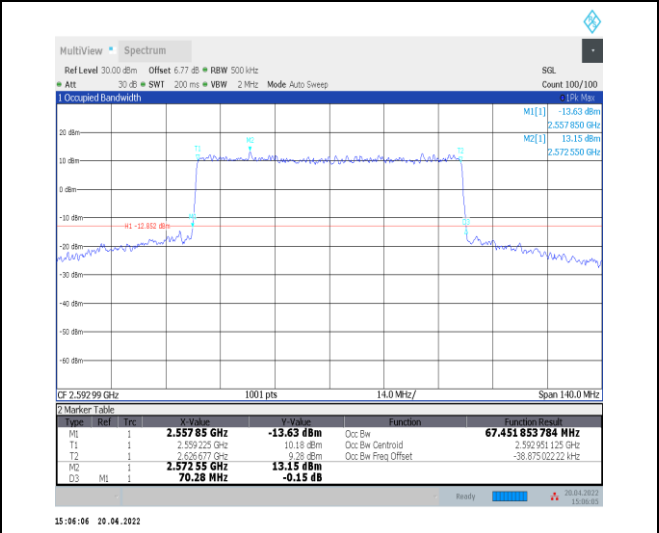
1-N41--30-70-M-8-CP-64QAM-Outer_Full-189@0-Ant 0-67.452-70.280-<=70-PASS
