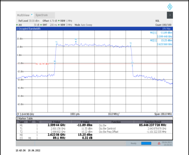
1-N41--30-90-H-5-DFT-256QAM-Outer_Full-240@0-A Ant0-85.446-89.100-≤90-PASS
