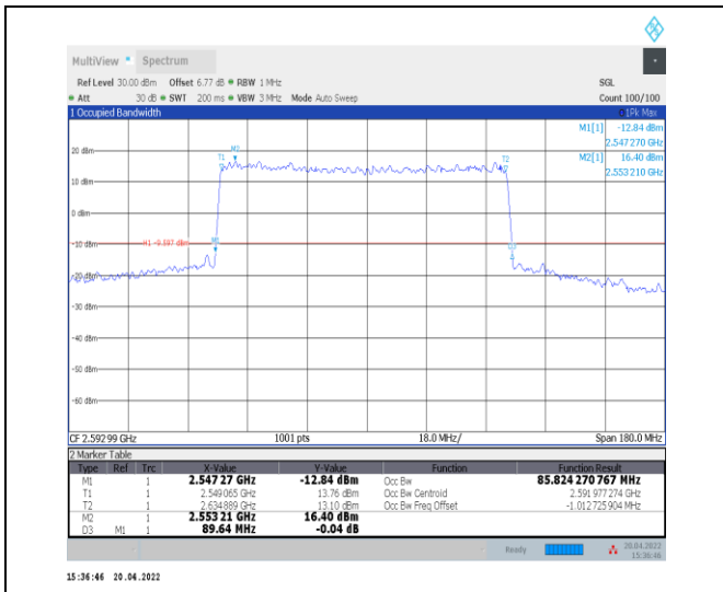
1-N41--30-90-M-3-DFT-16QAM-Outer_Full-240@0-A Ant0-85.824-89.640-≤90-PASS
