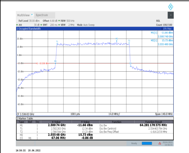
1-N41--30-70-L-1-DFT-QPSK-Outer_Full-180@0-Ant 0-64.281-67.060-<=70-PASS
