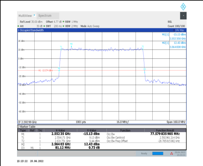
1-N41--30-80-M-9-CP-256QAM-Outer_Full-217@0-Ant Ant0-77.58-81.120-<80-PASS
