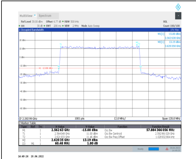
1-N41--30-60-M-8-CP-64QAM-Outer_Full-162@0-An t0-57.884-60.480-≤60-PASS
