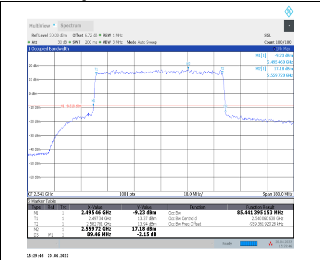
1-N41--30-90-L-1-DFT-QPSK-Outer_Full-240@0-Ant 0-85.441-89.460-≤90-PASS
