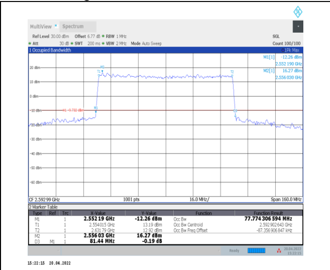
1-N41--30-80-M-7-CP-16QAM-Outer_Full-217@0-Ant nt0-77.774-81.440-<80-PASS
