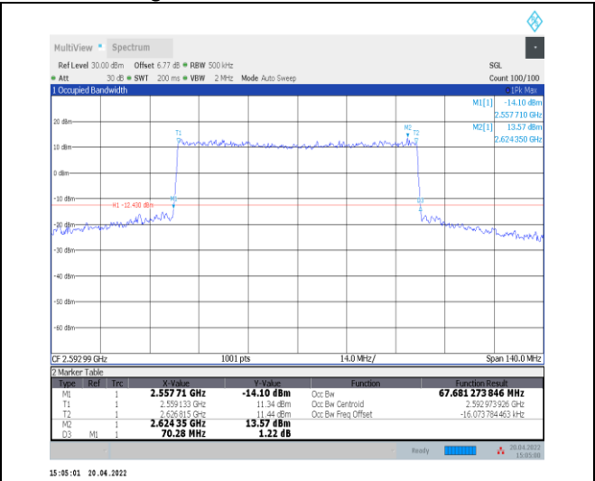
1-N41--30-70-M-6-CP-QPSK-Outer_Full-189@0-Ant 0-67.681-70.280-<=70-PASS
