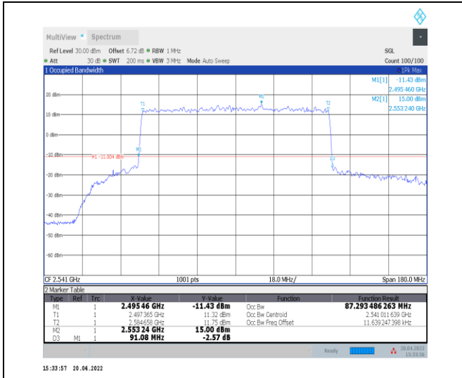
1-N41--30-90-L-8-CP-64QAM-Outer_Full-245@0-Ant 0-87.293-91.080-≤90-PASS
