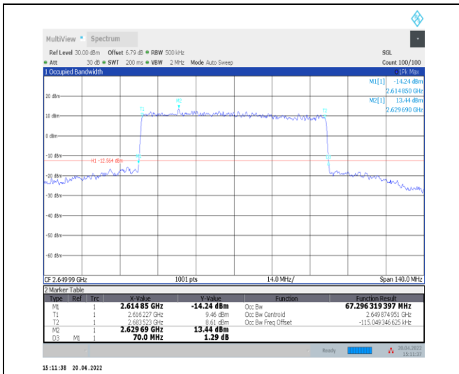
1-N41--30-70-H-8-CP-64QAM-Outer_Full-189@0-A t0-67.296-70.000-≤70-PASS
