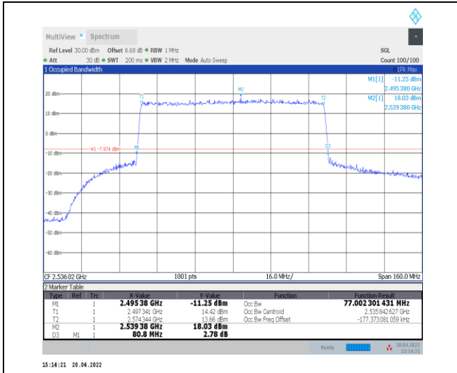
1-N41--30-80-L-3-DFT-16QAM-Outer_Full-216@0-A nt0-77.002-80.800-<math>\leq 80</math>-PASS
