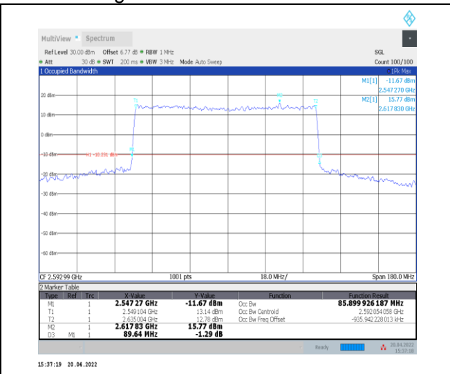
1-N41--30-90-M-4-DFT-64QAM-Outer_Full-240@0-O Ant0-85.9-89.640-≤90-PASS
