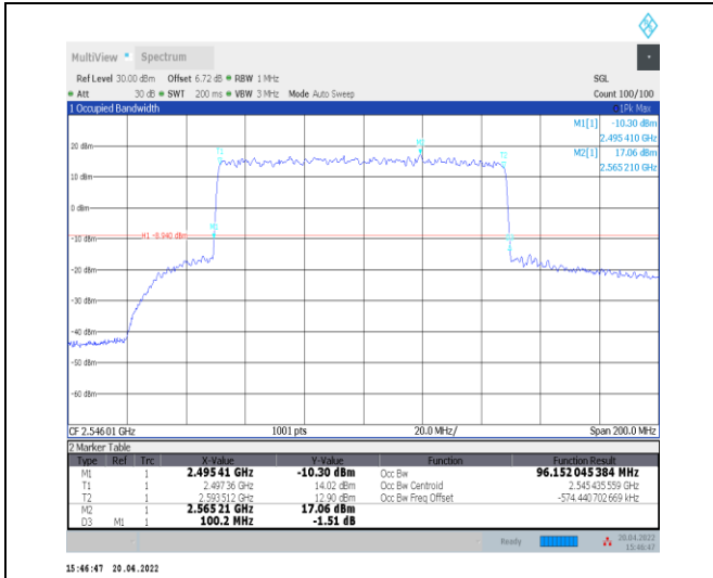
1-N41--30-100-L-1-DFT-QPSK-Outer_Full-270@0-A nt0-96.152-100.200-≤100-PASS
