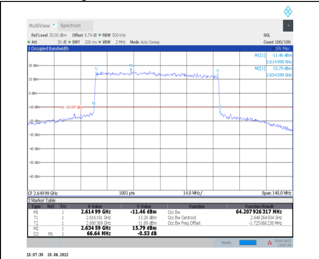
1-N41--30-70-H-1-DFT-QPSK-Outer_Full-180@0-An t0-64.208-66.640-≤70-PASS
