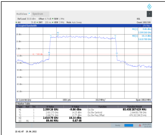
1-N41--30-90-H-2-DFT-PI2BPSK-Outer_Full-240@0-A Ant0-85.458-89.460-≤90-PASS
