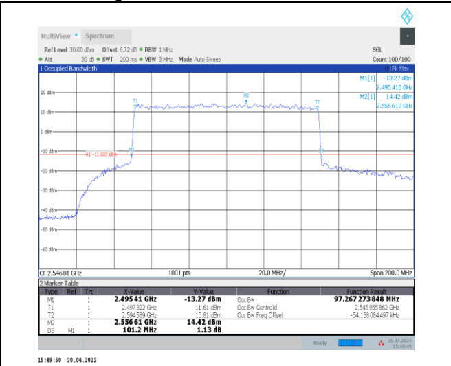
1-N41--30-100-L-6-CP-QPSK-Outer_Full-273@0-An t0-97.267-101.200-≤100-PASS
