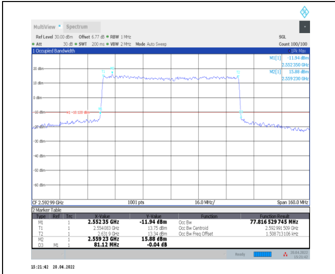
1-N41--30-80-M-6-CP-QPSK-Outer_Full-217@0-Ant 0-77.817-81.120-<80-PASS
