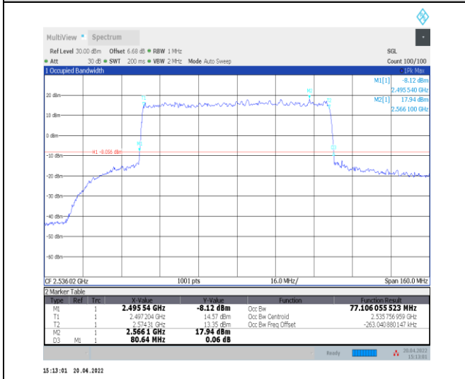
1-N41--30-80-L-1-DFT-QPSK-Outer_Full-216@0-Ant 0-77.106-80.640-≤80-PASS
