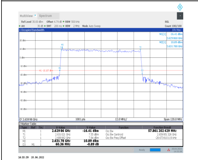
1-N41--30-60-H-9-CP-256QAM-Outer_Full-162@0-A nt0-57.861-60.360-<=60-PASS
