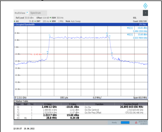
1-N41--30-30-L-3-DFT-16QAM-Outer_Full-75@0-An t0-26.895-28.800-≤30-PASS
