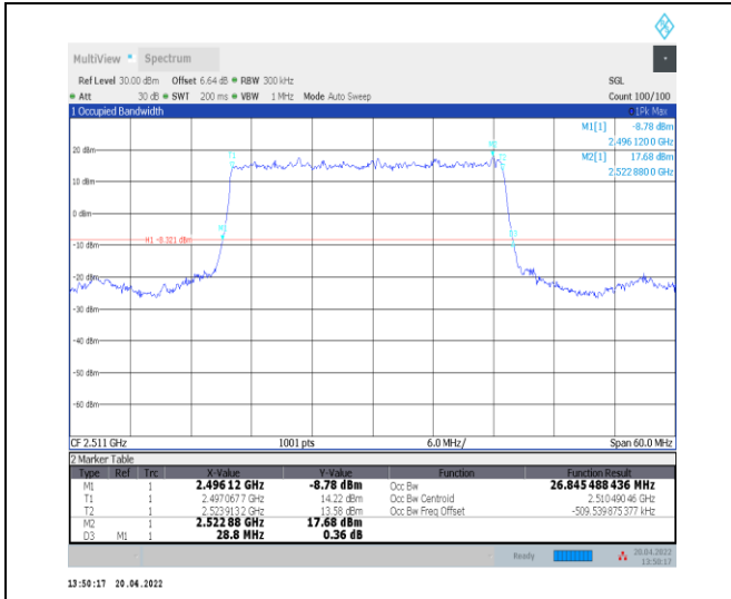
1-N41--30-30-L-2-DFT-PI2BPSK-Outer_Full-75@0-A nt0-26.845-28.800-≤30-PASS
