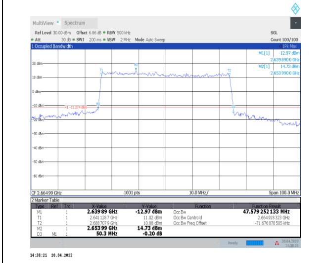
1-N41--30-50-H-8-CP-64QAM-Outer_Full-133@0-Ant t0-47.579-50.300-≤50-PASS
