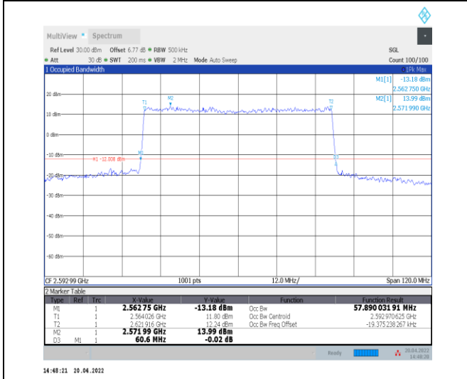
1-N41--30-60-M-6-CP-QPSK-Outer_Full-162@0-Ant 0-57.89-60.600-≤60-PASS
