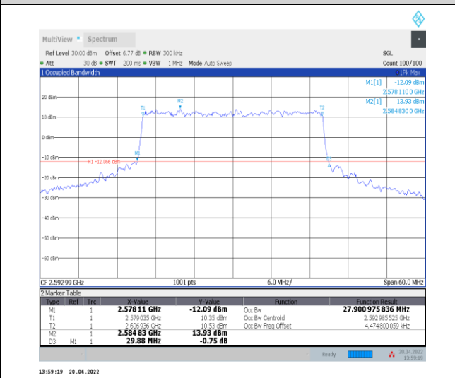
1-N41--30-30-M-8-CP-64QAM-Outer_Full-78@0-Ant 0-27.901-29.880-≤30-PASS
