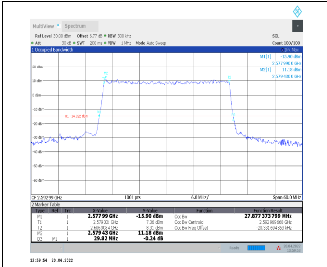
1-N41--30-30-M-9-CP-256QAM-Outer_Full-78@0-An t0-27.877-29.820-<=30-PASS
