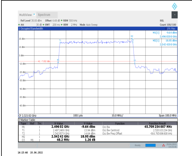
1-N41--30-50-L-2-DFT-PI2BPSK-Outer_Full-128@0-A Ant0-45.709-48.200-≤50-PASS
