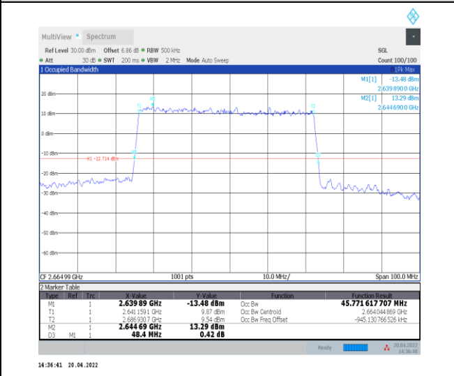
1-N41--30-50-H-5-DFT-256QAM-Outer_Full-128@0-A Ant0-45.772-48.400-≤50-PASS
