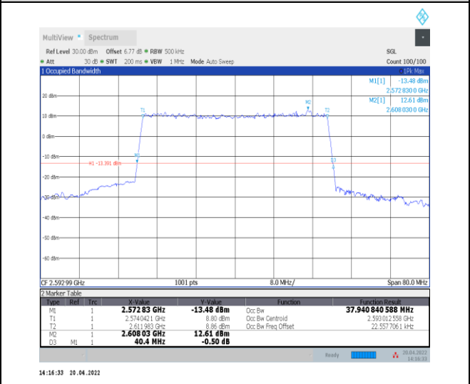
1-N41--30-40-M-9-CP-256QAM-Outer_Full-106@0-Ant 0-37.941-40.400-≤40-PASS
