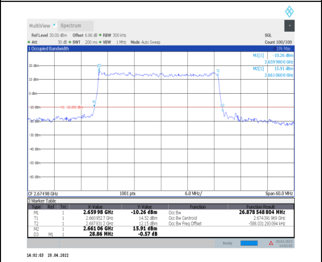
1-N41--30-30-H-3-DFT-16QAM-Outer_Full-75@0-An t0-26.879-28.860-<=30-PASS
