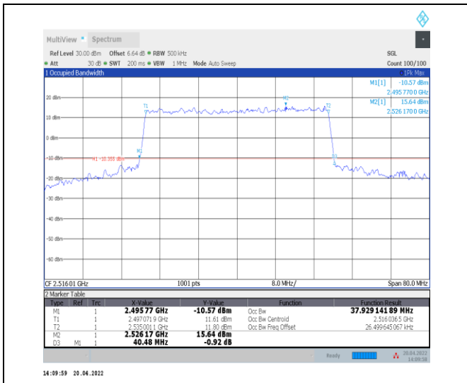
1-N41--30-40-L-7-CP-16QAM-Outer_Full-106@0-Ant 0-37.929-40.480-≤40-PASS
