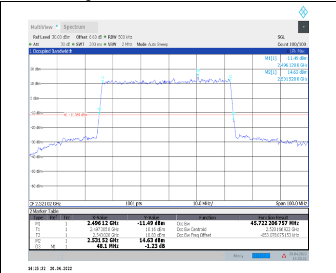
1-N41--30-50-L-5-DFT-256QAM-Outer_Full-128@0-A Ant0-45.722-48.100-≤50-PASS
