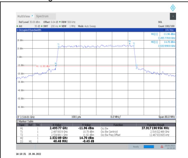
1-N41--30-40-L-8-CP-64QAM-Outer_Full-106@0-An t0-37.917-40.480-≤40-PASS
