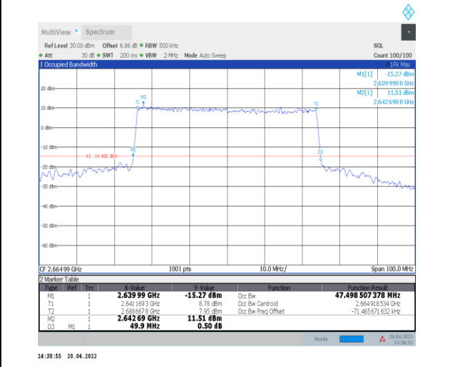
1-N41--30-50-H-9-CP-256QAM-Outer_Full-133@0-Ant t0-47.499-49.900-≤50-PASS
