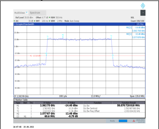
1-N41--30-60-M-5-DFT-256QAM-Outer_Full-162@0-A Ant0-58.071-60.600-≤60-PASS
