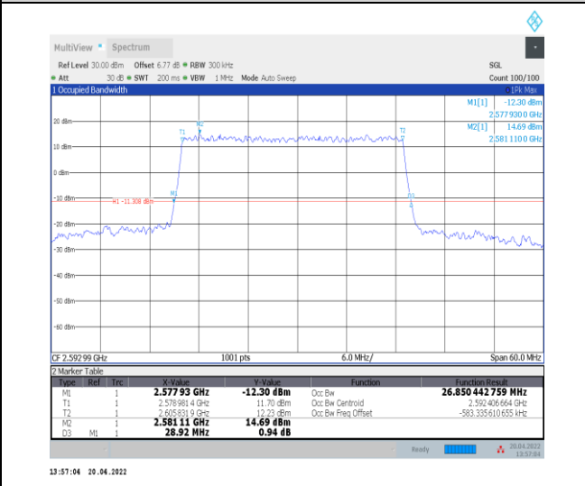
1-N41--30-30-M-4-DFT-64QAM-Outer_Full-75@0-Ant 0-26.85-28.920-≤30-PASS
