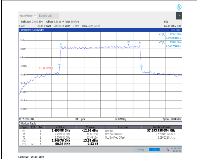
1-N41--30-60-L-7-CP-16QAM-Outer_Full-162@0-Ant0-57.894-60.360-≤60-PASS
