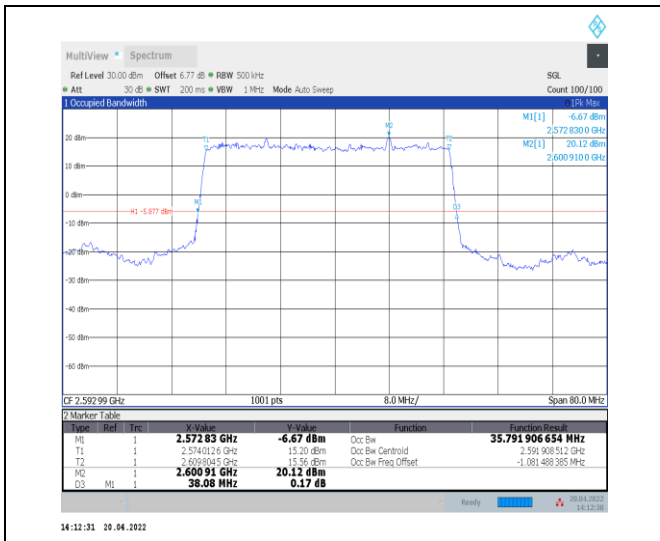
1-N41--30-40-M-2-DFT-PI2BPSK-Outer_Full-100@0-Ant0-35.792-38.080-≤40-PASS
