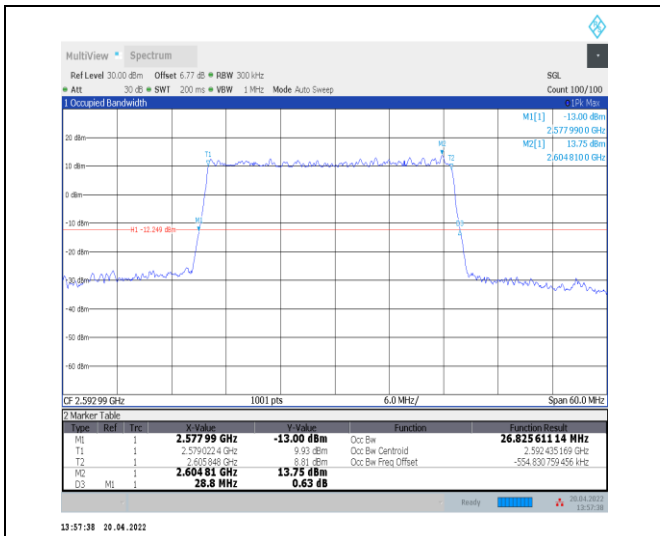
1-N41--30-30-M-5-DFT-256QAM-Outer_Full-75@0-A nt0-26.826-28.800-≤30-PASS
