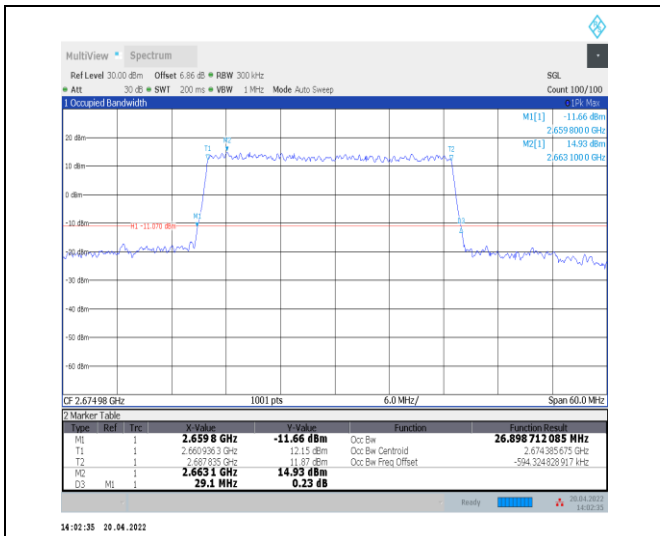
1-N41--30-30-H-4-DFT-64QAM-Outer_Full-75@0-Ant t0-26.899-29.100-<30-PASS
