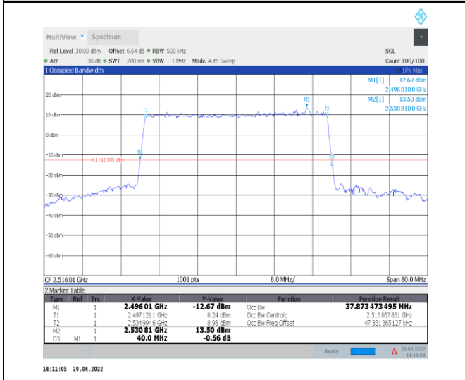
1-N41--30-40-L-9-CP-256QAM-Outer_Full-106@0-A nt0-37.873-40.000-≤40-PASS
