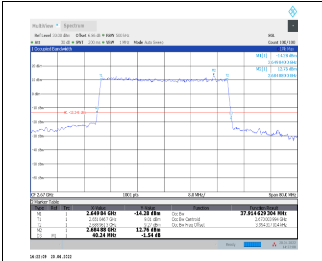
1-N41--30-40-H-9-CP-256QAM-Outer_Full-106@0-A nt0-37.915-40.240-≤40-PASS
