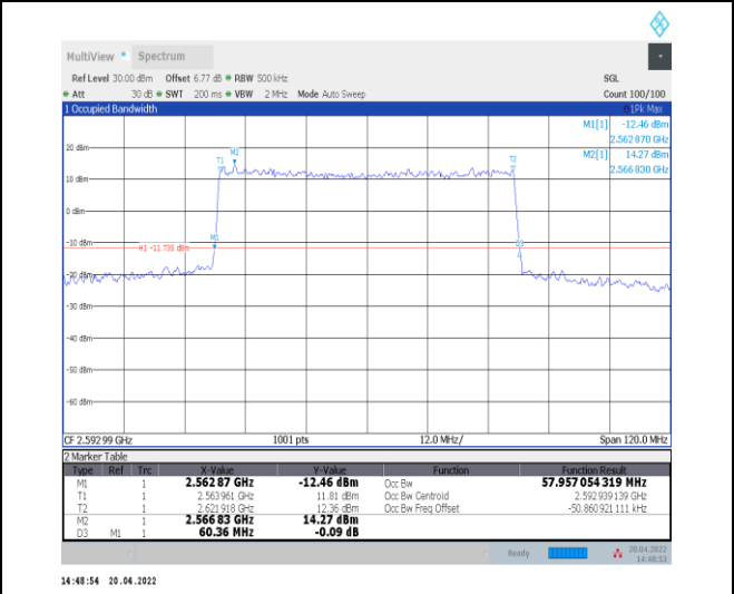
1-N41--30-60-M-7-CP-16QAM-Outer_Full-162@0-A nt0-57.957-60.360-≤60-PASS
