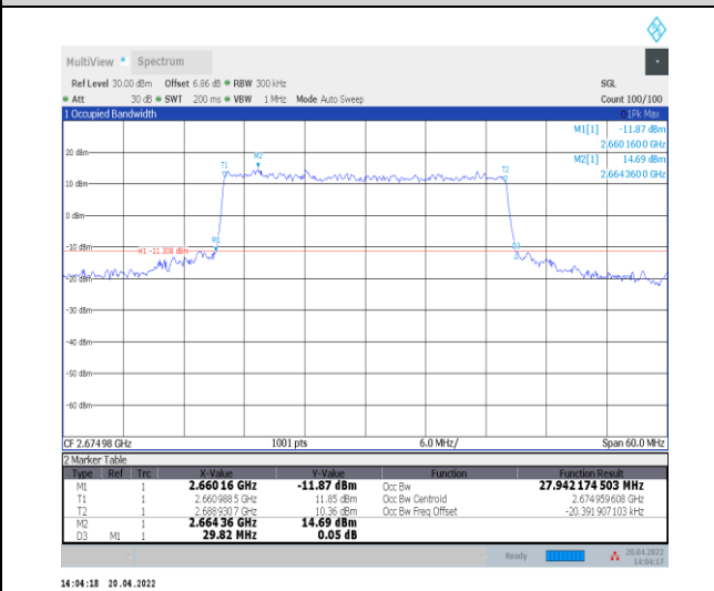
1-N41--30-30-H-7-CP-16QAM-Outer_Full-78@0-Ant 0-27.942-29.820-<30-PASS
