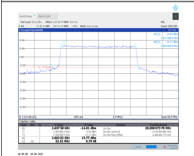
1-N41--30-30-H-6-CP-QPSK-Outer_Full-78@0-Ant 28.008-32.520-<30-PASS
