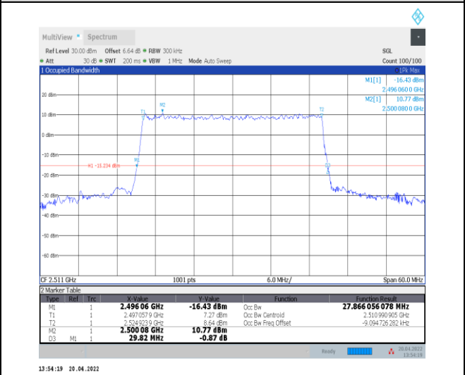
1-N41--30-30-L-9-CP-256QAM-Outer_Full-78@0-Ant0-27.866-29.820-<=30-PASS
