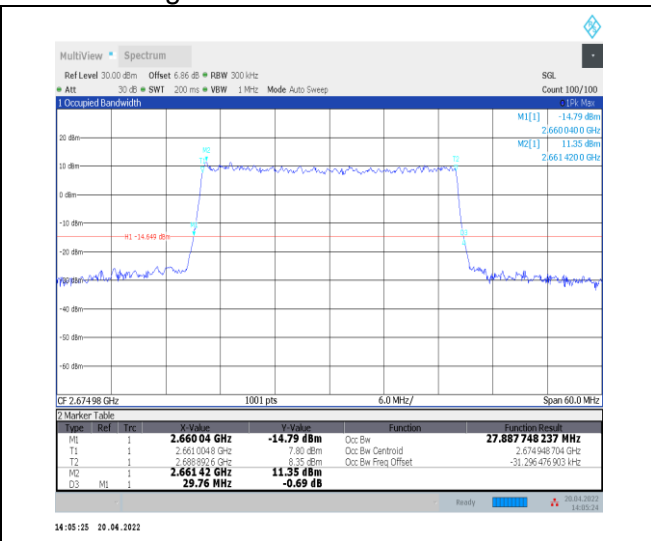
1-N41--30-30-H-9-CP-256QAM-Outer_Full-78@0-Ant 0-27.888-29.760-≤30-PASS
