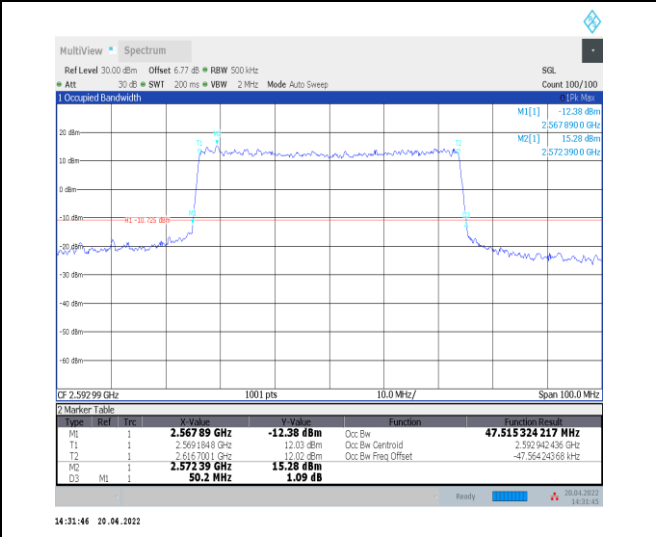
1-N41--30-50-M-6-CP-QPSK-Outer_Full-133@0-Ant 0-47.515-50.200-≤50-PASS
