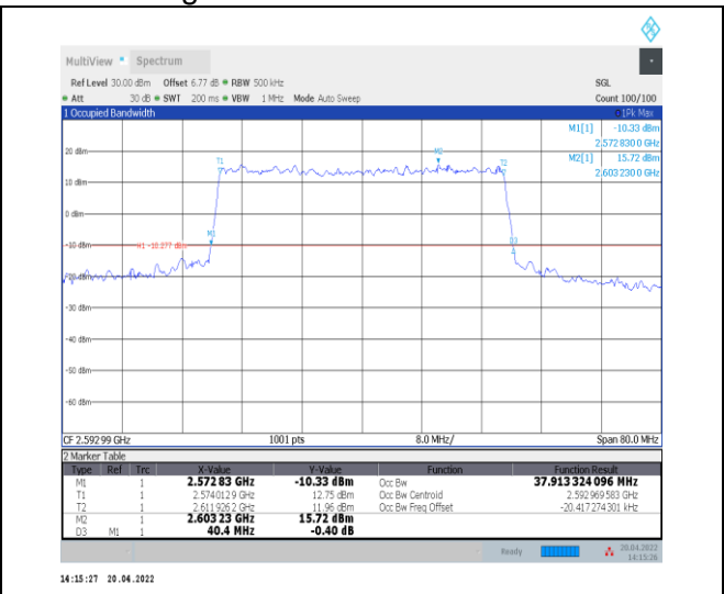
1-N41--30-40-M-7-CP-16QAM-Outer_Full-106@0-Ant nt0-37.913-40.400-≤40-PASS
