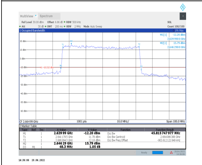
1-N41--30-50-H-4-DFT-64QAM-Outer_Full-128@0-A nt0-45.816-48.300-≤50-PASS
