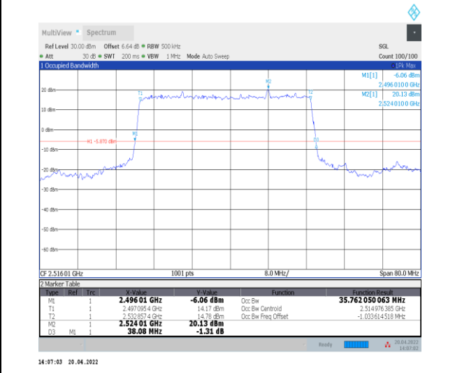
1-N41--30-40-L-2-DFT-PI2BPSK-Outer_Full-100@0-Ant 0-35.762-38.080-≤40-PASS
