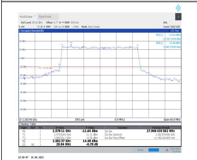
1-N41--30-30-M-7-CP-16QAM-Outer_Full-78@0-Ant 0-27.906-29.940-≤30-PASS
