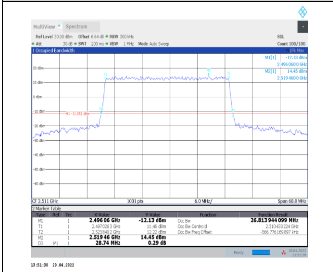
1-N41--30-30-L-4-DFT-64QAM-Outer_Full-75@0-Ant 0-26.814-28.740-≤30-PASS
