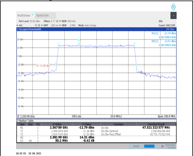
1-N41--30-50-M-8-CP-64QAM-Outer_Full-133@0-A nt0-47.521-50.200-<=50-PASS
