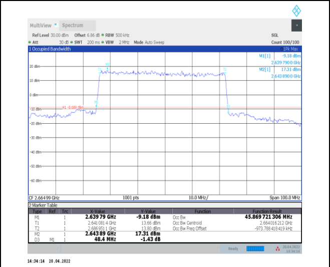
1-N41--30-50-H-1-DFT-QPSK-Outer_Full-128@0-An t0-45.87-48.400-<=50-PASS
