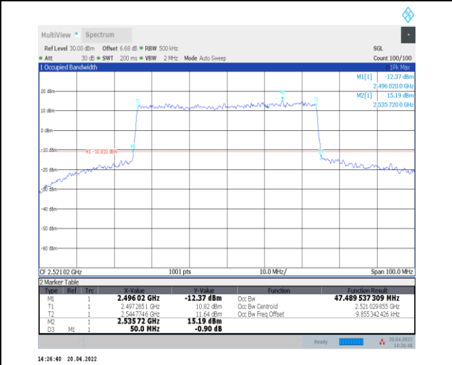
1-N41--30-50-L-7-CP-16QAM-Outer_Full-133@0-Ant0 t0-47.49-50.000-≤50-PASS
