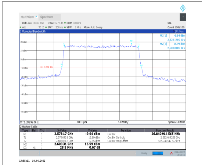
1-N41--30-30-M-1-DFT-QPSK-Outer_Full-75@0-Ant 0-26.841-28.800-≤30-PASS
