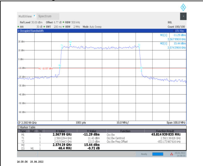
1-N41--30-50-M-4-DFT-64QAM-Outer_Full-128@0-A Ant0-45.815-48.400-≤50-PASS
