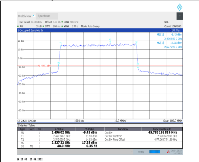
1-N41--30-50-L-1-DFT-QPSK-Outer_Full-128@0-Ant 0-45.793-48.000-≤50-PASS
