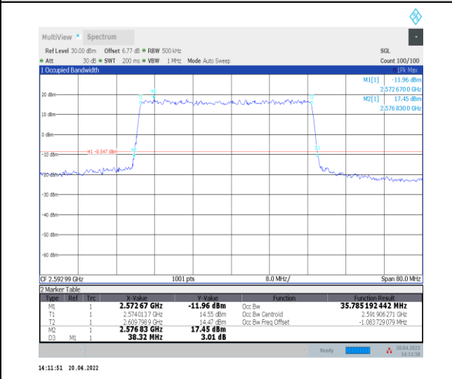
1-N41--30-40-M-1-DFT-QPSK-Outer_Full-100@0-An t0-35.785-38.320-≤40-PASS
