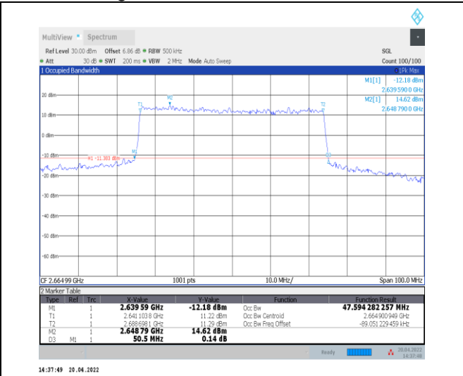
1-N41--30-50-H-7-CP-16QAM-Outer_Full-133@0-Ant t0-47.594-50.500-≤50-PASS
