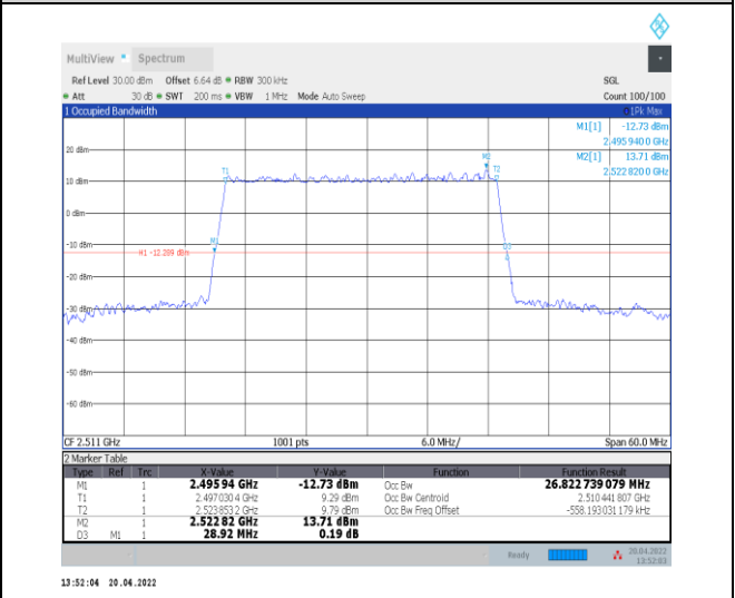
1-N41--30-30-L-5-DFT-256QAM-Outer_Full-75@0-A nt0-26.823-28.920-≤30-PASS
