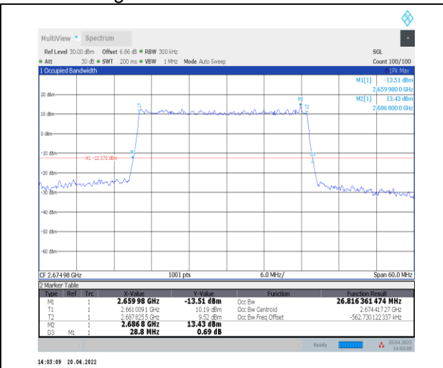
1-N41--30-30-H-5-DFT-256QAM-Outer_Full-75@0-Ant nt0-26.816-28.800-<30-PASS
