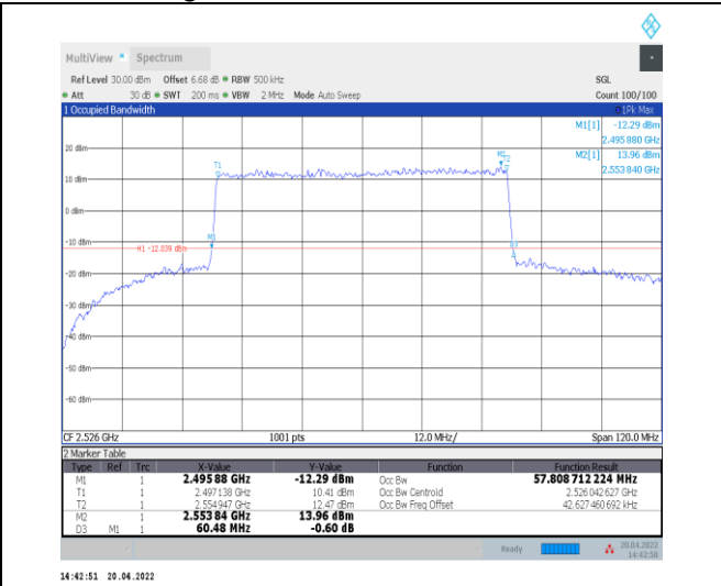
1-N41--30-60-L-6-CP-QPSK-Outer_Full-162@0-Ant0-57.809-60.480-≤60-PASS
