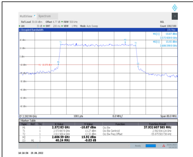
1-N41--30-40-M-6-CP-QPSK-Outer_Full-106@0-Ant 0-37.933-40.240-≤40-PASS
