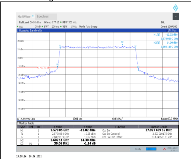
1-N41--30-30-M-6-CP-QPSK-Outer_Full-78@0-Ant0 -27.927-30.060-≤30-PASS
