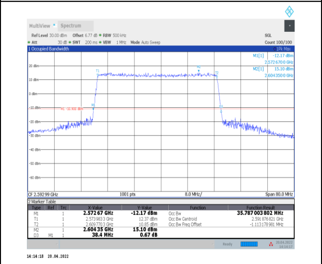
1-N41--30-40-M-5-DFT-256QAM-Outer_Full-100@0-Ant0-35.787-38.400-≤40-PASS
