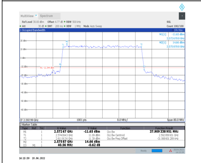
1-N41--30-40-M-8-CP-64QAM-Outer_Full-106@0-Ant t0-37.909-40.560-≤40-PASS
