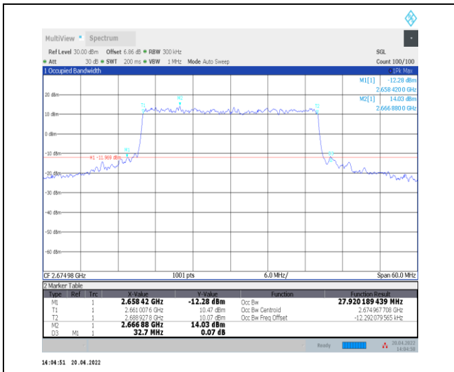
1-N41--30-30-H-8-CP-64QAM-Outer_Full-78@0-Ant 0-27.92-32.700-≤30-PASS
