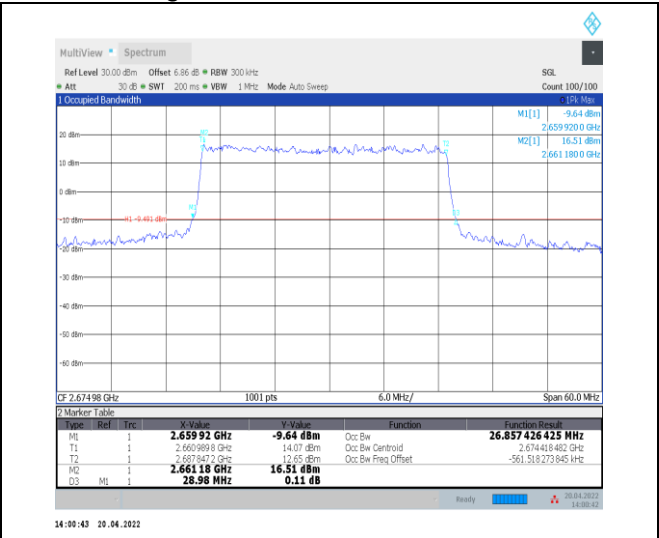
1-N41--30-30-H-1-DFT-QPSK-Outer_Full-75@0-Ant 0-26.857-28.980-<=30-PASS
