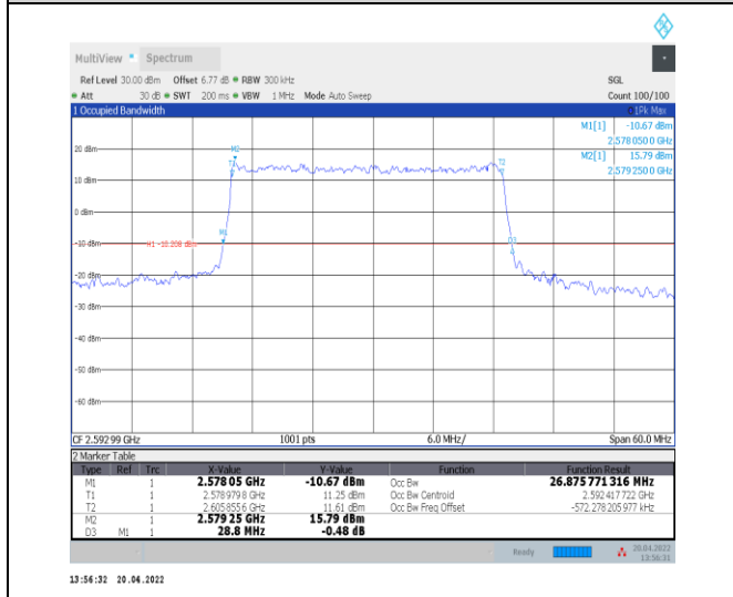
1-N41--30-30-M-3-DFT-16QAM-Outer_Full-75@0-Ant 0-26.876-28.800-≤30-PASS
