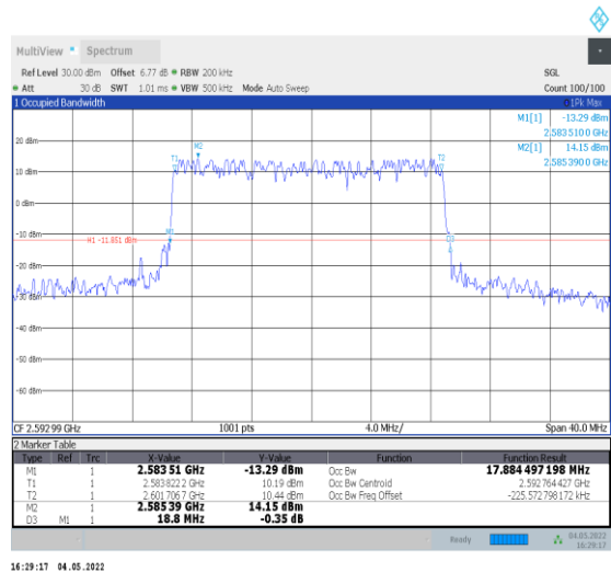
1-N41--30-20-M-3-DFT-16QAM-Outer_Full-50@0-Ant 0-17.884-18.800-≤20-PASS
