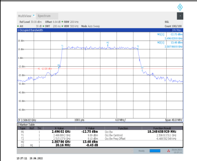
1-N41--30-20-L-8-CP-64QAM-Outer_Full-51@0-Ant 0-18.249-20.160-≤20-PASS
