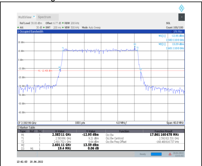
1-N41--30-20-M-5-DFT-256QAM-Outer_Full-50@0-Ant0-17.861-19.400-≤20-PASS
