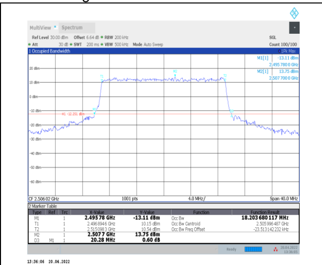
1-N41--30-20-L-6-CP-QPSK-Outer_Full-51@0-Ant0 18.204-20.280-≤20-PASS
