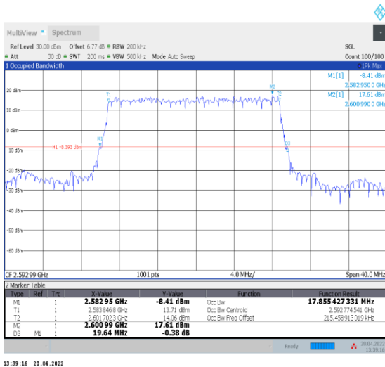
1-N41--30-20-M-2-DFT-PI2BPSK-Outer_Full-50@0-Ant 0-17.855-19.640-≤20-PASS
