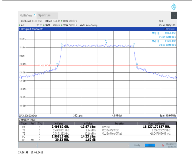
1-N41--30-20-L-7-CP-16QAM-Outer_Full-51@0-Ant0 -18.237-20.120-≤20-PASS
