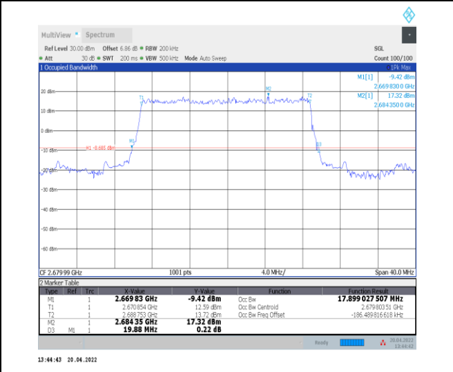
1-N41--30-20-H-2-DFT-PI2BPSK-Outer_Full-50@0-Ant 0-17.899-19.880-≤20-PASS
