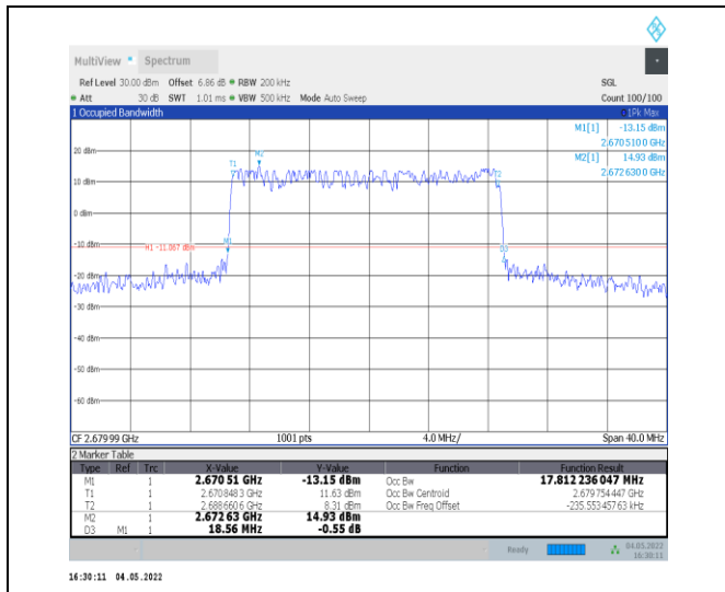
1-N41--30-20-H-3-DFT-16QAM-Outer_Full-50@0-An t0-17.812-18.560-<=20-PASS
