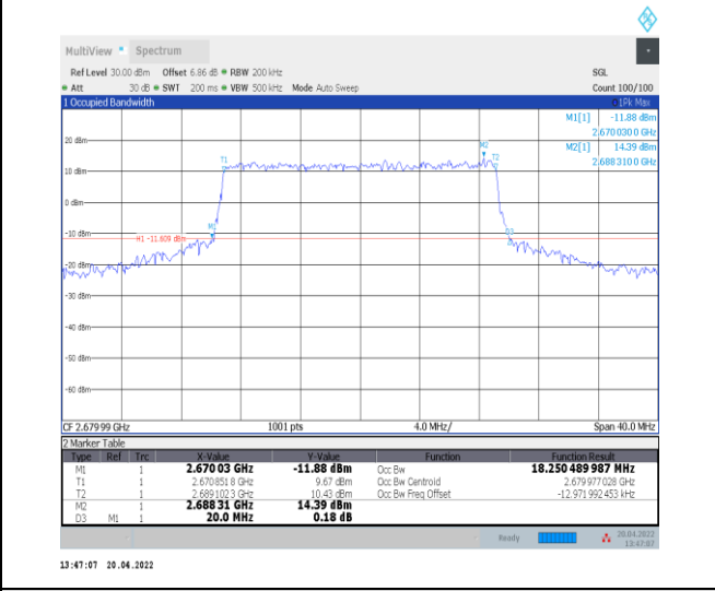
1-N41--30-20-H-6-CP-QPSK-Outer_Full-51@0-Ant0- 18.25-20.000-<=20-PASS
