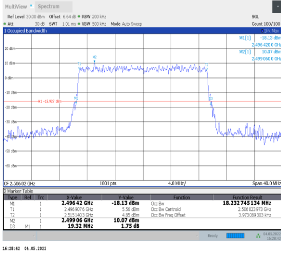
1-N41--30-20-L-9-CP-256QAM-Outer_Full-51@0-Ant 0-18.233-19.320-≤20-PASS
