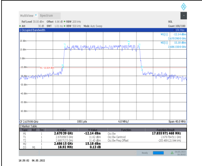
1-N41--30-20-H-1-DFT-QPSK-Outer_Full-50@0-Ant 0-17.856-18.920-≤20-PASS
