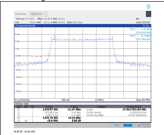
1-N41--30-20-H-4-DFT-64QAM-Outer_Full-50@0-An t0-17.915-19.600-<=20-PASS
