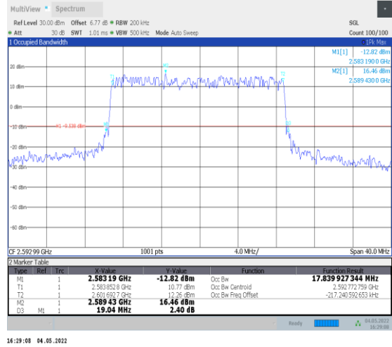
1-N41--30-20-M-1-DFT-QPSK-Outer_Full-50@0-Ant 0-17.84-19.040-≤20-PASS
