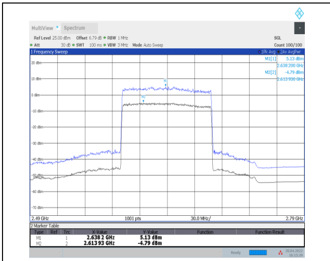
1-N41--30-100-H-1-DFT-256QAM-Outer_Full-270@ 0-Ant0-9.92-100%-0.00-9.92-PASS-≤13
