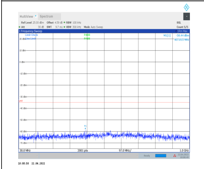
1-N38--30-40-H-1-DFT-PI2BPSK-Inner_1RB_Left-1 @ 1-30-1000-Ant0--58.44--35-PASS
