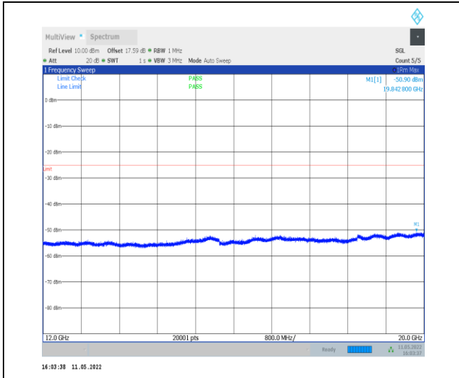
1-N38-PC2-30-40-L-1-DFT-QPSK-Edge_1RB_Left-1 @0-12000-20000-Ant0--50.90--25-PASS
