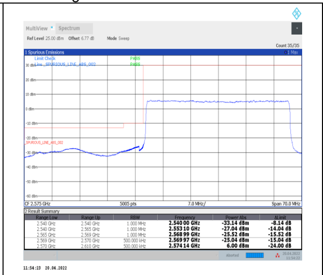
1-N38--30-40-L-3-DFT-PI2BPSK-Outer_Full-100@0-Ant0-PASS-see graph
