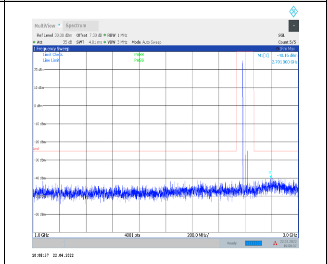
1-N38--30-40-H-1-DFT-PI2BPSK-Inner_1RB_Left-1 @ 1-1000-3000-Ant0--40.16--25-PASS
