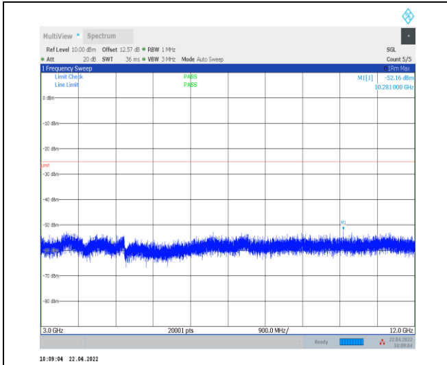
1-N38--30-40-H-1-DFT-PI2BPSK-Inner_1RB_Left-1 @ 1-3000-12000-Ant0--52.16--25-PASS
