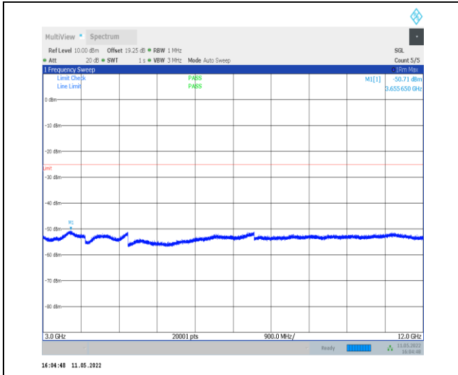
1-N38-PC2-30-40-M-1-DFT-QPSK-Edge_1RB_Left-1 @ 0-3000-12000-Ant0--50.71--25-PASS
