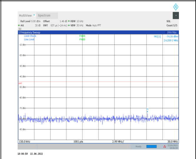
1-N38--30-40-M-1-DFT-PI2BPSK-Inner_1RB_Left-1 @ 1-0.15-30-Ant0--74.16--45-PASS
