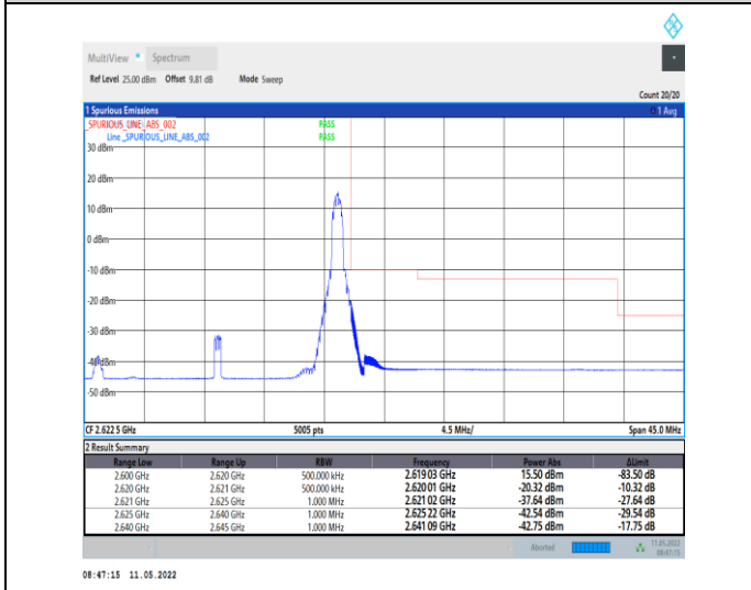
1-N38-PC2-30-20-H-5-CP-QPSK-Edge_1RB_Right-1@50-Ant0-PASS-see graph
