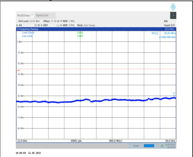
1-N38-PC2-30-40-M-1-DFT-QPSK-Edge_1RB_Left-1 @ 0-12000-20000-Ant0--50.83--25-PASS
