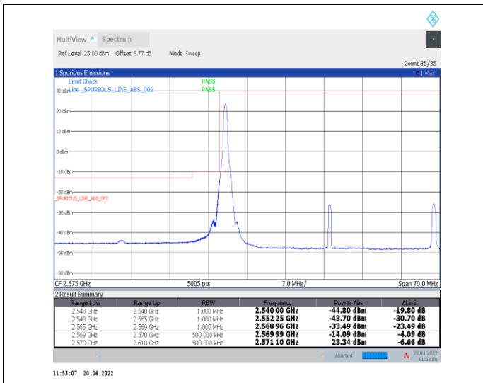
1-N38--30-40-L-1-DFT-PI2BPSK-Edge_1RB_Left-1@0-Ant0-PASS-see graph
