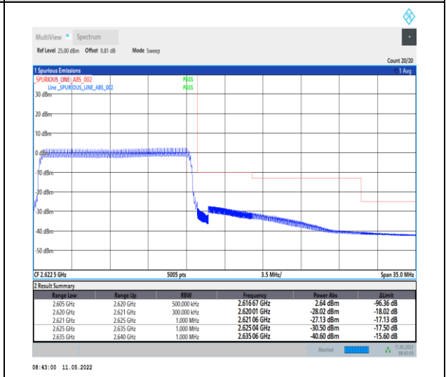
1-N38-PC2-30-15-H-6-CP-QPSK-Outer_Full-38@0-Ant0-PASS-see graph
