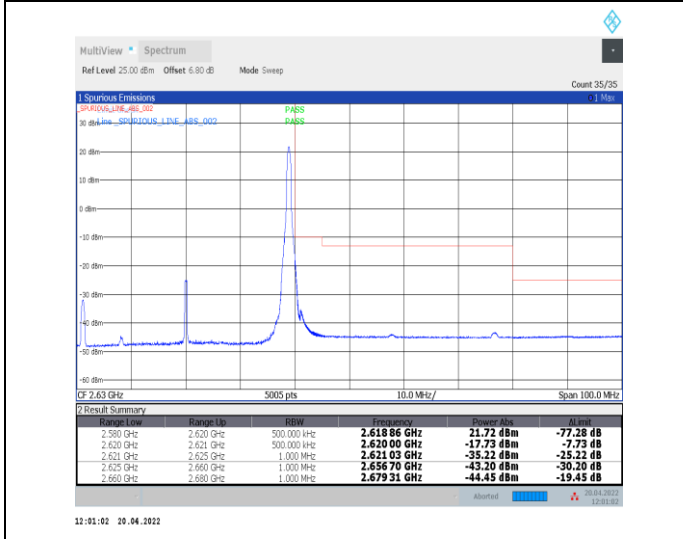
1-N38--30-40-H-5-CP-QPSK-Edge_1RB_Right-1@105-Ant0-PASS-see graph
