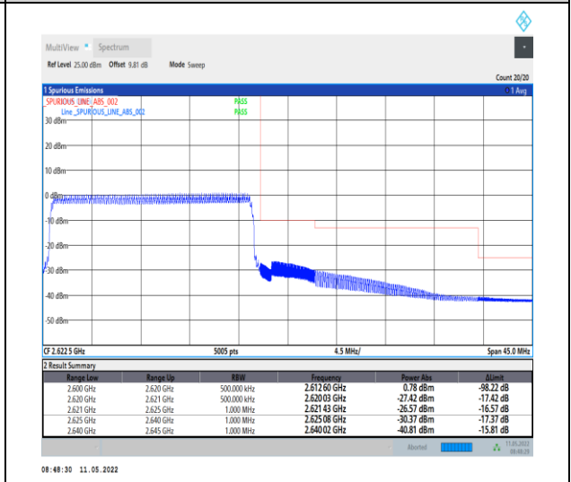
1-N38-PC2-30-20-H-6-CP-QPSK-Outer_Full-51@0-Ant0-PASS-see graph
