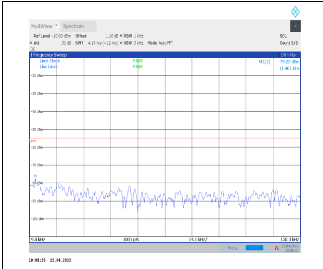
1-N38--30-40-H-1-DFT-PI2BPSK-Inner_1RB_Left-1 @ 1-0.009-0.15-Ant0--79.23--55-PASS
