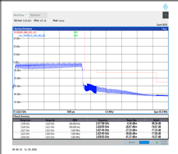
1-N38-PC2-30-30-H-6-CP-QPSK-Outer_Full-78@0-Ant0-PASS-see graph
