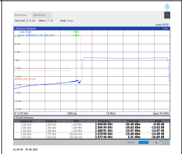
1-N38--30-40-L-6-CP-QPSK-Outer_Full-106@0-Ant0-PASS-see graph
