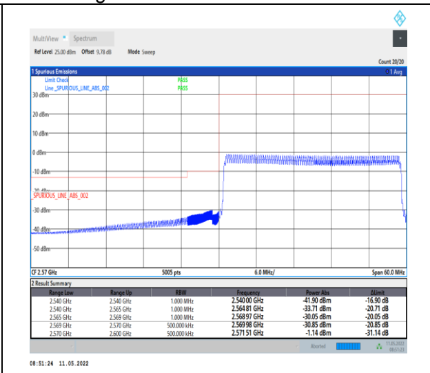
1-N38-PC2-30-30-L-6-CP-QPSK-Outer_Full-78@0-Ant0-PASS-see graph
