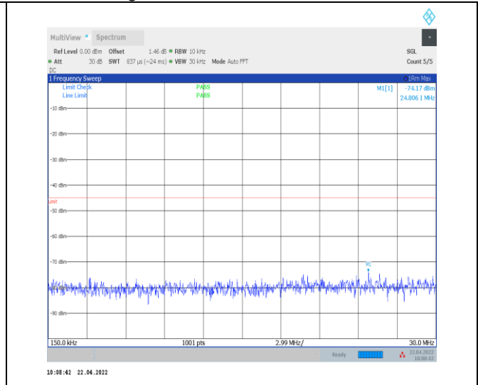
1-N38--30-40-H-1-DFT-PI2BPSK-Inner_1RB_Left-1 @ 1-0.15-30-Ant0--74.17--45-PASS
