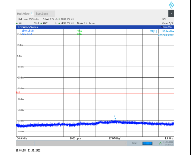
1-N38-PC2-30-40-H-1-DFT-QPSK-Edge_1RB_Left-1 @ 0-30-1000-Ant0--59.26--35-PASS
