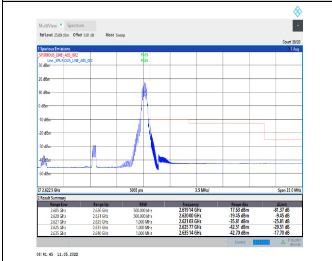
1-N38-PC2-30-15-H-5-CP-QPSK-Edge_1RB_Right-1@37-Ant0-PASS-see graph
