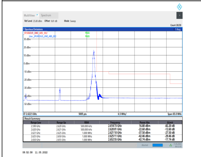
1-N38-PC2-30-30-H-5-CP-QPSK-Edge_1RB_Right-1@77-Ant0-PASS-see graph
