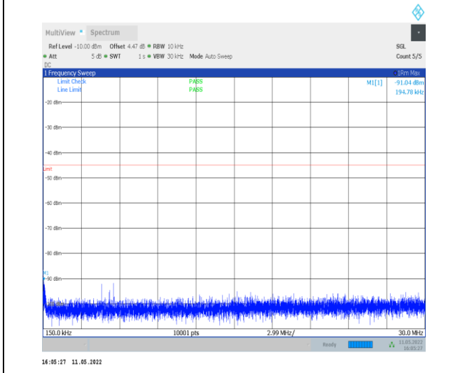
1-N38-PC2-30-40-H-1-DFT-QPSK-Edge_1RB_Left-1 @ 0-0.15-30-Ant0--91.04--45-PASS
