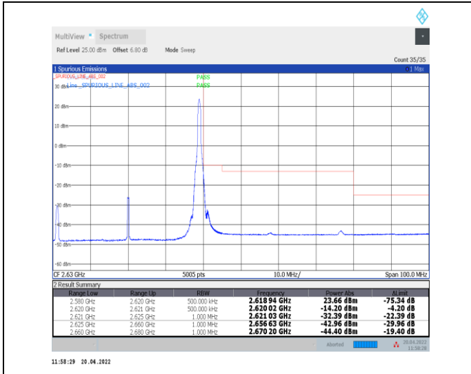
1-N38--30-40-H-2-DFT-PI2BPSK-Edge_1RB_Right-1@105-Ant0-PASS-see graph
