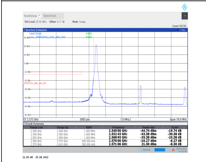
1-N38--30-40-L-4-CP-QPSK-Edge_1RB_Left-1@0-Ant0-PASS-see graph
