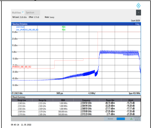
1-N38-PC2-30-15-L-6-CP-QPSK-Outer_Full-38@0-Ant0-PASS-see graph
