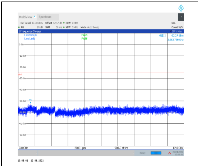
1-N38--30-40-L-1-DFT-PI2BPSK-Inner_1RB_Left-1 @ 1-3000-12000-Ant0--52.27--25-PASS
