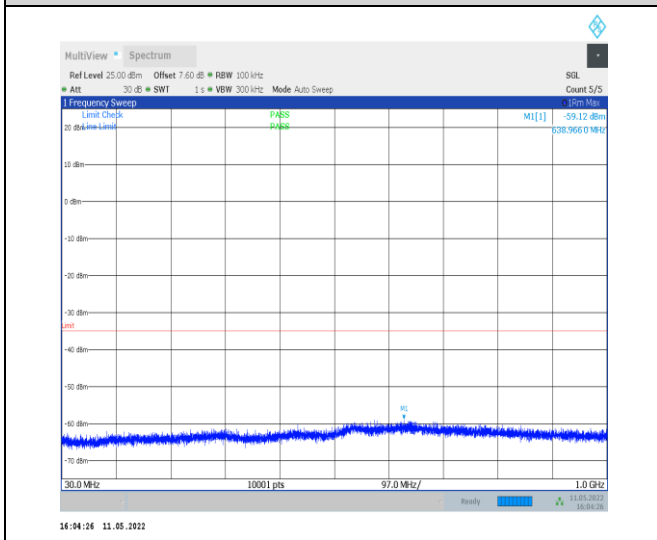
1-N38-PC2-30-40-M-1-DFT-QPSK-Edge_1RB_Left-1 @0-30-1000-Ant0--59.12--35-PASS
