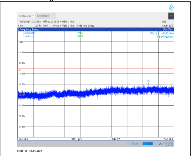
1-N38--30-40-L-1-DFT-PI2BPSK-Inner_1RB_Left-1 @ 1-12000-27000-Ant0--40.23--25-PASS
