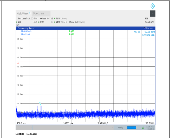
1-N38-PC2-30-40-M-1-DFT-QPSK-Edge_1RB_Left-1 @0-0.15-30-Ant0--92.36--45-PASS
