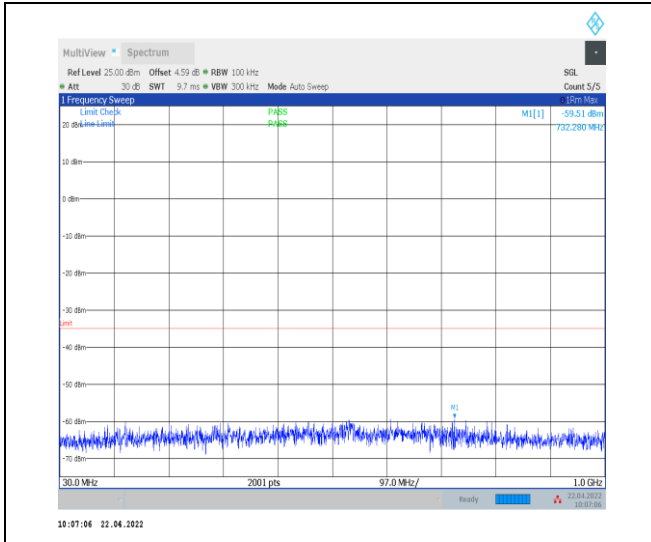
1-N38--30-40-M-1-DFT-PI2BPSK-Inner_1RB_Left-1 @ 1-30-1000-Ant0--59.51--35-PASS
