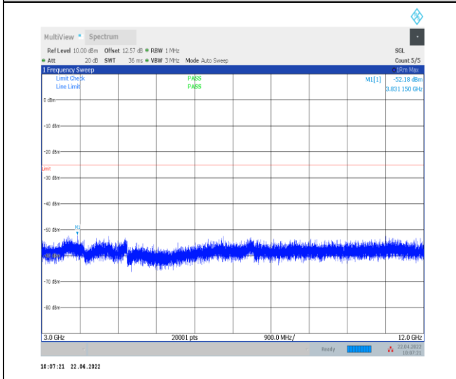
1-N38--30-40-M-1-DFT-PI2BPSK-Inner_1RB_Left-1 @ 1-3000-12000-Ant0--52.18--25-PASS
