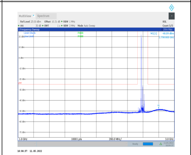
1-N38-PC2-30-40-M-1-DFT-QPSK-Edge_1RB_Left-1 @0-1000-3000-Ant0--48.09--25-PASS
