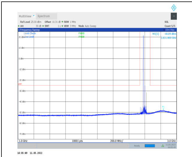
1-N38-PC2-30-40-H-1-DFT-QPSK-Edge_1RB_Left-1 @0-1000-3000-Ant0--48.09--25-PASS
