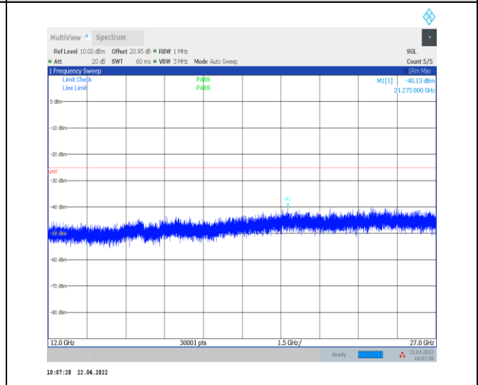
1-N38--30-40-M-1-DFT-PI2BPSK-Inner_1RB_Left-1 @ 1-12000-27000-Ant0--40.13--25-PASS
