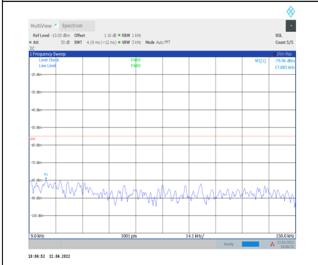
1-N38--30-40-M-1-DFT-PI2BPSK-Inner_1RB_Left-1 @ 1-0.009-0.15-Ant0--79.96--55-PASS
