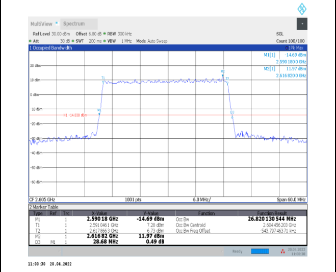
1-N38--30-30-H-5-DFT-256QAM-Outer_Full-75@0-A nt0-26.82-28.680-≤30-PASS
