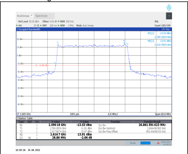
1-N38--30-30-H-3-DFT-16QAM-Outer_Full-75@0-An t0-26.862-28.860-≤30-PASS
