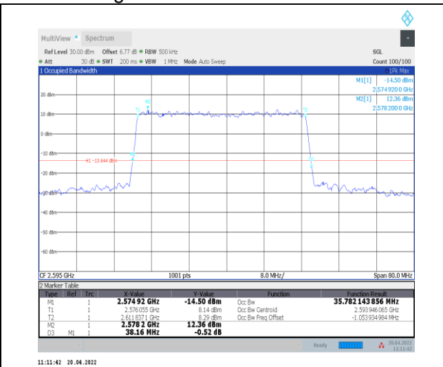
1-N38--30-40-M-5-DFT-256QAM-Outer_Full-100@0-A Ant0-35.782-38.160-≤40-PASS
