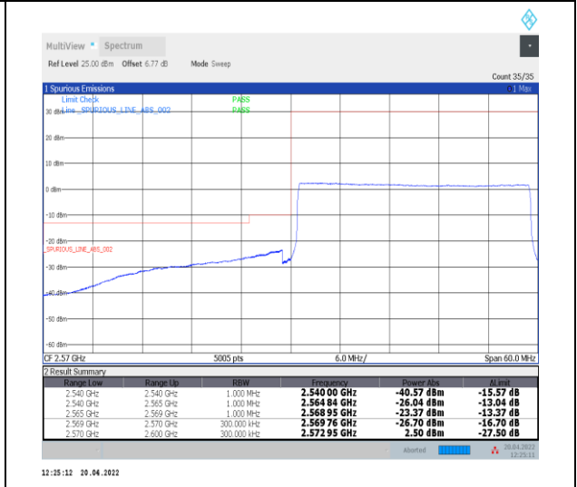
1-N38--30-30-L-6-CP-QPSK-Outer_Full-78@0-Ant0-PASS-see graph
