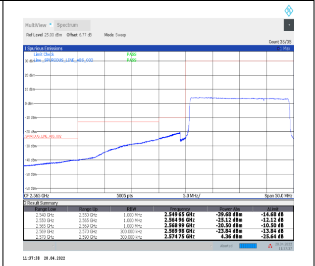
1-N38--30-20-L-6-CP-QPSK-Outer_Full-51@0-Ant0-PASS-see graph
