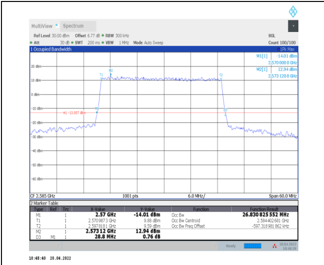
1-N38--30-30-L-4-DFT-64QAM-Outer_Full-75@0-Ant 0-26.831-28.800-≤30-PASS
