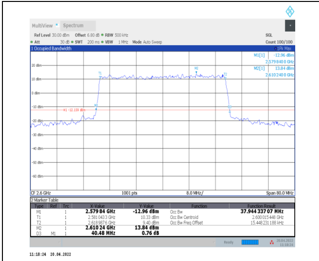
1-N38--30-40-H-7-CP-16QAM-Outer_Full-106@0-An t0-37.944-40.480-<math>\leq 40</math>-PASS
