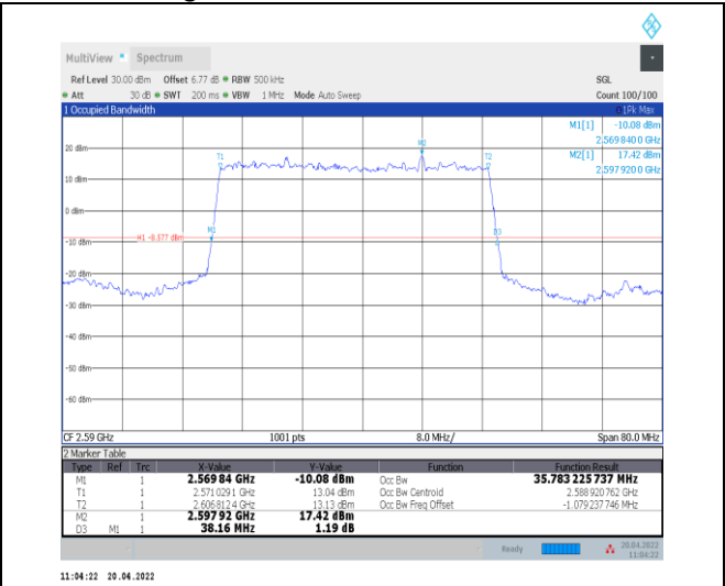
1-N38--30-40-L-2-DFT-PI2BPSK-Outer_Full-100@0-Ant 0-35.783-38.160-≤40-PASS
