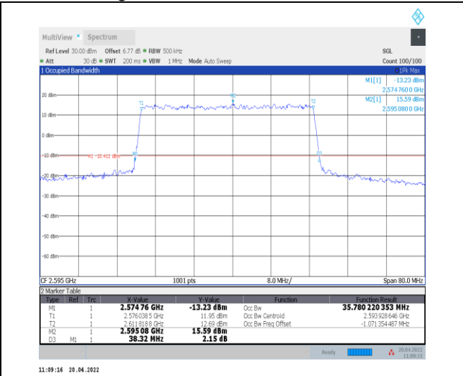
1-N38--30-40-M-1-DFT-QPSK-Outer_Full-100@0-A t0-35.78-38.320-<math>\leq 40</math>-PASS
