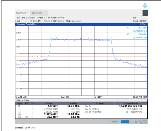
1-N38--30-20-L-7-CP-16QAM-Outer_Full-51@0-Ant0 -18.236-20.000-≤20-PASS
