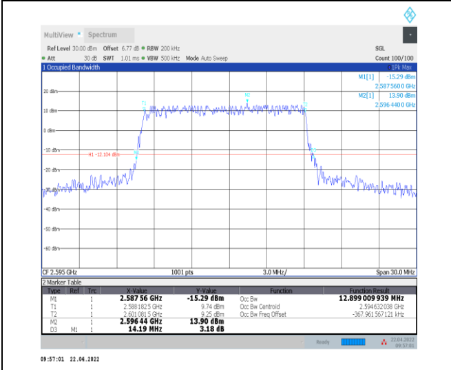
1-N38--30-15-M-3-DFT-16QAM-Outer_Full-36@0-Ant 0-12.899-14.190≤15-PASS
