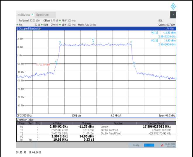
1-N38--30-20-M-1-DFT-QPSK-Outer_Full-50@0-Ant0 0-17.897-19.560-≤20-PASS
