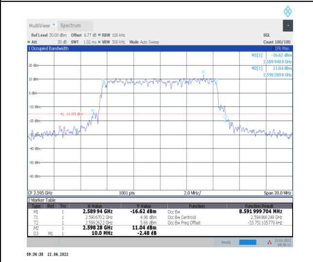
1-N38--30-10-M-3-DFT-16QAM-Outer_Full-24@0-Ant 0-8.592-10.000-≤10-PASS
