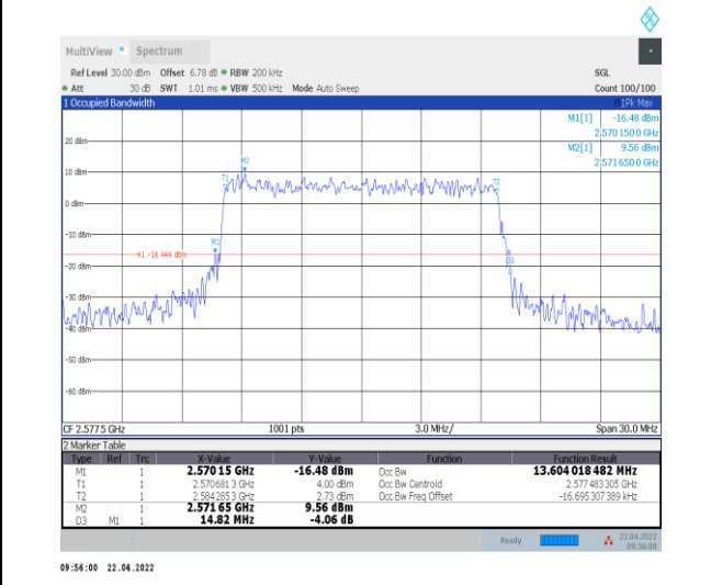
1-N38--30-15-L-9-CP-256QAM-Outer_Full-38@0-Ant0-13.604-14.820-≤15-PASS
