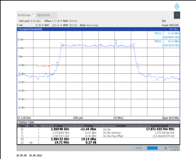
1-N38--30-20-L-2-DFT-PI2BPSK-Outer_Full-50@0-Ant0 -17.871-19.720≤20-PASS
