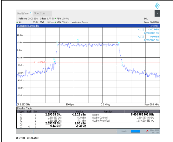
1-N38--30-10-M-6-CP-QPSK-Outer_Full-24@0-Ant 8.601-9.440≤10-PASS
