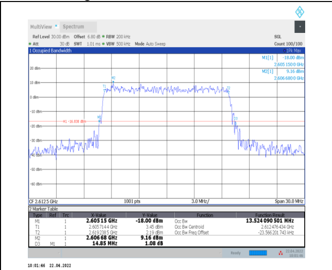
1-N38--30-15-H-9-CP-256QAM-Outer_Full-38@0-Ant 0-13.524-14.850≤15-PASS
