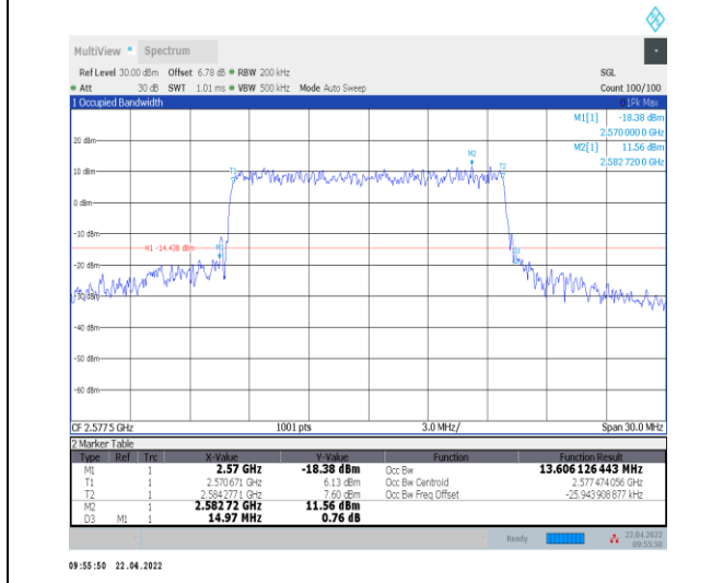
1-N38--30-15-L-8-CP-64QAM-Outer_Full-38@0-Ant0-13.606-14.970-≤15-PASS
