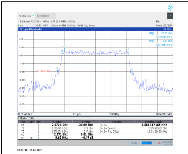
1-N38--30-10-L-9-CP-256QAM-Outer_Full-24@0-Ant 0-8.583-9.620-≤10-PASS
