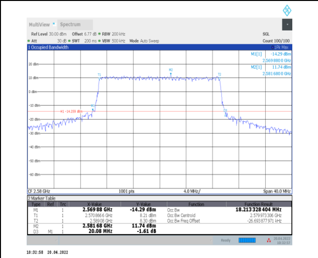
1-N38--30-20-L-6-CP-QPSK-Outer_Full-51@0-Ant 0-18.213-20.080-≤20-PASS
