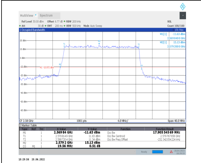
1-N38--30-20-L-1-DFT-QPSK-Outer_Full-50@0-Ant0 -17.906-19.560≤20-PASS
