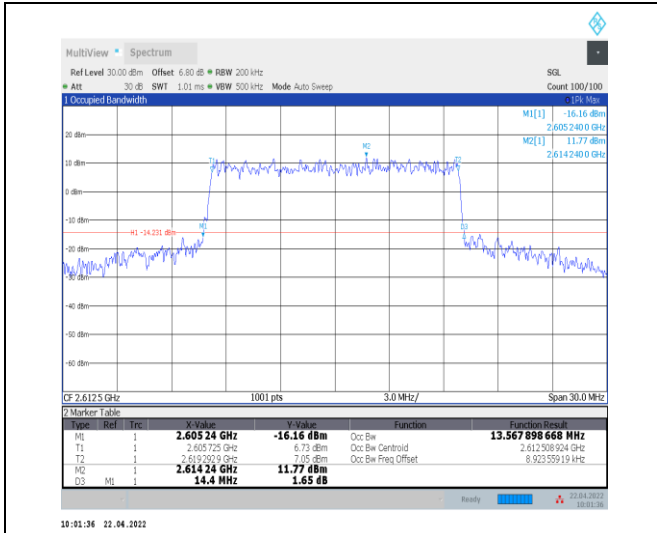
1-N38--30-15-H-8-CP-64QAM-Outer_Full-38@0-Ant 0-13.568-14.400≤15-PASS
