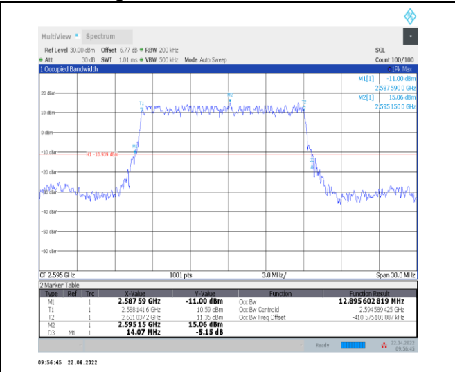
1-N38--30-15-M-2-DFT-PI2BPSK-Outer_Full-36@0-Ant 0-12.896-14.070≤15-PASS
