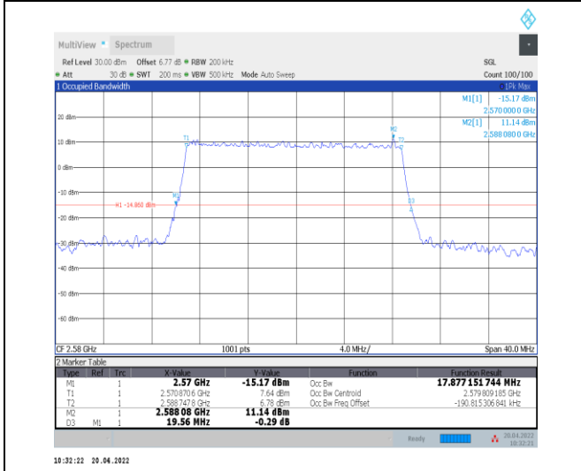
1-N38--30-20-L-5-DFT-256QAM-Outer_Full-50@0-Ant nt0-17.877-19.560-≤20-PASS
