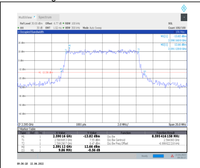
1-N38--30-10-M-1-DFT-QPSK-Outer_Full-24@0-Ant 0-8.595-9.860-≤10-PASS
