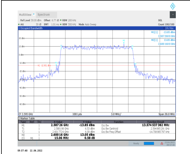
1-N38--30-15-M-7-CP-16QAM-Outer_Full-38@0-Ant 0-13.575-15.060-≤15-PASS
