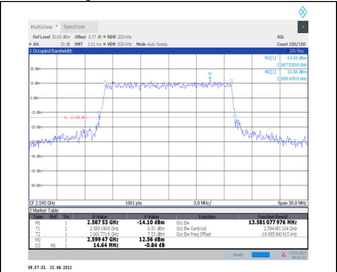
1-N38--30-15-M-6-CP-QPSK-Outer_Full-38@0-Ant0 -13.581-14.640-≤15-PASS
