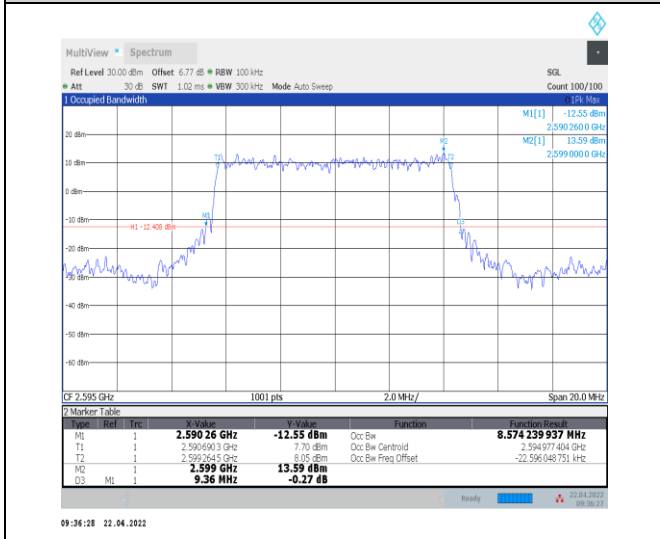
1-N38--30-10-M-2-DFT-PI2BPSK-Outer_Full-24@0-Ant 0-8.574-9.360-≤10-PASS
