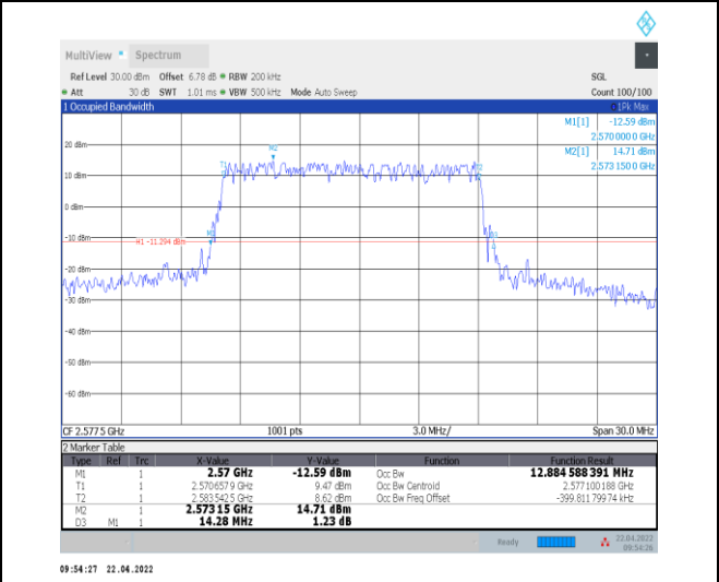
1-N38--30-15-L-1-DFT-QPSK-Outer_Full-36@0-Ant0 -12.885-14.280-≤15-PASS
