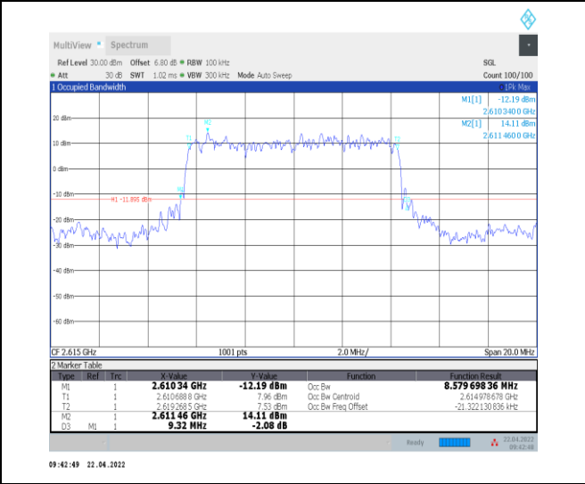
1-N38--30-10-H-2-DFT-PI2BPSK-Outer_Full-24@0-Ant 0-8.58-9.320-≤10-PASS
