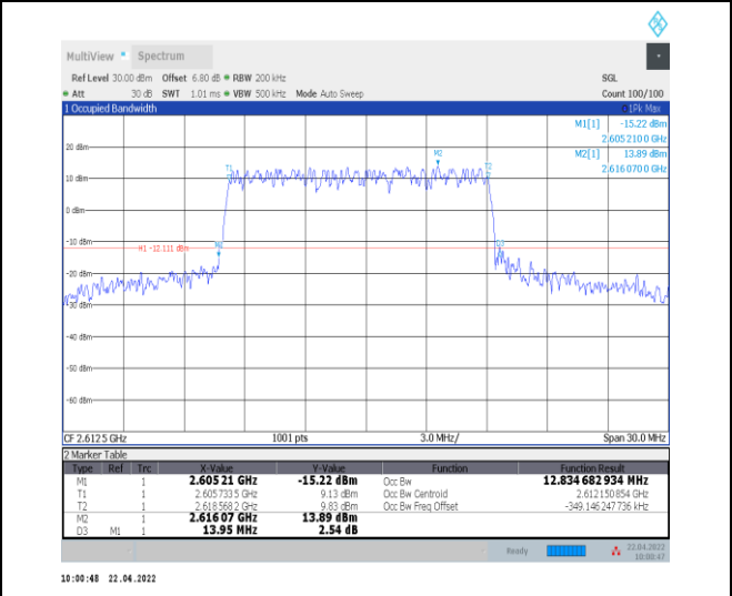
1-N38--30-15-H-3-DFT-16QAM-Outer_Full-36@0-An t0-12.835-13.950-≤15-PASS
