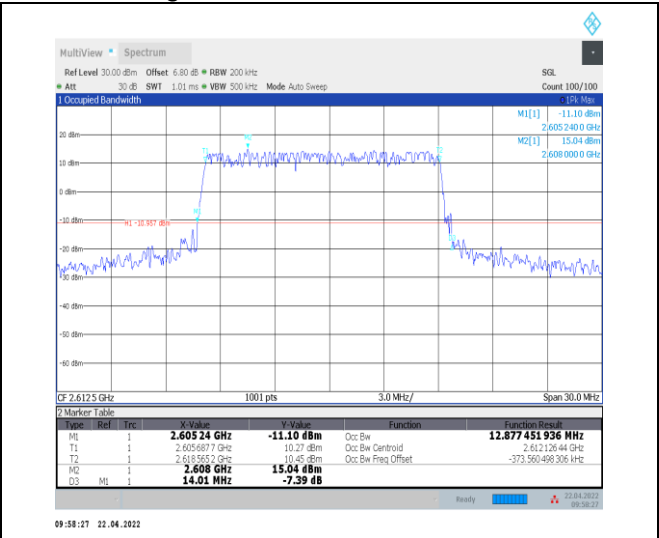
1-N38--30-15-H-1-DFT-QPSK-Outer_Full-36@0-Ant 0-12.877-14.010-≤15-PASS
