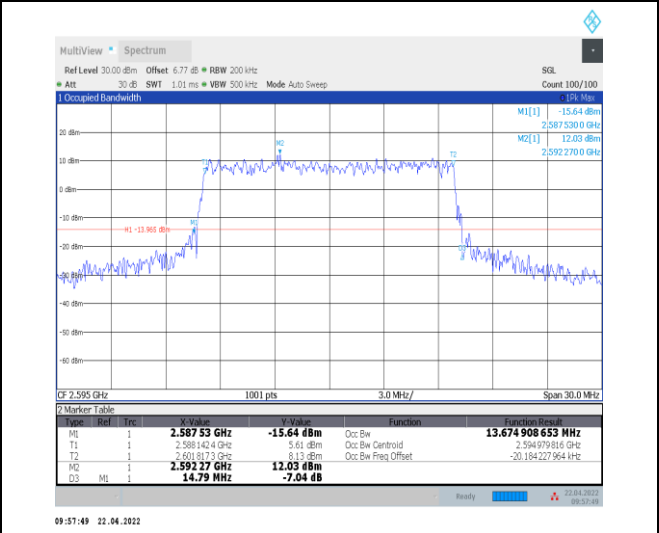
1-N38--30-15-M-8-CP-64QAM-Outer_Full-38@0-Ant 0-13.675-14.790-≤15-PASS
