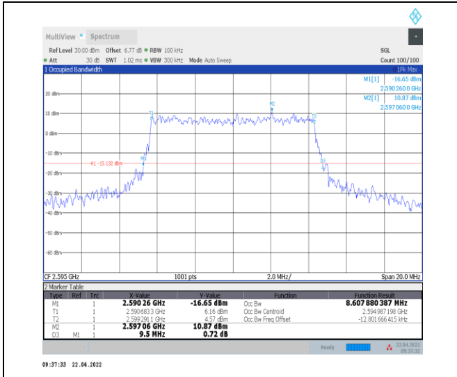
1-N38--30-10-M-8-CP-64QAM-Outer_Full-24@0-Ant 0-8.608-9.500-≤10-PASS
