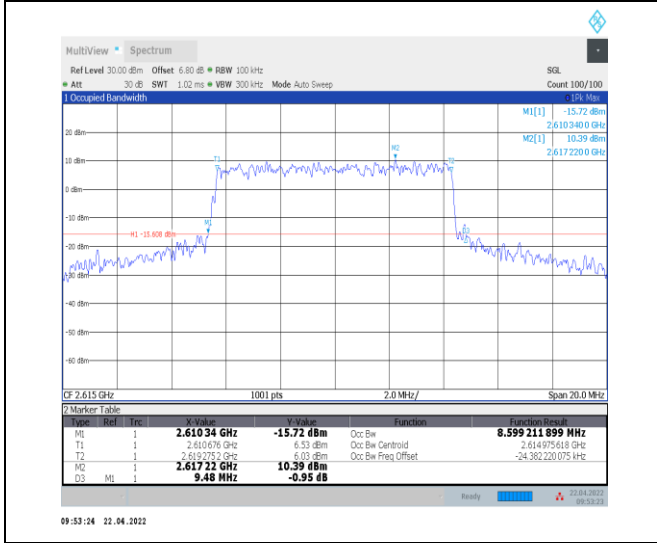
1-N38--30-10-H-1-DFT-QPSK-Outer_Full-24@0-Ant 0-8.599-9.480-≤10-PASS
