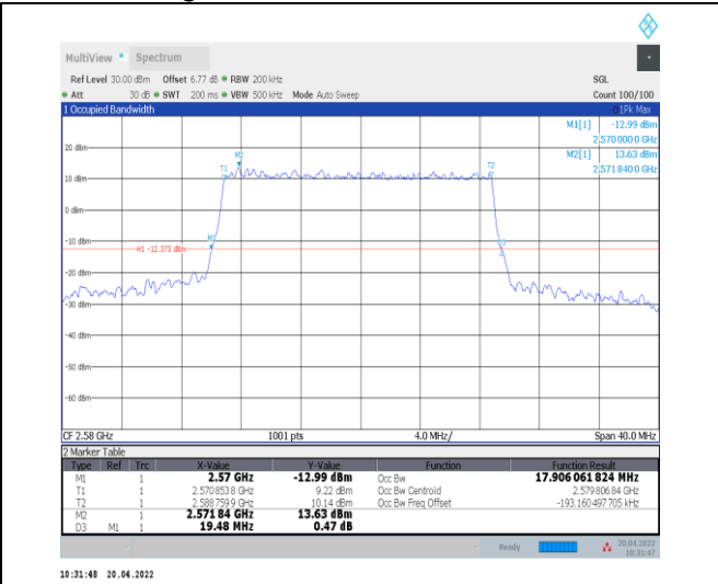
1-N38--30-20-L-4-DFT-64QAM-Outer_Full-50@0-Ant t0-17.906-19.480-≤20-PASS
