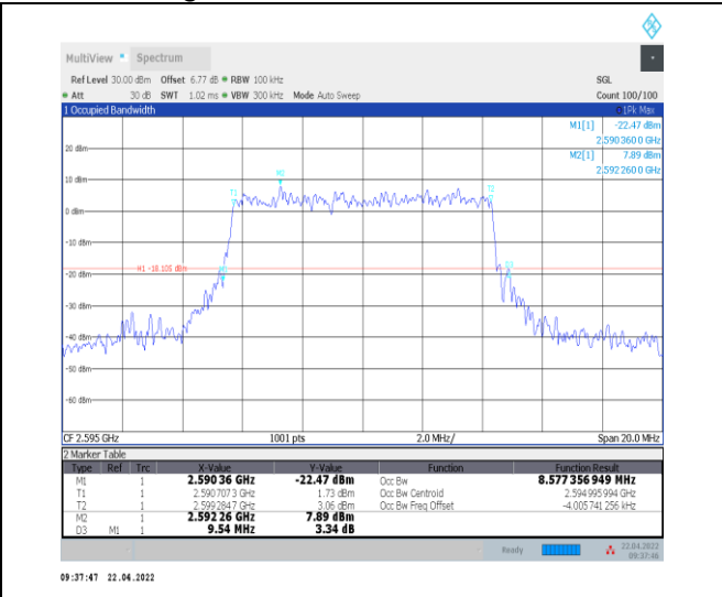
1-N38--30-10-M-9-CP-256QAM-Outer_Full-24@0-Ant 0-8.577-9.540-≤10-PASS
