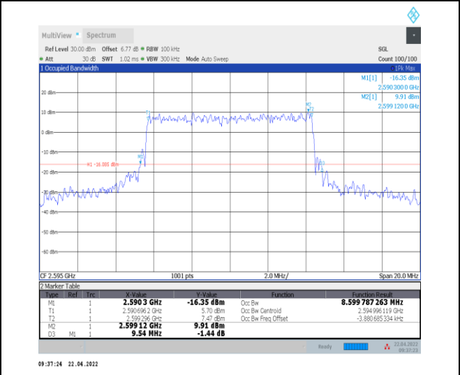
1-N38--30-10-M-7-CP-16QAM-Outer_Full-24@0-Ant 0-8.6-9.540≤10-PASS
