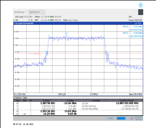
1-N38--30-15-M-4-DFT-64QAM-Outer_Full-36@0-Ant 0-12.887-14.250≤15-PASS
