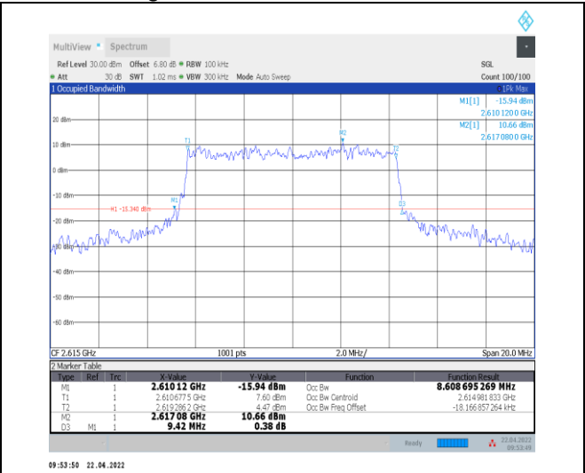
1-N38--30-10-H-8-CP-64QAM-Outer_Full-24@0-Ant 0-8.609-9.420-≤10-PASS
