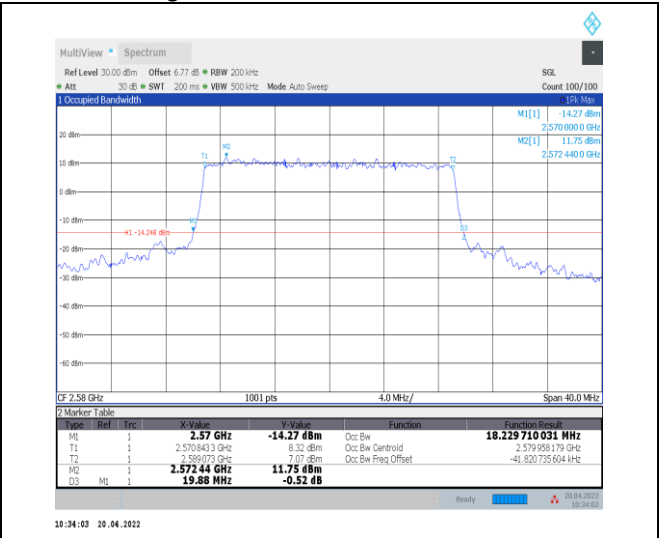
1-N38--30-20-L-8-CP-64QAM-Outer_Full-51@0-Ant0 0-18.23-19.880-≤20-PASS
