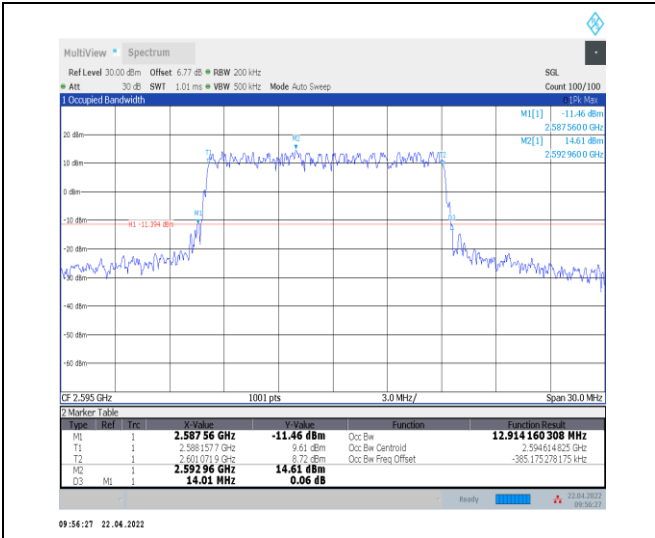
1-N38--30-15-M-1-DFT-QPSK-Outer_Full-36@0-Ant 0-12.914-14.010≤15-PASS
