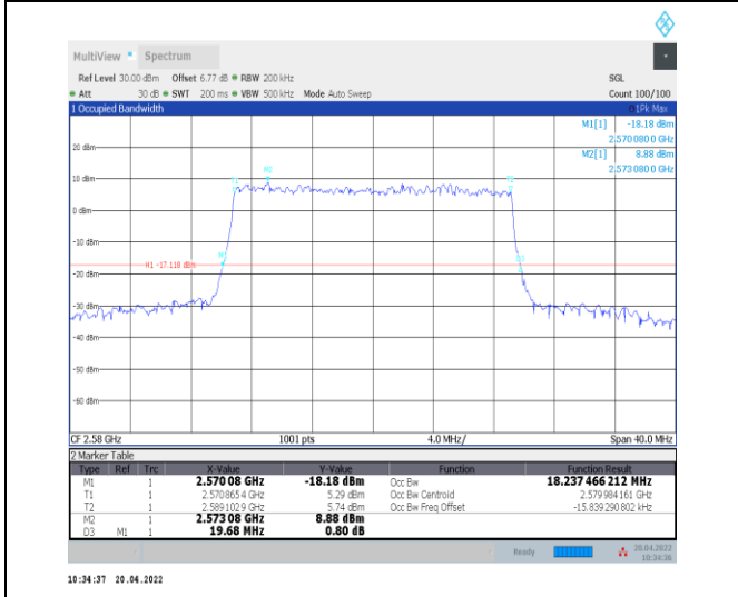
1-N38--30-20-L-9-CP-256QAM-Outer_Full-51@0-Ant0 0-18.237-19.680-≤20-PASS
