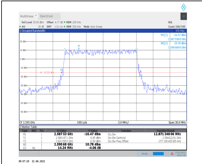
1-N38--30-15-M-5-DFT-256QAM-Outer_Full-36@0-A nt0-12.871-14.340-≤15-PASS
