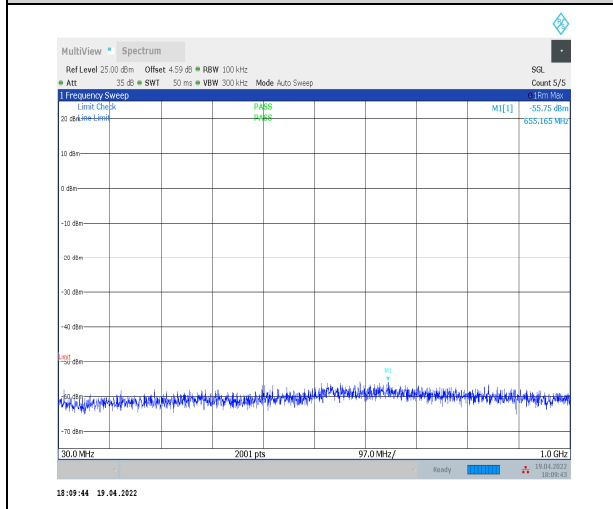
1-N30--15-10-H-1-DFT-PI2BPSK-Inner_1RB_Left-1 @1-30-1000-Ant0--55.75--50-PASS
