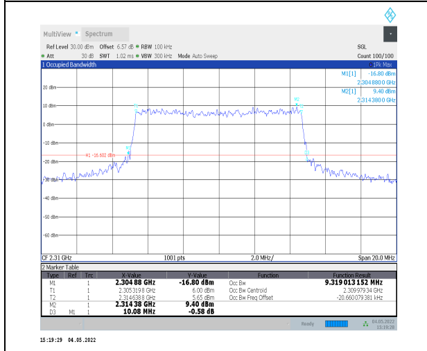
1-N30--15-10-L-8-CP-64QAM-Outer_Full-52@0-Ant 0-9.319-10.080≤10-PASS
