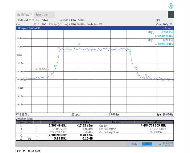
1-N30--15-5-M-7-CP-16QAM-Outer_Full-25@0-Ant0 -4.485-5.150-<math>\leq</math>5-PASS
