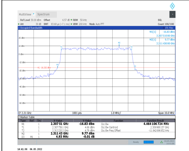
1-N30--15-5-M-6-CP-QPSK-Outer_Full-25@0-Ant0- 4.464-4.930-<math>\leq</math>5-PASS
