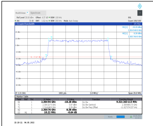
1-N30--15-10-L-6-CP-QPSK-Outer_Full-52@0-Ant-0 9.321-10.220≤10-PASS
