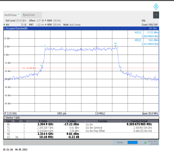
1-N30--15-10-M-8-CP-64QAM-Outer_Full-52@0-Ant 0-9.306-10.180-≤10-PASS
