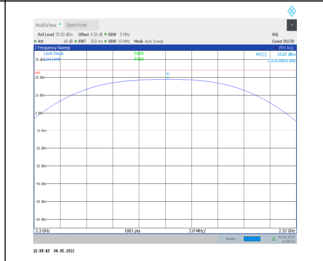
1-N30-PC3-15-10-L-3-DFT-PI2BPSK-Outter_Full-50 @0-2300-2320-Ant0-18.82-23.98-PASS
