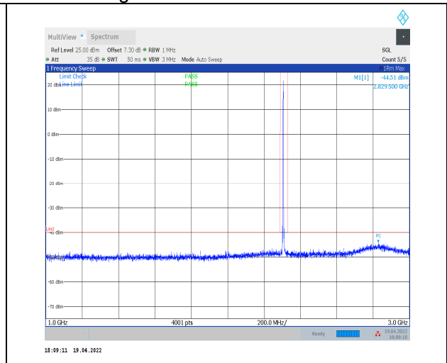
1-N30--15-10-M-1-DFT-PI2BPSK-Inner_1RB_Left-1 @1-1000-3000-Ant0--44.51--40-PASS
