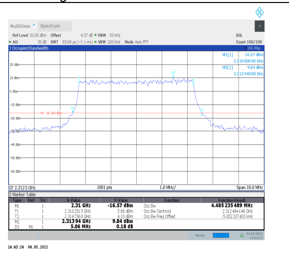
1-N30--15-5-H-8-CP-64QAM-Outer_Full-25@0-Ant0 4.485-5.060-≤5-PASS
