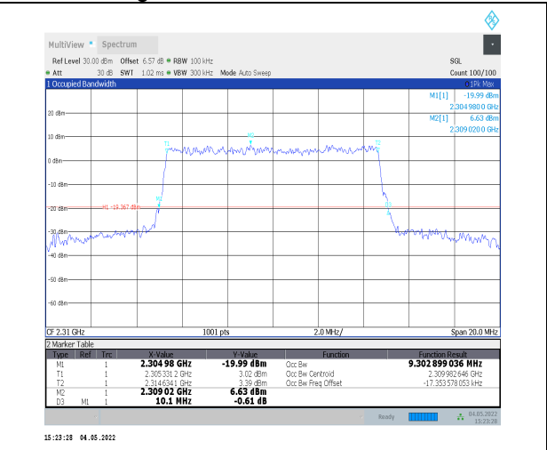
1-N30--15-10-H-9-CP-256QAM-Outer_Full-52@0-An t0-9.303-10.100-≤10-PASS
