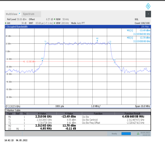
1-N30--15-5-H-2-DFT-PI2BPSK-Outer_Full-25@0-Ant0 4.457-4.950≤5-PASS
