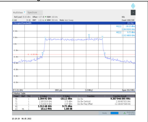
1-N30--15-10-L-7-CP-16QAM-Outer_Full-52@0-Ant0 -9.308-10.120≤10-PASS
