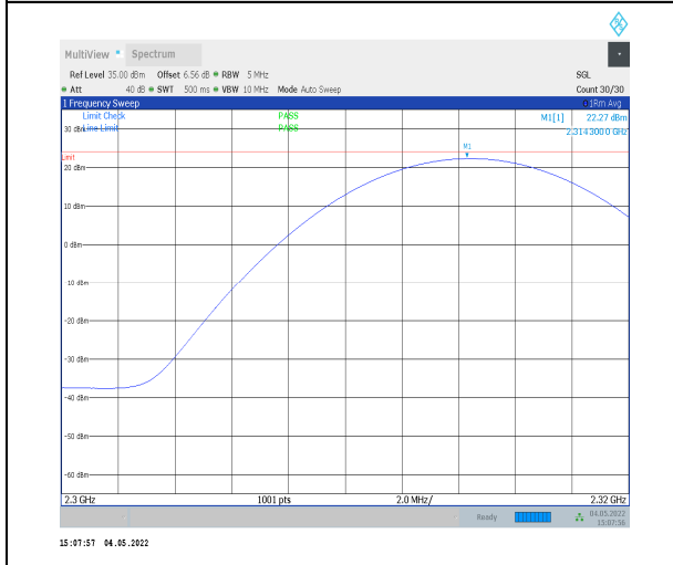
1-N30-PC3-15-10-L-2-DFT-PI2BPSK-Inner_1RB_Ri ght-1@50-2300-2320-Ant0-22.27-23.98-PASS
