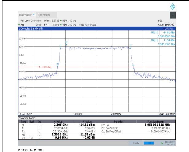
1-N30--15-10-L-4-DFT-64QAM-Outer_Full-50@0-A t0-8.951-9.640-≤10-PASS
