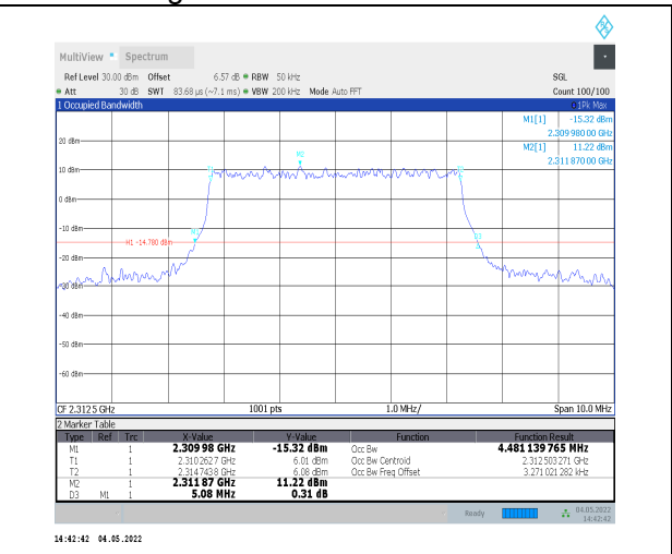
1-N30--15-5-H-4-DFT-64QAM-Outer_Full-25@0-Ant 0-4.481-5.080-≤5-PASS
