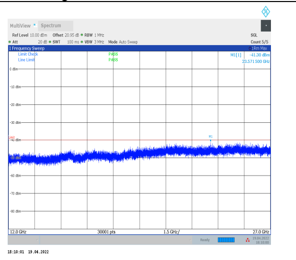
1-N30--15-10-H-1-DFT-PI2BPSK-Inner_1RB_Left-1 @1-12000-27000-Ant0--41.30--40-PASS
