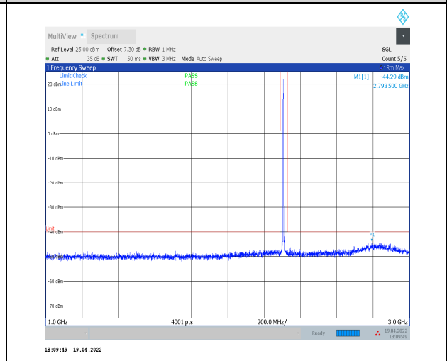
1-N30--15-10-H-1-DFT-PI2BPSK-Inner_1RB_Left-1 @1-1000-3000-Ant0--44.29--40-PASS
