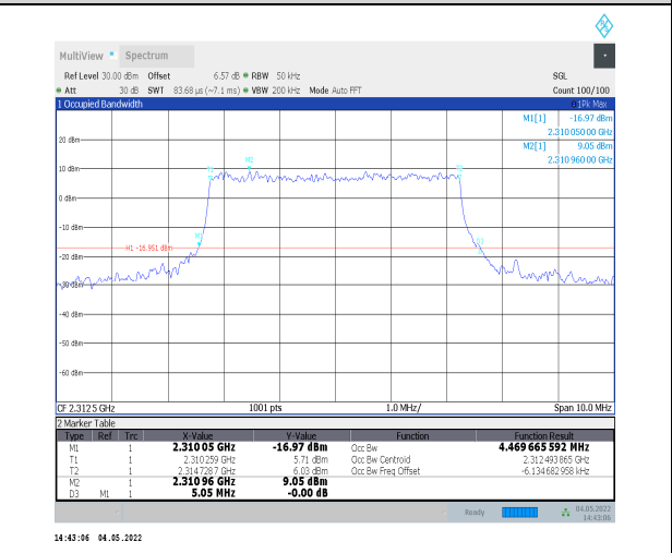
1-N30--15-5-H-6-CP-QPSK-Outer_Full-25@0-Ant0-4 .47-5.050-≤5-PASS
