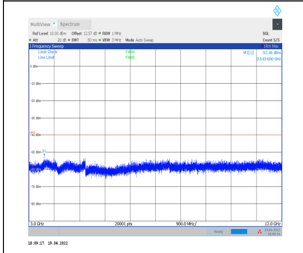
1-N30--15-10-M-1-DFT-PI2BPSK-Inner_1RB_Left-1 @1-3000-12000-Ant0--52.46--40-PASS
