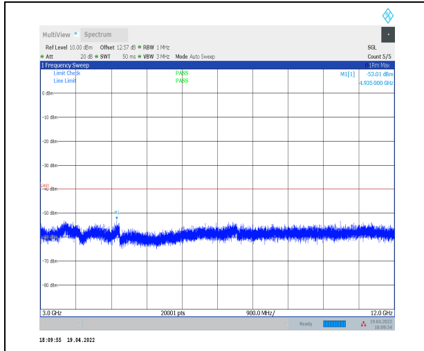
1-N30--15-10-H-1-DFT-PI2BPSK-Inner_1RB_Left-1 @1-3000-12000-Ant0--53.01--40-PASS
