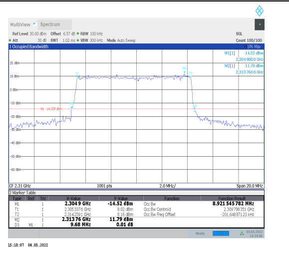
1-N30--15-10-L-1-DFT-QPSK-Outer_Full-50@0-Ant0 -8.922-9.680-≤10-PASS
