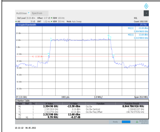
1-N30--15-10-H-2-DFT-PI2BPSK-Outer_Full-50@0-A Ant0-8.945-9.780-<=10-PASS
