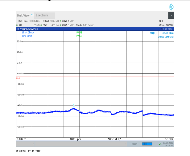
1-N26-824-849-PC3-15-20-H-1-DFT-PI2BPSK-Inner _1RB_Left-1@1-1000-6000-Ant0--42.36--13-PASS
