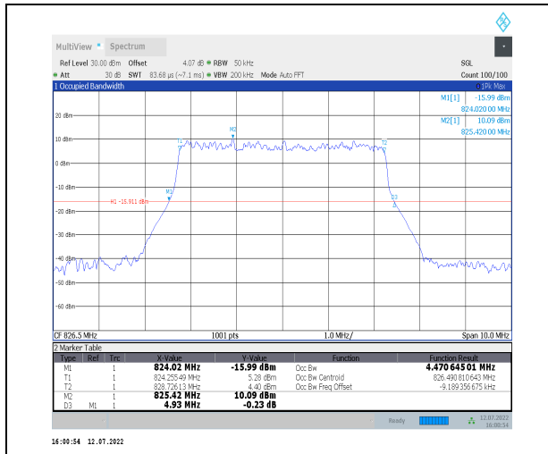
1-N26-824-849--15-5-L-5-DFT-256QAM-Outer_Full-25@0-Ant0-4.47-5.060-<math>\leq</math>5-PASS
