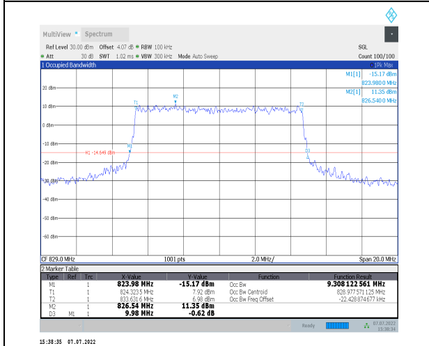
1-N26-824-849--15-10-L-8-CP-64QAM-Outer_Full-5 2@0-Ant0-9.308-9.980-<=10-PASS
