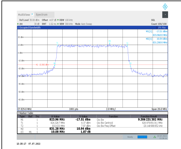
1-N26-824-849--15-10-L-6-CP-QPSK-Outer_Full-52 @0-Ant0-9.306-10.080-<=10-PASS
