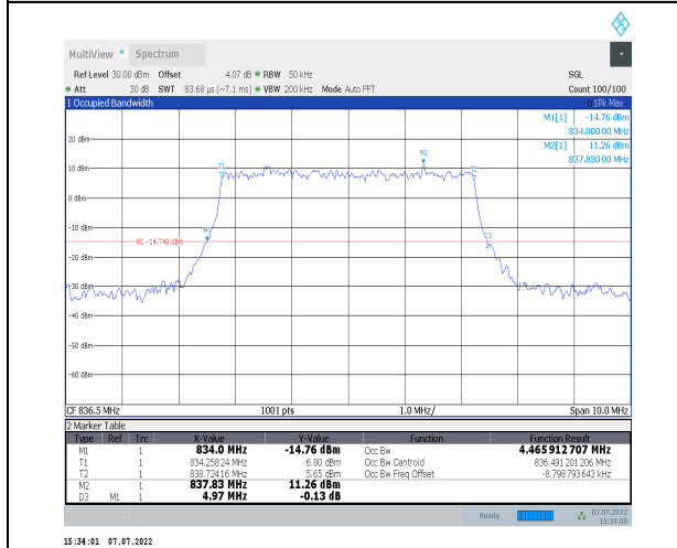
1-N26-824-849--15-5-M-6-CP-QPSK-Outer_Full-25 @0-Ant0-4.466-4.970-<5-PASS
