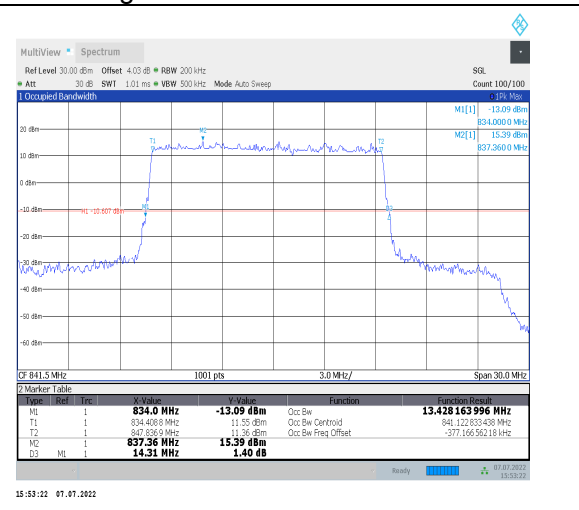
1-N26-824-849--15-15-H-2-DFT-PI2BPSK-Outer_Full-75@0-Ant0-13.428-14.310-<=15-PASS
