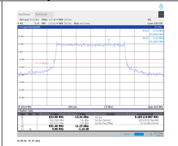
1-N26-824-849--15-10-L-7-CP-16QAM-Outer_Full-5 2@0-Ant0-9.283-9.980-<=10-PASS
