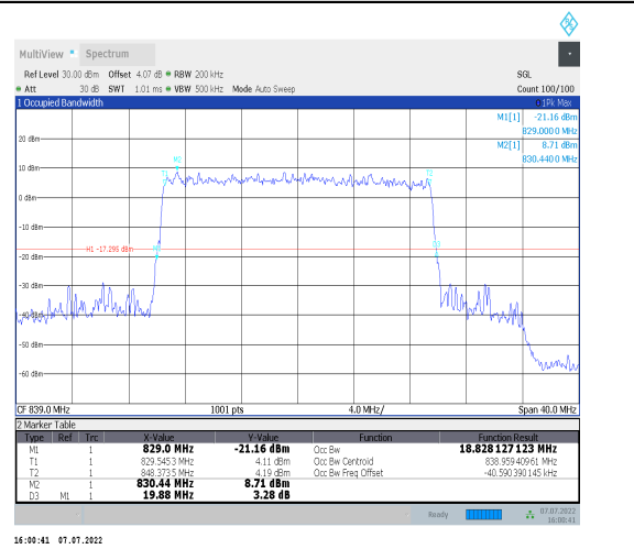
1-N26-824-849--15-20-H-9-CP-256QAM-Outer_Full-1 106@0-Ant0-18.828-19.880-≤20-PASS
