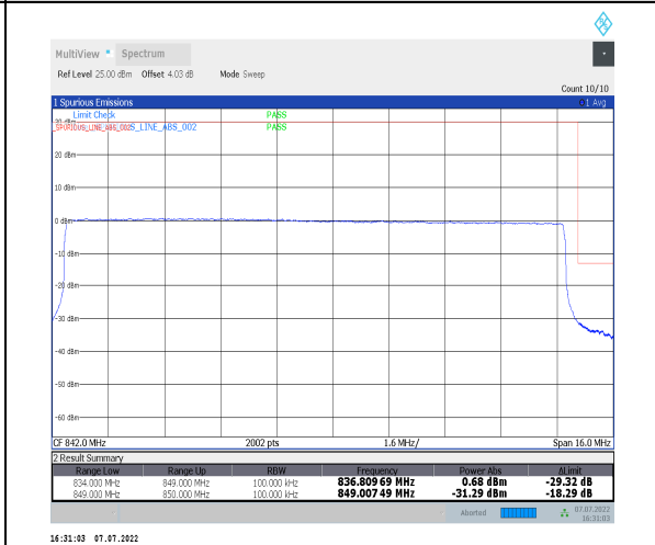
1-N26-824-849--15-15-H-6-CP-QPSK-Outer_Full-79@0-Ant0-seegraph-PASS-see graph
