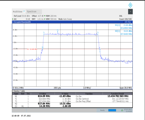
1-N26-824-849--15-15-L-2-DFT-PI2BPSK-Outer_Full7 5@0-Ant0-13.435-14.280-<=15-PASS
