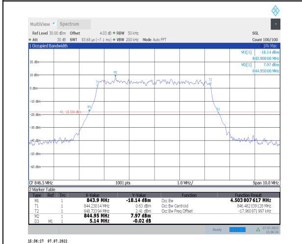
1-N26-824-849--15-5-H-9-CP-256QAM-Outer_Full-2 5@0-Ant0-4.504-5.140-<math>\leq</math>5-PASS
