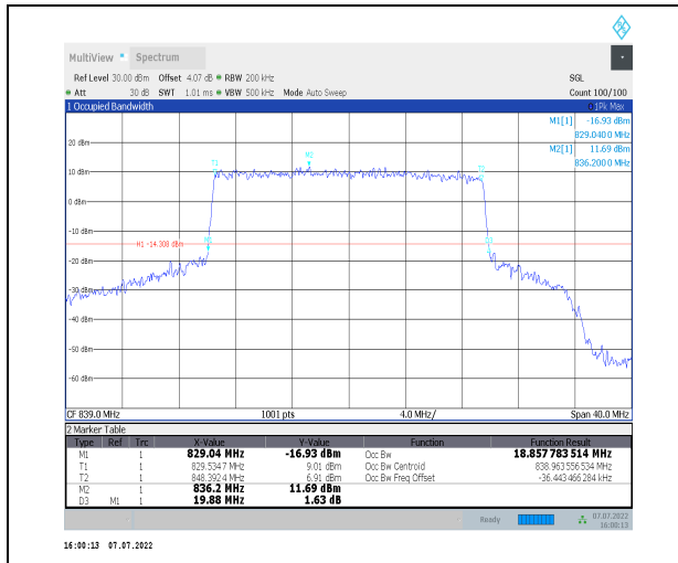
1-N26-824-849--15-20-H-6-CP-QPSK-Outer_Full-1 6@0-Ant0-18.858-19.880-≤20-PASS
