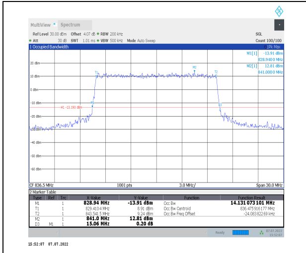
1-N26-824-849--15-15-M-6-CP-QPSK-Outer_Full-79 @0-Ant0-14.131-15.060-≤15-PASS
