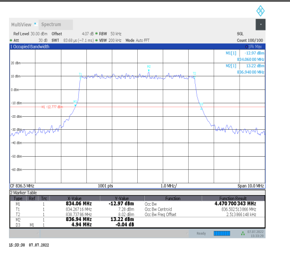
1-N26-824-849--15-5-M-3-DFT-16QAM-Outer_Full-2 5@0-Ant0-4.471-4.940-<5-PASS
