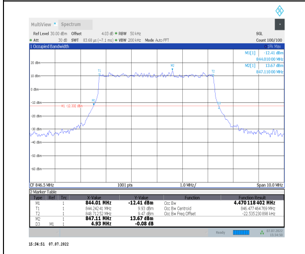
1-N26-824-849--15-5-H-1-DFT-QPSK-Outer_Full-25 @0-Ant0-4.47-4.930-<math>\leq</math>5-PASS
