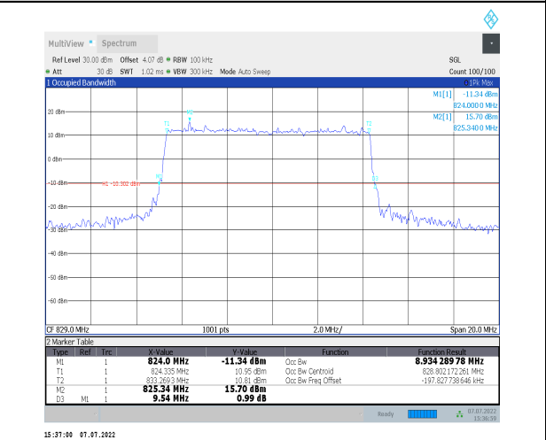
1-N26-824-849--15-10-L-1-DFT-QPSK-Outer_Full-50 @0-Ant0-8.934-9.540-<math>\leq</math>10-PASS
