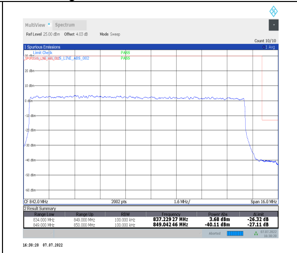
1-N26-824-849--15-15-H-3-DFT-PI2BPSK-Outer_Full-75@0-Ant0-seegraph-PASS-see graph
