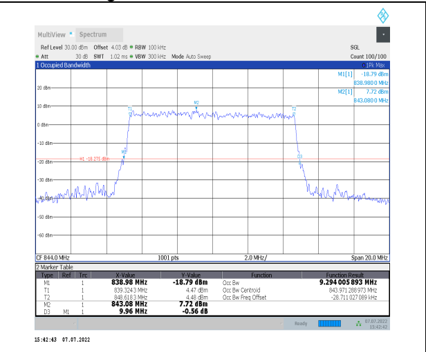
1-N26-824-849--15-10-H-9-CP-256QAM-Outer_Full5 2@0-Ant0-9.294-9.960-<=10-PASS
