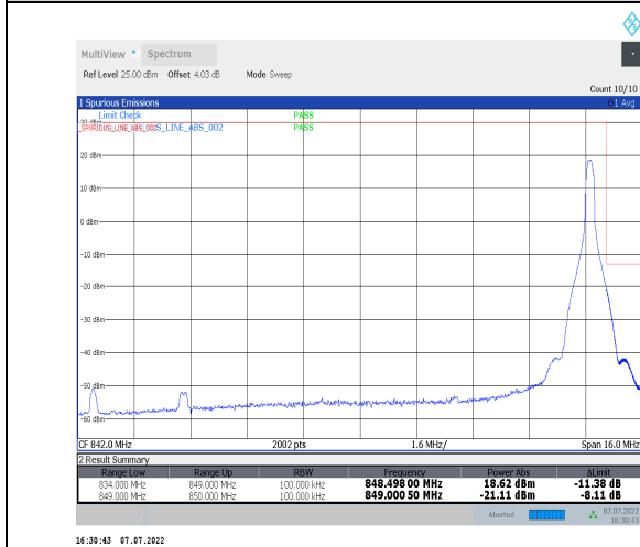
1-N26-824-849--15-15-H-5-CP-QPSK-Edge_1RB_Right-1@78-Ant0-seegraph-PASS-see graph
