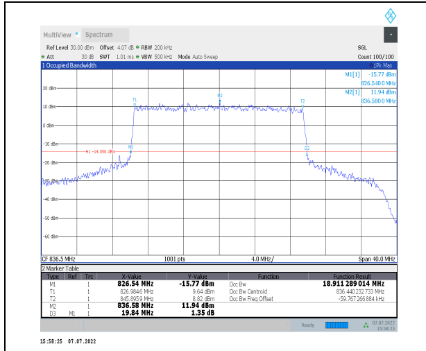
1-N26-824-849--15-20-M-7-CP-16QAM-Outer_Full-1 06@0-Ant0-18.911-19.840-<=20-PASS
