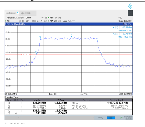
1-N26-824-849--15-5-M-1-DFT-QPSK-Outer_Full-25 @0-Ant0-4.477-5.110-<5-PASS
