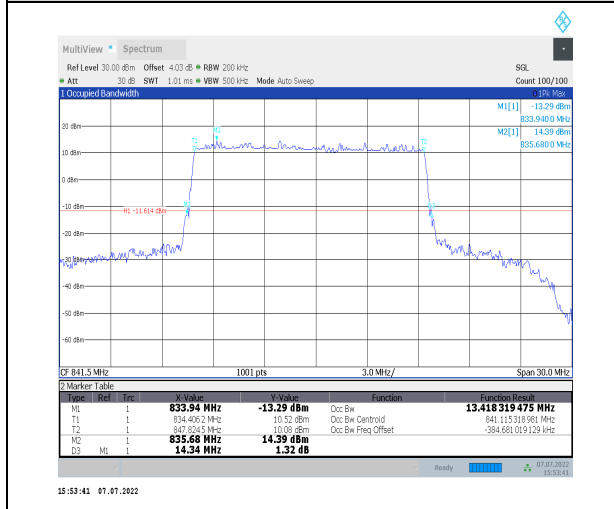
1-N26-824-849--15-15-H-3-DFT-16QAM-Outer_Full-75@0-Ant0-13.418-14.340-<=15-PASS
