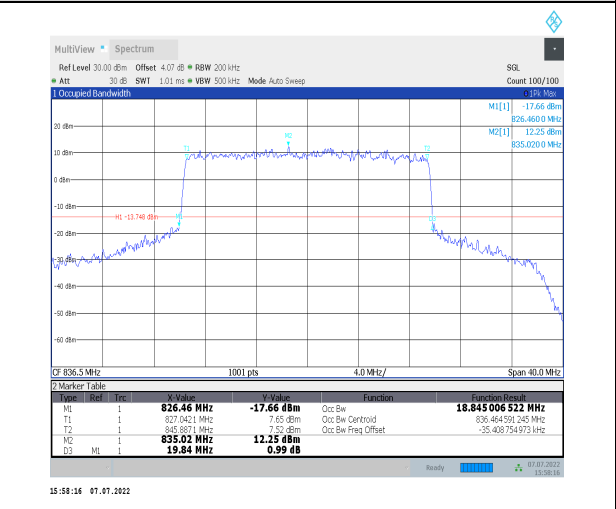
1-N26-824-849--15-20-M-6-CP-QPSK-Outer_Full-100@0-Ant0-18.845-19.840-<math>\leq 20</math>-PASS
