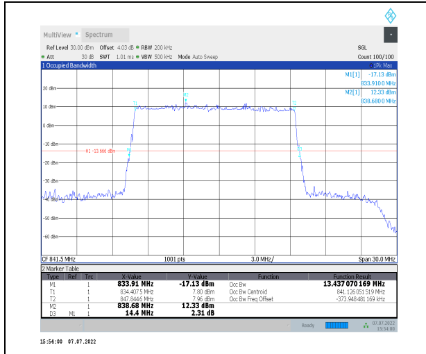
1-N26-824-849--15-15-H-5-DFT-256QAM-Outer_Full -75@0-Ant0-13.437-14.400-<=15-PASS
