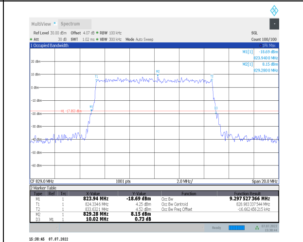
1-N26-824-849--15-10-L-9-CP-256QAM-Outer_Full-5 2@0-Ant0-9.298-10.020-<=10-PASS
