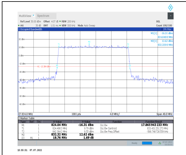
1-N26-824-849--15-20-L-4-DFT-64QAM-Outer_Full-100@0-Ant0-17.866-18.760-<math>\leq 20</math>-PASS
