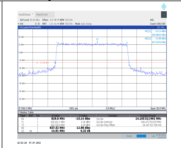
1-N26-824-849--15-15-M-7-CP-16QAM-Outer_Full-79 @0-Ant0-14.105-14.910-≤15-PASS
