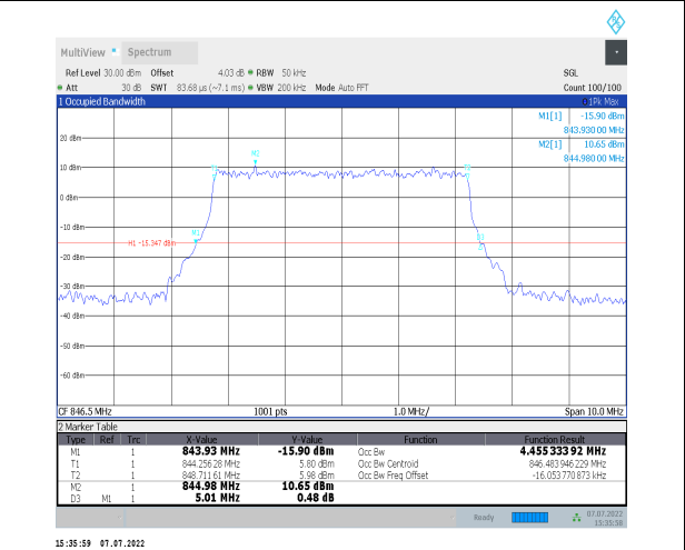
1-N26-824-849--15-5-H-6-CP-QPSK-Outer_Full-25 @0-Ant0-4.455-5.010-<math>\leq</math>5-PASS
