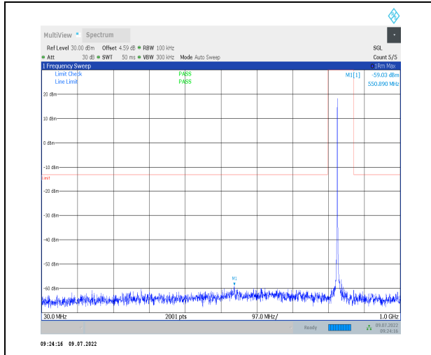
1-N26-824-849-PC3-15-20-H-1-DFT-PI2BPSK-Inner _1RB_Left-1@1-30-1000-Ant0--59.03--23-PASS
