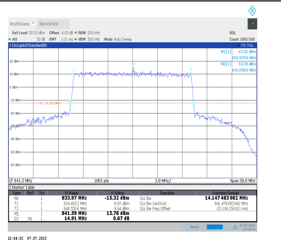
1-N26-824-849--15-15-H-8-CP-64QAM-Outer_Full-7 9@0-Ant0-14.147-14.910-<=15-PASS
