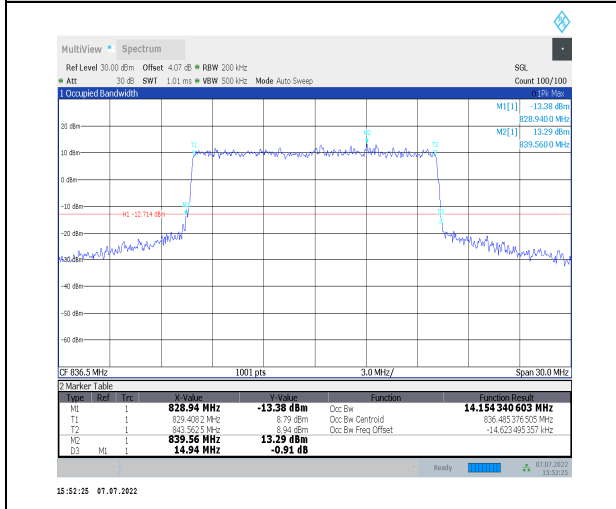
1-N26-824-849--15-15-M-8-CP-64QAM-Outer_Full-79 @0-Ant0-14.154-14.940-≤15-PASS
