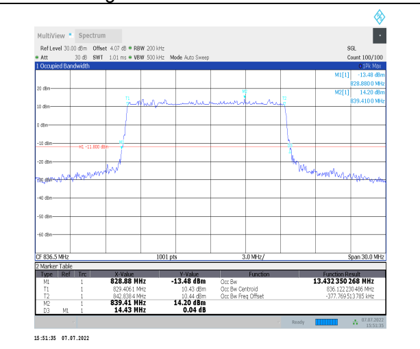
1-N26-824-849--15-15-M-3-DFT-16QAM-Outer_Full-75@0-Ant0-13.432-14.430-≤15-PASS
