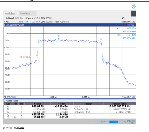
1-N26-824-849--15-20-H-7-CP-16QAM-Outer_Full-1 06@0-Ant0-18.908-19.840-≤20-PASS
