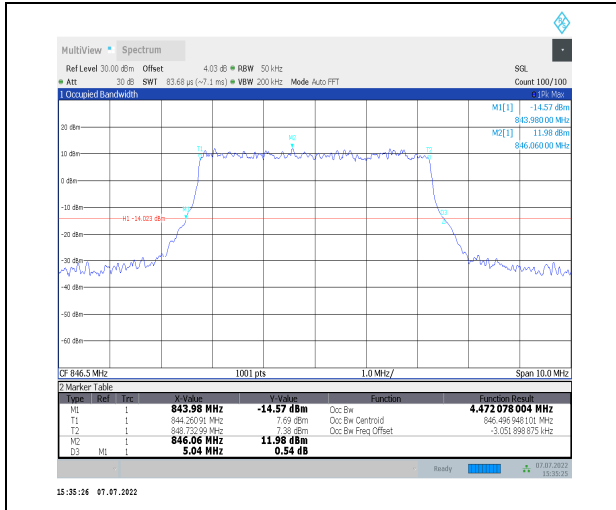
1-N26-824-849--15-5-H-3-DFT-16QAM-Outer_Full-2 5@0-Ant0-4.472-5.040-<math>\leq</math>5-PASS
