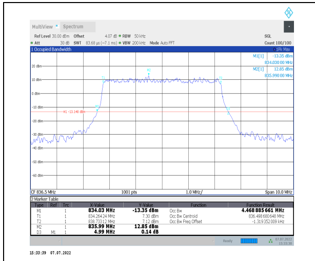
1-N26-824-849--15-5-M-4-DFT-64QAM-Outer_Full-2 5@0-Ant0-4.469-4.990-<5-PASS
