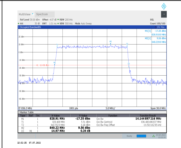
1-N26-824-849--15-15-M-9-CP-256QAM-Outer_Full-79 @0-Ant0-14.145-14.970-≤15-PASS
