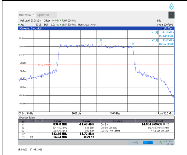
1-N26-824-849--15-15-H-7-CP-16QAM-Outer_Full-7 9@0-Ant0-14.085-14.940-<=15-PASS
