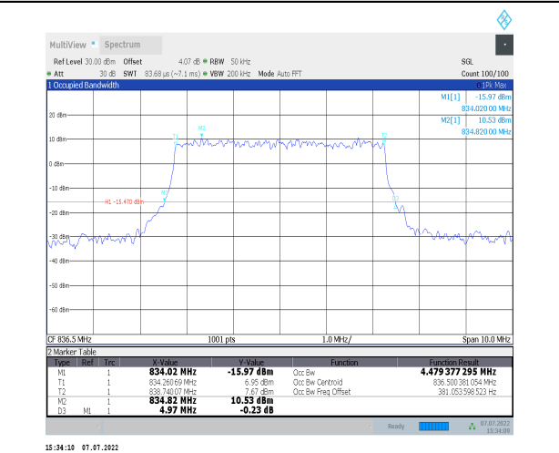
1-N26-824-849--15-5-M-7-CP-16QAM-Outer_Full-25 @0-Ant0-4.479-4.970-<5-PASS
