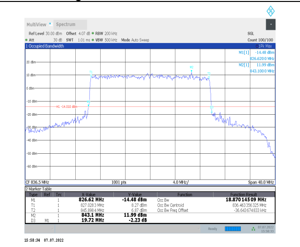
1-N26-824-849--15-20-M-8-CP-64QAM-Outer_Full-1 06@0-Ant0-18.87-19.720-<=20-PASS
