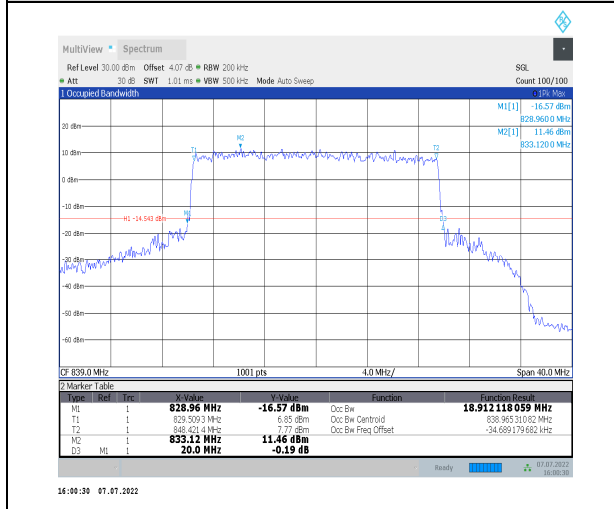
1-N26-824-849--15-20-H-8-CP-64QAM-Outer_Full-1 06@0-Ant0-18.912-20.000-≤20-PASS
