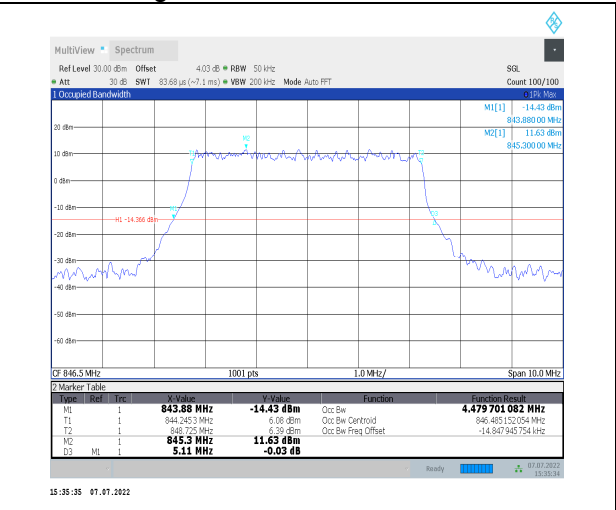
1-N26-824-849--15-5-H-4-DFT-64QAM-Outer_Full-2 5@0-Ant0-4.48-5.110-<math>\leq</math>5-PASS
