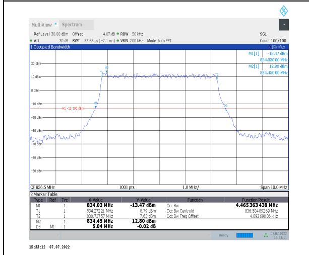
1-N26-824-849--15-5-M-2-DFT-PI2BPSK-Outer_Full -25@0-Ant0-4.465-5.040-<5-PASS
