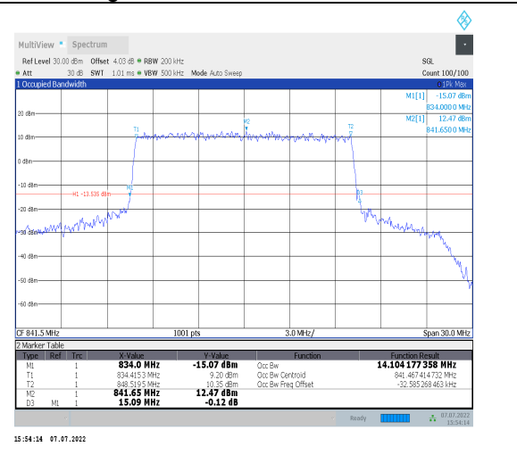
1-N26-824-849--15-15-H-6-CP-QPSK-Outer_Full-79 @0-Ant0-14.104-15.090-<=15-PASS
