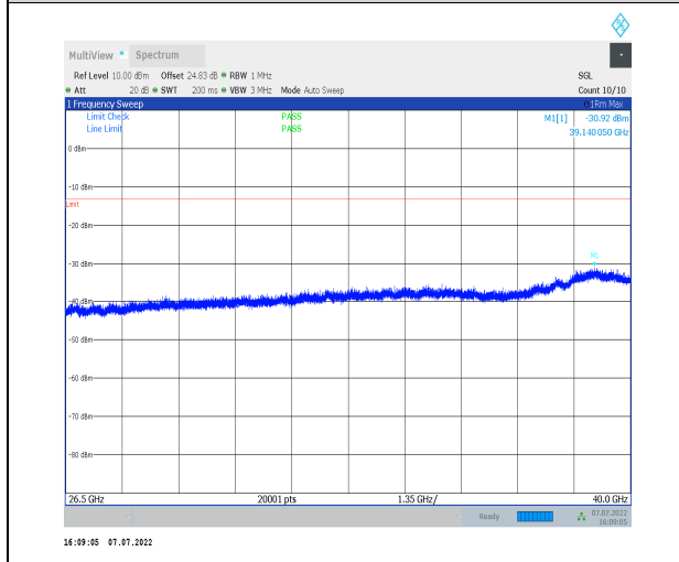
1-N26-824-849-PC3-15-20-H-1-DFT-PI2BPSK-Inner _1RB_Left-1@1-26500-40000-Ant0--30.92--13-PAS
