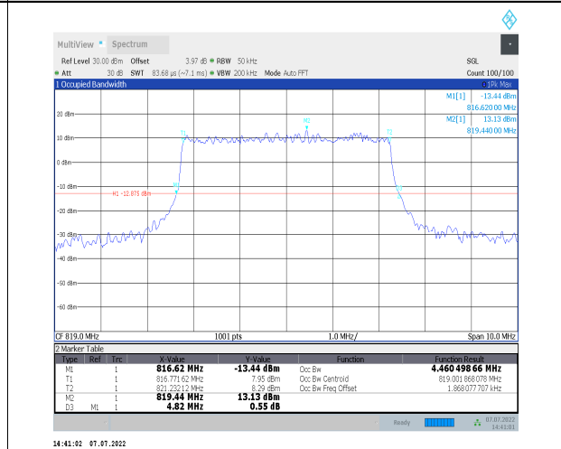
1-N26-814-824--15-5-M-3-DFT-16QAM-Outer_Full-25@0-Ant0-4.46-4.820-≤5-PASS
