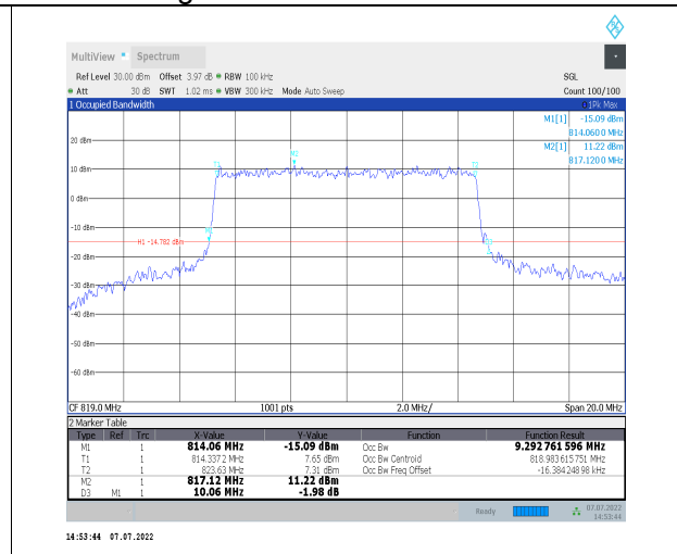
1-N26-814-824--15-10-M-7-CP-16QAM-Outer_Full-5 2@0-Ant0-9.293-10.060-≤10-PASS
