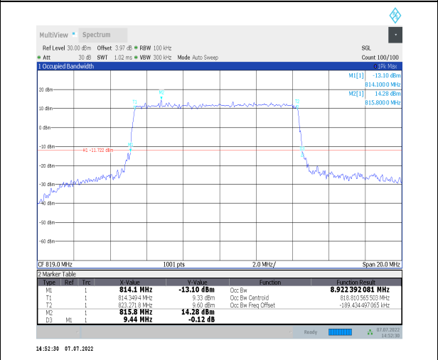
1-N26-814-824--15-10-M-1-DFT-QPSK-Outer_Full-5 0@0-Ant0-8.922-9.440-<math>\leq 10</math>-PASS
