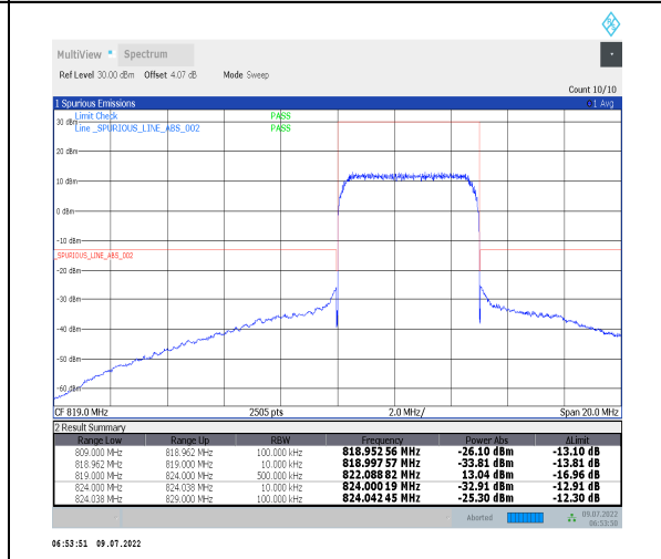
1-N26-814-824--15-5-H-6-CP-QPSK-Outer_Full-25@0-Ant0-PASS-see graph
