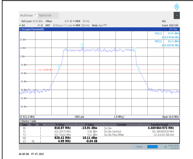
1-N26-814-824--15-5-H-5-DFT-256QAM-Outer_Full-25 25@0-Ant0-4.47-4.990-≤5-PASS
