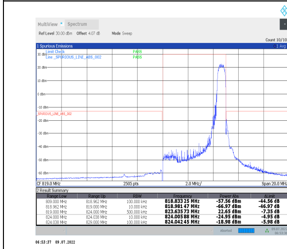
1-N26-814-824--15-5-H-5-CP-QPSK-Edge_1RB_Right-1@24-Ant0-PASS-see graph
