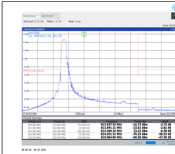
1-N26-814-824--15-10-M-1-DFT-PI2BPSK-Edge_1RB_Left-1@0-Ant0-PASS-see graph
