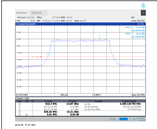
1-N26-814-824--15-5-M-8-CP-64QAM-Outer_Full-25 @0-Ant0-4.48-5.010-<math>\leq</math>5-PASS
