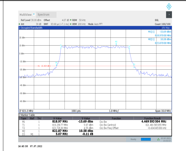
1-N26-814-824--15-5-H-6-CP-QPSK-Outer_Full-25 @0-Ant0-4.47-5.070-≤5-PASS
