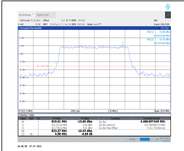
1-N26-814-824--15-5-H-7-CP-16QAM-Outer_Full-25 @0-Ant0-4.487-4.980-<math>\leq 5</math>-PASS
