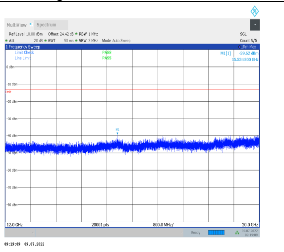
1-N26-814-824-PC3-15-10-M-1-DFT-PI2BPSK-Inner _1RB_Left-1@1-12000-20000-Ant0--39.62--13-PASS
