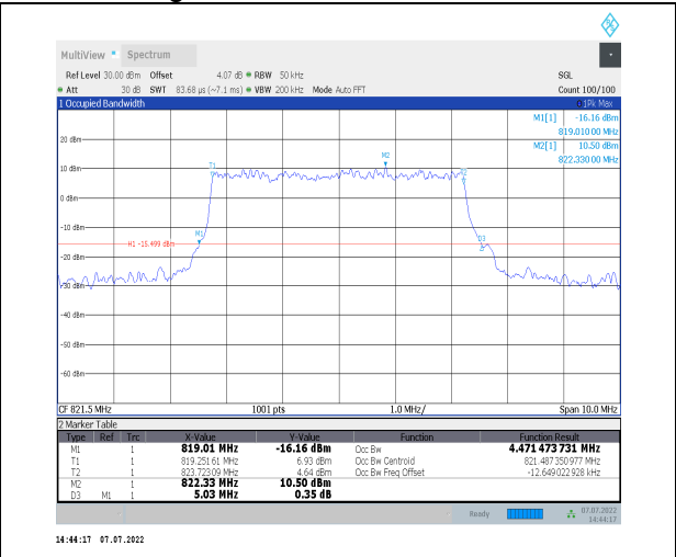
1-N26-814-824--15-5-H-8-CP-64QAM-Outer_Full-25 @0-Ant0-4.471-5.030-<math>\leq 5</math>-PASS
