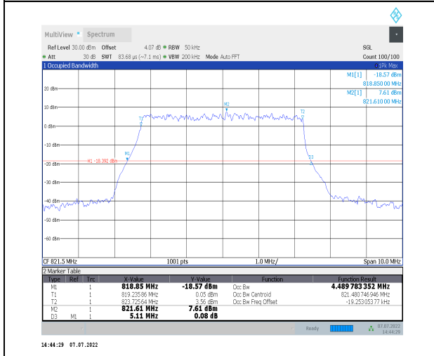
1-N26-814-824--15-5-H-9-CP-256QAM-Outer_Full-2 5@0-Ant0-4.49-5.110-<math>\leq 5</math>-PASS
