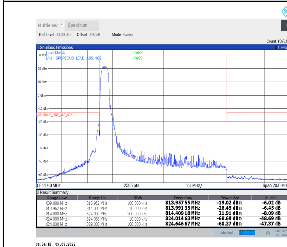
1-N26-814-824--15-10-M-4-CP-QPSK-Edge_1RB_Left-1@0-Ant0-PASS-see graph
