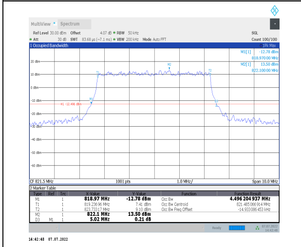
1-N26-814-824--15-5-H-1-DFT-QPSK-Outer_Full-25 @0-Ant0-4.496-5.020-<math>\leq</math>5-PASS
