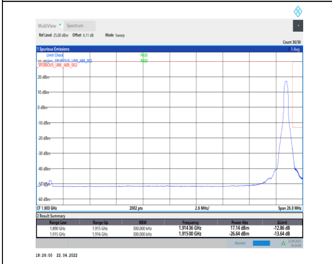
1-N25--15-25-H-5-CP-QPSK-Edge_1RB_Right-1 @ 132 -Ant0-seegraph-PASS-see graph
