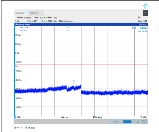
1-N25--15-40-M-1-DFT-PI2BPSK-Inner_1RB_Left-1 @ 1-3000-12000-Ant0--34.32--13-PASS
