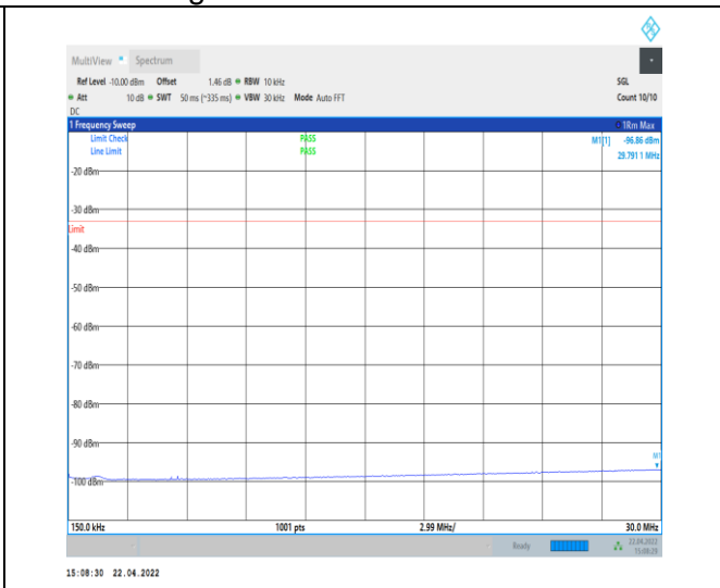
1-N25--15-40-H-1-DFT-PI2BPSK-Inner_1RB_Left-1 @ 1-0.15-30-Ant0--96.86--33-PASS
