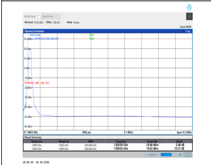
1-N25--15-40-L-4-CP-QPSK-Edge_1RB_Left-1@0-Ant0-seegraph-PASS-see graph
