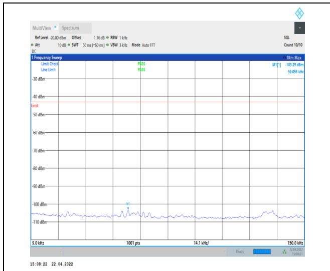
1-N25--15-40-H-1-DFT-PI2BPSK-Inner_1RB_Left-1 @ 1-0.009-0.15-Ant0--103.29--43-PASS
