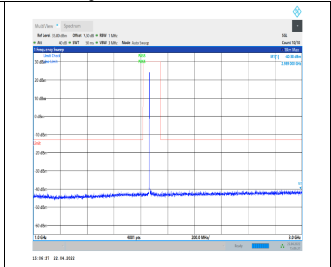
1-N25--15-40-M-1-DFT-PI2BPSK-Inner_1RB_Left-1 @ 1-1000-3000-Ant0--40.38--13-PASS
