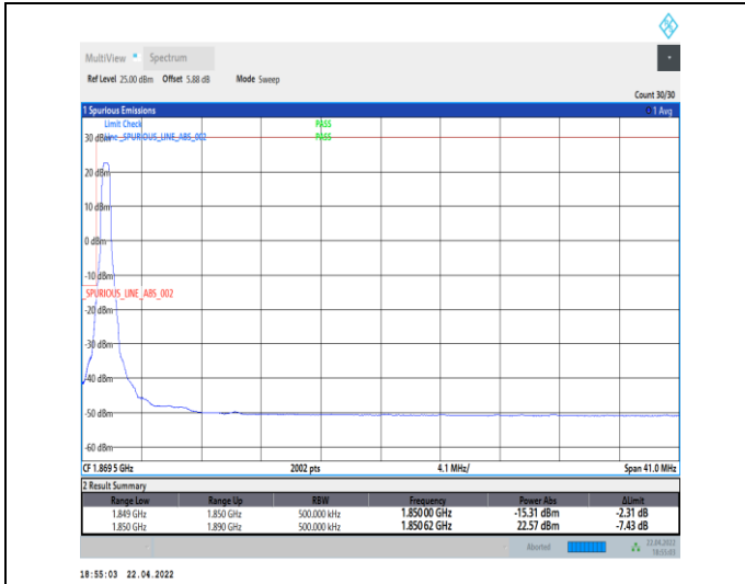
1-N25--15-40-L-1-DFT-PI2BPSK-Edge_1RB_Left-1@0-Ant0-seegraph-PASS-see graph
