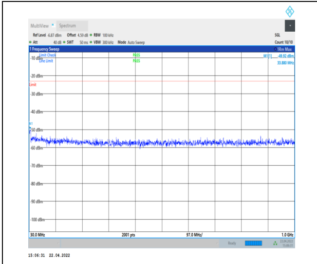
1-N25--15-40-M-1-DFT-PI2BPSK-Inner_1RB_Left-1 @ 1-30-1000-Ant0--49.92--23-PASS
