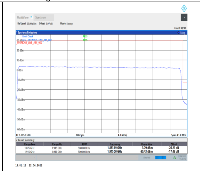
1-N25--15-40-H-3-DFT-PI2BPSK-Outer_Full-216 @0-Ant0-seegraph-PASS-see graph
