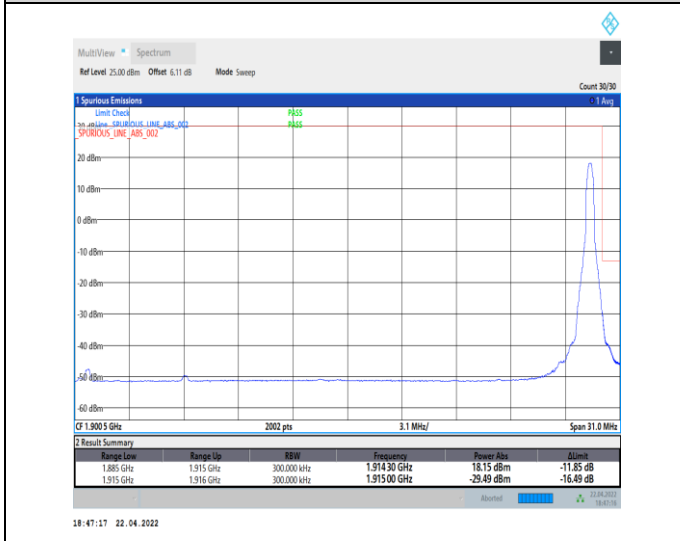
1-N25--15-30-H-5-CP-QPSK-Edge_1RB_Right-1 @ 159 -Ant0-seegraph-PASS-see graph
