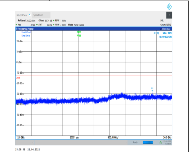
1-N25--15-40-H-1-DFT-PI2BPSK-Inner_1RB_Left-1 @ 1-12000-20000-Ant0--28.37--13-PASS
