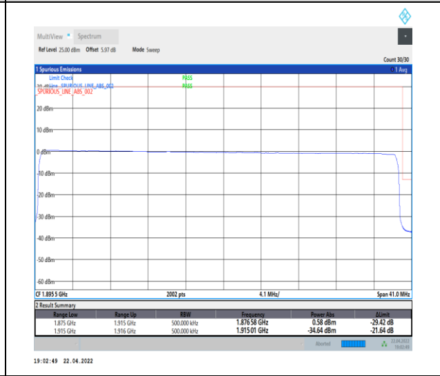
1-N25--15-40-H-6-CP-QPSK-Outer_Full-216 @0-A -nt0-seegraph-PASS-see graph
