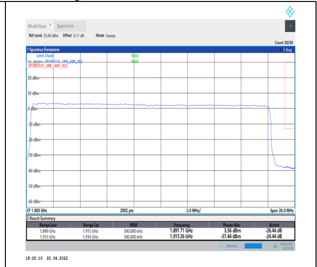
1-N25--15-25-H-3-DFT-PI2BPSK-Outer_Full-128 @ 0-Ant0-seegraph-PASS-see graph
