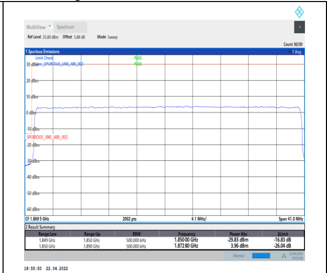
1-N25--15-40-L-3-DFT-PI2BPSK-Outer_Full-216@0-Ant0-seegraph-PASS-see graph
