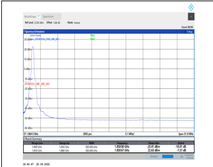
1-N25--15-30-L-1-DFT-PI2BPSK-Edge_1RB_Left-1@0-Ant0-seegraph-PASS-see graph
