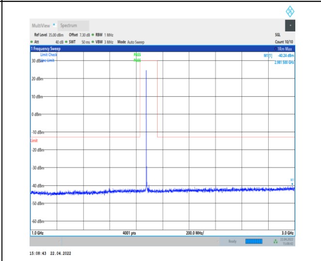
1-N25--15-40-H-1-DFT-PI2BPSK-Inner_1RB_Left-1 @ 1-1000-3000-Ant0--40.24--13-PASS
