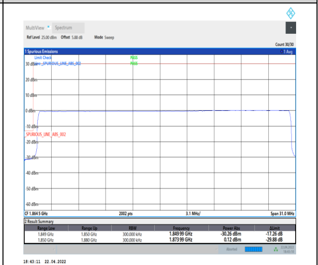
1-N25--15-30-L-6-CP-QPSK-Outer_Full-160@0-Ant0-seegraph-PASS-see graph
