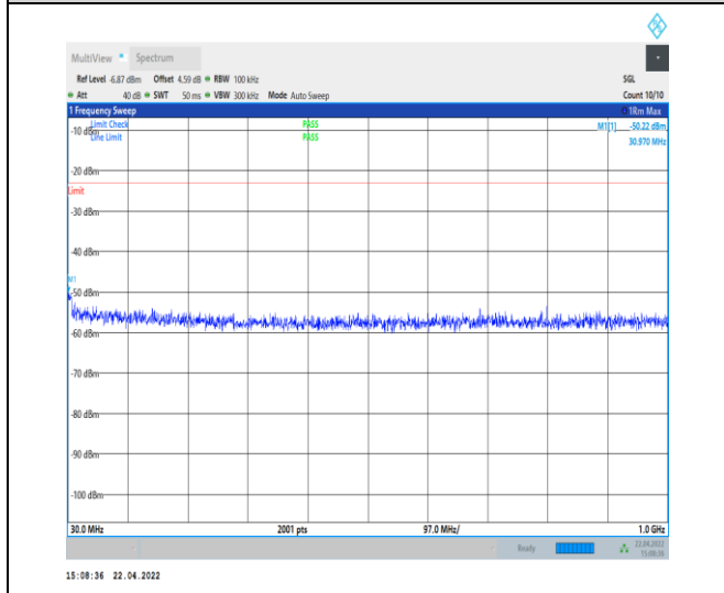
1-N25--15-40-H-1-DFT-PI2BPSK-Inner_1RB_Left-1 @ 1-30-1000-Ant0--50.22--23-PASS
