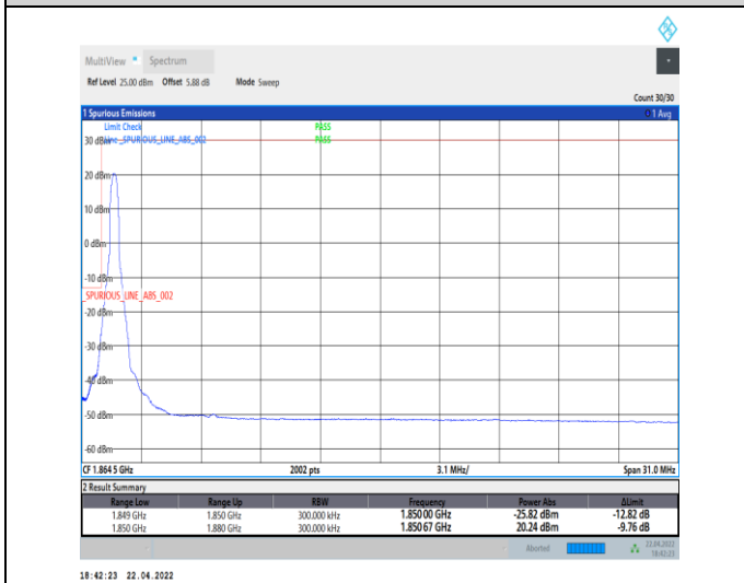
1-N25--15-30-L-4-CP-QPSK-Edge_1RB_Left-1@0-Ant0-seegraph-PASS-see graph
