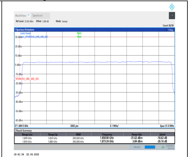
1-N25--15-30-L-3-DFT-PI2BPSK-Outer_Full-160@0-Ant0-seegraph-PASS-see graph
