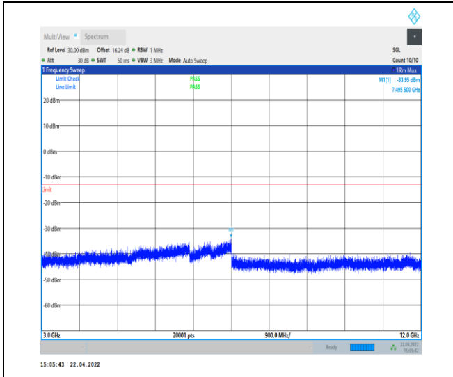
1-N25--15-40-L-1-DFT-PI2BPSK-Inner_1RB_Left-1 @ 1-3000-12000-Ant0--33.95--13-PASS
