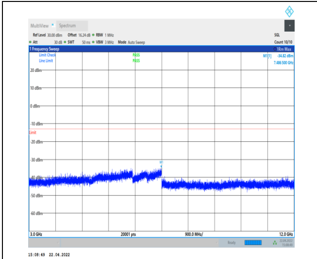
1-N25--15-40-H-1-DFT-PI2BPSK-Inner_1RB_Left-1 @ 1-3000-12000-Ant0--34.82--13-PASS
