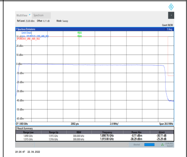
1-N25--15-25-H-6-CP-QPSK-Outer_Full-133 @ 0-A nt0-seegraph-PASS-see graph
