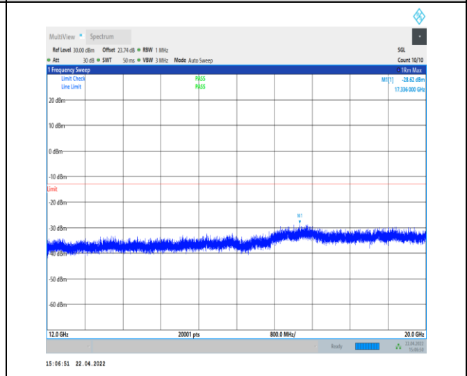
1-N25--15-40-M-1-DFT-PI2BPSK-Inner_1RB_Left-1 @ 1-12000-20000-Ant0--28.62--13-PASS
