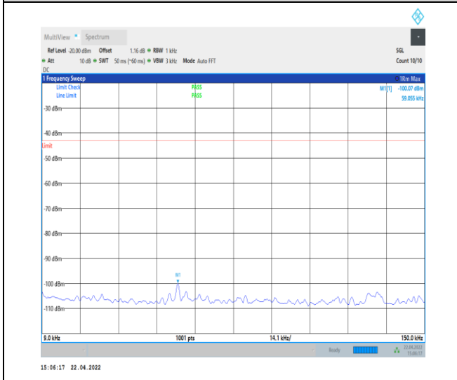
1-N25--15-40-M-1-DFT-PI2BPSK-Inner_1RB_Left-1 @ 1-0.009-0.15-Ant0--100.07--43-PASS
