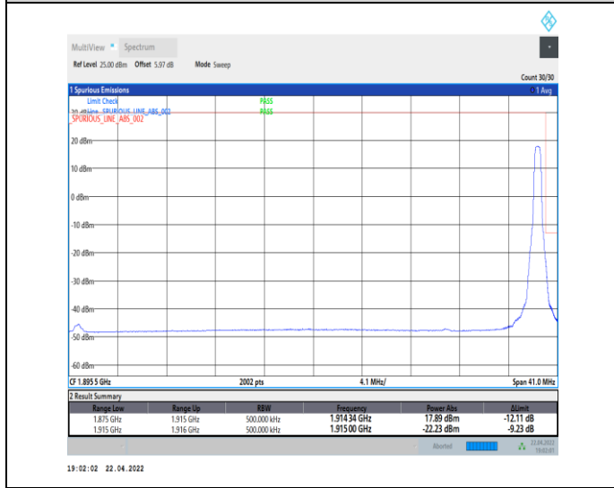
1-N25--15-40-H-5-CP-QPSK-Edge_1RB_Right-1 @215 -Ant0-seegraph-PASS-see graph
