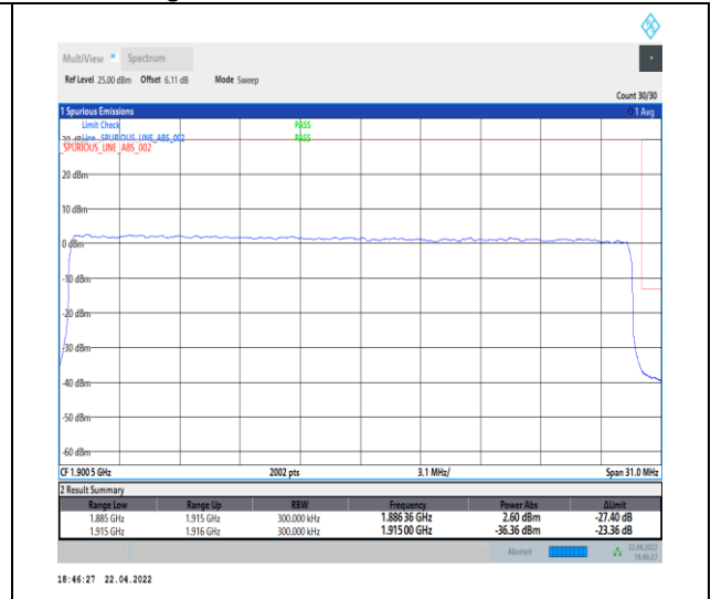
1-N25--15-30-H-3-DFT-PI2BPSK-Outer_Full-160 @ 0-Ant0-seegraph-PASS-see graph
