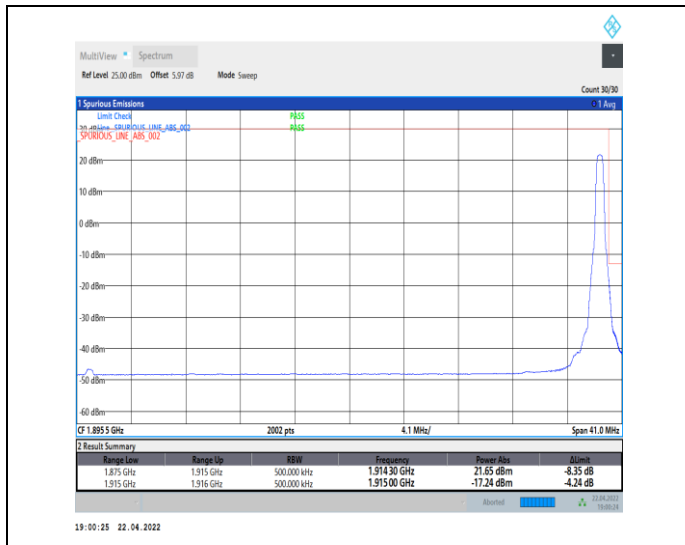
1-N25--15-40-H-2-DFT-PI2BPSK-Edge_1RB_Right-1 @215-Ant0-seegraph-PASS-see graph
