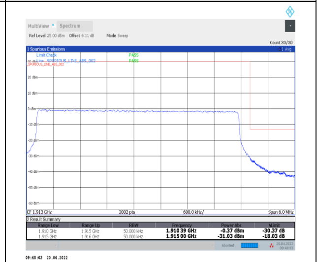
1-N25--15-5-H-6-CP-QPSK-Outer_Full-25@0-Ant0-seegraph-PASS-see graph
