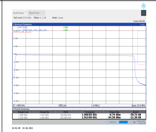
1-N25--15-15-H-6-CP-QPSK-Outer_Full-79@0-Ant0-seegraph-PASS-see graph
