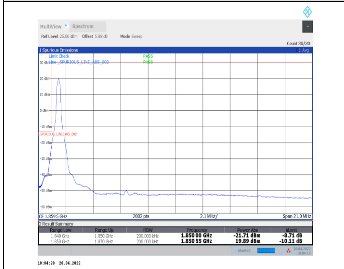
1-N25--15-20-L-4-CP-QPSK-Edge_1RB_Left-1@0-Ant0-seegraph-PASS-see graph
