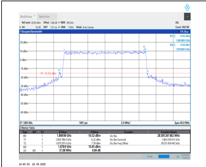
1-N25--15-30-L-6-CP-QPSK-Outer_Full-160@0-Ant0 -28.505-31.080-≤30-PASS
