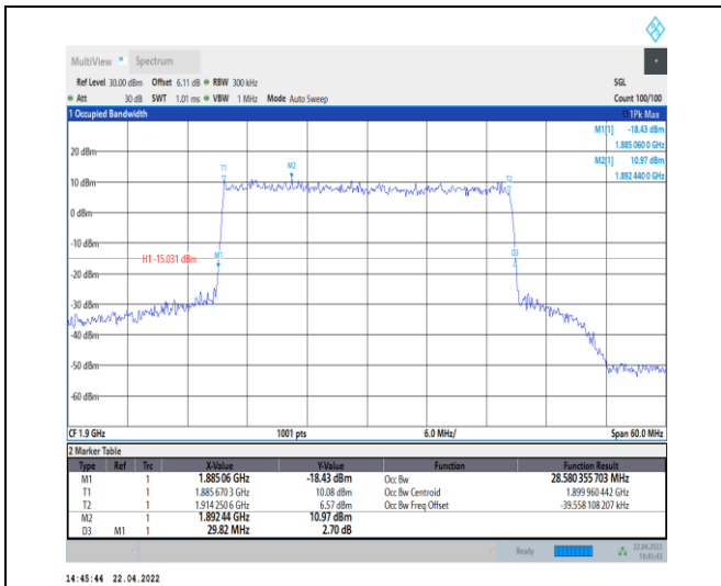
1-N25--15-30-H-4-DFT-64QAM-Outer_Full-160@0-A nt0-28.58-29.820-≤30-PASS
