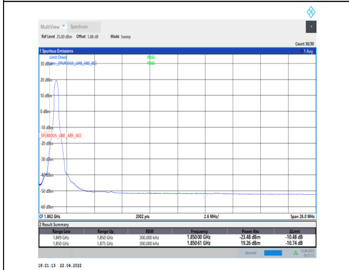
1-N25--15-25-L-4-CP-QPSK-Edge_1RB_Left-1@0-Ant0-seegraph-PASS-see graph
