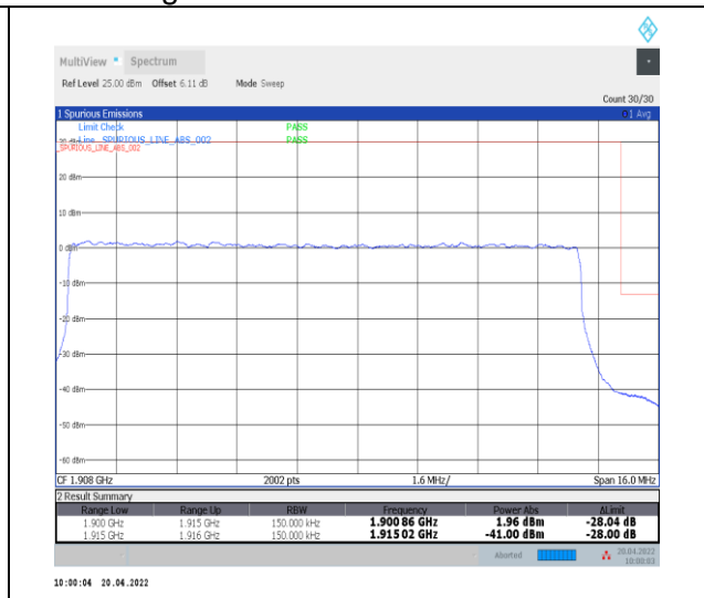
1-N25--15-15-H-3-DFT-PI2BPSK-Outer_Full-75@0-Ant0-seegraph-PASS-see graph
