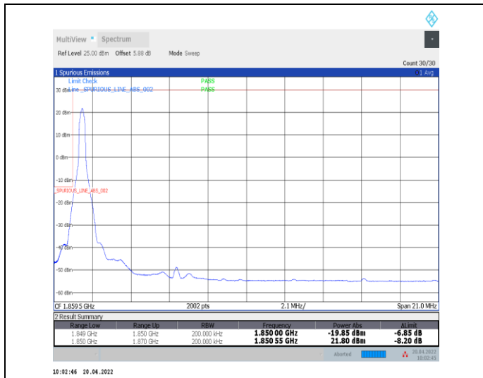
1-N25--15-20-L-1-DFT-PI2BPSK-Edge_1RB_Left-1@0-Ant0-seegraph-PASS-see graph
