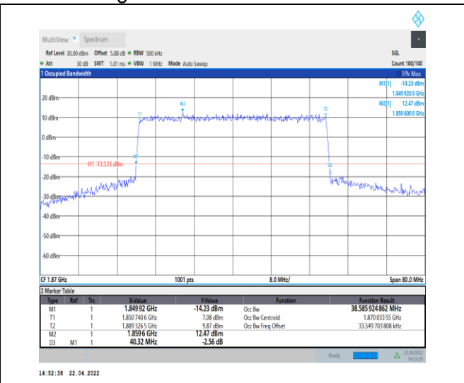
1-N25--15-40-L-4-DFT-64QAM-Outer_Full-216@0-A nt0-38.586-40.320-≤40-PASS
