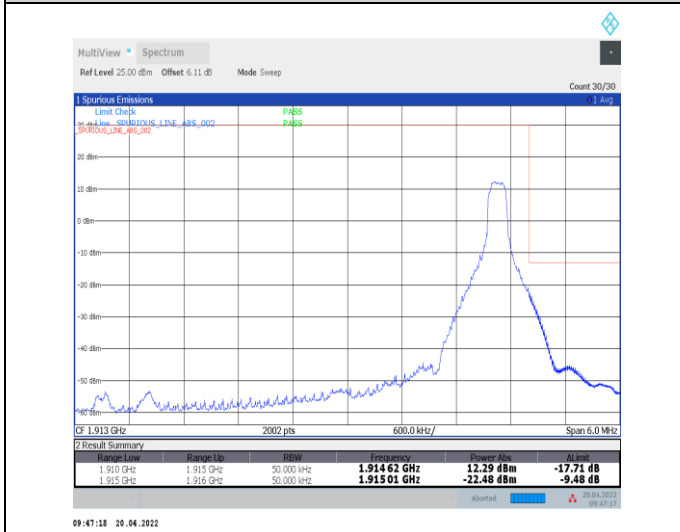
1-N25--15-5-H-5-CP-QPSK-Edge_1RB_Right-1@24-Ant0-seegraph-PASS-see graph
