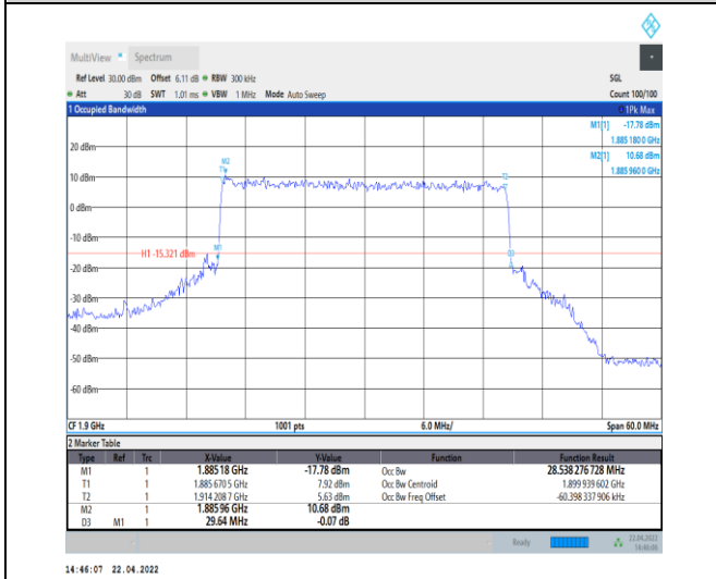
1-N25--15-30-H-6-CP-QPSK-Outer_Full-160@0-Ant 0-28.538-29.640-≤30-PASS
