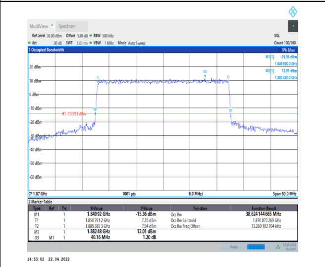
1-N25--15-40-L-6-CP-QPSK-Outer_Full-216@0-Ant0 -38.624-40.160-≤40-PASS
