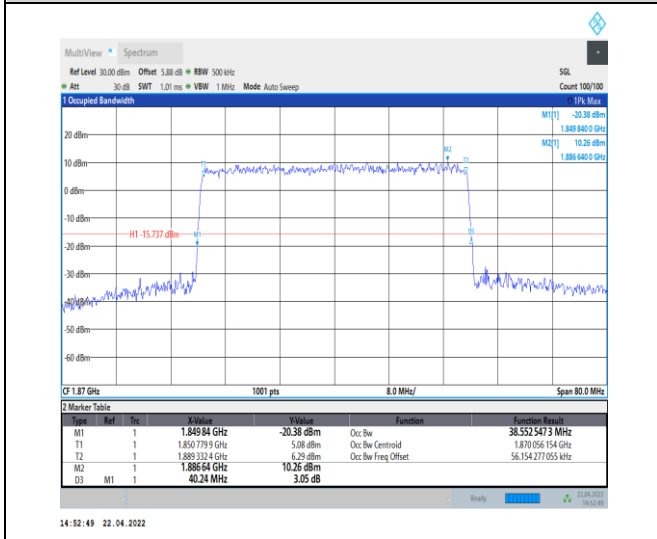
1-N25--15-40-L-5-DFT-256QAM-Outer_Full-216@0-A Ant0-38.553-40.240-≤40-PASS
