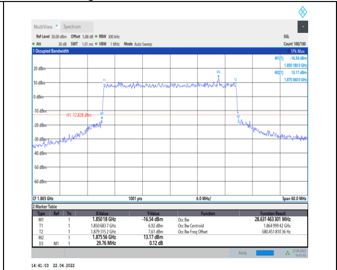
1-N25--15-30-L-7-CP-16QAM-Outer_Full-160@0-Ant0 -28.631-29.760-≤30-PASS
