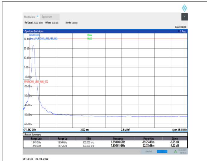
1-N25--15-25-L-1-DFT-PI2BPSK-Edge_1RB_Left-1@0-Ant0-seegraph-PASS-see graph
