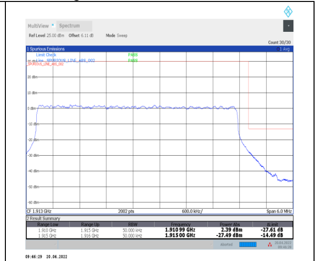
1-N25--15-5-H-3-DFT-PI2BPSK-Outer_Full-25@0-Ant0-seegraph-PASS-see graph
