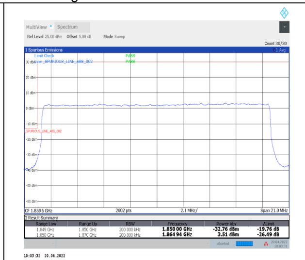
1-N25--15-20-L-3-DFT-PI2BPSK-Outer_Full-100@0-Ant0-seegraph-PASS-see graph
