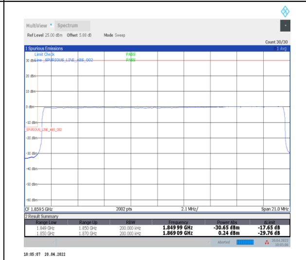
1-N25--15-20-L-6-CP-QPSK-Outer_Full-106@0-Ant0-seegraph-PASS-see graph
