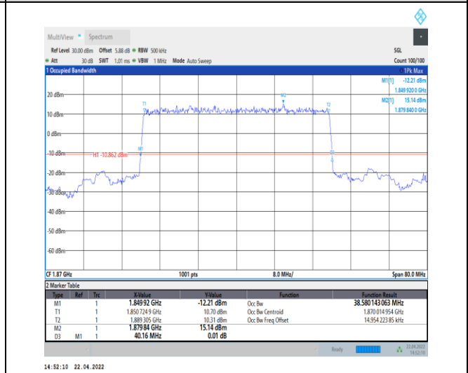
1-N25--15-40-L-2-DFT-PI2BPSK-Outer_Full-216@0-Ant Ant0-38.58-40.160-≤40-PASS
