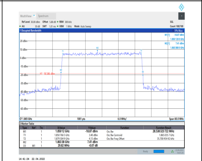
1-N25--15-30-L-9-CP-256QAM-Outer_Full-160@0-Ant0 -28.538-29.820-≤30-PASS
