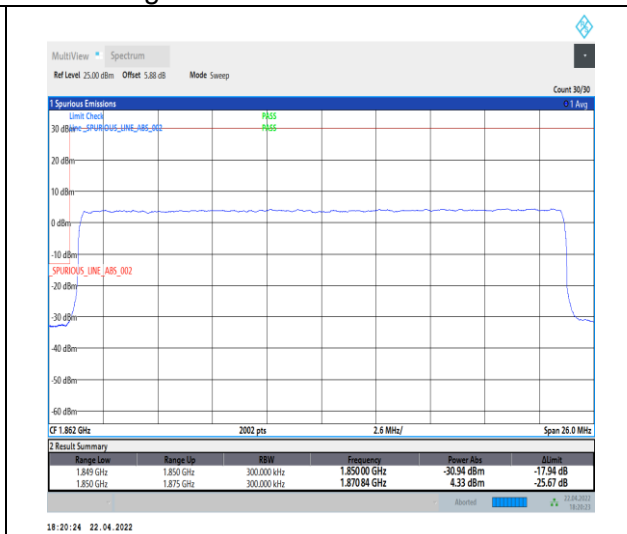
1-N25--15-25-L-3-DFT-PI2BPSK-Outer_Full-128@0-Ant0-seegraph-PASS-see graph
