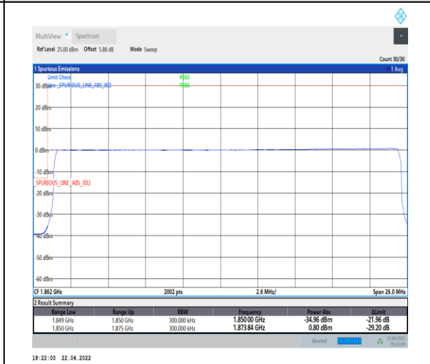
1-N25--15-25-L-6-CP-QPSK-Outer_Full-133@0-Ant0-seegraph-PASS-see graph
