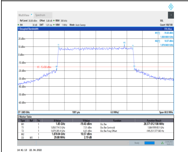
1-N25--15-30-L-8-CP-64QAM-Outer_Full-160@0-Ant0 -28.571-29.880-≤30-PASS
