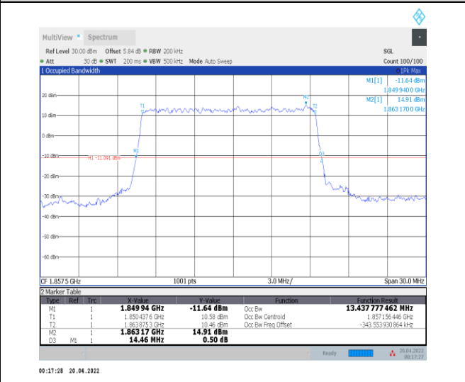
1-N25--15-15-L-2-DFT-PI2BPSK-Outer_Full-75@0-Ant1 -13.438-14.460-≤15-PASS
