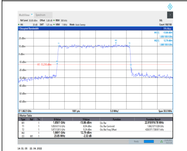
1-N25--15-25-L-3-DFT-16QAM-Outer_Full-128@0-Ant 0-22.919-23.850-≤25-PASS
