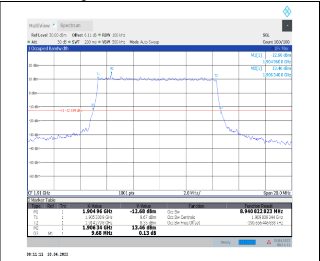
1-N25--15-10-H-1-DFT-QPSK-Outer_Full-50@0-Ant 0-8.941-9.680-≤10-PASS
