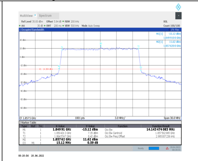
1-N25--15-15-L-8-CP-64QAM-Outer_Full-79@0-Ant 0-14.143-15.120-≤15-PASS
