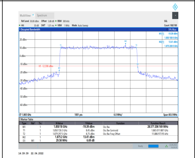
1-N25--15-30-L-1-DFT-QPSK-Outer_Full-160@0-Ant 0-28.571-29.580-≤30-PASS
