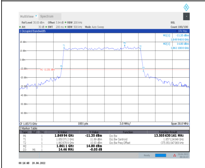
1-N25--15-15-L-1-DFT-QPSK-Outer_Full-75@0-Ant0 -13.506-14.460-≤15-PASS
