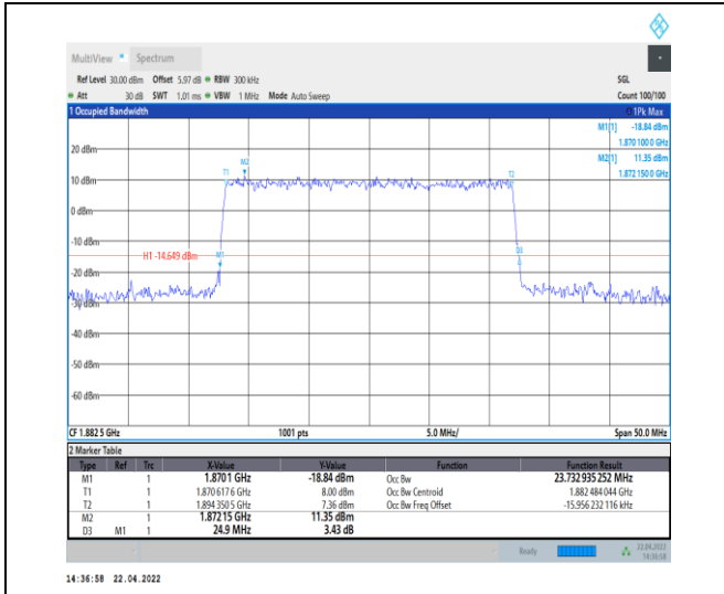
1-N25--15-25-M-8-CP-64QAM-Outer_Full-133@0-A nt0-23.733-24.900-≤25-PASS
