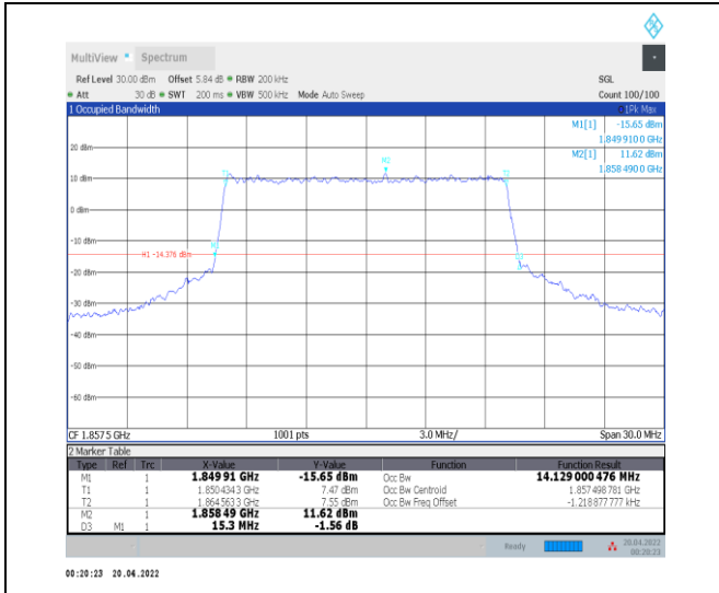
1-N25--15-15-L-7-CP-16QAM-Outer_Full-79@0-Ant 0-14.129-15.300-≤15-PASS
