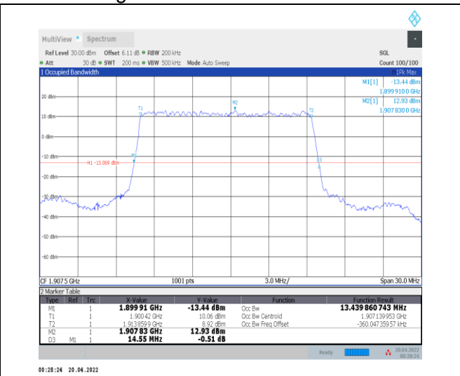
1-N25--15-15-H-2-DFT-PI2BPSK-Outer_Full-75@0-Ant 0-13.44-14.550-≤15-PASS
