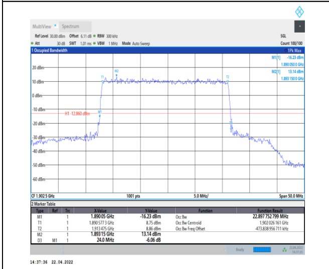
1-N25--15-25-H-1-DFT-QPSK-Outer_Full-128@0-A t0-22.898-24.000-≤25-PASS
