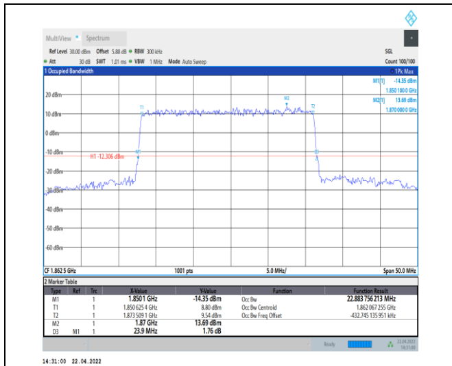
1-N25--15-25-L-1-DFT-QPSK-Outer_Full-128@0-Ant 0-22.884-23.900-≤25-PASS
