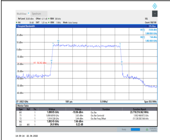
1-N25--15-25-H-9-CP-256QAM-Outer_Full-133@0-A nt0-23.718-24.900-≤25-PASS
