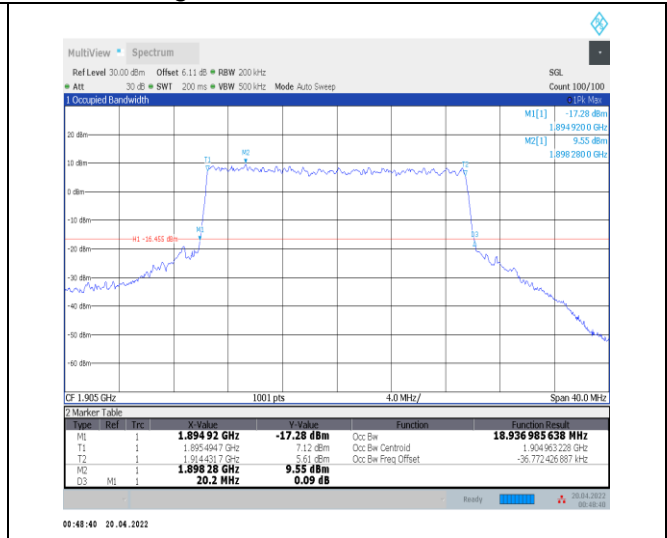
1-N25--15-20-H-7-CP-16QAM-Outer_Full-106@0-Ant t0-18.937-20.200-≤20-PASS
