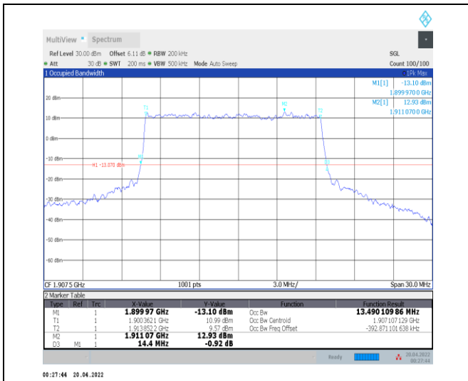
1-N25--15-15-H-1-DFT-QPSK-Outer_Full-75@0-Ant 0-13.49-14.400-≤15-PASS
