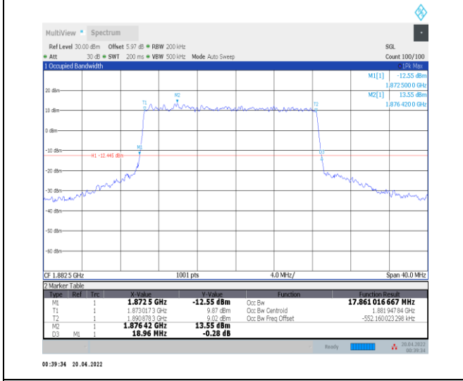
1-N25--15-20-M-1-DFT-QPSK-Outer_Full-100@0-An t0-17.861-18.960-<=20-PASS
