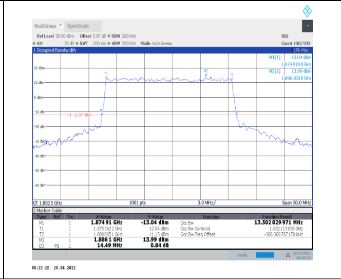
1-N25--15-15-M-1-DFT-QPSK-Outer_Full-75@0-Ant 0-13.503-14.490-≤15-PASS
