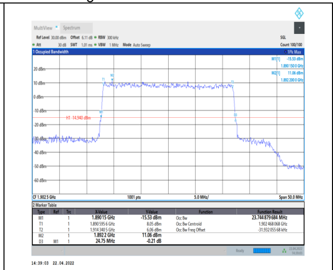
1-N25--15-25-H-8-CP-64QAM-Outer_Full-133@0-An t0-23.745-24.750-≤25-PASS
