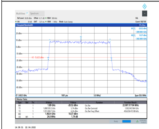
1-N25--15-25-H-5-DFT-256QAM-Outer_Full-128@0-A Ant0-22.902-24.000-<=25-PASS
