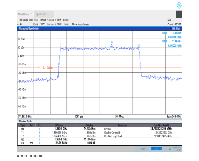
1-N25--15-25-L-8-CP-64QAM-Outer_Full-133@0-An t0-23.769-24.850-<=25-PASS
