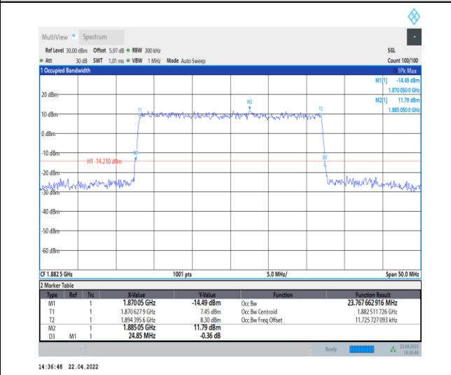
1-N25--15-25-M-7-CP-16QAM-Outer_Full-133@0-A nt0-23.768-24.850-≤25-PASS
