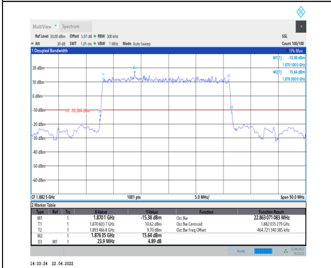
1-N25--15-25-M-2-DFT-PI2BPSK-Outer_Full-128@0 -Ant0-22.863-23.900-≤25-PASS
