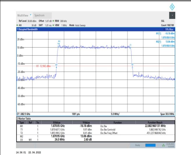
1-N25--15-25-M-3-DFT-16QAM-Outer_Full-128@0-A nt0-22.883-24.000-≤25-PASS
