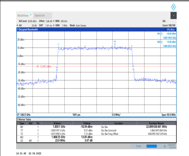
1-N25--15-25-L-4-DFT-64QAM-Outer_Full-128@0-Ant 0-22.899-23.900-≤25-PASS
