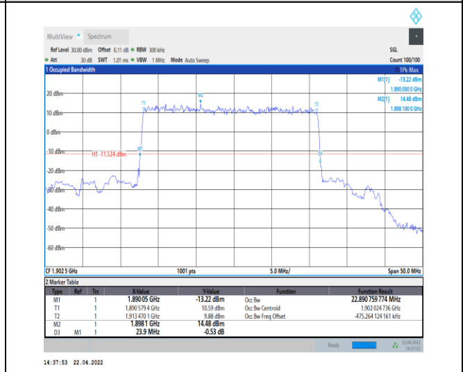
1-N25--15-25-H-2-DFT-PI2BPSK-Outer_Full-128@0-A Ant0-22.891-23.900-≤25-PASS
