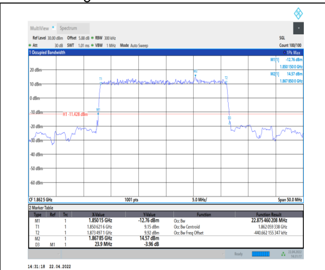
1-N25--15-25-L-2-DFT-PI2BPSK-Outer_Full-128@0-Ant 0-22.875-23.900-≤25-PASS
