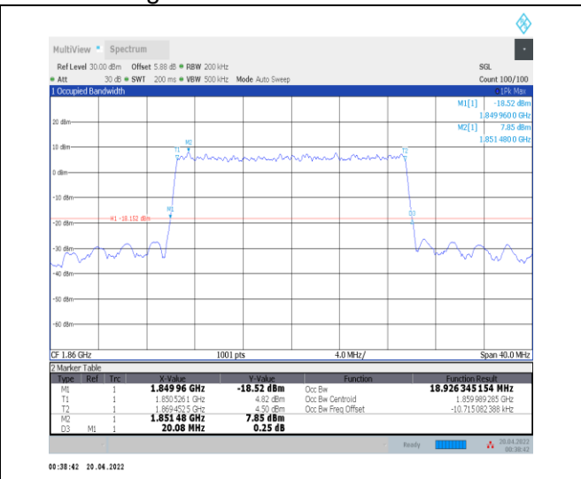
1-N25--15-20-L-9-CP-256QAM-Outer_Full-106@0-A nt0-18.926-20.080-<=20-PASS
