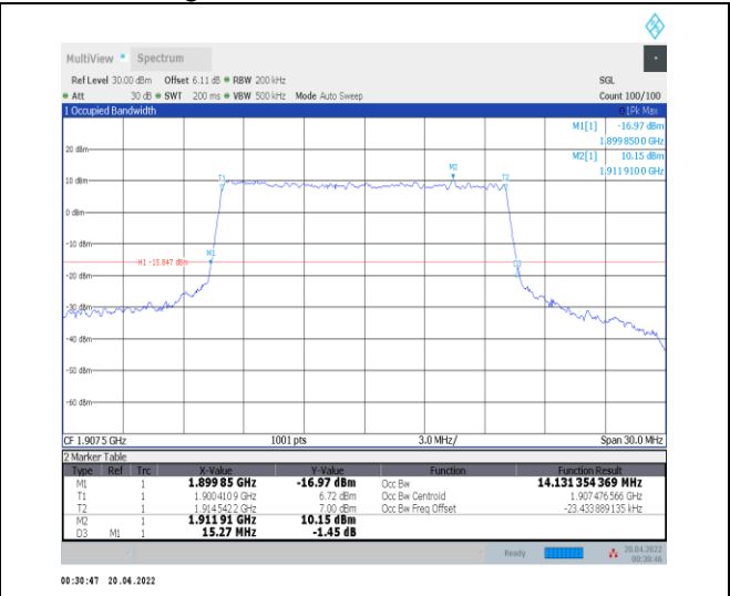
1-N25--15-15-H-6-CP-QPSK-Outer_Full-79@0-Ant0 14.131-15.270-≤15-PASS
