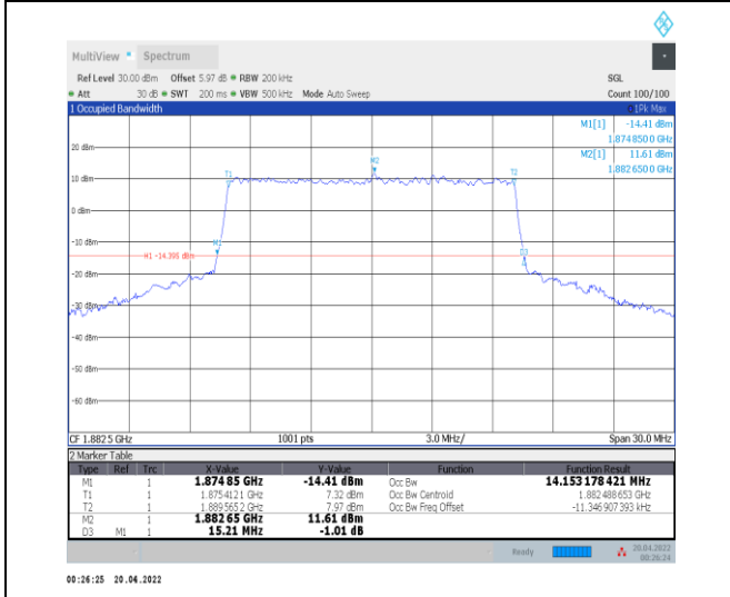
1-N25--15-15-M-8-CP-64QAM-Outer_Full-79@0-Ant0 0-14.153-15.210-≤15-PASS
