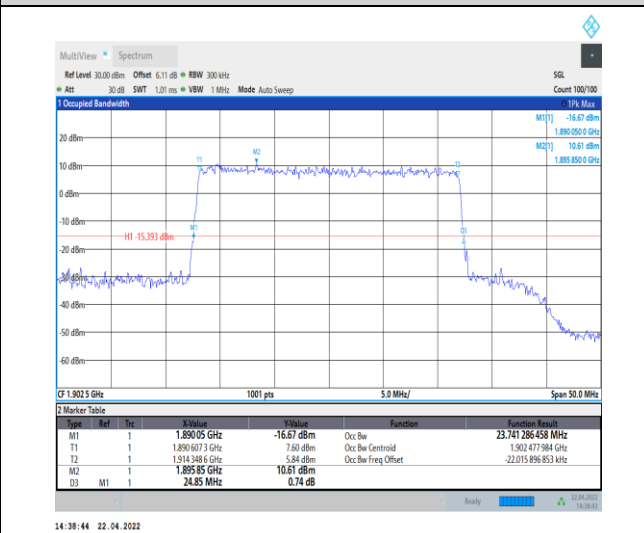
1-N25--15-25-H-6-CP-QPSK-Outer_Full-133@0-Ant 0-23.741-24.850-<=25-PASS
