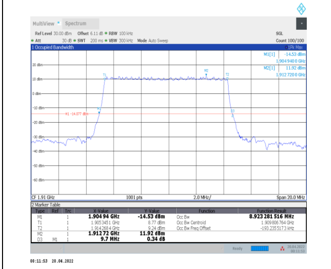
1-N25--15-10-H-2-DFT-PI2BPSK-Outer_Full-50@0-Ant 0-8.923-9.700-≤10-PASS
