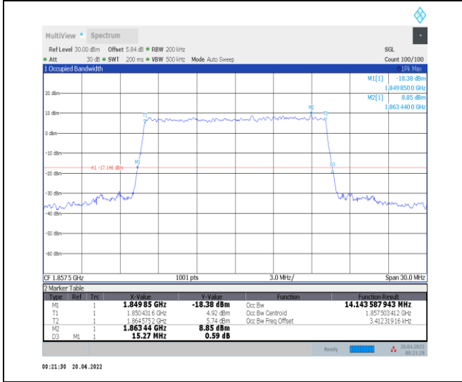
1-N25--15-15-L-9-CP-256QAM-Outer_Full-79@0-Ant t0-14.144-15.270-≤15-PASS
