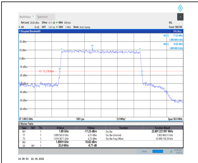
1-N25--15-25-H-7-CP-16QAM-Outer_Full-133@0-An t0-23.801-25.000-≤25-PASS
