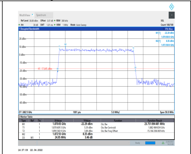
1-N25--15-25-M-9-CP-256QAM-Outer_Full-133@0-A Ant0-23.751-24.950-≤25-PASS
