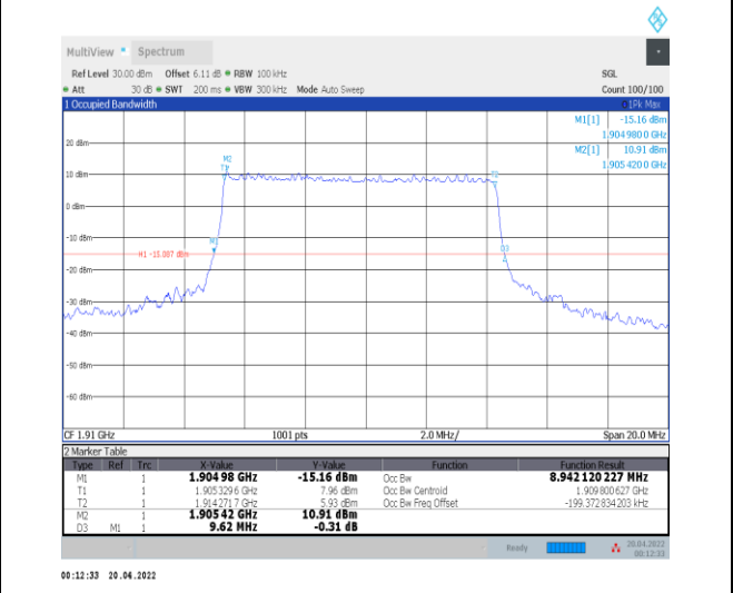
1-N25--15-10-H-3-DFT-16QAM-Outer_Full-50@0-Ant t0-8.942-9.620-≤10-PASS
