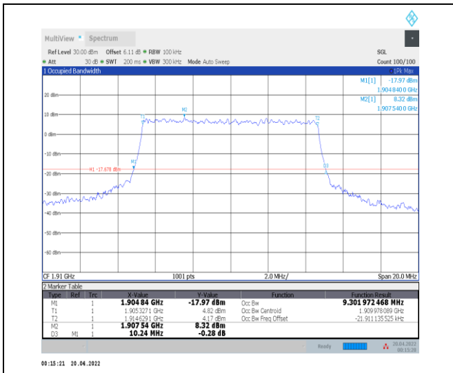
1-N25--15-10-H-8-CP-64QAM-Outer_Full-52@0-Ant 0-9.302-10.240-≤10-PASS
