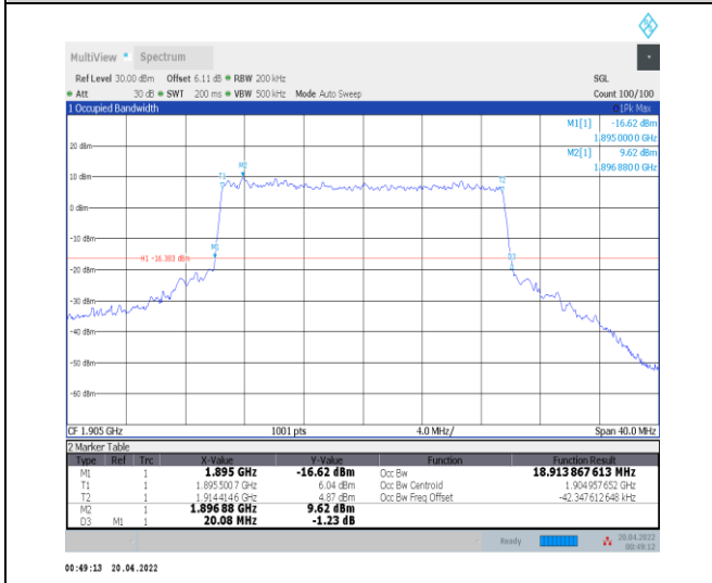
1-N25--15-20-H-8-CP-64QAM-Outer_Full-106@0-Ant t0-18.914-20.080-≤20-PASS
