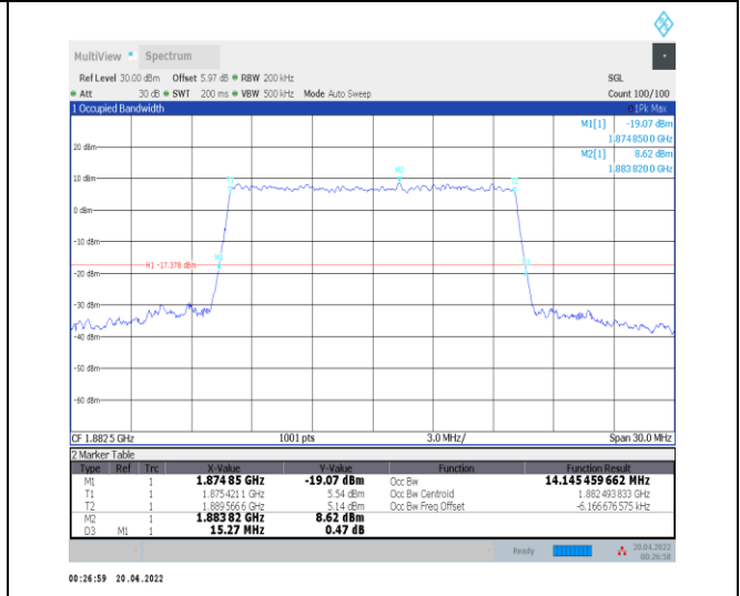
1-N25--15-15-M-9-CP-256QAM-Outer_Full-79@0-Ant0 nt-14.145-15.270-≤15-PASS
