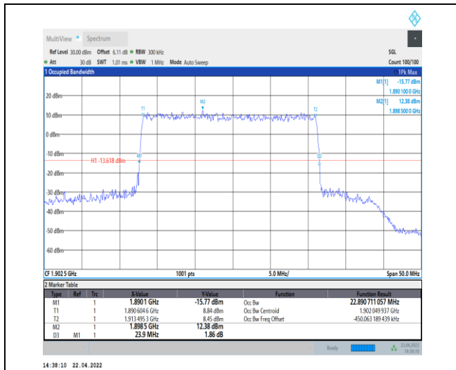
1-N25--15-25-H-3-DFT-16QAM-Outer_Full-128@0-A nt0-22.891-23.900-<=25-PASS
