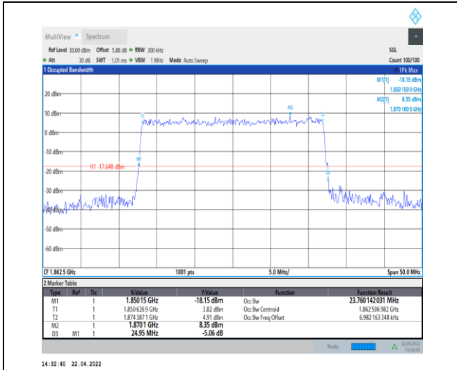
1-N25--15-25-L-9-CP-256QAM-Outer_Full-133@0-A nt0-23.76-24.950-≤25-PASS
