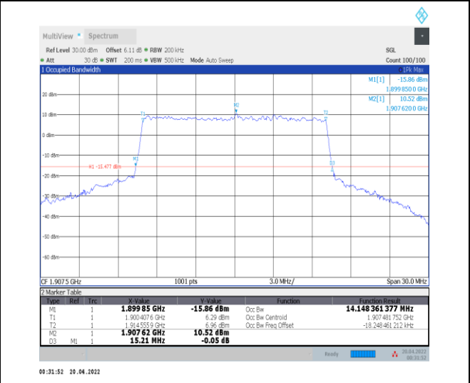
1-N25--15-15-H-8-CP-64QAM-Outer_Full-79@0-Ant 0-14.148-15.210-≤15-PASS
