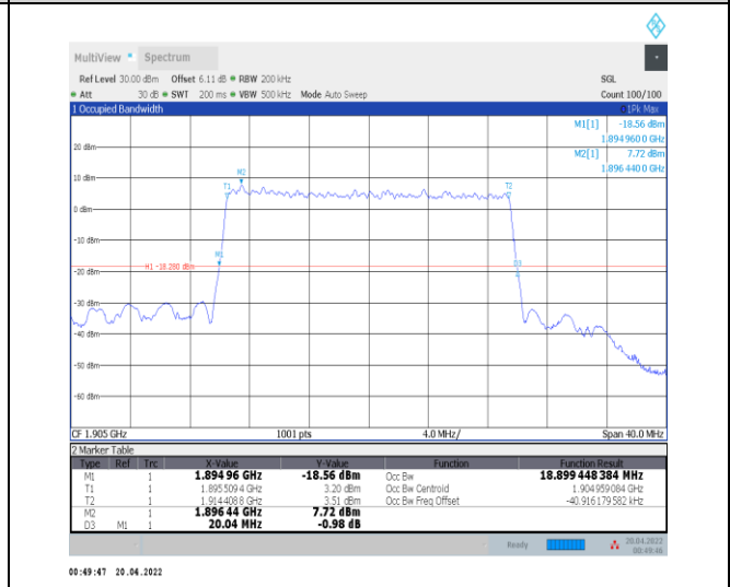
1-N25--15-20-H-9-CP-256QAM-Outer_Full-106@0-Ant nt0-18.899-20.040-≤20-PASS
