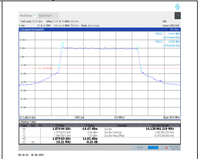
1-N25--15-15-M-7-CP-16QAM-Outer_Full-79@0-Ant0 -14.131-15.210-≤15-PASS
