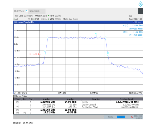
1-N25--15-15-H-4-DFT-64QAM-Outer_Full-75@0-Ant t0-13.427-14.520-≤15-PASS
