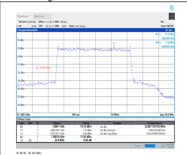
1-N25--15-25-H-4-DFT-64QAM-Outer_Full-128@0-A nt0-22.867-23.900-<=25-PASS
