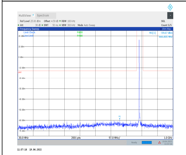
1-N14--15-10-H-1-DFT-PI2BPSK-Inner_1RB_Left-1 @1-30-1000-Ant0--59.67--13-PASS
