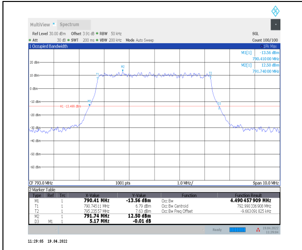
1-N14--15-5-M-4-DFT-64QAM-Outer_Full-25@0-Ant 0-4.49-5.170-<math>\leq</math>5-PASS
