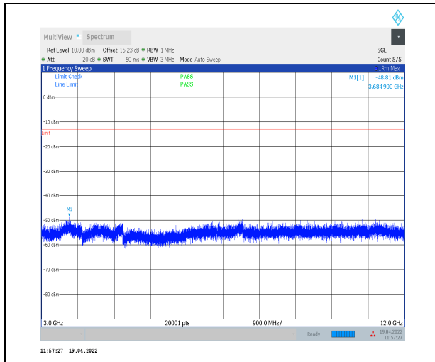
1-N14--15-10-H-1-DFT-PI2BPSK-Inner_1RB_Left-1 @1-3000-12000-Ant0--48.81--13-PASS
