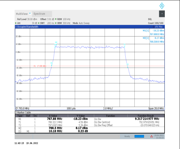
1-N14--15-10-L-9-CP-256QAM-Outer_Full-52@0-Ant 0-9.317-10.180≤10-PASS
