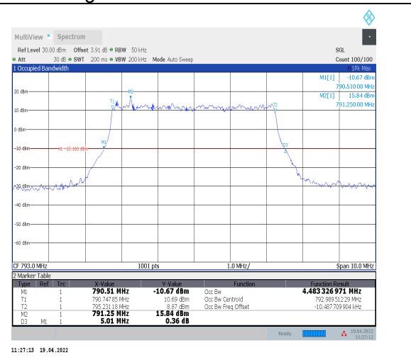
1-N14--15-5-M-1-DFT-QPSK-Outer_Full-25@0-Ant0- 4.483-5.010-≤5-PASS
