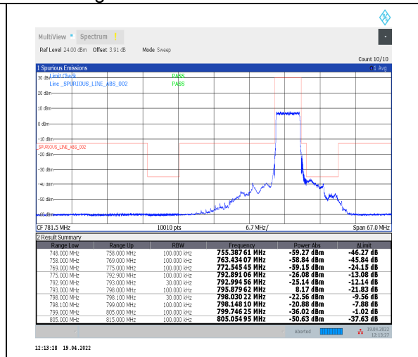
1-N14--15-5-H-3-DFT-PI2BPSK-Outer_Full-25@0 -Ant0-PASS-see graph
