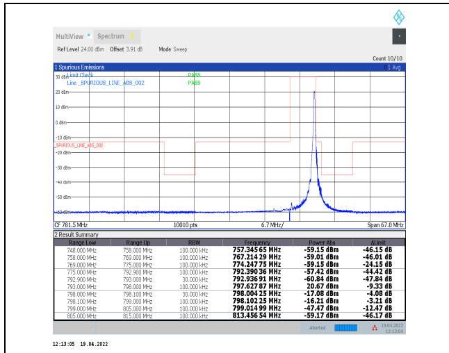
1-N14--15-5-H-2-DFT-PI2BPSK-Edge_1RB_Right-1@2 4-Ant0-PASS-see graph
