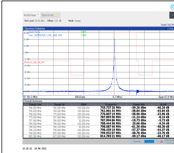
1-N14--15-10-L-1-DFT-PI2BPSK-Edge_1RB_Left-1@0-Ant0-PASS-see graph
