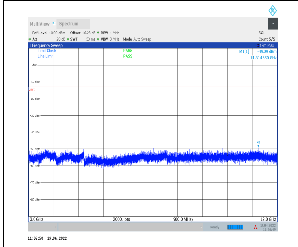
1-N14--15-10-M-1-DFT-PI2BPSK-Inner_1RB_Left-1 @1-3000-12000-Ant0--49.09--13-PASS
