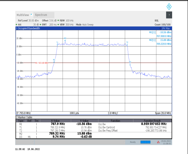
1-N14--15-10-L-1-DFT-QPSK-Outer_Full-50@0-Ant0 -8.96-9.740-≤10-PASS
