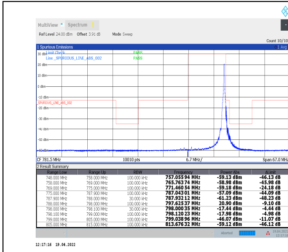
1-N14--15-10-H-2-DFT-PI2BPSK-Edge_1RB_Right-1@51-Ant0-PASS-see graph
