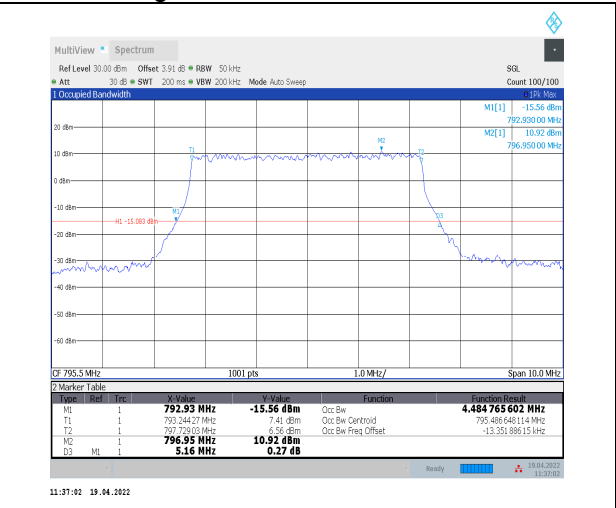
1-N14--15-5-H-8-CP-64QAM-Outer_Full-25@0-Ant0- 4.485-5.160-≤5-PASS
