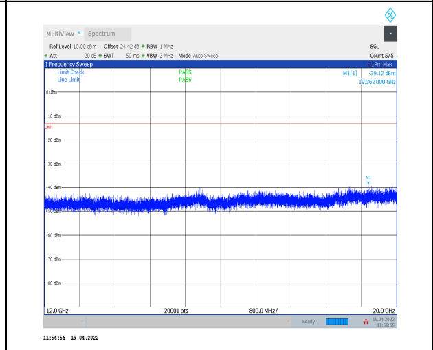
1-N14--15-10-M-1-DFT-PI2BPSK-Inner_1RB_Left-1 @1-12000-20000-Ant0--39.12--13-PASS
