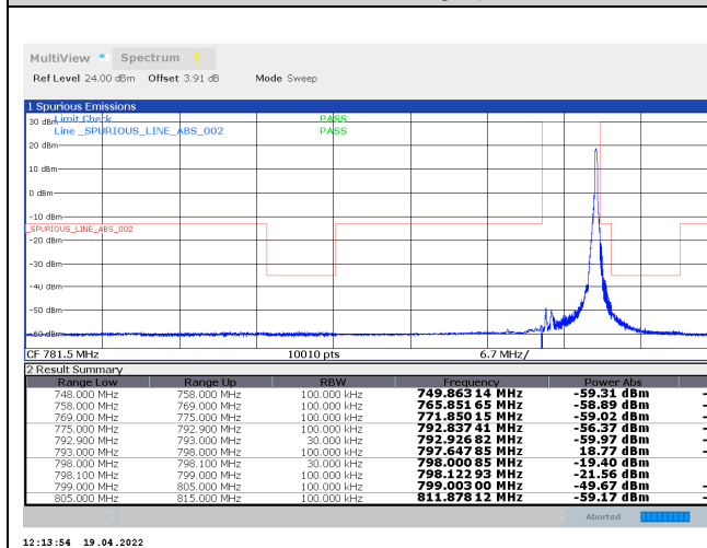
1-N14--15-5-H-5-CP-QPSK-Edge_1RB_Right-1@24-A nt0-PASS-see graph
