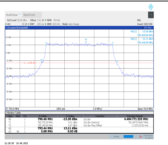
1-N14--15-5-M-3-DFT-16QAM-Outer_Full-25@0-Ant 0-4.485-5.080-≤5-PASS
