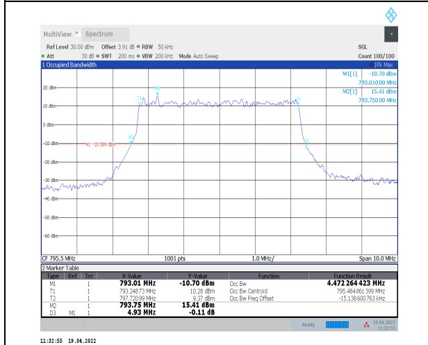
1-N14--15-5-H-1-DFT-QPSK-Outer_Full-25@0-Ant0 4.472-4.930-≤5-PASS
