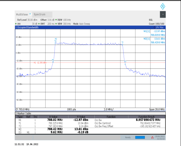
1-N14--15-10-H-3-DFT-16QAM-Outer_Full-50@0-Ant 0-8.958-9.620-<math>\leq 10</math>-PASS
