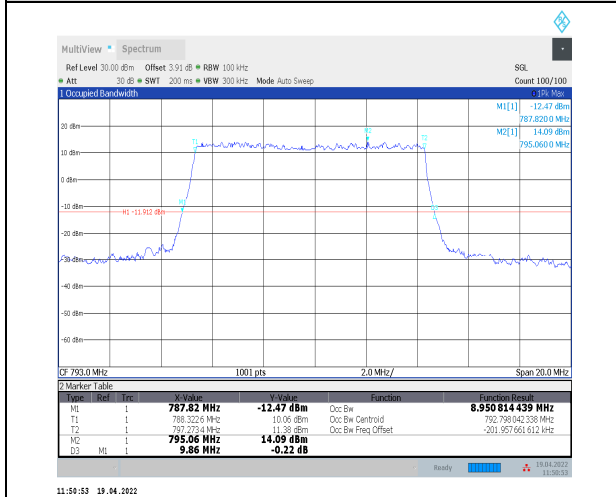
1-N14--15-10-H-2-DFT-PI2BPSK-Outer_Full-50@0- Ant0-8.951-9.860-<math>\leq 10</math>-PASS
