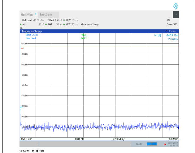
1-N14--15-10-M-1-DFT-PI2BPSK-Inner_1RB_Left-1 @1-0.15-30-Ant0--84.28--23-PASS
