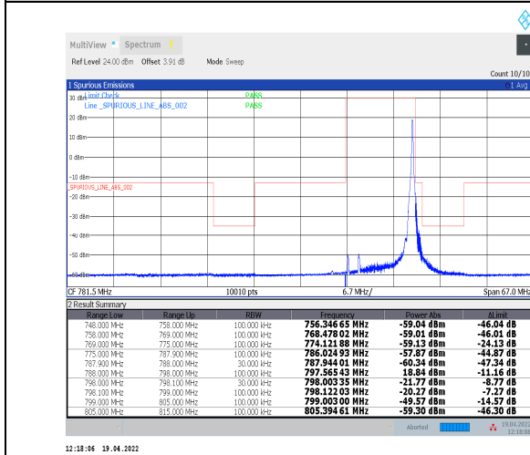
1-N14--15-10-H-5-CP-QPSK-Edge_1RB_Right-1@51-Ant0-PASS-see graph
