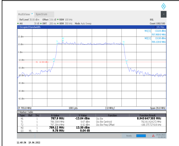
1-N14--15-10-L-4-DFT-64QAM-Outer_Full-50@0-A t0-8.946-9.780≤10-PASS
