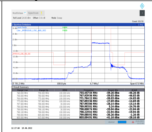
1-N14--15-10-H-3-DFT-PI2BPSK-Outer_Full-50@0-Ant0-PASS-see graph
