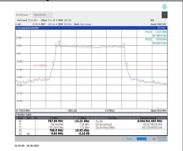
1-N14--15-10-H-5-DFT-256QAM-Outer_Full-50@0-Ant nt0-8.947-9.640-≤10-PASS
