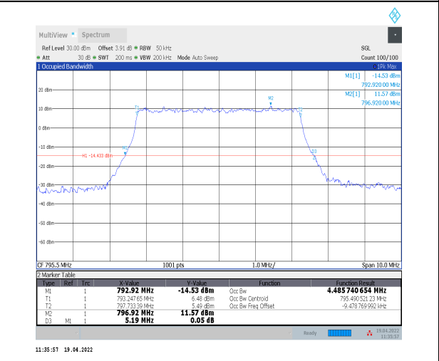
1-N14--15-5-H-6-CP-QPSK-Outer_Full-25@0-Ant0-4 .486-5.190-≤5-PASS
