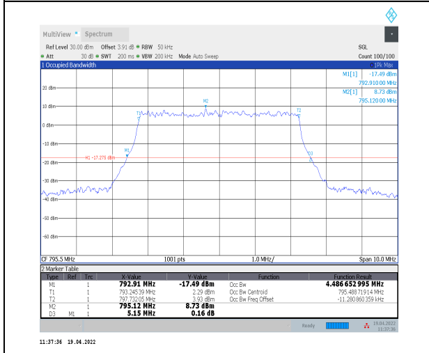
1-N14--15-5-H-9-CP-256QAM-Outer_Full-25@0-Ant 0-4.487-5.150-≤5-PASS
