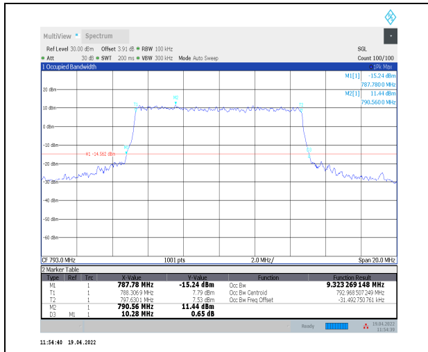
1-N14--15-10-H-8-CP-64QAM-Outer_Full-52@0-An 0-9.323-10.280-≤10-PASS
