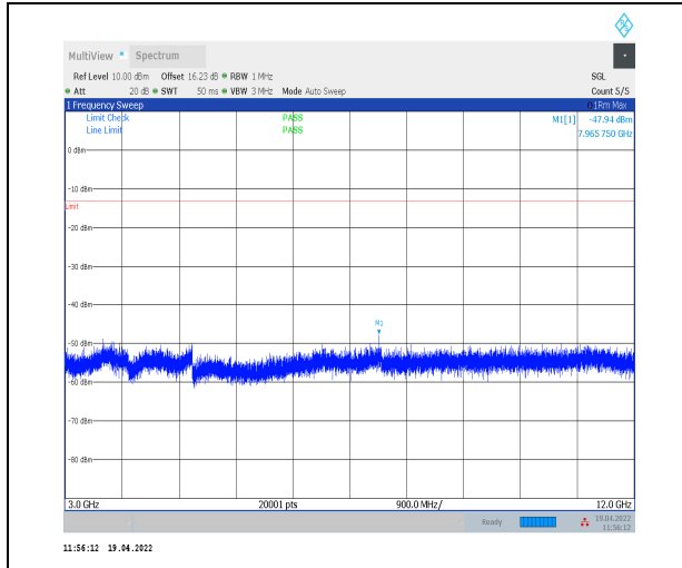
1-N14--15-10-L-1-DFT-PI2BPSK-Inner_1RB_Left-1 @1-3000-12000-Ant0--47.94--13-PASS
