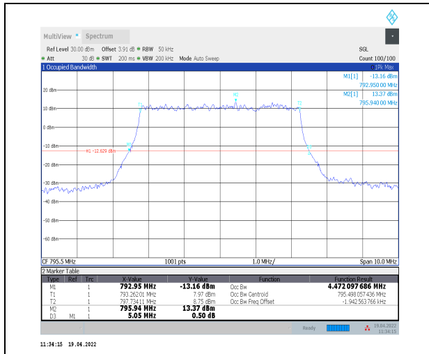
1-N14--15-5-H-3-DFT-16QAM-Outer_Full-25@0-Ant 0-4.472-5.050-≤5-PASS
