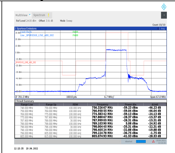
1-N14--15-10-L-3-DFT-PI2BPSK-Outer_Full-50@0-Ant0-PASS-see graph
