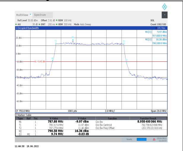
1-N14--15-10-M-2-DFT-PI2BPSK-Outer_Full-50@0-Ant 0-8.958-9.740≤10-PASS
