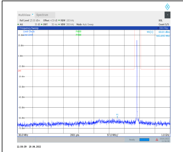
1-N14--15-10-M-1-DFT-PI2BPSK-Inner_1RB_Left-1 @1-30-1000-Ant0--60.01--13-PASS
