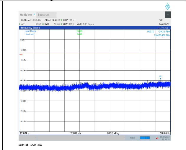
1-N14--15-10-L-1-DFT-PI2BPSK-Inner_1RB_Left-1 @ 1-12000-20000-Ant0--39.22--13-PASS
