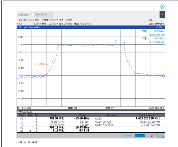
1-N14--15-5-H-7-CP-16QAM-Outer_Full-25@0-Ant0 -4.484-5.160-≤5-PASS
