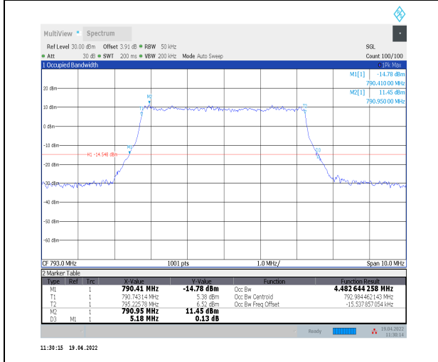
1-N14--15-5-M-6-CP-QPSK-Outer_Full-25@0-Ant0- 4.483-5.180-<math>\leq</math>5-PASS
