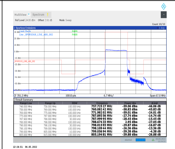
1-N14--15-10-H-6-CP-QPSK-Outer_Full-52@0-Ant0-PASS-see graph
