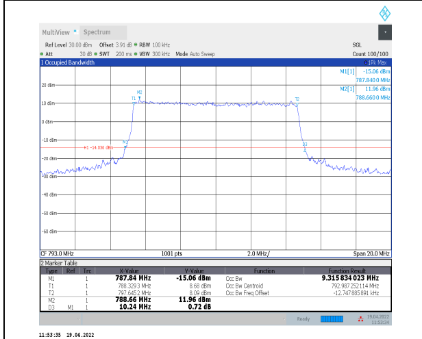
1-N14--15-10-H-6-CP-QPSK-Outer_Full-52@0-Ant0 9.316-10.240-≤10-PASS
