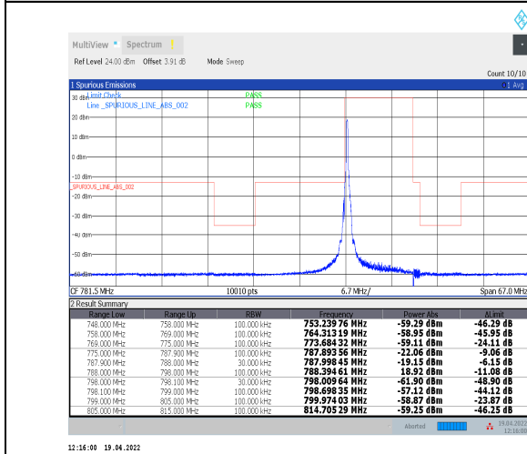
1-N14--15-10-L-4-CP-QPSK-Edge_1RB_Left-1@0-Ant0-PASS-see graph
