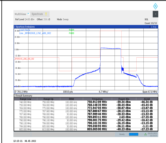
1-N14--15-10-L-6-CP-QPSK-Outer_Full-52@0-Ant0-PASS-see graph
