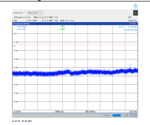
1-N14--15-10-H-1-DFT-PI2BPSK-Inner_1RB_Left-1 @1-12000-20000-Ant0--39.70--13-PASS
