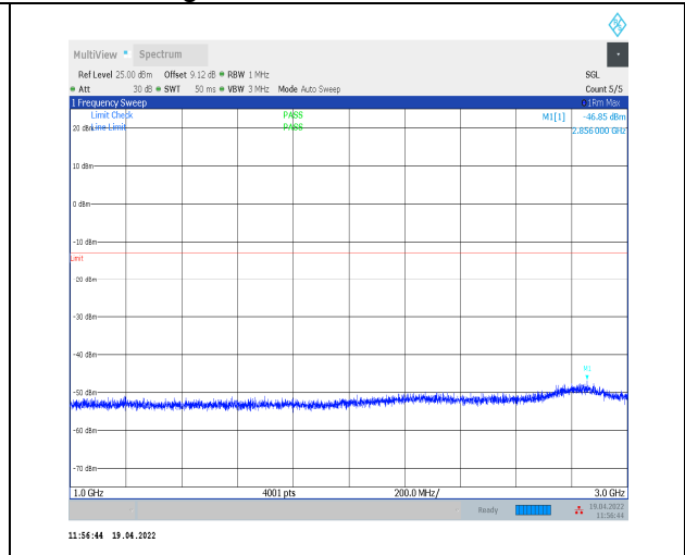
1-N14--15-10-M-1-DFT-PI2BPSK-Inner_1RB_Left-1 @1-1000-3000-Ant0--46.85--13-PASS
