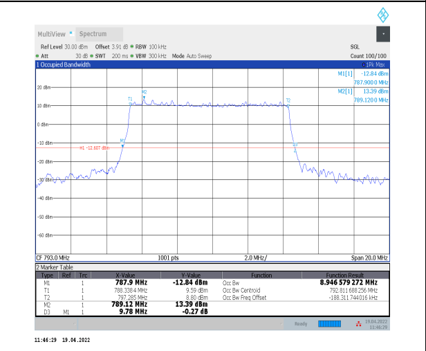
1-N14--15-10-M-4-DFT-64QAM-Outer_Full-50@0-Ant 0-8.947-9.780≤10-PASS
