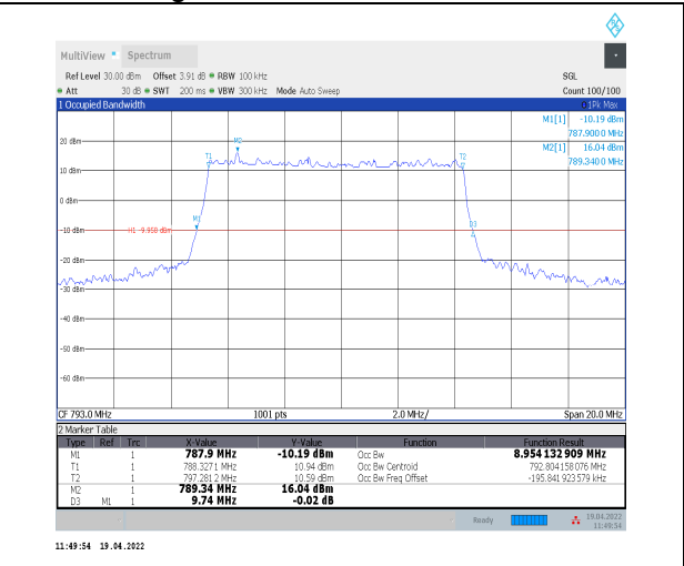
1-N14--15-10-H-1-DFT-QPSK-Outer_Full-50@0-Ant 0-8.954-9.740-<math>\leq 10</math>-PASS
