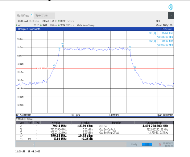
1-N14--15-5-M-5-DFT-256QAM-Outer_Full-25@0-An t0-4.492-5.140-<math>\leq</math>5-PASS
