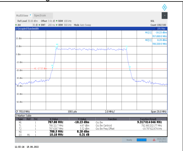
1-N14--15-10-H-9-CP-256QAM-Outer_Full-52@0-An t0-9.317-10.180-≤10-PASS
