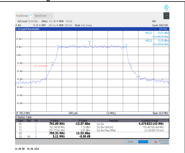
1-N14--15-5-H-4-DFT-64QAM-Outer_Full-25@0-Ant 0-4.476-5.110-≤5-PASS
