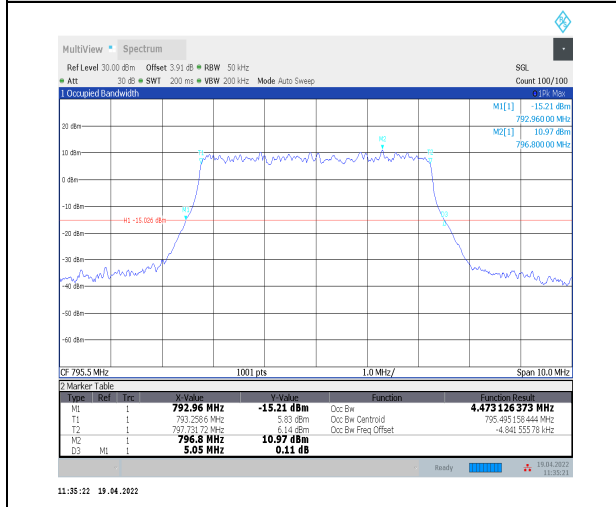
1-N14--15-5-H-5-DFT-256QAM-Outer_Full-25@0-Ant 0-4.473-5.050-≤5-PASS
