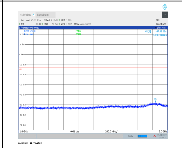
1-N14--15-10-H-1-DFT-PI2BPSK-Inner_1RB_Left-1 @1-1000-3000-Ant0--47.42--13-PASS
