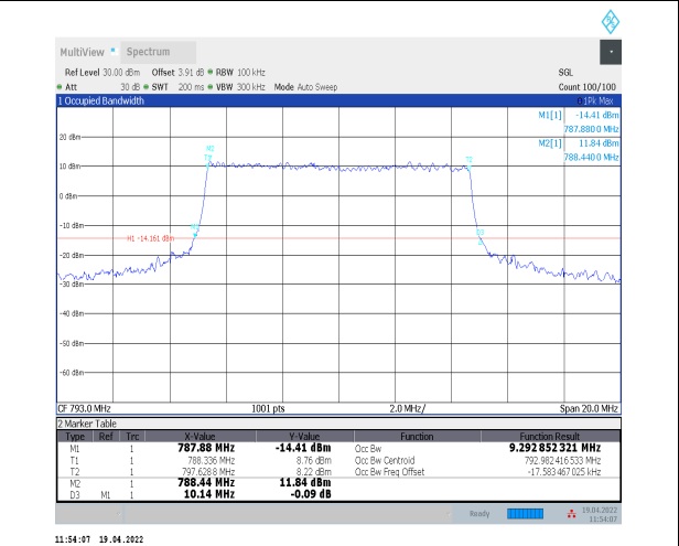
1-N14--15-10-H-7-CP-16QAM-Outer_Full-52@0-Ant 0-9.293-10.140-≤10-PASS
