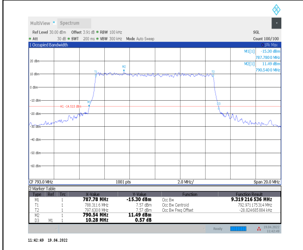
1-N14--15-10-L-8-CP-64QAM-Outer_Full-52@0-Ant 0-9.319-10.280≤10-PASS
