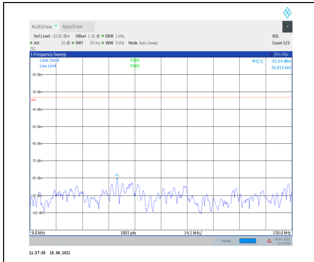
1-N14--15-10-H-1-DFT-PI2BPSK-Inner_1RB_Left-1 @1-0.009-0.15-Ant0--81.64--33-PASS
