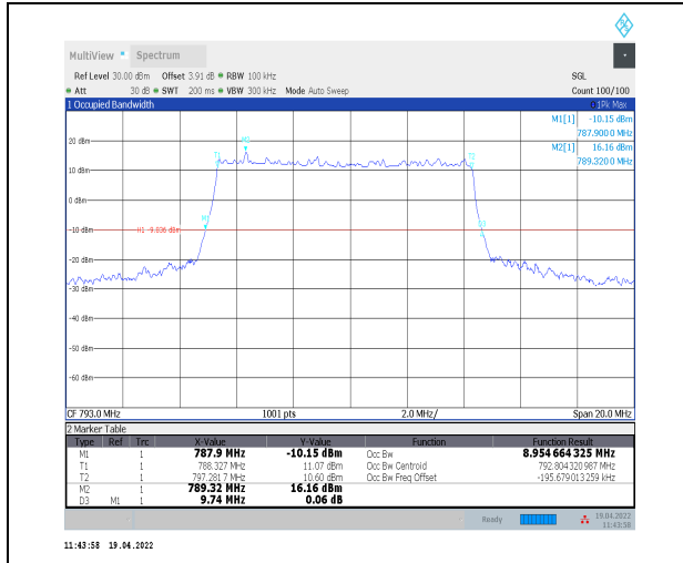
1-N14--15-10-M-1-DFT-QPSK-Outer_Full-50@0-Ant 0-8.955-9.740≤10-PASS
