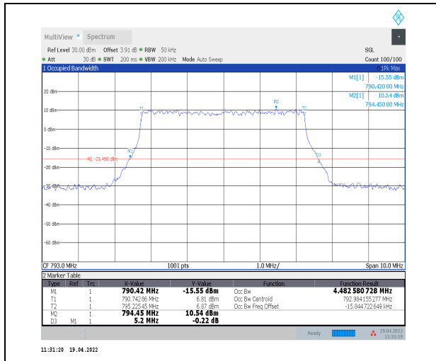
1-N14--15-5-M-8-CP-64QAM-Outer_Full-25@0-Ant0 -4.483-5.200-≤5-PASS
