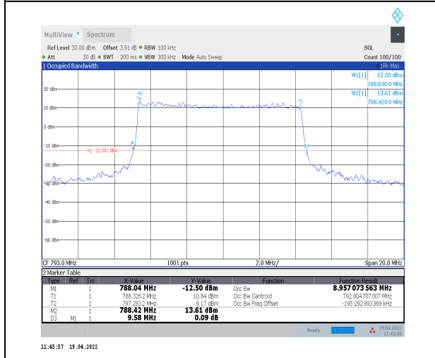
1-N14--15-10-M-3-DFT-16QAM-Outer_Full-50@0-Ant 0-8.957-9.580≤10-PASS
