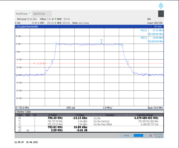
1-N14--15-5-M-7-CP-16QAM-Outer_Full-25@0-Ant0- -4.479-5.090-<math>\leq</math>5-PASS
