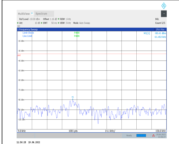
1-N14--15-10-M-1-DFT-PI2BPSK-Inner_1RB_Left-1 @1-0.009-0.15-Ant0--80.41--33-PASS
