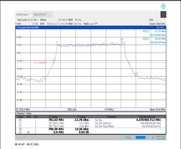
1-N13--15-5-H-2-DFT-PI2BPSK-Outer_Full-25@0-Ant0 -4.479-5.000-≤5-PASS
