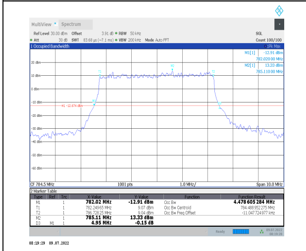
1-N13--15-5-H-1-DFT-QPSK-Outer_Full-25@0-Ant0 4.479-4.950-≤5-PASS
