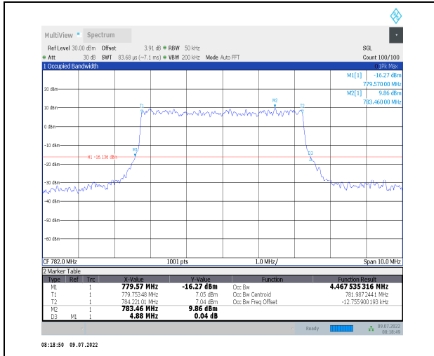
1-N13--15-5-M-8-CP-64QAM-Outer_Full-25@0-Ant0 -4.468-4.880-≤5-PASS
