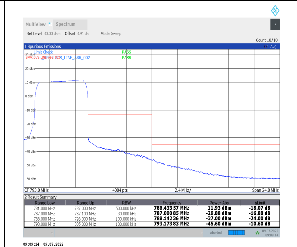
1-N13-PC3-15-5-H-6-CP-QPSK-Outer_Full-25@0-Ant0-PASS-see graph
