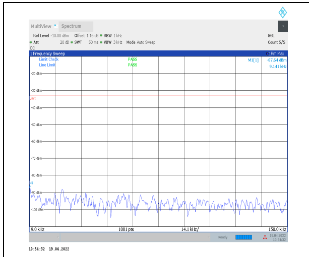
1-N12--15-15-H-1-DFT-PI2BPSK-Inner_1RB_Left-1 @1-0.009-0.15-Ant0--87.64--33-PASS
