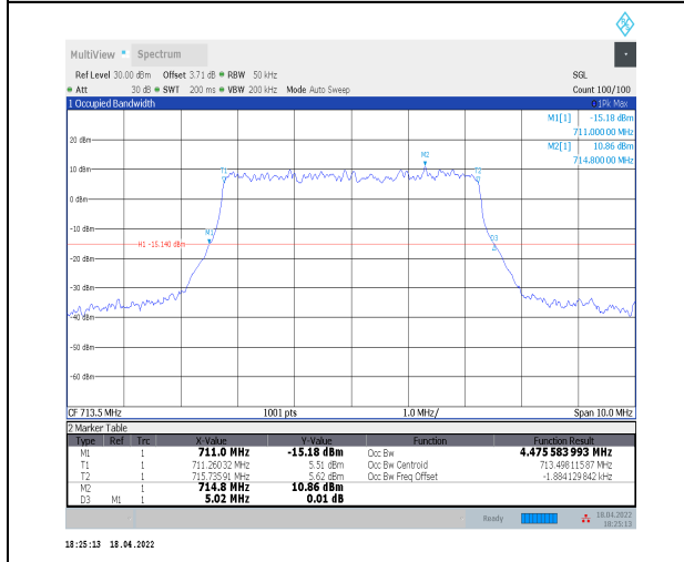
1-N12--15-5-H-5-DFT-256QAM-Outer_Full-25@0-Ant t0-4.476-5.020-<math>\leq</math>5-PASS
