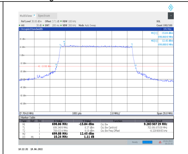
1-N12--15-10-L-7-CP-16QAM-Outer_Full-52@0-Ant 0-9.284-10.240≤10-PASS
