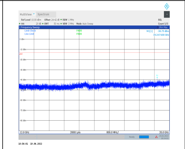
1-N12--15-15-M-1-DFT-PI2BPSK-Inner_1RB_Left-1 @1-12000-20000-Ant0--38.79--13-PASS
