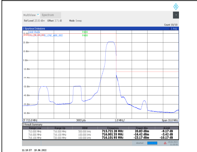
1-N12--15-5-H-5-CP-QPSK-Edge_1RB_Right-1@24-A nt0-PASS-see graph
