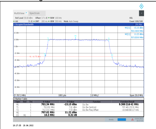
1-N12--15-10-M-6-CP-QPSK-Outer_Full-52@0-Ant0 -9.3-10.300-≤10-PASS
