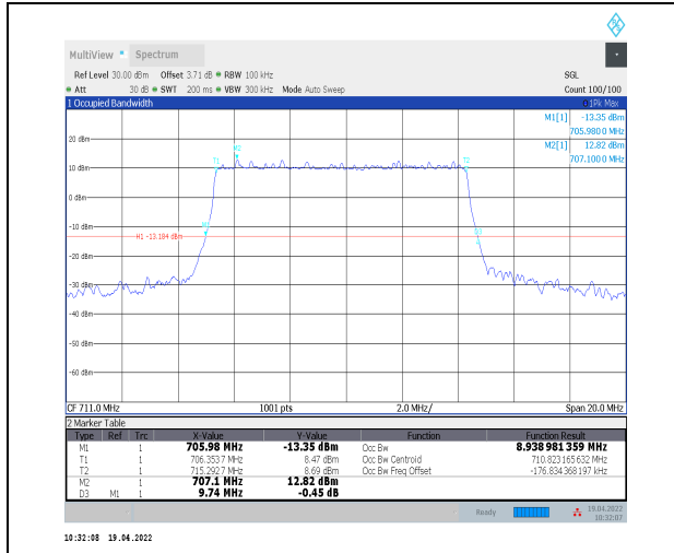
1-N12--15-10-H-4-DFT-64QAM-Outer_Full-50@0-Ant t0-8.939-9.740-≤10-PASS
