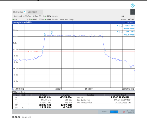
1-N12--15-15-H-6-CP-QPSK-Outer_Full-79@0-Ant0- 14.124-15.270-<=15-PASS
