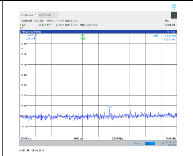
1-N12--15-15-M-1-DFT-PI2BPSK-Inner_1RB_Left-1 @1-0.15-30-Ant0--84.35--23-PASS
