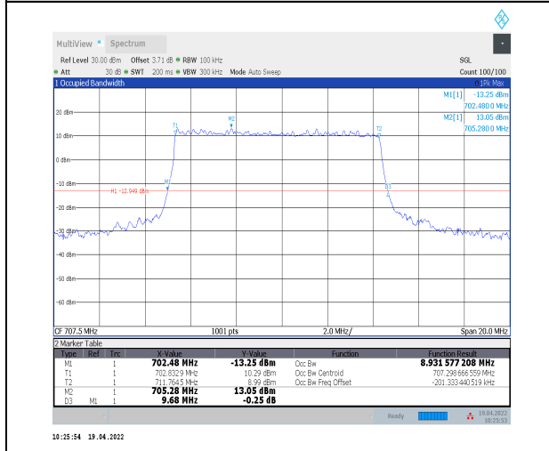
1-N12--15-10-M-3-DFT-16QAM-Outer_Full-50@0-Ant t0-8.932-9.680-<=10-PASS
