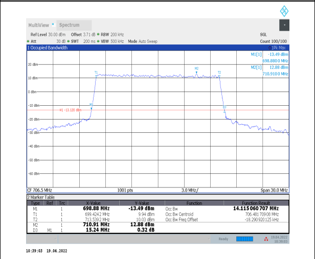
1-N12--15-15-L-6-CP-QPSK-Outer_Full-79@0-Ant0 14.115-15.240≤15-PASS
