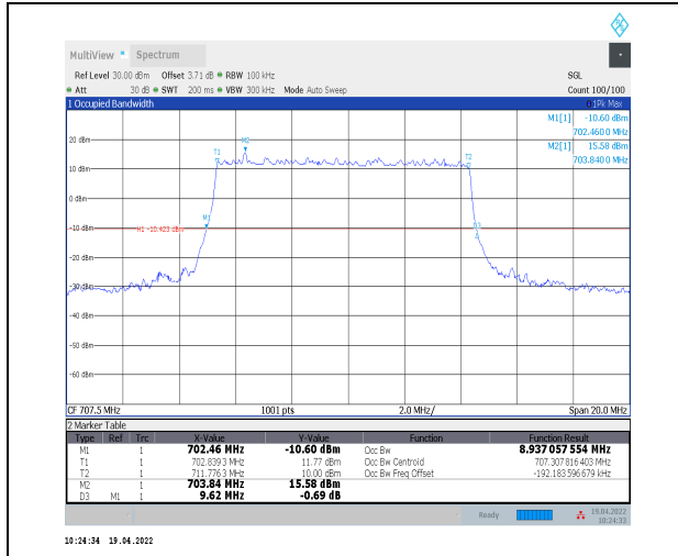
1-N12--15-10-M-1-DFT-QPSK-Outer_Full-50@0-Ant 0-8.937-9.620-<=10-PASS
