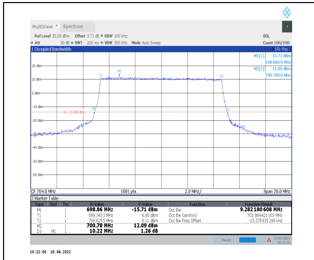
1-N12--15-10-L-6-CP-QPSK-Outer_Full-52@0-Ant0 9.282-10.220≤10-PASS
