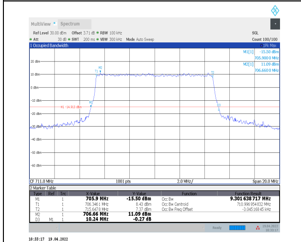
1-N12--15-10-H-6-CP-QPSK-Outer_Full-52@0-Ant0 9.302-10.240-≤10-PASS
