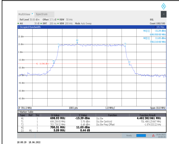
1-N12--15-5-L-7-CP-16QAM-Outer_Full-25@0-Ant0- 4.482-5.090-<math>\leq</math>5-PASS
