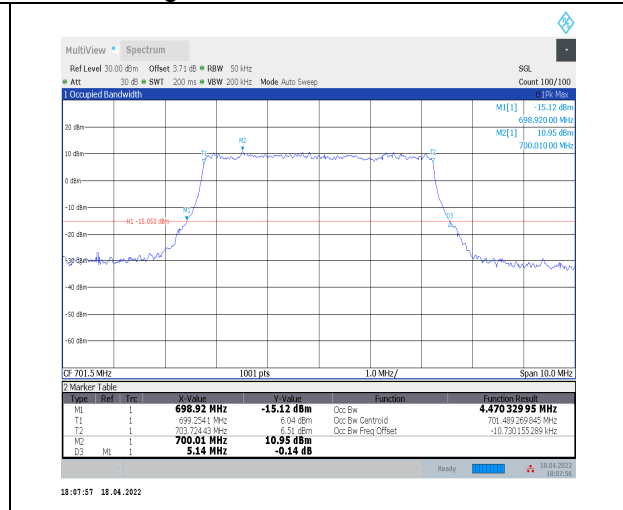
1-N12--15-5-L-6-CP-QPSK-Outer_Full-25@0-Ant0-4 .47-5.140-<math>\leq</math>5-PASS
