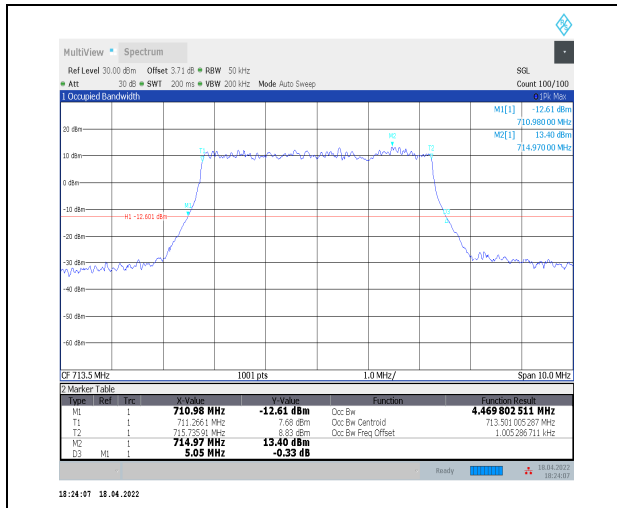
1-N12--15-5-H-3-DFT-16QAM-Outer_Full-25@0-Ant 0-4.47-5.050-<math>\leq</math>5-PASS
