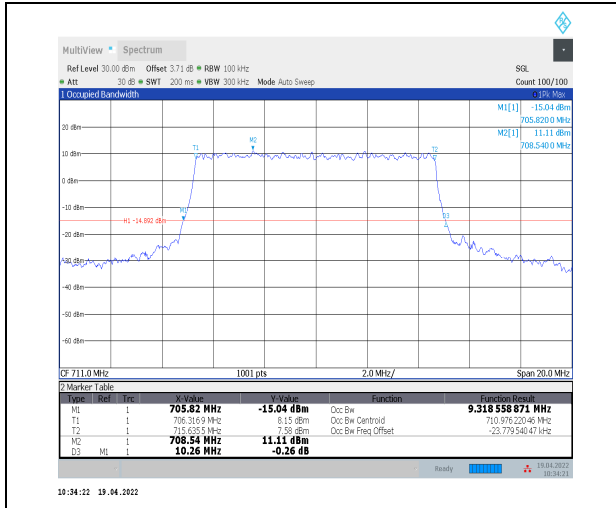
1-N12--15-10-H-8-CP-64QAM-Outer_Full-52@0-Ant 0-9.319-10.260-≤10-PASS
