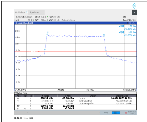
1-N12--15-15-L-7-CP-16QAM-Outer_Full-79@0-Ant0 -14.096-15.090≤15-PASS
