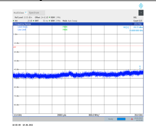
1-N12--15-15-H-1-DFT-PI2BPSK-Inner_1RB_Left-1 @1-12000-20000-Ant0--39.72--13-PASS
