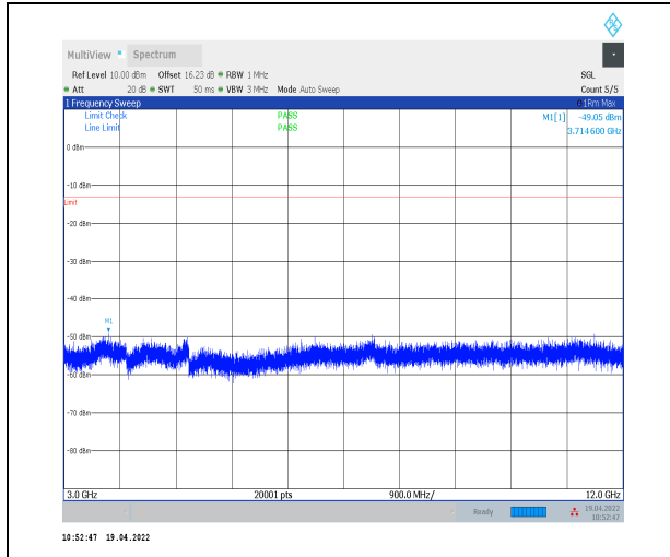
1-N12--15-15-L-1-DFT-PI2BPSK-Inner_1RB_Left-1 @1-3000-12000-Ant0--49.05--13-PASS
