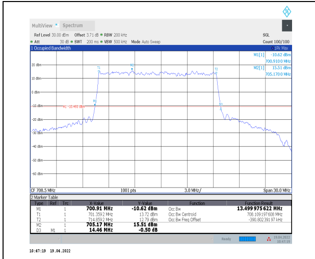
1-N12--15-15-H-1-DFT-QPSK-Outer_Full-75@0-Ant 0-13.5-14.460≤15-PASS
