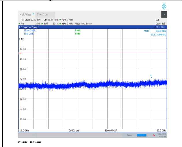
1-N12--15-15-L-1-DFT-PI2BPSK-Inner_1RB_Left-1@ 1-12000-20000-Ant0--39.83--13-PASS
