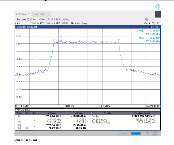
1-N12--15-10-H-1-DFT-QPSK-Outer_Full-50@0-Ant 0-8.943-9.720-<=10-PASS
