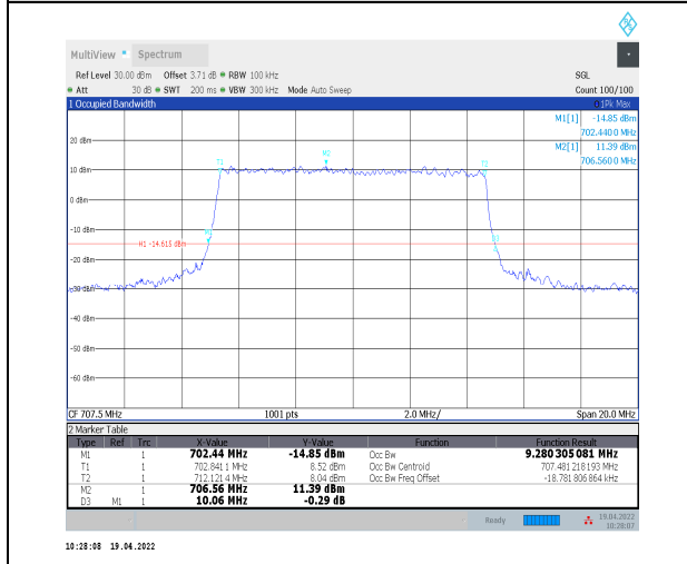
1-N12--15-10-M-7-CP-16QAM-Outer_Full-52@0-Ant 0-9.28-10.060-≤10-PASS
