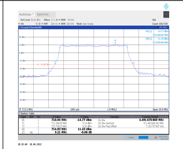
1-N12--15-5-H-6-CP-QPSK-Outer_Full-25@0-Ant0-4 .492-5.210-<math>\leq</math>5-PASS
