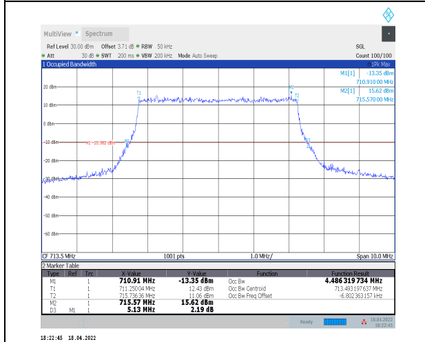
1-N12--15-5-H-1-DFT-QPSK-Outer_Full-25@0-Ant0 4.486-5.130-≤5-PASS
