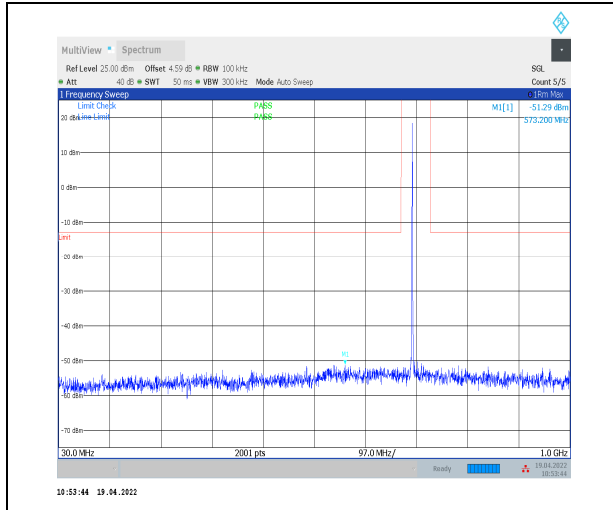
1-N12--15-15-M-1-DFT-PI2BPSK-Inner_1RB_Left-1 @1-30-1000-Ant0--51.29--13-PASS
