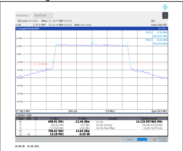
1-N12--15-15-L-8-CP-64QAM-Outer_Full-79@0-Ant 0-14.135-15.180≤15-PASS
