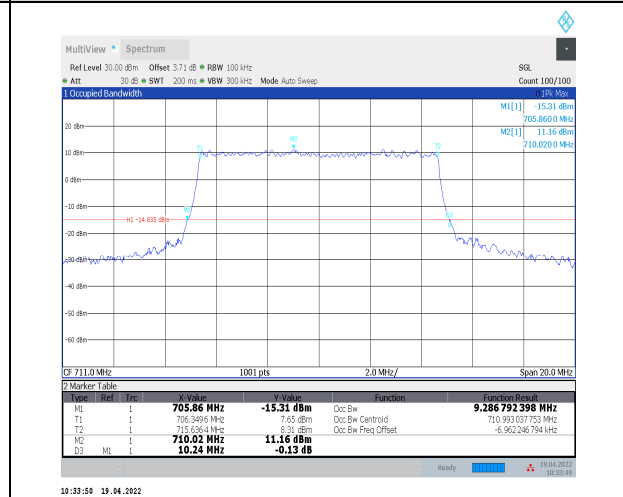
1-N12--15-10-H-7-CP-16QAM-Outer_Full-52@0-Ant 0-9.287-10.240-≤10-PASS
