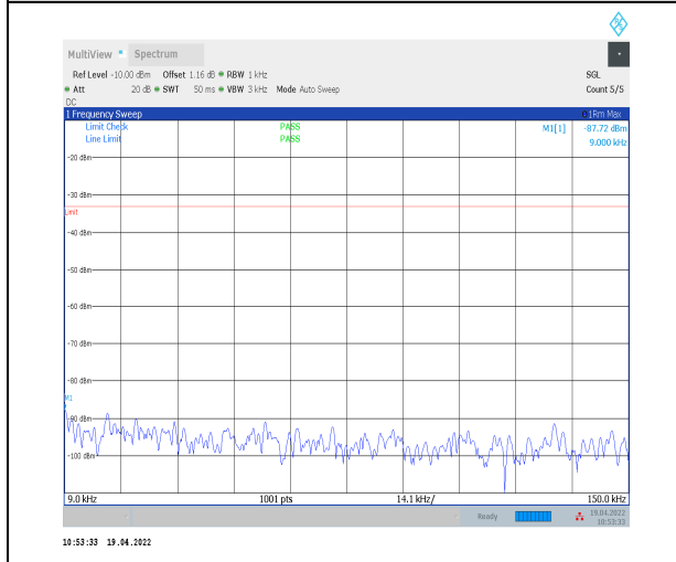
1-N12--15-15-M-1-DFT-PI2BPSK-Inner_1RB_Left-1 @1-0.009-0.15-Ant0--87.72--33-PASS
