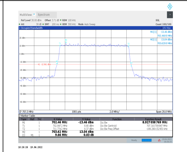
1-N12--15-10-M-4-DFT-64QAM-Outer_Full-50@0-A nt0-8.927-9.660-<=10-PASS
