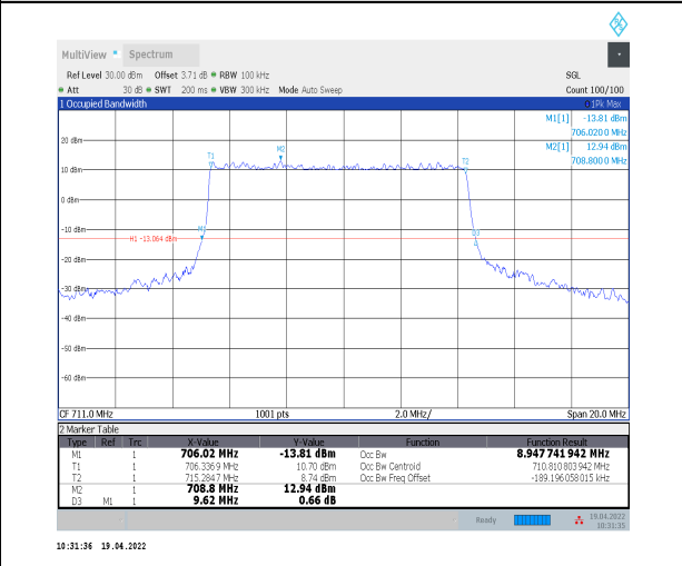
1-N12--15-10-H-3-DFT-16QAM-Outer_Full-50@0-Ant t0-8.948-9.620-<=10-PASS
