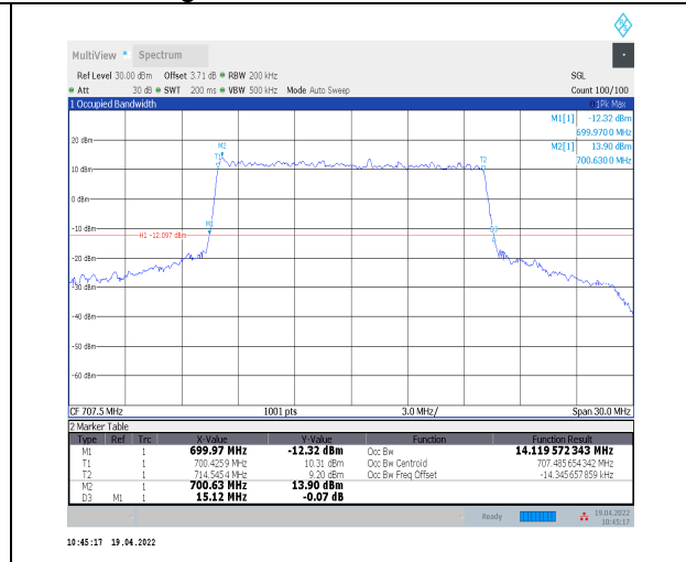
1-N12--15-15-M-7-CP-16QAM-Outer_Full-79@0-Ant0-0-14.12-15.120-≤15-PASS
