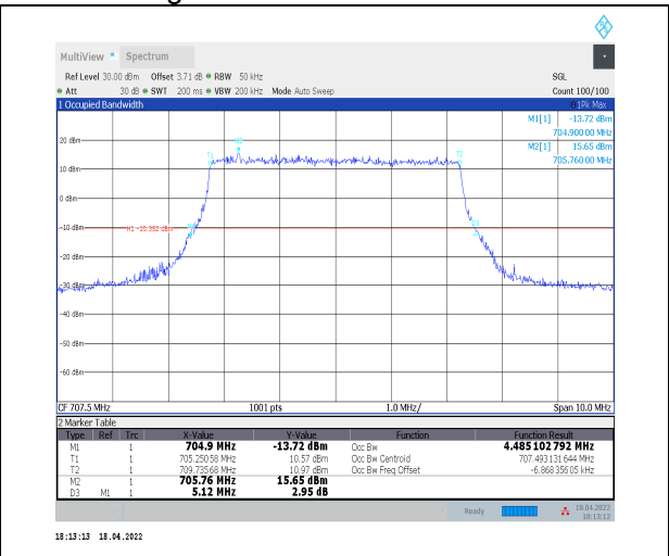
1-N12--15-5-M-1-DFT-QPSK-Outer_Full-25@0-Ant0 -4.485-5.120≤5-PASS
