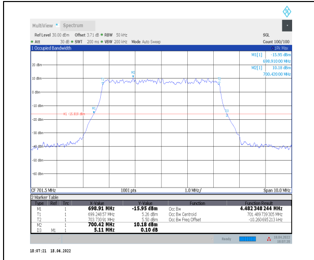
1-N12--15-5-L-5-DFT-256QAM-Outer_Full-25@0-Ant 0-4.482-5.110-<math>\leq</math>5-PASS
