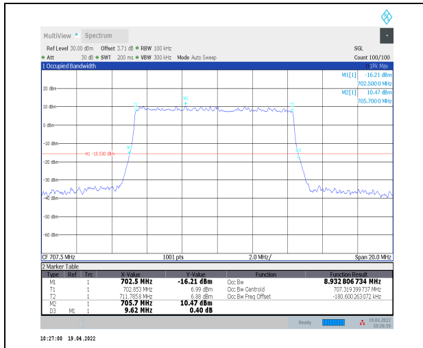
1-N12--15-10-M-5-DFT-256QAM-Outer_Full-50@0-A nt0-8.933-9.620-≤10-PASS
