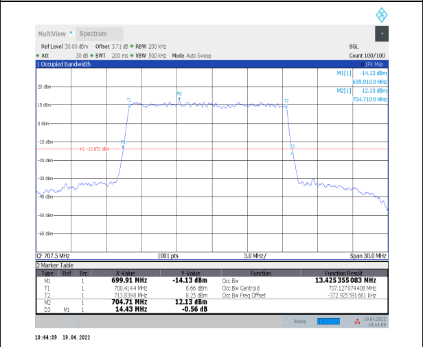
1-N12--15-15-M-5-DFT-256QAM-Outer_Full-75@0-Ant0-13.425-14.430-≤15-PASS
