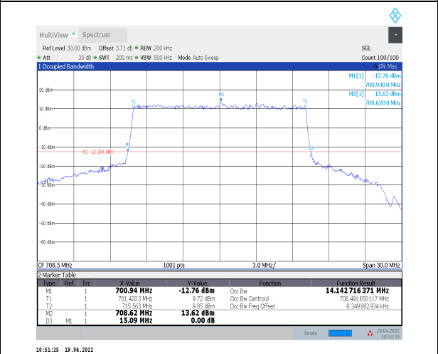
1-N12--15-15-H-8-CP-64QAM-Outer_Full-79@0-Ant 0-14.143-15.090-<=15-PASS
