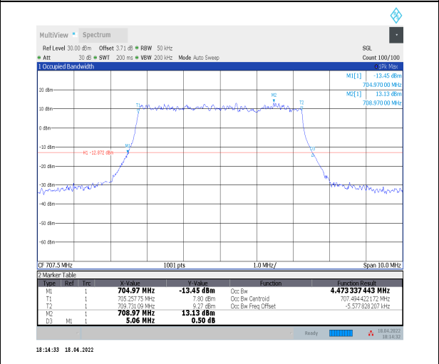
1-N12--15-5-M-3-DFT-16QAM-Outer_Full-25@0-Ant 0-4.473-5.060≤5-PASS
