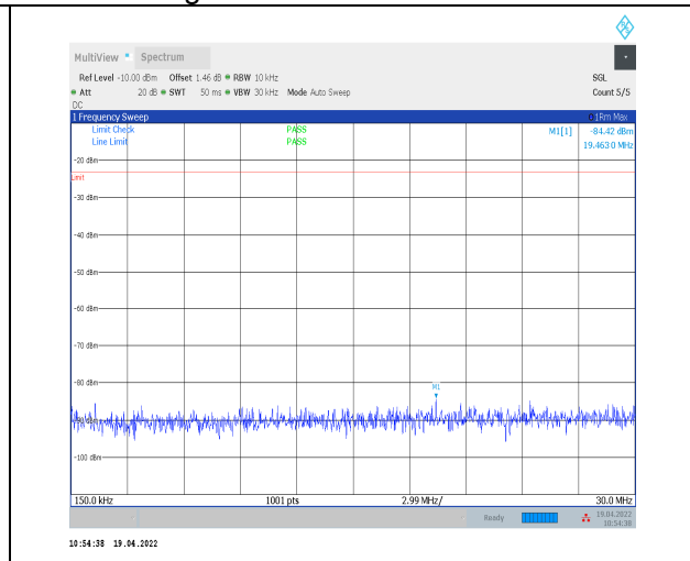
1-N12--15-15-H-1-DFT-PI2BPSK-Inner_1RB_Left-1 @1-0.15-30-Ant0--84.42--23-PASS
