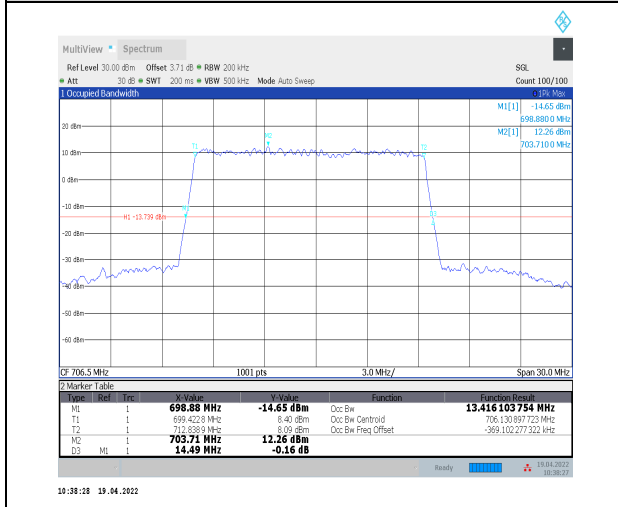
1-N12--15-15-L-5-DFT-256QAM-Outer_Full-75@0-A nt0-13.416-14.490≤15-PASS
