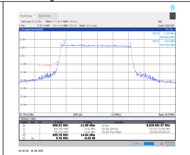
1-N12--15-10-L-3-DFT-16QAM-Outer_Full-50@0-An t0-8.928-9.760-≤10-PASS
