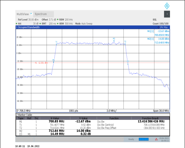
1-N12--15-15-H-4-DFT-64QAM-Outer_Full-75@0-An t0-13.416-14.490≤15-PASS
