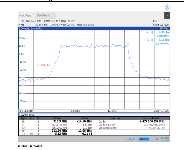
1-N12--15-5-H-4-DFT-64QAM-Outer_Full-25@0-Ant 0-4.477-5.130-<math>\leq</math>5-PASS
