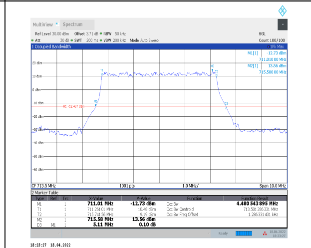
1-N12--15-5-H-2-DFT-PI2BPSK-Outer_Full-25@0-Ant0 4.481-5.110-≤5-PASS
