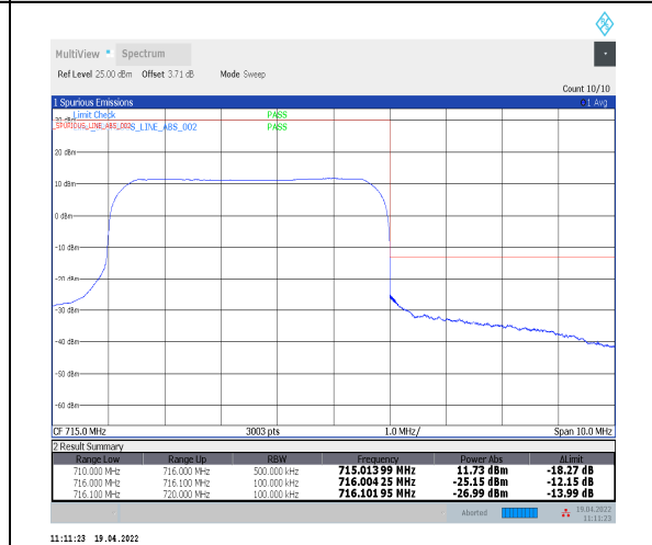
1-N12--15-5-H-6-CP-QPSK-Outer_Full-25@0-Ant 0-PASS-see graph
