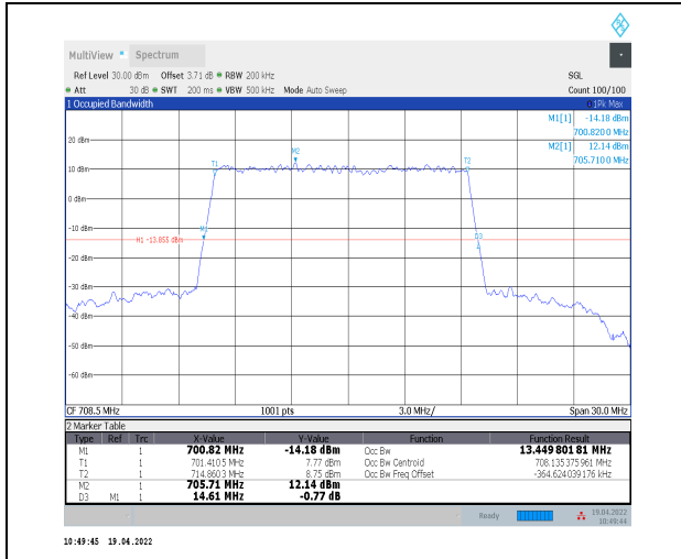
1-N12--15-15-H-5-DFT-256QAM-Outer_Full-75@0-A nt0-13.45-14.610-<=15-PASS
