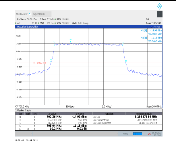
1-N12--15-10-M-8-CP-64QAM-Outer_Full-52@0-Ant 0-9.296-10.200-≤10-PASS
