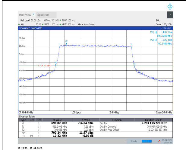
1-N12--15-10-L-8-CP-64QAM-Outer_Full-52@0-Ant0 -9.294-10.220≤10-PASS
