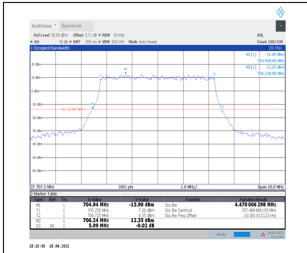
1-N12--15-5-M-4-DFT-64QAM-Outer_Full-25@0-Ant 0-4.47-5.090-≤5-PASS
