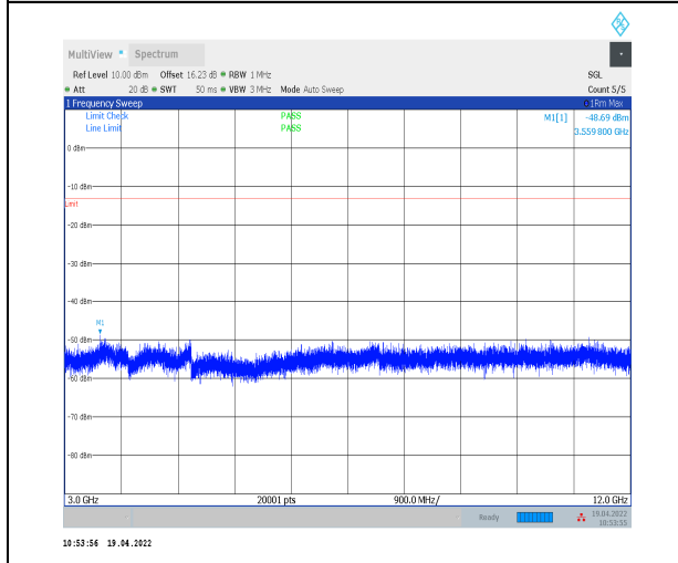
1-N12--15-15-M-1-DFT-PI2BPSK-Inner_1RB_Left-1 @1-3000-12000-Ant0--48.69--13-PASS
