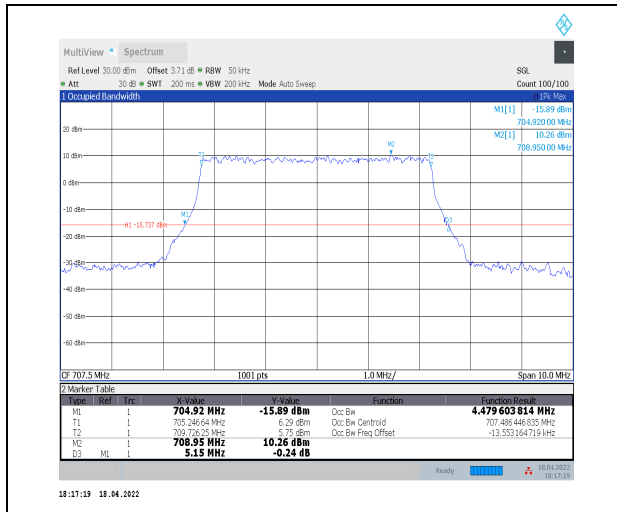
1-N12--15-5-M-8-CP-64QAM-Outer_Full-25@0-Ant0 -4.48-5.150-≤5-PASS
