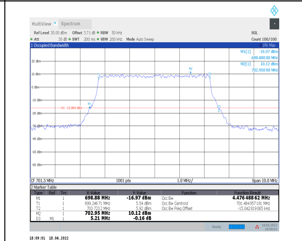
1-N12--15-5-L-8-CP-64QAM-Outer_Full-25@0-Ant0- 4.476-5.210-<math>\leq</math>5-PASS
