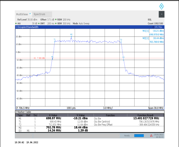
1-N12--15-15-L-2-DFT-PI2BPSK-Outer_Full-75@0-A n0-13.401-14.340-≤15-PASS
