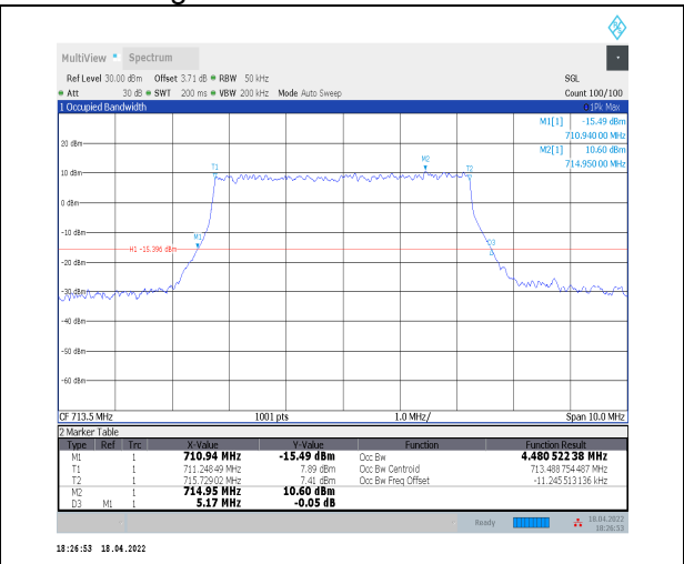
1-N12--15-5-H-8-CP-64QAM-Outer_Full-25@0-Ant0-4.481-5.170-<math>\leq 5</math>-PASS
