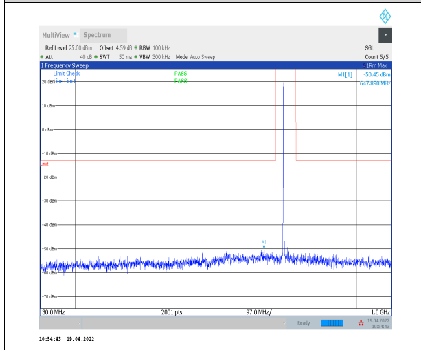
1-N12--15-15-H-1-DFT-PI2BPSK-Inner_1RB_Left-1 @1-30-1000-Ant0--50.45--13-PASS
