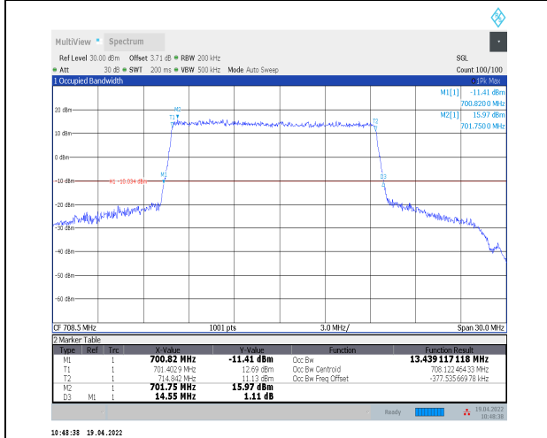
1-N12--15-15-H-3-DFT-16QAM-Outer_Full-75@0-An t0-13.439-14.550≤15-PASS
