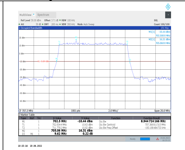
1-N12--15-10-M-2-DFT-PI2BPSK-Outer_Full-50@0- Ant0-8.945-9.620-<=10-PASS
