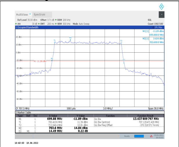
1-N12--15-15-M-3-DFT-16QAM-Outer_Full-75@0-Ant0-13.438-14.490-≤15-PASS
