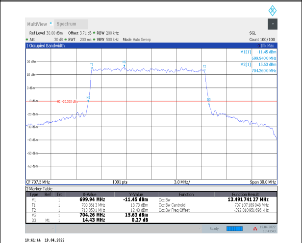
1-N12--15-15-M-1-DFT-QPSK-Outer_Full-75@0-Ant 0-13.492-14.430≤15-PASS
