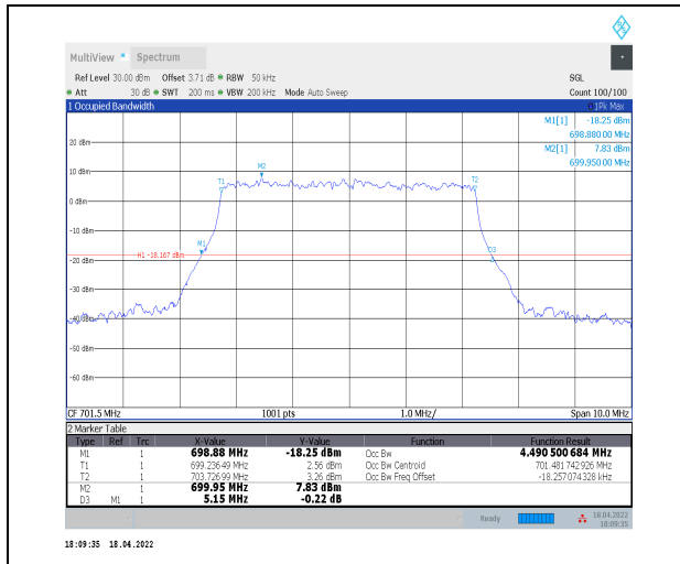
1-N12--15-5-L-9-CP-256QAM-Outer_Full-25@0-Ant0 -4.491-5.150≤5-PASS
