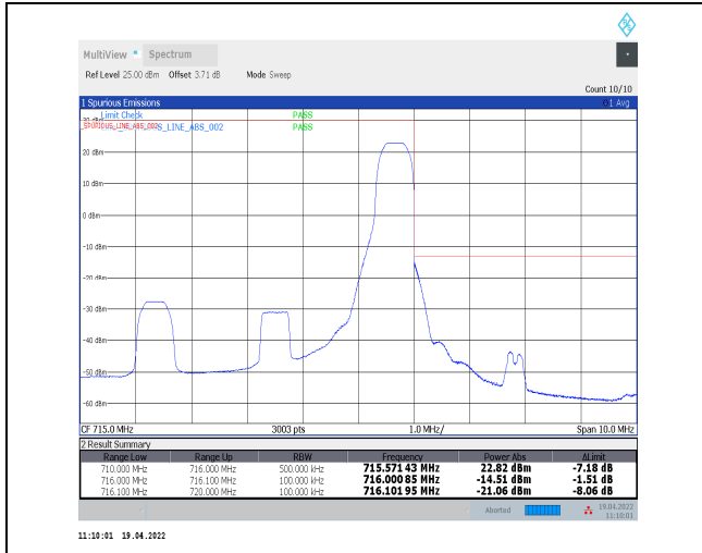
1-N12--15-5-H-2-DFT-PI2BPSK-Edge_1RB_Right-1@2 4-Ant0-PASS-see graph
