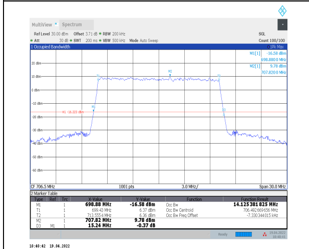
1-N12--15-15-L-9-CP-256QAM-Outer_Full-79@0-Ant 0-14.125-15.240≤15-PASS
