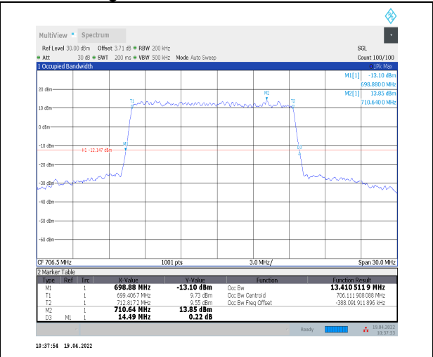
1-N12--15-15-L-4-DFT-64QAM-Outer_Full-75@0-An t0-13.411-14.490≤15-PASS
