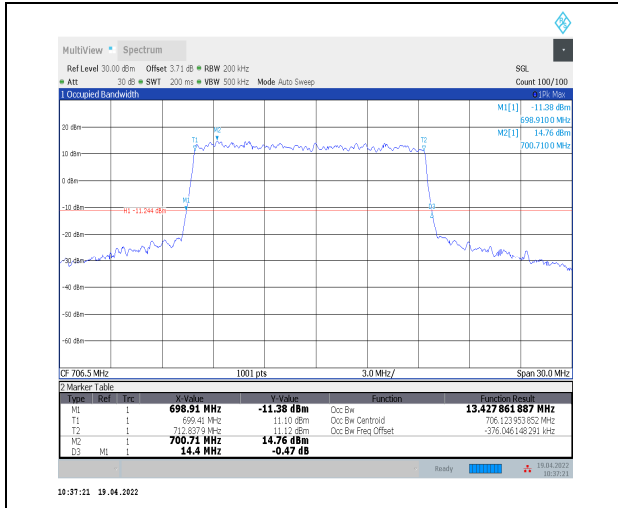
1-N12--15-15-L-3-DFT-16QAM-Outer_Full-75@0-Ant 0-13.428-14.400≤15-PASS
