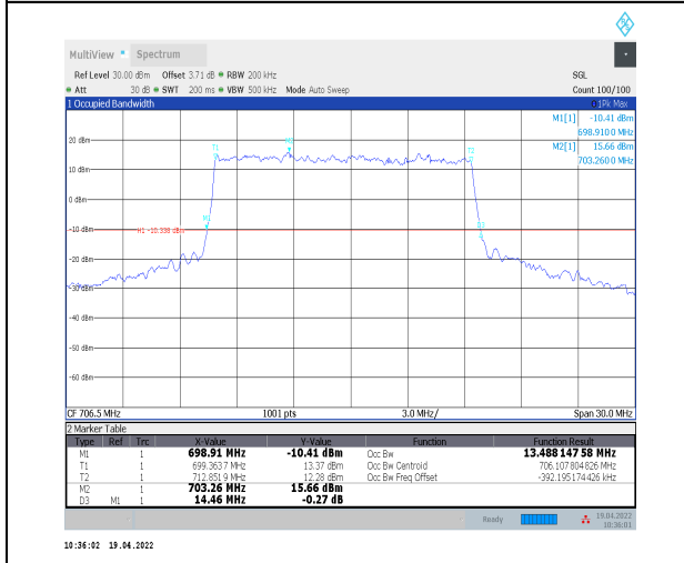
1-N12--15-15-L-1-DFT-QPSK-Outer_Full-75@0-Ant0 -13.488-14.460-≤15-PASS
