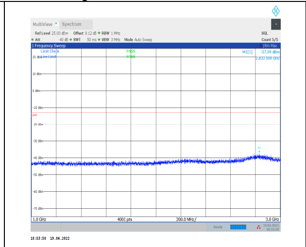
1-N12--15-15-M-1-DFT-PI2BPSK-Inner_1RB_Left-1 @1-1000-3000-Ant0--37.39--13-PASS
