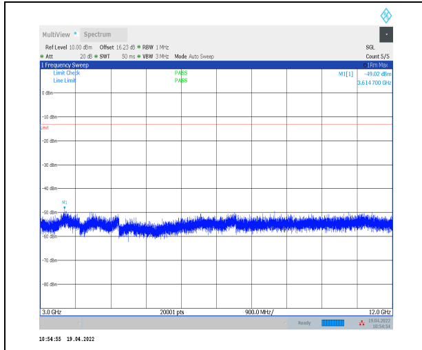
1-N12--15-15-H-1-DFT-PI2BPSK-Inner_1RB_Left-1 @1-3000-12000-Ant0--49.02--13-PASS
