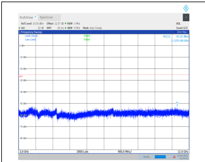
1-N7--15-40-H-1-DFT-PI2BPSK-Inner_1RB_Left-1@ 1-3000-12000-Ant0--52.32--25-PASS
