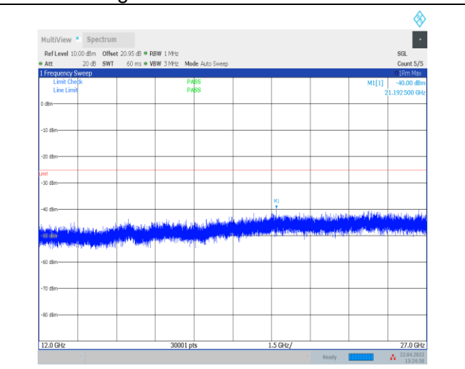
1-N7--15-40-H-1-DFT-PI2BPSK-Inner_1RB_Left-1@ 1-12000-27000-Ant0--40.00--25-PASS
