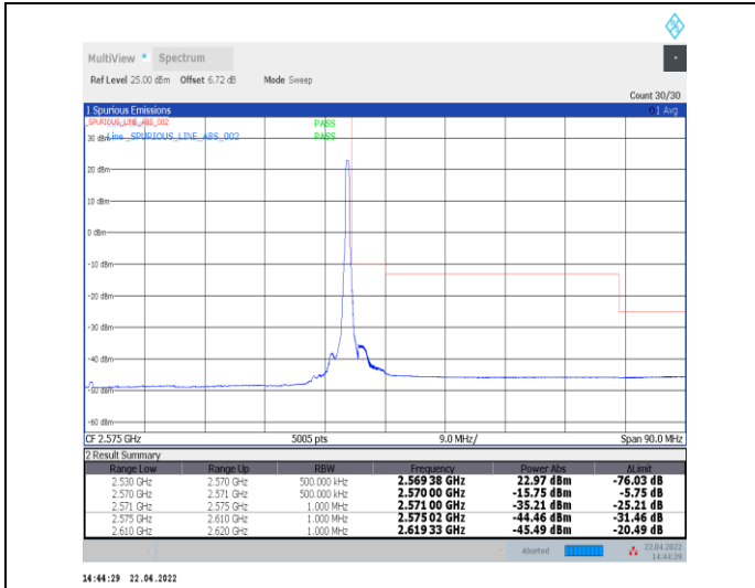
1-N7--15-40-H-2-DFT-PI2BPSK-Edge_1RB_Right-1@2 15-Ant0-PASS-see graph
