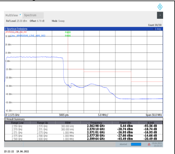
1-N7--15-20-H-3-DFT-PI2BPSK-Outer_Full-100@0-Ant0-PASS-see graph
