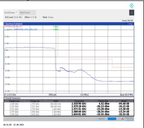
1-N7--15-25-H-3-DFT-PI2BPSK-Outer_Full-128@ 0-Ant0-PASS-see graph
