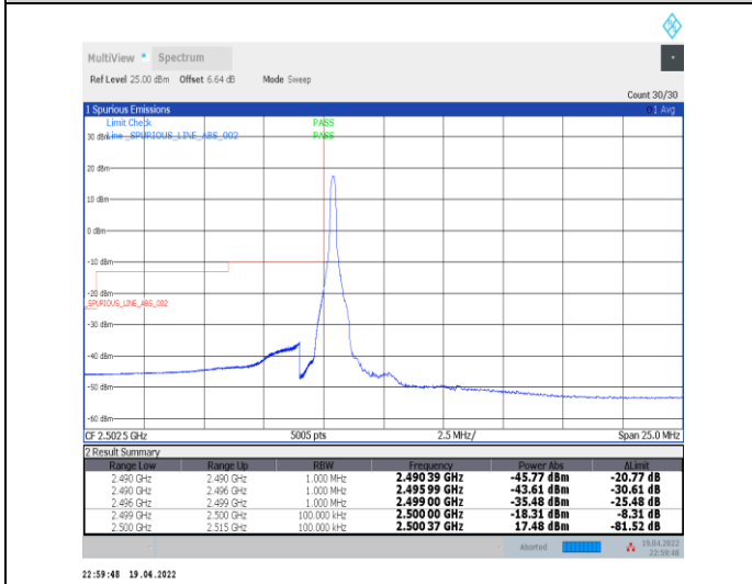
1-N7--15-10-L-4-CP-QPSK-Edge_1RB_Left-1@0-Ant0-PASS-see graph
