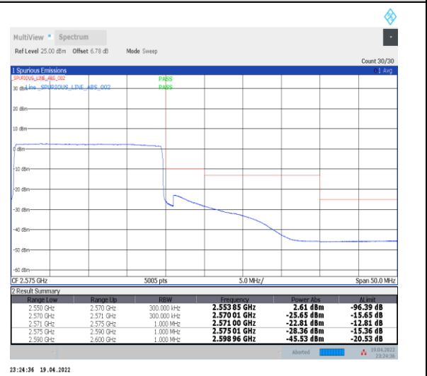
1-N7--15-20-H-6-CP-QPSK-Outer_Full-106@0-Ant0-PASS-see graph
