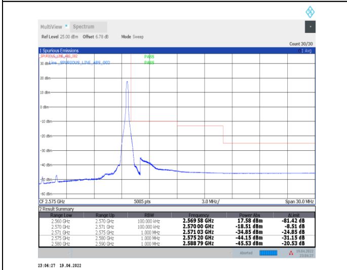
1-N7--15-10-H-5-CP-QPSK-Edge_1RB_Right-1@51-A nt0-PASS-see graph
