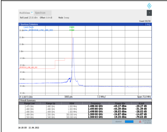
1-N7--15-30-L-4-CP-QPSK-Edge_1RB_Left-1@0-Ant0-PASS-see graph
