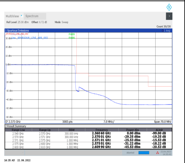
1-N7--15-30-H-6-CP-QPSK-Outer_Full-160@0-Ant0- PASS-see graph
