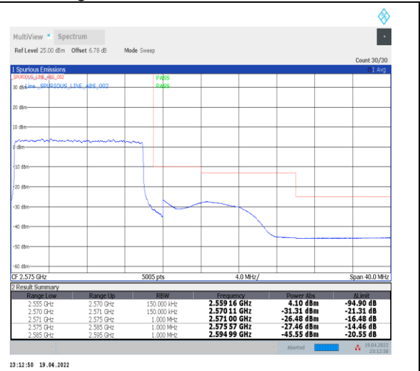
1-N7--15-15-H-3-DFT-PI2BPSK-Outer_Full-75@0 -Ant0-PASS-see graph
