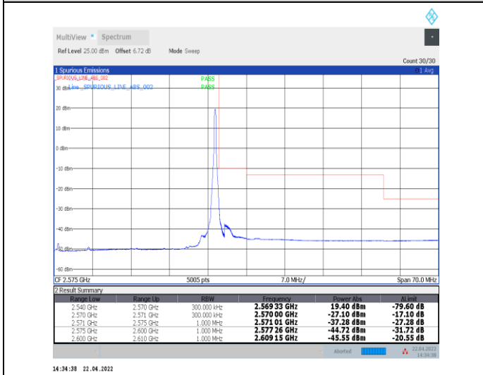
1-N7--15-30-H-5-CP-QPSK-Edge_1RB_Right-1@159- Ant0-PASS-see graph
