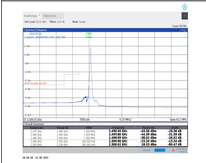
1-N7--15-25-L-4-CP-QPSK-Edge_1RB_Left-1@0-Ant0-PASS-see graph
