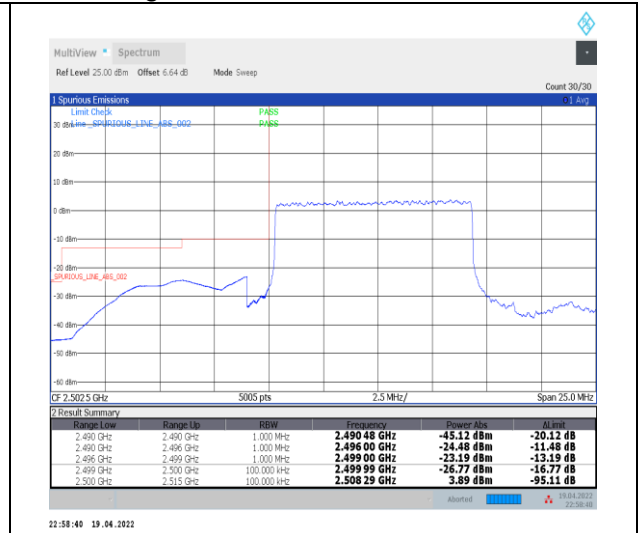
1-N7--15-10-L-3-DFT-PI2BPSK-Outer_Full-50@0-Ant0-PASS-see graph
