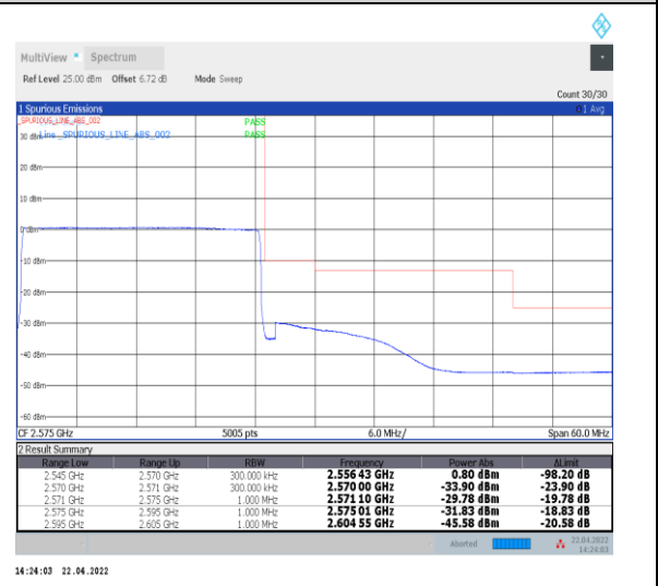
1-N7--15-25-H-6-CP-QPSK-Outer_Full-133@0-Ant0- PASS-see graph
