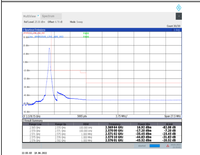
1-N7--15-5-H-5-CP-QPSK-Edge_1RB_Right-1@24-Ant0-PASS-see graph
