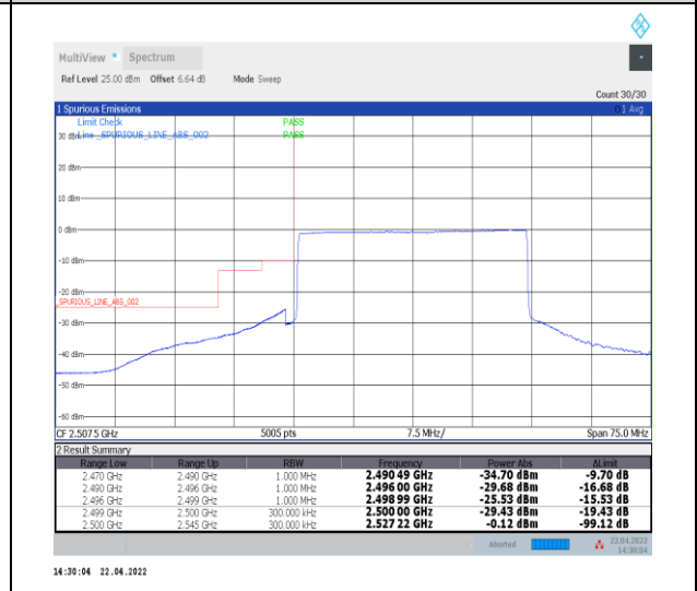
1-N7--15-30-L-6-CP-QPSK-Outer_Full-160@0-Ant0-PASS-see graph
