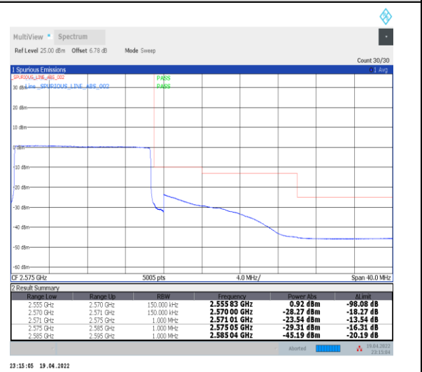
1-N7--15-15-H-6-CP-QPSK-Outer_Full-79@0-Ant 0-PASS-see graph
