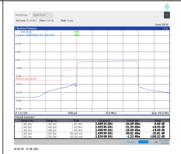
1-N7--15-40-L-6-CP-QPSK-Outer_Full-216@0-Ant0-PASS-see graph
