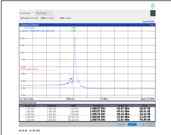
1-N7--15-30-L-1-DFT-PI2BPSK-Edge_1RB_Left-1@0-Ant0-PASS-see graph
