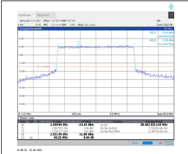
1-N7--15-40-L-7-CP-16QAM-Outer_Full-216@0-Ant 0-38.55-40.320-≤40-PASS
