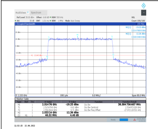
1-N7--15-40-M-8-CP-64QAM-Outer_Full-216@0-Ant0 0-38.585-40.320-≤40-PASS
