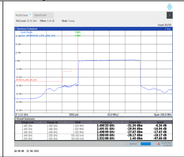
1-N7--15-40-L-3-DFT-PI2BPSK-Outer_Full-216@0-Ant0-PASS-see graph
