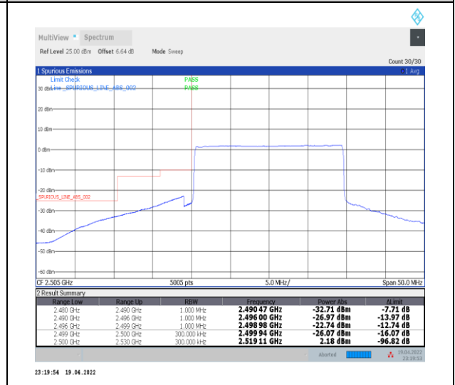
1-N7--15-20-L-6-CP-QPSK-Outer_Full-106@0-Ant0-PASS-see graph
