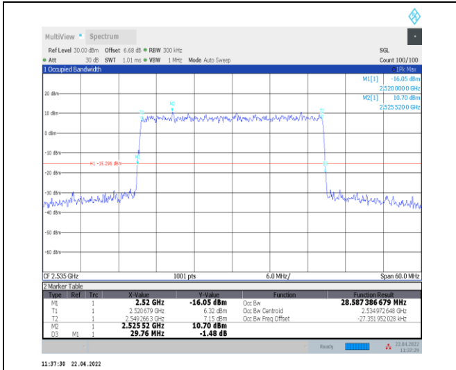
1-N7--15-30-M-5-DFT-256QAM-Outer_Full-160@0-A nt0-28.587-29.760-≤30-PASS
