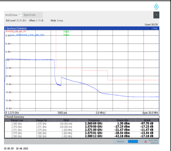
1-N7--15-10-H-6-CP-QPSK-Outer_Full-52@0-Ant 0-PASS-see graph
