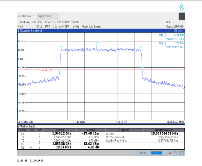
1-N7--15-30-H-3-DFT-16QAM-Outer_Full-160@0-An t0-28.565-29.640-<=30-PASS
