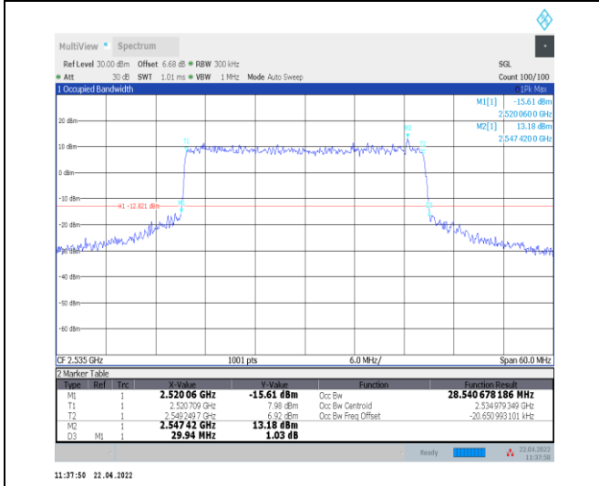
1-N7--15-30-M-7-CP-16QAM-Outer_Full-160@0-Ant 0-28.541-29.940-≤30-PASS
