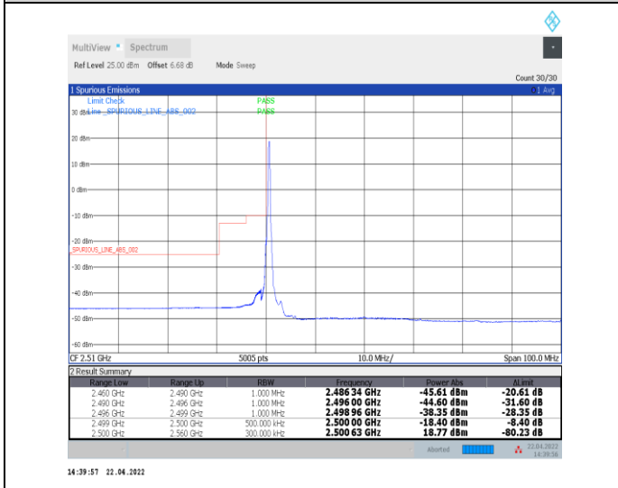
1-N7--15-40-L-4-CP-QPSK-Edge_1RB_Left-1@0-Ant0-PASS-see graph
