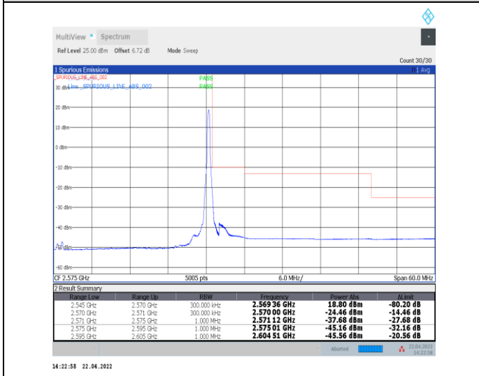
1-N7--15-25-H-5-CP-QPSK-Edge_1RB_Right-1@132- Ant0-PASS-see graph
