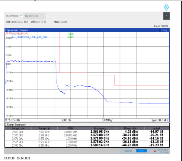
1-N7--15-10-H-3-DFT-PI2BPSK-Outer_Full-50@0 -Ant0-PASS-see graph
