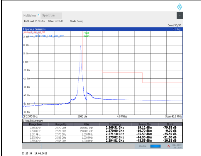
1-N7--15-15-H-5-CP-QPSK-Edge_1RB_Right-1@78-A nt0-PASS-see graph
