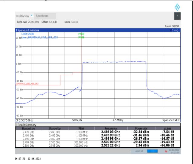
1-N7--15-30-L-3-DFT-PI2BPSK-Outer_Full-160@0-Ant0-PASS-see graph
