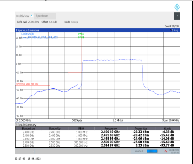
1-N7--15-20-L-3-DFT-PI2BPSK-Outer_Full-100@0-Ant0-PASS-see graph
