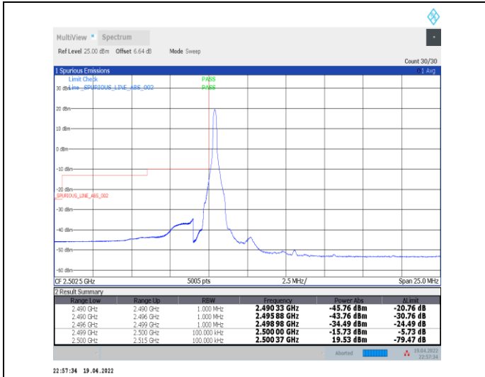
1-N7--15-10-L-1-DFT-PI2BPSK-Edge_1RB_Left-1@0-Ant0-PASS-see graph
