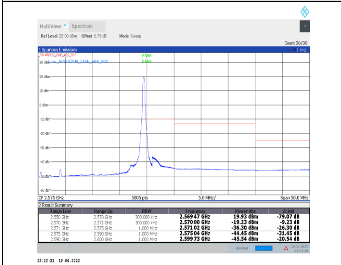
1-N7--15-20-H-5-CP-QPSK-Edge_1RB_Right-1@105-Ant0-PASS-see graph
