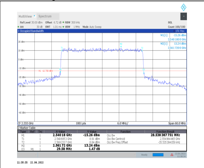
1-N7--15-30-H-1-DFT-QPSK-Outer_Full-160@0-Ant 0-28.539-29.580-<=30-PASS
