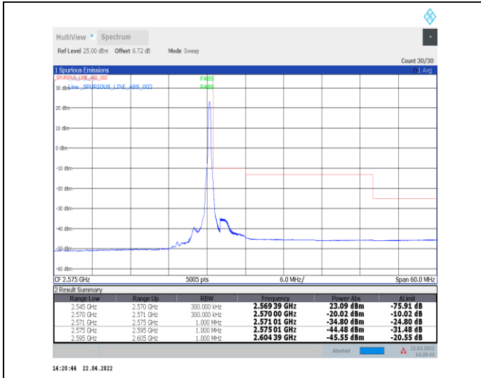
1-N7--15-25-H-2-DFT-PI2BPSK-Edge_1RB_Right-1@1 32-Ant0-PASS-see graph
