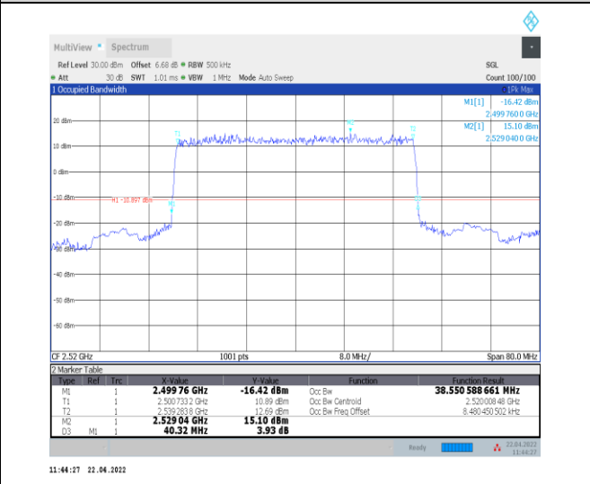
1-N7--15-40-L-2-DFT-PI2BPSK-Outer_Full-216@0-Ant0 nt0-38.552-40.320-≤40-PASS
