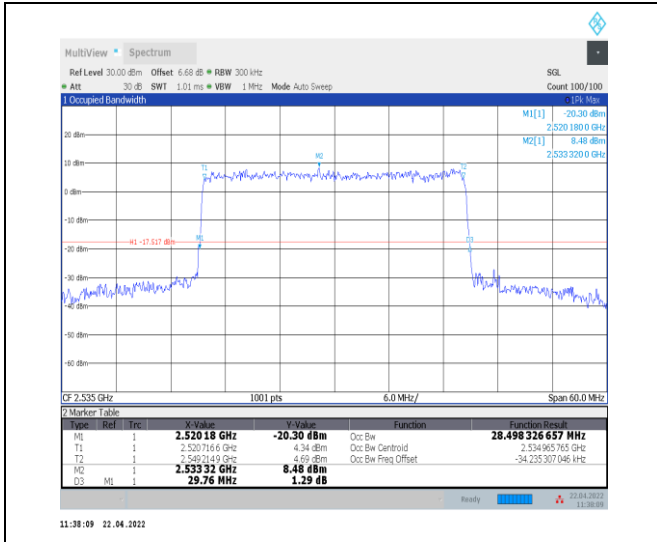
1-N7--15-30-M-9-CP-256QAM-Outer_Full-160@0-A nt0-28.5-29.760-<=30-PASS
