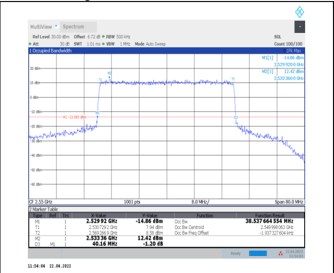
1-N7--15-40-H-6-CP-QPSK-Outer_Full-216@0-Ant0- 38.55-40.160-<math>\leq 40</math>-PASS
