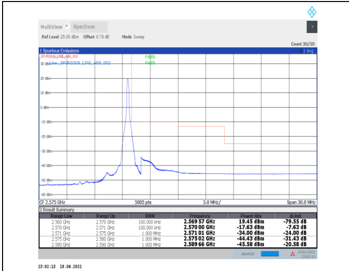
1-N7--15-10-H-2-DFT-PI2BPSK-Edge_1RB_Right-1@5 1-Ant0-PASS-see graph
