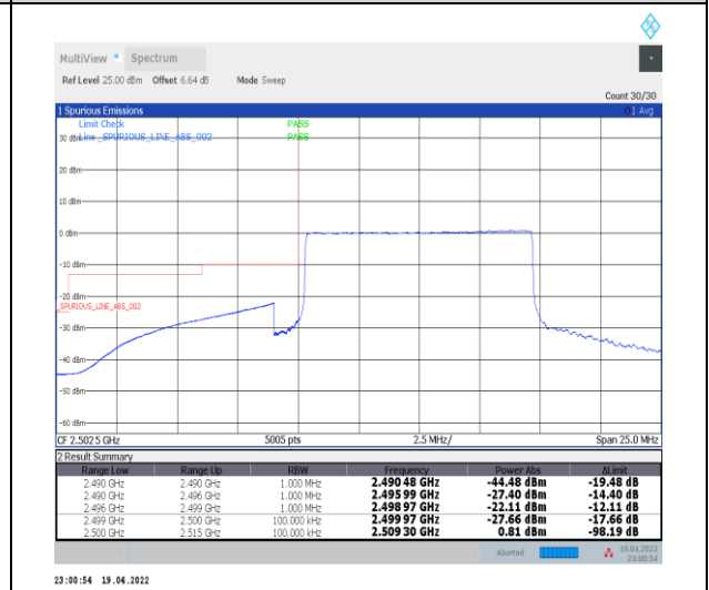
1-N7--15-10-L-6-CP-QPSK-Outer_Full-52@0-Ant0-PASS-see graph
