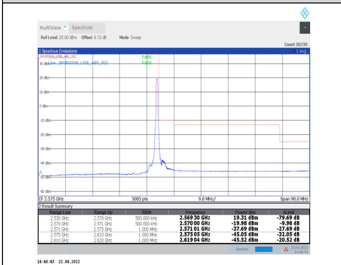
1-N7--15-40-H-5-CP-QPSK-Edge_1RB_Right-1@215-Ant0-PASS-see graph
