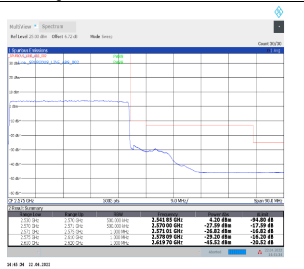
1-N7--15-40-H-3-DFT-PI2BPSK-Outer_Full-216@0-Ant0-PASS-see graph
