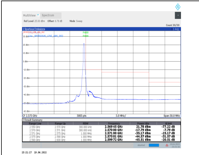
1-N7--15-20-H-2-DFT-PI2BPSK-Edge_1RB_Right-1@105-Ant0-PASS-see graph
