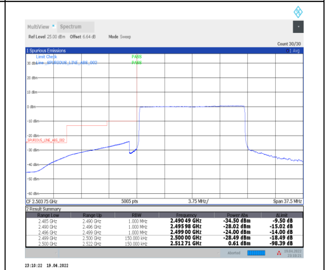
1-N7--15-15-L-6-CP-QPSK-Outer_Full-79@0-Ant0-PASS-see graph
