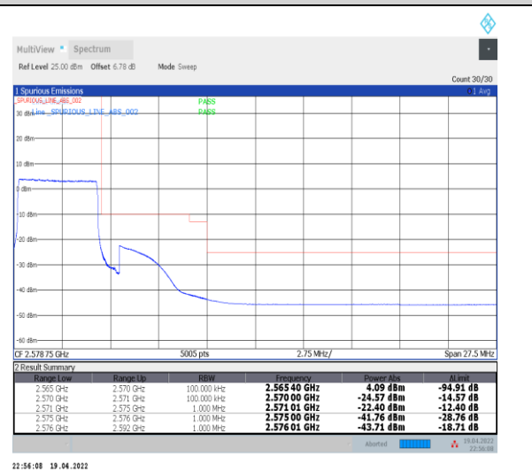
1-N7--15-5-H-6-CP-QPSK-Outer_Full-25@0-Ant0-PASS-see graph
