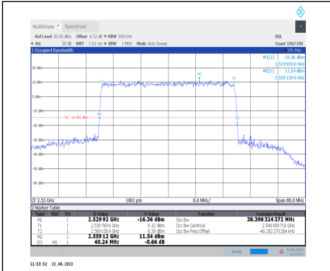
1-N7--15-40-H-5-DFT-256QAM-Outer_Full-216@0-A nt0-38.398-40.240-<math>\leq 40</math>-PASS
