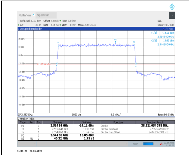
1-N7--15-40-M-2-DFT-PI2BPSK-Outer_Full-216@0-Ant0-38.537-40.320-≤40-PASS
