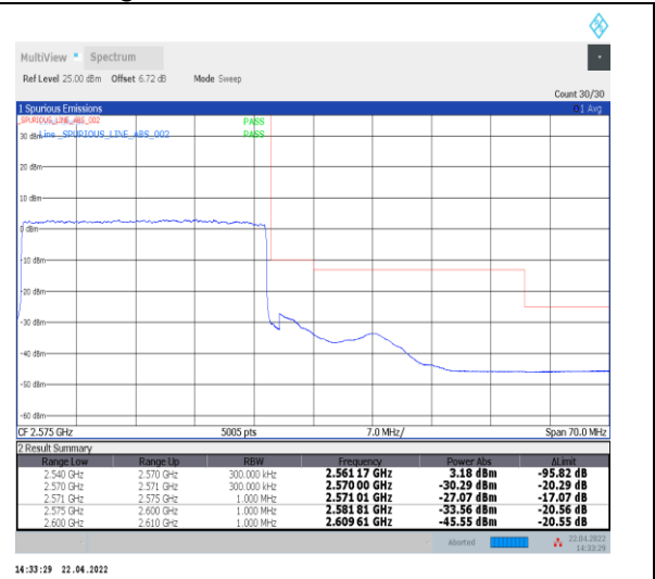
1-N7--15-30-H-3-DFT-PI2BPSK-Outer_Full-160@ 0-Ant0-PASS-see graph
