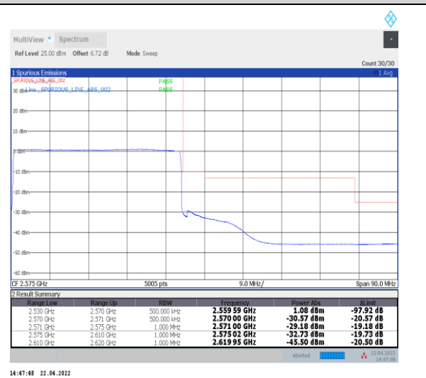
1-N7--15-40-H-6-CP-QPSK-Outer_Full-216@0-Ant0-PASS-see graph
