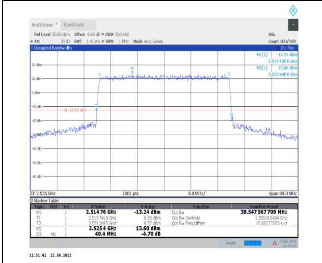
1-N7--15-40-M-4-DFT-64QAM-Outer_Full-216@0-Ant0-38.57-40.400-≤40-PASS
