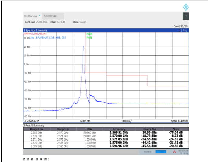
1-N7--15-15-H-2-DFT-PI2BPSK-Edge_1RB_Right-1@7 8-Ant0-PASS-see graph
