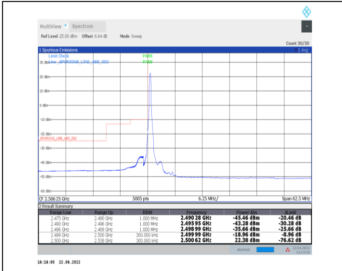
1-N7--15-25-L-1-DFT-PI2BPSK-Edge_1RB_Left-1@0-Ant0-PASS-see graph
