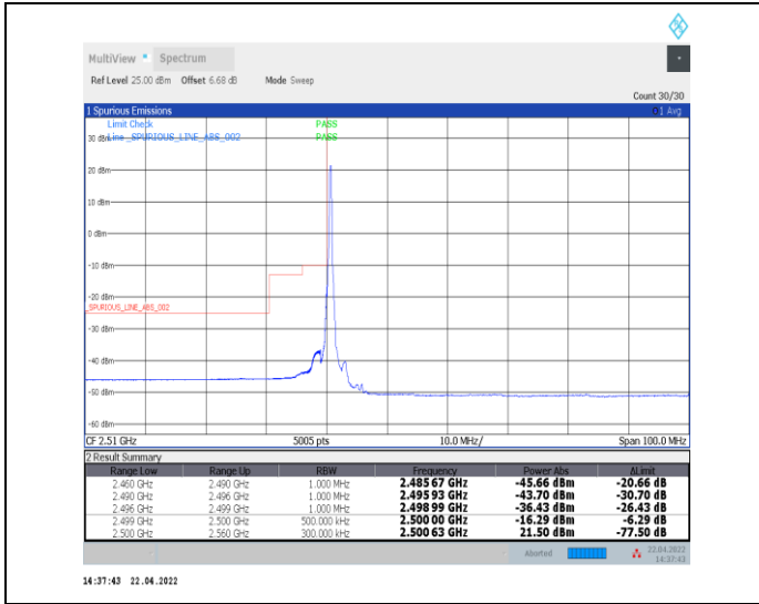
1-N7--15-40-L-1-DFT-PI2BPSK-Edge_1RB_Left-1@0-Ant0-PASS-see graph
