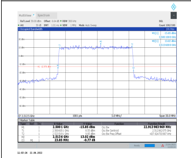
1-N7--15-25-L-3-DFT-16QAM-Outer_Full-128@0-Ant0 0-22.914-23.850-≤25-PASS
