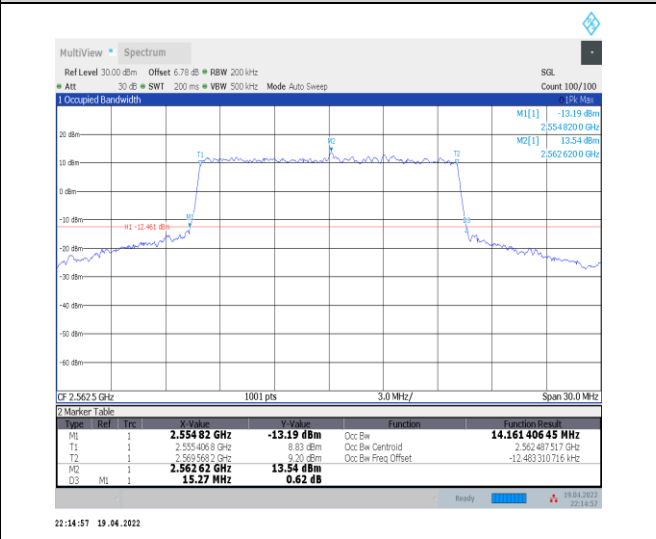
1-N7--15-15-H-8-CP-64QAM-Outer_Full-79@0-Ant0-14.161-15.270-≤15-PASS
