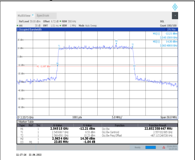
1-N7--15-25-H-4-DFT-64QAM-Outer_Full-128@0-An t0-22.852-23.850-<=25-PASS
