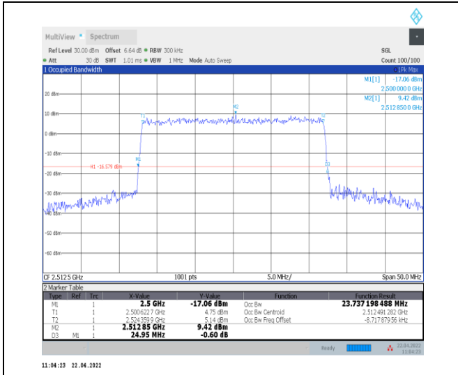
1-N7--15-25-L-9-CP-256QAM-Outer_Full-133@0-An t0-23.737-24.950-<25-PASS
