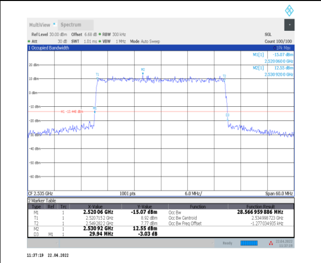
1-N7--15-30-M-4-DFT-64QAM-Outer_Full-160@0-Ant t0-28.567-29.940-≤30-PASS
