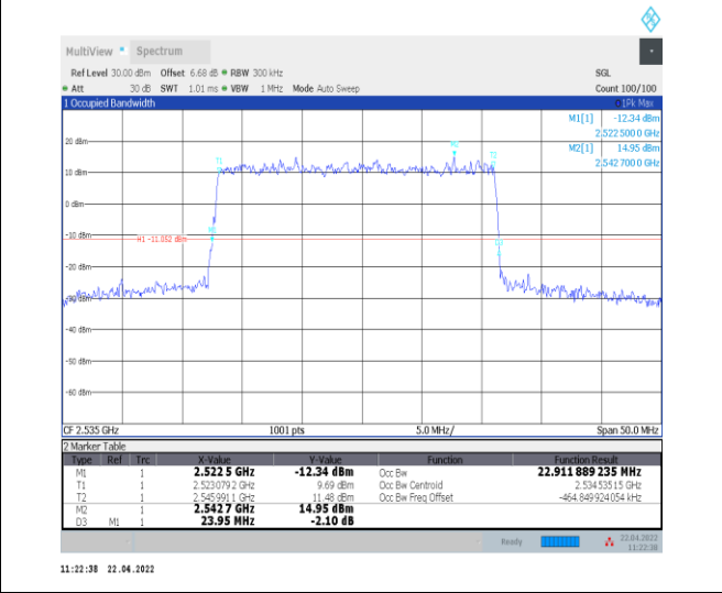
1-N7--15-25-M-3-DFT-16QAM-Outer_Full-128@0-An t0-22.912-23.950-<25-PASS
