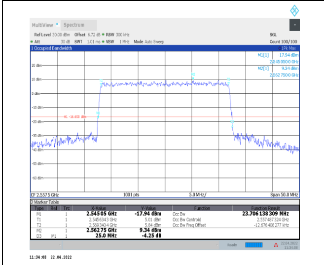
1-N7--15-25-H-9-CP-256QAM-Outer_Full-133@0-Ant t0-23.706-25.000-≤25-PASS
