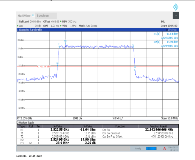
1-N7--15-25-M-1-DFT-QPSK-Outer_Full-128@0-Ant 0-22.843-23.900-<25-PASS
