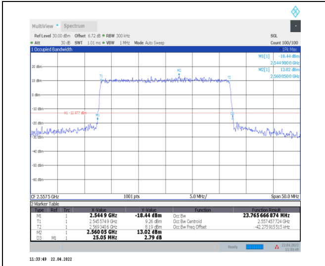
1-N7--15-25-H-7-CP-16QAM-Outer_Full-133@0-Ant 0-23.766-25.050-≤25-PASS
