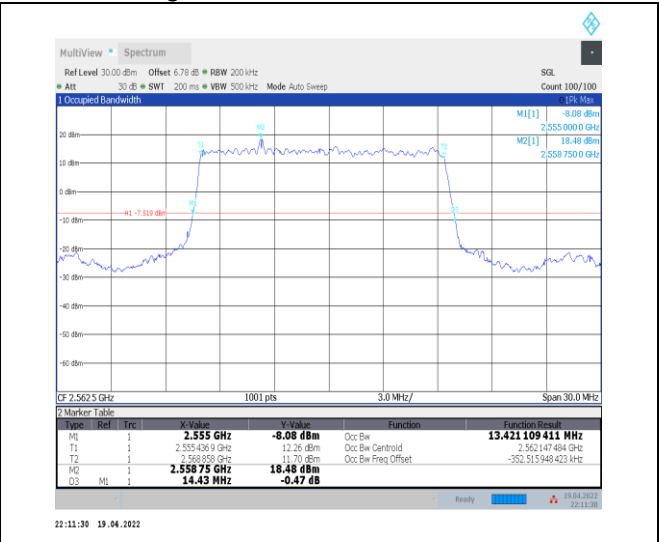
1-N7--15-15-H-2-DFT-PI2BPSK-Outer_Full-75@0-Ant0-13.421-14.430-≤15-PASS
