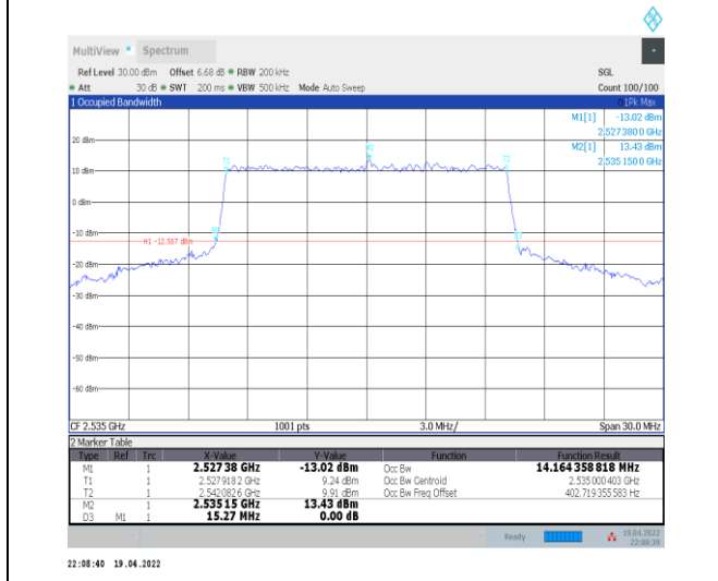
1-N7--15-15-M-8-CP-64QAM-Outer_Full-79@0-Ant0-14.164-15.270-≤15-PASS
