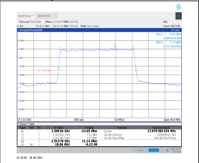
1-N7--15-20-L-5-DFT-256QAM-Outer_Full-100@0-Ant 0-17.88-18.960-≤20-PASS
