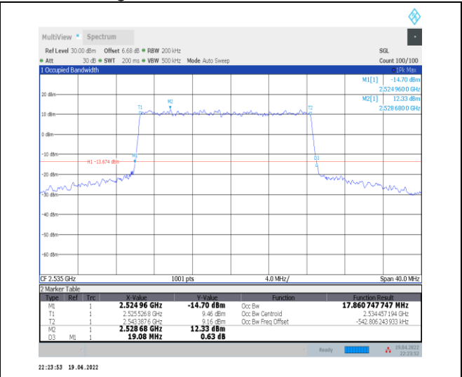
1-N7--15-20-M-4-DFT-64QAM-Outer_Full-100@0-An t0-17.861-19.080-≤20-PASS
