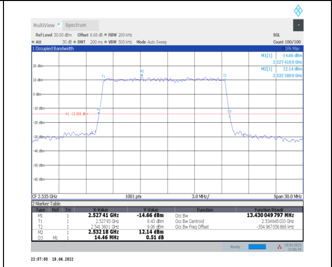
1-N7--15-15-M-5-DFT-256QAM-Outer_Full-75@0-Ant 0-13.43-14.460-≤15-PASS
