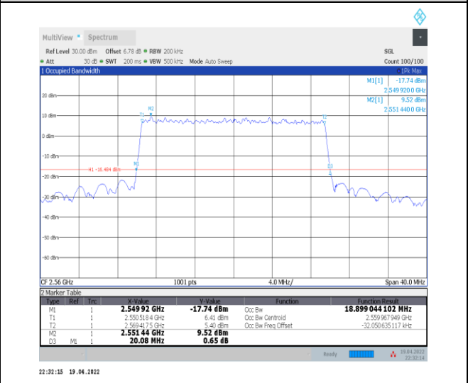
1-N7--15-20-H-9-CP-256QAM-Outer_Full-106@0-Ant0-18.899-20.080-≤20-PASS
