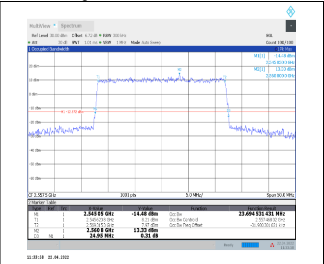
1-N7--15-25-H-8-CP-64QAM-Outer_Full-133@0-Ant 0-23.695-24.950-≤25-PASS
