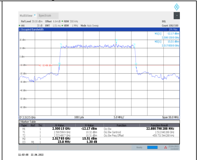
1-N7--15-25-L-2-DFT-PI2BPSK-Outer_Full-128@0-Ant0 -22.881-23.800-≤25-PASS
