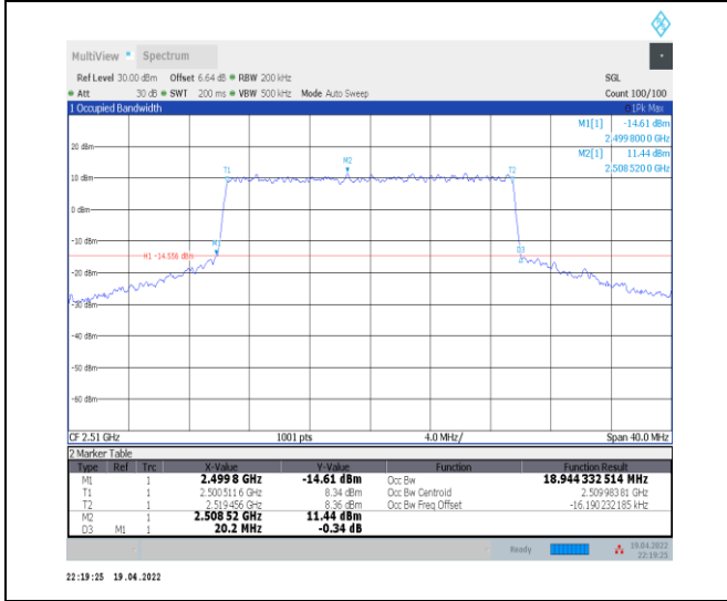
1-N7--15-20-L-6-CP-QPSK-Outer_Full-106@0-Ant 0-18.944-20.200-≤20-PASS
