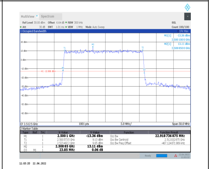
1-N7--15-25-L-4-DFT-64QAM-Outer_Full-128@0-Ant0 0-22.919-23.850-≤25-PASS
