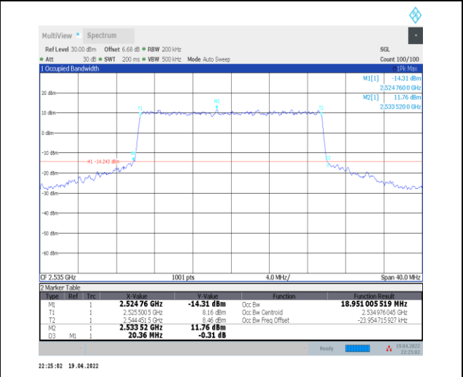
1-N7--15-20-M-6-CP-QPSK-Outer_Full-106@0-Ant0 -18.951-20.360-≤20-PASS
