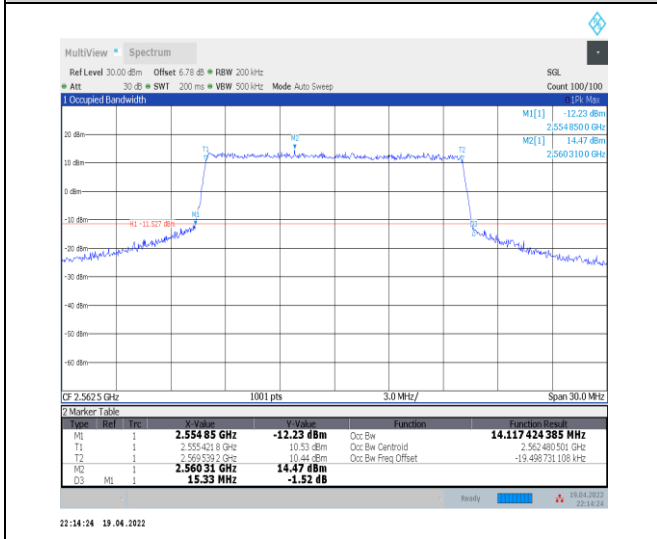
1-N7--15-15-H-7-CP-16QAM-Outer_Full-79@0-Ant0-14.117-15.330-≤15-PASS
