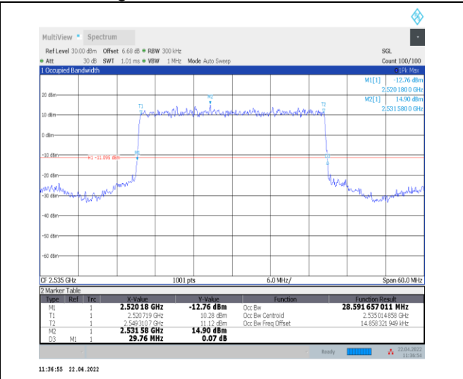
1-N7--15-30-M-2-DFT-PI2BPSK-Outer_Full-160@0-Ant 0-28.592-29.760-≤30-PASS
