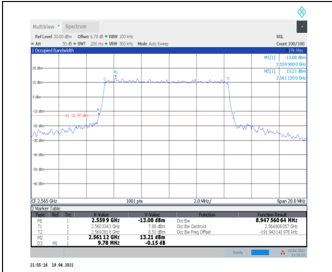
1-N7--15-10-H-4-DFT-64QAM-Outer_Full-50@0-Ant 0-8.948-9.780≤10-PASS
