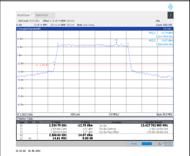
1-N7--15-15-H-4-DFT-64QAM-Outer_Full-75@0-Ant0-13.428-14.610-≤15-PASS
