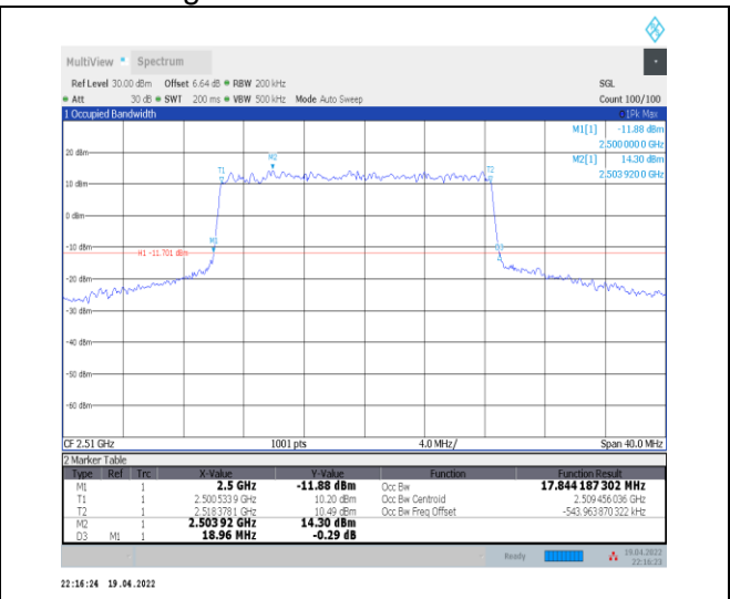
1-N7--15-20-L-1-DFT-QPSK-Outer_Full-100@0-Ant0 -17.844-18.960-≤20-PASS
