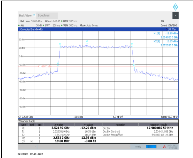
1-N7--15-20-M-3-DFT-16QAM-Outer_Full-100@0-An t0-17.9-19.080-≤20-PASS
