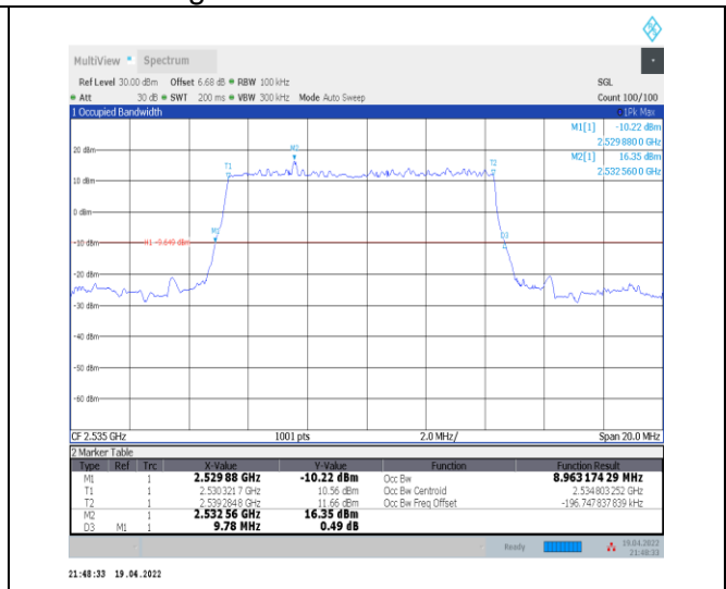
1-N7--15-10-M-2-DFT-PI2BPSK-Outer_Full-50@0-Ant0-8.963-9.780-≤10-PASS
