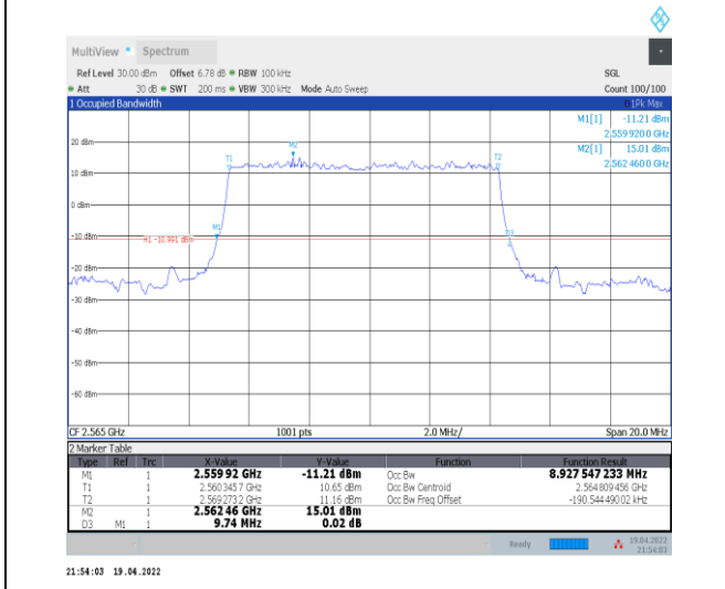
1-N7--15-10-H-2-DFT-PI2BPSK-Outer_Full-50@0-A nt0-8.928-9.740-≤10-PASS
