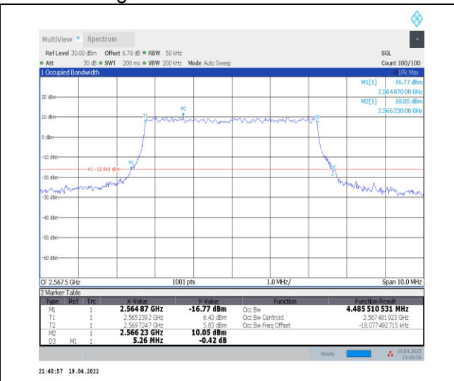
1-N7--15-5-H-8-CP-64QAM-Outer_Full-25@0-Ant0-4 .486-5.260-≤5-PASS
