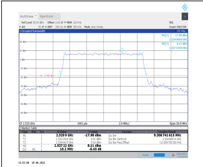
1-N7--15-10-M-9-CP-256QAM-Outer_Full-52@0-Ant 0-9.309-10.200-≤10-PASS
