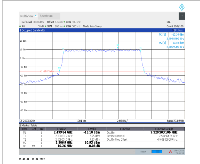
1-N7--15-10-L-8-CP-64QAM-Outer_Full-52@0-Ant0-9 .32-10.260-≤10-PASS
