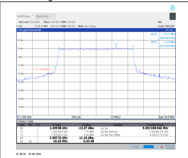
1-N7--15-10-L-7-CP-16QAM-Outer_Full-52@0-Ant0-9 .302-10.180-≤10-PASS
