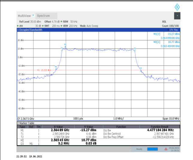
1-N7--15-5-H-6-CP-QPSK-Outer_Full-25@0-Ant0-4.477-5.200-≤5-PASS
