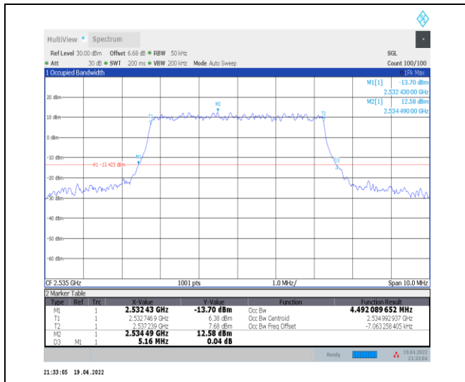
1-N7--15-5-M-4-DFT-64QAM-Outer_Full-25@0-Ant0 -4.492-5.160-≤5-PASS
