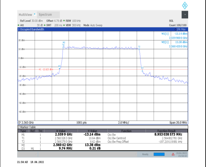
1-N7--15-10-H-3-DFT-16QAM-Outer_Full-50@0-Ant 0-8.953-9.740-≤10-PASS
