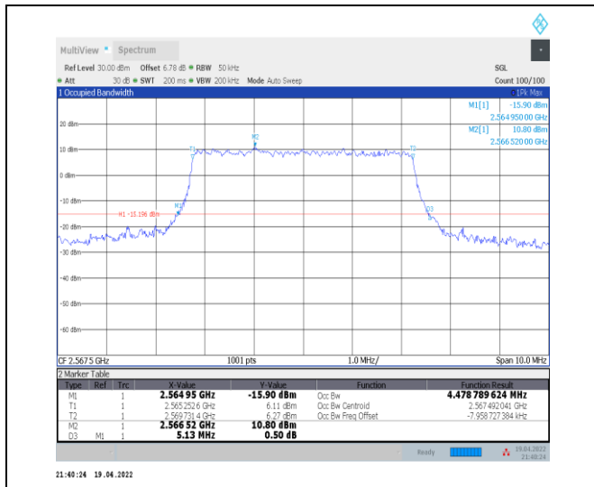
1-N7--15-5-H-7-CP-16QAM-Outer_Full-25@0-Ant0-4 .479-5.130-≤5-PASS
