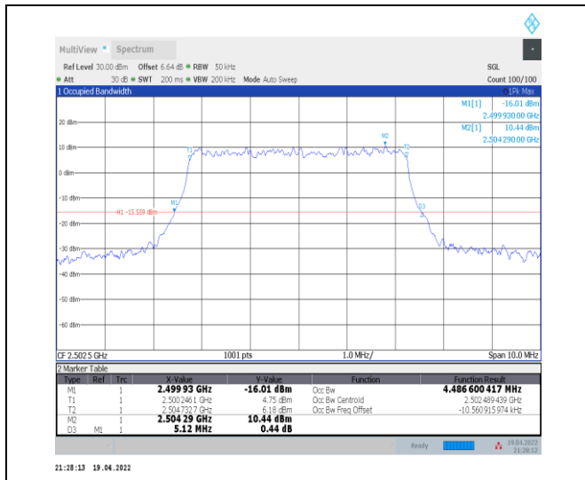
1-N7--15-5-L-5-DFT-256QAM-Outer_Full-25@0-Ant0 -4.487-5.120-≤5-PASS
