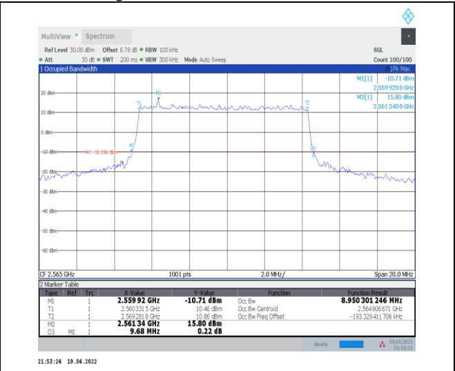
1-N7--15-10-H-1-DFT-QPSK-Outer_Full-50@0-Ant0 8.95-9.680-≤10-PASS
