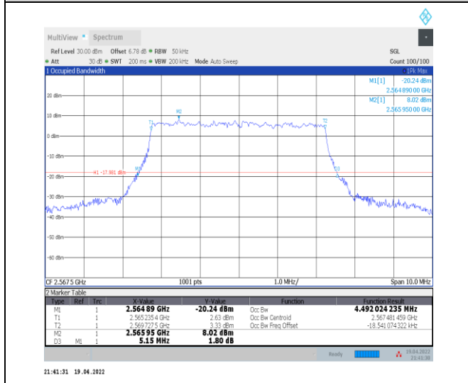
1-N7--15-5-H-9-CP-256QAM-Outer_Full-25@0-Ant0-4 4.492-5.150-≤5-PASS
