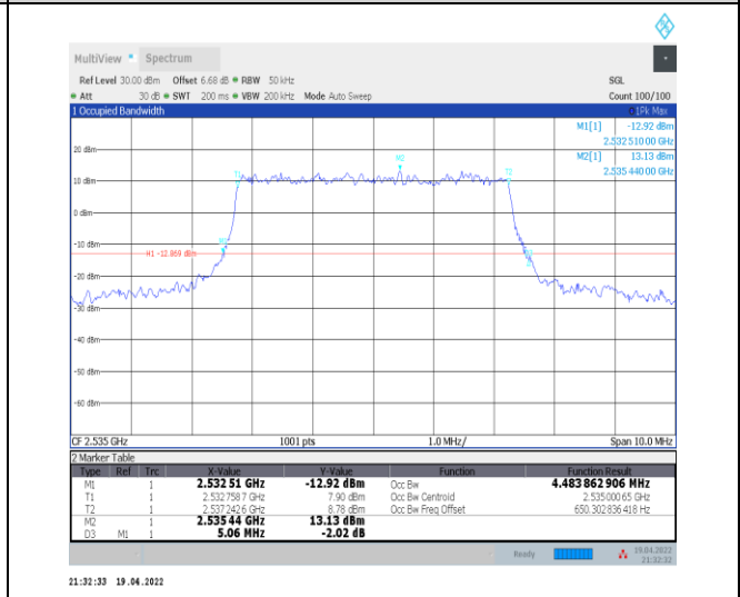
1-N7--15-5-M-3-DFT-16QAM-Outer_Full-25@0-Ant0-4.484-5.060-≤5-PASS
