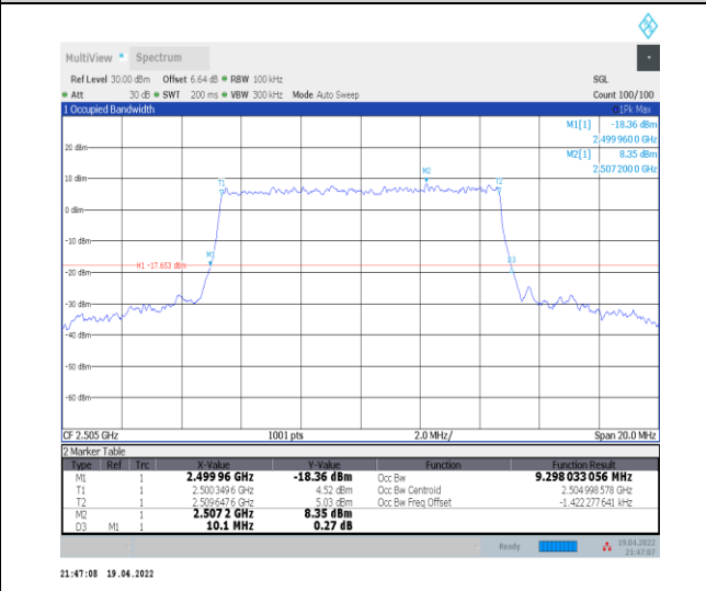
1-N7--15-10-L-9-CP-256QAM-Outer_Full-52@0-Ant0-9 .298-10.100-≤10-PASS
