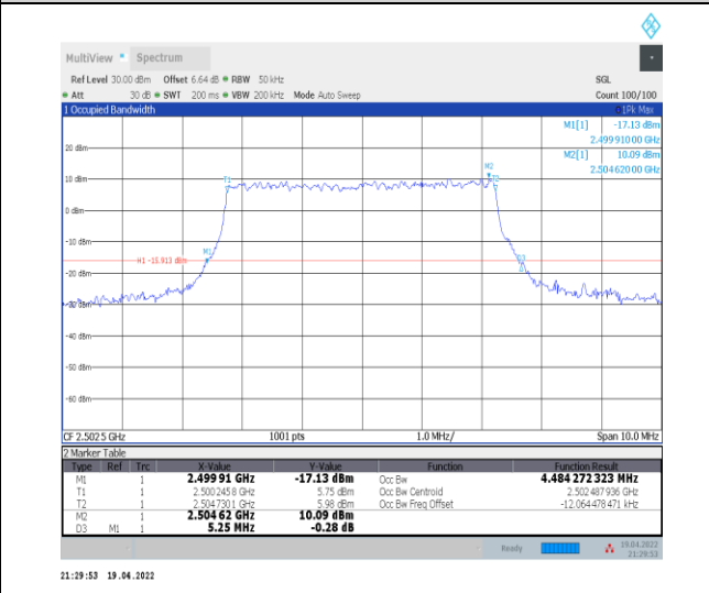
1-N7--15-5-L-8-CP-64QAM-Outer_Full-25@0-Ant0-4 .484-5.250-≤5-PASS
