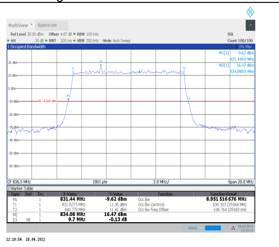
1-N5--15-10-M-2-DFT-PI2BPSK-Outer_Full-50@0-Ant0 -8.952-9.700-≤10-PASS
