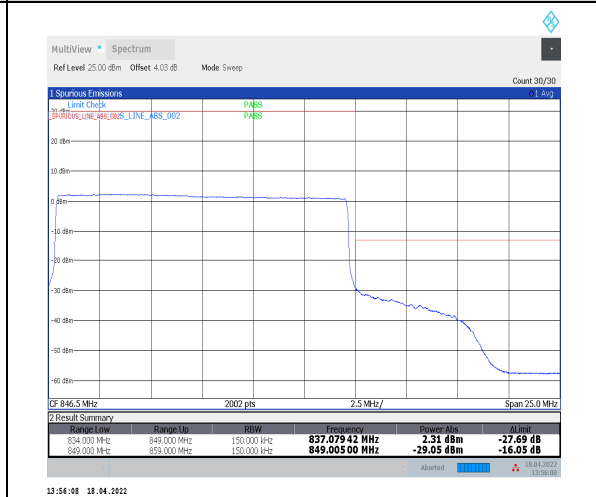
1-N5--15-15-H-6-CP-QPSK-Outer_Full-79@0-Ant0-seegraph-PASS-see graph
