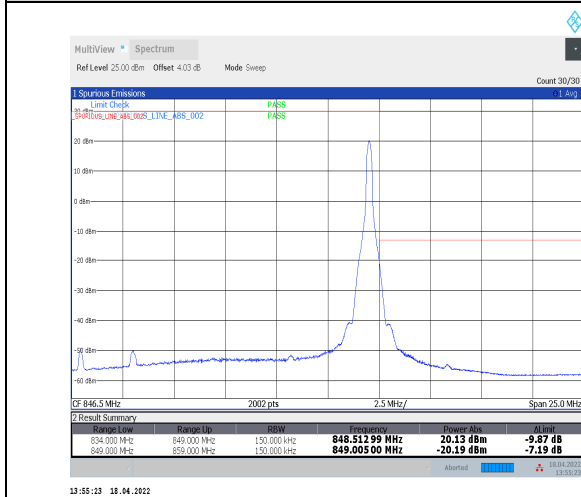
1-N5--15-15-H-5-CP-QPSK-Edge_1RB_Right-1@78-Ant0-seegraph-PASS-see graph
