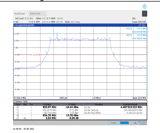
1-N5--15-5-M-1-DFT-QPSK-Outer_Full-25@0-Ant0-4.487-5.050-<=5-PASS
