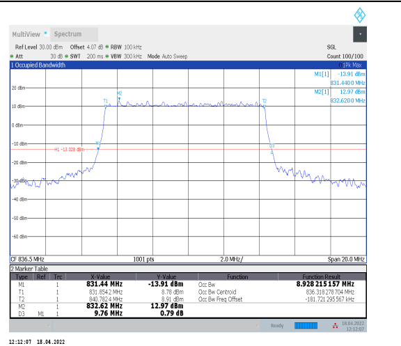
1-N5--15-10-M-4-DFT-64QAM-Outer_Full-50@0-Ant0 0-8.928-9.760-≤10-PASS
