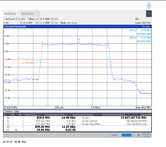
1-N5--15-20-H-5-DFT-256QAM-Outer_Full-100@0-An nt0-17.847-18.960-≤20-PASS
