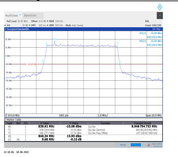
1-N5--15-10-H-1-DFT-QPSK-Outer_Full-50@0-Ant0- 8.949-9.680-≤10-PASS
