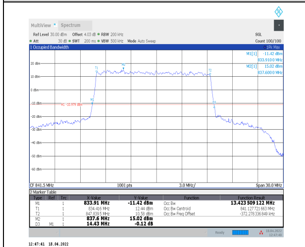
1-N5--15-15-H-3-DFT-16QAM-Outer_Full-75@0-Ant 0-13.424-14.430≤15-PASS
