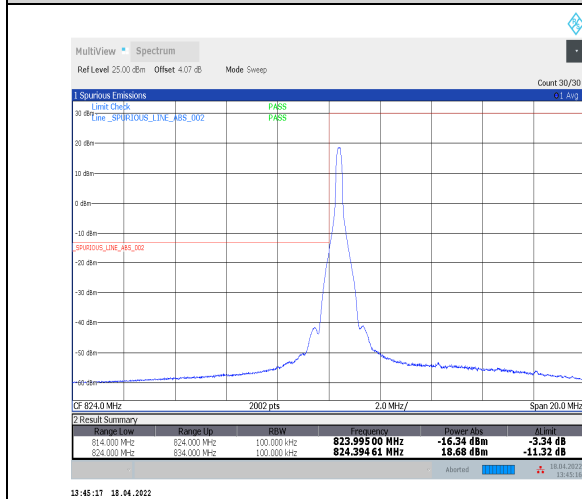
1-N5--15-10-L-4-CP-QPSK-Edge_1RB_Left-1@0-Ant0-seegraph-PASS-see graph
