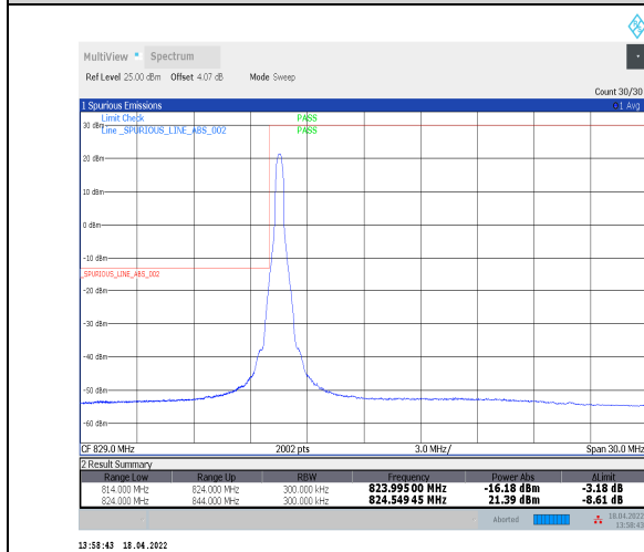
1-N5--15-20-L-4-CP-QPSK-Edge_1RB_Left-1@0-Ant0-seegraph-PASS-see graph
