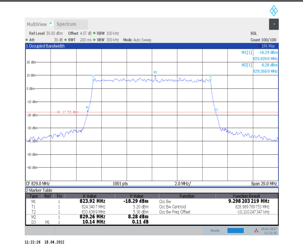
1-N5--15-10-L-9-CP-256QAM-Outer_Full-52@0-Ant0-9 -9.298-10.140-≤10-PASS
