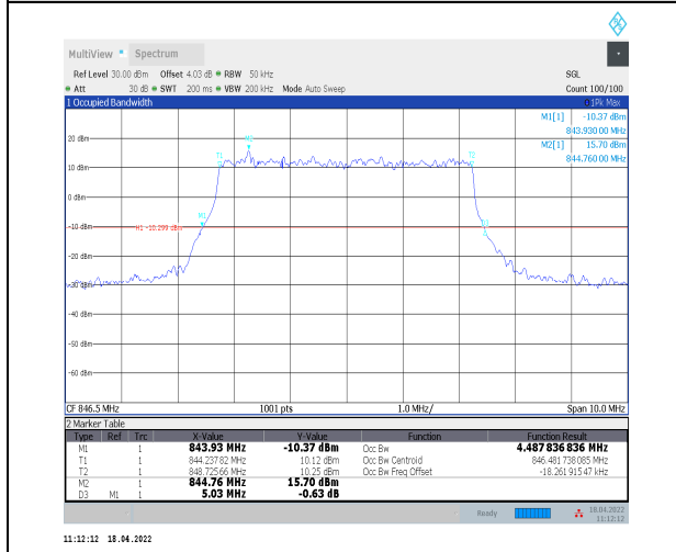
1-N5--15-5-H-1-DFT-QPSK-Outer_Full-25@0-Ant0-4.488-5.030-≤5-PASS
