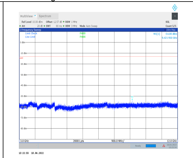
1-N5--15-20-M-1-DFT-PI2BPSK-Inner_1RB_Left-1@ 1-3000-12000-Ant0--54.00--13-PASS
