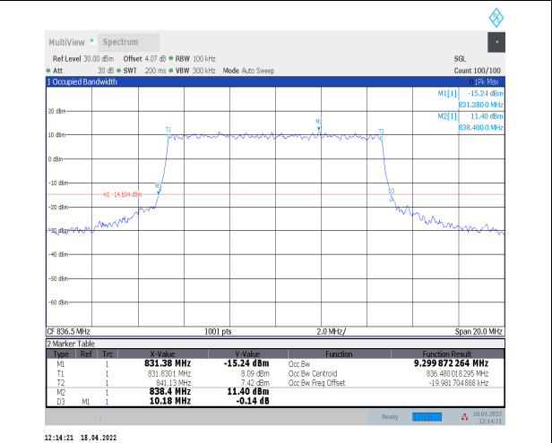
1-N5--15-10-M-8-CP-64QAM-Outer_Full-52@0-Ant0 -9.3-10.180≤10-PASS
