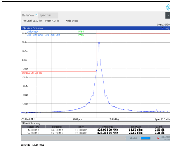
1-N5--15-10-L-1-DFT-PI2BPSK-Edge_1RB_Left-1@0-Ant0-seegraph-PASS-see graph
