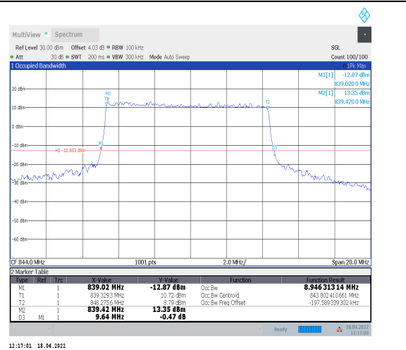
1-N5--15-10-H-3-DFT-16QAM-Outer_Full-50@0-Ant 0-8.946-9.640-≤10-PASS
