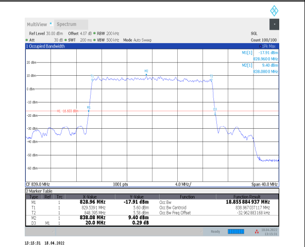
1-N5--15-20-H-9-CP-256QAM-Outer_Full-106@0-Ant-0-18.856-20.000-≤20-PASS
