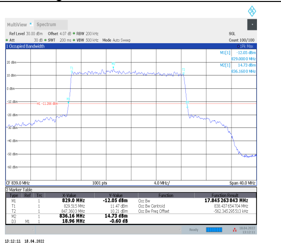
1-N5--15-20-H-3-DFT-16QAM-Outer_Full-100@0-An t0-17.845-18.960-≤20-PASS
