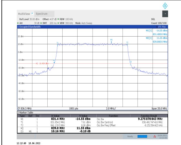
1-N5--15-10-M-7-CP-16QAM-Outer_Full-52@0-Ant0 -9.275-10.160≤10-PASS
