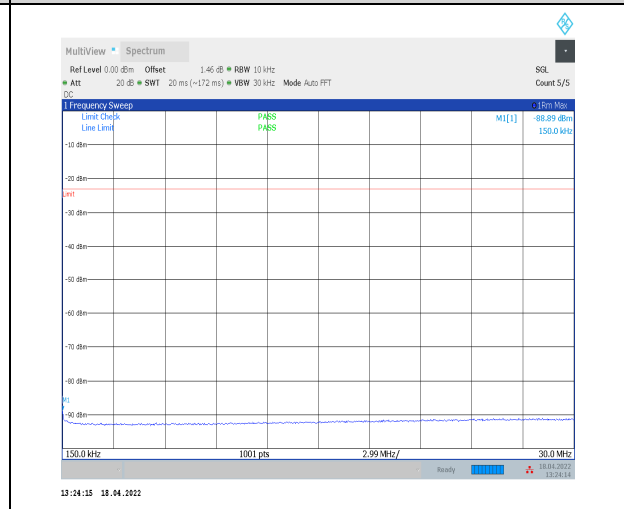
1-N5--15-20-H-1-DFT-PI2BPSK-Inner_1RB_Left-1@ 1-0.15-30-Ant0--88.89--23-PASS
