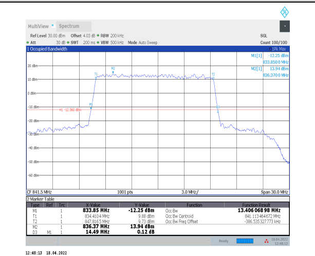
1-N5--15-15-H-4-DFT-64QAM-Outer_Full-75@0-Ant 0-13.406-14.490≤15-PASS
