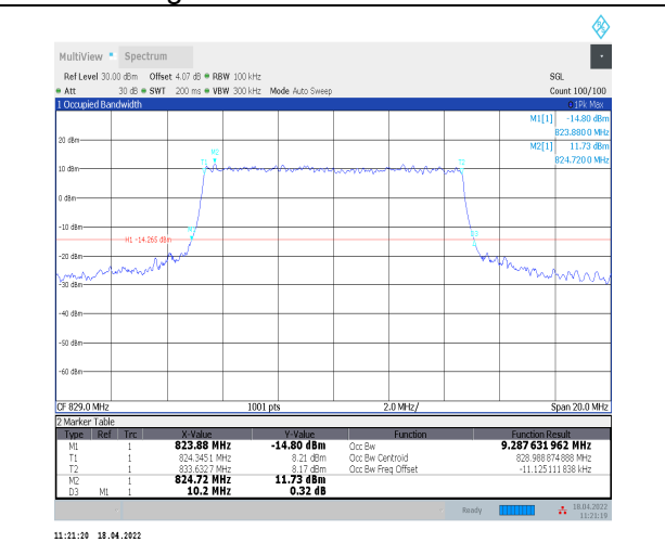
1-N5--15-10-L-7-CP-16QAM-Outer_Full-52@0-Ant0-9 9.288-10.200-≤10-PASS
