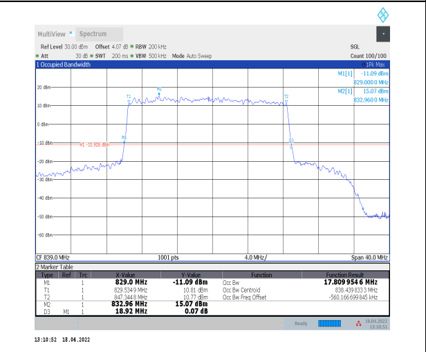
1-N5--15-20-H-1-DFT-QPSK-Outer_Full-100@0-Ant 0-17.81-18.920-≤20-PASS
