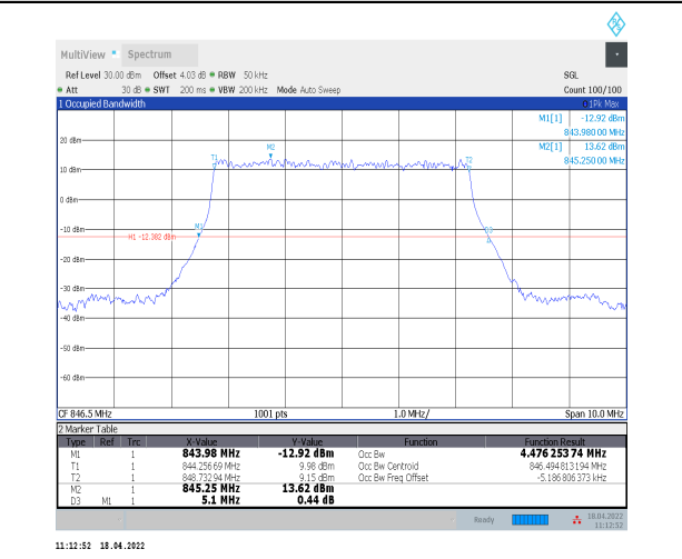
1-N5--15-5-H-2-DFT-PI2BPSK-Outer_Full-25@0-Ant0-4.476-5.100-≤5-PASS
