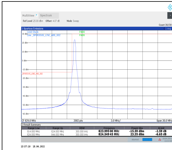
1-N5--15-20-L-1-DFT-PI2BPSK-Edge_1RB_Left-1@0-Ant0-seegraph-PASS-see graph
