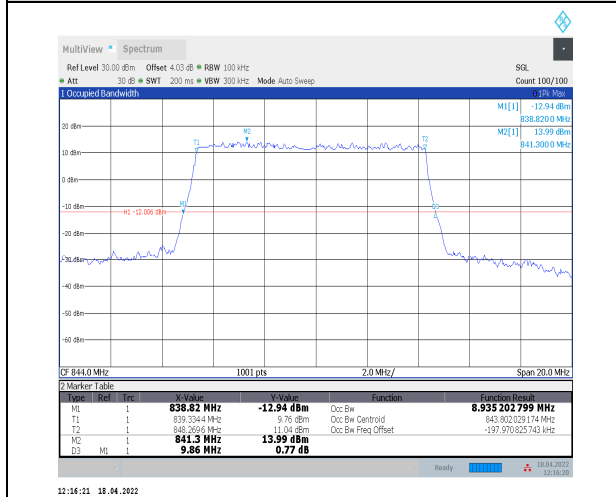
1-N5--15-10-H-2-DFT-PI2BPSK-Outer_Full-50@0-A nt0-8.935-9.860-≤10-PASS
