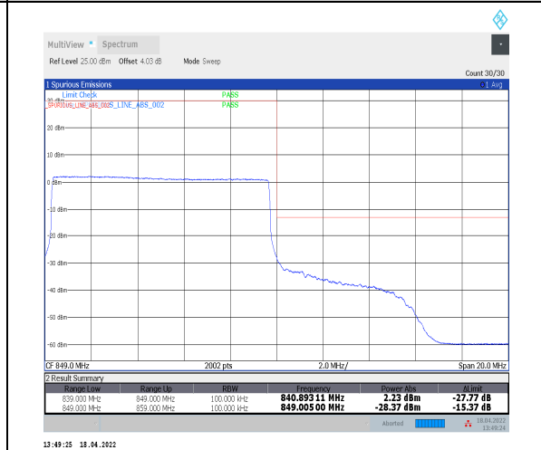
1-N5--15-10-H-6-CP-QPSK-Outer_Full-52@0-Ant0-seegraph-PASS-see graph
