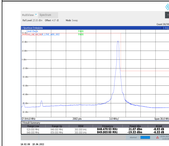
1-N5--15-20-H-5-CP-QPSK-Edge_1RB_Right-1@105-Ant0-seegraph-PASS-see graph
