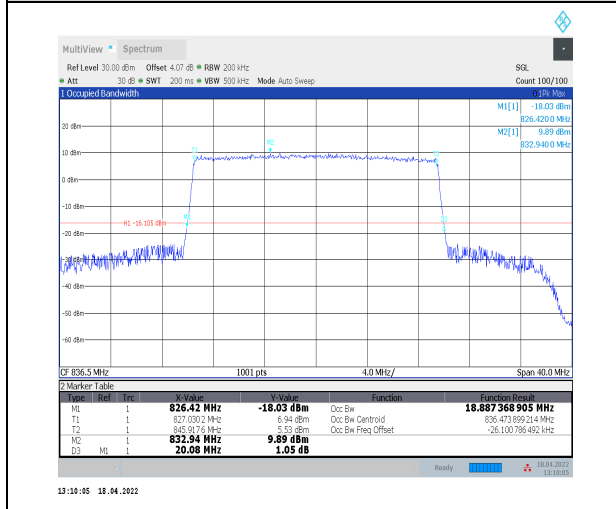
1-N5--15-20-M-9-CP-256QAM-Outer_Full-106@0-A nt0-18.887-20.080-≤20-PASS
