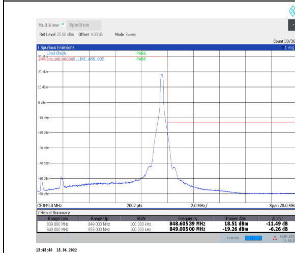
1-N5--15-10-H-5-CP-QPSK-Edge_1RB_Right-1@51-Ant0-seegraph-PASS-see graph
