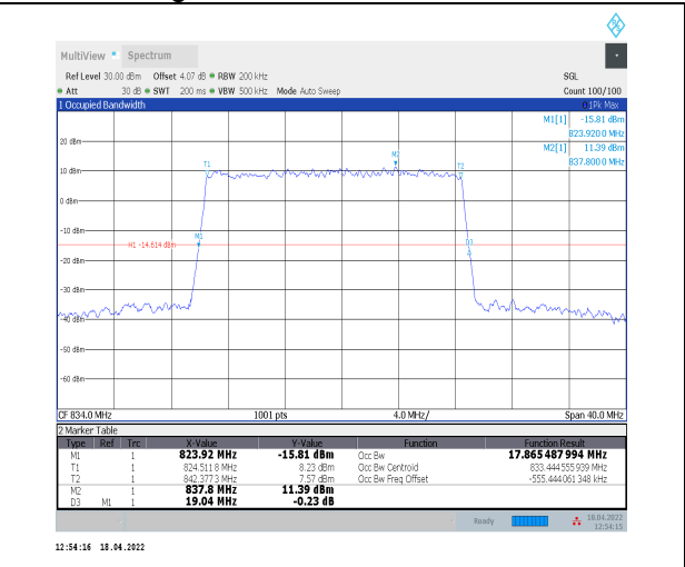
1-N5--15-20-L-5-DFT-256QAM-Outer_Full-100@0-Ant0-17.865-19.040-<20-PASS
