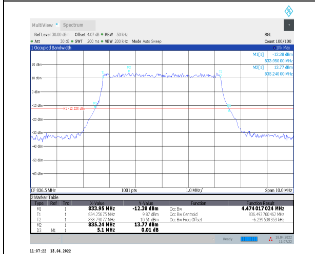
1-N5--15-5-M-2-DFT-PI2BPSK-Outer_Full-25@0-Ant0-4.474-5.100-<=5-PASS
