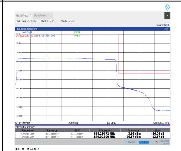
1-N5--15-20-H-6-CP-QPSK-Outer_Full-106@0-Ant0-seegraph-PASS-see graph
