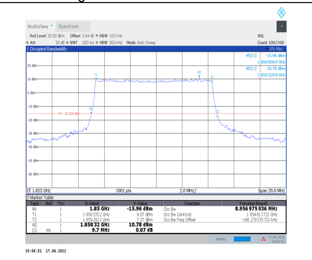
1-N2--15-10-L-3-DFT-16QAM-Outer_Full-50@0-Ant0 -8.957-9.700-≤10-PASS
