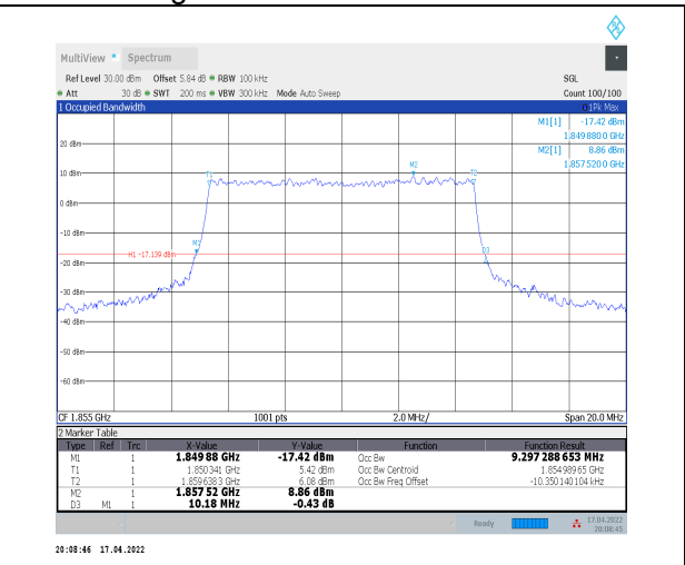
1-N2--15-10-L-7-CP-16QAM-Outer_Full-52@0-Ant0-9 9.297-10.180-≤10-PASS
