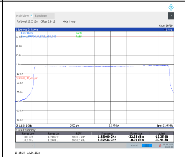
1-N2--15-10-L-6-CP-QPSK-Outer_Full-52@0-Ant0-seegraph-PASS-see graph
