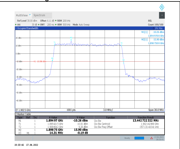
1-N2--15-15-H-2-DFT-PI2BPSK-Outer_Full-75@0-A nt0-13.443-14.310≤15-PASS
