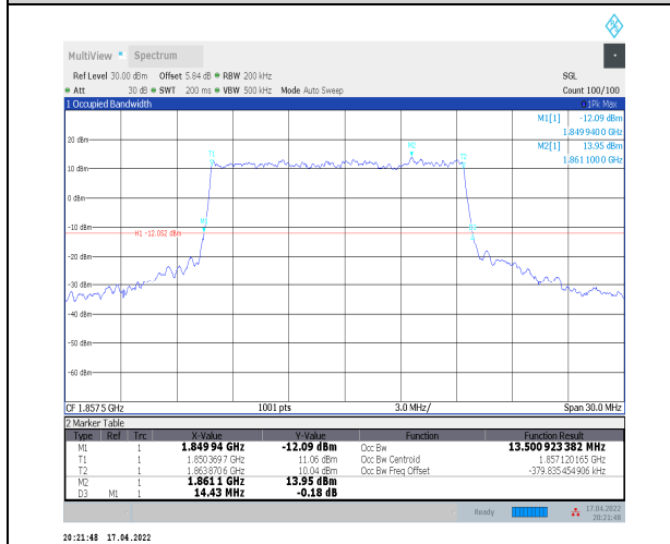
1-N2--15-15-L-1-DFT-QPSK-Outer_Full-75@0-Ant0 13.501-14.430≤15-PASS
