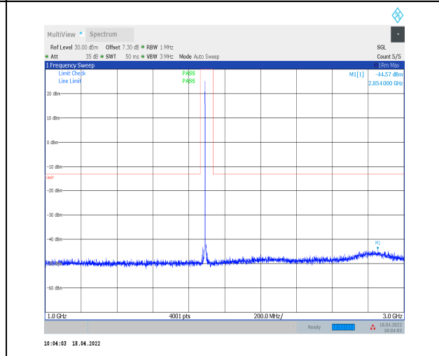
1-N2--15-20-H-1-DFT-PI2BPSK-Inner_1RB_Left-1@ 1-1000-3000-Ant0--44.57--13-PASS
