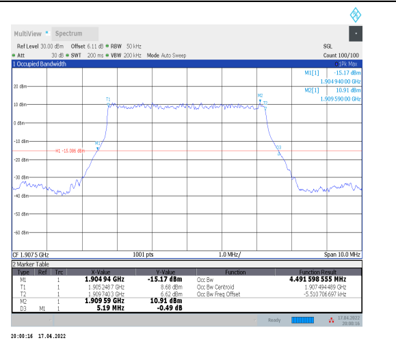
1-N2--15-5-H-2-DFT-PI2BPSK-Outer_Full-25@0-Ant0-4.492-5.190-≤5-PASS
