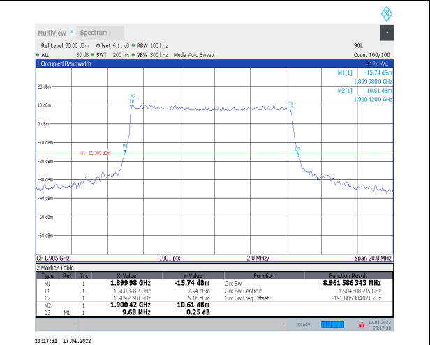
1-N2--15-10-H-3-DFT-16QAM-Outer_Full-50@0-Ant 0-8.962-9.680-≤10-PASS
