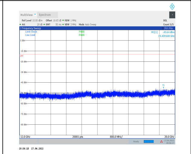
1-N2--15-20-M-1-DFT-PI2BPSK-Inner_1RB_Left-1@ 1-12000-20000-Ant0--45.64--13-PASS
