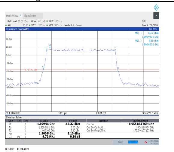
1-N2--15-10-H-5-DFT-256QAM-Outer_Full-50@0-An t0-8.956-9.720-<=10-PASS
