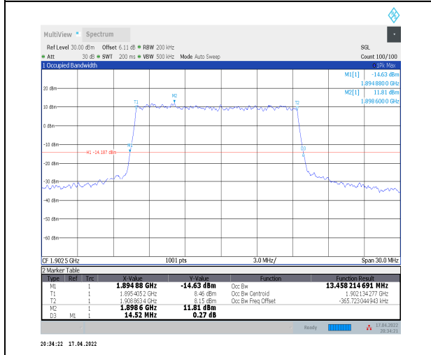
1-N2--15-15-H-3-DFT-16QAM-Outer_Full-75@0-Ant 0-13.458-14.520≤15-PASS
