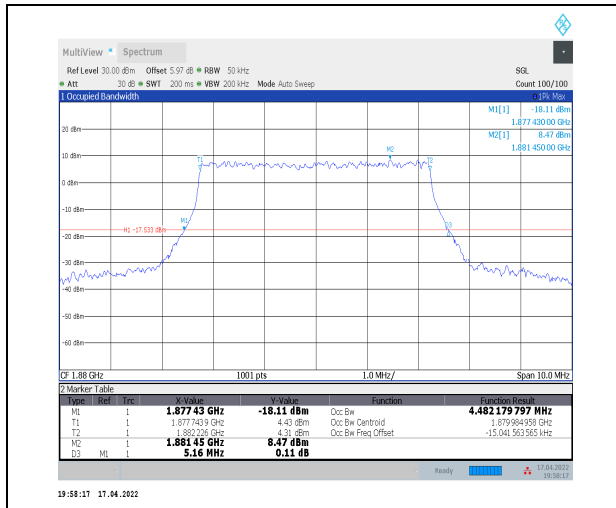
1-N2--15-5-M-8-CP-64QAM-Outer_Full-25@0-Ant0-4.482-5.160-≤5-PASS
