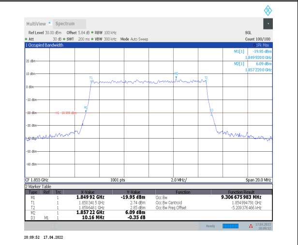
1-N2--15-10-L-9-CP-256QAM-Outer_Full-52@0-Ant0-9 9.307-10.160-≤10-PASS
