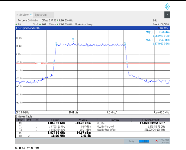
1-N2--15-20-M-2-DFT-PI2BPSK-Outer_Full-100@0-Ant 0-17.873-18.960-≤20-PASS
