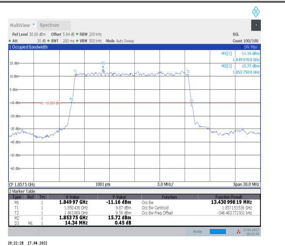
1-N2--15-15-L-2-DFT-PI2BPSK-Outer_Full-75@0-An t0-13.431-14.340≤15-PASS
