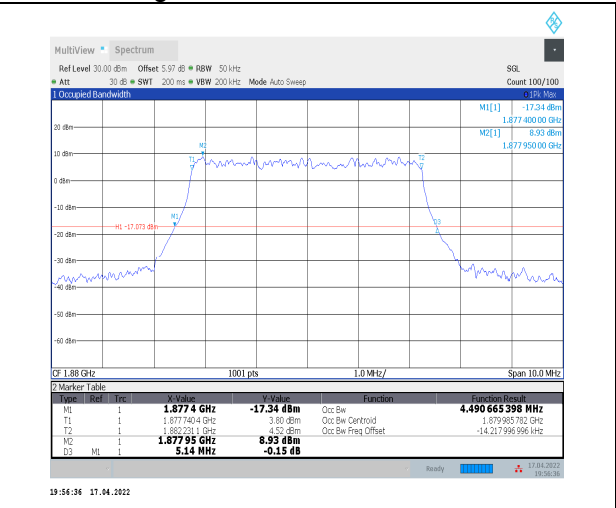
1-N2--15-5-M-5-DFT-256QAM-Outer_Full-25@0-Ant 0-4.491-5.140≤5-PASS
