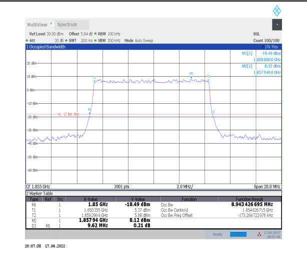
1-N2--15-10-L-5-DFT-256QAM-Outer_Full-50@0-Ant 0-8.943-9.620-≤10-PASS
