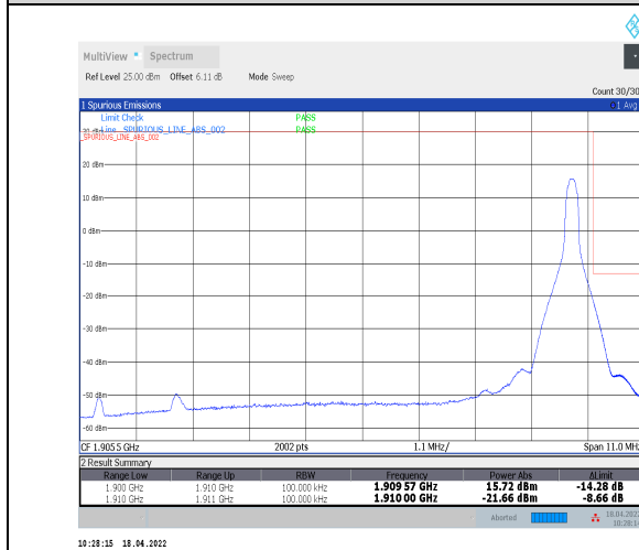
1-N2--15-10-H-5-CP-QPSK-Edge_1RB_Right-1@51-Ant0-seegraph-PASS-see graph
