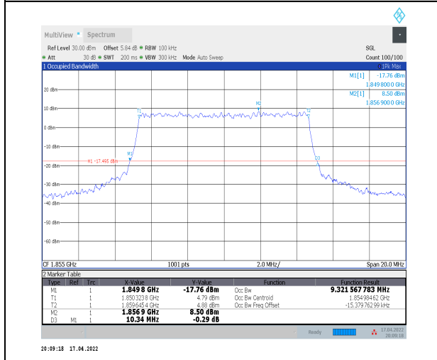
1-N2--15-10-L-8-CP-64QAM-Outer_Full-52@0-Ant0-9 9.322-10.340-≤10-PASS
