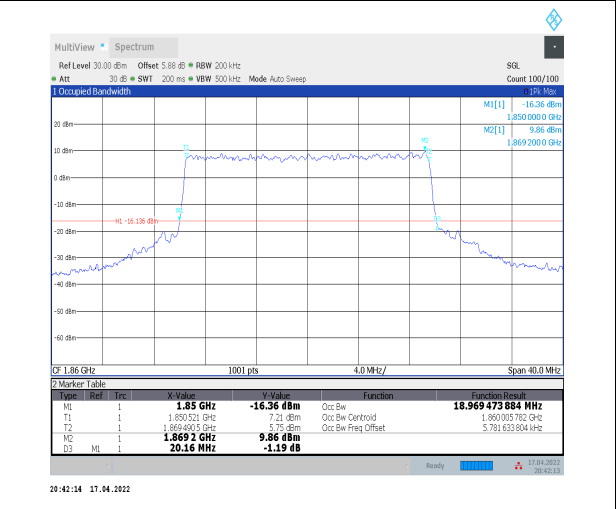
1-N2--15-20-L-7-CP-16QAM-Outer_Full-106@0-Ant0-18.969-20.160-<math>\leq 20</math>-PASS
