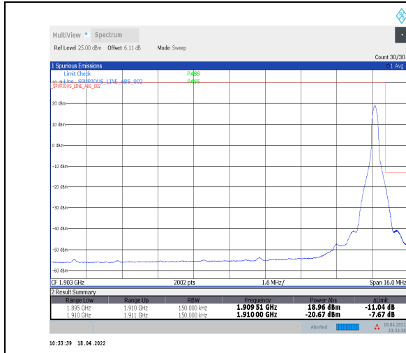
1-N2--15-15-H-2-DFT-PI2BPSK-Edge_1RB_Right-1@78-Ant0-seegraph-PASS-see graph
