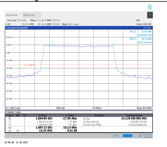
1-N2--15-15-H-6-CP-QPSK-Outer_Full-79@0-Ant0-1 4.129-15.240-<=15-PASS
