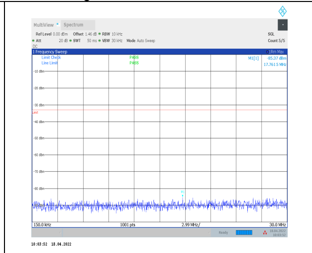
1-N2--15-20-H-1-DFT-PI2BPSK-Inner_1RB_Left-1@ 1-0.15-30-Ant0--85.37--33-PASS
