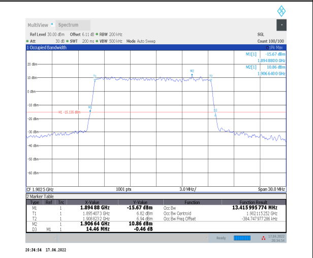
1-N2--15-15-H-4-DFT-64QAM-Outer_Full-75@0-Ant 0-13.416-14.460≤15-PASS
