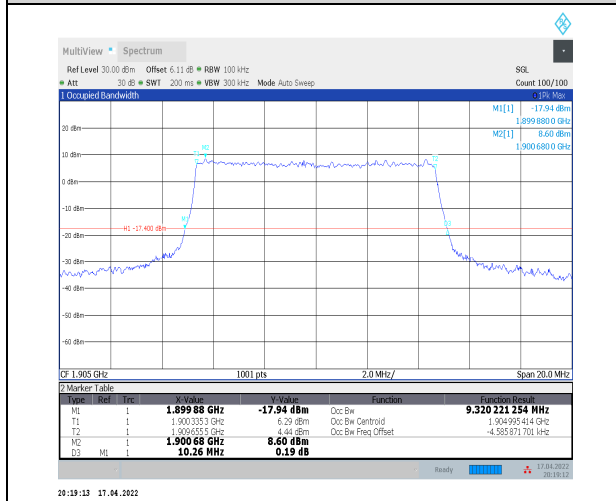
1-N2--15-10-H-6-CP-QPSK-Outer_Full-52@0-Ant0-9 .32-10.260-<=10-PASS
