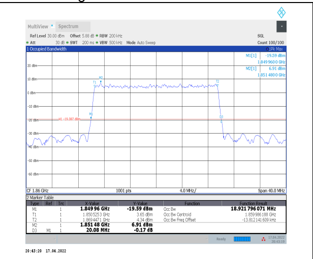
1-N2--15-20-L-9-CP-256QAM-Outer_Full-106@0-Ant 0-18.922-20.080-≤20-PASS
