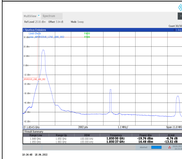
1-N2--15-10-L-4-CP-QPSK-Edge_1RB_Left-1@0-Ant0-seegraph-PASS-see graph
