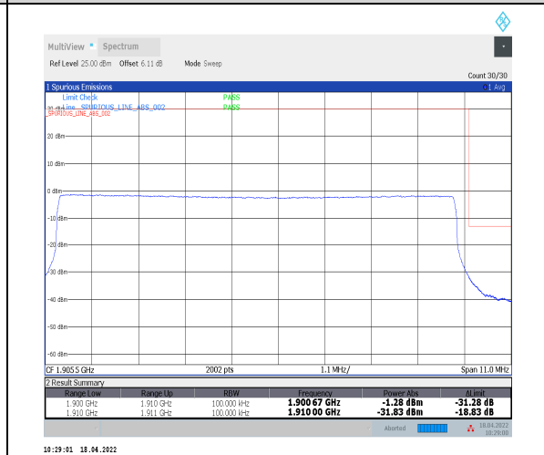
1-N2--15-10-H-6-CP-QPSK-Outer_Full-52@0-Ant0-seegraph-PASS-see graph
