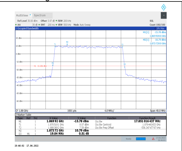
1-N2--15-20-M-4-DFT-64QAM-Outer_Full-100@0-An t0-17.851-19.040-≤20-PASS
