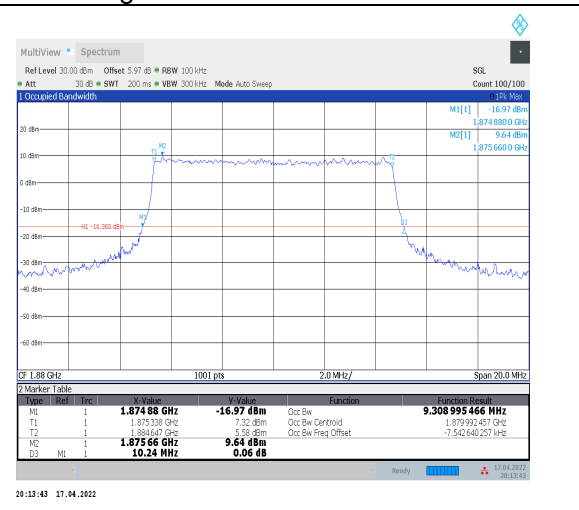
1-N2--15-10-M-6-CP-QPSK-Outer_Full-52@0-Ant0-9 .309-10.240-≤10-PASS
