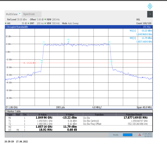
1-N2--15-20-L-3-DFT-16QAM-Outer_Full-100@0-Ant 0-17.877-18.920≤20-PASS
