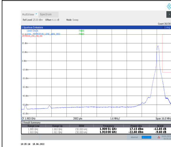
1-N2--15-15-H-5-CP-QPSK-Edge_1RB_Right-1@78-Ant0-seegraph-PASS-see graph
