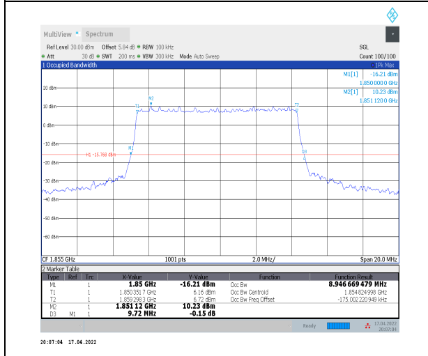
1-N2--15-10-L-4-DFT-64QAM-Outer_Full-50@0-Ant 0-8.947-9.720-≤10-PASS
