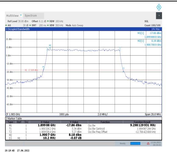
1-N2--15-10-H-7-CP-16QAM-Outer_Full-52@0-Ant0- 9.298-10.200-<=10-PASS
