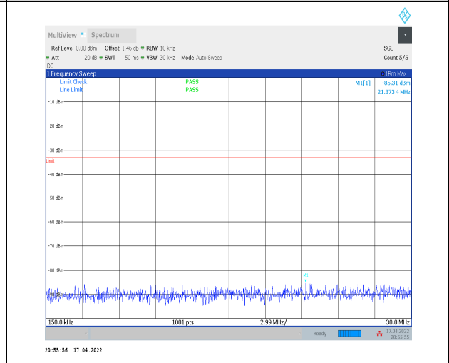
1-N2--15-20-M-1-DFT-PI2BPSK-Inner_1RB_Left-1@ 1-0.15-30-Ant0--85.31--33-PASS
