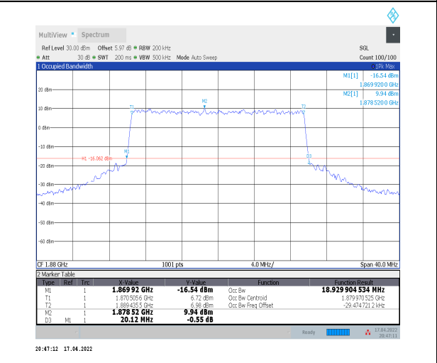
1-N2--15-20-M-6-CP-QPSK-Outer_Full-106@0-Ant0- 18.93-20.120-≤20-PASS
