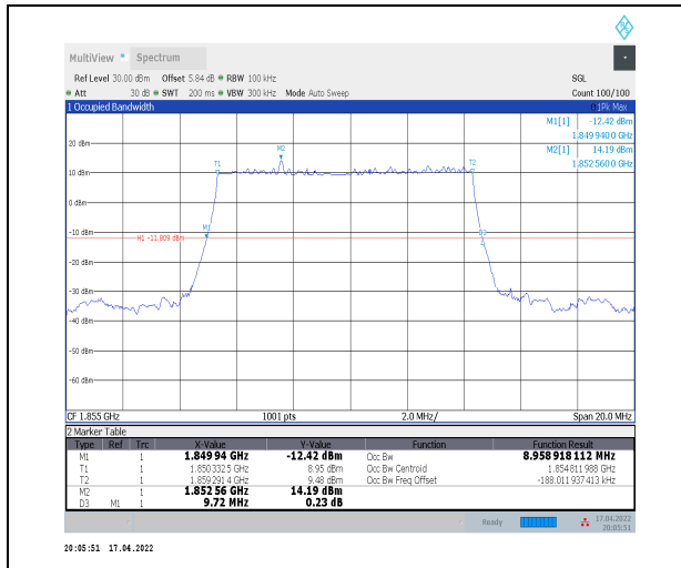
1-N2--15-10-L-2-DFT-PI2BPSK-Outer_Full-50@0-Ant t0-8.959-9.720-≤10-PASS
