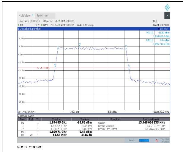
1-N2--15-15-H-5-DFT-256QAM-Outer_Full-75@0-Ant t0-13.448-14.580-<=15-PASS
