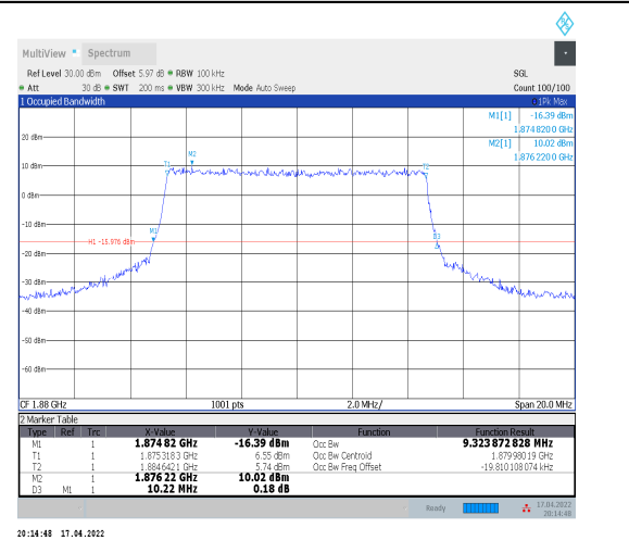
1-N2--15-10-M-8-CP-64QAM-Outer_Full-52@0-Ant0 -9.324-10.220-≤10-PASS
