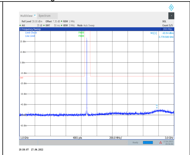
1-N2--15-20-M-1-DFT-PI2BPSK-Inner_1RB_Left-1@ 1-1000-3000-Ant0--43.94--13-PASS
