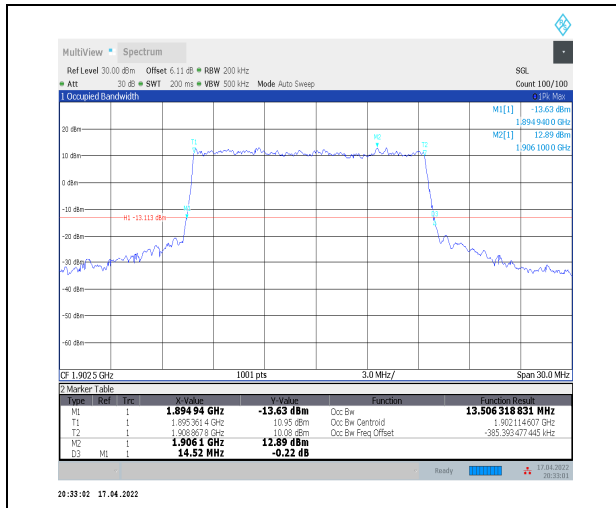
1-N2--15-15-H-1-DFT-QPSK-Outer_Full-75@0-Ant-0 13.506-14.520≤15-PASS
