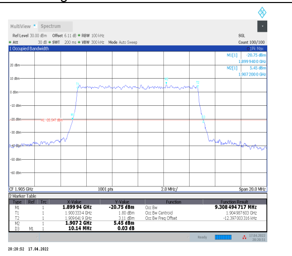
1-N2--15-10-H-9-CP-256QAM-Outer_Full-52@0-Ant 0-9.308-10.140≤10-PASS
