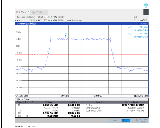
1-N2--15-10-H-2-DFT-PI2BPSK-Outer_Full-50@0-A nt0-8.968-9.680-≤10-PASS
