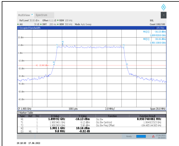
1-N2--15-10-H-4-DFT-64QAM-Outer_Full-50@0-Ant 0-8.951-9.800-<=10-PASS
