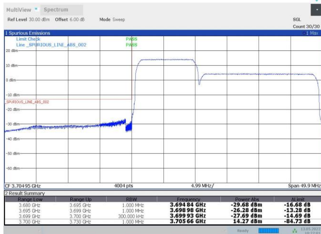
43-43-10MHz-20MHz-QPSK-QPSK-44645-44789-50RB#0-100RB#0
