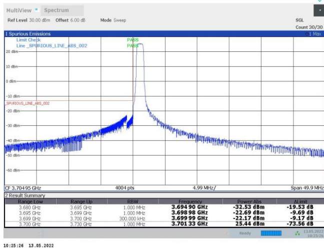
43-43-10MHz-20MHz-QPSK-QPSK-44645-44789-50RB#0-100RB#0
