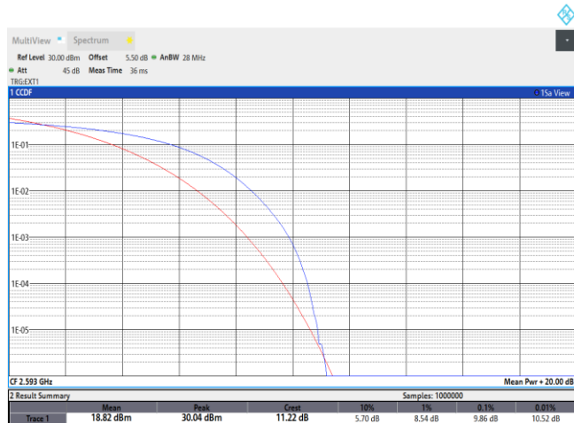
41-41-20MHz-20MHz-QPSK-QPSK-40521-40719-100RB#0-100RB#0
