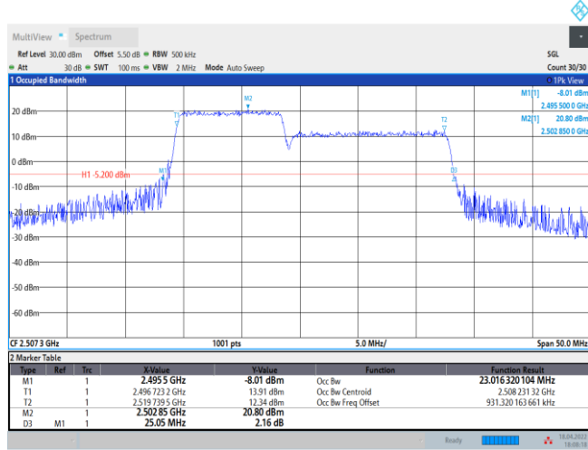
41-41-10MHz-15MHz-QPSK-QPSK-39703-39823-50RB#0-75RB#0
