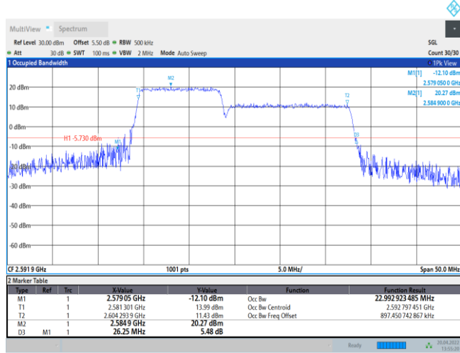
41-41-10MHz-15MHz-QPSK-QPSK-40549-40669-50RB#0-75RB#0
