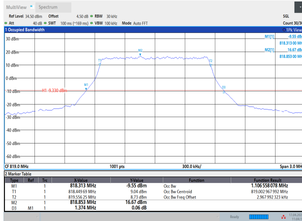
Band26-1.4MHz-QPSK-26740-6RB#0
