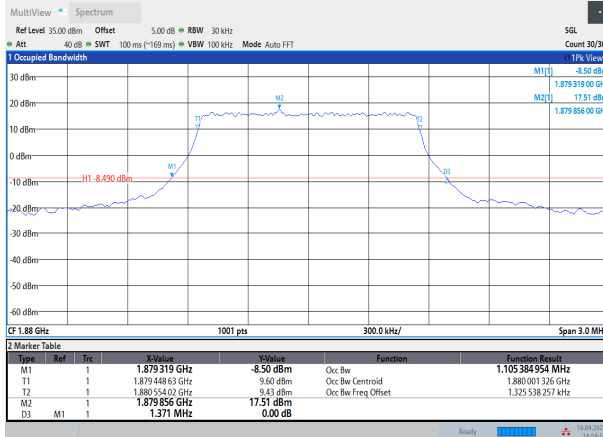
Band2-1.4MHz-QPSK-18900-6RB#0
