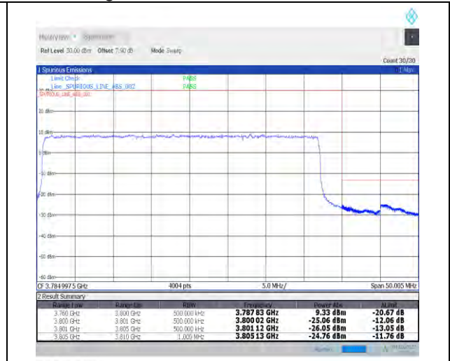
1-N78-3700-3800--30-40-H-3-DFT-PI2BPSK-Outer_Full-100@0-Ant0-PASS-see graph
