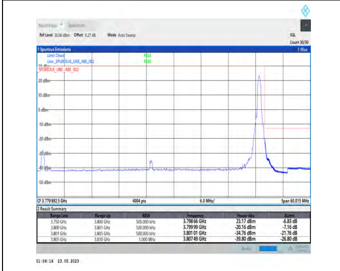
1-N78-3700-3800-PC1-30-50-H-5-CP-QPSK-Edge_1RB_Right-1@132-Ant0-1--PASS-see graph
