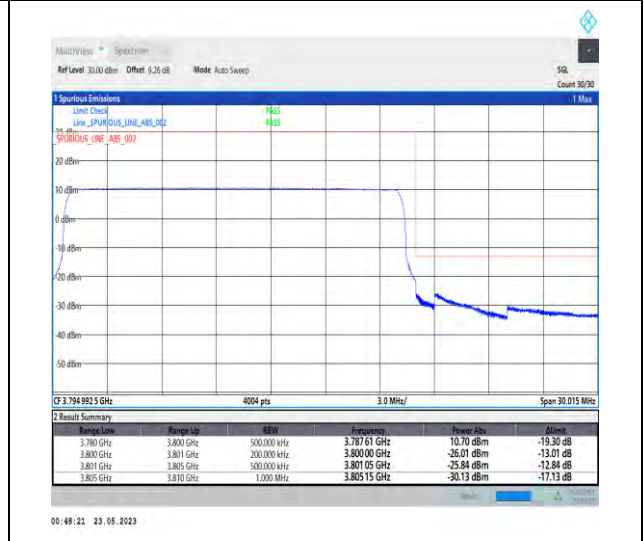
1-N78-3700-3800-PC1-30-20-H-6-CP-QPSK-Outer_Full-51@0-Ant0-1--PASS-see graph
