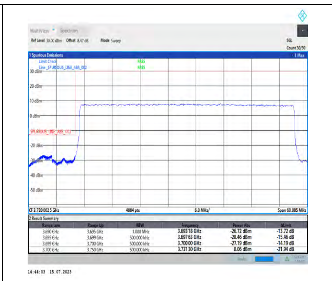
1-N78-3700-3800-PC1-30-50-L-3-DFT-PI2BPSK-Outer_Full-128@0-Ant0-1--PASS-see graph
