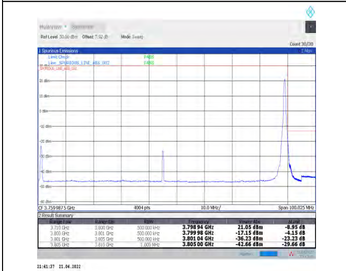
1-N78-3700-3800--30-90-H-5-CP-QPSK-Edge_1RB_R ight-1@244-Ant0-PASS-see graph
