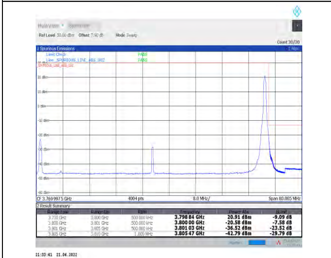
1-N78-3700-3800--30-70-H-5-CP-QPSK-Edge_1RB_R ight-1@188-Ant0-PASS-see graph
