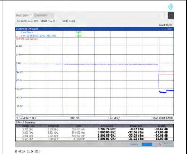
1-N78-3700-3800--30-100-H-6-CP-QPSK-Outer_F ull-273@0-Ant0-PASS-see graph
