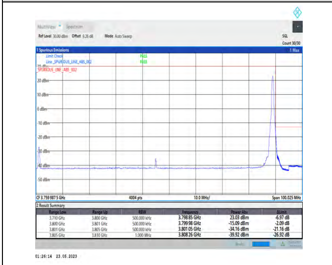
1-N78-3700-3800-PC1-30-90-H-5-CP-QPSK-Edge_1RB_Right-1@244-Ant0-1--PASS-see graph
