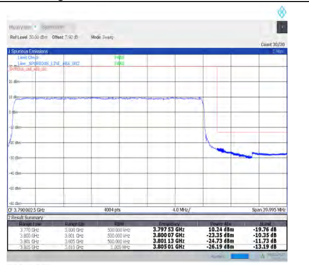
1-N78-3700-3800--30-30-H-3-DFT-PI2BPSK-Outer_Full-75@0-Ant0-PASS-see graph
