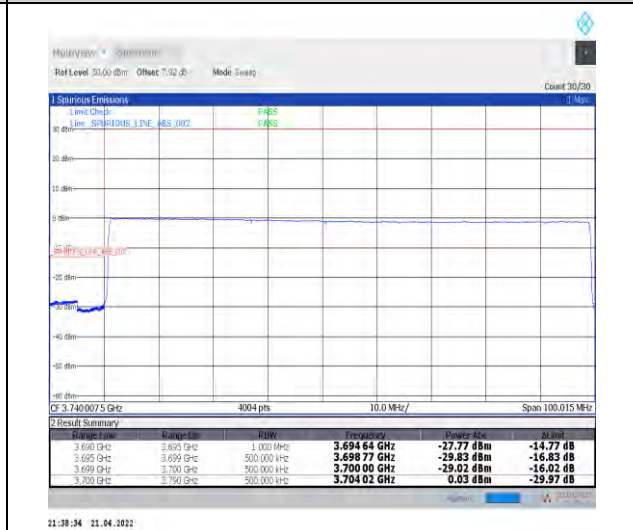
1-N78-3700-3800--30-90-L-6-CP-QPSK-Outer_Ful_I-245@0-Ant0-PASS-see graph
