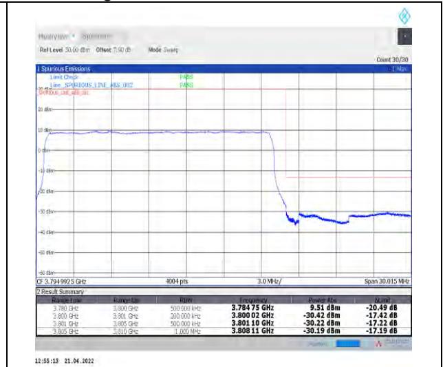
1-N78-3700-3800--30-20-H-3-DFT-PI2BPSK-Outer_Full-50@0-Ant0-PASS-see graph
