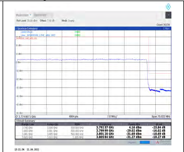
1-N78-3700-3800--30-60-H-3-DFT-PI2BPSK-Outer_Full-162@0-Ant0-PASS-see graph
