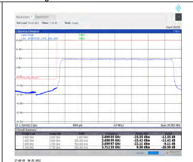
1-N78-3700-3800--30-30-L-3-DFT-PI2BPSK-Outer_Full-75@0-Ant0-PASS-see graph
