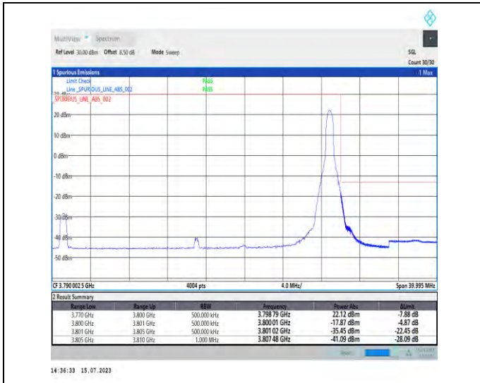
1-N78-3700-3800-PC1-30-30-H-2-DFT-PI2BPSK-Edge_1RB_Right-1@77-Ant0-1--PASS-see graph
