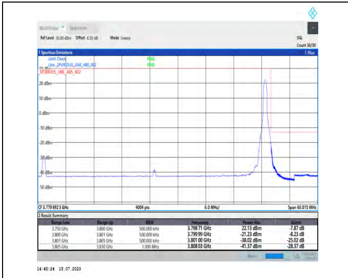
1-N78-3700-3800-PC1-30-50-H-2-DFT-PI2BPSK-Edge_1RB_Right-1@132-Ant0-1--PASS-see graph
