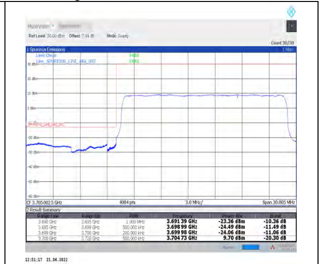
1-N78-3700-3800--30-20-L-3-DFT-PI2BPSK-Outer_Full-50@0-Ant0-PASS-see graph
