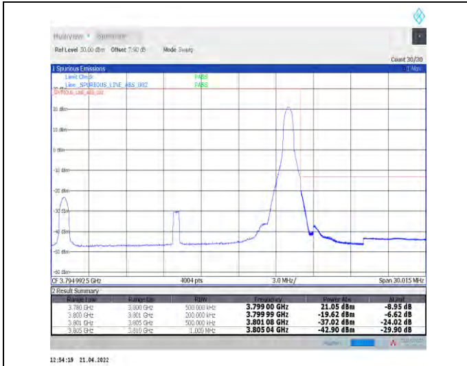
1-N78-3700-3800--30-20-H-2-DFT-PI2BPSK-Edge_1R_B_Right-1@50-Ant0-PASS-see graph
