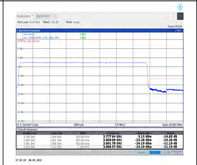
1-N78-3700-3800--30-40-H-6-CP-QPSK-Outer_Fu ll-106@0-Ant0-PASS-see graph
