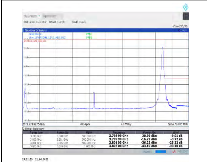
1-N78-3700-3800--30-60-H-5-CP-QPSK-Edge_1RB_R ight-1@161-Ant0-PASS-see graph
