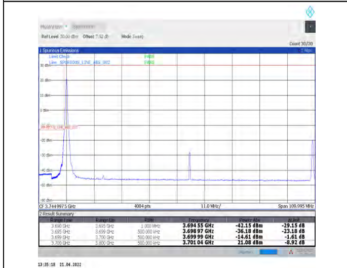
1-N78-3700-3800--30-100-L-4-CP-QPSK-Edge_1RB_Left-1@0-Ant0-PASS-see graph
