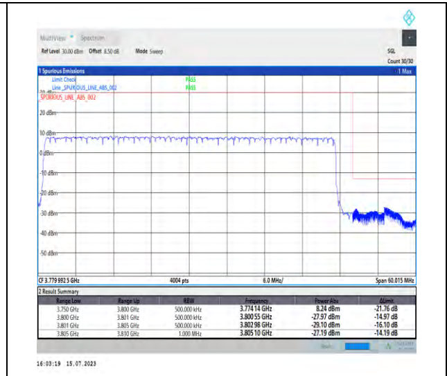
1-N78-3700-3800-PC1-30-50-H-3-DFT-PI2BPSK-Outer_Full-128@0-Ant0-1--PASS-see graph
