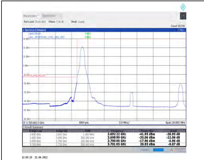
1-N78-3700-3800--30-20-L-1-DFT-PI2BPSK-Edge_1R_B_Left-1@0-Ant0-PASS-see graph
