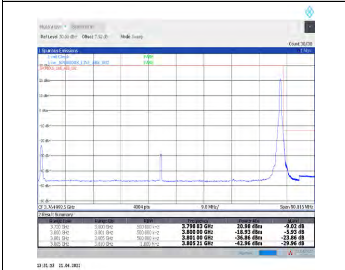
1-N78-3700-3800--30-80-H-5-CP-QPSK-Edge_1RB_R ight-1@216-Ant0-PASS-see graph
