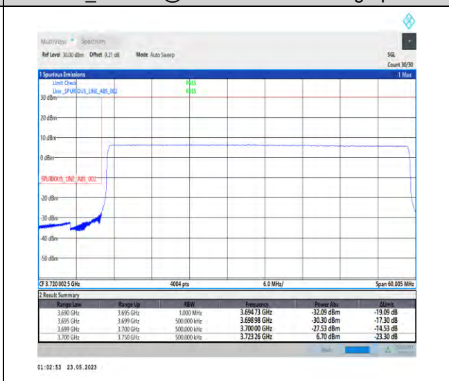
1-N78-3700-3800-PC1-30-50-L-6-CP-QPSK-Outer_Full-133@0-Ant0-1--PASS-see graph
