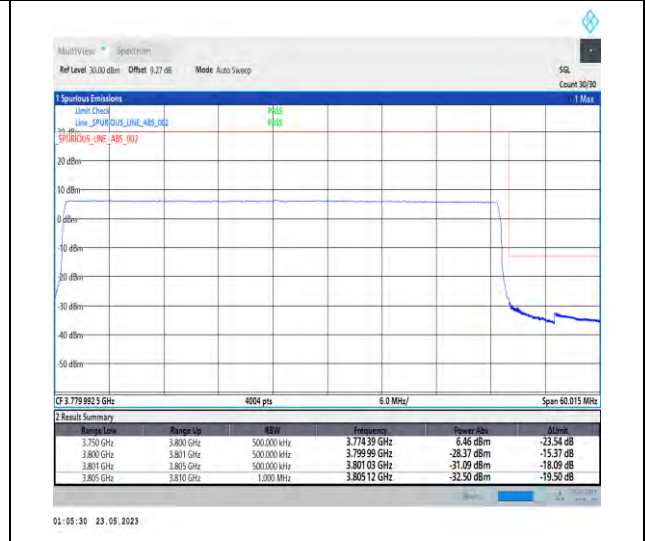
1-N78-3700-3800-PC1-30-50-H-6-CP-QPSK-Outer_Full-133@0-Ant0-1--PASS-see graph
