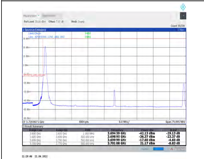
1-N78-3700-3800--30-70-L-4-CP-QPSK-Edge_1RB_L_eft-1@0-Ant0-PASS-see graph
