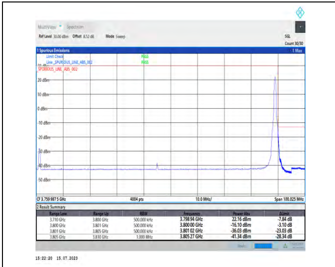
1-N78-3700-3800-PC1-30-90-H-2-DFT-PI2BPSK-Edge_1RB_Right-1@244-Ant0-1--PASS-see graph
