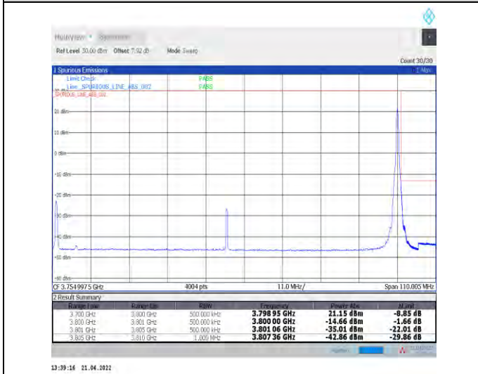
1-N78-3700-3800--30-100-H-5-CP-QPSK-Edge_1RB_Right-1@272-Ant0-PASS-see graph
