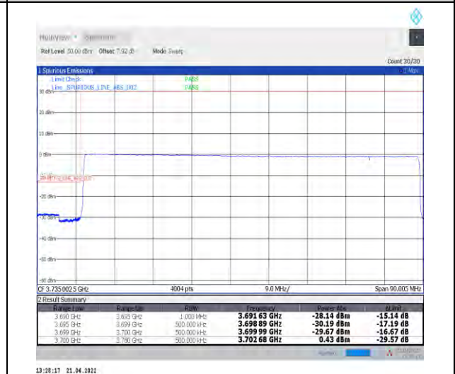
1-N78-3700-3800--30-80-L-6-CP-QPSK-Outer_Ful_I-217@0-Ant0-PASS-see graph
