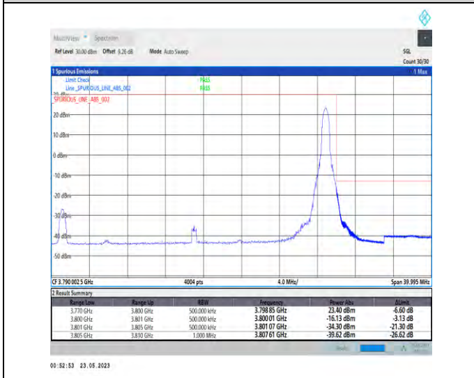
1-N78-3700-3800-PC1-30-30-H-5-CP-QPSK-Edge_1RB_Right-1@77-Ant0-1--PASS-see graph
