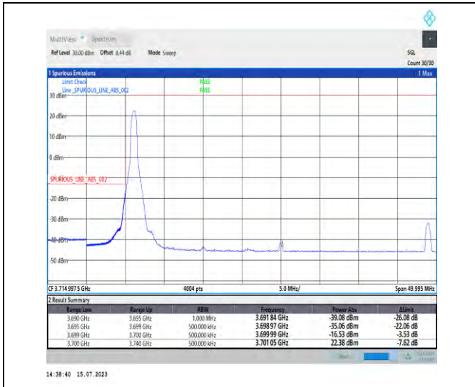
1-N78-3700-3800-PC1-30-40-L-1-DFT-PI2BPSK-Edge_1_RB_Left-1@0-Ant0-1--PASS-see graph
