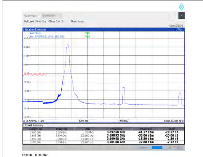
1-N78-3700-3800--30-30-L-4-CP-QPSK-Edge_1RB_L_eft-1@0-Ant0-PASS-see graph
