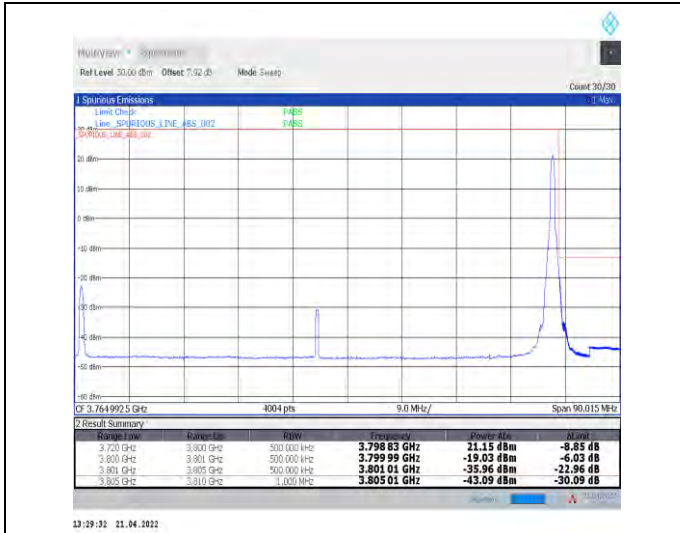
1-N78-3700-3800--30-80-H-2-DFT-PI2BPSK-Edge_1R_B_Right-1@216-Ant0-PASS-see graph
