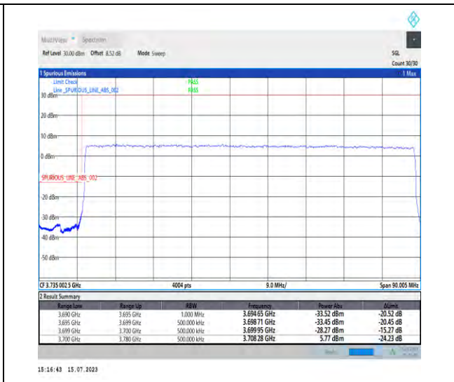
1-N78-3700-3800-PC1-30-80-L-3-DFT-PI2BPSK-Outer_Full-216@0-Ant0-1--PASS-see graph
