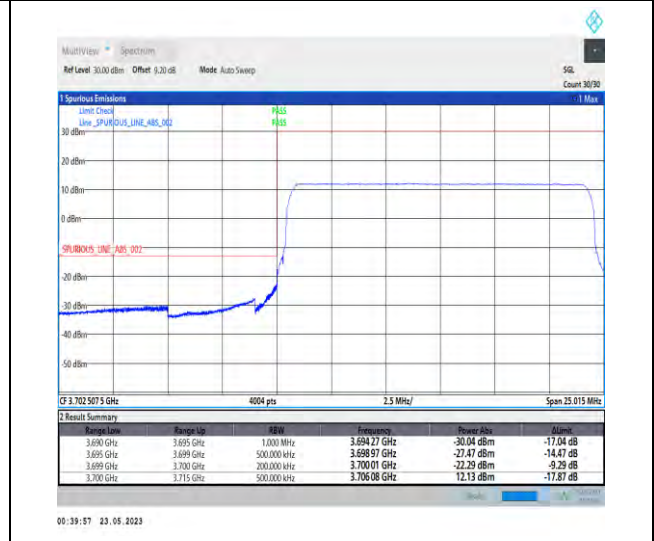
1-N78-3700-3800-PC1-30-15-L-6-CP-QPSK-Outer_Full-38@0-Ant0-1--PASS-see graph
