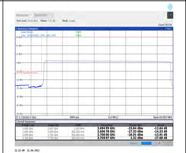
1-N78-3700-3800--30-50-L-6-CP-QPSK-Outer_Ful_I-133@0-Ant0-PASS-see graph
