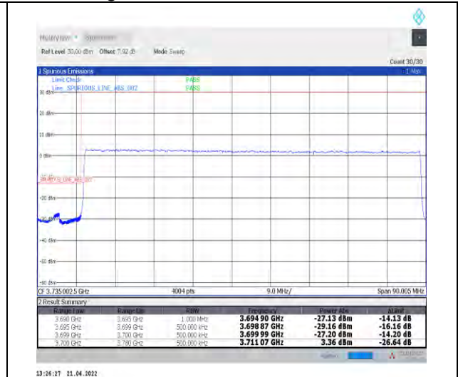
1-N78-3700-3800--30-80-L-3-DFT-PI2BPSK-Outer_Full-216@0-Ant0-PASS-see graph
