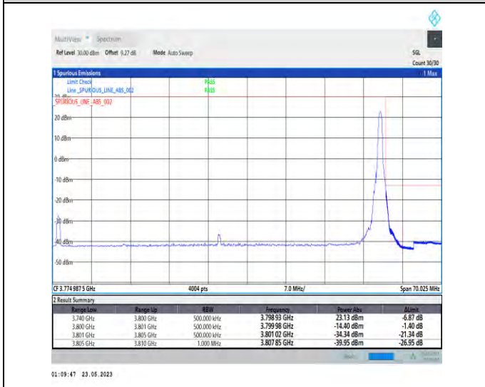
1-N78-3700-3800-PC1-30-60-H-5-CP-QPSK-Edge_1RB_Right-1@161-Ant0-1--PASS-see graph
