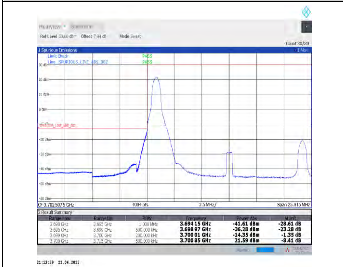
1-N78-3700-3800--30-15-L-4-CP-QPSK-Edge_1RB_L_eft-1@0-Ant0-PASS-see graph
