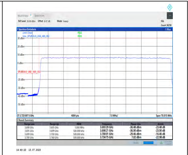
1-N78-3700-3800-PC1-30-60-L-3-DFT-PI2BPSK-Outer_Full-162@0-Ant0-1--PASS-see graph
