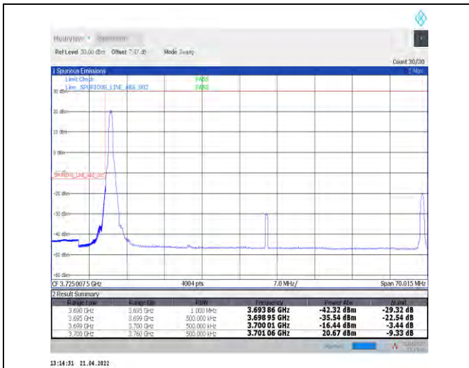
1-N78-3700-3800--30-60-L-1-DFT-PI2BPSK-Edge_1R_B_Left-1@0-Ant0-PASS-see graph
