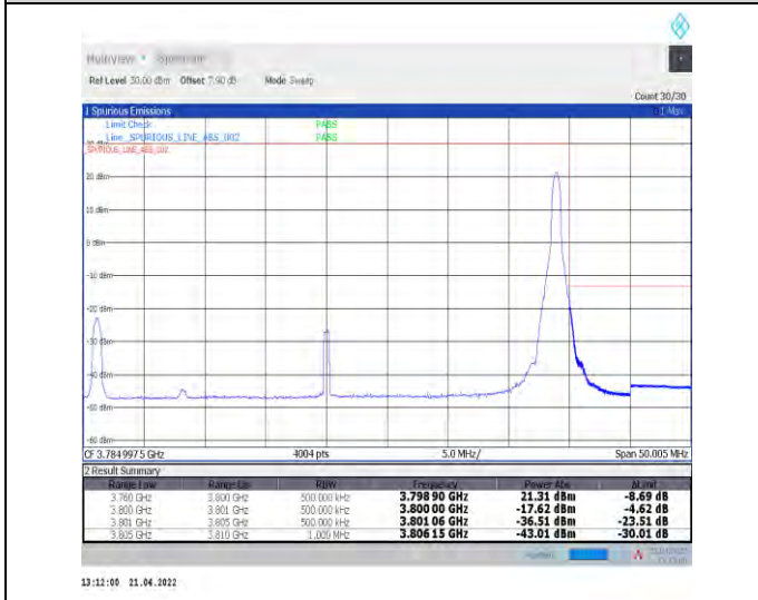
1-N78-3700-3800--30-40-H-5-CP-QPSK-Edge_1RB_R ight-1@105-Ant0-PASS-see graph
