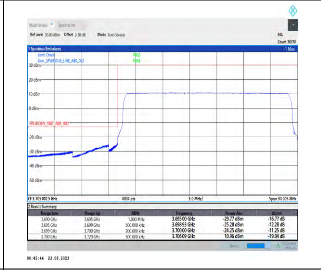
1-N78-3700-3800-PC1-30-20-L-6-CP-QPSK-Outer_Full-51@0-Ant0-1--PASS-see graph
