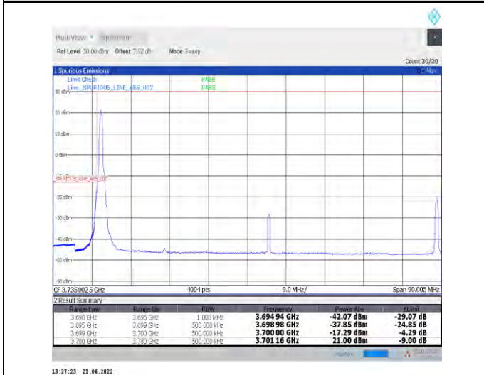
1-N78-3700-3800--30-80-L-4-CP-QPSK-Edge_1RB_L_eft-1@0-Ant0-PASS-see graph
