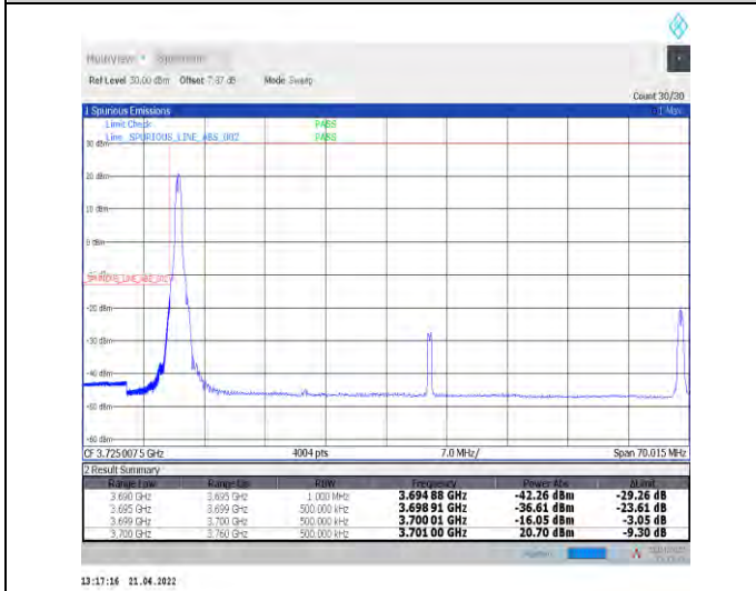
1-N78-3700-3800--30-60-L-4-CP-QPSK-Edge_1RB_L_eft-1@0-Ant0-PASS-see graph
