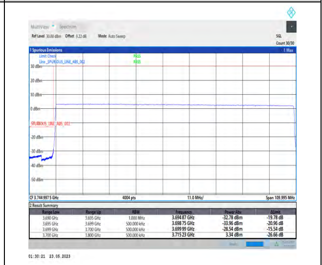
1-N78-3700-3800-PC1-30-100-L-6-CP-QPSK-Outer_Full-273@0-Ant0-1--PASS-see graph
