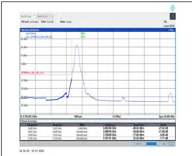
1-N78-3700-3800-PC1-30-20-L-1-DFT-PI2BPSK-Edge_e_1RB_Left-1@0-Ant0-1--PASS-see graph
