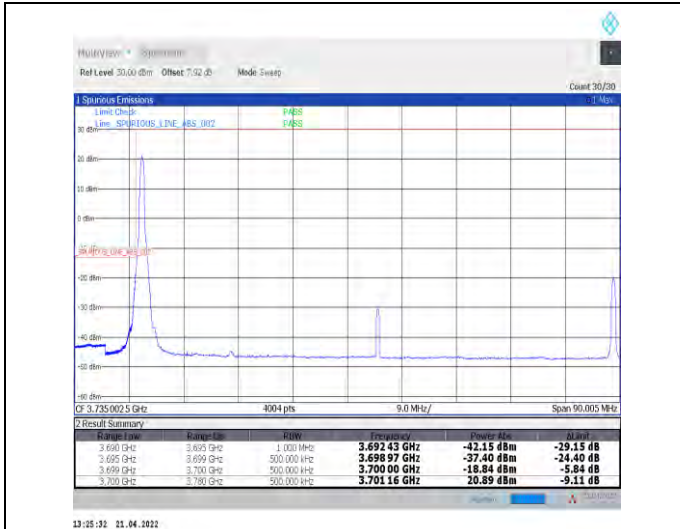
1-N78-3700-3800--30-80-L-1-DFT-PI2BPSK-Edge_1R_B_Left-1@0-Ant0-PASS-see graph
