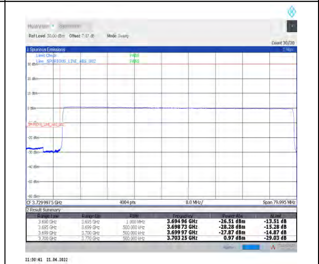
1-N78-3700-3800--30-70-L-6-CP-QPSK-Outer_Ful_I-189@0-Ant0-PASS-see graph
