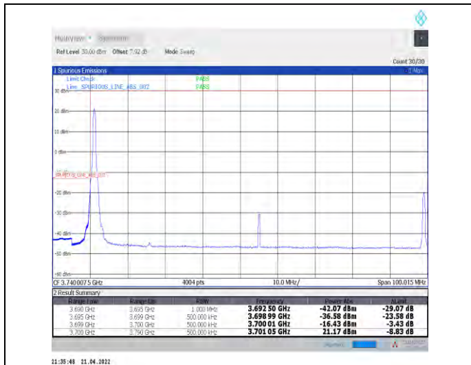
1-N78-3700-3800--30-90-L-1-DFT-PI2BPSK-Edge_1R_B_Left-1@0-Ant0-PASS-see graph
