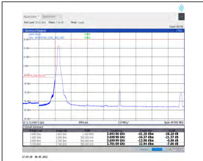
1-N78-3700-3800--30-40-L-1-DFT-PI2BPSK-Edge_1R_B_Left-1@0-Ant0-PASS-see graph
