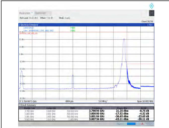
1-N78-3700-3800--30-40-H-2-DFT-PI2BPSK-Edge_1R_B_Right-1@105-Ant0-PASS-see graph
