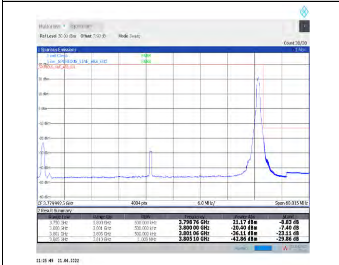
1-N78-3700-3800--30-50-H-5-CP-QPSK-Edge_1RB_R ight-1@132-Ant0-PASS-see graph
