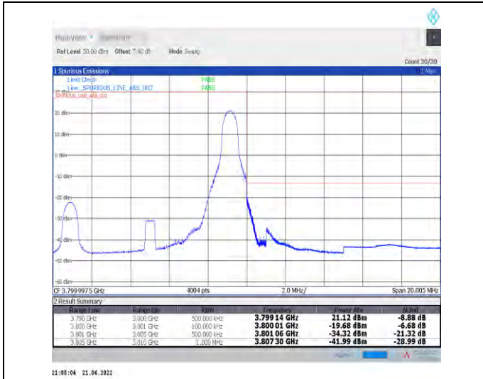
1-N78-3700-3800--30-10-H-2-DFT-PI2BPSK-Edge_1R B_Right-1@23-Ant0-PASS-see graph
