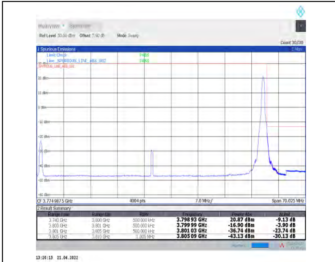
1-N78-3700-3800--30-60-H-2-DFT-PI2BPSK-Edge_1R_B_Right-1@161-Ant0-PASS-see graph
