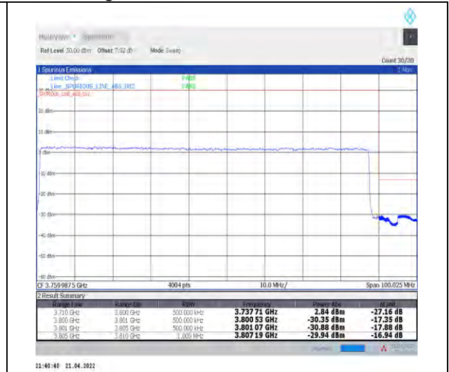
1-N78-3700-3800--30-90-H-3-DFT-PI2BPSK-Outer_Full-240@0-Ant0-PASS-see graph
