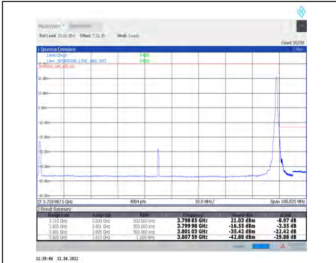
1-N78-3700-3800--30-90-H-2-DFT-PI2BPSK-Edge_1R_B_Right-1@244-Ant0-PASS-see graph
