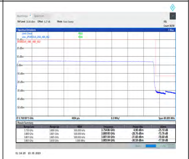
1-N78-3700-3800-PC1-30-70-H-6-CP-QPSK-Outer_Full-189@0-Ant0-1--PASS-see graph
