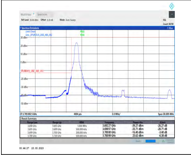
1-N78-3700-3800-PC1-30-20-L-4-CP-QPSK-Edge_1RB_Left-1@0-Ant0-1--PASS-see graph
