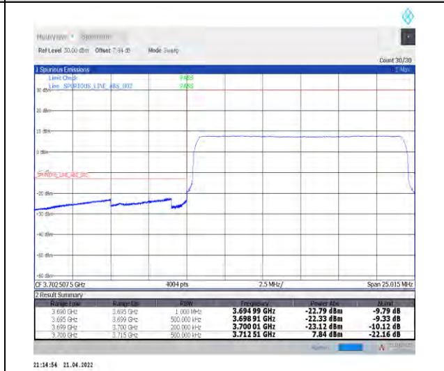
1-N78-3700-3800--30-15-L-6-CP-QPSK-Outer_Ful l-38@0-Ant0-PASS-see graph
