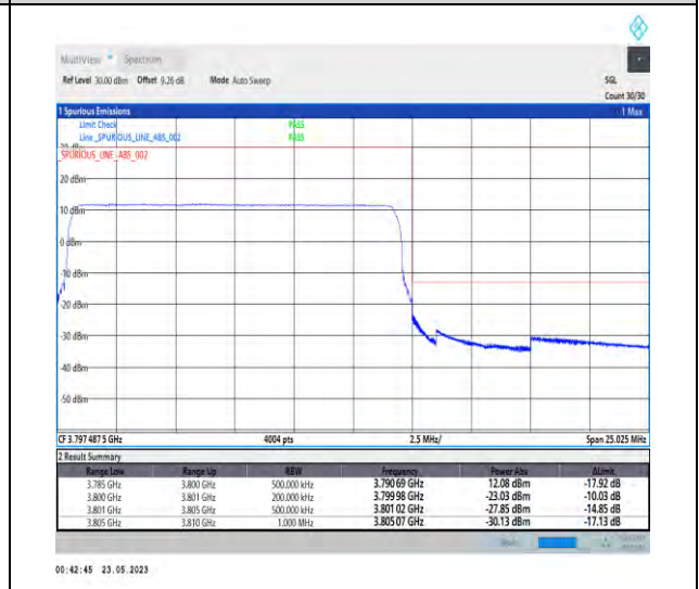
1-N78-3700-3800-PC1-30-15-H-6-CP-QPSK-Outer_Full-38@0-Ant0-1--PASS-see graph
