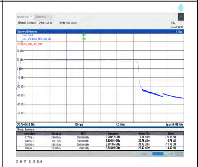
1-N78-3700-3800-PC1-30-30-H-6-CP-QPSK-Outer_Full-78@0-Ant0-1--PASS-see graph
