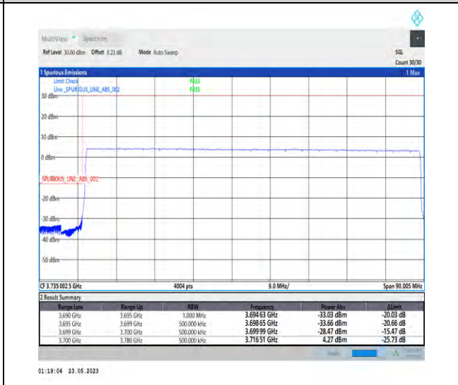
1-N78-3700-3800-PC1-30-80-L-6-CP-QPSK-Outer_Full-217@0-Ant0-1--PASS-see graph
