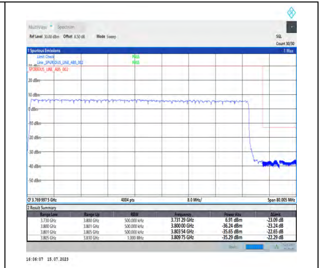
1-N78-3700-3800-PC1-30-70-H-3-DFT-PI2BPSK-Outer_Full-180@0-Ant0-1--PASS-see graph
