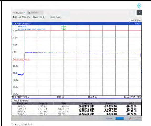
1-N78-3700-3800--30-100-L-6-CP-QPSK-Outer_F ull-273@0-Ant0-PASS-see graph
