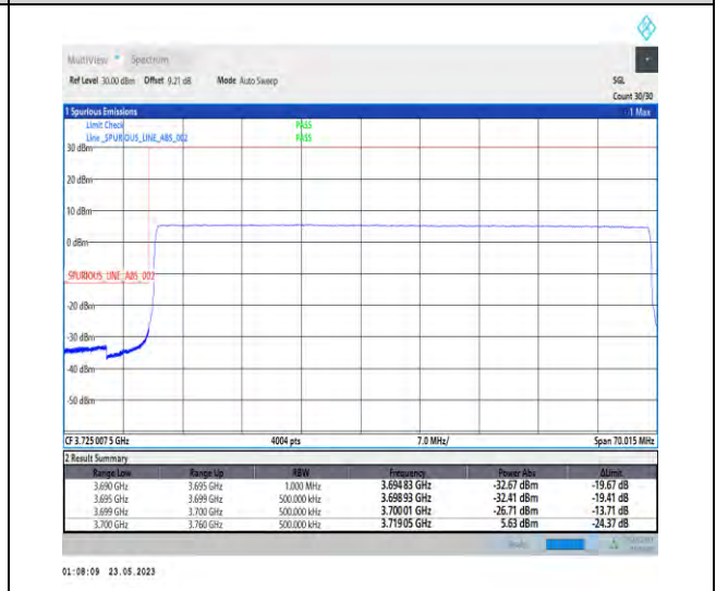
1-N78-3700-3800-PC1-30-60-L-6-CP-QPSK-Outer_Full-162@0-Ant0-1--PASS-see graph
