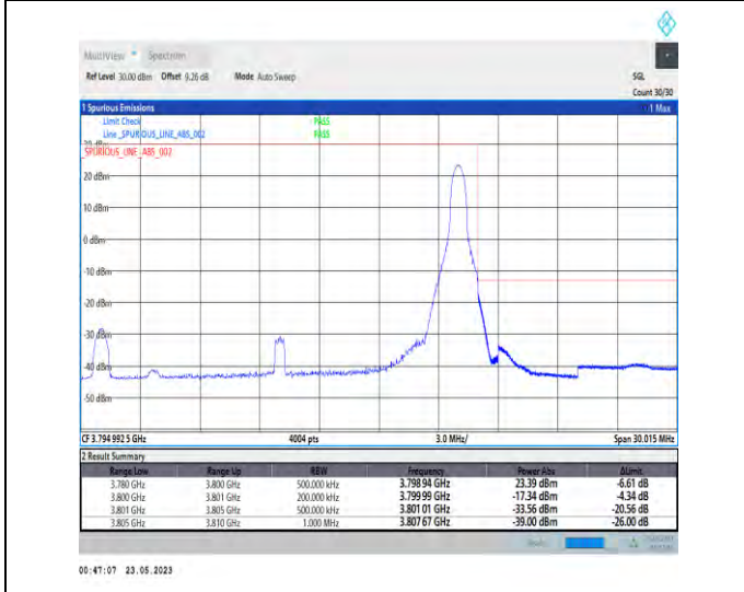
1-N78-3700-3800-PC1-30-20-H-5-CP-QPSK-Edge_1RB_Right-1@50-Ant0-1--PASS-see graph
