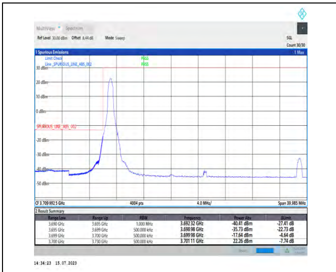
1-N78-3700-3800-PC1-30-30-L-1-DFT-PI2BPSK-Edge_e_1RB_Left-1@0-Ant0-1--PASS-see graph
