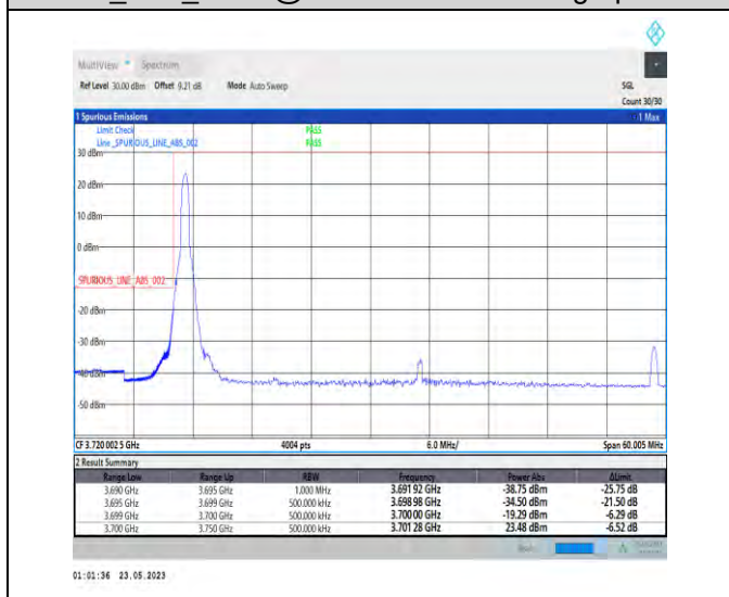
1-N78-3700-3800-PC1-30-50-L-4-CP-QPSK-Edge_1_RB_Left-1@0-Ant0-1--PASS-see graph
