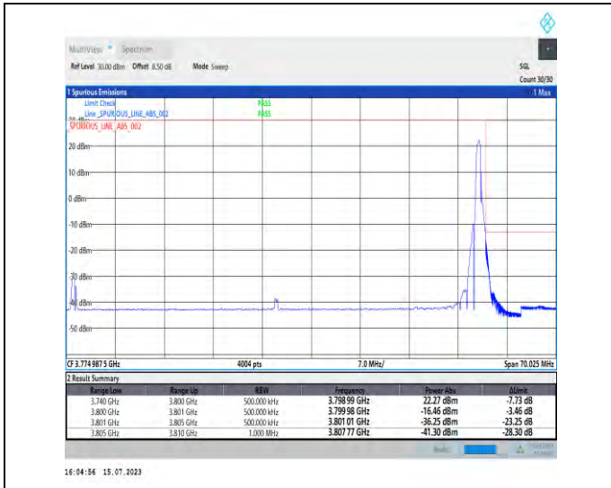
1-N78-3700-3800-PC1-30-60-H-2-DFT-PI2BPSK-Edge_1RB_Right-1@161-Ant0-1--PASS-see graph
