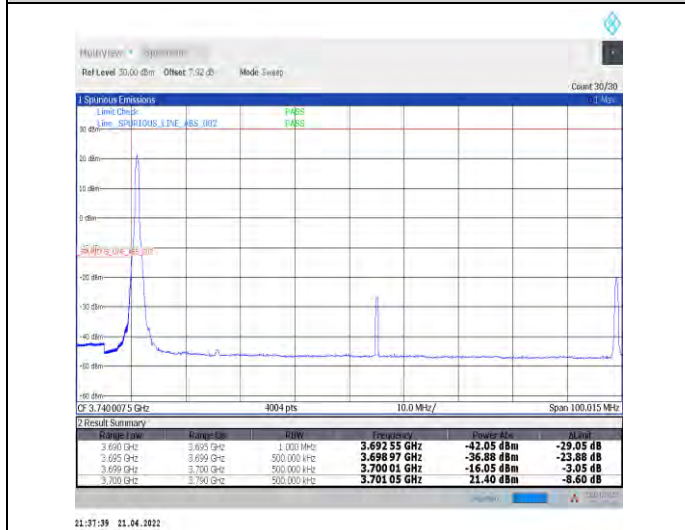
1-N78-3700-3800--30-90-L-4-CP-QPSK-Edge_1RB_L_eft-1@0-Ant0-PASS-see graph
