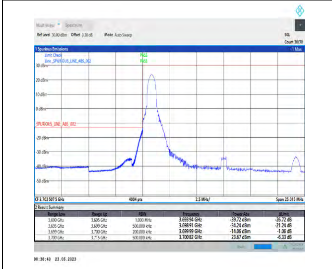
1-N78-3700-3800-PC1-30-15-L-4-CP-QPSK-Edge_1RB_Left-1@0-Ant0-1--PASS-see graph
