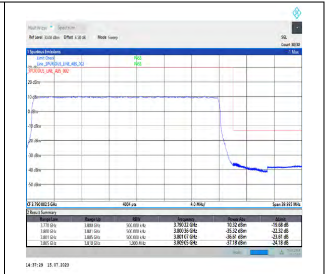
1-N78-3700-3800-PC1-30-30-H-3-DFT-PI2BPSK-Outer_Full-75@0-Ant0-1--PASS-see graph
