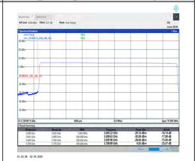
1-N78-3700-3800-PC1-30-70-L-6-CP-QPSK-Outer_Full-189@0-Ant0-1--PASS-see graph
