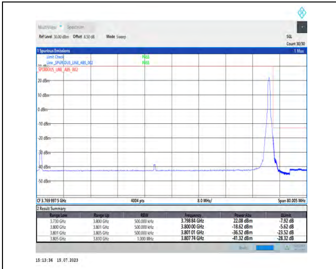
1-N78-3700-3800-PC1-30-70-H-2-DFT-PI2BPSK-Edge_1RB_Right-1@188-Ant0-1--PASS-see graph
