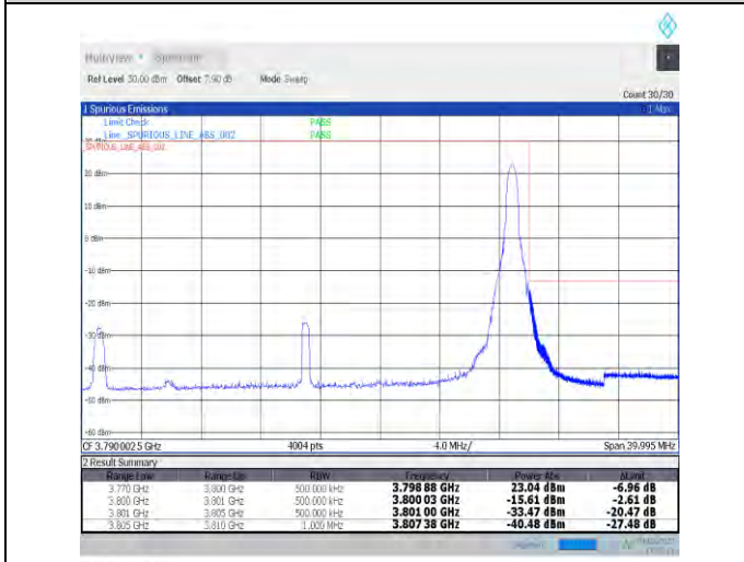
1-N78-3700-3800--30-30-H-2-DFT-PI2BPSK-Edge_1R_B_Right-1@77-Ant0-PASS-see graph
