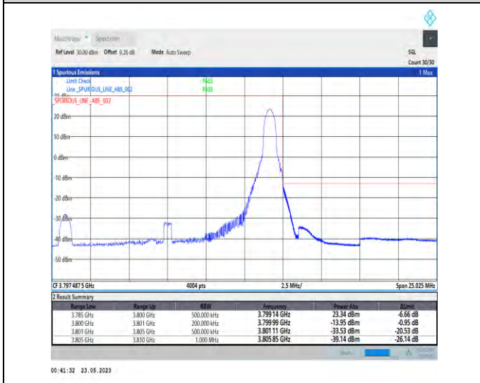
1-N78-3700-3800-PC1-30-15-H-5-CP-QPSK-Edge_1RB_Right-1@37-Ant0-1--PASS-see graph
