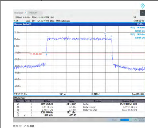
1-N78-3700-3800-PC1-30-100-L-8-CP-64QAM-Outer_Full-273@0-Ant0-97.21-100.800-≤100-PASS
