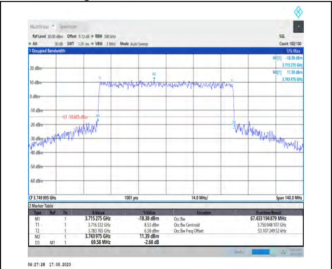
1-N78-3700-3800-PC1-30-70-M-8-CP-64QAM-Outer _Full-189@0-Ant0-67.433-69.580-≤70-PASS
