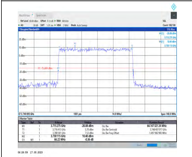
1-N78-3700-3800-PC1-30-70-M-5-DFT-256QAM-Outer_Full-180@0-Ant0-64.167-66.220-≤70-PASS
