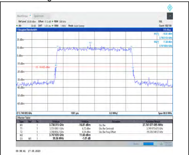
1-N78-3700-3800-PC1-30-40-M-9-CP-256QAM-Outer_Full-106@0-Ant0-37.761-39.360-≤40-PASS
