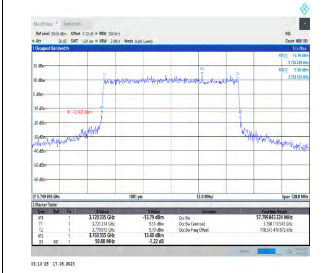
1-N78-3700-3800-PC1-30-60-M-8-CP-64QAM-Outer_Full-162@0-Ant0-57.8-59.880-≤60-PASS
