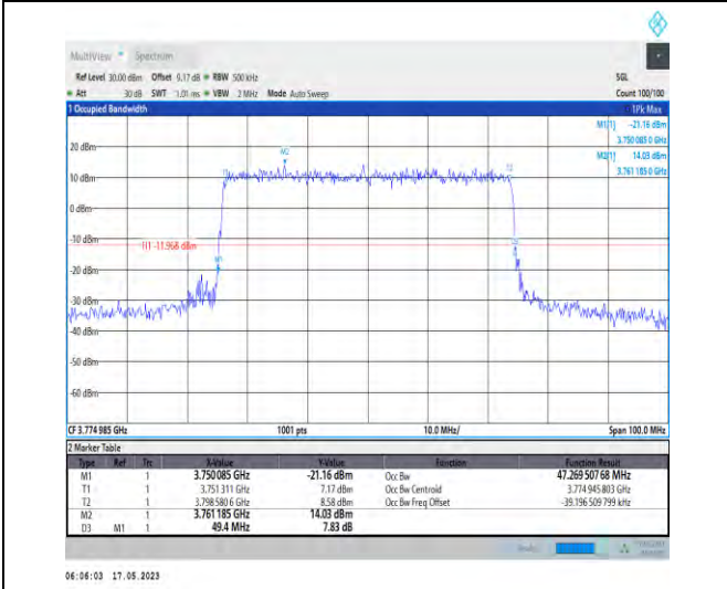
1-N78-3700-3800-PC1-30-50-H-6-CP-QPSK-Outer_Full-133@0-Ant0-47.27-49.400-≤50-PASS
