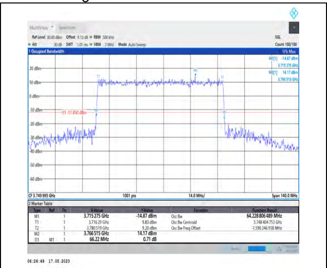
1-N78-3700-3800-PC1-30-70-M-4-DFT-64QAM-Outer_Full-180@0-Ant0-64.229-66.220-≤70-PASS
