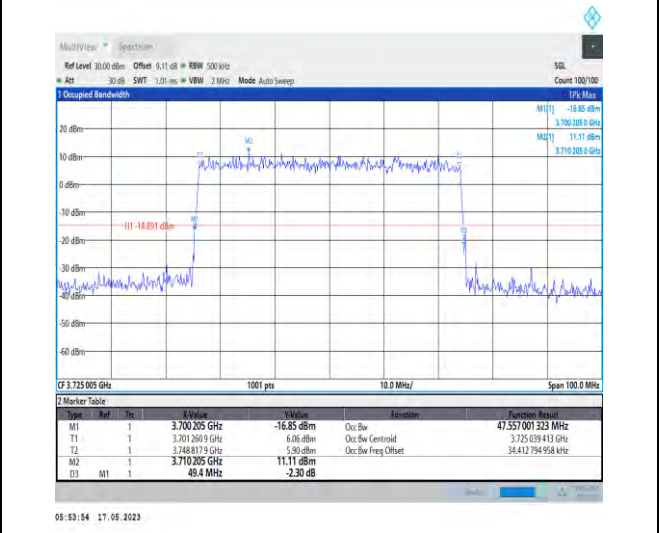
1-N78-3700-3800-PC1-30-50-L-9-CP-256QAM-Outer_Full-133@0-Ant0-47.557-49.400-≤50-PASS
