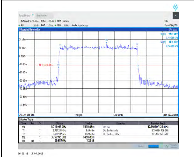
1-N78-3700-3800-PC1-30-60-M-4-DFT-64QAM-Outer_Full-162@0-Ant0-57.691-59.880-≤60-PASS
