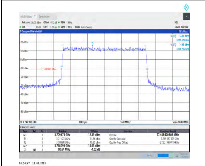
1-N78-3700-3800-PC1-30-80-M-6-CP-QPSK-Outer_Full-217@0-Ant0-77.449-80.640-≤80-PASS
