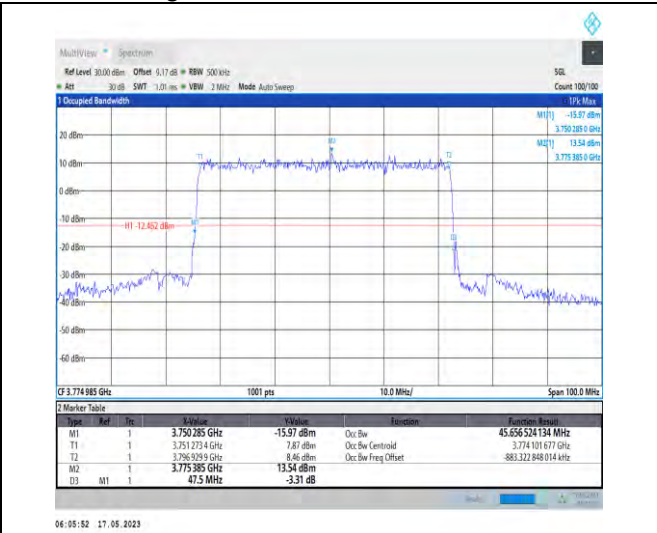
1-N78-3700-3800-PC1-30-50-H-5-DFT-256QAM-Outer_Full-128@0-Ant0-45.657-47.500-≤50-PASS
