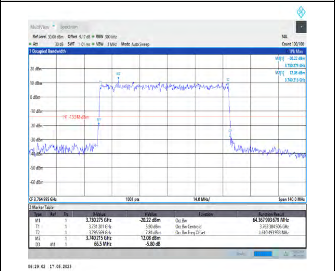
1-N78-3700-3800-PC1-30-70-H-5-DFT-256QAM-Outer_Full-180@0-Ant0-64.368-66.500-≤70-PASS
