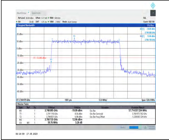
1-N78-3700-3800-PC1-30-60-H-7-CP-16QAM-Outer _Full-162@0-Ant0-57.715-59.760-≤60-PASS
