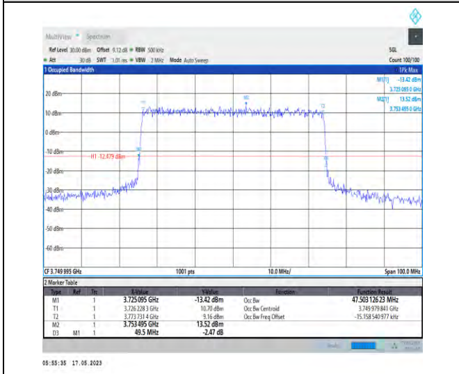
1-N78-3700-3800-PC1-30-50-M-7-CP-16QAM-Outer _Full-133@0-Ant0-47.503-49.500-≤50-PASS
