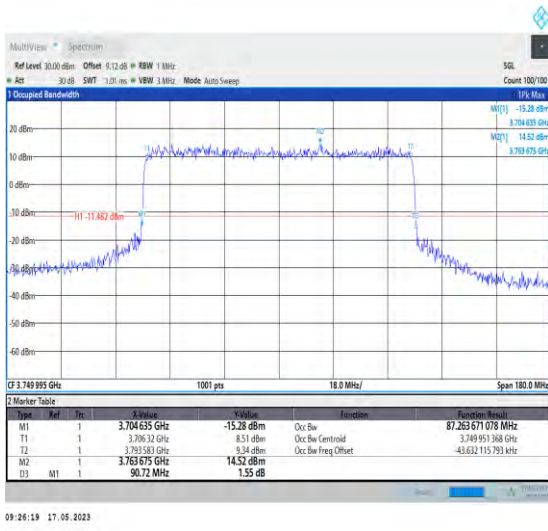
1-N78-3700-3800-PC1-30-90-M-7-CP-16QAM-Outer _Full-245@0-Ant0-87.264-90.720-<90-PASS
