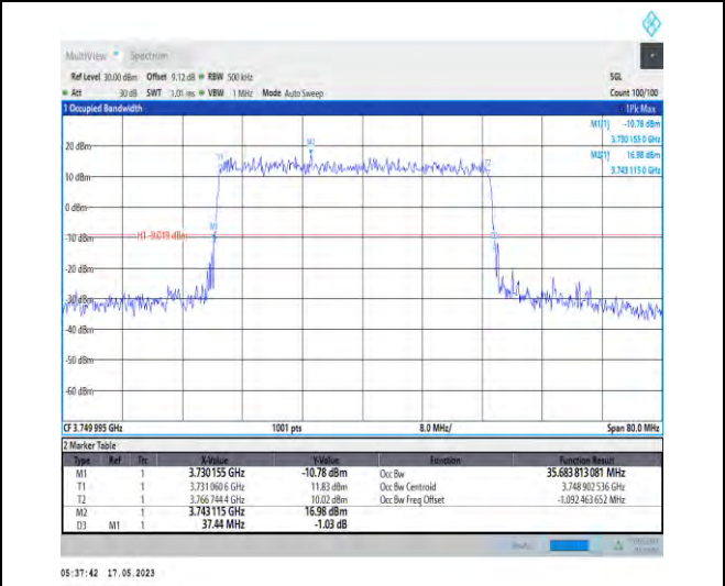
1-N78-3700-3800-PC1-30-40-M-3-DFT-16QAM-Outer_Full-100@0-Ant0-35.684-37.440-≤40-PASS
