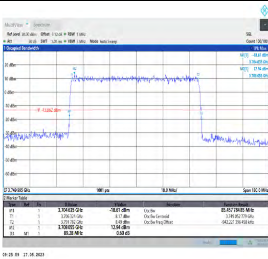
1-N78-3700-3800-PC1-30-90-M-5-DFT-256QAM-Out er_Full-240@0-Ant0-85.458-89.280-<90-PASS
