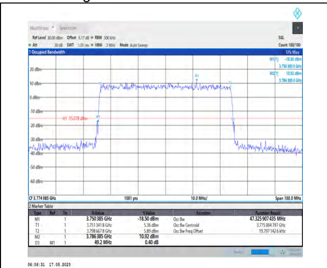
1-N78-3700-3800-PC1-30-50-H-9-CP-256QAM-Outer_Full-133@0-Ant0-47.326-49.200-≤50-PASS
