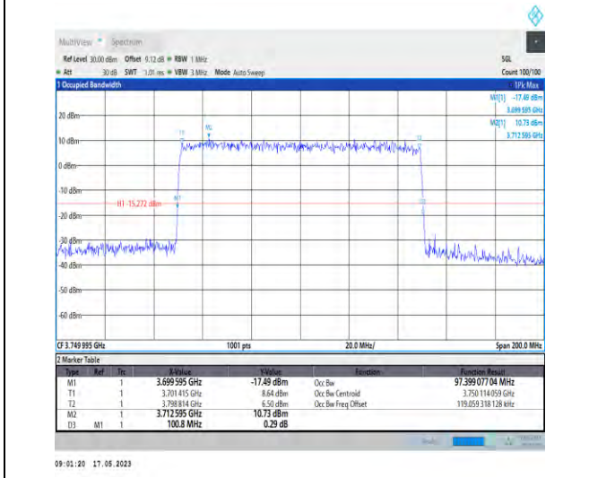
1-N78-3700-3800-PC1-30-100-L-9-CP-256QAM-Outer_Full-273@0-Ant0-97.399-100.800-≤100-PASS
