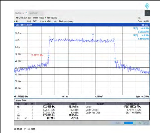
1-N78-3700-3800-PC1-30-50-M-8-CP-64QAM-Outer _Full-133@0-Ant0-47.398-49.200-≤50-PASS
