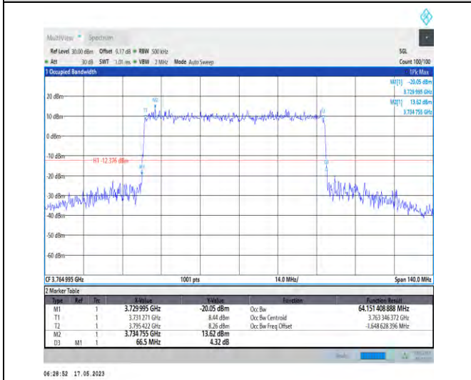
1-N78-3700-3800-PC1-30-70-H-4-DFT-64QAM-Outer_Full-180@0-Ant0-64.151-66.500-≤70-PASS
