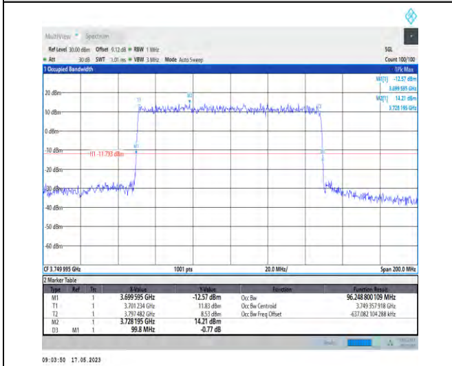
1-N78-3700-3800-PC1-30-100-M-4-DFT-64QAM-Out_Full-270@0-Ant0-96.249-99.800-≤100-PASS
