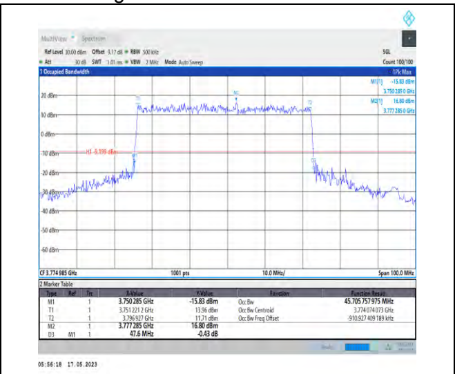
1-N78-3700-3800-PC1-30-50-H-1-DFT-QPSK-Outer_Full-128@0-Ant0-45.706-47.600-≤50-PASS
