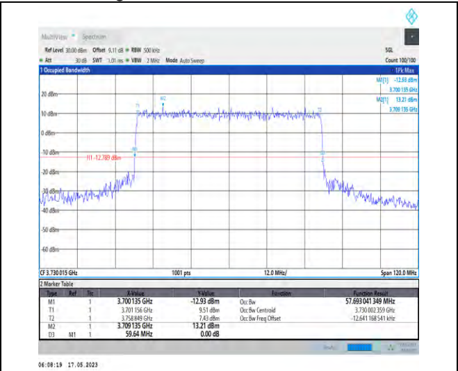
1-N78-3700-3800-PC1-30-60-L-8-CP-64QAM-Outer _Full-162@0-Ant0-57.693-59.640-≤60-PASS
