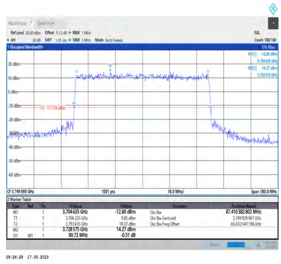
1-N78-3700-3800-PC1-30-90-M-8-CP-64QAM-Outer _Full-245@0-Ant0-87.41-90.720-<90-PASS
