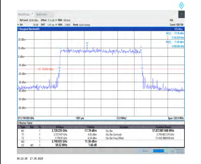
1-N78-3700-3800-PC1-30-60-M-9-CP-256QAM-Outer_Full-162@0-Ant0-57.873-59.520-≤60-PASS
