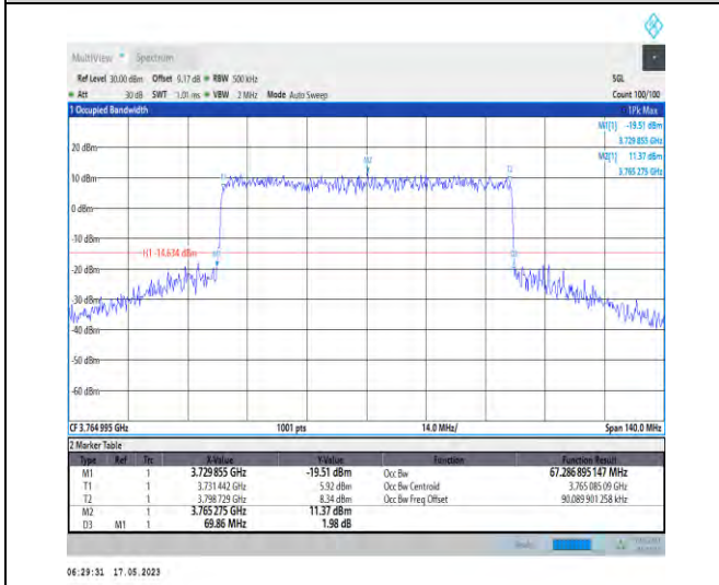
1-N78-3700-3800-PC1-30-70-H-8-CP-64QAM-Outer_Full-189@0-Ant0-67.287-69.860-≤70-PASS
