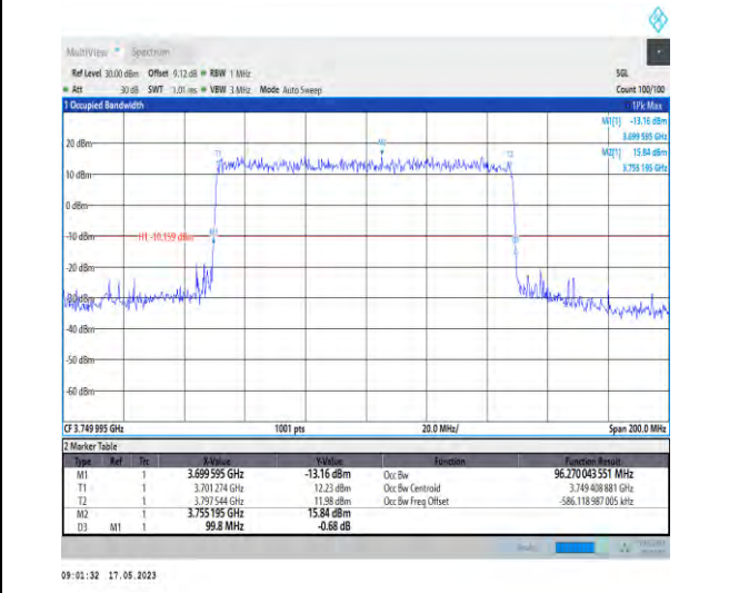
1-N78-3700-3800-PC1-30-100-M-1-DFT-QPSK-Outer_Full-270@0-Ant0-96.27-99.800-≤100-PASS
