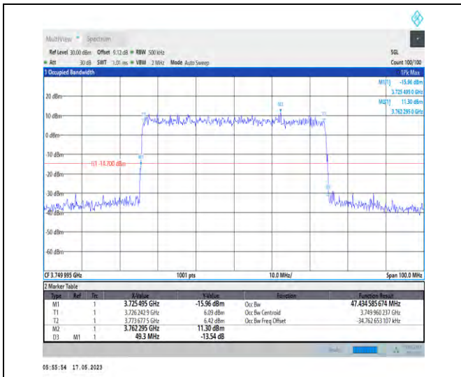
1-N78-3700-3800-PC1-30-50-M-9-CP-256QAM-Outer_Full-133@0-Ant0-47.435-49.300-≤50-PASS
