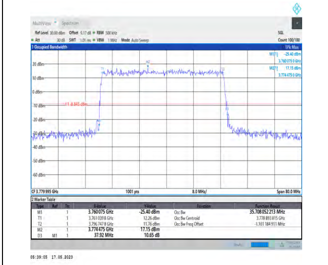
1-N78-3700-3800-PC1-30-40-H-1-DFT-QPSK-Outer_Full-100@0-Ant0-35.708-37.920-≤40-PASS
