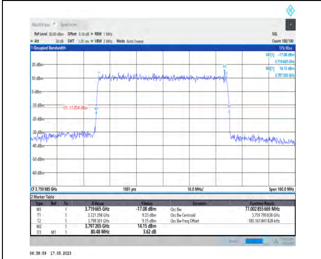
1-N78-3700-3800-PC1-30-80-H-5-DFT-256QAM-Outer_Full-216@0-Ant0-77.003-80.480-≤80-PASS
