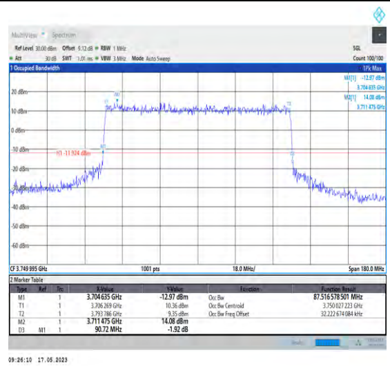
1-N78-3700-3800-PC1-30-90-M-6-CP-QPSK-Outer_ Full-245@0-Ant0-87.517-90.720-<90-PASS
