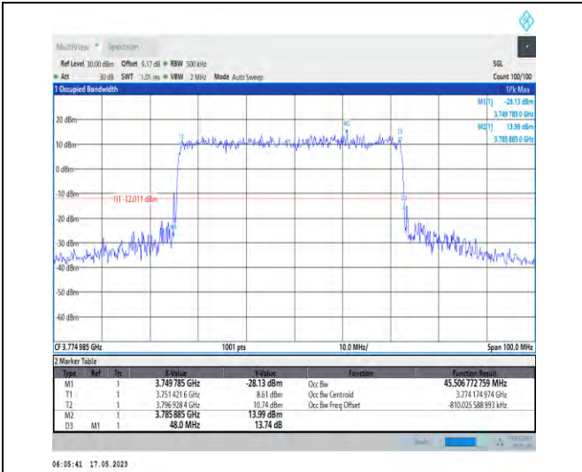
1-N78-3700-3800-PC1-30-50-H-4-DFT-64QAM-Outer_Full-128@0-Ant0-45.507-48.000-≤50-PASS
