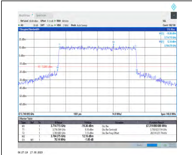
1-N78-3700-3800-PC1-30-70-M-7-CP-16QAM-Outer _Full-189@0-Ant0-67.32-70.140-≤70-PASS
