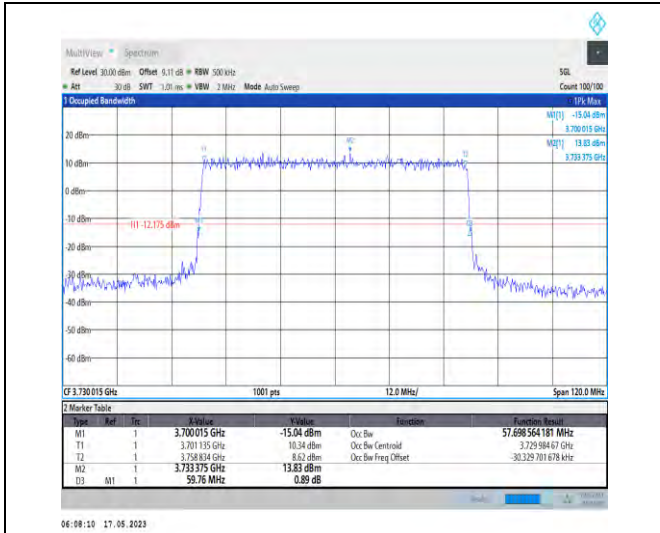
1-N78-3700-3800-PC1-30-60-L-7-CP-16QAM-Outer _Full-162@0-Ant0-57.699-59.760-≤60-PASS
