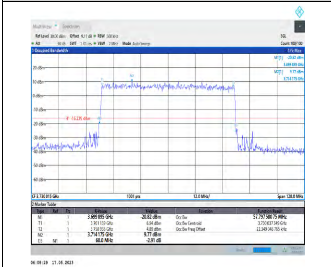
1-N78-3700-3800-PC1-30-60-L-9-CP-256QAM-Outer _Full-162@0-Ant0-57.798-60.000-≤60-PASS
