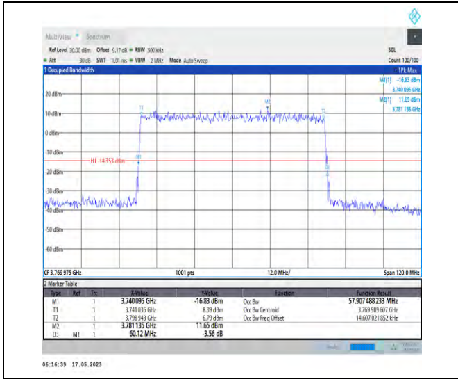
1-N78-3700-3800-PC1-30-60-H-5-DFT-256QAM-Out er_Full-162@0-Ant0-57.907-60.120-≤60-PASS
