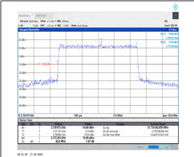
1-N78-3700-3800-PC1-30-60-H-1-DFT-QPSK-Outer_Full-162@0-Ant0-57.734-60.000-≤60-PASS
