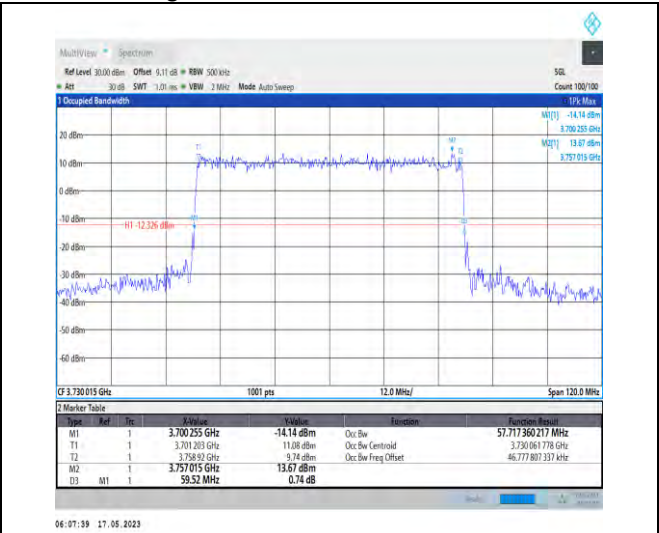
1-N78-3700-3800-PC1-30-60-L-4-DFT-64QAM-Outer_Full-162@0-Ant0-57.717-59.520-≤60-PASS
