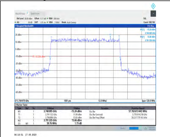
1-N78-3700-3800-PC1-30-60-H-2-DFT-PI2BPSK-Outer_Full-162@0-Ant0-57.764-59.760-≤60-PASS
