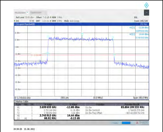
1-N78-3700-3800--30-90-L-1-DFT-QPSK-Outer_Full- 240@0-Ant0-85.804-88.920-≤90-PASS
