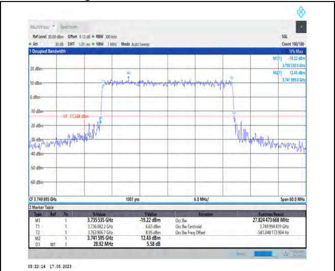
1-N78-3700-3800-PC1-30-30-M-8-CP-64QAM-Outer _Full-78@0-Ant0-27.824-28.920-≤30-PASS
