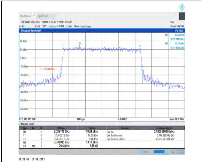
1-N78-3700-3800-PC1-30-30-M-7-CP-16QAM-Outer _Full-78@0-Ant0-27.806-29.400-≤30-PASS
