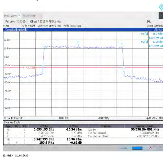
1-N78-3700-3800--30-100-L-4-DFT-64QAM-Outer_F ull-270@0-Ant0-96.331-100.600-≤100-PASS
