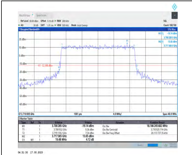
1-N78-3700-3800-PC1-30-20-L-7-CP-16QAM-Outer _Full-51@0-Ant0-18.186-19.480-≤20-PASS
