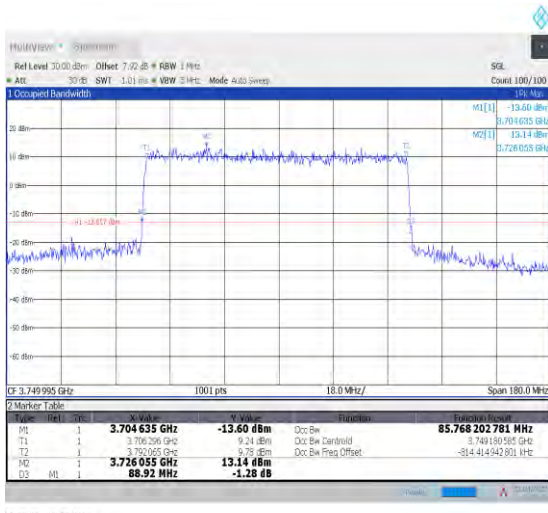
1-N78-3700-3800--30-90-M-3-DFT-16QAM-Outer_Full ull-240@0-Ant0-85.768-88.920-≤90-PASS
