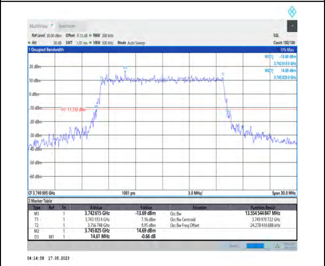
1-N78-3700-3800-PC1-30-15-M-8-CP-64QAM-Outer _Full-38@0-Ant0-13.555-14.610-≤15-PASS
