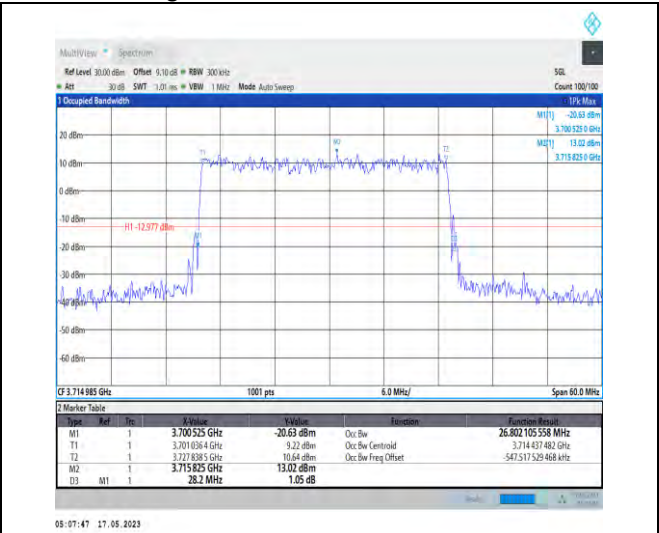
1-N78-3700-3800-PC1-30-30-L-5-DFT-256QAM-Outer_Full-75@0-Ant0-26.802-28.200-≤30-PASS
