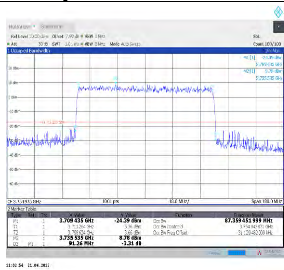
1-N78-3700-3800--30-90-H-9-CP-256QAM-Outer_Full -245@0-Ant0-87.359-91.260-≤90-PASS
