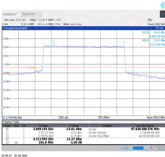
1-N78-3700-3800--30-100-H-7-CP-16QAM-Outer_Full-273@0-Ant0-97.637-101.600-<=100-PASS
