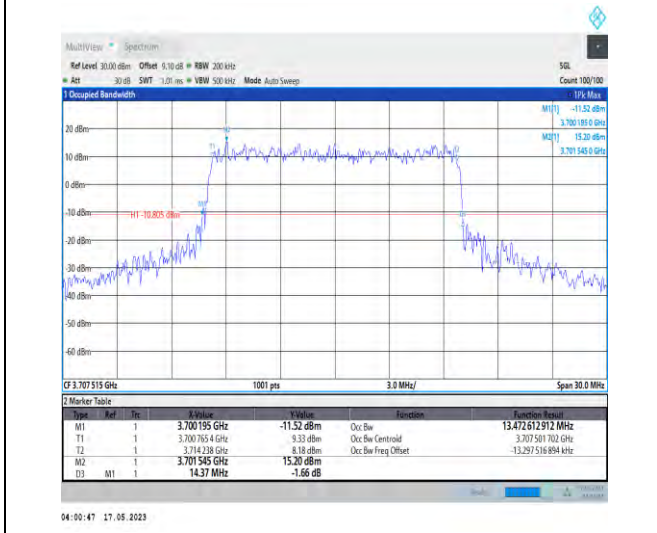
1-N78-3700-3800-PC1-30-15-L-8-CP-64QAM-Outer_Full-38@0-Ant0-13.473-14.370-≤15-PASS
