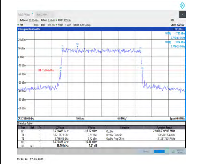
1-N78-3700-3800-PC1-30-30-H-9-CP-256QAM-Outer_Full-78@0-Ant0-27.828-29.160-≤30-PASS
