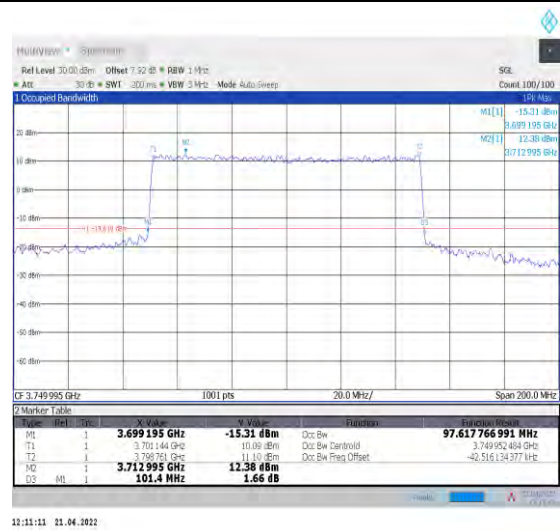
1-N78-3700-3800--30-100-M-7-CP-16QAM-Outer_Full-273@0-Ant0-97.618-101.400-≤100-PASS
