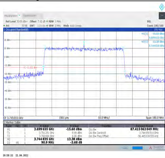
1-N78-3700-3800--30-90-L-7-CP-16QAM-Outer_Full -245@0-Ant0-87.415-90.900-<=90-PASS
