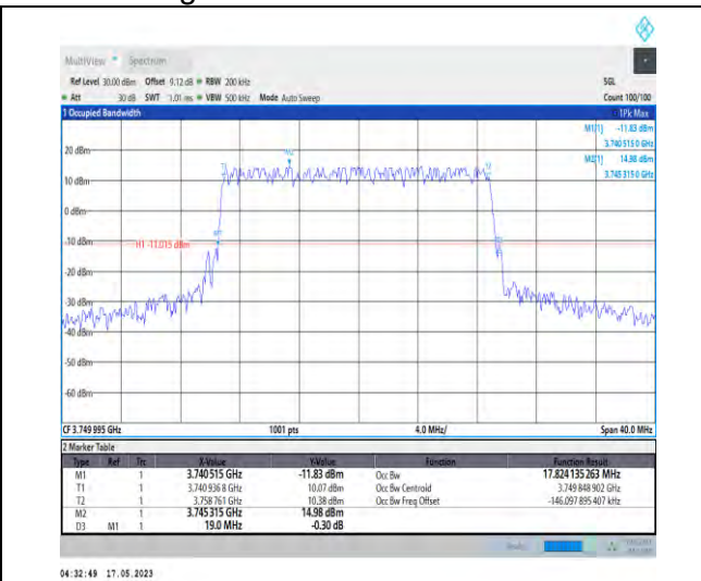
1-N78-3700-3800-PC1-30-20-M-3-DFT-16QAM-Outer_Full-50@0-Ant0-17.824-19.000-≤20-PASS
