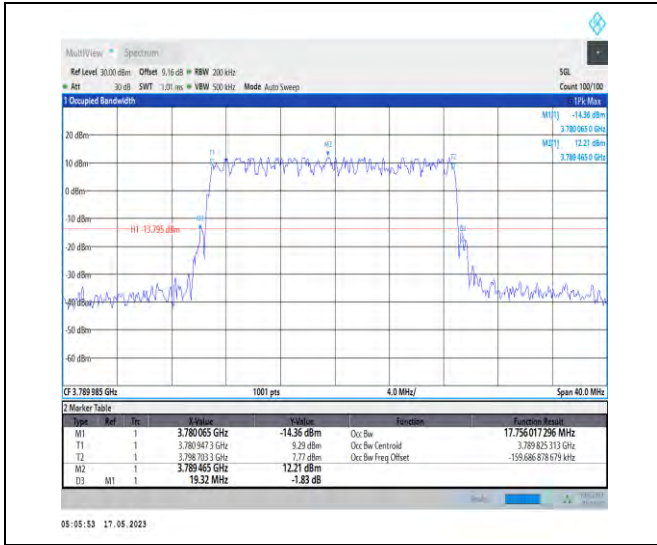
1-N78-3700-3800-PC1-30-20-H-5-DFT-256QAM-Out er_Full-50@0-Ant0-17.756-19.320-≤20-PASS
