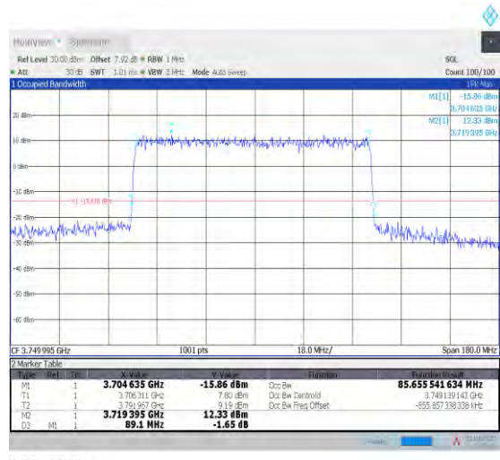
1-N78-3700-3800--30-90-M-4-DFT-64QAM-Outer_Full ull-240@0-Ant0-85.656-89.100-≤90-PASS
