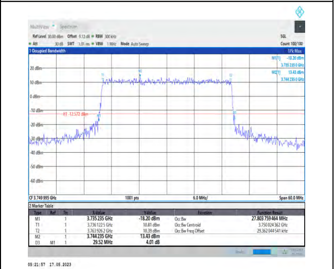
1-N78-3700-3800-PC1-30-30-M-6-CP-QPSK-Outer_Full-78@0-Ant0-27.804-29.520-≤30-PASS
