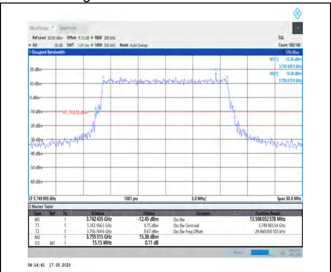
1-N78-3700-3800-PC1-30-15-M-6-CP-QPSK-Outer Full-38@0-Ant0-13.598-15.150-≤15-PASS
