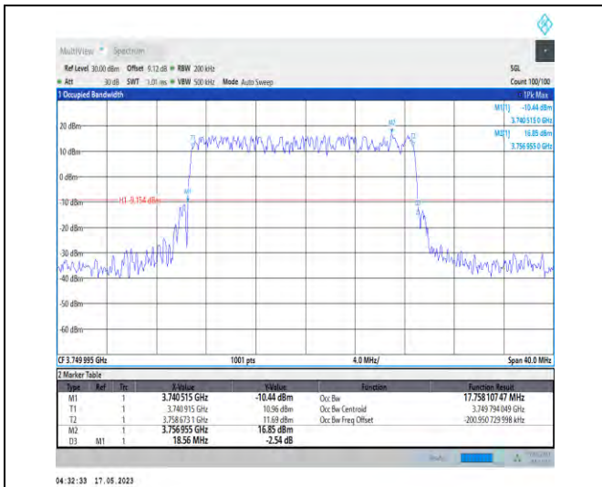
1-N78-3700-3800-PC1-30-20-M-2-DFT-PI2BPSK-Outer_Full-50@0-Ant0-17.758-18.560-≤20-PASS
