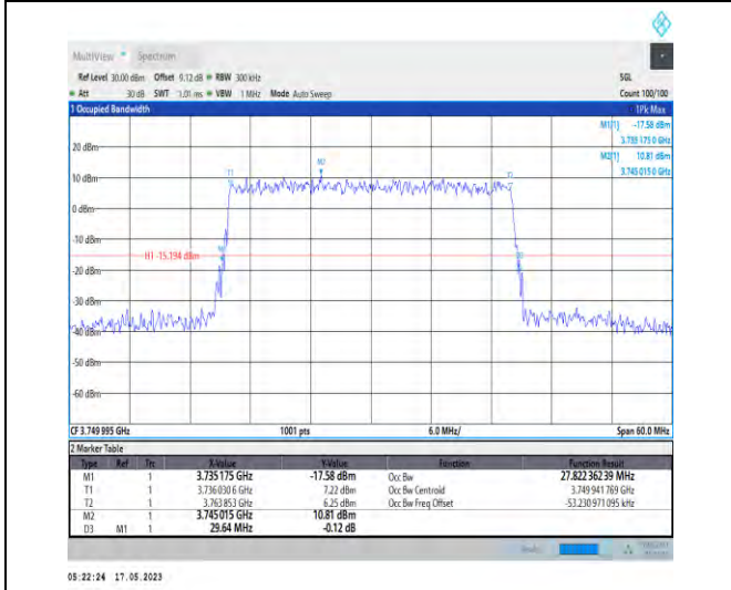
1-N78-3700-3800-PC1-30-30-M-9-CP-256QAM-Outer _Full-78@0-Ant0-27.822-29.640-≤30-PASS
