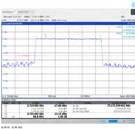
1-N78-3700-3800--30-80-H-5-DFT-256QAM-Outer_Full-216@0-Ant0-77.172-80.800-≤80-PASS
