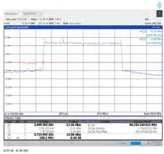
1-N78-3700-3800--30-100-M-1-DFT-QPSK-Outer_F ull-270@0-Ant0-96.354-100.200-≤100-PASS
