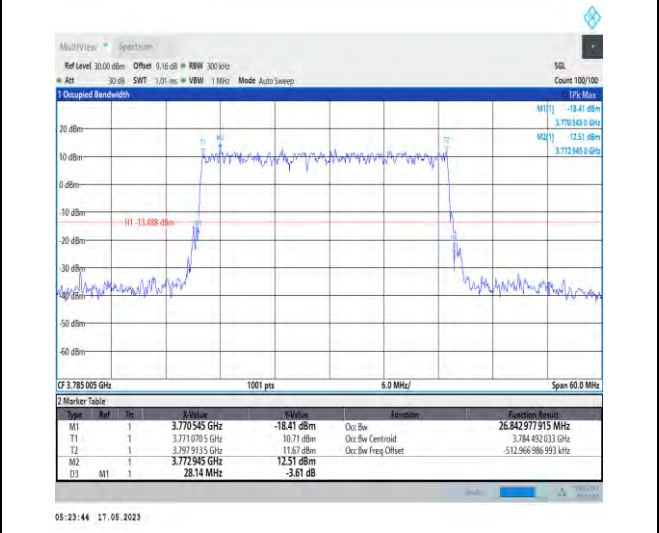
1-N78-3700-3800-PC1-30-30-H-5-DFT-256QAM-Outer_Full-75@0-Ant0-26.843-28.140-≤30-PASS
