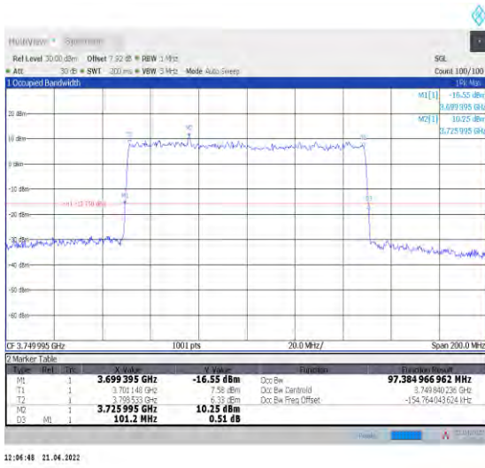
1-N78-3700-3800--30-100-L-9-CP-256QAM-Outer_F ull-273@0-Ant0-97.385-101.200-≤100-PASS
