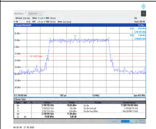
1-N78-3700-3800-PC1-30-20-M-5-DFT-256QAM-Outer_Full-50@0-Ant0-17.81-19.080-≤20-PASS
