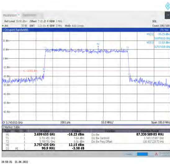
1-N78-3700-3800--30-90-L-8-CP-64QAM-Outer_Full -245@0-Ant0-87.331-90.900-<=90-PASS
