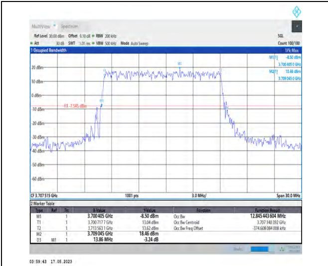
1-N78-3700-3800-PC1-30-15-L-2-DFT-PI2BPSK-Out er_Full-36@0-Ant0-12.845-13.860-≤15-PASS
