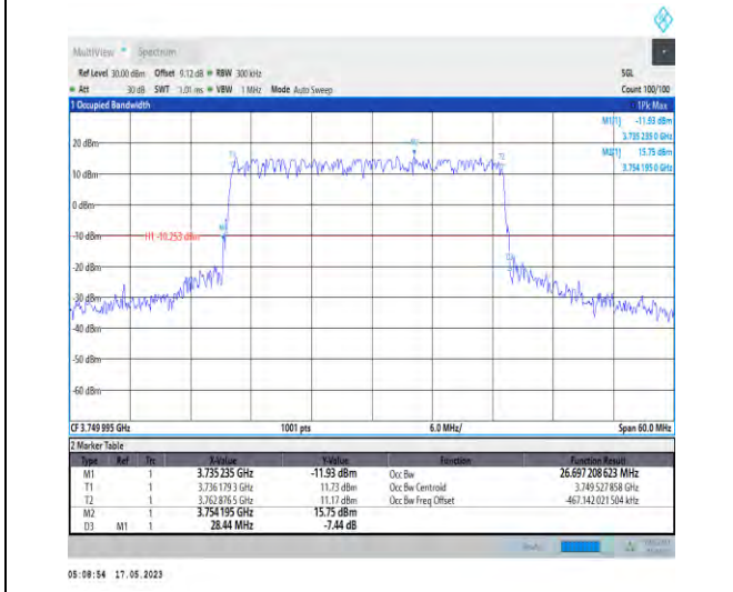
1-N78-3700-3800-PC1-30-30-M-1-DFT-QPSK-Outer_Full-75@0-Ant0-26.697-28.440-≤30-PASS
