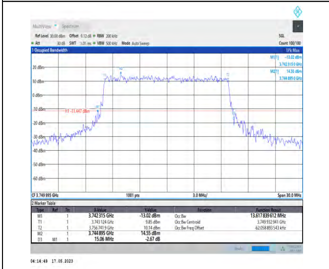
1-N78-3700-3800-PC1-30-15-M-7-CP-16QAM-Outer _Full-38@0-Ant0-13.618-15.060-≤15-PASS
