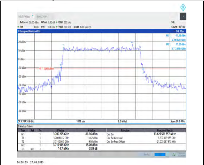
1-N78-3700-3800-PC1-30-15-L-7-CP-16QAM-Outer_Full-38@0-Ant0-13.626-14.700-≤15-PASS
