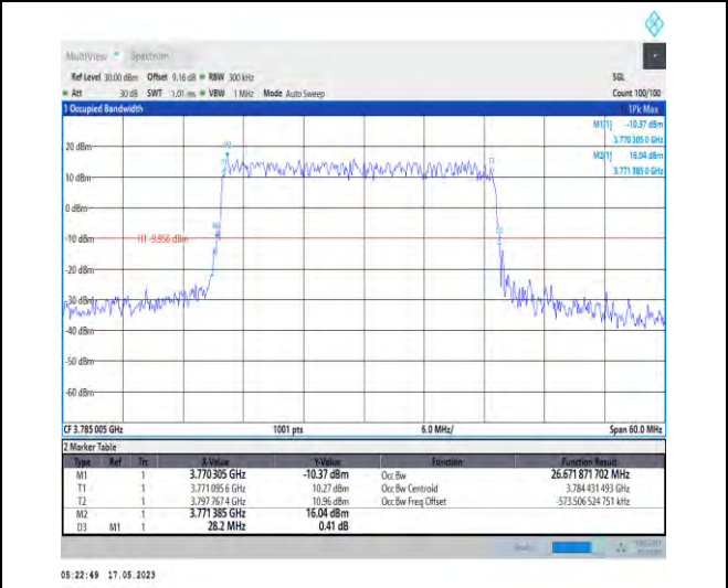
1-N78-3700-3800-PC1-30-30-H-1-DFT-QPSK-Outer _Full-75@0-Ant0-26.672-28.200-≤30-PASS
