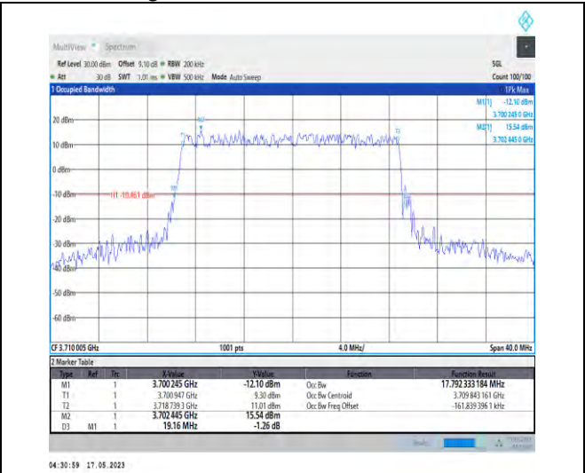
1-N78-3700-3800-PC1-30-20-L-4-DFT-64QAM-Outer_Full-50@0-Ant0-17.792-19.160-≤20-PASS
