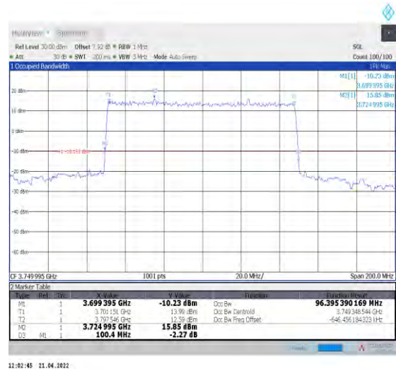
1-N78-3700-3800--30-100-L-2-DFT-PI2BPSK-Outer_Full Full-270@0-Ant0-96.395-100.400-≤100-PASS
