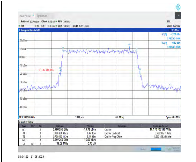
1-N78-3700-3800-PC1-30-20-H-9-CP-256QAM-Outer_Full-51@0-Ant0-18.171-19.520-≤20-PASS
