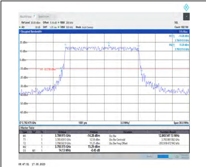
1-N78-3700-3800-PC1-30-15-H-4-DFT-64QAM-Outer_Full-36@0-Ant0-12.844-14.130-≤15-PASS
