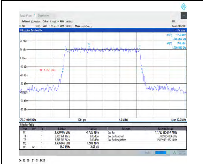
1-N78-3700-3800-PC1-30-20-L-5-DFT-256QAM-Outer_Full-50@0-Ant0-17.785-19.000-≤20-PASS
