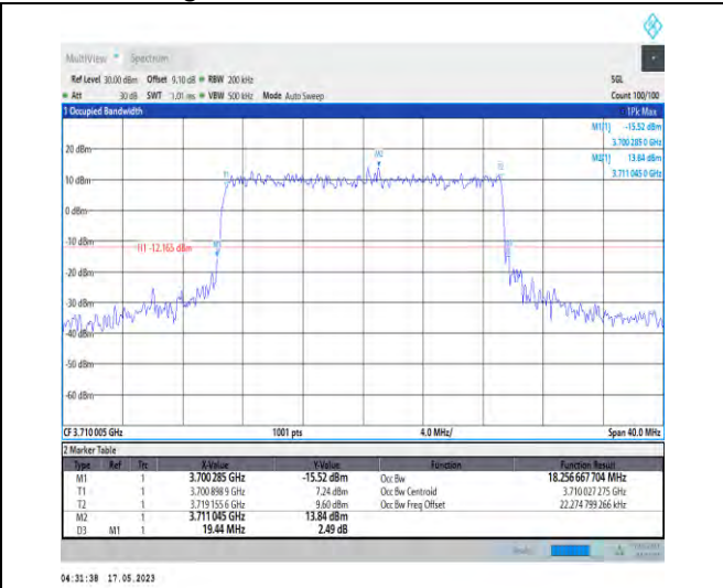
1-N78-3700-3800-PC1-30-20-L-8-CP-64QAM-Outer _Full-51@0-Ant0-18.257-19.440-≤20-PASS
