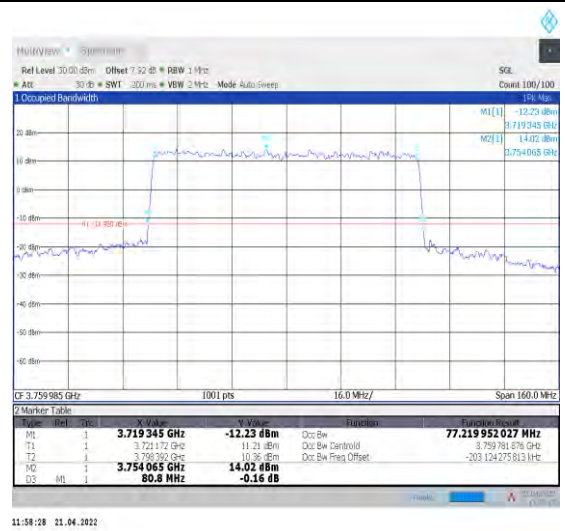
1-N78-3700-3800--30-80-H-4-DFT-64QAM-Outer_Fu II-216@0-Ant0-77.22-80.800-≤80-PASS
