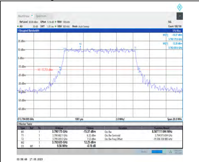
1-N78-3700-3800-PC1-30-10-H-8-CP-64QAM-Outer_Full-24@0-Ant0-8.587-9.560-≤10-PASS
