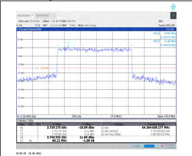
1-N78-3700-3800--30-70-H-3-DFT-16QAM-Outer_Fu II-180@0-Ant0-64.365-66.220-≤70-PASS
