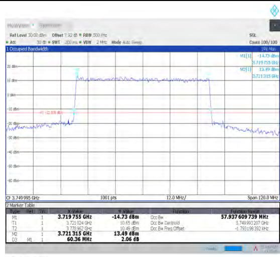
1-N78-3700-3800--30-60-M-3-DFT-16QAM-Outer_Full-162@0-Ant0-57.938-60.360-≤60-PASS
