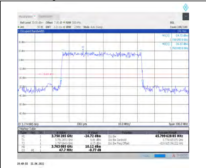
1-N78-3700-3800--30-50-H-5-DFT-256QAM-Outer_F ull-128@0-Ant0-45.8-47.700-≤50-PASS
