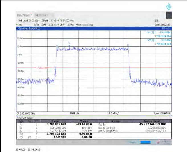
1-N78-3700-3800--30-50-L-5-DFT-256QAM-Outer_F ull-128@0-Ant0-45.758-47.900-<math>\leq 50</math>-PASS
