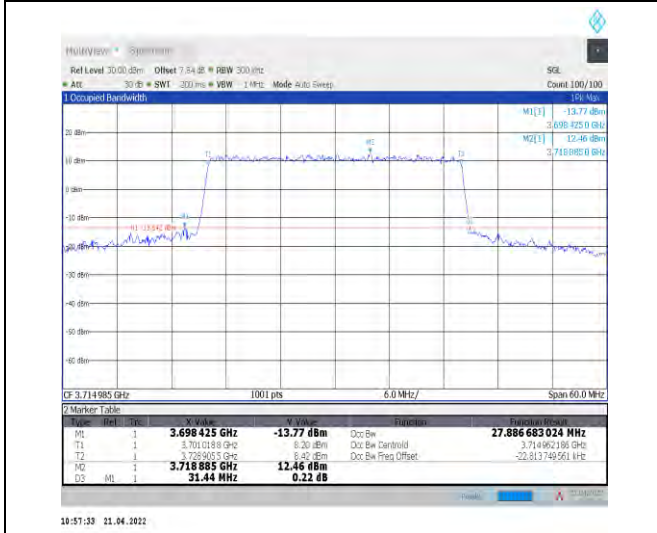
1-N78-3700-3800--30-30-L-6-CP-QPSK-Outer_Full-78@0-Ant0-27.887-31.440-<math>\leq</math>30-PASS
