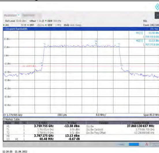
1-N78-3700-3800--30-40-H-8-CP-64QAM-Outer_Full -106@0-Ant0-37.86-40.480-≤40-PASS
