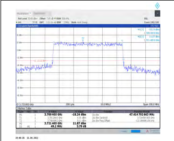
1-N78-3700-3800--30-50-L-8-CP-64QAM-Outer_Full -133@0-Ant0-47.415-49.200-≤50-PASS
