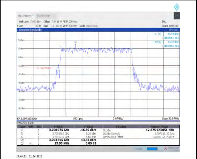
1-N78-3700-3800--30-15-L-5-DFT-256QAM-Outer_Full-36@0-Ant0-12.875-13.950-≤15-PASS
