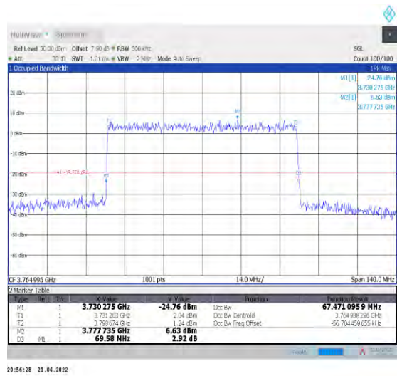
1-N78-3700-3800--30-70-H-9-CP-256QAM-Outer_Full -189@0-Ant0-67.471-69.580-≤70-PASS
