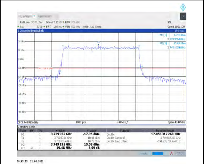
1-N78-3700-3800--30-20-M-1-DFT-QPSK-Outer_Full -50@0-Ant0-17.856-19.480-<=20-PASS
