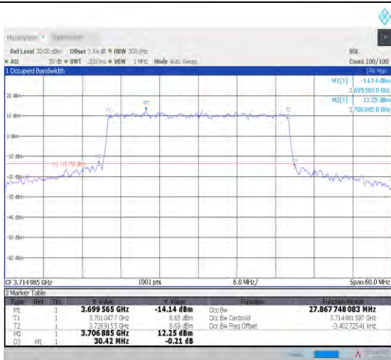
1-N78-3700-3800--30-30-L-8-CP-64QAM-Outer_Full -78@0-Ant0-27.868-30.420-<30-PASS
