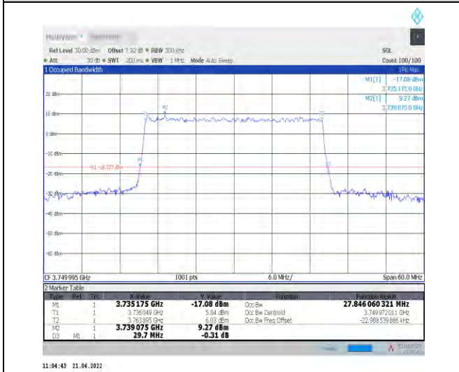
1-N78-3700-3800--30-30-M-9-CP-256QAM-Outer_F ull-78@0-Ant0-27.846-29.700-<30-PASS
