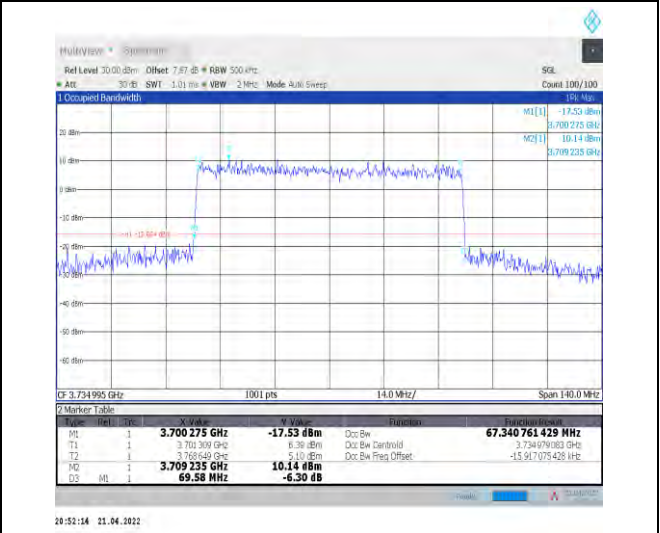
1-N78-3700-3800--30-70-L-7-CP-16QAM-Outer_Full -189@0-Ant0-67.341-69.580-≤70-PASS
