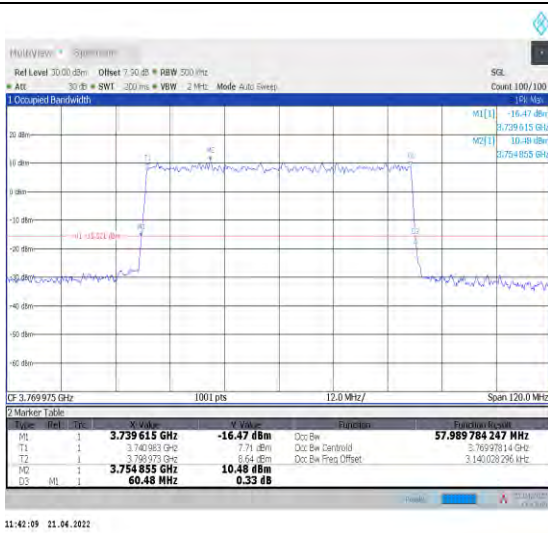
1-N78-3700-3800--30-60-H-5-DFT-256QAM-Outer_Full-162@0-Ant0-57.99-60.480-≤60-PASS
