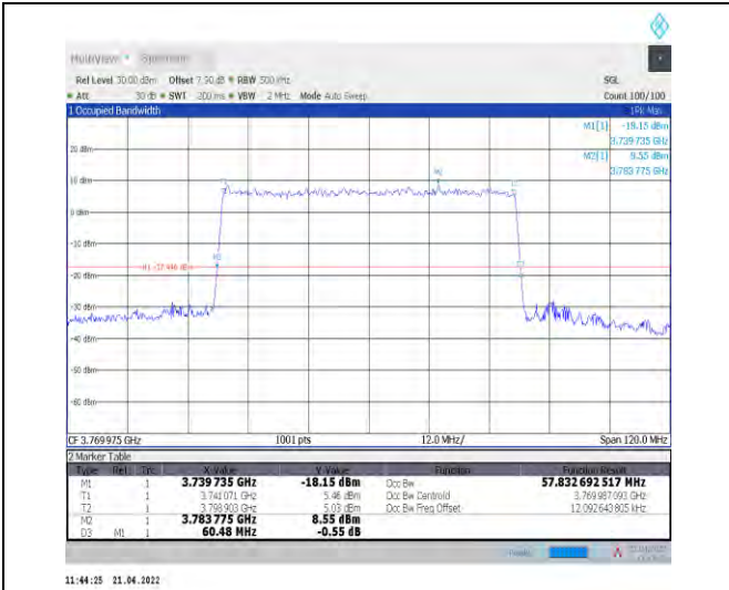
1-N78-3700-3800--30-60-H-9-CP-256QAM-Outer_Fu II-162@0-Ant0-57.833-60.480-≤60-PASS
