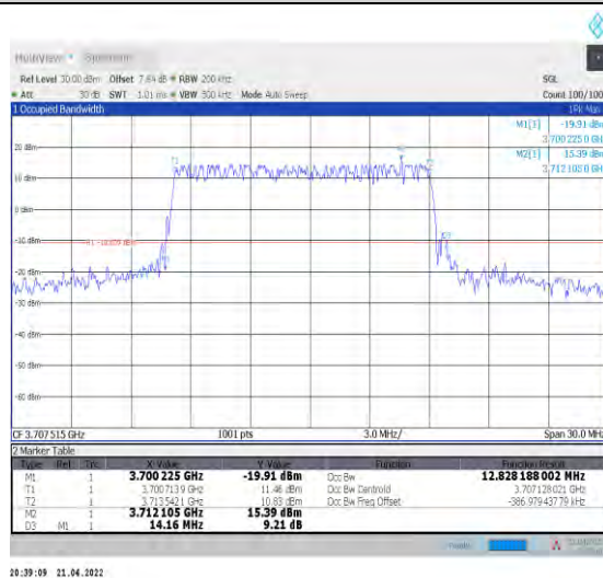
1-N78-3700-3800--30-15-L-1-DFT-QPSK-Outer_Full- 36@0-Ant0-12.828-14.160-≤15-PASS
