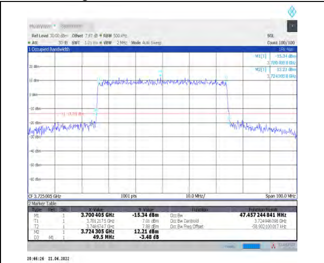
1-N78-3700-3800--30-50-L-7-CP-16QAM-Outer_Full -133@0-Ant0-47.457-49.500-≤50-PASS
