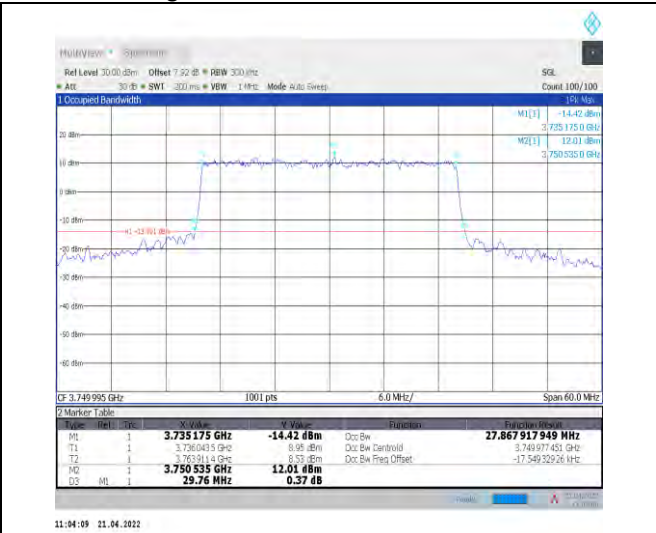
1-N78-3700-3800--30-30-M-8-CP-64QAM-Outer_Ful I-78@0-Ant0-27.868-29.760-<30-PASS
