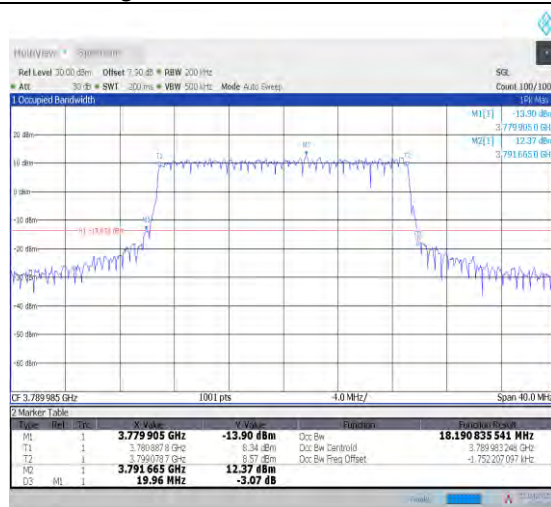
1-N78-3700-3800--30-20-H-6-CP-QPSK-Outer_Full-51@0-Ant0-18.191-19.960-<=20-PASS
