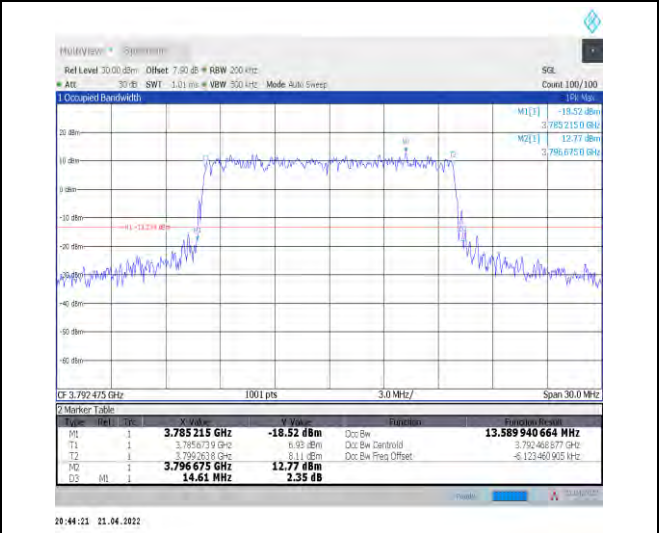
1-N78-3700-3800--30-15-H-7-CP-16QAM-Outer_Full-38@0-Ant0-13.59-14.610-≤15-PASS
