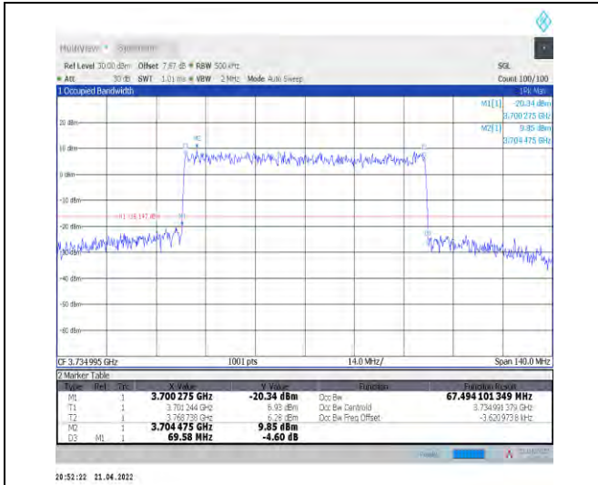
1-N78-3700-3800--30-70-L-8-CP-64QAM-Outer_Full -189@0-Ant0-67.494-69.580-≤70-PASS
