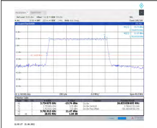
1-N78-3700-3800--30-30-M-5-DFT-256QAM-Outer_Full-75@0-Ant0-26.834-28.920-<=30-PASS
