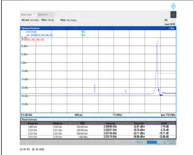
1-N78-3450-3550-PC1-30-70-H-5-CP-QPSK-Edge_1RB_Right-1@188-Ant0-1--PASS-see graph
