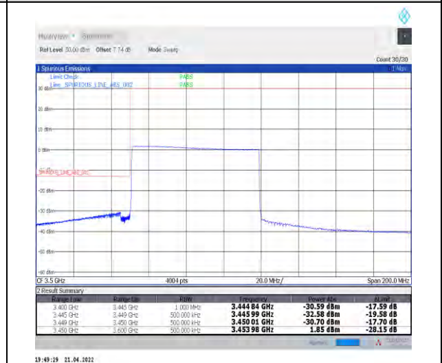
1-N78-3450-3550--30-70-L-6-CP-QPSK-Outer_Ful l-189@0-Ant0-PASS-see graph
