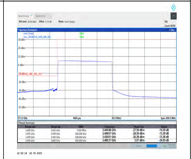
1-N78-3450-3550-PC1-30-70-L-6-CP-QPSK-Outer_Full-189@0-Ant0-1--PASS-see graph
