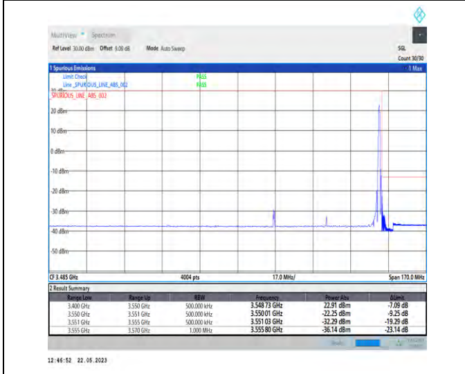
1-N78-3450-3550-PC1-30-50-H-5-CP-QPSK-Edge_1RB_Right-1@132-Ant0-1--PASS-see graph
