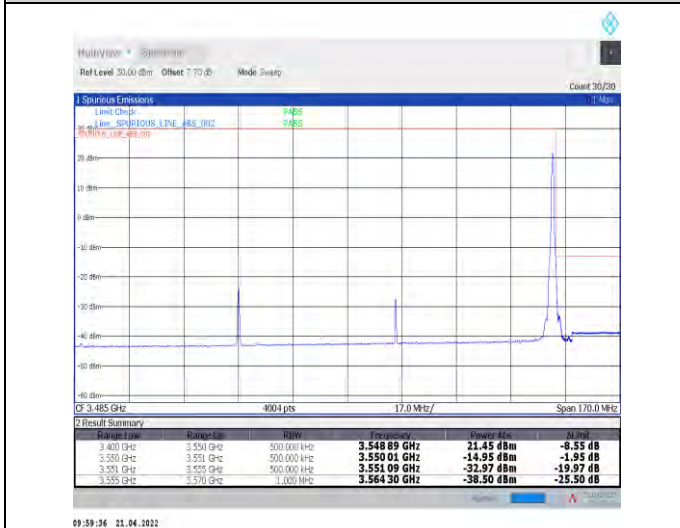
1-N78-3450-3550--30-100-H-5-CP-QPSK-Edge_1RB_Right-1@272-Ant0-PASS-see graph
