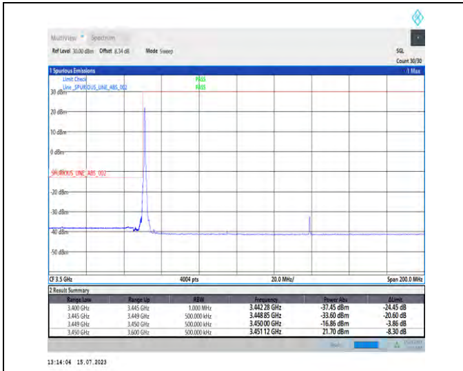
1-N78-3450-3550-PC1-30-90-L-1-DFT-PI2BPSK-Edge_1RB_Left-1@0-Ant0-1--PASS-see graph
