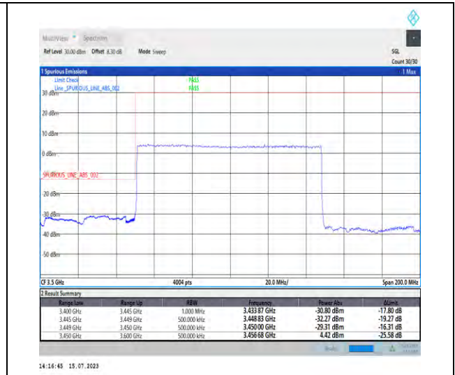
1-N78-3450-3550-PC1-30-100-L-3-DFT-PI2BPSK-Outer_Full-270@0-Ant0-1--PASS-see graph
