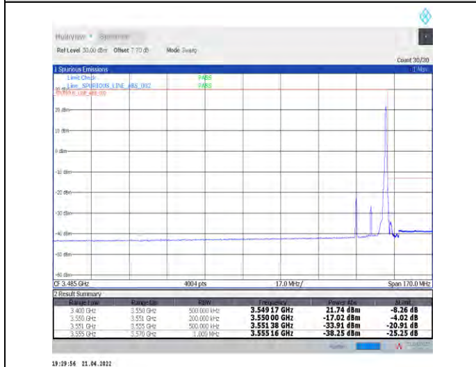
1-N78-3450-3550--30-15-H-5-CP-QPSK-Edge_1RB_R ight-1@37-Ant0-PASS-see graph
