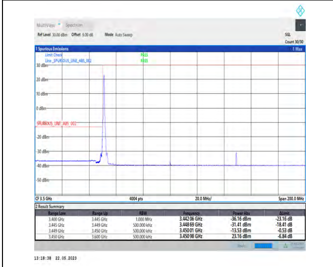
1-N78-3450-3550-PC1-30-100-L-4-CP-QPSK-Edge_1RB_Left-1@0-Ant0-1--PASS-see graph
