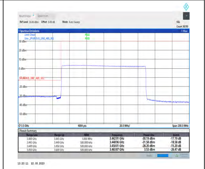
1-N78-3450-3550-PC1-30-100-L-6-CP-QPSK-Outer_Full-273@0-Ant0-1--PASS-see graph
