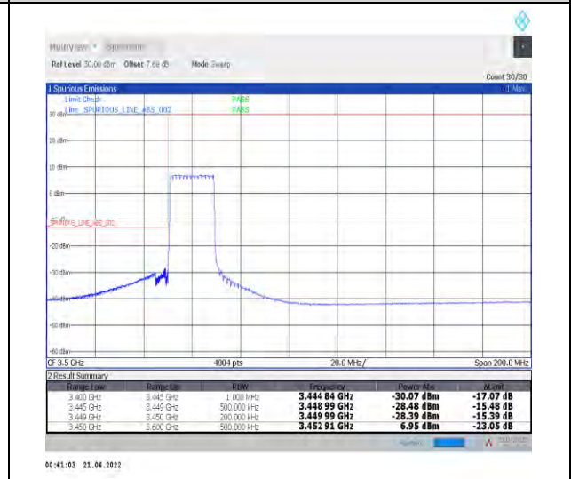
1-N78-3450-3550--30-20-L-6-CP-QPSK-Outer_Ful l-51@0-Ant0-PASS-see graph
