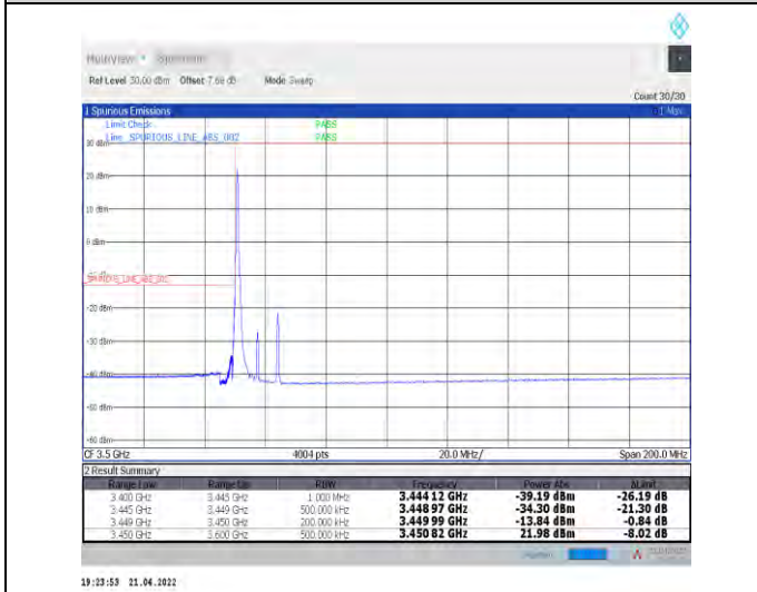
1-N78-3450-3550--30-15-L-4-CP-QPSK-Edge_1RB_L_eft-1@0-Ant0-PASS-see graph
