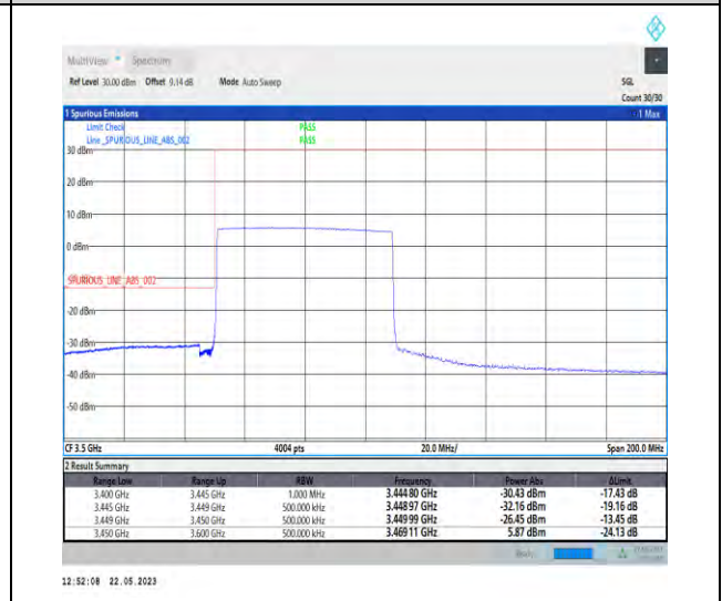
1-N78-3450-3550-PC1-30-60-L-6-CP-QPSK-Outer_Full-162@0-Ant0-1--PASS-see graph
