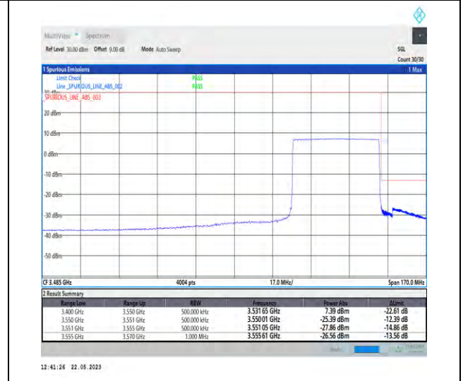
1-N78-3450-3550-PC1-30-40-H-6-CP-QPSK-Outer_Full-106@0-Ant0-1--PASS-see graph
