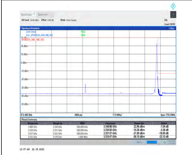
1-N78-3450-3550-PC1-30-80-H-5-CP-QPSK-Edge_1RB_Right-1@216-Ant0-1--PASS-see graph
