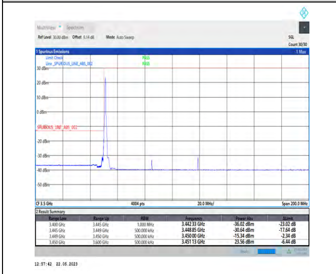
1-N78-3450-3550-PC1-30-70-L-4-CP-QPSK-Edge_1RB_Left-1@0-Ant0-1--PASS-see graph
