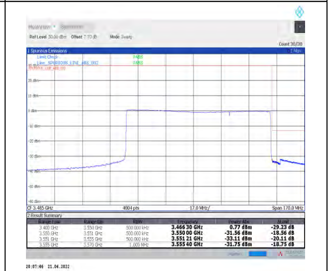
1-N78-3450-3550--30-90-H-6-CP-QPSK-Outer_Fu ll-245@0-Ant0-PASS-see graph
