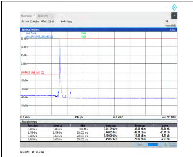
1-N78-3450-3550-PC1-30-15-L-1-DFT-PI2BPSK-Edge_1_RB_Left-1@0-Ant0-1--PASS-see graph
