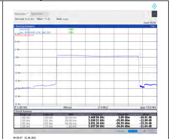
1-N78-3450-3550--30-100-H-3-DFT-PI2BPSK-Out er_Full-270@0-Ant0-PASS-see graph
