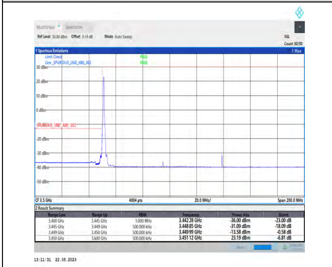
1-N78-3450-3550-PC1-30-90-L-4-CP-QPSK-Edge_1RB_Left-1@0-Ant0-1--PASS-see graph
