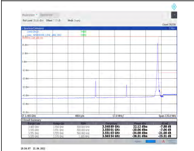
1-N78-3450-3550--30-70-H-5-CP-QPSK-Edge_1RB_R ight-1@188-Ant0-PASS-see graph
