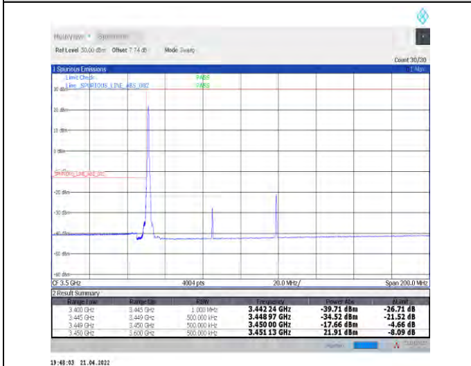
1-N78-3450-3550--30-70-L-4-CP-QPSK-Edge_1RB_L eft-1@0-Ant0-PASS-see graph
