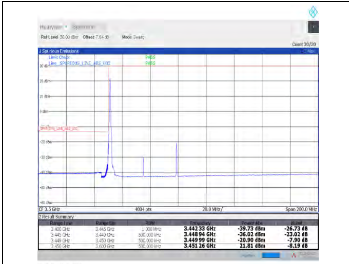
1-N78-3450-3550--30-50-L-1-DFT-PI2BPSK-Edge_1R_B_Left-1@0-Ant0-PASS-see graph
