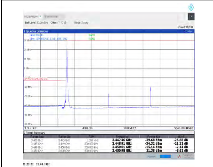
1-N78-3450-3550--30-100-L-4-CP-QPSK-Edge_1RB_Left-1@0-Ant0-PASS-see graph
