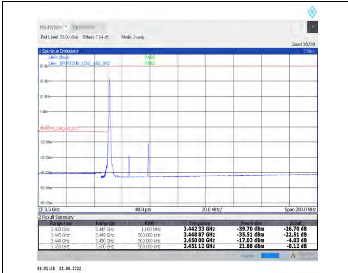
1-N78-3450-3550--30-30-L-1-DFT-PI2BPSK-Edge_1R_B_Left-1@0-Ant0-PASS-see graph
