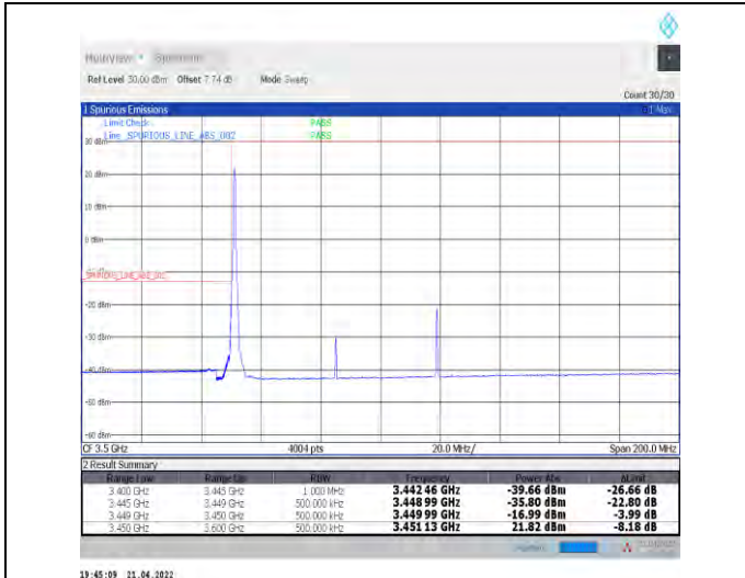
1-N78-3450-3550--30-70-L-1-DFT-PI2BPSK-Edge_1R_B_Left-1@0-Ant0-PASS-see graph
