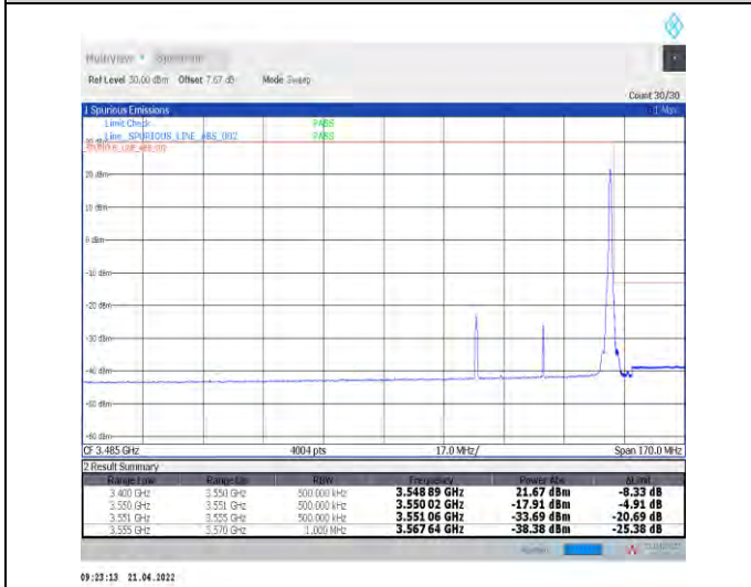
1-N78-3450-3550--30-40-H-5-CP-QPSK-Edge_1RB_R ight-1@105-Ant0-PASS-see graph
