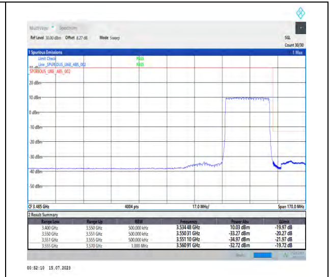
1-N78-3450-3550-PC1-30-30-H-3-DFT-PI2BPSK-Outer_Full-75@0-Ant0-1--PASS-see graph
