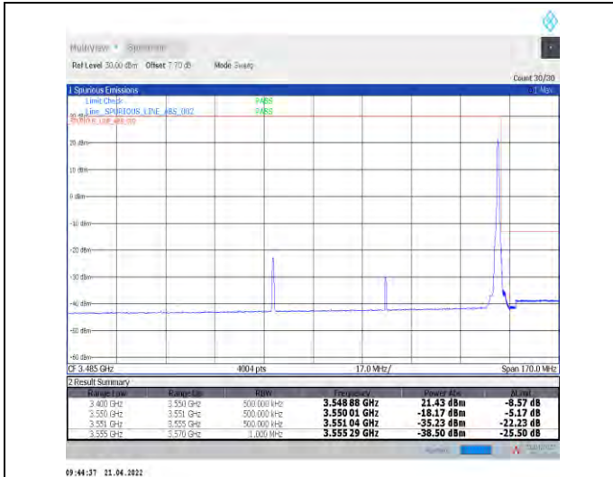
1-N78-3450-3550--30-80-H-2-DFT-PI2BPSK-Edge_1R_B_Right-1@216-Ant0-PASS-see graph
