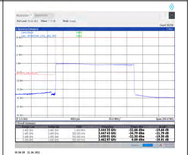
1-N78-3450-3550--30-100-L-6-CP-QPSK-Outer_F ull-273@0-Ant0-PASS-see graph
