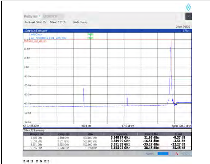
1-N78-3450-3550--30-90-H-2-DFT-PI2BPSK-Edge_1R_B_Right-1@244-Ant0-PASS-see graph
