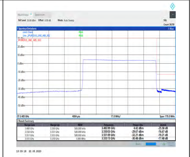
1-N78-3450-3550-PC1-30-80-H-6-CP-QPSK-Outer_Full-217@0-Ant0-1--PASS-see graph
