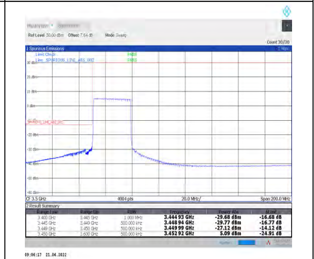
1-N78-3450-3550--30-30-L-6-CP-QPSK-Outer_Ful l-78@0-Ant0-PASS-see graph
