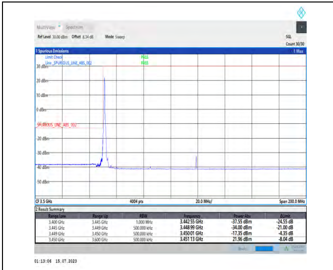
1-N78-3450-3550-PC1-30-70-L-1-DFT-PI2BPSK-Edge_1RB_Left-1@0-Ant0-1--PASS-see graph
