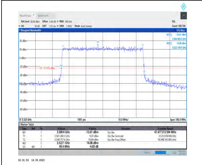
1-N78-3450-3550-PC1-30-50-H-6-CP-QPSK-Outer_Full-133@0-Ant0-47.477-49.400-≤50-PASS
