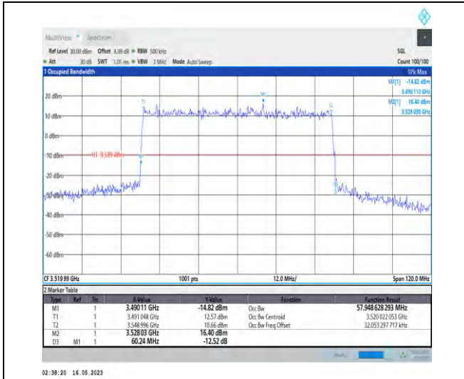
1-N78-3450-3550-PC1-30-60-H-1-DFT-QPSK-Outer_Full-162@0-Ant0-57.949-60.240-≤60-PASS
