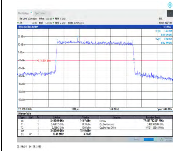
1-N78-3450-3550-PC1-30-80-M-6-CP-QPSK-Outer_Full-217@0-Ant0-77.455-80.480-≤80-PASS
