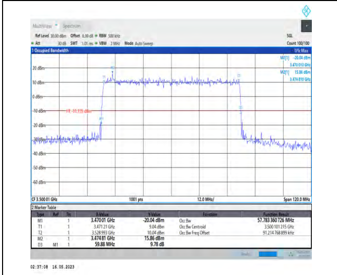
1-N78-3450-3550-PC1-30-60-M-4-DFT-64QAM-Outer_Full-162@0-Ant0-57.783-59.880-≤60-PASS
