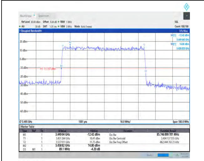
1-N78-3450-3550-PC1-30-90-L-2-DFT-PI2BPSK-Out er_Full-240@0-Ant0-85.611-88.920-≤90-PASS
