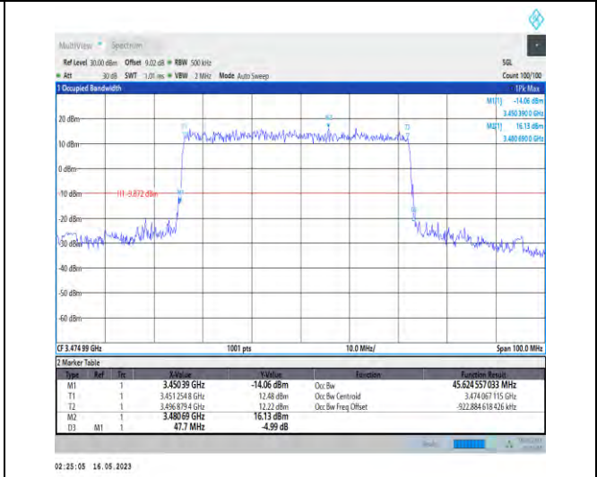
1-N78-3450-3550-PC1-30-50-L-1-DFT-QPSK-Outer_Full-128@0-Ant0-45.625-47.700-≤50-PASS
