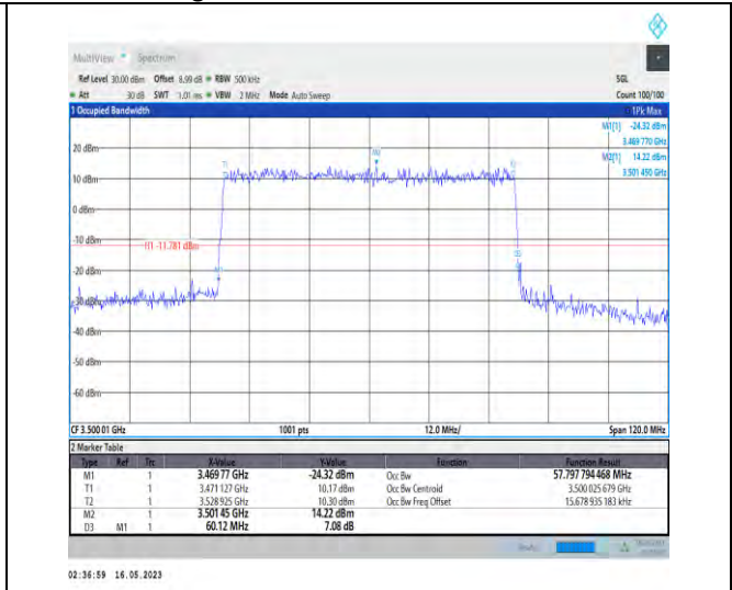
1-N78-3450-3550-PC1-30-60-M-3-DFT-16QAM-Outer_Full-162@0-Ant0-57.798-60.120-≤60-PASS
