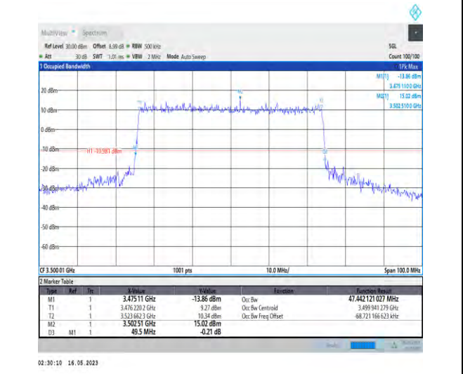
1-N78-3450-3550-PC1-30-50-M-8-CP-64QAM-Outer_Full-133@0-Ant0-47.442-49.500-≤50-PASS
