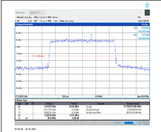
1-N78-3450-3550-PC1-30-40-H-9-CP-256QAM-Outer_Full-106@0-Ant0-37.794-39.600-≤40-PASS
