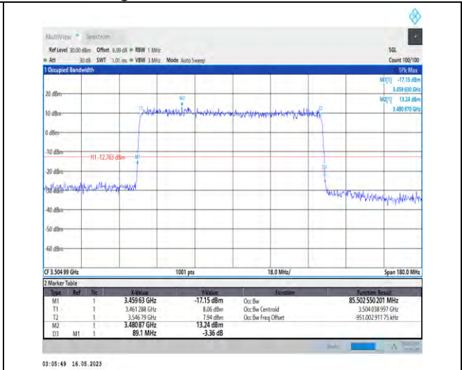
1-N78-3450-3550-PC1-30-90-H-5-DFT-256QAM-Outer_Full-240@0-Ant0-85.503-89.100-≤90-PASS
