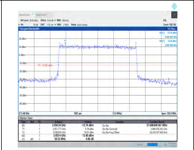
1-N78-3450-3550-PC1-30-60-L-6-CP-QPSK-Outer_Full-162@0-Ant0-57.699-59.520-≤60-PASS
