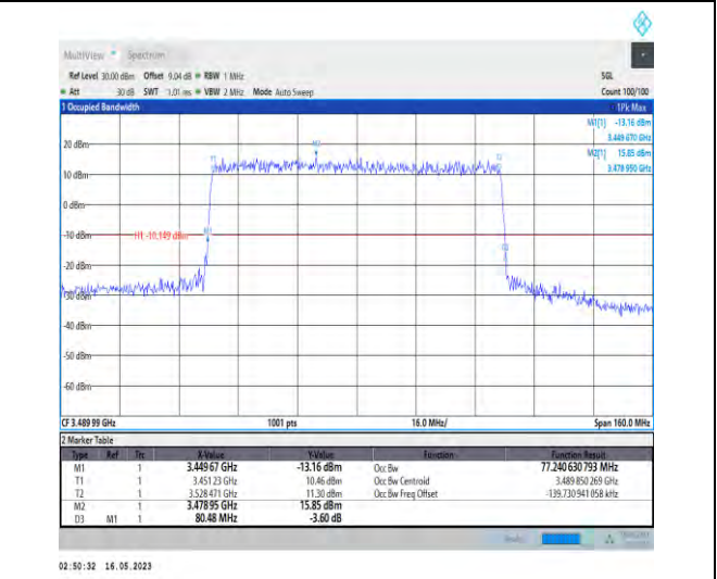
1-N78-3450-3550-PC1-30-80-L-4-DFT-64QAM-Outer_Full-216@0-Ant0-77.241-80.480-≤80-PASS
