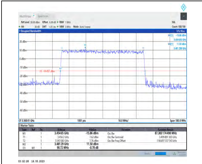
1-N78-3450-3550-PC1-30-90-M-9-CP-256QAM-Out er_Full-245@0-Ant0-87.383-90.720-≤90-PASS
