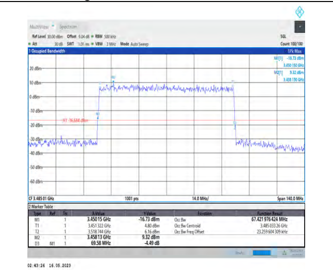
1-N78-3450-3550-PC1-30-70-L-9-CP-256QAM-Outer_Full-189@0-Ant0-67.422-69.580-≤70-PASS
