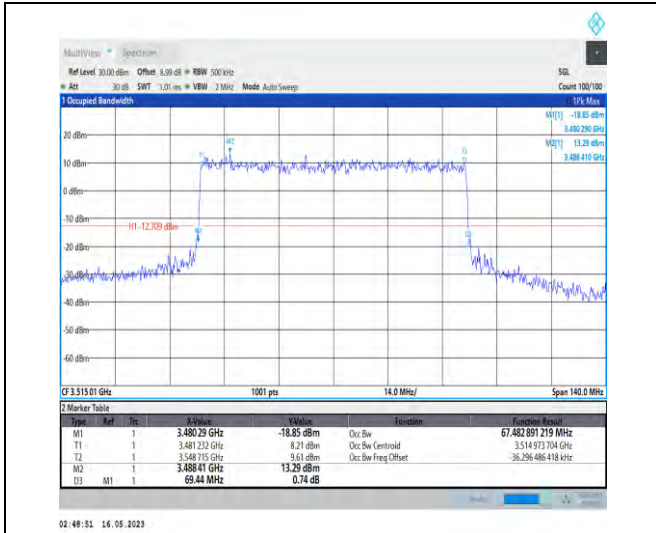
1-N78-3450-3550-PC1-30-70-H-6-CP-QPSK-Outer_Full-189@0-Ant0-67.483-69.440-≤70-PASS
