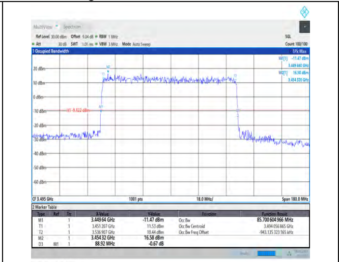
1-N78-3450-3550-PC1-30-90-L-3-DFT-16QAM-Outer_Full-240@0-Ant0-85.701-88.920-≤90-PASS
