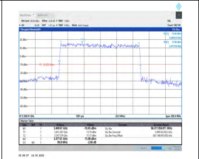
1-N78-3450-3550-PC1-30-100-M-1-DFT-QPSK-Outer_Full-270@0-Ant0-96.312-99.800-≤100-PASS
