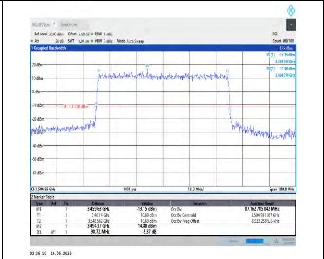
1-N78-3450-3550-PC1-30-90-H-7-CP-16QAM-Outer_Full-245@0-Ant0-87.163-90.720-≤90-PASS
