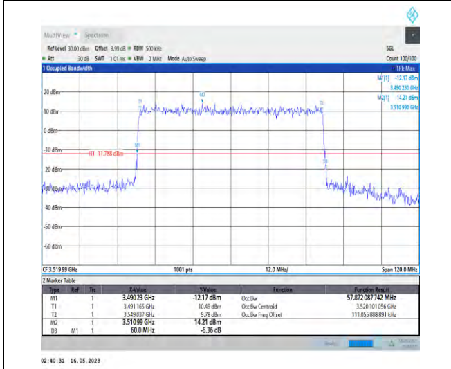
1-N78-3450-3550-PC1-30-60-H-3-DFT-16QAM-Outer_Full-162@0-Ant0-57.872-60.000-≤60-PASS
