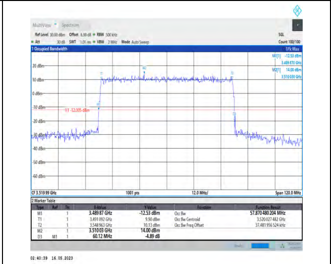
1-N78-3450-3550-PC1-30-60-H-4-DFT-64QAM-Outer_Full-162@0-Ant0-57.87-60.120-≤60-PASS
