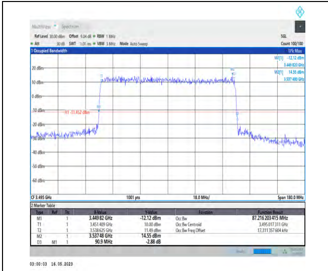
1-N78-3450-3550-PC1-30-90-L-6-CP-QPSK-Outer_Full-245@0-Ant0-87.216-90.900-<math>\leq 90</math>-PASS
