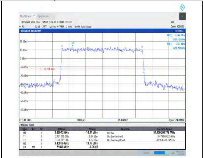
1-N78-3450-3550-PC1-30-60-L-4-DFT-64QAM-Outer_Full-162@0-Ant0-57.9-59.880-≤60-PASS
