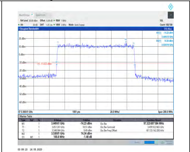
1-N78-3450-3550-PC1-30-100-L-8-CP-64QAM-Outer_Full-273@0-Ant0-97.323-100.800-≤100-PASS
