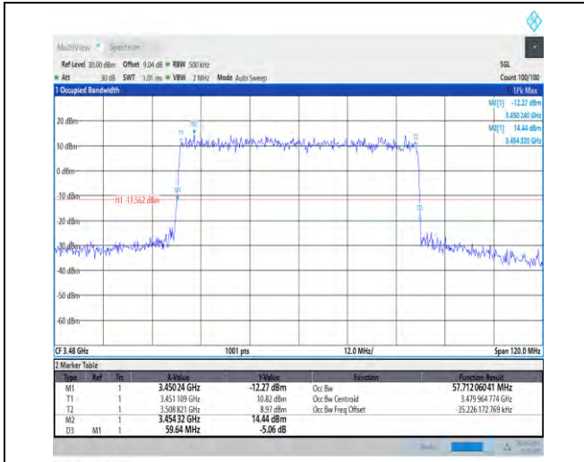
1-N78-3450-3550-PC1-30-60-L-3-DFT-16QAM-Outer_Full-162@0-Ant0-57.712-59.640-≤60-PASS
