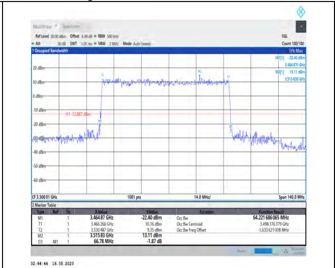
1-N78-3450-3550-PC1-30-70-M-4-DFT-64QAM-Out_r_Full-180@0-Ant0-64.222-66.780-≤70-PASS
