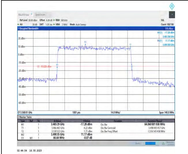
1-N78-3450-3550-PC1-30-70-M-5-DFT-256QAM-Out_Full-180@0-Ant0-64.06-66.640-≤70-PASS
