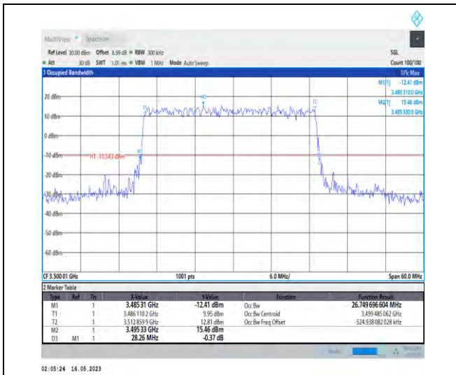
1-N78-3450-3550-PC1-30-30-M-3-DFT-16QAM-Out er_Full-75@0-Ant0-26.75-28.260-≤30-PASS
