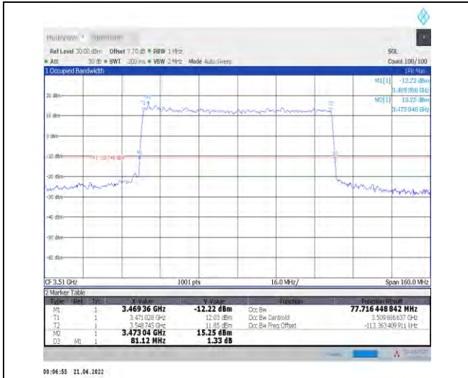
1-N78-3450-3550--30-80-H-7-CP-16QAM-Outer_Full -217@0-Ant0-77.716-81.120-≤80-PASS
