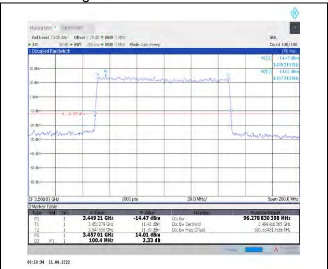
1-N78-3450-3550--30-100-L-4-DFT-64QAM-Outer_F ull-270@0-Ant0-96.279-100.400-≤100-PASS
