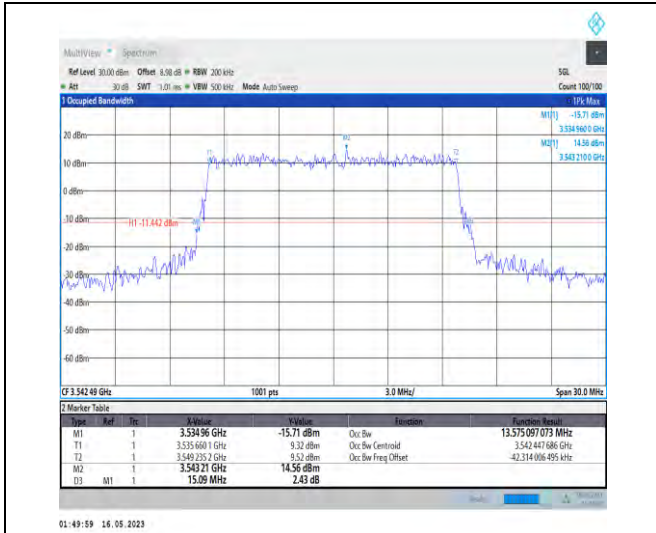
1-N78-3450-3550-PC1-30-15-H-8-CP-64QAM-Outer_Full-38@0-Ant0-13.575-15.090-≤15-PASS
