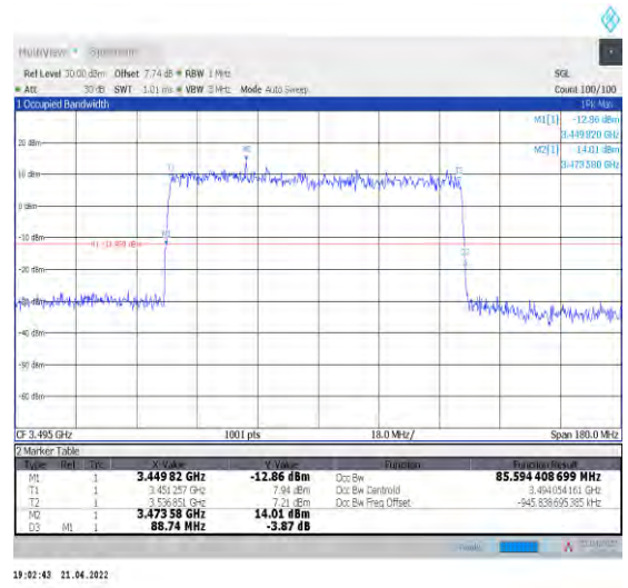
1-N78-3450-3550--30-90-L-5-DFT-256QAM-Outer_Full-240@0-Ant0-85.594-88.740-<=90-PASS
