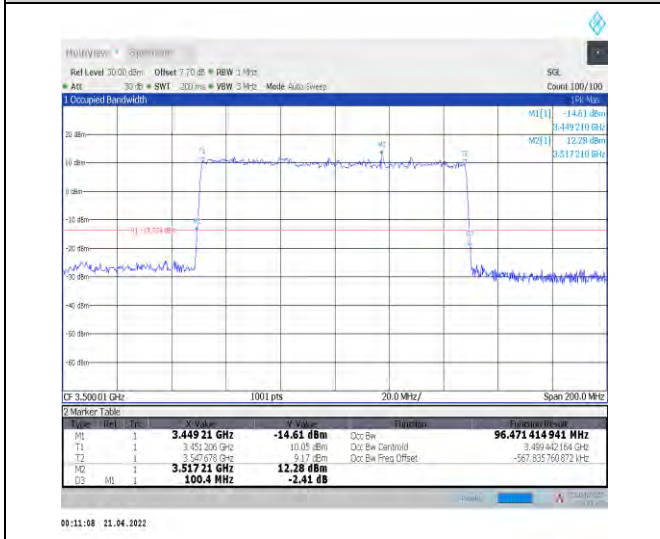
1-N78-3450-3550--30-100-L-5-DFT-256QAM-Outer_F ull-270@0-Ant0-96.471-100.400-≤100-PASS
