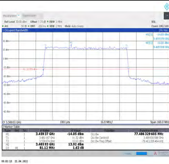
1-N78-3450-3550--30-80-M-8-CP-64QAM-Outer_Full -217@0-Ant0-77.486-81.120-≤80-PASS
