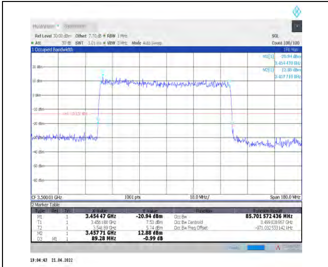
1-N78-3450-3550--30-90-M-5-DFT-256QAM-Outer_Full-240@0-Ant0-85.702-89.280-<math>\leq 90</math>-PASS
