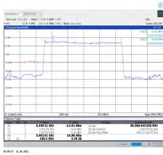
1-N78-3450-3550--30-100-L-2-DFT-PI2BPSK-Outer_Full Full-270@0-Ant0-96.366-100.400-≤100-PASS
