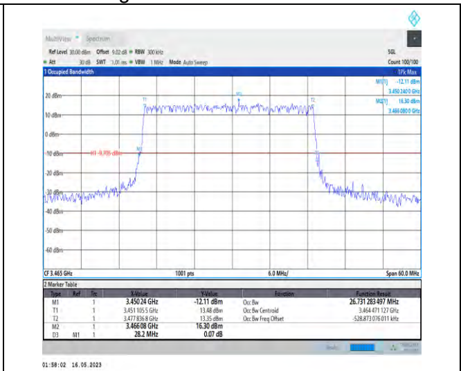
1-N78-3450-3550-PC1-30-30-L-1-DFT-QPSK-Outer_Full-75@0-Ant0-26.731-28.200-≤30-PASS
