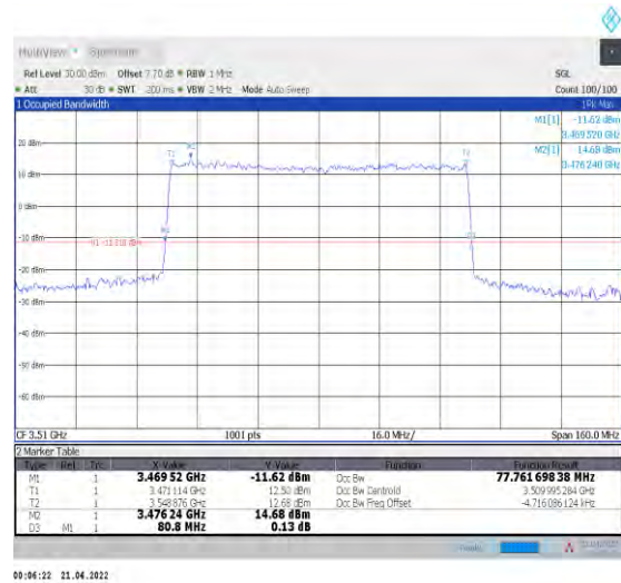
1-N78-3450-3550--30-80-H-6-CP-QPSK-Outer_Full-217@0-Ant0-77.762-80.800-<math>\leq 80</math>-PASS
