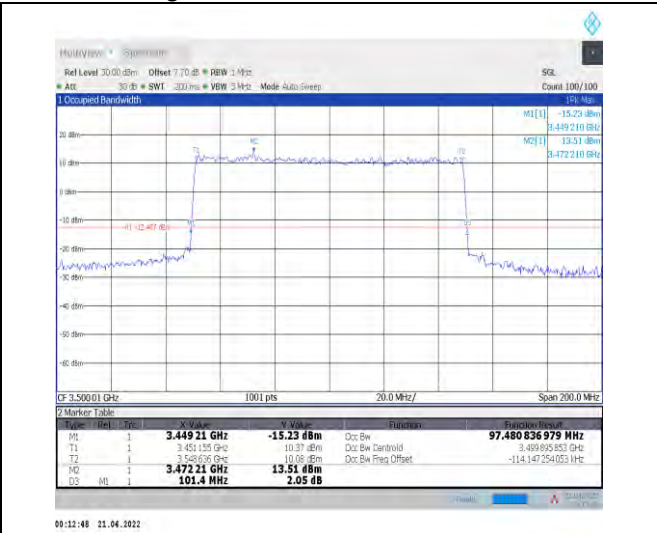
1-N78-3450-3550--30-100-L-8-CP-64QAM-Outer_Fu II-273@0-Ant0-97.481-101.400-≤100-PASS
