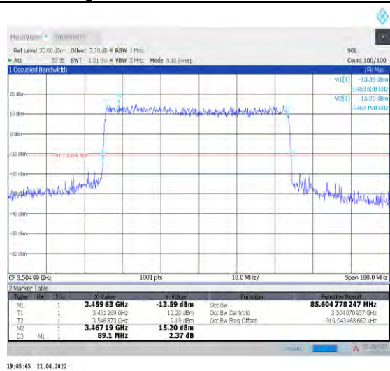
1-N78-3450-3550--30-90-H-1-DFT-QPSK-Outer_Full-240@0-Ant0-85.605-89.100-<=90-PASS
