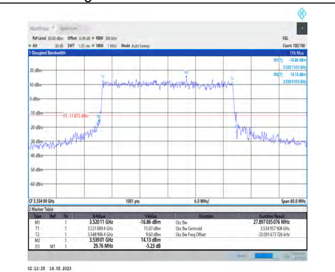
1-N78-3450-3550-PC1-30-30-H-7-CP-16QAM-Outer_Full-78@0-Ant0-27.897-29.760-≤30-PASS
