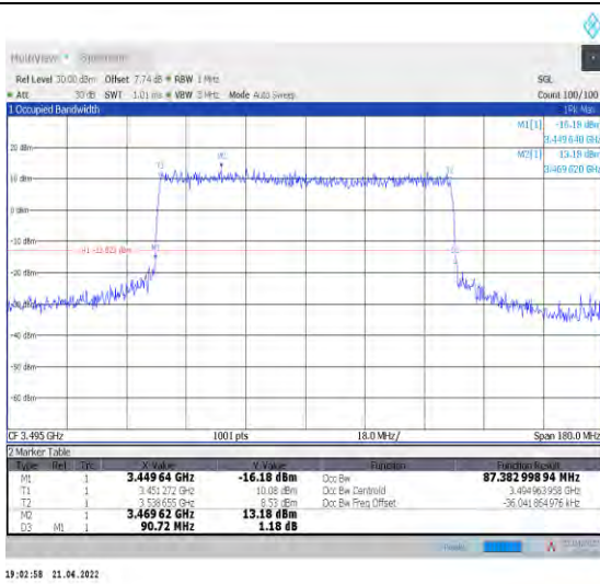
1-N78-3450-3550--30-90-L-6-CP-QPSK-Outer_Full-2 -45@0-Ant0-87.383-90.720≤90-PASS
