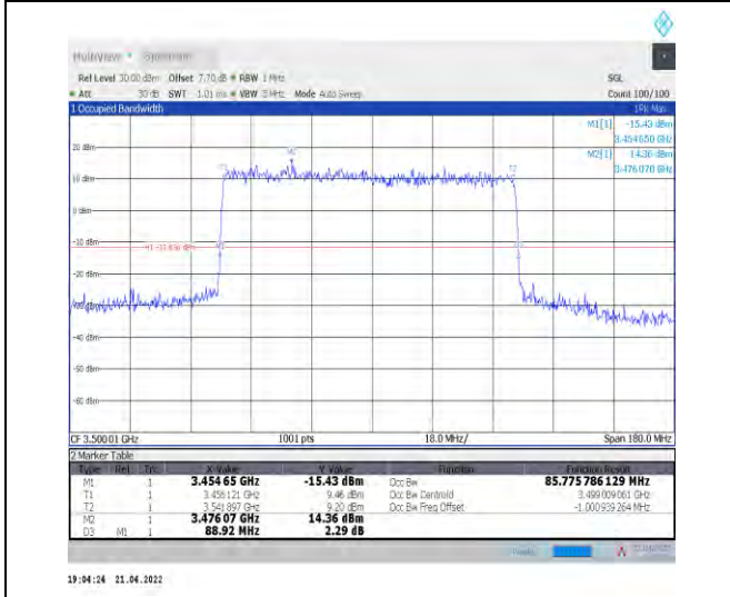
1-N78-3450-3550--30-90-M-3-DFT-16QAM-Outer_Full -240@0-Ant0-85.776-88.920-≤90-PASS
