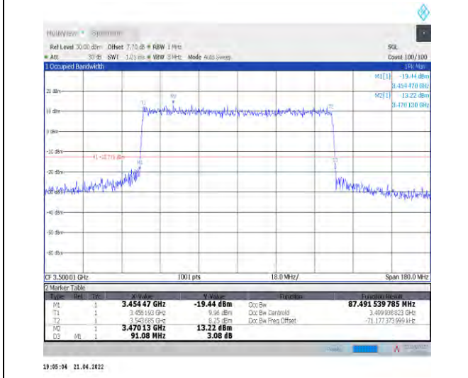
1-N78-3450-3550--30-90-M-7-CP-16QAM-Outer_Full-245@0-Ant0-87.492-91.080-<math>\leq 90</math>-PASS
