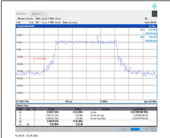
1-N78-3450-3550-PC1-30-10-H-7-CP-16QAM-Outer_Full-24@0-Ant0-8.538-9.420-≤10-PASS
