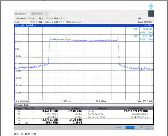
1-N78-3450-3550--30-100-M-7-CP-16QAM-Outer_Full -273@0-Ant0-97.511-101.400-≤100-PASS
