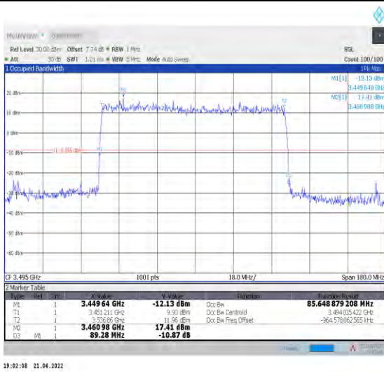
1-N78-3450-3550--30-90-L-2-DFT-PI2BPSK-Outer_Full-240@0-Ant0-85.649-89.280-<=90-PASS
