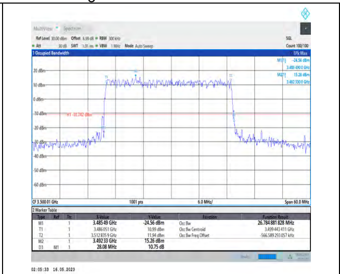
1-N78-3450-3550-PC1-30-30-M-4-DFT-64QAM-Outer er_Full-75@0-Ant0-26.785-28.080-≤30-PASS
