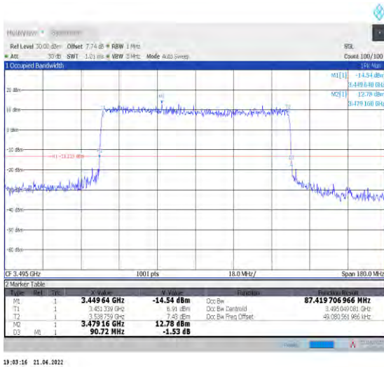
1-N78-3450-3550--30-90-L-8-CP-64QAM-Outer_Full -245@0-Ant0-87.42-90.720≤90-PASS
