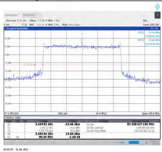
1-N78-3450-3550--30-90-L-7-CP-16QAM-Outer_Full -245@0-Ant0-87.558-90.540≤90-PASS
