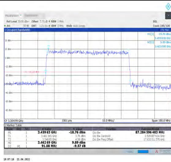
1-N78-3450-3550--30-90-H-9-CP-256QAM-Outer_Full -245@0-Ant0-87.285-91.080-≤90-PASS
