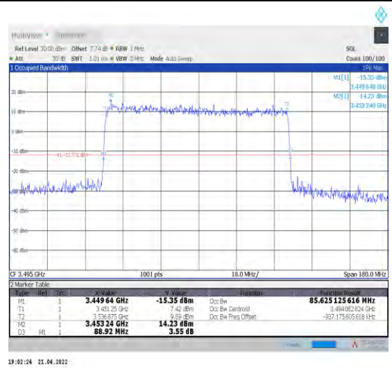
1-N78-3450-3550--30-90-L-3-DFT-16QAM-Outer_Full-240@0-Ant0-85.625-88.920-<=90-PASS
