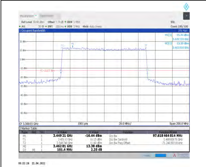
1-N78-3450-3550--30-100-H-7-CP-16QAM-Outer_Full-273@0-Ant0-97.618-101.400-≤100-PASS
