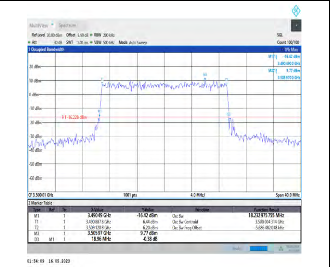
1-N78-3450-3550-PC1-30-20-M-9-CP-256QAM-Outer_Full-51@0-Ant0-18.233-18.960-≤20-PASS
