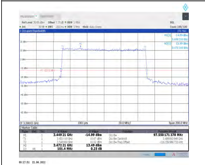
1-N78-3450-3550--30-100-M-8-CP-64QAM-Outer_Full -273@0-Ant0-97.55-101.400-≤100-PASS
