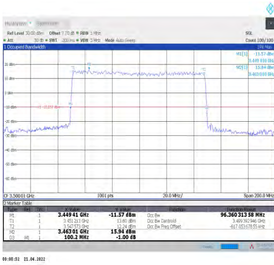
1-N78-3450-3550--30-100-L-1-DFT-QPSK-Outer_Full I-270@0-Ant0-96.36-100.200-≤100-PASS
