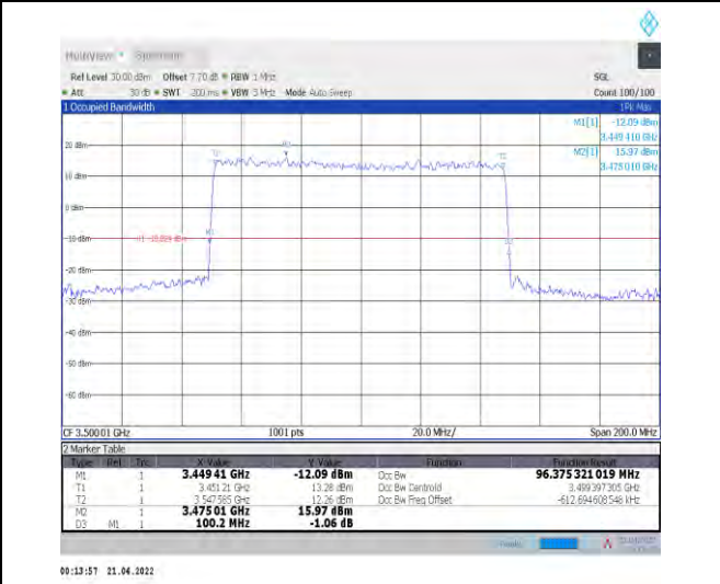
1-N78-3450-3550--30-100-M-1-DFT-QPSK-Outer_F ull-270@0-Ant0-96.375-100.200-≤100-PASS
