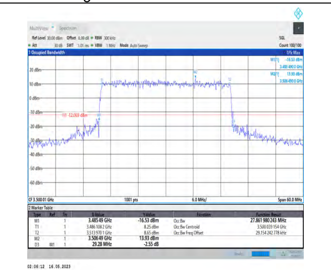
1-N78-3450-3550-PC1-30-30-M-8-CP-64QAM-Outer_Full-78@0-Ant0-27.862-29.280-≤30-PASS
