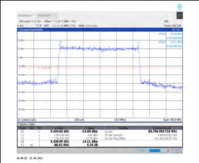
1-N78-3450-3550--30-90-M-4-DFT-64QAM-Outer_Full -240@0-Ant0-85.705-88.920-≤90-PASS
