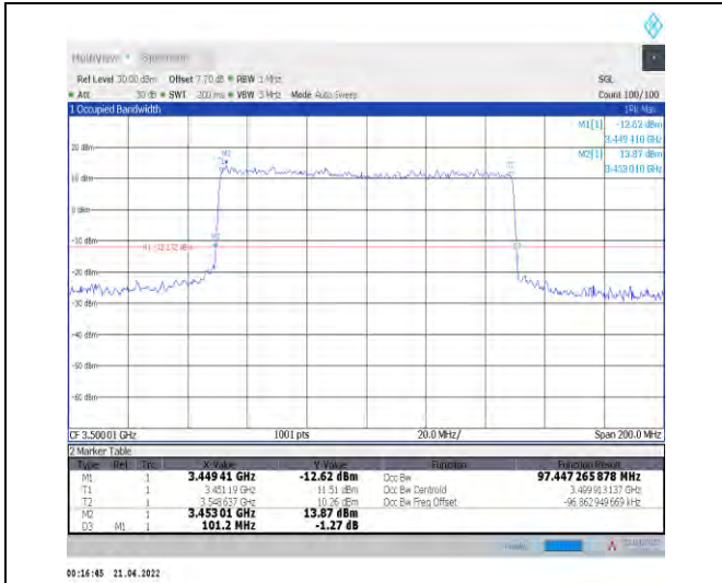
1-N78-3450-3550--30-100-M-6-CP-QPSK-Outer_Full -273@0-Ant0-97.447-101.200-≤100-PASS
