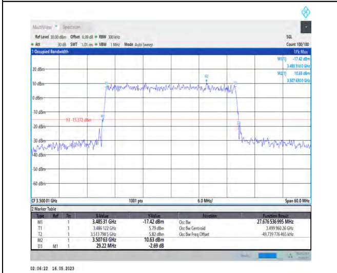
1-N78-3450-3550-PC1-30-30-M-9-CP-256QAM-Outer_Full-78@0-Ant0-27.677-29.220-≤30-PASS
