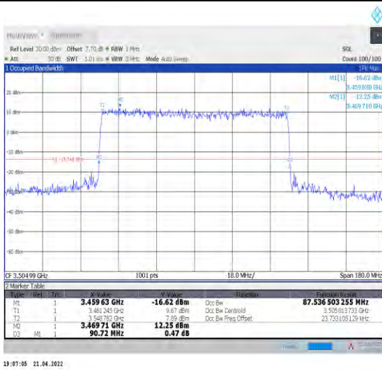
1-N78-3450-3550--30-90-H-8-CP-64QAM-Outer_Full -245@0-Ant0-87.537-90.720-≤90-PASS
