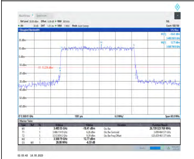
1-N78-3450-3550-PC1-30-30-M-5-DFT-256QAM-Outer er_Full-75@0-Ant0-26.739-28.080-≤30-PASS
