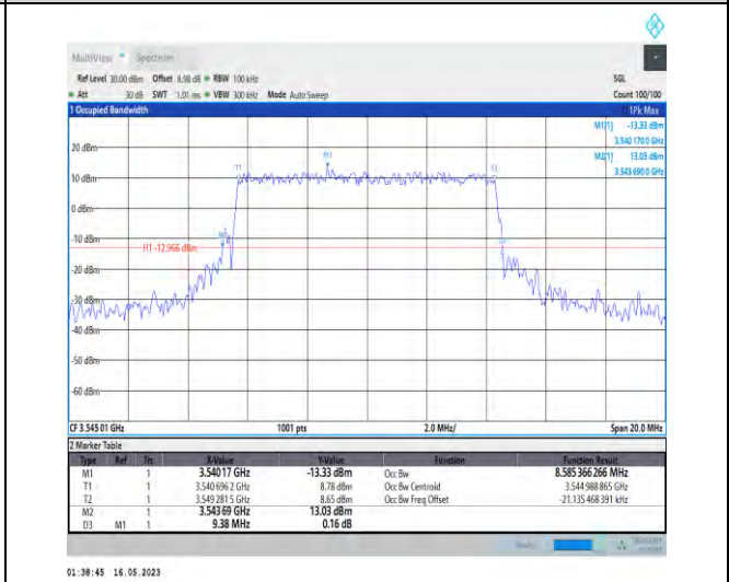
1-N78-3450-3550-PC1-30-10-H-6-CP-QPSK-Outer_Full-24@0-Ant0-8.585-9.380-≤10-PASS
