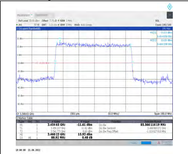
1-N78-3450-3550--30-90-M-2-DFT-PI2BPSK-Outer_Full -240@0-Ant0-85.566-88.920-≤90-PASS
