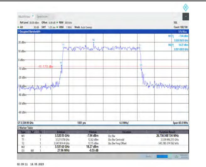
1-N78-3450-3550-PC1-30-30-H-1-DFT-QPSK-Outer_Full-75@0-Ant0-26.736-27.960-≤30-PASS
