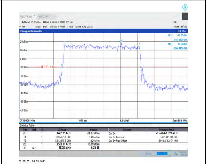
1-N78-3450-3550-PC1-30-30-M-2-DFT-PI2BPSK-Outer _Full-75@0-Ant0-26.74-28.080-≤30-PASS
