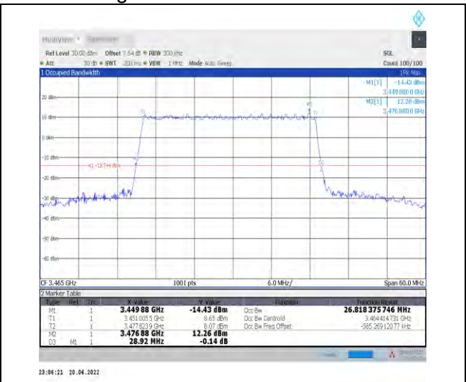
1-N78-3450-3550--30-30-L-5-DFT-256QAM-Outer_Full ull-75@0-Ant0-26.818-28.920-≤30-PASS
