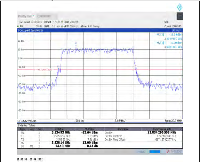
1-N78-3450-3550--30-15-H-5-DFT-256QAM-Outer_F ull-36@0-Ant0-12.854-14.130-≤15-PASS
