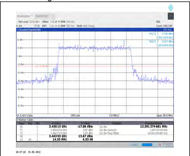
1-N78-3450-3550--30-15-L-7-CP-16QAM-Outer_Full -38@0-Ant0-13.591-14.550-≤15-PASS
