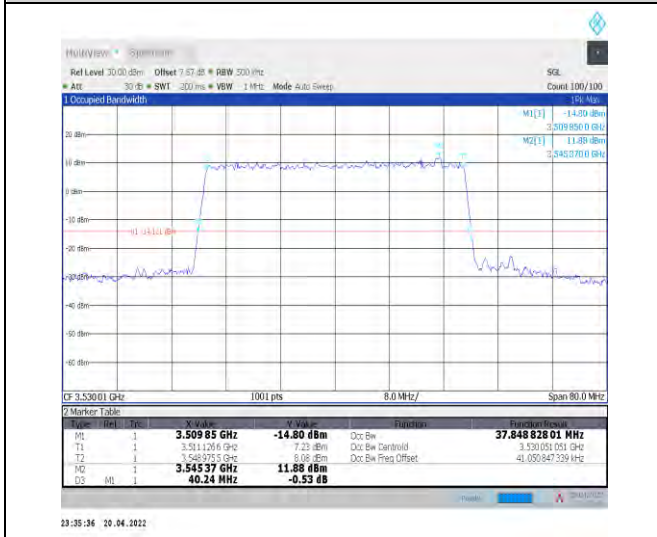
1-N78-3450-3550--30-40-H-9-CP-256QAM-Outer_Fu ll-106@0-Ant0-37.849-40.240-≤40-PASS
