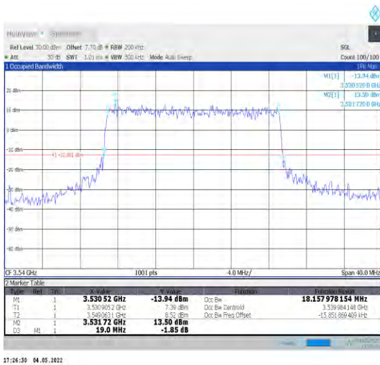
1-N78-3450-3550--30-20-H-7-CP-16QAM-Outer_Full-51@0-Ant0-18.158-19.000-≤20-PASS
