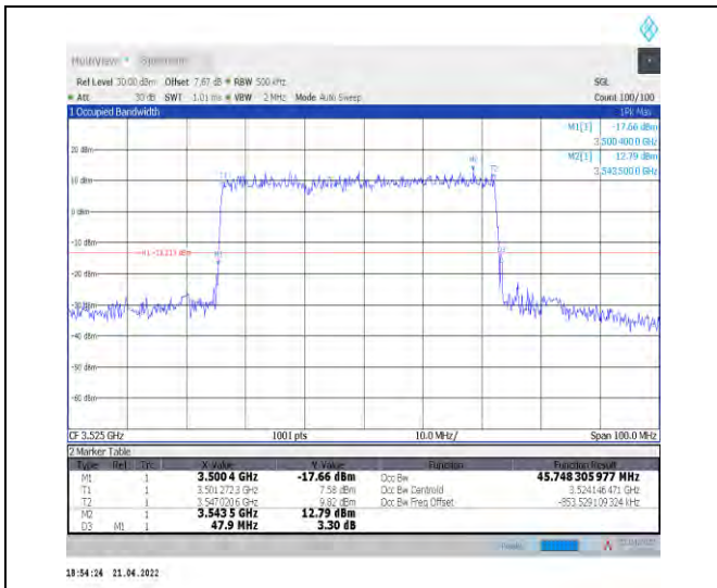
1-N78-3450-3550--30-50-H-4-DFT-64QAM-Outer_Fu II-128@0-Ant0-45.748-47.900-≤50-PASS
