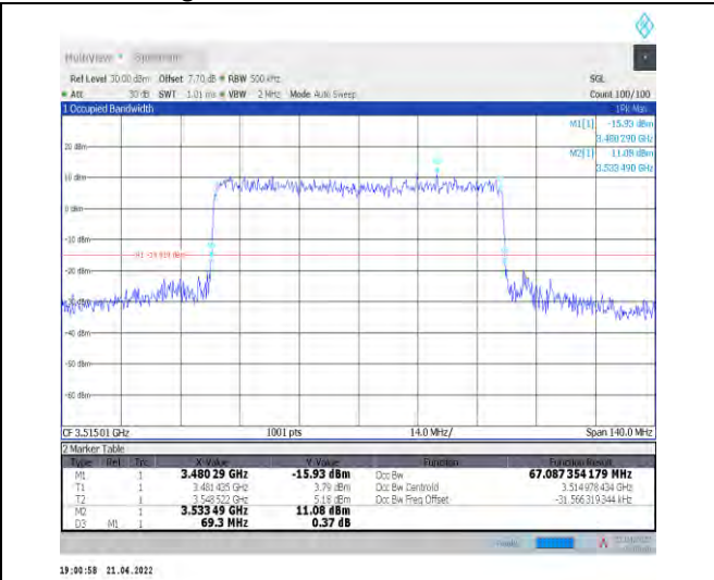
1-N78-3450-3550--30-70-H-7-CP-16QAM-Outer_Full-189@0-Ant0-67.087-69.300-≤70-PASS
