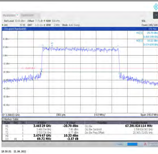
1-N78-3450-3550--30-70-M-7-CP-16QAM-Outer_Full -189@0-Ant0-67.392-69.720-≤70-PASS
