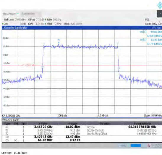
1-N78-3450-3550--30-70-M-1-DFT-QPSK-Outer_Full -180@0-Ant0-64.315-66.220-≤70-PASS
