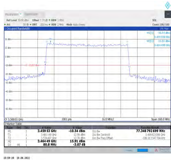
1-N78-3450-3550--30-80-M-3-DFT-16QAM-Outer_Full ull-216@0-Ant0-77.349-80.800≤80-PASS
