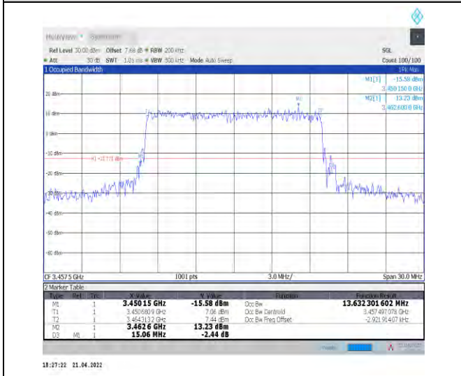
1-N78-3450-3550--30-15-L-8-CP-64QAM-Outer_Full -38@0-Ant0-13.632-15.060-≤15-PASS
