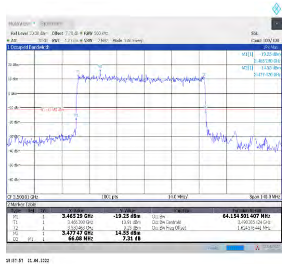
1-N78-3450-3550--30-70-M-2-DFT-PI2BPSK-Outer_Full Full-180@0-Ant0-64.155-66.080-≤70-PASS
