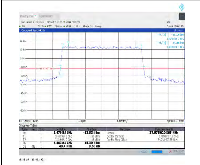
1-N78-3450-3550--30-40-M-6-CP-QPSK-Outer_Full-106@0-Ant0-37.975-40.400-<math>\leq 40</math>-PASS
