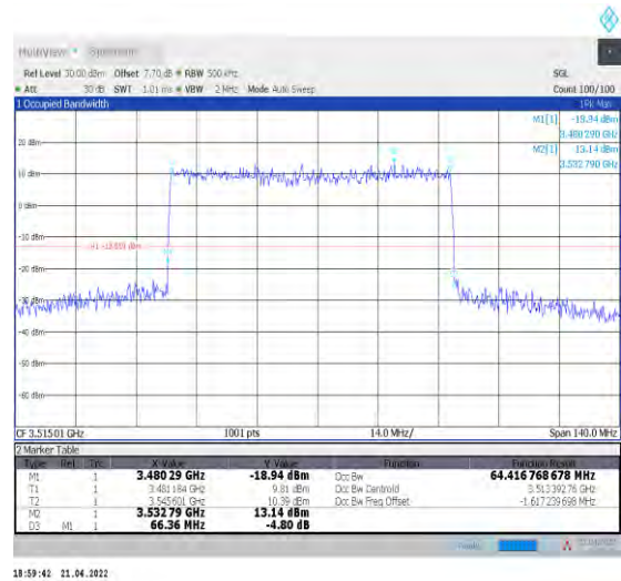
1-N78-3450-3550--30-70-H-1-DFT-QPSK-Outer_Full -180@0-Ant0-64.417-66.360-≤70-PASS
