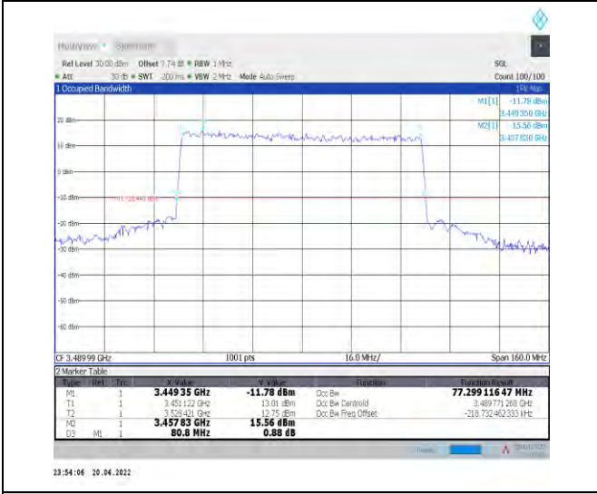
1-N78-3450-3550--30-80-L-3-DFT-16QAM-Outer_Ful-I-216@0-Ant0-77.299-80.800-≤80-PASS
