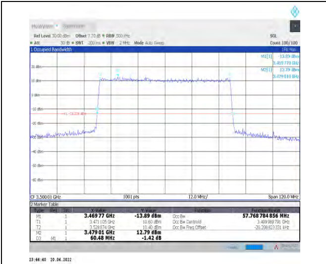
1-N78-3450-3550--30-60-M-6-CP-QPSK-Outer_Full-162@0-Ant0-57.769-60.480-<math>\leq 60</math>-PASS
