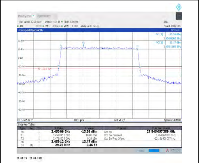
1-N78-3450-3550--30-30-L-7-CP-16QAM-Outer_Full-78 -78@0-Ant0-27.845-29.760-≤30-PASS
