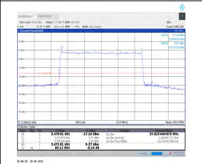
1-N78-3450-3550--30-60-M-9-CP-256QAM-Outer_Full-162@0-Ant0-57.825-60.120-<math>\leq 60</math>-PASS
