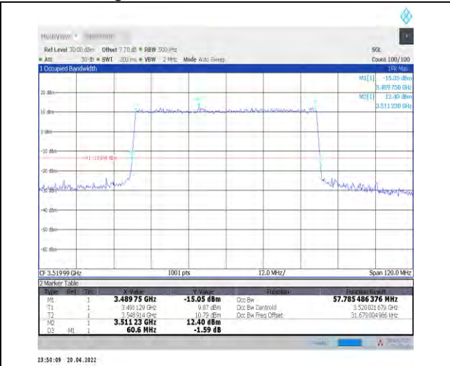
1-N78-3450-3550--30-60-H-6-CP-QPSK-Outer_Full-162@0-Ant0-57.785-60.600-≤60-PASS
