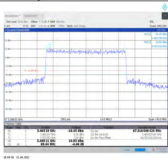
1-N78-3450-3550--30-70-M-8-CP-64QAM-Outer_Ful I-189@0-Ant0-67.316-69.440-≤70-PASS
