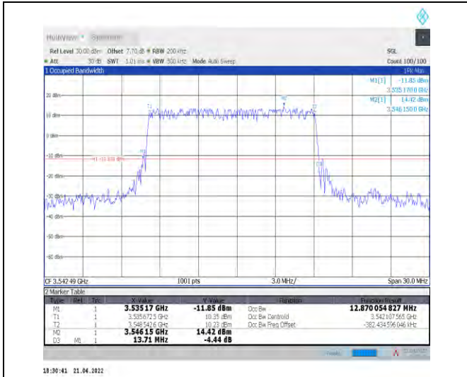
1-N78-3450-3550--30-15-H-4-DFT-64QAM-Outer_Fu ll-36@0-Ant0-12.87-13.710-≤15-PASS
