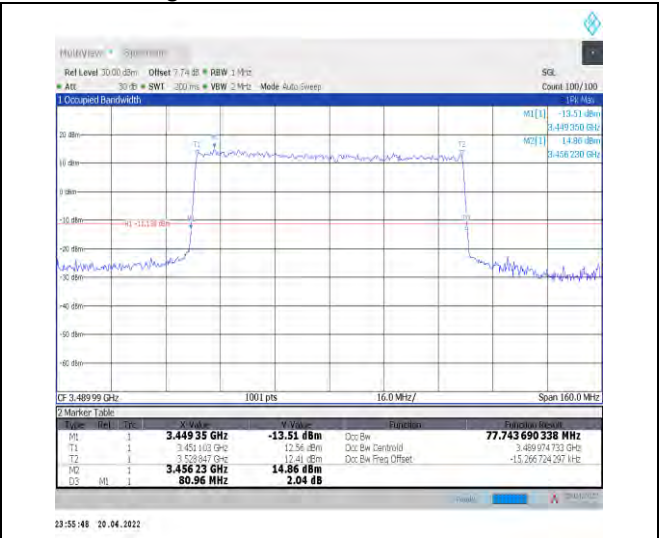
1-N78-3450-3550--30-80-L-6-CP-QPSK-Outer_Full-217@0-Ant0-77.744-80.960-<math>\leq 80</math>-PASS
