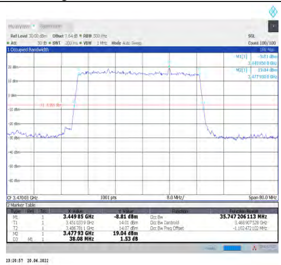
1-N78-3450-3550--30-40-L-2-DFT-PI2BPSK-Outer_Full-100@0-Ant0-35.747-38.080-≤40-PASS
