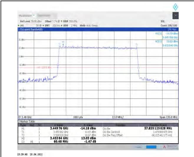
1-N78-3450-3550--30-60-L-7-CP-16QAM-Outer_Full -162@0-Ant0-57.835-60.480-≤60-PASS
