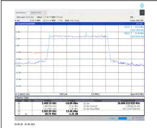
1-N78-3450-3550--30-30-M-1-DFT-QPSK-Outer_Full -75@0-Ant0-26.807-28.740-<30-PASS
