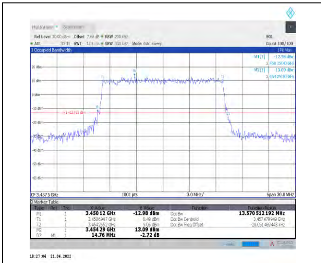
1-N78-3450-3550--30-15-L-6-CP-QPSK-Outer_Full_3 8@0-Ant0-13.571-14.760-≤15-PASS
