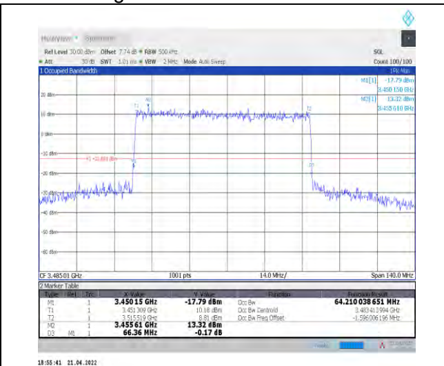
1-N78-3450-3550--30-70-L-1-DFT-QPSK-Outer_Full-180@0-Ant0-64.21-66.360-≤70-PASS
