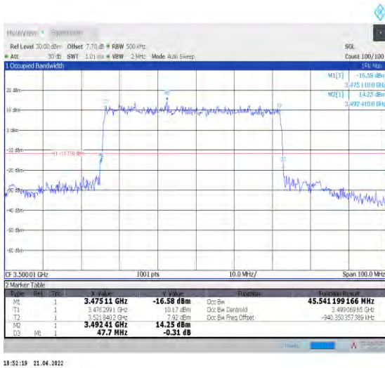
1-N78-3450-3550--30-50-M-3-DFT-16QAM-Outer_Full Full-128@0-Ant0-45.541-47.700-≤50-PASS
