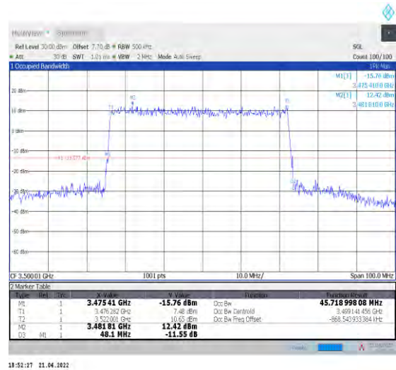
1-N78-3450-3550--30-50-M-4-DFT-64QAM-Outer_Full Full-128@0-Ant0-45.719-48.100-≤50-PASS
