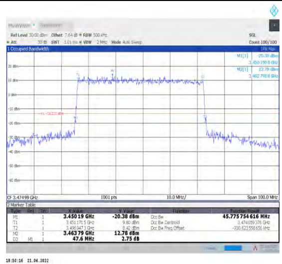
1-N78-3450-3550--30-50-L-3-DFT-16QAM-Outer_Full-128@0-Ant0-45.776-47.600-≤50-PASS
