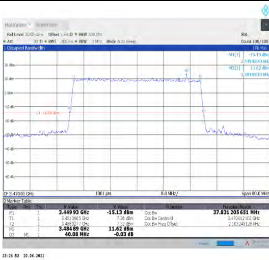
1-N78-3450-3550--30-40-L-9-CP-256QAM-Outer_Fu II-106@0-Ant0-37.831-40.080-≤40-PASS
