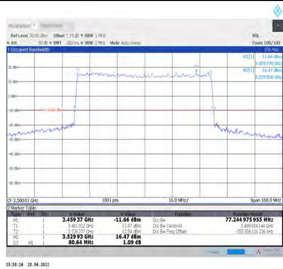
1-N78-3450-3550--30-80-M-1-DFT-QPSK-Outer_Full -216@0-Ant0-77.245-80.640≤80-PASS
