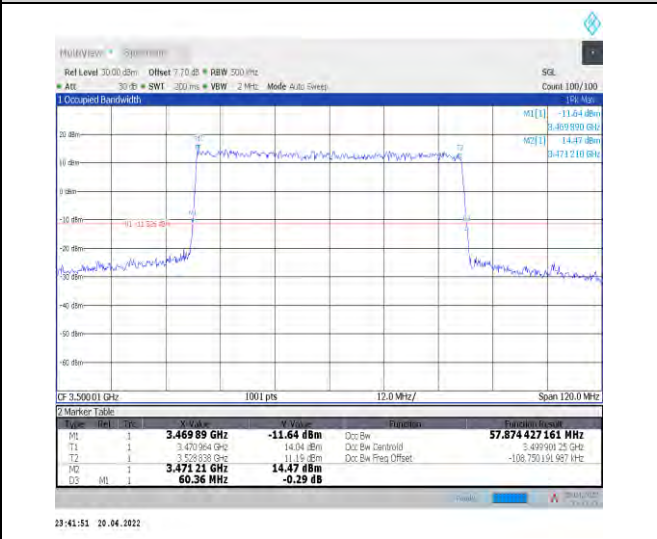
1-N78-3450-3550--30-60-M-1-DFT-QPSK-Outer_Full -162@0-Ant0-57.874-60.360-≤60-PASS
