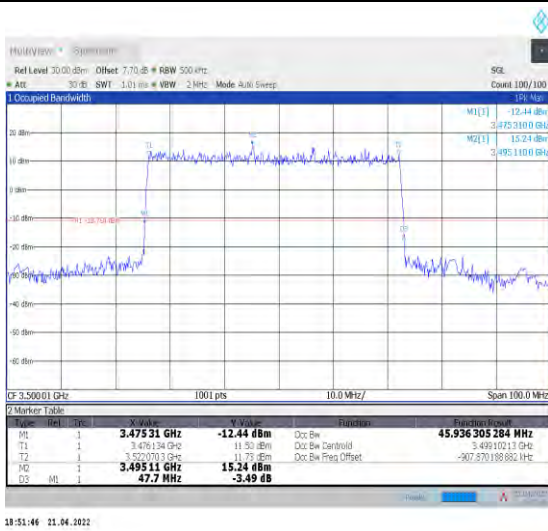
1-N78-3450-3550--30-50-M-1-DFT-QPSK-Outer_Full -128@0-Ant0-45.936-47.700-≤50-PASS
