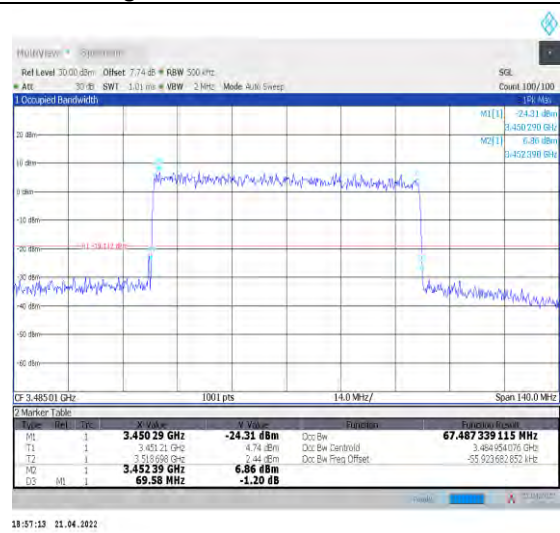
1-N78-3450-3550--30-70-L-9-CP-256QAM-Outer_Fu II-189@0-Ant0-67.487-69.580-≤70-PASS
