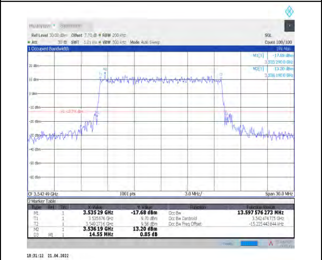
1-N78-3450-3550--30-15-H-7-CP-16QAM-Outer_Full-38@0-Ant0-13.598-14.550-≤15-PASS
