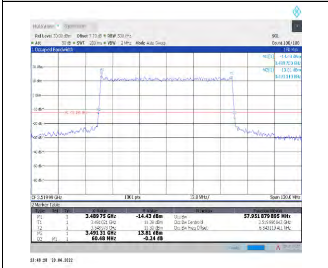
1-N78-3450-3550--30-60-H-3-DFT-16QAM-Outer_Fu ll-162@0-Ant0-57.952-60.480-≤60-PASS
