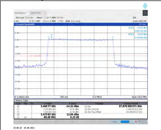
1-N78-3450-3550--30-60-M-7-CP-16QAM-Outer_Full-162@0-Ant0-57.879-60.480-<math>\leq 60</math>-PASS
