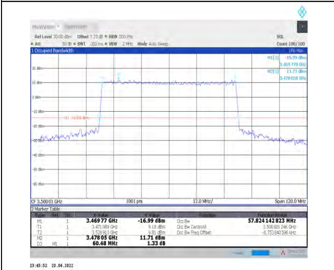
1-N78-3450-3550--30-60-M-8-CP-64QAM-Outer_Full-162@0-Ant0-57.824-60.480-<math>\leq 60</math>-PASS
