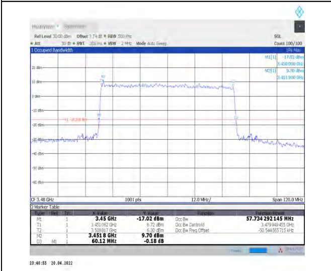
1-N78-3450-3550--30-60-L-9-CP-256QAM-Outer_Fu ll-162@0-Ant0-57.734-60.120-≤60-PASS
