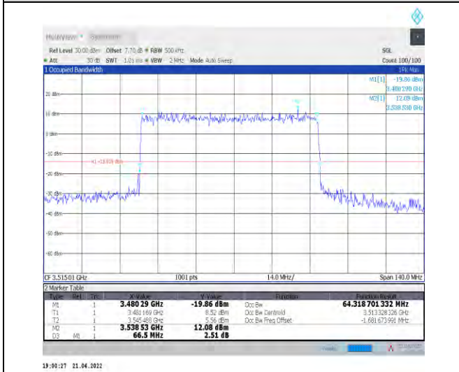
1-N78-3450-3550--30-70-H-4-DFT-64QAM-Outer_Fu II-180@0-Ant0-64.319-66.500-≤70-PASS
