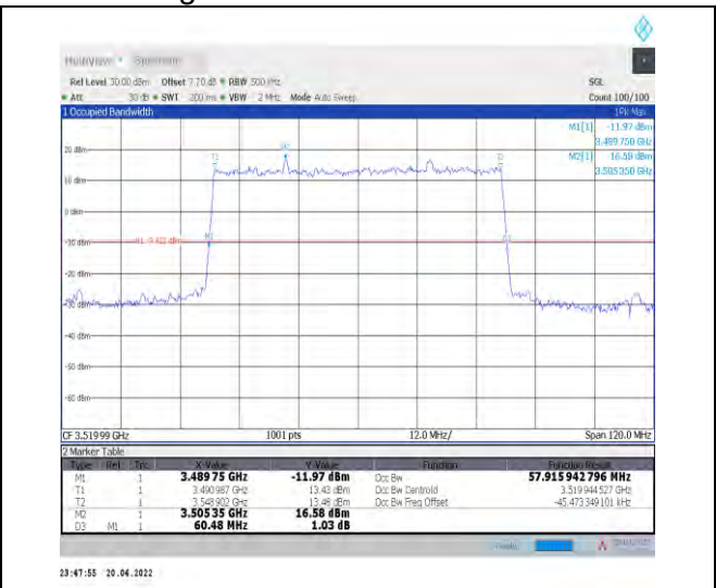
1-N78-3450-3550--30-60-H-2-DFT-PI2BPSK-Outer_Full Full-162@0-Ant0-57.916-60.480-≤60-PASS
