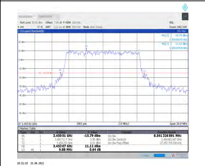
1-N78-3450-3550--30-10-L-8-CP-64QAM-Outer_Full-24@0-Ant0-8.541-9.880-≤10-PASS
