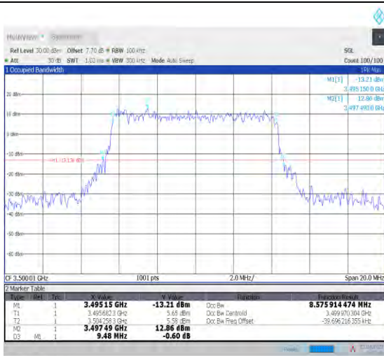
1-N78-3450-3550--30-10-M-4-DFT-64QAM-Outer_Full-24@0-Ant0-8.576-9.480-≤10-PASS
