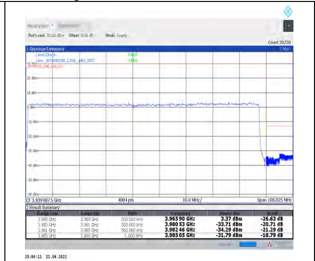
1-N77-3700-3980--30-90-H-3-DFT-PI2BPSK-Outer_Full-240@0-Ant0-PASS-see graph
