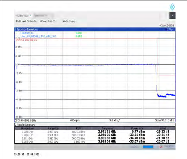
1-N77-3700-3980--30-80-H-6-CP-QPSK-Outer_Full-217@0-Ant0-PASS-see graph
