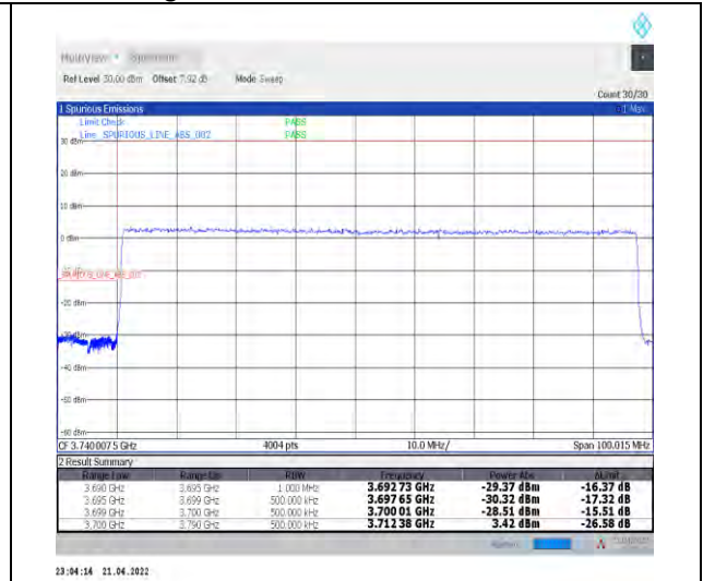
1-N77-3700-3980--30-90-L-3-DFT-PI2BPSK-Outer_Full-240@0-Ant0-PASS-see graph
