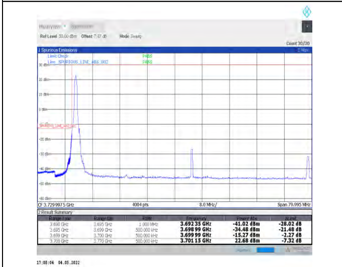
1-N77-3700-3980--30-70-L-4-CP-QPSK-Edge_1RB_L_eft-1@0-Ant0-PASS-see graph
