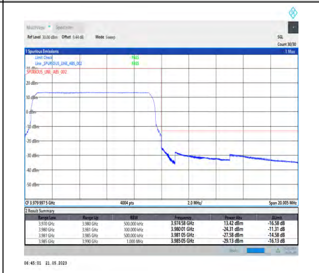
1-N77-3700-3980-PC1-30-10-H-6-CP-QPSK-Outer_Full-24@0-Ant0-1--PASS-see graph
