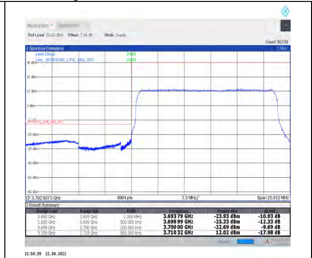
1-N77-3700-3980--30-15-L-3-DFT-PI2BPSK-Outer_Full-36@0-Ant0-PASS-see graph
