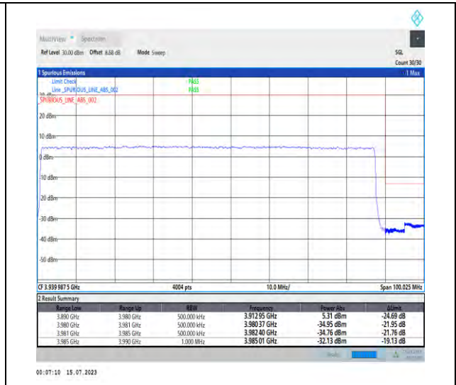
1-N77-3700-3980-PC1-30-90-H-3-DFT-PI2BPSK-Outer_Full-240@0-Ant0-1--PASS-see graph
