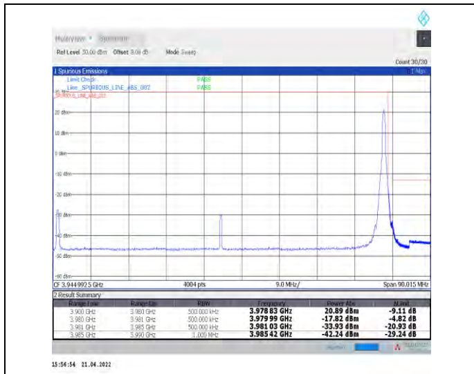
1-N77-3700-3980--30-80-H-2-DFT-PI2BPSK-Edge_1R_B_Right-1@216-Ant0-PASS-see graph
