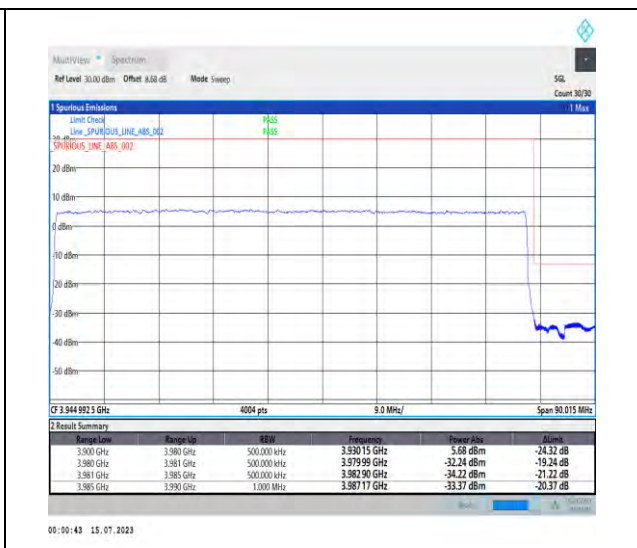
1-N77-3700-3980-PC1-30-80-H-3-DFT-PI2BPSK-Outer_Full-216@0-Ant0-1--PASS-see graph
