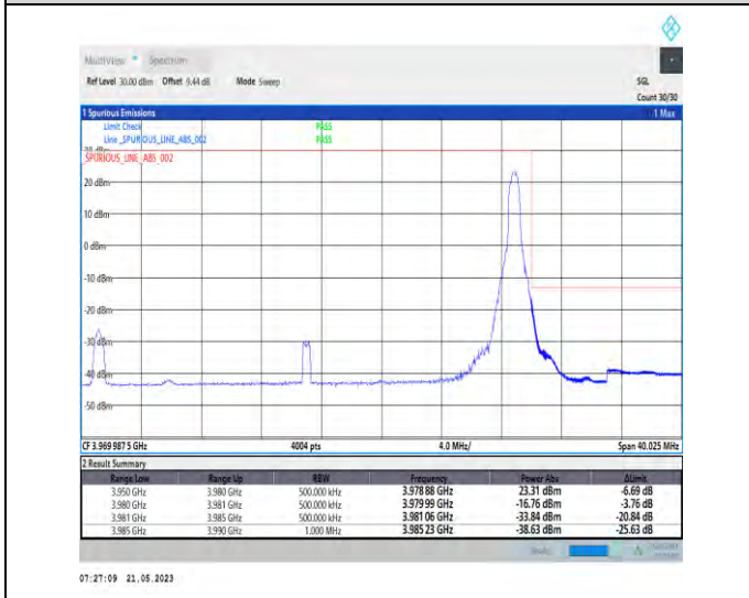
1-N77-3700-3980-PC1-30-30-H-5-CP-QPSK-Edge_1RB_Right-1@77-Ant0-1--PASS-see graph
