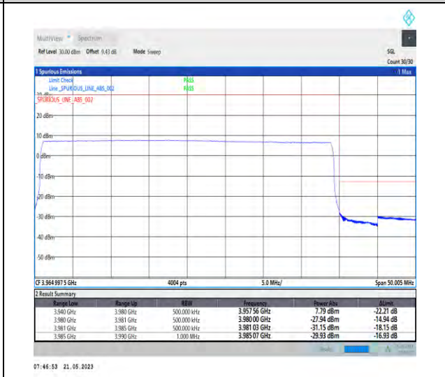
1-N77-3700-3980-PC1-30-40-H-6-CP-QPSK-Outer_Full-106@0-Ant0-1--PASS-see graph
