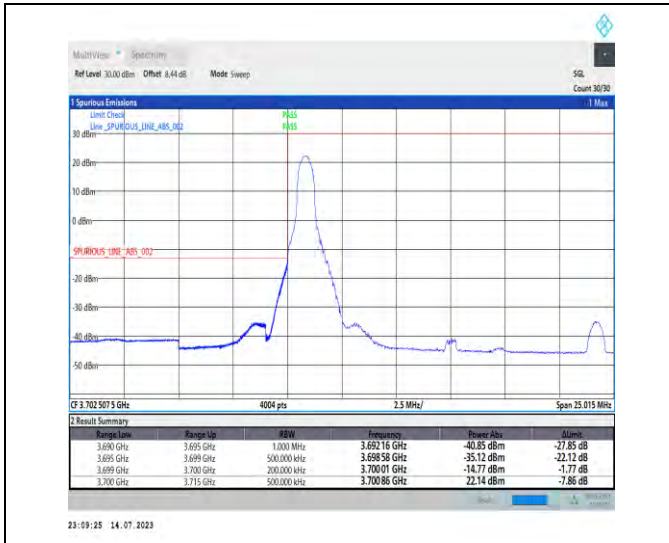
1-N77-3700-3980-PC1-30-15-L-1-DFT-PI2BPSK-Edge_e_1RB_Left-1@0-Ant0-1--PASS-see graph
