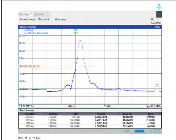
1-N77-3700-3980-PC1-30-15-L-4-CP-QPSK-Edge_1RB_Left-1@0-Ant0-1--PASS-see graph
