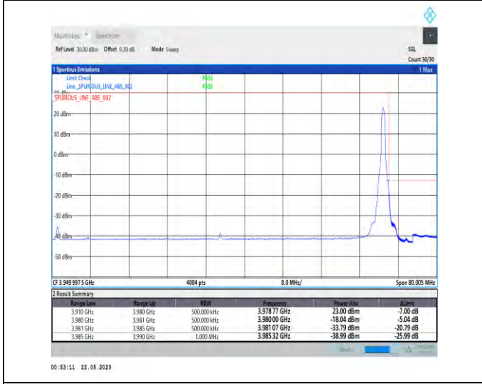
1-N77-3700-3980-PC1-30-70-H-5-CP-QPSK-Edge_1RB_Right-1@188-Ant0-1--PASS-see graph
