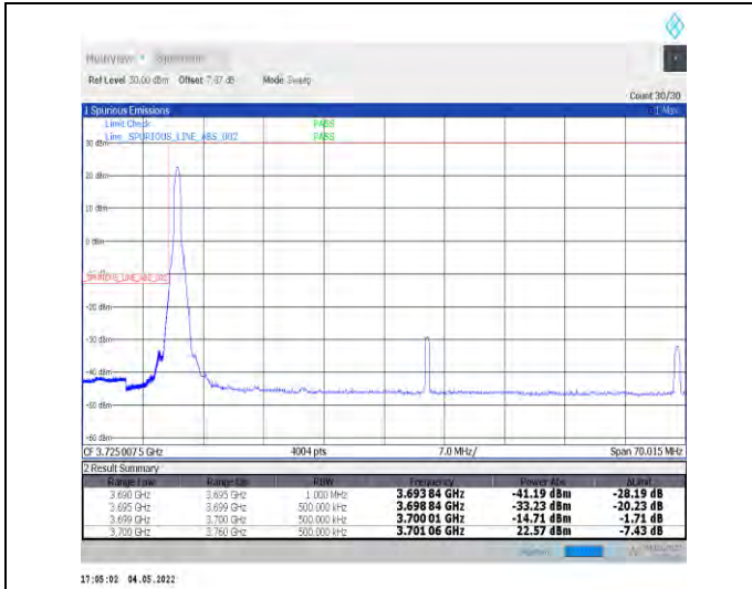
1-N77-3700-3980--30-60-L-1-DFT-PI2BPSK-Edge_1R_B_Left-1@0-Ant0-PASS-see graph
