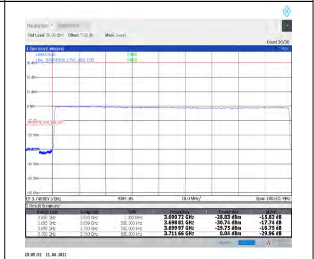
1-N77-3700-3980--30-90-L-6-CP-QPSK-Outer_Ful_I-245@0-Ant0-PASS-see graph
