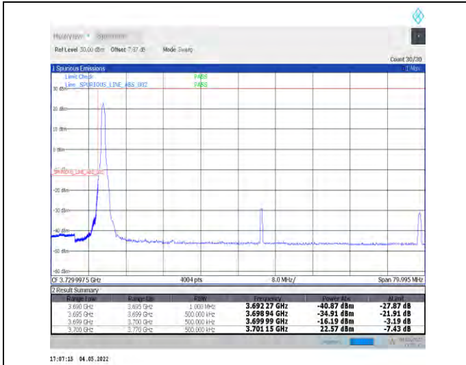
1-N77-3700-3980--30-70-L-1-DFT-PI2BPSK-Edge_1R_B_Left-1@0-Ant0-PASS-see graph
