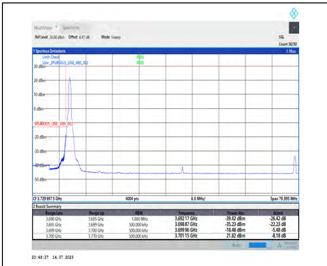
1-N77-3700-3980-PC1-30-70-L-1-DFT-PI2BPSK-Edge_1_RB_Left-1@0-Ant0-1--PASS-see graph
