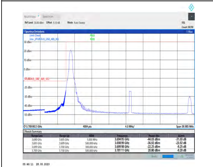
1-N77-3700-3980-PC1-30-30-L-4-CP-QPSK-Edge_1RB_Left-1@0-Ant0-1--PASS-see graph
