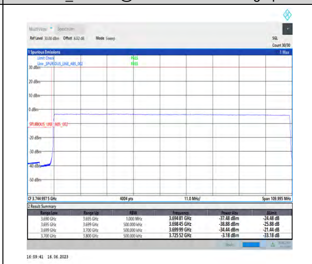
1-N77-3700-3980-PC1-30-100-L-6-CP-QPSK-Outer_Full-273@0-Ant0-1--PASS-see graph
