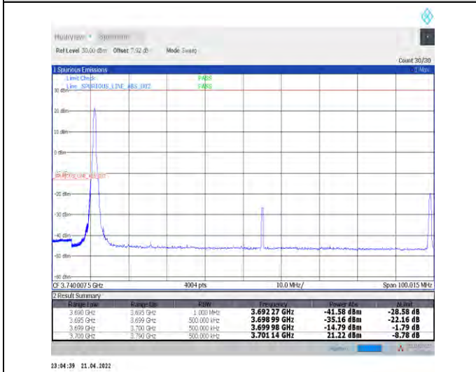
1-N77-3700-3980--30-90-L-4-CP-QPSK-Edge_1RB_L_eft-1@0-Ant0-PASS-see graph
