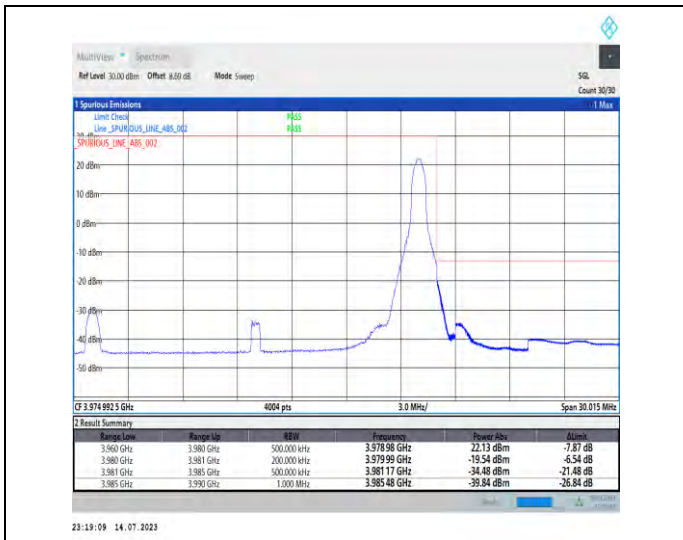
1-N77-3700-3980-PC1-30-20-H-2-DFT-PI2BPSK-Edge_1RB_Right-1@50-Ant0-1--PASS-see graph
