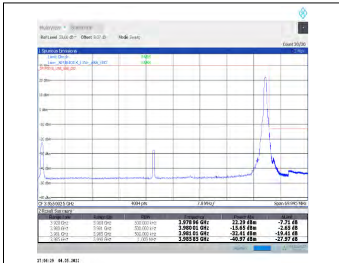
1-N77-3700-3980--30-60-H-2-DFT-PI2BPSK-Edge_1R_B_Right-1@161-Ant0-PASS-see graph
