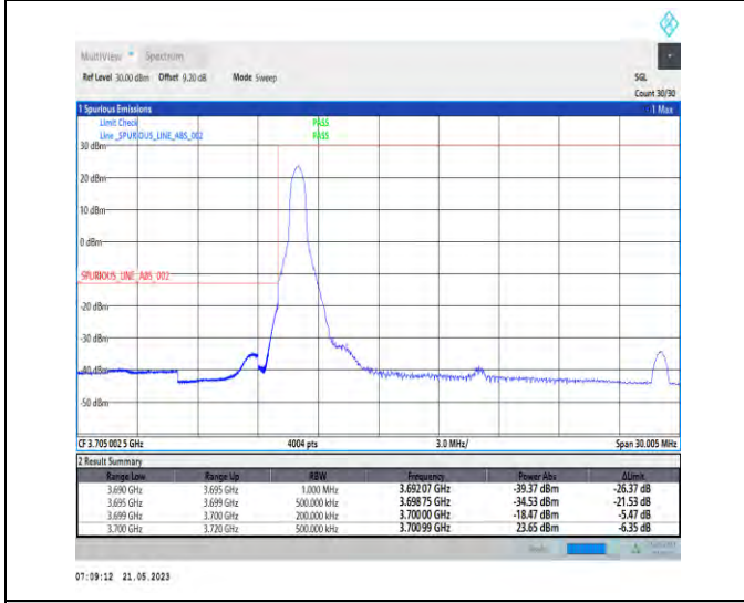
1-N77-3700-3980-PC1-30-20-L-4-CP-QPSK-Edge_1RB_Left-1@0-Ant0-1--PASS-see graph
