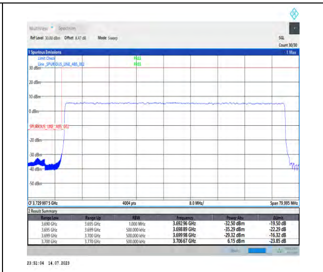
1-N77-3700-3980-PC1-30-70-L-3-DFT-PI2BPSK-Outer_Full-180@0-Ant0-1--PASS-see graph
