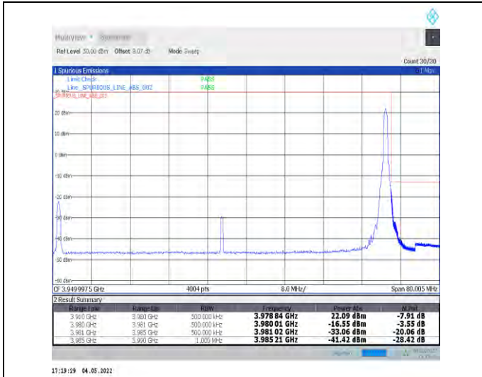
1-N77-3700-3980--30-70-H-2-DFT-PI2BPSK-Edge_1R_B_Right-1@188-Ant0-PASS-see graph
