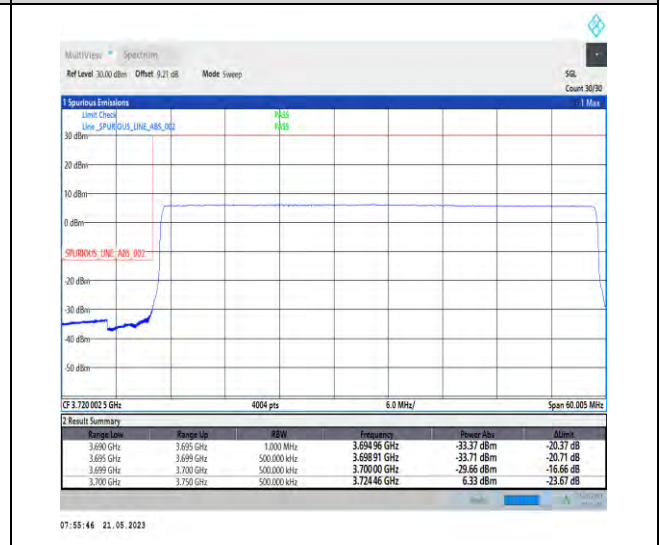
1-N77-3700-3980-PC1-30-50-L-6-CP-QPSK-Outer_Full-133@0-Ant0-1--PASS-see graph
