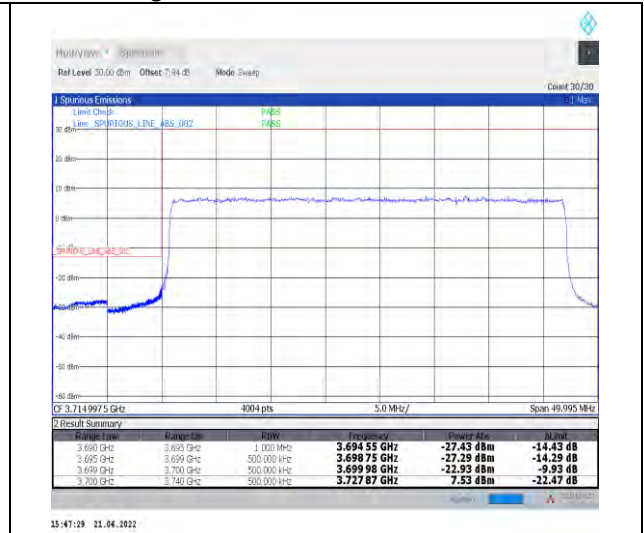
1-N77-3700-3980--30-40-L-3-DFT-PI2BPSK-Outer_Full-100@0-Ant0-PASS-see graph
