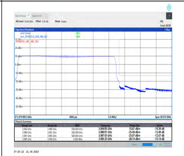
1-N77-3700-3980-PC1-30-20-H-6-CP-QPSK-Outer_Full-51@0-Ant0-1--PASS-see graph
