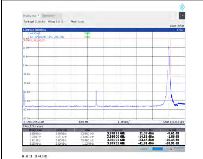
1-N77-3700-3980--30-100-H-5-CP-QPSK-Edge_1RB_Right-1@272-Ant0-PASS-see graph
