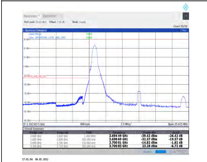
1-N77-3700-3980--30-15-L-4-CP-QPSK-Edge_1RB_L_eft-1@0-Ant0-PASS-see graph
