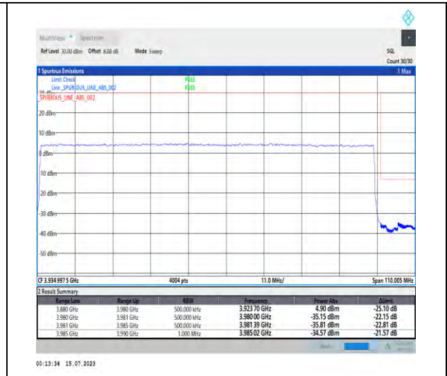
1-N77-3700-3980-PC1-30-100-H-3-DFT-PI2BPSK-Outer_Full-270@0-Ant0-1--PASS-see graph
