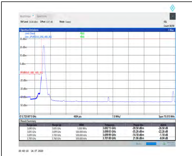
1-N77-3700-3980-PC1-30-60-L-1-DFT-PI2BPSK-Edge_1_RB_Left-1@0-Ant0-1--PASS-see graph
