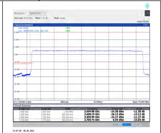
1-N77-3700-3980--30-70-L-3-DFT-PI2BPSK-Outer_Full-180@0-Ant0-PASS-see graph
