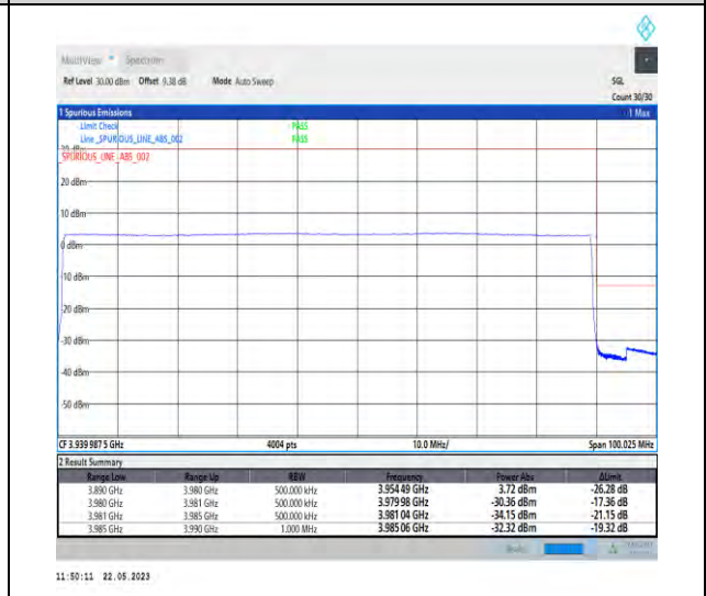
1-N77-3700-3980-PC1-30-90-H-6-CP-QPSK-Outer_Full-245@0-Ant0-1--PASS-see graph
