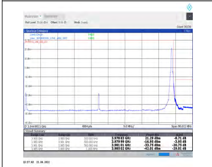
1-N77-3700-3980--30-80-H-5-CP-QPSK-Edge_1RB_Right-1@216-Ant0-PASS-see graph
