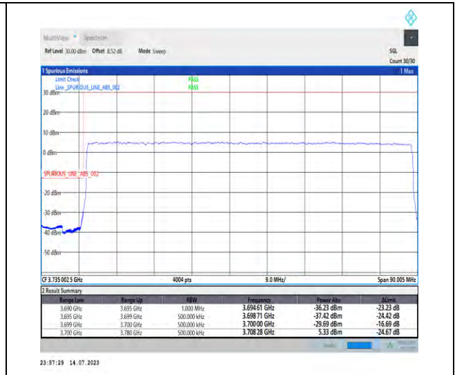
1-N77-3700-3980-PC1-30-80-L-3-DFT-PI2BPSK-Outer_Full-216@0-Ant0-1--PASS-see graph
