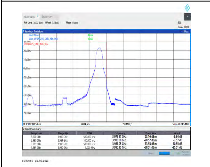
1-N77-3700-3980-PC1-30-10-H-5-CP-QPSK-Edge_1RB_Right-1@23-Ant0-1--PASS-see graph
