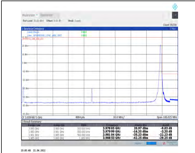
1-N77-3700-3980--30-90-H-2-DFT-PI2BPSK-Edge_1R_B_Right-1@244-Ant0-PASS-see graph
