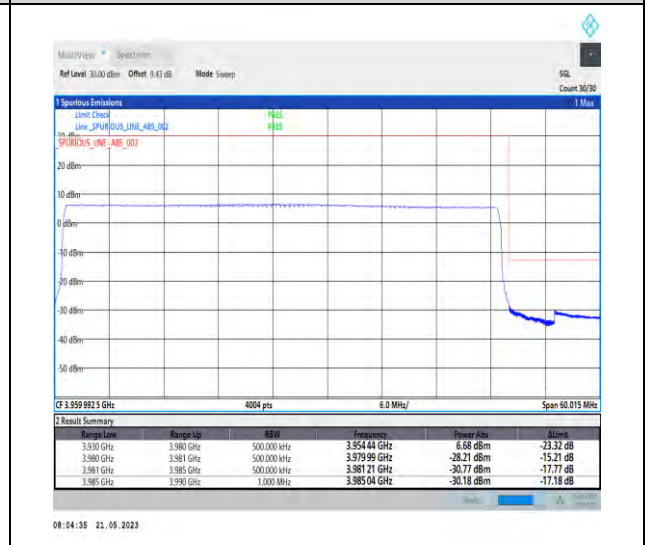
1-N77-3700-3980-PC1-30-50-H-6-CP-QPSK-Outer_Full-133@0-Ant0-1--PASS-see graph
