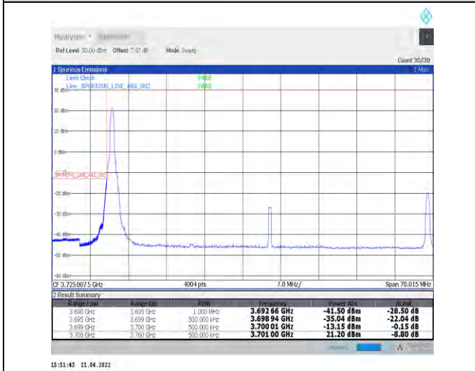
1-N77-3700-3980--30-60-L-4-CP-QPSK-Edge_1RB_L_eft-1@0-Ant0-PASS-see graph
