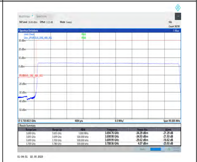
1-N77-3700-3980-PC1-30-80-L-6-CP-QPSK-Outer_Full-217@0-Ant0-1--PASS-see graph
