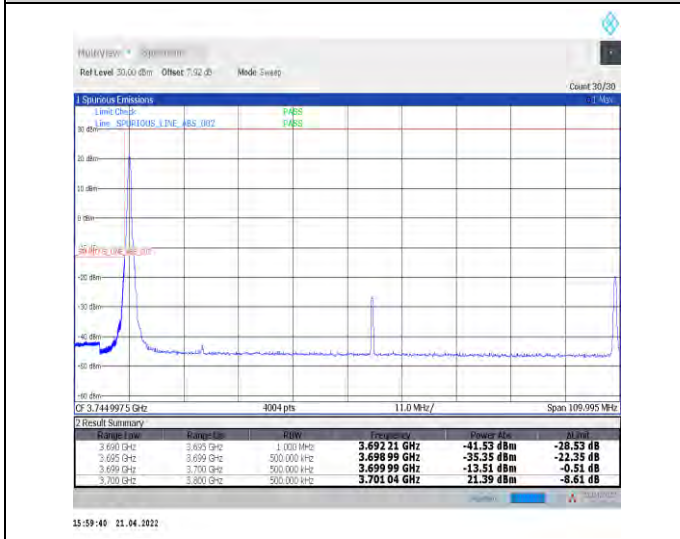
1-N77-3700-3980--30-100-L-4-CP-QPSK-Edge_1RB_Left-1@0-Ant0-PASS-see graph
