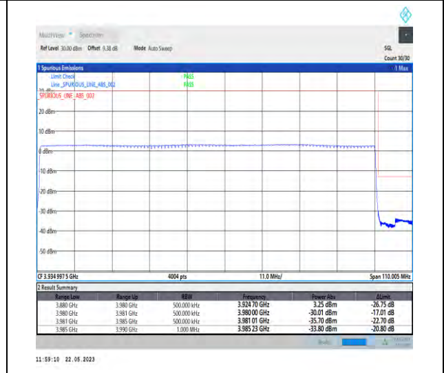
1-N77-3700-3980-PC1-30-100-H-6-CP-QPSK-Outer_Full-273@0-Ant0-1--PASS-see graph
