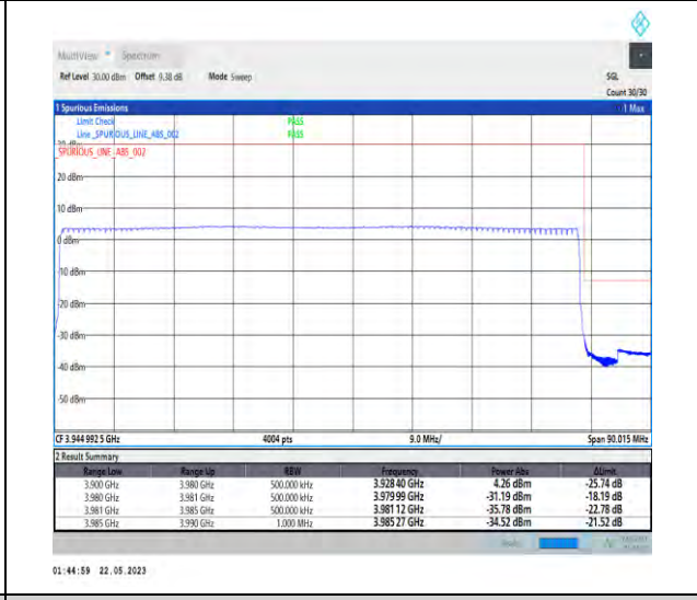
1-N77-3700-3980-PC1-30-80-H-6-CP-QPSK-Outer_Full-217@0-Ant0-1--PASS-see graph
