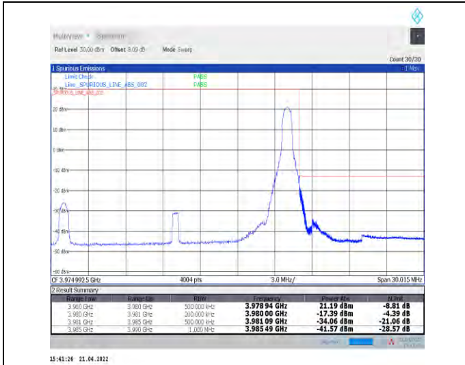
1-N77-3700-3980--30-20-H-2-DFT-PI2BPSK-Edge_1R_B_Right-1@50-Ant0-PASS-see graph
