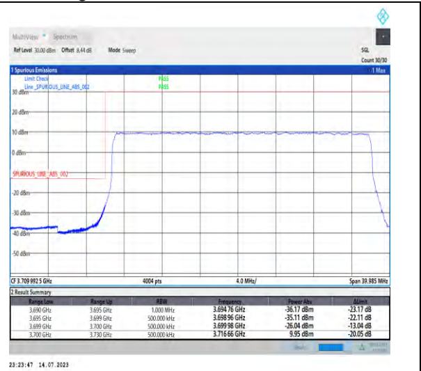
1-N77-3700-3980-PC1-30-30-L-3-DFT-PI2BPSK-Outer_Full-75@0-Ant0-1--PASS-see graph
