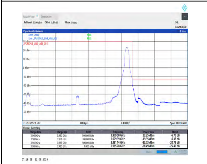
1-N77-3700-3980-PC1-30-20-H-5-CP-QPSK-Edge_1RB_Right-1@50-Ant0-1--PASS-see graph
