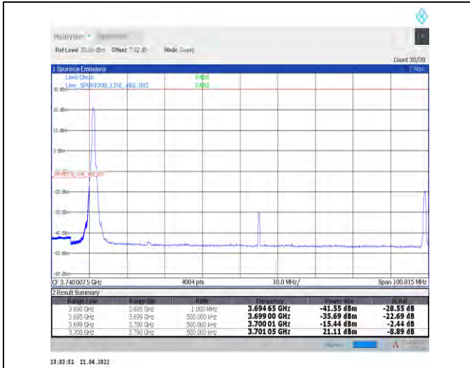
1-N77-3700-3980--30-90-L-1-DFT-PI2BPSK-Edge_1R_B_Left-1@0-Ant0-PASS-see graph
