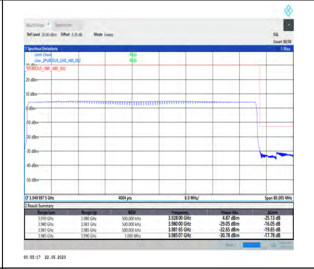
1-N77-3700-3980-PC1-30-70-H-6-CP-QPSK-Outer_Full-189@0-Ant0-1--PASS-see graph
