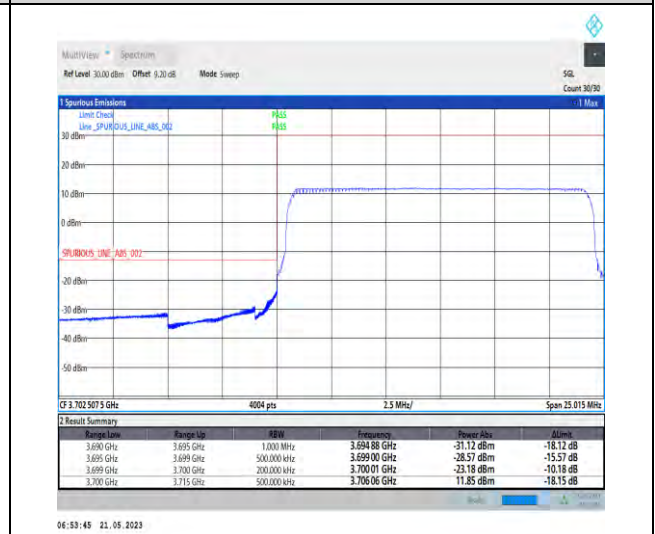
1-N77-3700-3980-PC1-30-15-L-6-CP-QPSK-Outer_Full-38@0-Ant0-1--PASS-see graph
