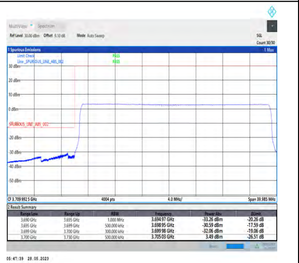
1-N77-3700-3980-PC1-30-30-L-6-CP-QPSK-Outer_Full-78@0-Ant0-1--PASS-see graph
