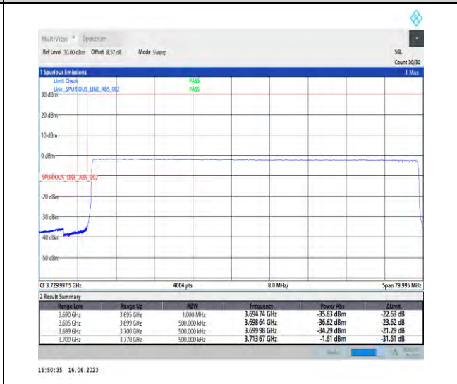
1-N77-3700-3980-PC1-30-70-L-6-CP-QPSK-Outer_Full-189@0-Ant0-1--PASS-see graph
