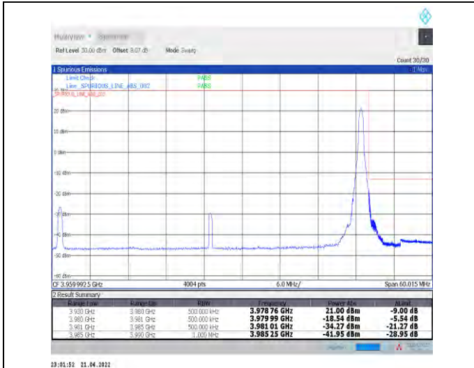
1-N77-3700-3980--30-50-H-2-DFT-PI2BPSK-Edge_1R_B_Right-1@132-Ant0-PASS-see graph
