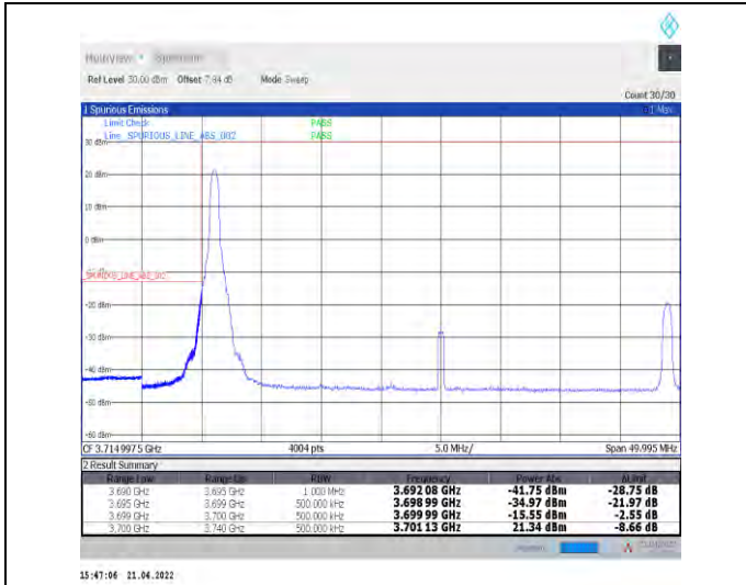
1-N77-3700-3980--30-40-L-1-DFT-PI2BPSK-Edge_1R_B_Left-1@0-Ant0-PASS-see graph
