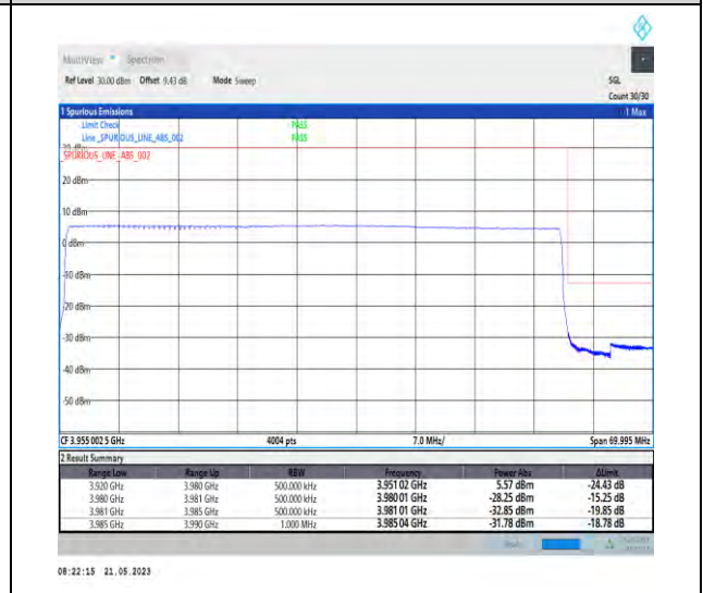
1-N77-3700-3980-PC1-30-60-H-6-CP-QPSK-Outer_Full-162@0-Ant0-1--PASS-see graph
