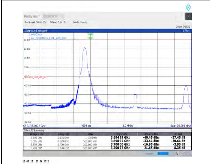
1-N77-3700-3980--30-20-L-4-CP-QPSK-Edge_1RB_L_eft-1@0-Ant0-PASS-see graph
