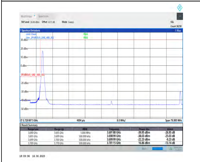
1-N77-3700-3980-PC1-30-70-L-4-CP-QPSK-Edge_1_RB_Left-1@0-Ant0-1--PASS-see graph
