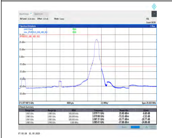
1-N77-3700-3980-PC1-30-15-H-5-CP-QPSK-Edge_1RB_Right-1@37-Ant0-1--PASS-see graph
