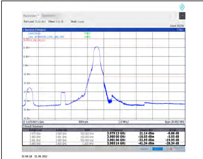
1-N77-3700-3980--30-10-H-2-DFT-PI2BPSK-Edge_1R_B_Right-1@23-Ant0-PASS-see graph
