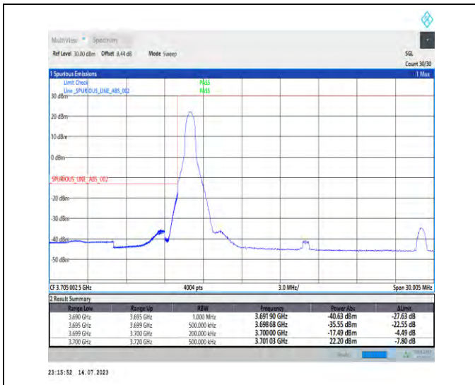
1-N77-3700-3980-PC1-30-20-L-1-DFT-PI2BPSK-Edge_e_1RB_Left-1@0-Ant0-1--PASS-see graph
