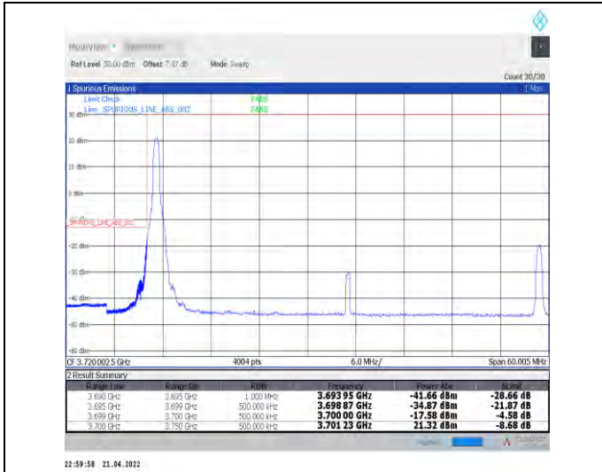
1-N77-3700-3980--30-50-L-1-DFT-PI2BPSK-Edge_1R_B_Left-1@0-Ant0-PASS-see graph
