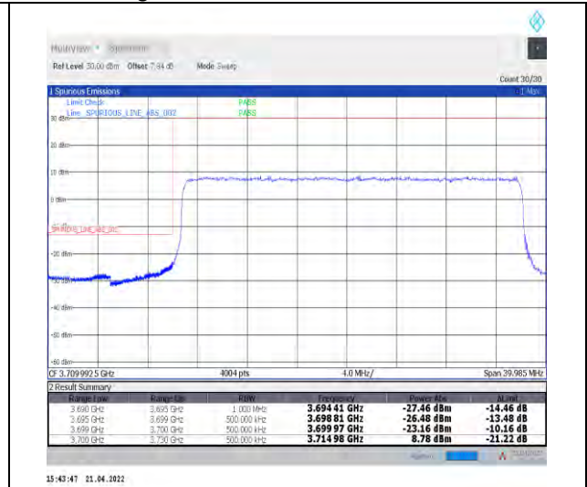
1-N77-3700-3980--30-30-L-3-DFT-PI2BPSK-Outer_Full-75@0-Ant0-PASS-see graph
