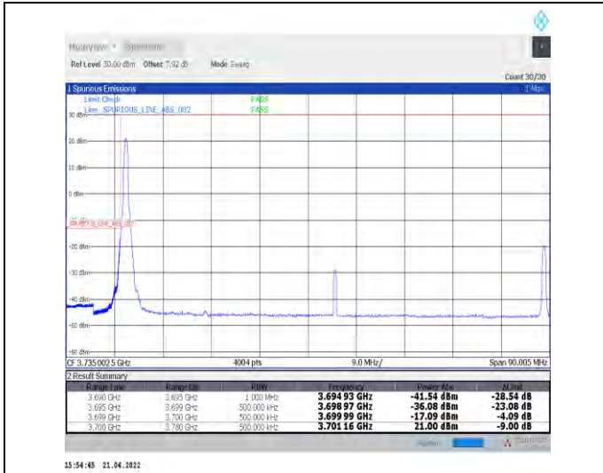
1-N77-3700-3980--30-80-L-1-DFT-PI2BPSK-Edge_1R_B_Left-1@0-Ant0-PASS-see graph
