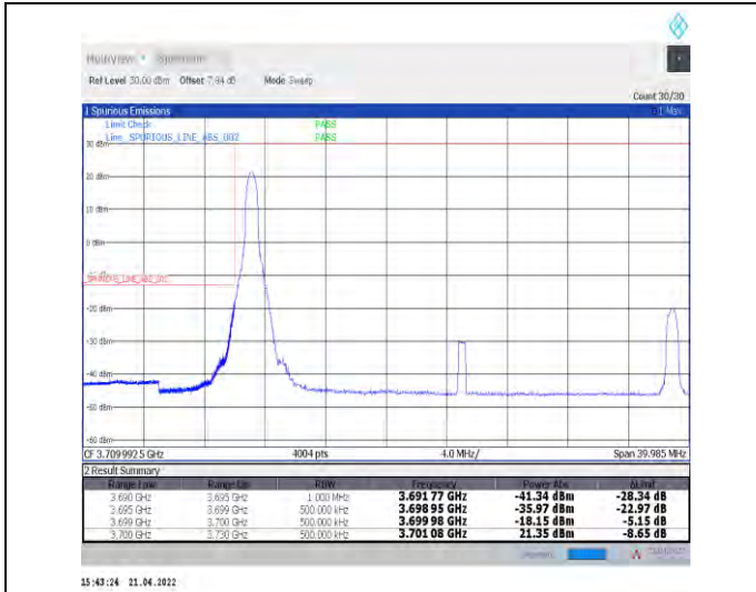
1-N77-3700-3980--30-30-L-1-DFT-PI2BPSK-Edge_1R_B_Left-1@0-Ant0-PASS-see graph
