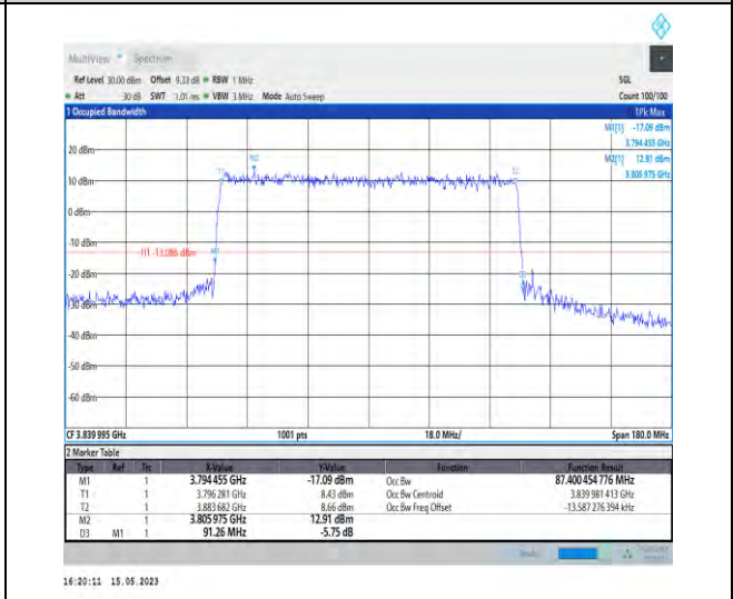
1-N77-3700-3980-PC1-30-90-M-8-CP-64QAM-Outer_Full-245@0-Ant0-87.4-91.260-≤90-PASS
