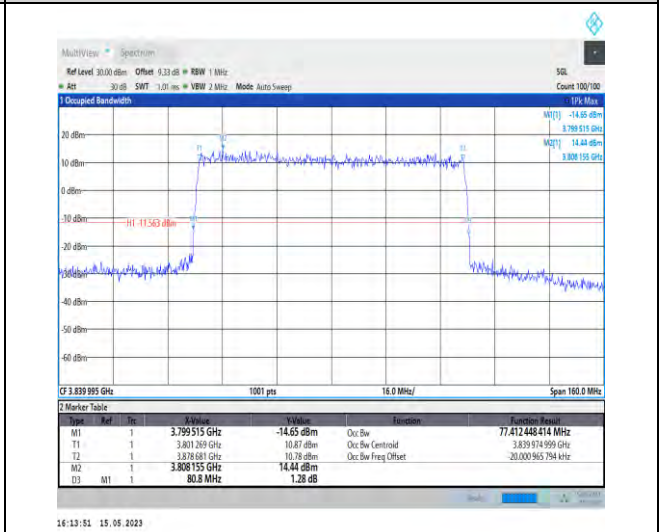
1-N77-3700-3980-PC1-30-80-M-7-CP-16QAM-Outer_Full-217@0-Ant0-77.412-80.800-≤80-PASS
