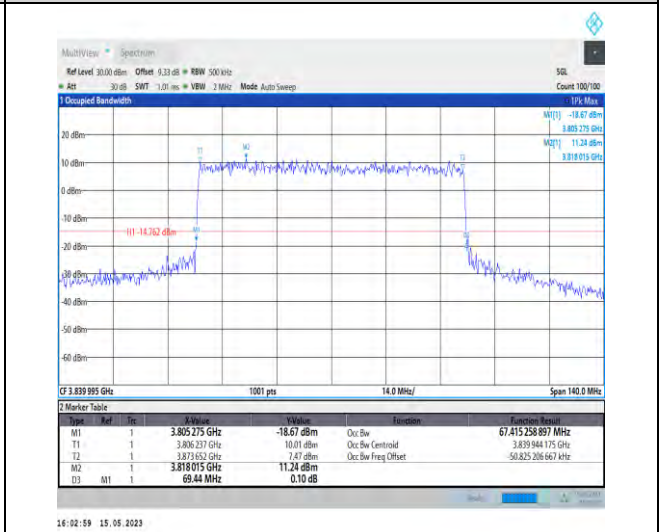
1-N77-3700-3980-PC1-30-70-M-6-CP-QPSK-Outer_Full-189@0-Ant0-67.415-69.440-≤70-PASS
