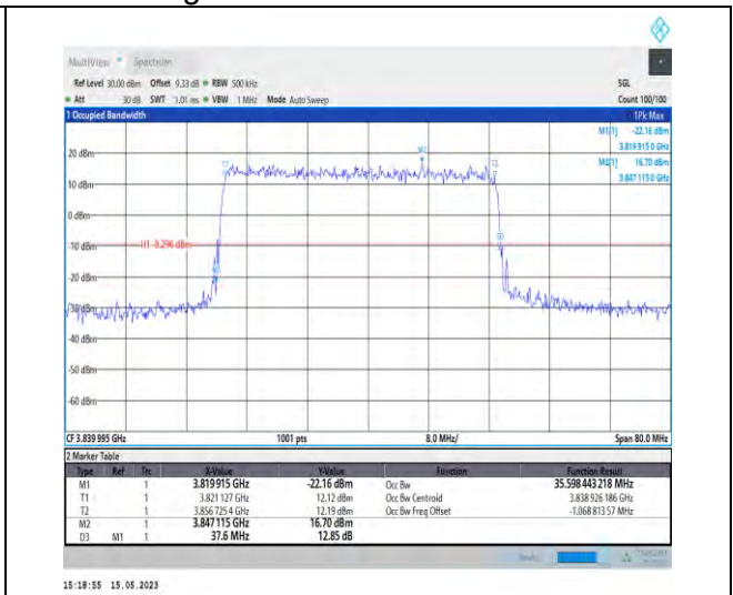
1-N77-3700-3980-PC1-30-40-M-1-DFT-QPSK-Outer_Full-100@0-Ant0-35.598-37.600-≤40-PASS
