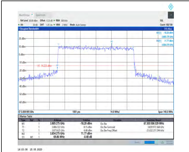
1-N77-3700-3980-PC1-30-70-M-7-CP-16QAM-Outer_Full-189@0-Ant0-67.303-69.860-≤70-PASS
