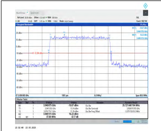
1-N77-3700-3980-PC1-30-40-H-3-DFT-16QAM-Outer_Full-100@0-Ant0-35.722-37.840-≤40-PASS
