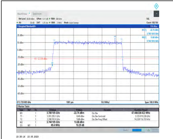
1-N77-3700-3980-PC1-30-50-L-6-CP-QPSK-Outer_Full-133@0-Ant0-47.448-49.400-≤50-PASS
