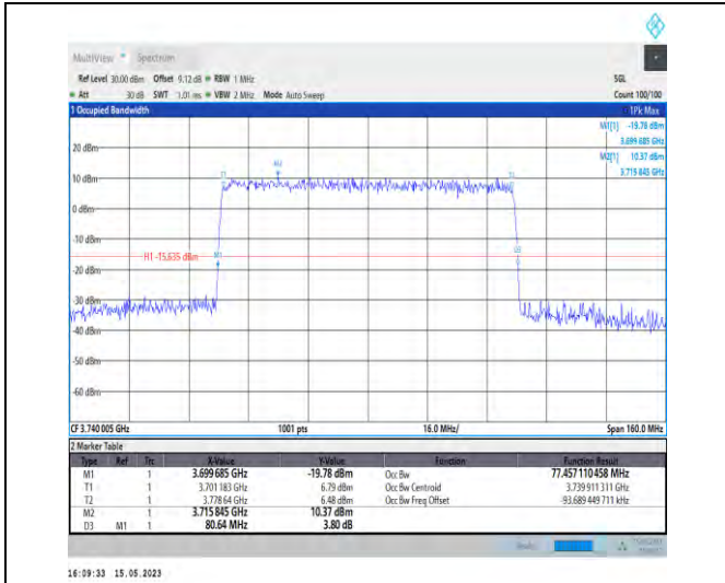
1-N77-3700-3980-PC1-30-80-L-9-CP-256QAM-Outer_Full-217@0-Ant0-77.457-80.640-≤80-PASS
