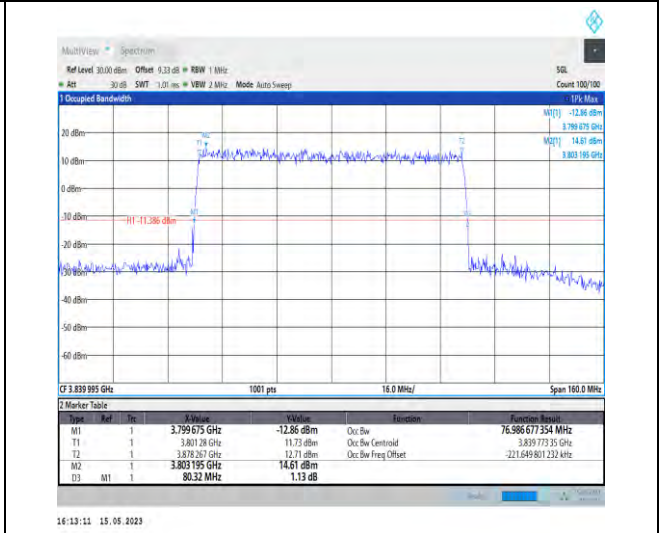
1-N77-3700-3980-PC1-30-80-M-3-DFT-16QAM-Outer_Full-216@0-Ant0-76.987-80.320-≤80-PASS
