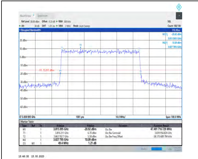
1-N77-3700-3980-PC1-30-50-M-9-CP-256QAM-Outer_Full-133@0-Ant0-47.492-49.400-≤50-PASS
