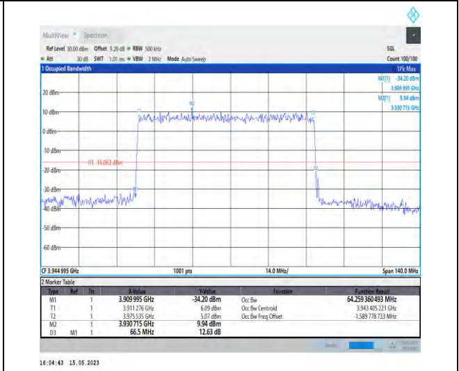
1-N77-3700-3980-PC1-30-70-H-5-DFT-256QAM-Out er_Full-180@0-Ant0-64.259-66.500-≤70-PASS
