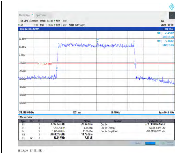
1-N77-3700-3980-PC1-30-80-M-4-DFT-64QAM-Outer_Full-216@0-Ant0-77.173-80.640-≤80-PASS
