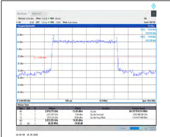
1-N77-3700-3980-PC1-30-70-H-2-DFT-PI2BPSK-Out er_Full-180@0-Ant0-64.148-66.360-≤70-PASS
