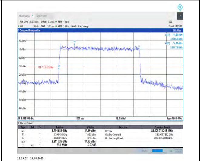
1-N77-3700-3980-PC1-30-90-M-4-DFT-64QAM-Outer_Full-240@0-Ant0-85.403-89.100-≤90-PASS
