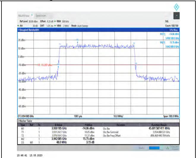
1-N77-3700-3980-PC1-30-50-H-1-DFT-QPSK-Outer_Full-128@0-Ant0-45.692-48.000-≤50-PASS
