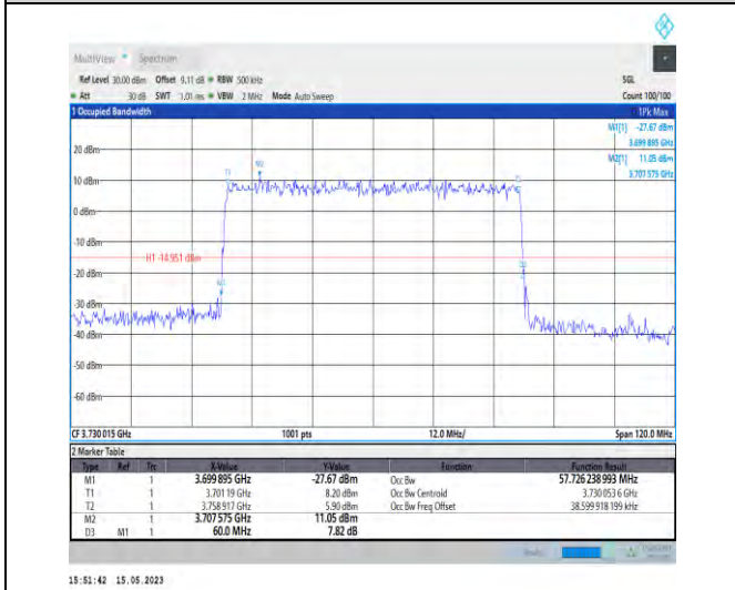
1-N77-3700-3980-PC1-30-60-L-5-DFT-256QAM-Outer_Full-162@0-Ant0-57.726-60.000-≤60-PASS
