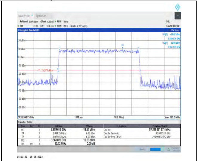
1-N77-3700-3980-PC1-30-90-H-9-CP-256QAM-Outer_Full-245@0-Ant0-87.398-90.720-<=90-PASS
