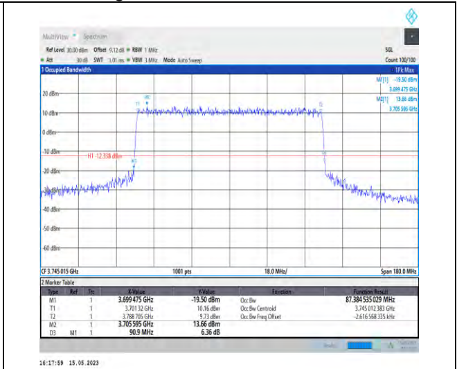
1-N77-3700-3980-PC1-30-90-L-7-CP-16QAM-Outer_Full-245@0-Ant0-87.385-90.900-≤90-PASS
