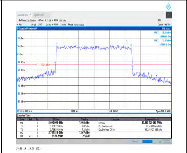
1-N77-3700-3980-PC1-30-70-L-7-CP-16QAM-Outer_Full-189@0-Ant0-67.365-69.860-≤70-PASS
