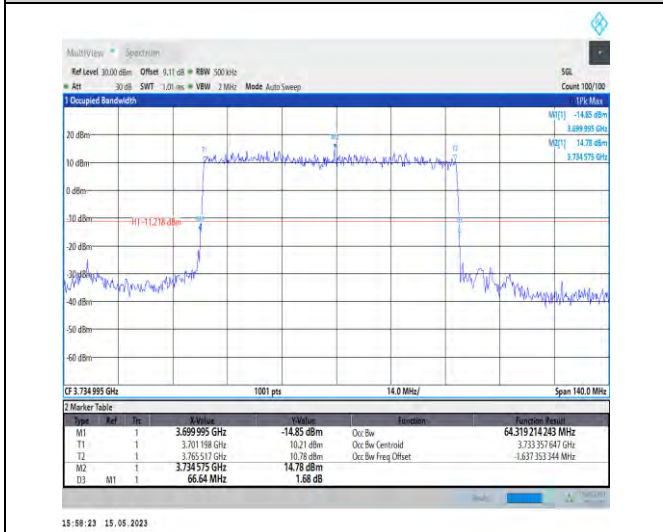
1-N77-3700-3980-PC1-30-70-L-2-DFT-PI2BPSK-Outer_Full-180@0-Ant0-64.319-66.640-≤70-PASS
