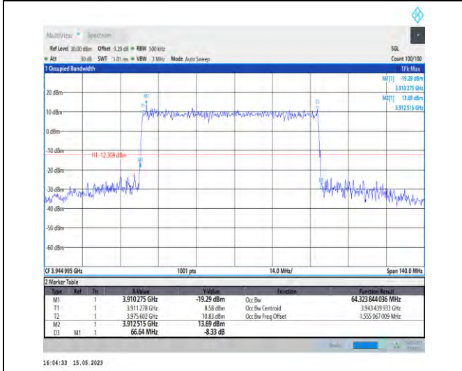
1-N77-3700-3980-PC1-30-70-H-4-DFT-64QAM-Out er_Full-180@0-Ant0-64.324-66.640-≤70-PASS
