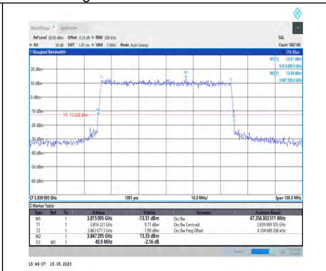
1-N77-3700-3980-PC1-30-50-M-6-CP-QPSK-Outer_Full-133@0-Ant0-47.356-49.900-≤50-PASS
