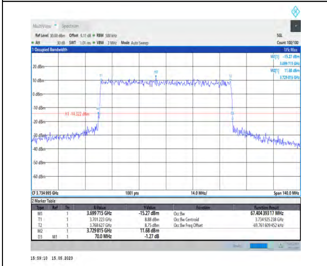
1-N77-3700-3980-PC1-30-70-L-6-CP-QPSK-Outer_Full-189@0-Ant0-67.404-70.000-≤70-PASS
