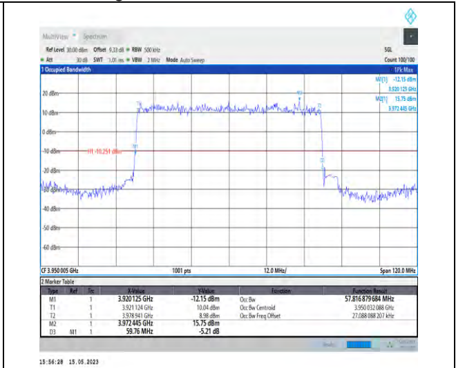
1-N77-3700-3980-PC1-30-60-H-2-DFT-PI2BPSK-Outer_Full-162@0-Ant0-57.817-59.760-≤60-PASS
