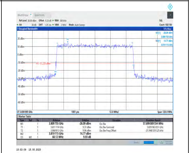
1-N77-3700-3980-PC1-30-60-M-1-DFT-QPSK-Outer_Full-162@0-Ant0-57.699-60.120-≤60-PASS
