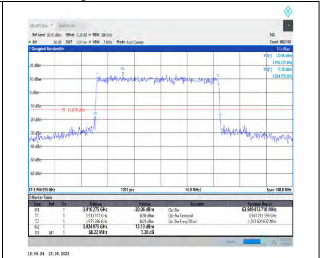
1-N77-3700-3980-PC1-30-70-H-3-DFT-16QAM-Out er_Full-180@0-Ant0-63.949-66.220-≤70-PASS
