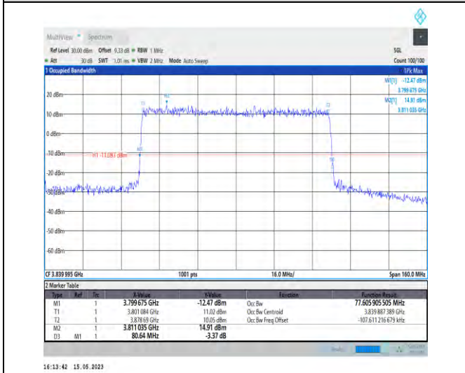
1-N77-3700-3980-PC1-30-80-M-6-CP-QPSK-Outer_Full-217@0-Ant0-77.606-80.640-≤80-PASS
