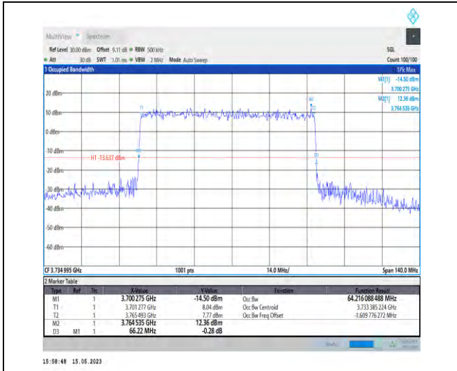
1-N77-3700-3980-PC1-30-70-L-4-DFT-64QAM-Outer_Full-180@0-Ant0-64.216-66.220-≤70-PASS
