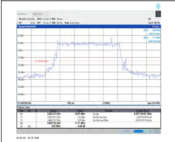
1-N77-3700-3980-PC1-30-10-M-6-CP-QPSK-Outer_Full-24@0-Ant0-8.597-9.920-≤10-PASS
