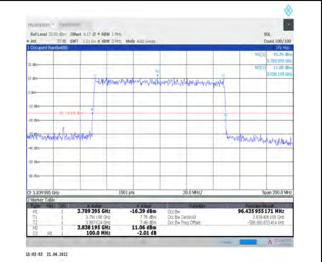
1-N77-3700-3980--30-100-M-5-DFT-256QAM-Outer_Full-270@0-Ant0-96.436-100.000-≤100-PASS
