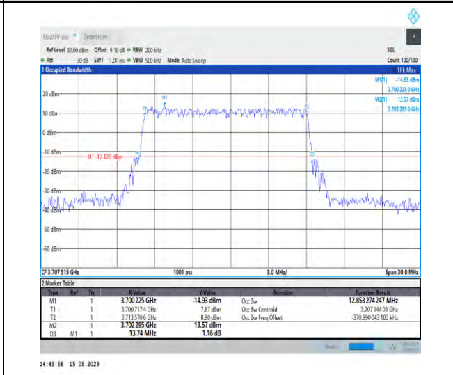
1-N77-3700-3980-PC1-30-15-L-5-DFT-256QAM-Outer_Full-36@0-Ant0-12.853-13.740-≤15-PASS
