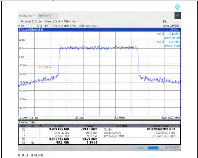
1-N77-3700-3980--30-90-H-1-DFT-QPSK-Outer_Full-240@0-Ant0-85.82-89.100-<math>\leq 90</math>-PASS
