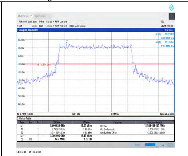
1-N77-3700-3980-PC1-30-15-L-7-CP-16QAM-Outer_Full-38@0-Ant0-13.585-14.700-≤15-PASS
