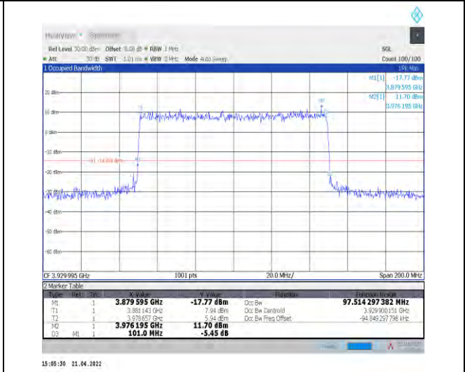
1-N77-3700-3980--30-100-H-8-CP-64QAM-Outer_Full-273@0-Ant0-97.514-101.000-<=100-PASS
