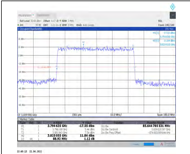
1-N77-3700-3980--30-90-M-5-DFT-256QAM-Outer_Full-240@0-Ant0-85.645-88.920-≤90-PASS
