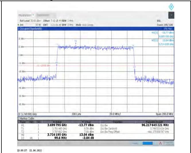
1-N77-3700-3980--30-100-L-4-DFT-64QAM-Outer_Full-270@0-Ant0-96.218-99.600-≤100-PASS
