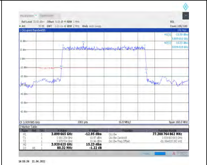
1-N77-3700-3980--30-80-H-2-DFT-PI2BPSK-Outer_Full Full-216@0-Ant0-77.301-80.320-≤80-PASS
