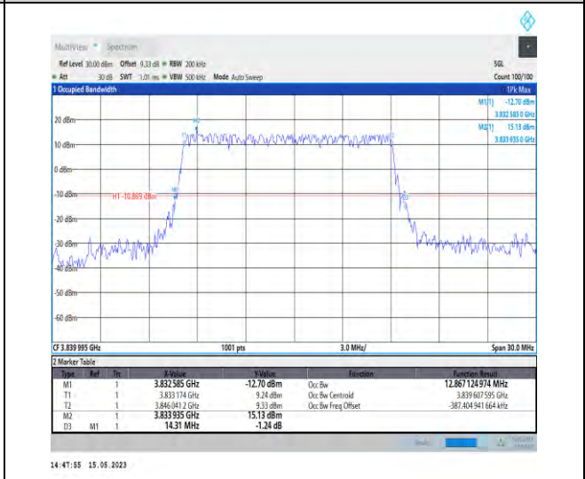
1-N77-3700-3980-PC1-30-15-M-4-DFT-64QAM-Outer_Full-36@0-Ant0-12.867-14.310-≤15-PASS
