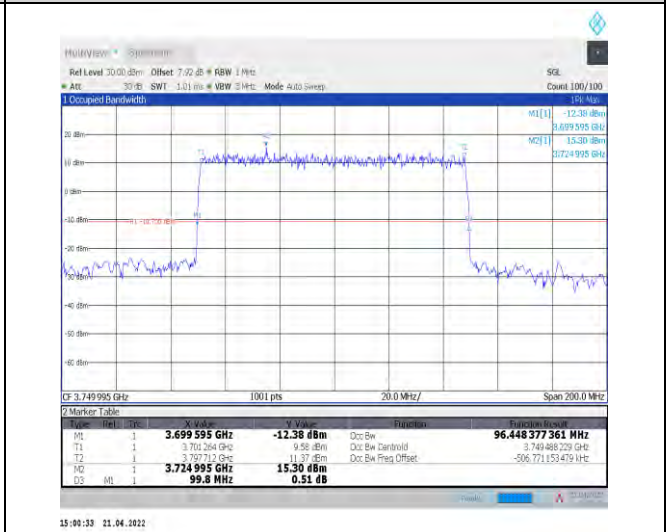
1-N77-3700-3980--30-100-L-2-DFT-Pl2BPSK-Outer_Fu Full-270@0-Ant0-96.448-99.800-≤100-PASS
