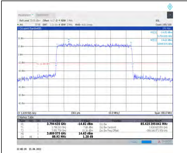
1-N77-3700-3980--30-90-M-1-DFT-QPSK-Outer_Full -240@0-Ant0-85.425-88.920-≤90-PASS
