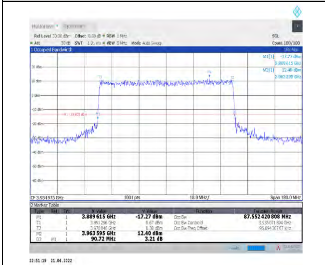
1-N77-3700-3980--30-90-H-6-CP-QPSK-Outer_Full-245@0-Ant0-87.552-90.720-<=90-PASS
