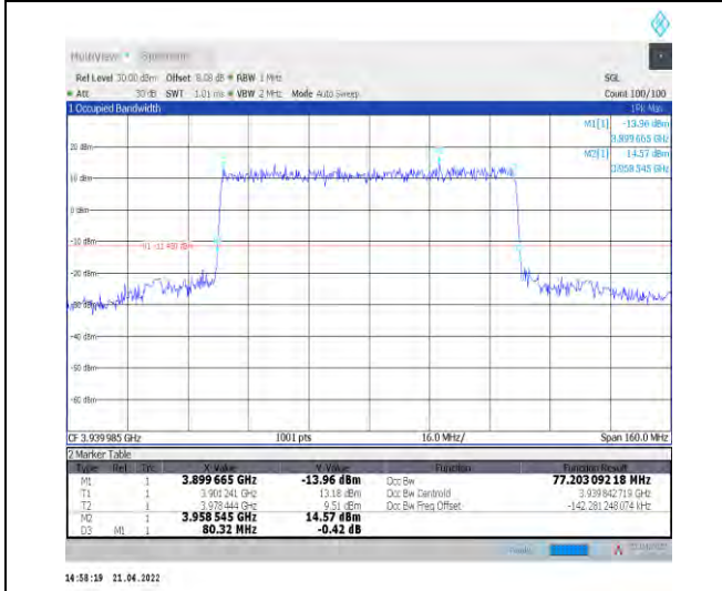
1-N77-3700-3980--30-80-H-1-DFT-QPSK-Outer_Full -216@0-Ant0-77.203-80.320-≤80-PASS
