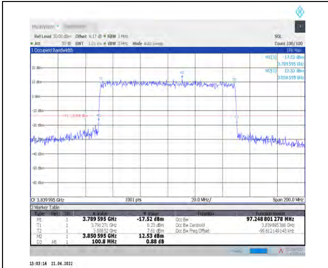
1-N77-3700-3980--30-100-M-6-CP-QPSK-Outer_Full-273@0-Ant0-97.249-100.800-≤100-PASS
