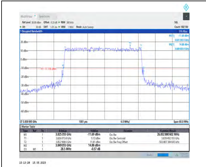
1-N77-3700-3980-PC1-30-30-M-3-DFT-16QAM-Outer_Full-75@0-Ant0-26.833-28.500-≤30-PASS
