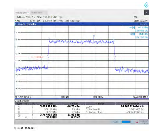
1-N77-3700-3980--30-100-L-5-DFT-256QAM-Outer_Full-270@0-Ant0-96.269-99.800-≤100-PASS
