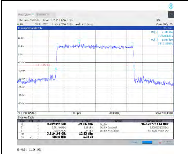
1-N77-3700-3980--30-100-M-4-DFT-64QAM-Outer_Full-270@0-Ant0-96.054-100.000-≤100-PASS
