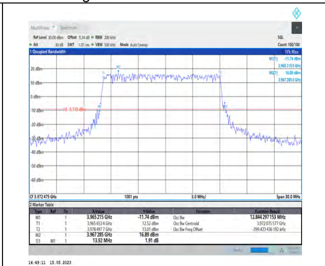
1-N77-3700-3980-PC1-30-15-H-1-DFT-QPSK-Outer_Full-36@0-Ant0-12.844-13.920-≤15-PASS
