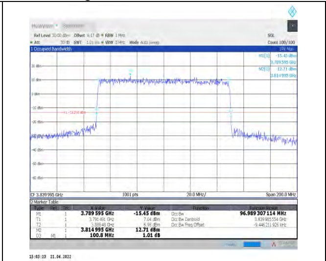
1-N77-3700-3980--30-100-M-7-CP-16QAM-Outer_Full-273@0-Ant0-96.989-100.800-≤100-PASS
