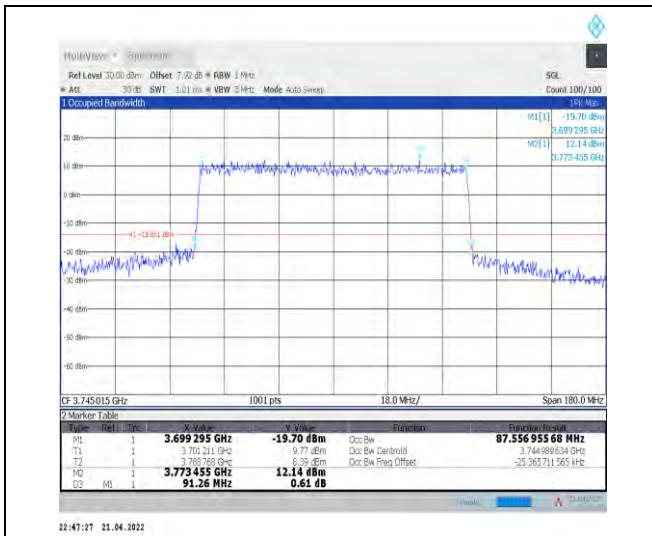
1-N77-3700-3980--30-90-L-6-CP-QPSK-Outer_Full-245@0-Ant0-87.557-91.260-<math>\leq 90</math>-PASS
