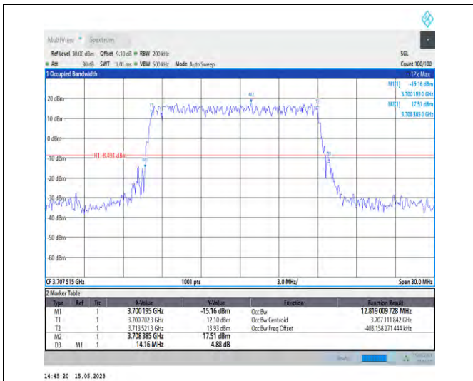
1-N77-3700-3980-PC1-30-15-L-2-DFT-PI2BPSK-Out er_Full-36@0-Ant0-12.819-14.160-≤15-PASS
