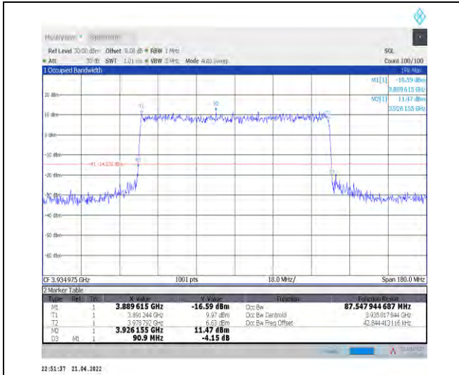
1-N77-3700-3980--30-90-H-8-CP-64QAM-Outer_Full -245@0-Ant0-87.548-90.900-≤90-PASS
