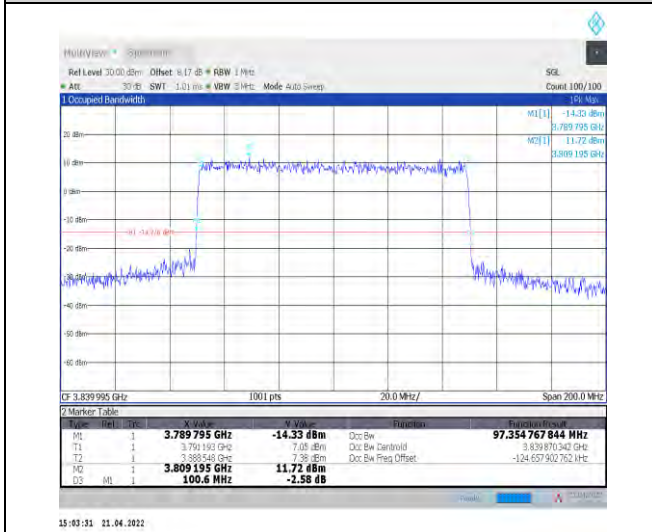
1-N77-3700-3980--30-100-M-8-CP-64QAM-Outer_Full-273@0-Ant0-97.355-100.600-≤100-PASS
