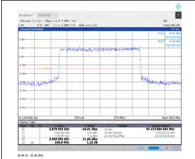
1-N77-3700-3980--30-100-H-7-CP-16QAM-Outer_Full-273@0-Ant0-97.474-100.800-<=100-PASS
