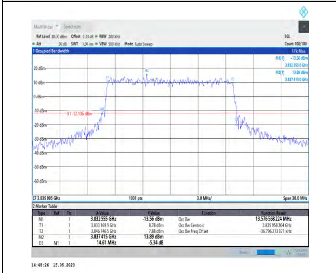
1-N77-3700-3980-PC1-30-15-M-7-CP-16QAM-Outer_Full-38@0-Ant0-13.577-14.610-≤15-PASS
