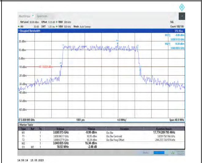
1-N77-3700-3980-PC1-30-20-M-1-DFT-QPSK-Outer_Full-50@0-Ant0-17.774-18.920-≤20-PASS
