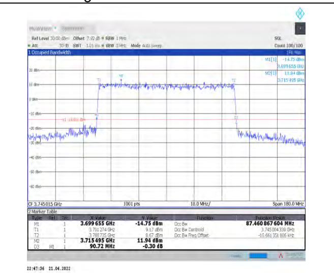
1-N77-3700-3980--30-90-L-7-CP-16QAM-Outer_Full-245@0-Ant0-87.461-90.720-<math>\leq 90</math>-PASS
