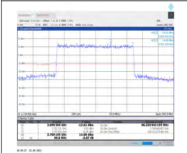
1-N77-3700-3980--30-100-L-1-DFT-QPSK-Outer_Fu ll-270@0-Ant0-96.336-99.800-≤100-PASS
