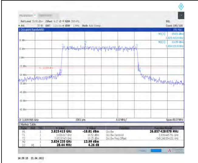
1-N77-3700-3980--30-30-M-1-DFT-QPSK-Outer_Full -75@0-Ant0-26.857-28.440-<30-PASS
