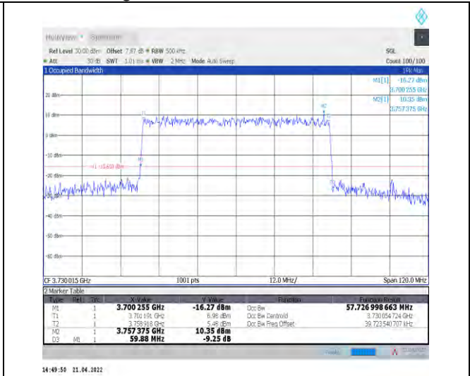
1-N77-3700-3980--30-60-L-8-CP-64QAM-Outer_Full 162@0-Ant0-57.727-59.880-≤60-PASS
