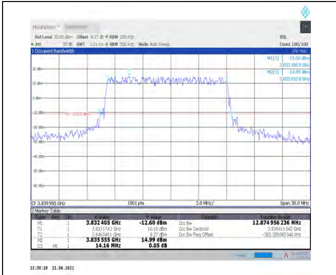
1-N77-3700-3980--30-15-M-1-DFT-QPSK-Outer_Full -36@0-Ant0-12.875-14.160-≤15-PASS
