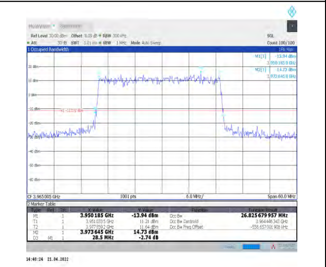
1-N77-3700-3980--30-30-H-1-DFT-QPSK-Outer_Full -75@0-Ant0-26.826-28.500-≤30-PASS
