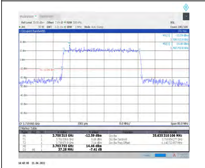
1-N77-3700-3980--30-40-L-3-DFT-16QAM-Outer_Full -100@0-Ant0-35.643-37.280-≤40-PASS
