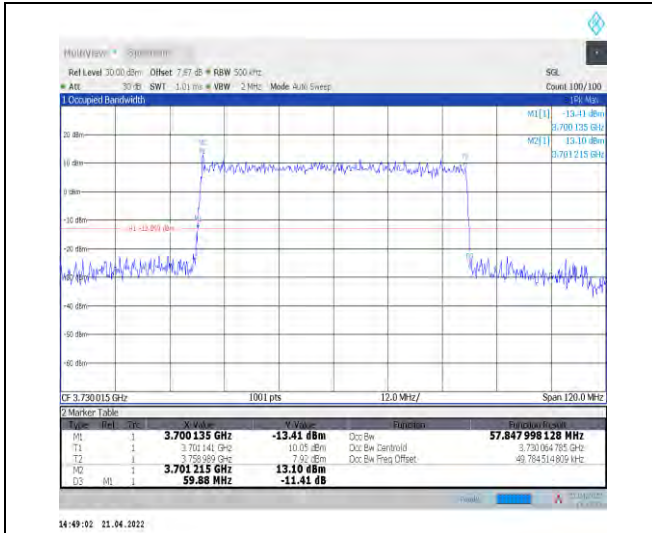
1-N77-3700-3980--30-60-L-3-DFT-16QAM-Outer_Fu I1-162@0-Ant0-57.848-59.880-≤60-PASS
