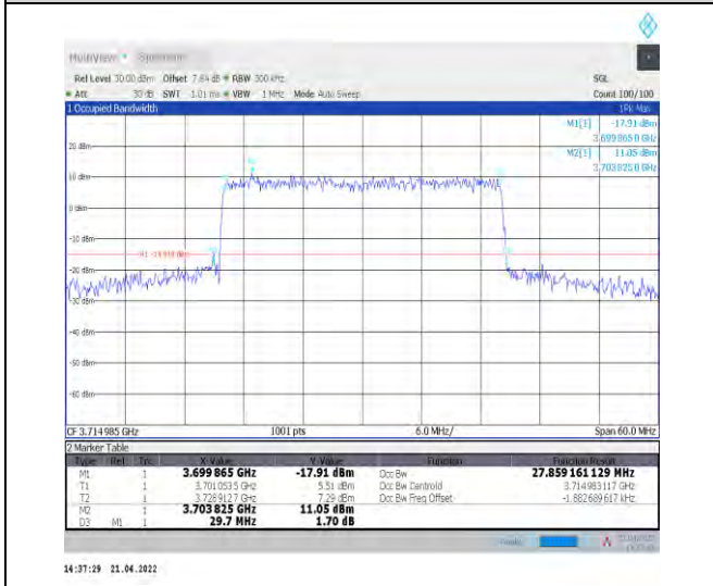
1-N77-3700-3980--30-30-L-6-CP-QPSK-Outer_Full-78@0-Ant0-27.859-29.700-≤30-PASS
