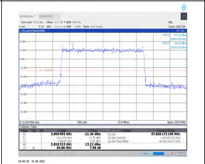
1-N77-3700-3980--30-60-M-1-DFT-QPSK-Outer_Full -162@0-Ant0-57.836-59.880-≤60-PASS
