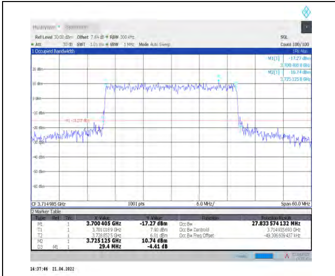
1-N77-3700-3980--30-30-L-8-CP-64QAM-Outer_Full -78@0-Ant0-27.833-29.400-<30-PASS
