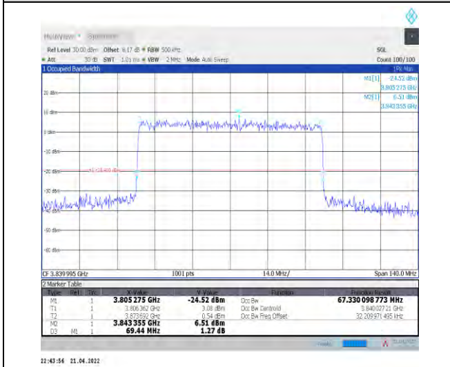
1-N77-3700-3980--30-70-M-9-CP-256QAM-Outer_Full ull-189@0-Ant0-67.33-69.440-≤70-PASS
