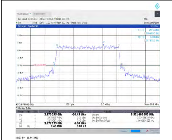
1-N77-3700-3980--30-10-H-9-CP-256QAM-Outer_F ull-24@0-Ant0-8.571-9.460-≤10-PASS
