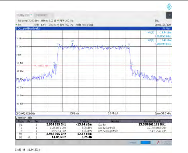
1-N77-3700-3980--30-15-H-7-CP-16QAM-Outer_Full-38@0-Ant0-13.589-14.850-≤15-PASS
