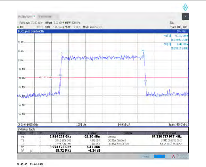
1-N77-3700-3980--30-70-H-9-CP-256QAM-Outer_Fu ll-189@0-Ant0-67.331-69.720-<=70-PASS
