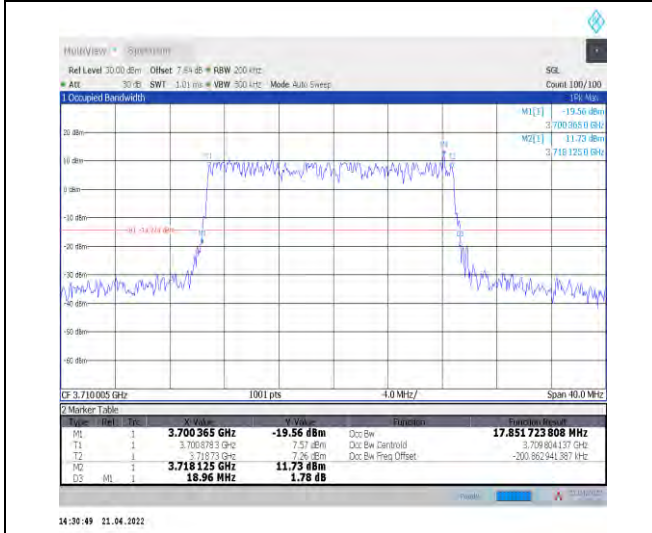
1-N77-3700-3980--30-20-L-5-DFT-256QAM-Outer_Fu ll-50@0-Ant0-17.852-18.960-<math>\leq 20</math>-PASS
