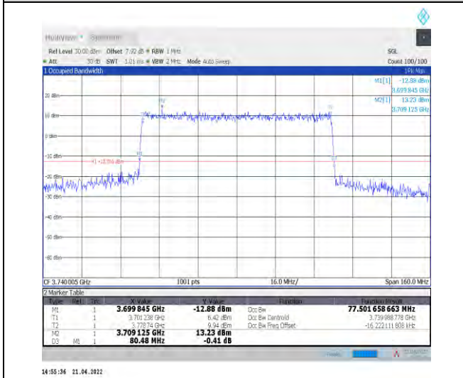
1-N77-3700-3980--30-80-L-7-CP-16QAM-Outer_Full-217@0-Ant0-77.502-80.480-<math>\leq 80</math>-PASS
