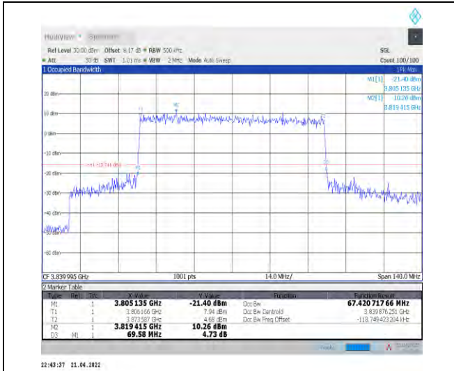
1-N77-3700-3980--30-70-M-7-CP-16QAM-Outer_Full I-189@0-Ant0-67.421-69.580-≤70-PASS
