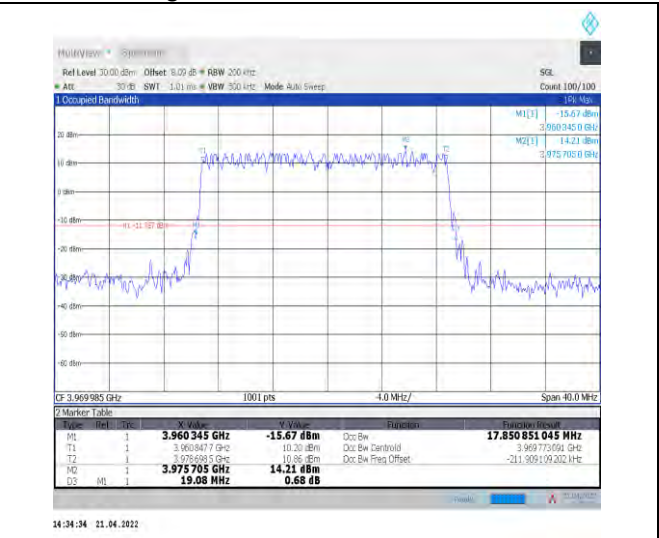
1-N77-3700-3980--30-20-H-2-DFT-PI2BPSK-Outer_Full Full-50@0-Ant0-17.851-19.080-≤20-PASS
