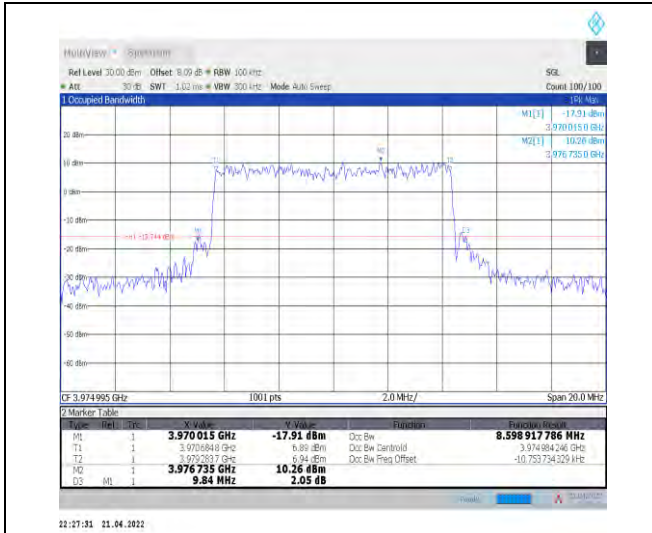
1-N77-3700-3980--30-10-H-7-CP-16QAM-Outer_Full -24@0-Ant0-8.599-9.840-≤10-PASS
