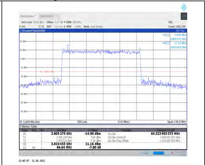
1-N77-3700-3980--30-70-M-4-DFT-64QAM-Outer_Full-180@0-Ant0-64.324-66.640-≤70-PASS
