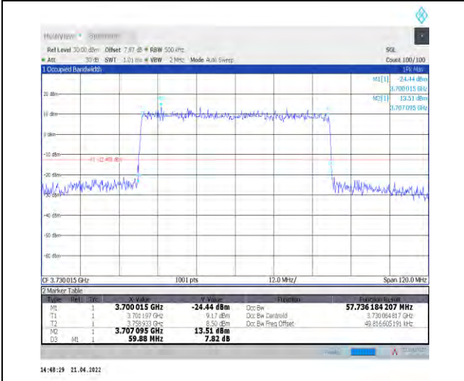
1-N77-3700-3980--30-60-L-1-DFT-QPSK-Outer_Full -162@0-Ant0-57.736-59.880-≤60-PASS
