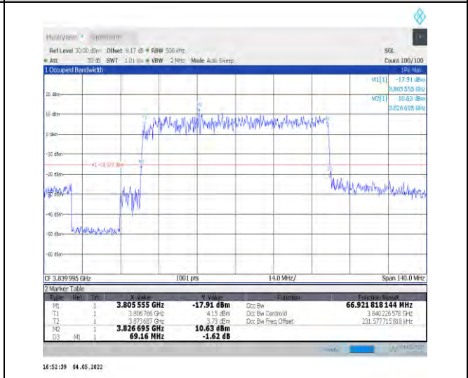
1-N77-3700-3980--30-70-M-6-CP-QPSK-Outer_Full-189@0-Ant0-66.922-69.160-≤70-PASS
