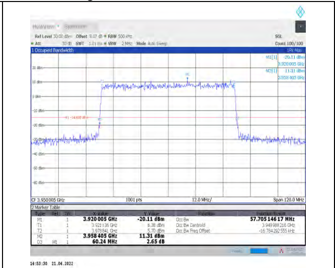
1-N77-3700-3980--30-60-H-6-CP-QPSK-Outer_Full-162@0-Ant0-57.705-60.240-≤60-PASS
