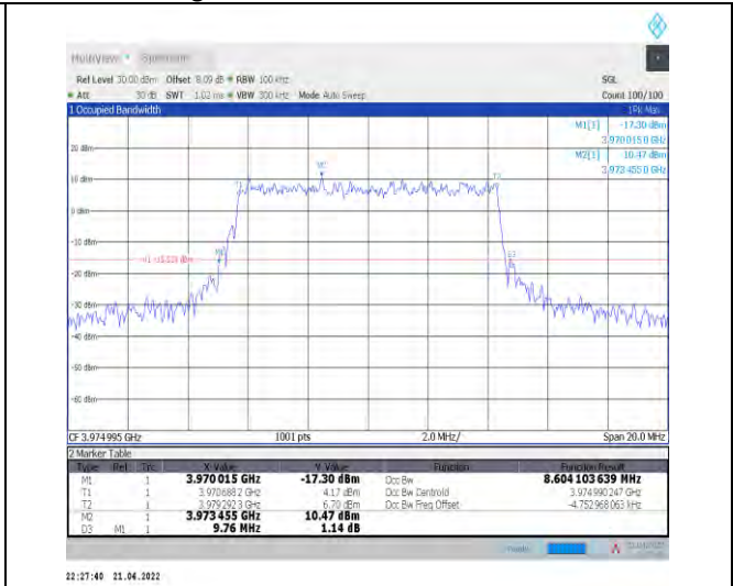
1-N77-3700-3980--30-10-H-8-CP-64QAM-Outer_Full -24@0-Ant0-8.604-9.760-≤10-PASS
