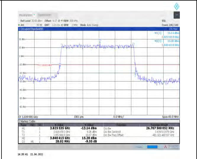
1-N77-3700-3980--30-30-M-2-DFT-PI2BPSK-Outer_Full Full-75@0-Ant0-26.71-28.020-<30-PASS
