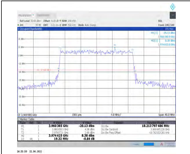
1-N77-3700-3980--30-20-H-9-CP-256QAM-Outer_Full-51@0-Ant0-18.214-19.320-≤20-PASS
