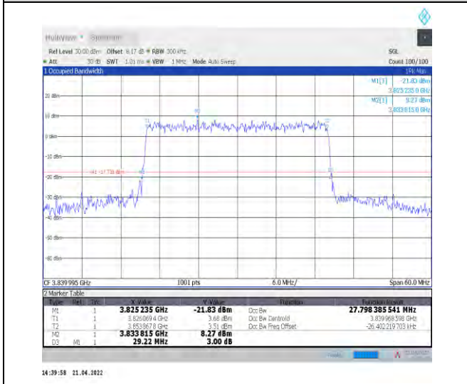
1-N77-3700-3980--30-30-M-9-CP-256QAM-Outer_Full I-78@0-Ant0-27.798-29.220-≤30-PASS
