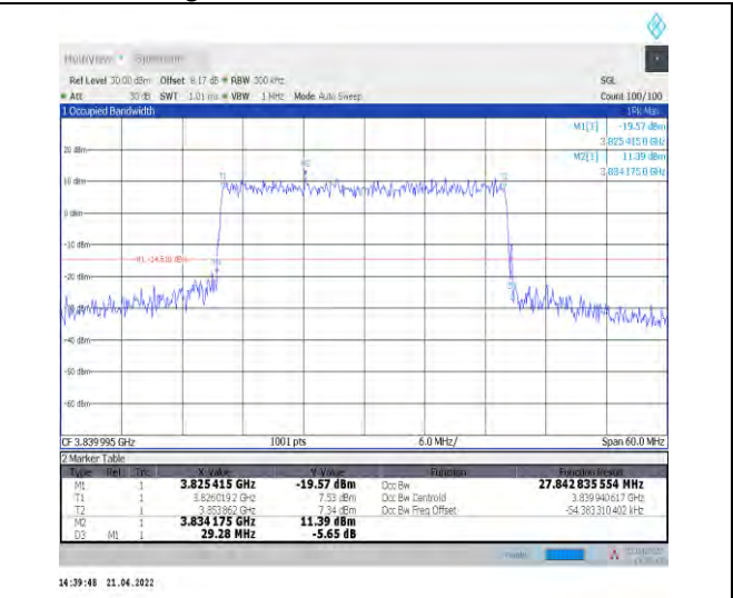
1-N77-3700-3980--30-30-M-8-CP-64QAM-Outer_Full -78@0-Ant0-27.843-29.280-≤30-PASS
