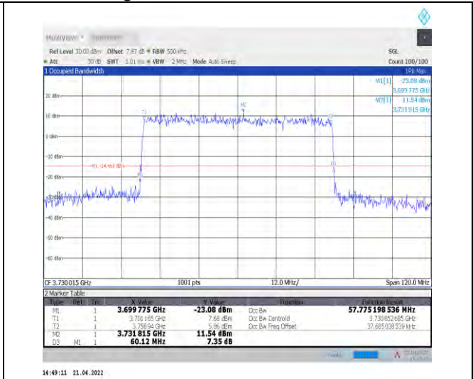
1-N77-3700-3980--30-60-L-4-DFT-64QAM-Outer_Ful I-162@0-Ant0-57.775-60.120-≤60-PASS
