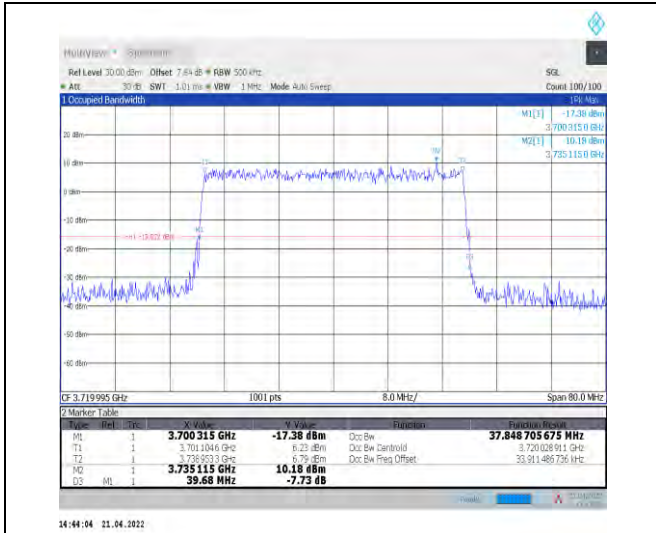
1-N77-3700-3980--30-40-L-9-CP-256QAM-Outer_Fu II-106@0-Ant0-37.853-39.680-≤40-PASS
