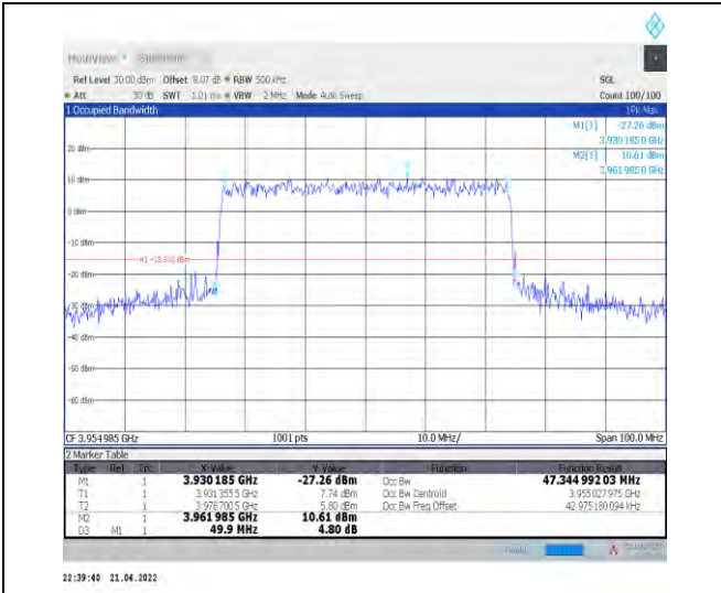
1-N77-3700-3980--30-50-H-8-CP-64QAM-Outer_Full -133@0-Ant0-47.345-49.900-≤50-PASS
