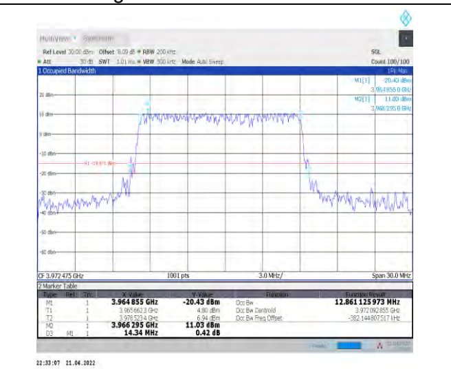
1-N77-3700-3980--30-15-H-5-DFT-256QAM-Outer_Full-36@0-Ant0-12.861-14.340-≤15-PASS
