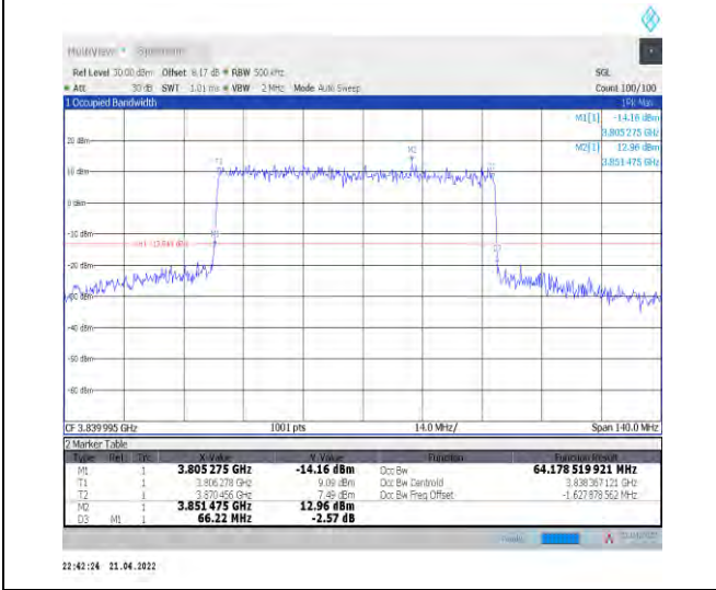
1-N77-3700-3980--30-70-M-1-DFT-QPSK-Outer_Full -180@0-Ant0-64.179-66.220-≤70-PASS
