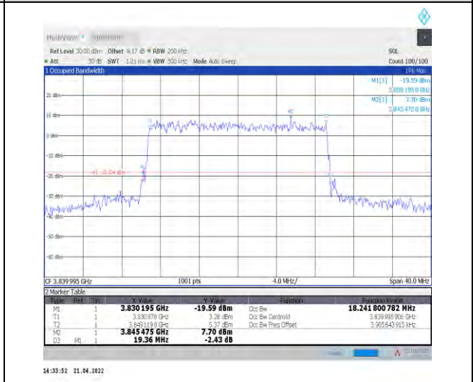
1-N77-3700-3980--30-20-M-9-CP-256QAM-Outer_Full-51@0-Ant0-18.242-19.360-≤20-PASS
