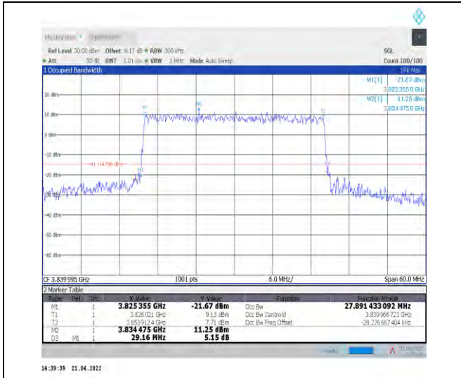
1-N77-3700-3980--30-30-M-7-CP-16QAM-Outer_Full I-78@0-Ant0-27.893-29.160-≤30-PASS
