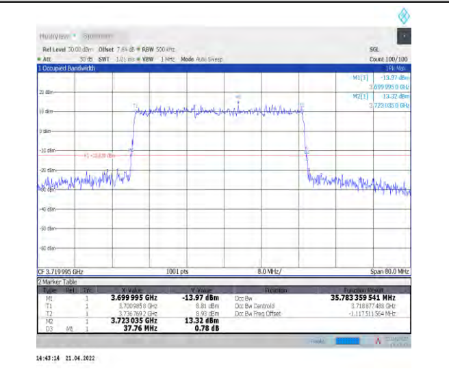
1-N77-3700-3980--30-40-L-4-DFT-64QAM-Outer_Full -100@0-Ant0-35.791-37.760-≤40-PASS
