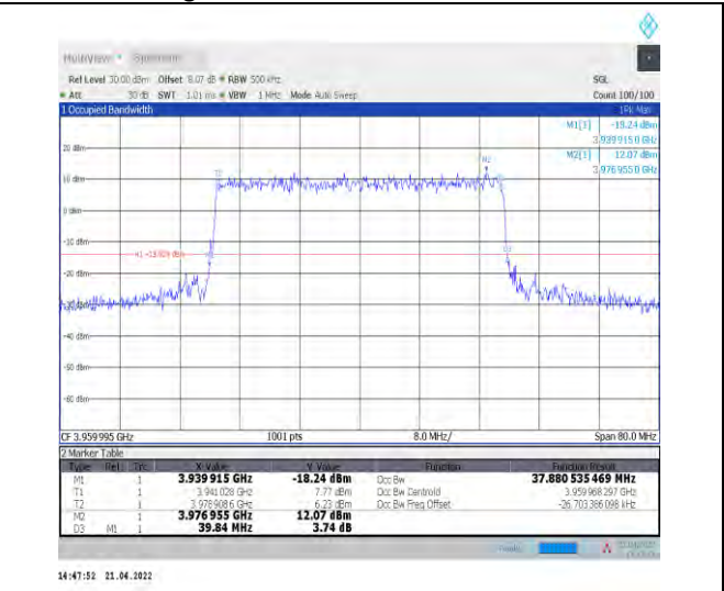
1-N77-3700-3980--30-40-H-8-CP-64QAM-Outer_Full -106@0-Ant0-37.892-39.840-<math>\leq 40</math>-PASS
