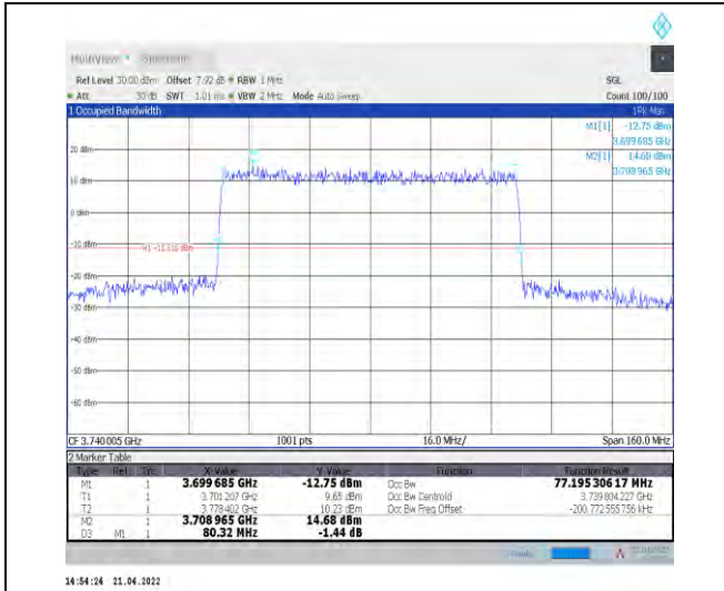
1-N77-3700-3980--30-80-L-1-DFT-QPSK-Outer_Full -216@0-Ant0-77.195-80.320-≤80-PASS
