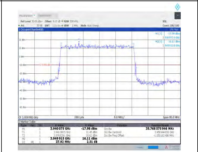
1-N77-3700-3980--30-40-M-9-CP-256QAM-Outer_Full-106@0-Ant0-37.71-39.440-≤40-PASS
