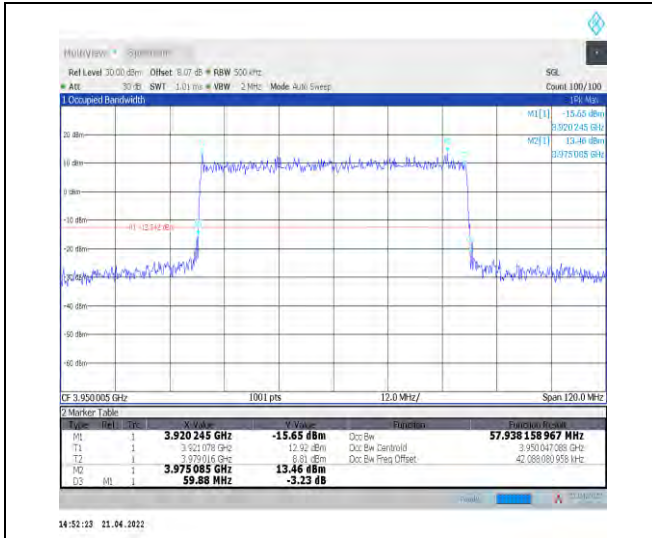
1-N77-3700-3980--30-60-H-1-DFT-QPSK-Outer_Full -162@0-Ant0-57.938-59.880-≤60-PASS
