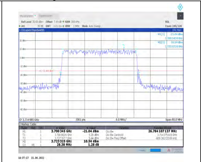
1-N77-3700-3980--30-30-L-5-DFT-256QAM-Outer_F ull-75@0-Ant0-26.784-28.380-≤30-PASS
