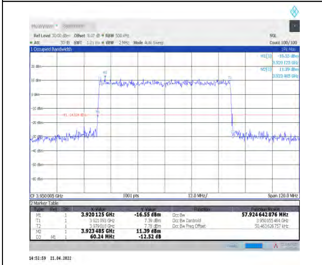
1-N77-3700-3980--30-60-H-3-DFT-16QAM-Outer_Full ull-162@0-Ant0-57.925-60.240-≤60-PASS
