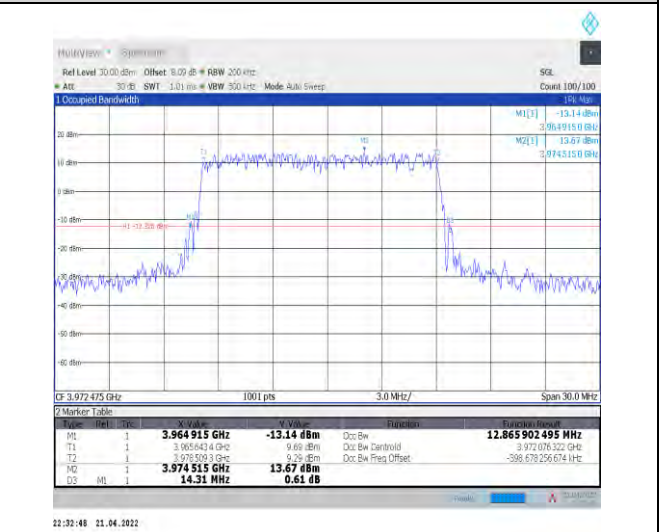
1-N77-3700-3980--30-15-H-3-DFT-16QAM-Outer_Full-36@0-Ant0-12.866-14.310-≤15-PASS
