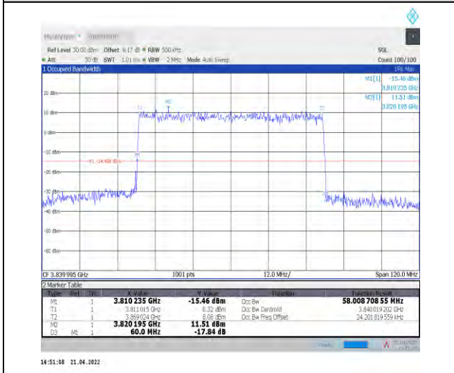
1-N77-3700-3980--30-60-M-4-DFT-64QAM-Outer_Full-162@0-Ant0-58.009-60.000-≤60-PASS
