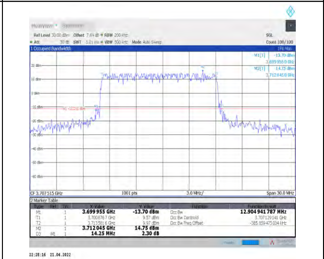
1-N77-3700-3980--30-15-L-1-DFT-QPSK-Outer_Full- 36@0-Ant0-12.905-14.250-≤15-PASS
