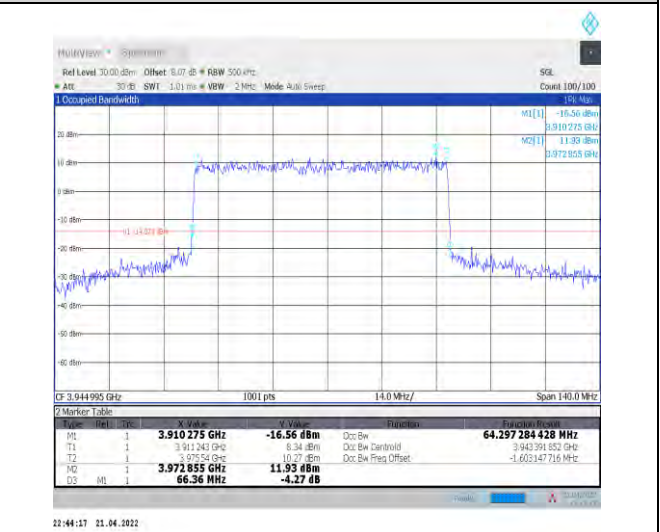
1-N77-3700-3980--30-70-H-1-DFT-QPSK-Outer_Full -180@0-Ant0-64.297-66.360-≤70-PASS
