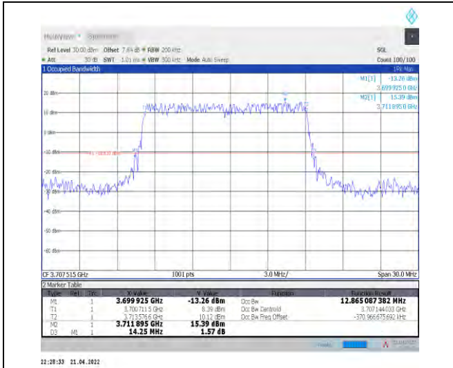
1-N77-3700-3980--30-15-L-2-DFT-PI2BPSK-Outer_Full-36@0-Ant0-12.865-14.250-≤15-PASS
