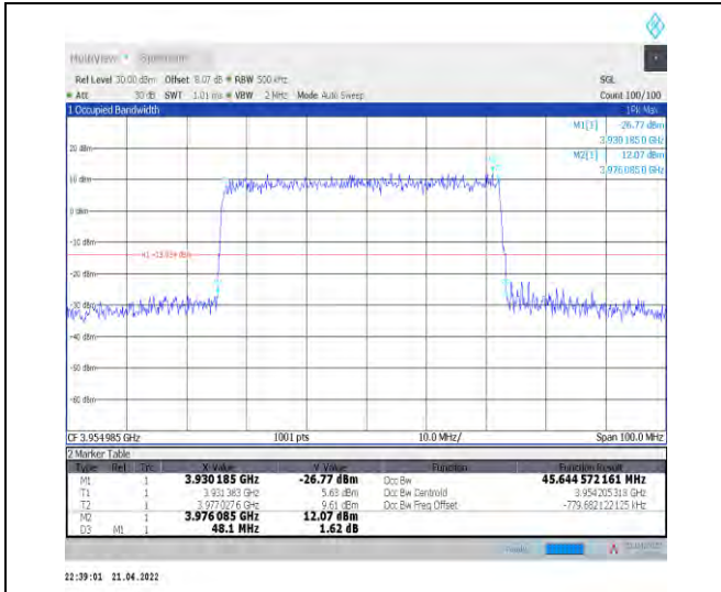
1-N77-3700-3980--30-50-H-4-DFT-64QAM-Outer_Full-128@0-Ant0-45.645-48.100-≤50-PASS
