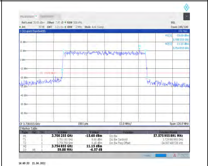
1-N77-3700-3980--30-60-L-6-CP-QPSK-Outer_Full-1 62@0-Ant0-57.576-59.880-≤60-PASS
