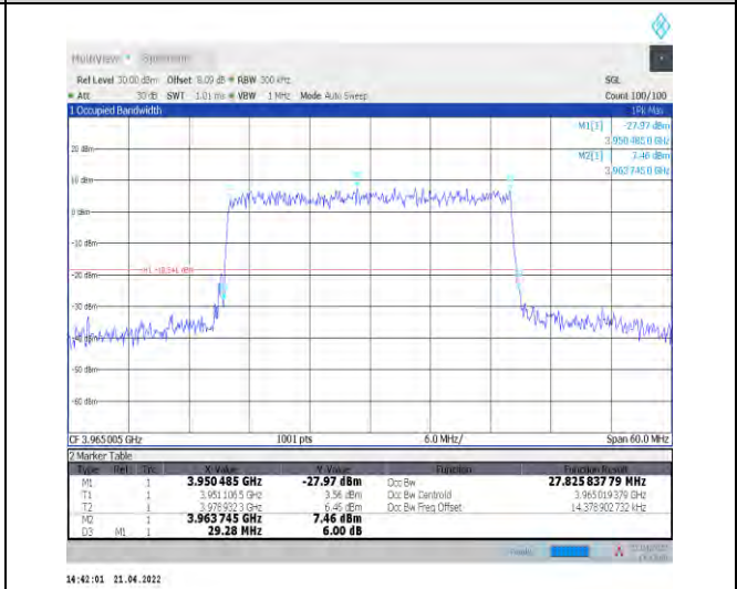
1-N77-3700-3980--30-30-H-9-CP-256QAM-Outer_Fu ll-78@0-Ant0-27.825-29.280-≤30-PASS
