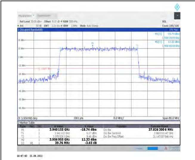
1-N77-3700-3980--30-40-H-7-CP-16QAM-Outer_Full -106@0-Ant0-37.823-39.760-<math>\leq 40</math>-PASS
