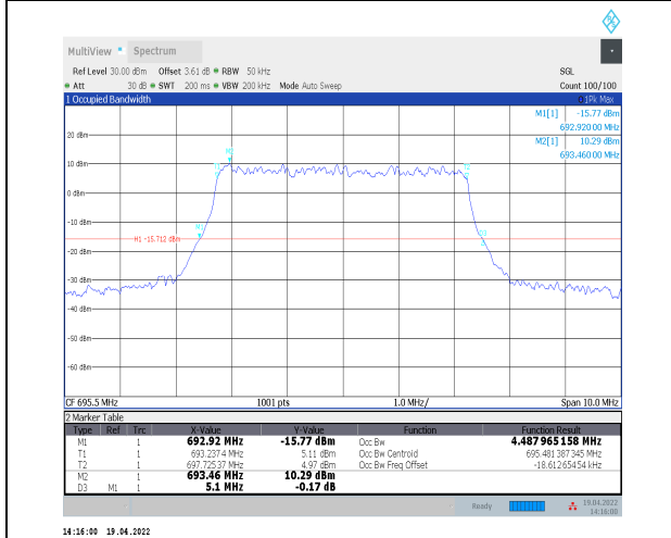
1-N71--15-5-H-5-DFT-256QAM-Outer_Full-25@0-Ant t0-4.488-5.100-≤5-PASS
