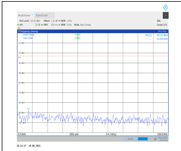
1-N71--15-20-H-1-DFT-PI2BPSK-Inner_1RB_Left-1 @1-0.009-0.15-Ant0--89.52--33-PASS
