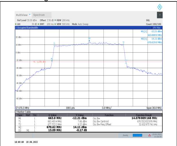
1-N71--15-15-L-8-CP-64QAM-Outer_Full-79@0-Ant 0-14.079-15.090-≤15-PASS
