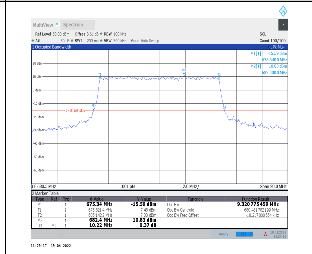
1-N71--15-10-M-8-CP-64QAM-Outer_Full-52@0-Ant 0-9.321-10.220-≤10-PASS
