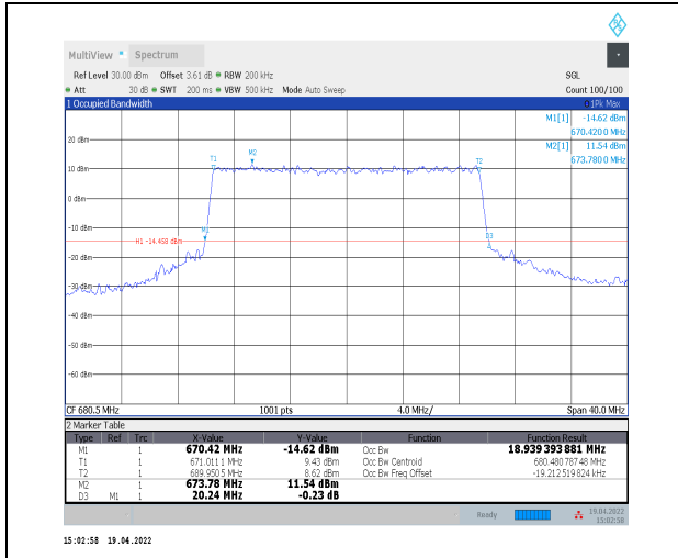
1-N71--15-20-M-7-CP-16QAM-Outer_Full-106@0-An t0-18.939-20.240-<math>\leq 20</math>-PASS
