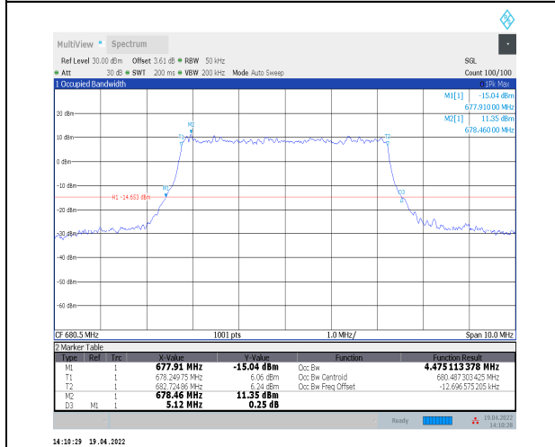
1-N71--15-5-M-6-CP-QPSK-Outer_Full-25@0-Ant0-4 .475-5.120-<math>\leq 5</math>-PASS
