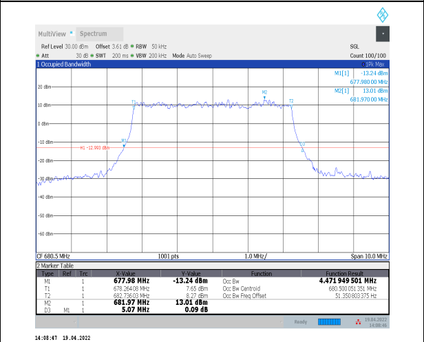
1-N71--15-5-M-3-DFT-16QAM-Outer_Full-25@0-Ant 0-4.472-5.070-≤5-PASS
