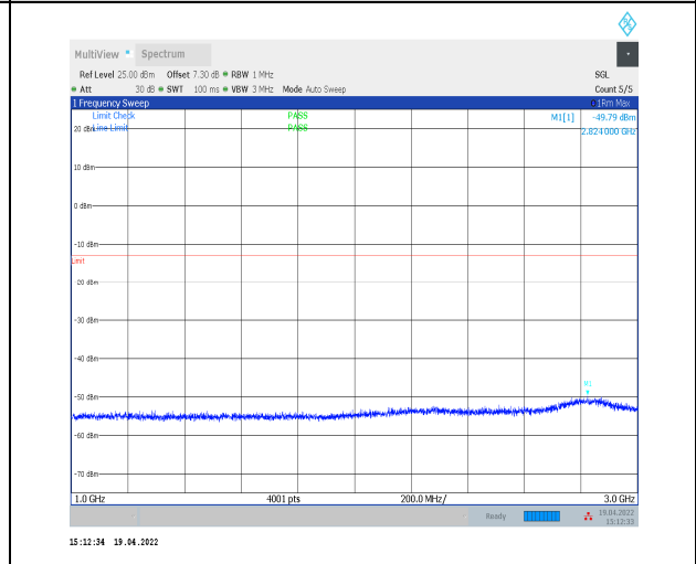
1-N71--15-20-H-1-DFT-PI2BPSK-Inner_1RB_Left-1 @1-1000-3000-Ant0--49.79--13-PASS
