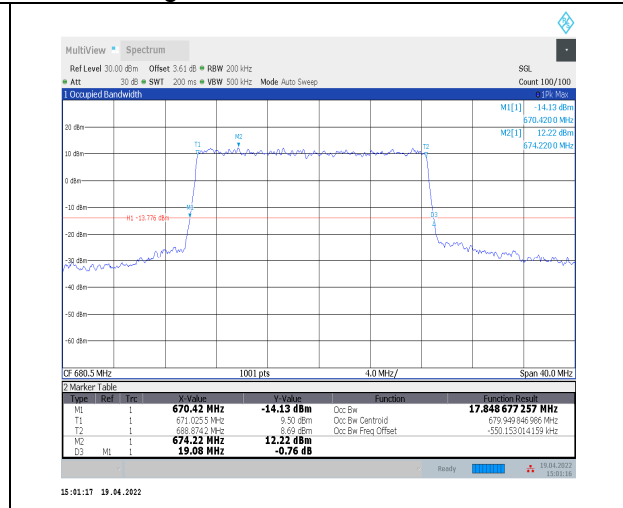
1-N71--15-20-M-4-DFT-64QAM-Outer_Full-100@0-Ant Ant0-17.849-19.080-≤20-PASS
