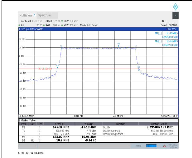
1-N71--15-10-M-7-CP-16QAM-Outer_Full-52@0-Ant 0-9.295-10.200-≤10-PASS
