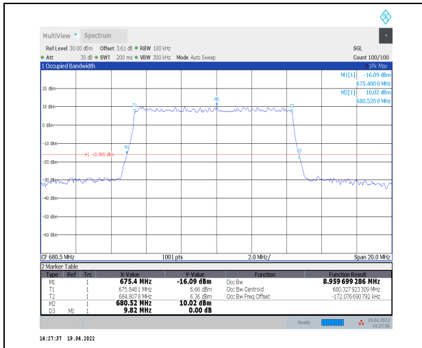
1-N71--15-10-M-5-DFT-256QAM-Outer_Full-50@0-A nt0-8.96-9.820-≤10-PASS
