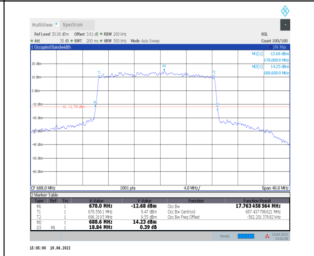
1-N71--15-20-H-1-DFT-QPSK-Outer_Full-100@0-An t0-17.763-18.840-<math>\leq 20</math>-PASS
