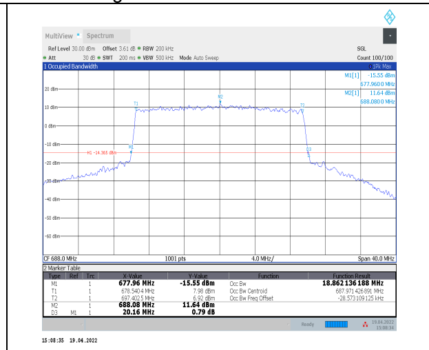
1-N71--15-20-H-7-CP-16QAM-Outer_Full-106@0-An t0-18.862-20.160-<math>\leq 20</math>-PASS
