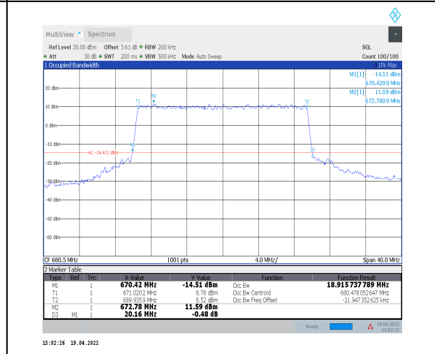
1-N71--15-20-M-6-CP-QPSK-Outer_Full-106@0-Ant 0-18.916-20.160-≤20-PASS
