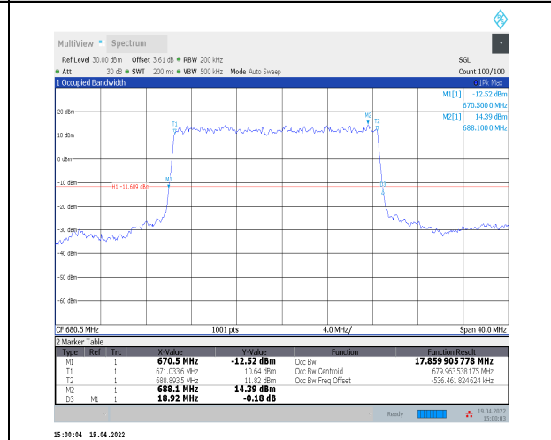
1-N71--15-20-M-2-DFT-PI2BPSK-Outer_Full-100@0-Ant 0-17.86-18.920-≤20-PASS
