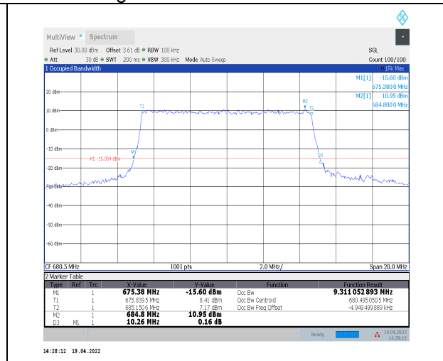
1-N71--15-10-M-6-CP-QPSK-Outer_Full-52@0-Ant0 -9.311-10.260-≤10-PASS
