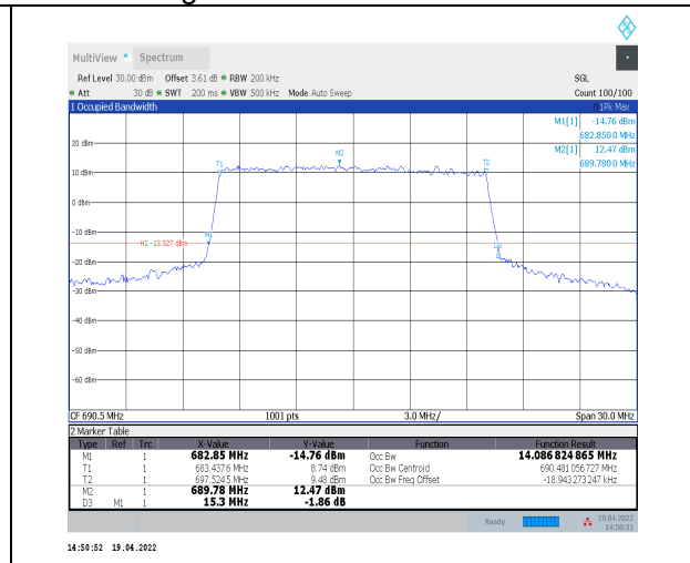
1-N71--15-15-H-6-CP-QPSK-Outer_Full-79@0-Ant0- 14.087-15.300≤15-PASS
