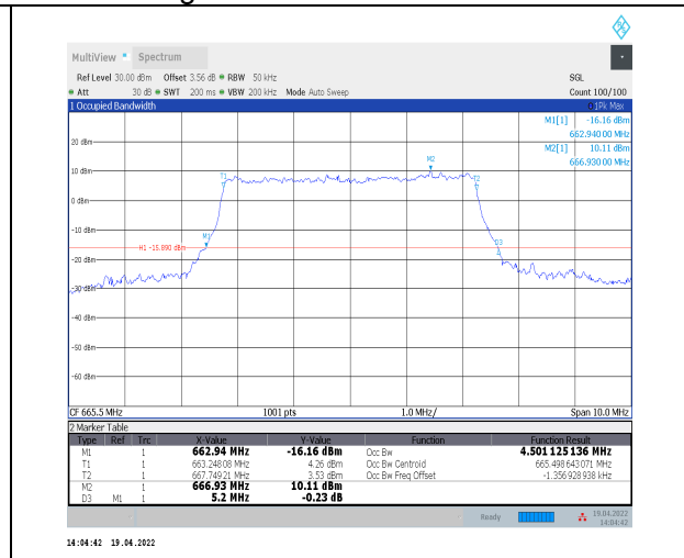
1-N71--15-5-L-6-CP-QPSK-Outer_Full-25@0-Ant0-4 .501-5.200-<math>\leq 5</math>-PASS
