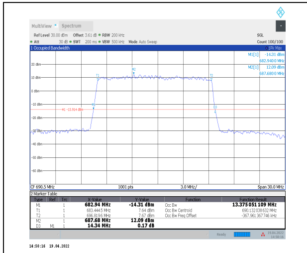
1-N71--15-15-H-5-DFT-256QAM-Outer_Full-75@0-A nt0-13.375-14.340≤15-PASS
