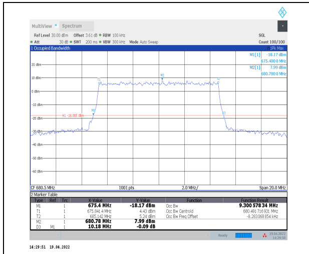
1-N71--15-10-M-9-CP-256QAM-Outer_Full-52@0-Ant t0-9.301-10.180-<=10-PASS
