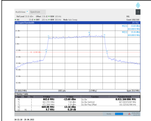
1-N71--15-10-L-4-DFT-64QAM-Outer_Full-50@0-Ant 0-8.921-9.700-≤10-PASS
