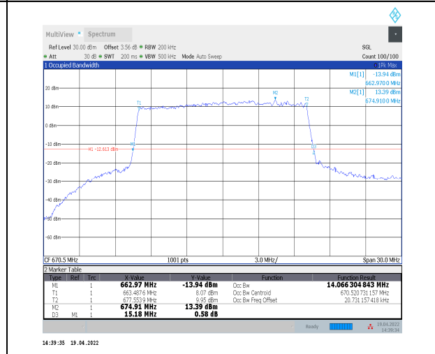
1-N71--15-15-L-6-CP-QPSK-Outer_Full-79@0-Ant0 14.066-15.180≤15-PASS
