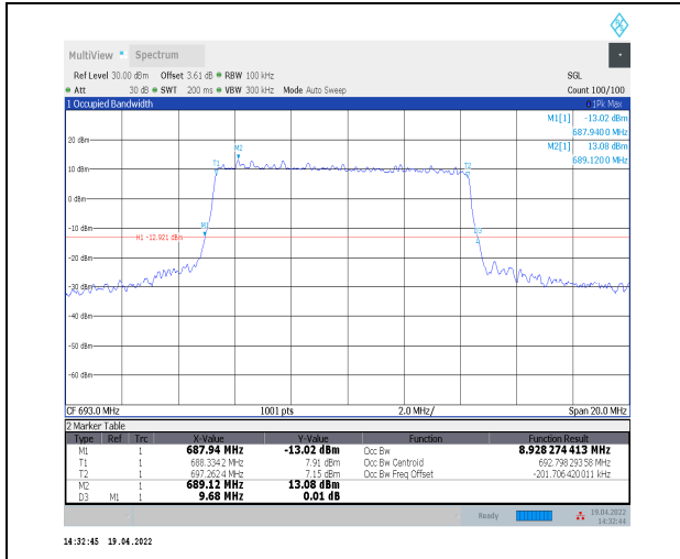
1-N71--15-10-H-4-DFT-64QAM-Outer_Full-50@0-Ant t0-8.928-9.680-≤10-PASS
