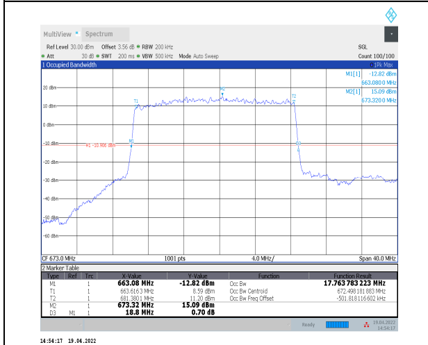
1-N71--15-20-L-2-DFT-PI2BPSK-Outer_Full-100@0-Ant0 Ant0-17.764-18.800-<=20-PASS
