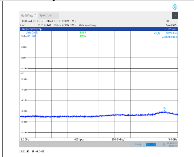
1-N71--15-20-M-1-DFT-PI2BPSK-Inner_1RB_Left-1 @1-1000-3000-Ant0--50.27--13-PASS
