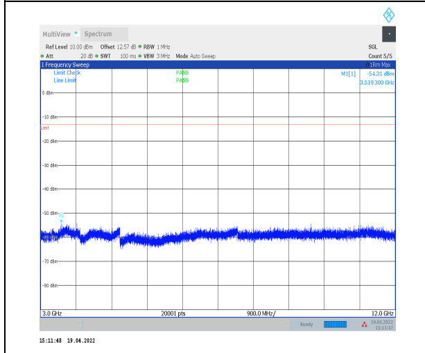
1-N71--15-20-M-1-DFT-PI2BPSK-Inner_1RB_Left-1 @1-3000-12000-Ant0--54.31--13-PASS
