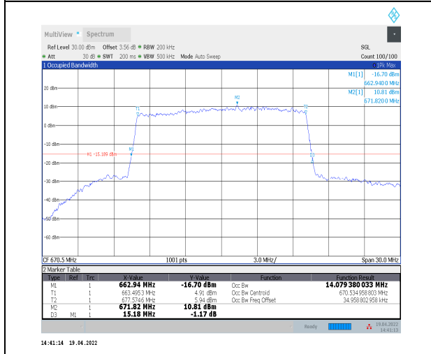
1-N71--15-15-L-9-CP-256QAM-Outer_Full-79@0-Ant 0-14.079-15.180-≤15-PASS
