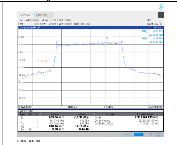
1-N71--15-10-L-3-DFT-16QAM-Outer_Full-50@0-An t0-8.94-9.580-≤10-PASS
