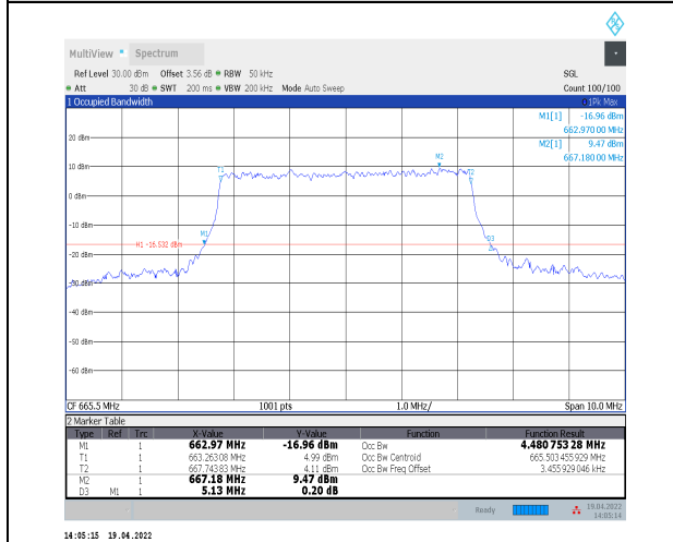
1-N71--15-5-L-7-CP-16QAM-Outer_Full-25@0-Ant0- 4.481-5.130-<math>\leq 5</math>-PASS
