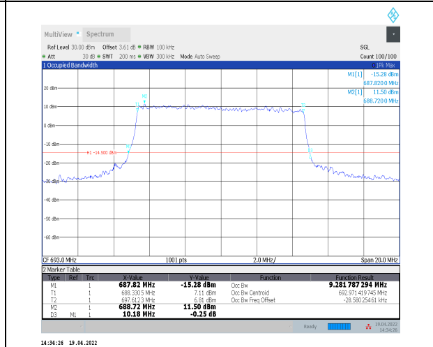
1-N71--15-10-H-7-CP-16QAM-Outer_Full-52@0-Ant 0-9.282-10.180-≤10-PASS
