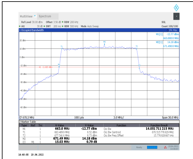
1-N71--15-15-L-7-CP-16QAM-Outer_Full-79@0-Ant0 -14.052-15.030-≤15-PASS
