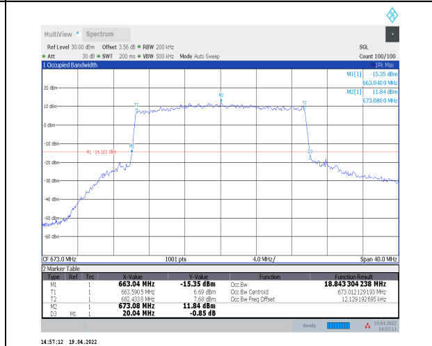
1-N71--15-20-L-7-CP-16QAM-Outer_Full-106@0-Ant0 t0-18.843-20.040-<math>\leq 20</math>-PASS
