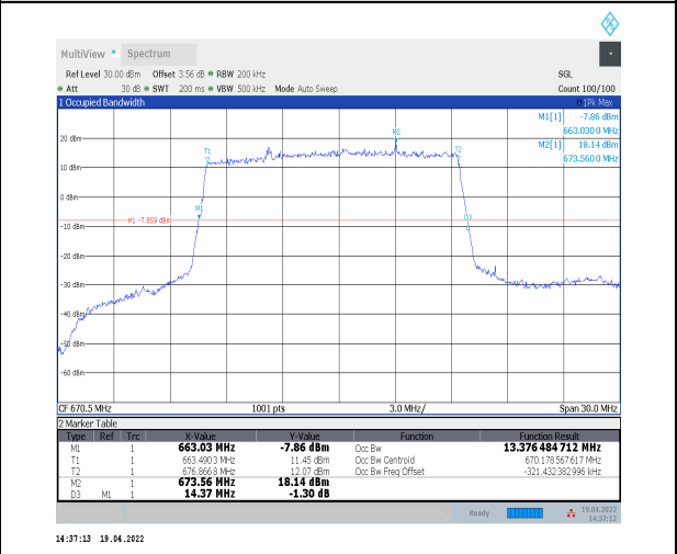
1-N71--15-15-L-2-DFT-PI2BPSK-Outer_Full-75@0-A n0-13.376-14.370-≤15-PASS
