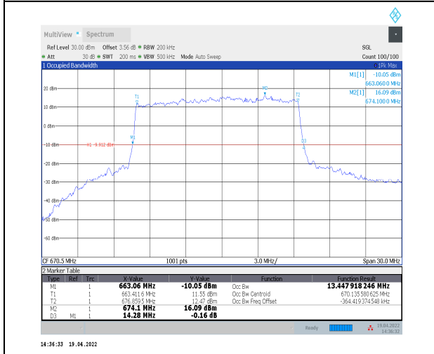
1-N71--15-15-L-1-DFT-QPSK-Outer_Full-75@0-Ant0 -13.448-14.280-≤15-PASS
