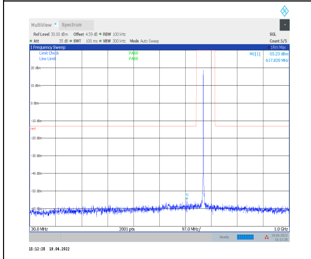
1-N71--15-20-H-1-DFT-PI2BPSK-Inner_1RB_Left-1 @1-30-1000-Ant0--55.23--13-PASS
