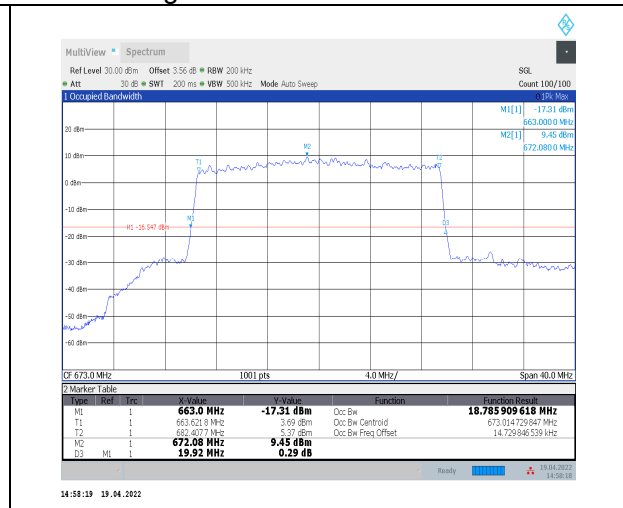
1-N71--15-20-L-9-CP-256QAM-Outer_Full-106@0-Ant 0-18.786-19.920-≤20-PASS
