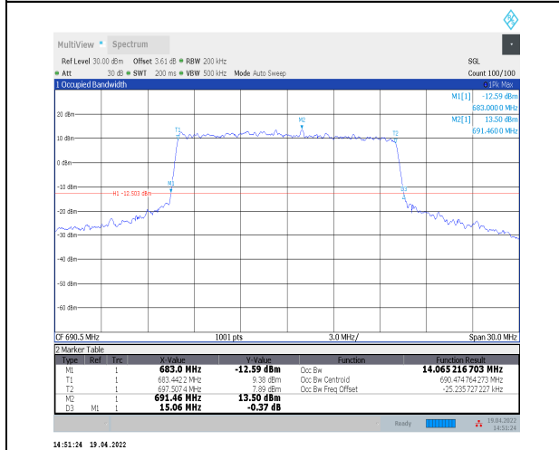
1-N71--15-15-H-7-CP-16QAM-Outer_Full-79@0-Ant 0-14.065-15.060≤15-PASS
