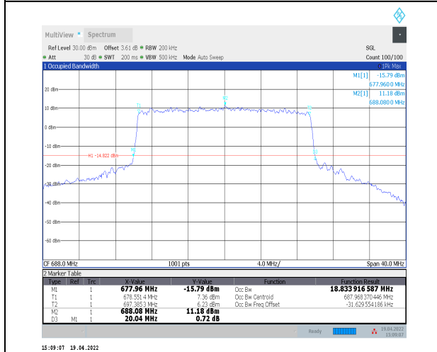
1-N71--15-20-H-8-CP-64QAM-Outer_Full-106@0-An t0-18.834-20.040-<math>\leq 20</math>-PASS
