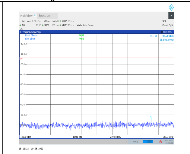
1-N71--15-20-H-1-DFT-PI2BPSK-Inner_1RB_Left-1 @1-0.15-30-Ant0--85.08--23-PASS
