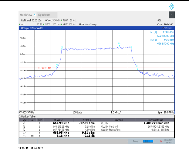
1-N71--15-5-L-8-CP-64QAM-Outer_Full-25@0-Ant0- 4.488-5.180-<math>\leq 5</math>-PASS
