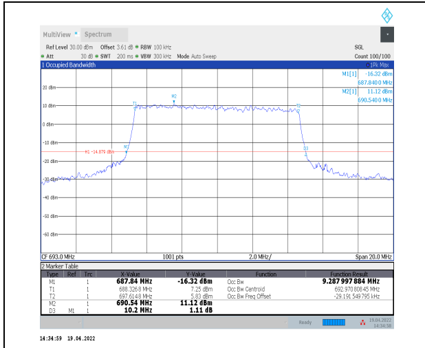
1-N71--15-10-H-8-CP-64QAM-Outer_Full-52@0-Ant 0-9.288-10.200-≤10-PASS
