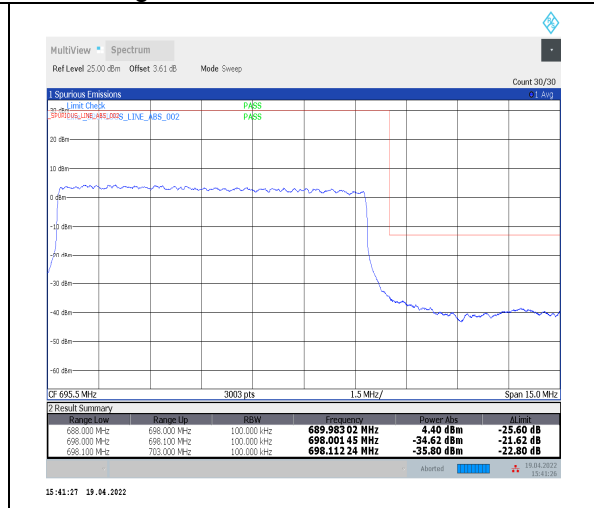
1-N71--15-10-H-3-DFT-PI2BPSK-Outer_Full-50@ 0-Ant0-PASS-see graph
