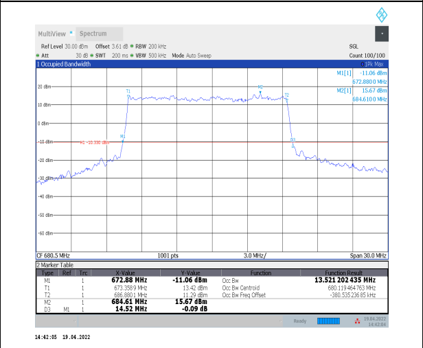
1-N71--15-15-M-1-DFT-QPSK-Outer_Full-75@0-Ant 0-13.521-14.520-≤15-PASS
