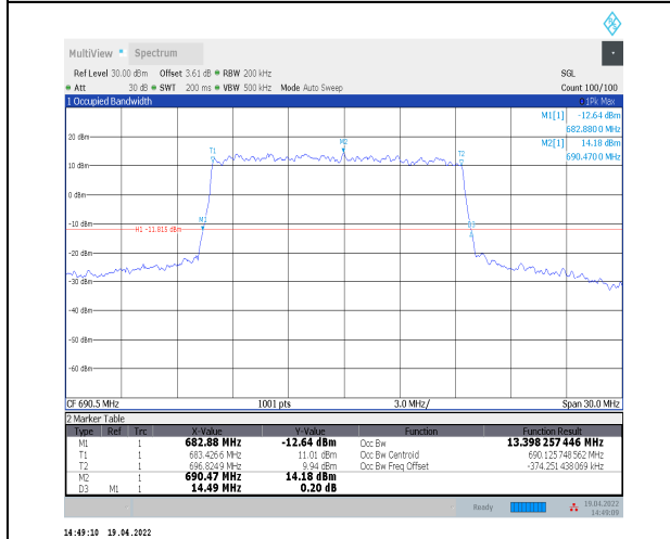
1-N71--15-15-H-3-DFT-16QAM-Outer_Full-75@0-Ant 0-13.398-14.490≤15-PASS
