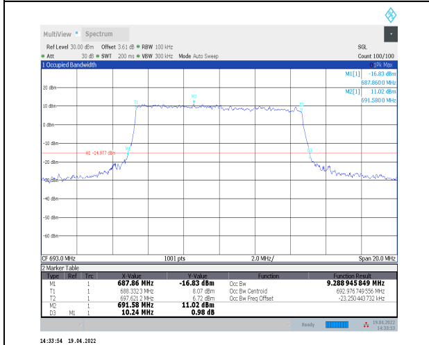
1-N71--15-10-H-6-CP-QPSK-Outer_Full-52@0-Ant0 9.289-10.240-≤10-PASS
