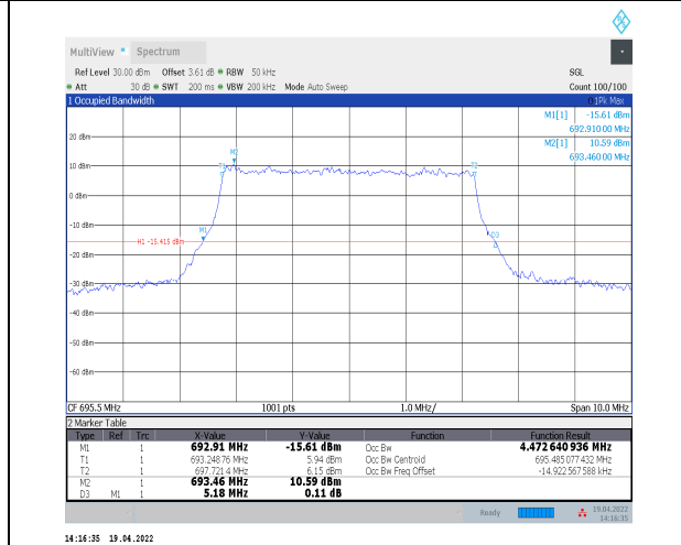
1-N71--15-5-H-6-CP-QPSK-Outer_Full-25@0-Ant0-4 .473-5.180-≤5-PASS
