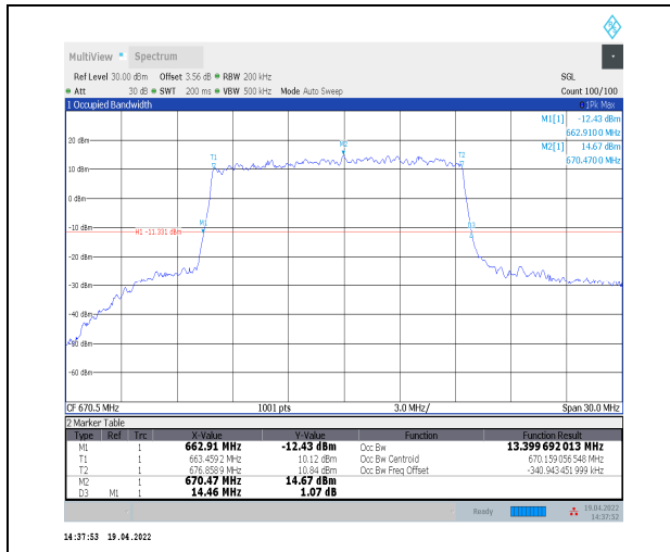
1-N71--15-15-L-3-DFT-16QAM-Outer_Full-75@0-Ant 0-13.4-14.460≤15-PASS
