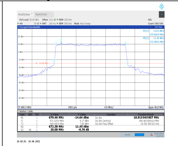
1-N71--15-20-M-8-CP-64QAM-Outer_Full-106@0-A nt0-18.915-20.080-<math>\leq 20</math>-PASS
