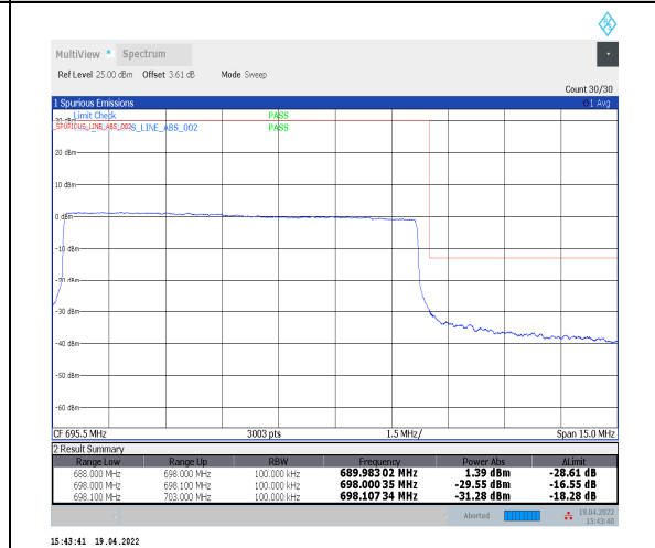
1-N71--15-10-H-6-CP-QPSK-Outer_Full-52@0-Ant0- PASS-see graph
