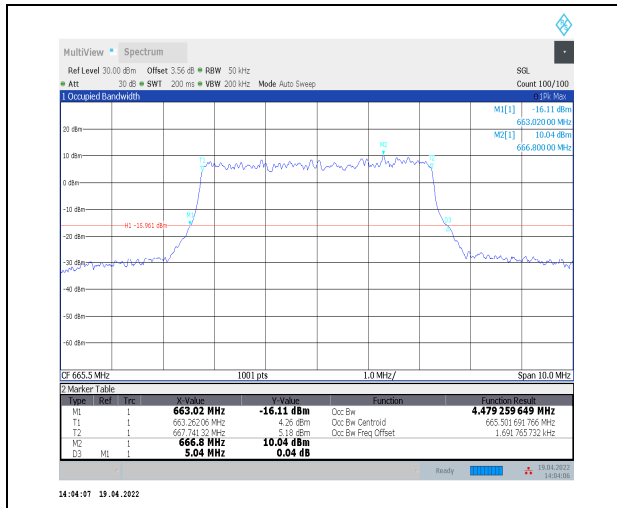
1-N71--15-5-L-5-DFT-256QAM-Outer_Full-25@0-Ant 0-4.479-5.040-<math>\leq 5</math>-PASS
