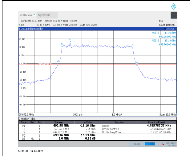
1-N71--15-5-H-1-DFT-QPSK-Outer_Full-25@0-Ant0 4.486-5.000≤5-PASS
