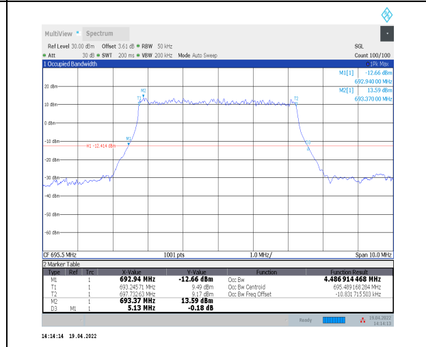
1-N71--15-5-H-2-DFT-PI2BPSK-Outer_Full-25@0-Ant0 4.487-5.130≤5-PASS
