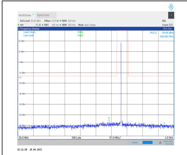
1-N71--15-20-M-1-DFT-PI2BPSK-Inner_1RB_Left-1 @1-30-1000-Ant0--56.06--13-PASS
