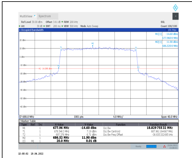
1-N71--15-20-H-6-CP-QPSK-Outer_Full-106@0-An t0-18.83-20.000-<math>\leq 20</math>-PASS
