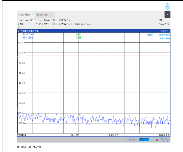
1-N71--15-20-M-1-DFT-PI2BPSK-Inner_1RB_Left-1 @1-0.009-0.15-Ant0--88.59--33-PASS
