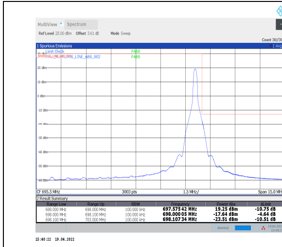
1-N71--15-10-H-2-DFT-PI2BPSK-Edge_1RB_Right-1@ 51-Ant0-PASS-see graph
