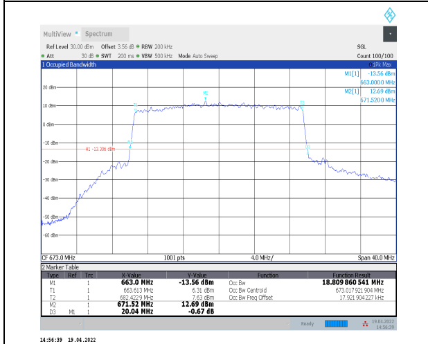
1-N71--15-20-L-6-CP-QPSK-Outer_Full-106@0-Ant0 -18.81-20.040-<math>\leq 20</math>-PASS
