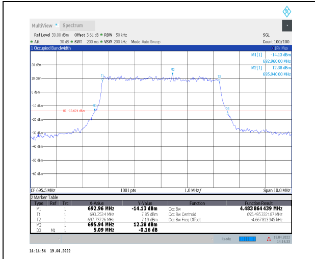
1-N71--15-5-H-3-DFT-16QAM-Outer_Full-25@0-Ant 0-4.484-5.090-≤5-PASS
