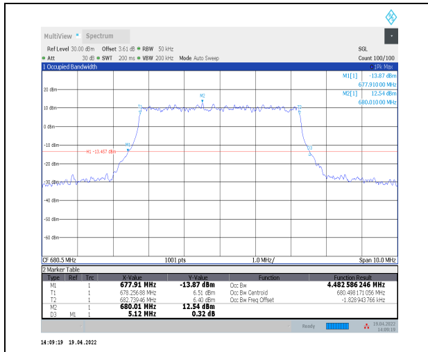
1-N71--15-5-M-4-DFT-64QAM-Outer_Full-25@0-Ant 0-4.483-5.120-<math>\leq 5</math>-PASS
