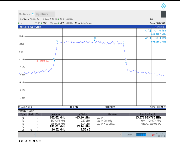
1-N71--15-15-H-4-DFT-64QAM-Outer_Full-75@0-Ant 0-13.377-14.520≤15-PASS
