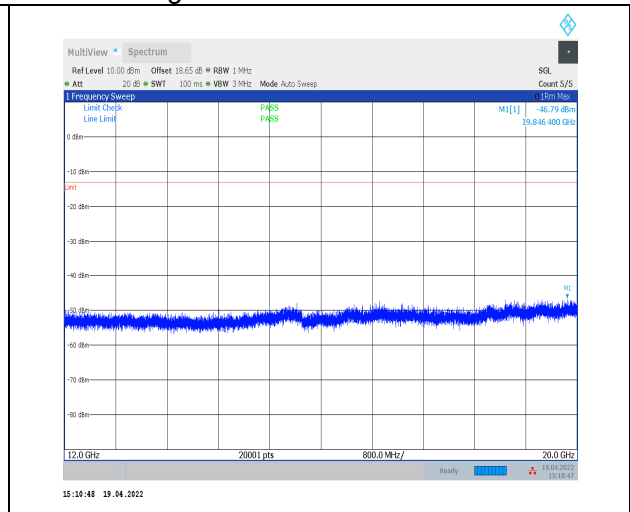
1-N71--15-20-L-1-DFT-PI2BPSK-Inner_1RB_Left-1 @ 1-12000-20000-Ant0--46.79--13-PASS
