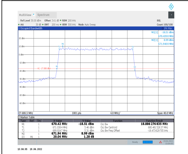
1-N71--15-20-M-9-CP-256QAM-Outer_Full-106@0-A nt0-18.886-20.040-<math>\leq 20</math>-PASS
