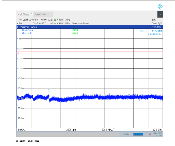
1-N71--15-20-H-1-DFT-PI2BPSK-Inner_1RB_Left-1 @1-3000-12000-Ant0--54.42--13-PASS
