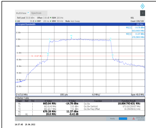
1-N71--15-20-L-8-CP-64QAM-Outer_Full-106@0-Ant 0-18.807-20.000-≤20-PASS
