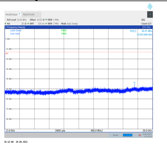
1-N71--15-20-H-1-DFT-PI2BPSK-Inner_1RB_Left-1 @1-12000-20000-Ant0--46.91--13-PASS
