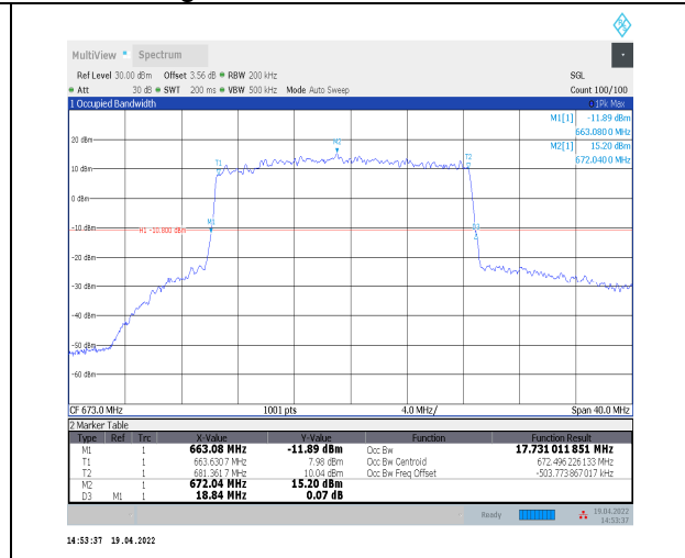
1-N71--15-20-L-1-DFT-QPSK-Outer_Full-100@0-Ant 0-17.731-18.840-<=20-PASS
