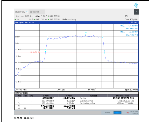
1-N71--15-15-L-5-DFT-256QAM-Outer_Full-75@0-A nt0-13.354-14.310≤15-PASS
