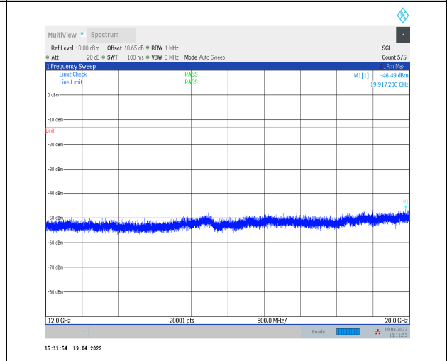
1-N71--15-20-M-1-DFT-PI2BPSK-Inner_1RB_Left-1 @1-12000-20000-Ant0--46.49--13-PASS
