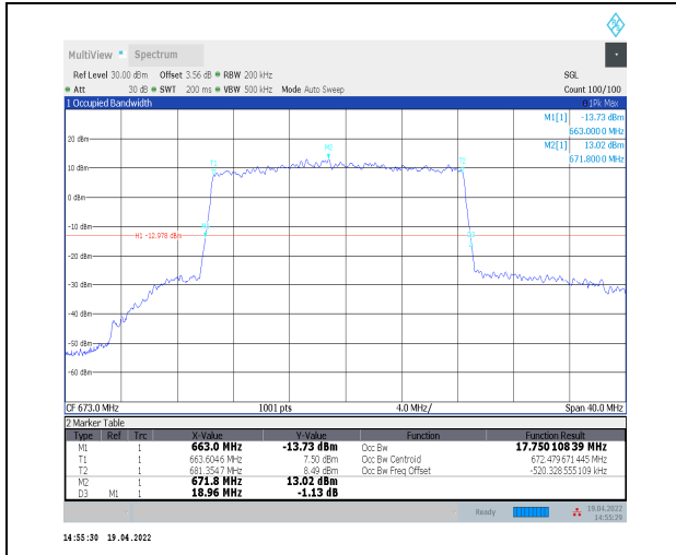
1-N71--15-20-L-4-DFT-64QAM-Outer_Full-100@0-A nt0-17.75-18.960-<math>\leq 20</math>-PASS
