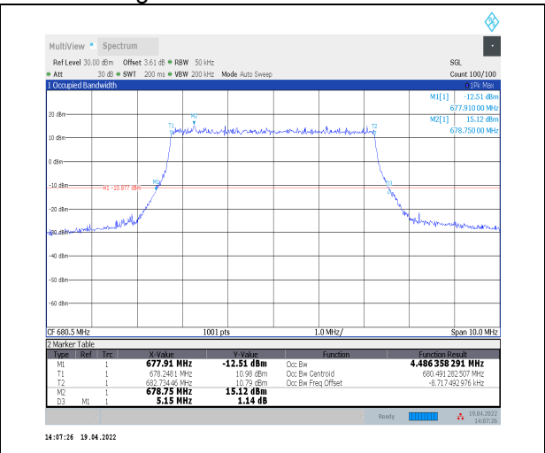
1-N71--15-5-M-1-DFT-QPSK-Outer_Full-25@0-Ant0 -4.486-5.150-≤5-PASS
