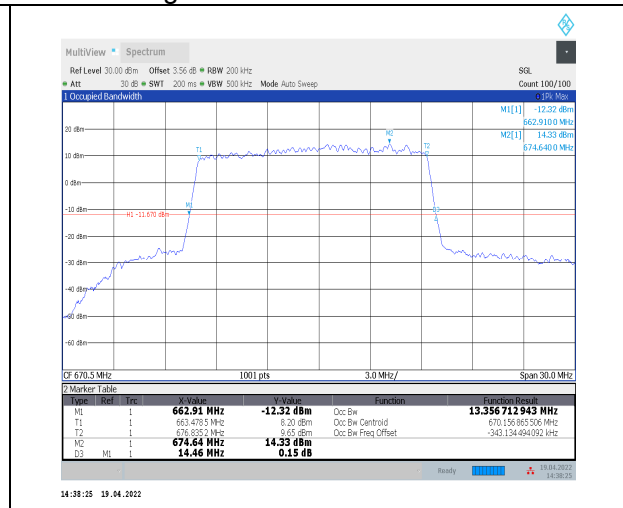
1-N71--15-15-L-4-DFT-64QAM-Outer_Full-75@0-Ant t0-13.357-14.460≤15-PASS
