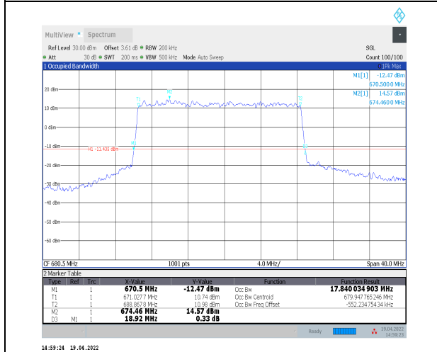
1-N71--15-20-M-1-DFT-QPSK-Outer_Full-100@0-Ant 0-17.84-18.920-≤20-PASS
