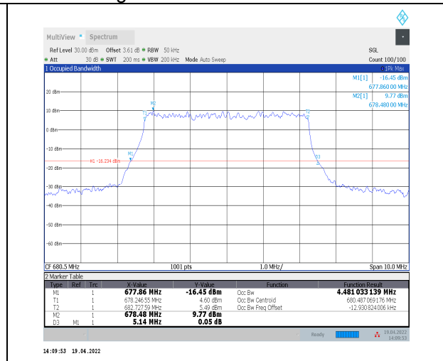
1-N71--15-5-M-5-DFT-256QAM-Outer_Full-25@0-A nt0-4.481-5.140-<math>\leq 5</math>-PASS
