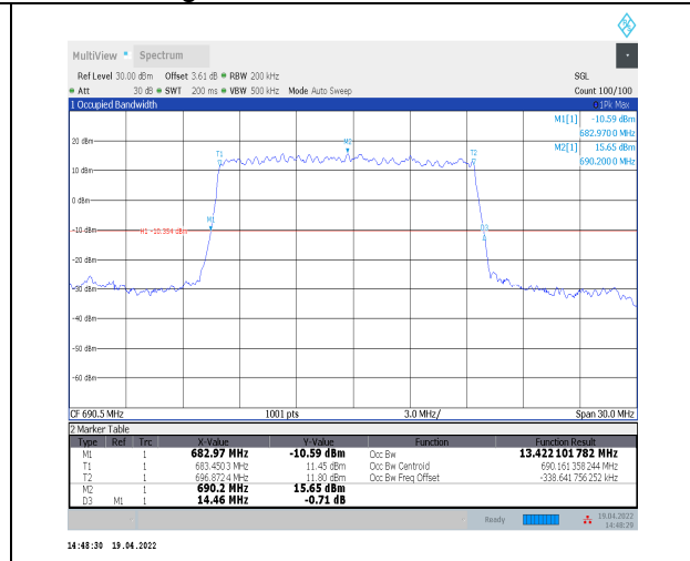
1-N71--15-15-H-2-DFT-PI2BPSK-Outer_Full-75@0-Ant 0-13.422-14.460≤15-PASS
