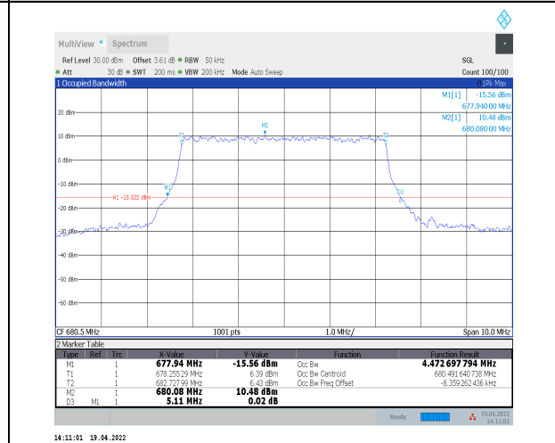
1-N71--15-5-M-7-CP-16QAM-Outer_Full-25@0-Ant0 -4.473-5.110-<math>\leq 5</math>-PASS
