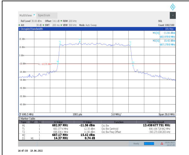
1-N71--15-15-H-1-DFT-QPSK-Outer_Full-75@0-Ant 0-13.459-14.370≤15-PASS
