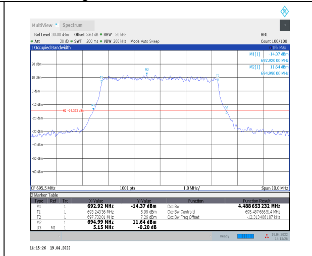
1-N71--15-5-H-4-DFT-64QAM-Outer_Full-25@0-Ant 0-4.489-5.150-≤5-PASS
