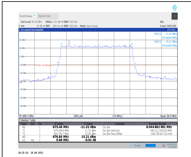
1-N71--15-10-M-1-DFT-QPSK-Outer_Full-50@0-Ant 0-8.945-9.680≤10-PASS
