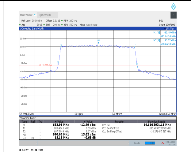
1-N71--15-15-H-8-CP-64QAM-Outer_Full-79@0-Ant 0-14.11-15.150≤15-PASS
