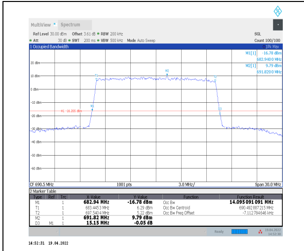
1-N71--15-15-H-9-CP-256QAM-Outer_Full-79@0-Ant t0-14.095-15.150-<=15-PASS
