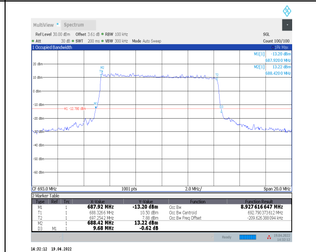
1-N71--15-10-H-3-DFT-16QAM-Outer_Full-50@0-Ant t0-8.928-9.680-<=10-PASS
