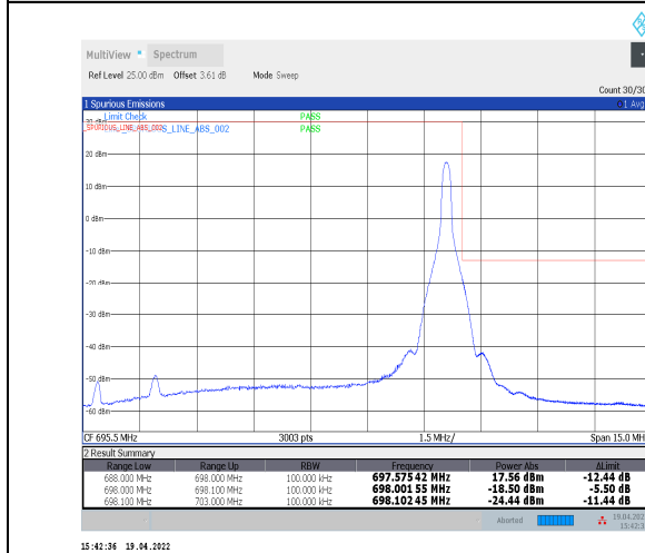
1-N71--15-10-H-5-CP-QPSK-Edge_1RB_Right-1@51- Ant0-PASS-see graph
