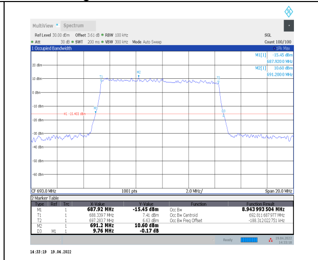
1-N71--15-10-H-5-DFT-256QAM-Outer_Full-50@0-Ant nt0-8.944-9.760-≤10-PASS
