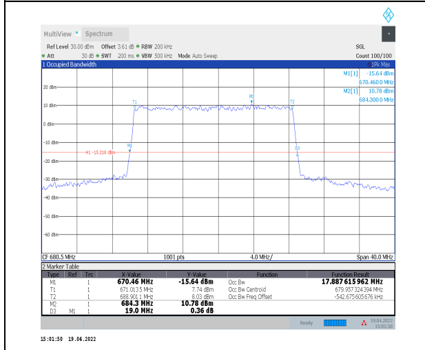
1-N71--15-20-M-5-DFT-256QAM-Outer_Full-100@0-Ant Ant0-17.888-19.000-≤20-PASS
