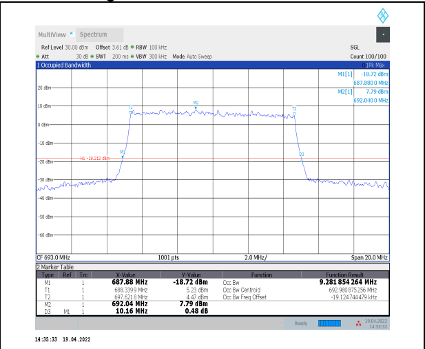
1-N71--15-10-H-9-CP-256QAM-Outer_Full-52@0-An 10-9.282-10.160-≤10-PASS
