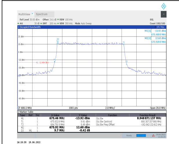
1-N71--15-10-M-3-DFT-16QAM-Outer_Full-50@0-Ant t0-8.949-9.700≤10-PASS
