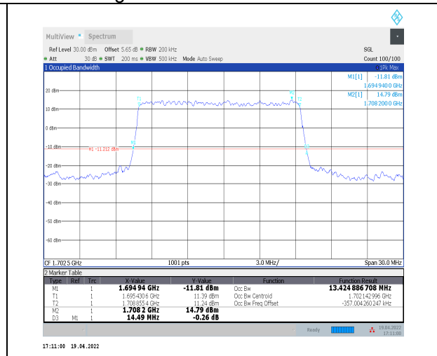
1-N70--15-15-H-2-DFT-PI2BPSK-Outer_Full-75@0-Ant 2-13.425-14.490≤15-PASS
