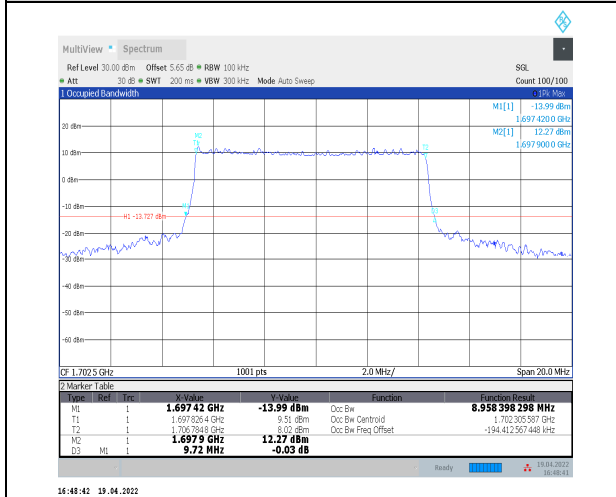
1-N70--15-10-M-3-DFT-16QAM-Outer_Full-50@0-Ant t2-8.958-9.720≤10-PASS
