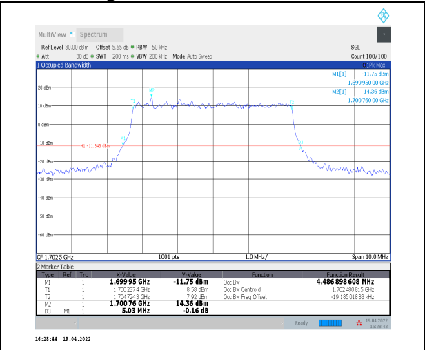
1-N70--15-5-M-1-DFT-QPSK-Outer_Full-25@0-Ant2 -4.487-5.030-≤5-PASS
