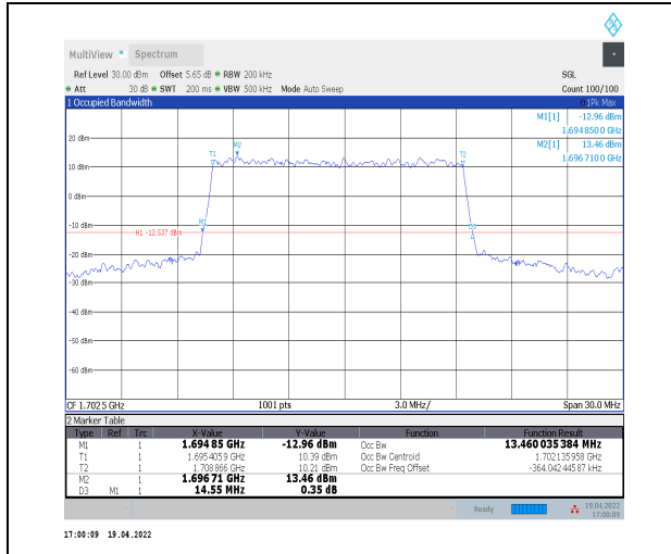
1-N70--15-15-L-3-DFT-16QAM-Outer_Full-75@0-Ant 2-13.46-14.550-≤15-PASS
