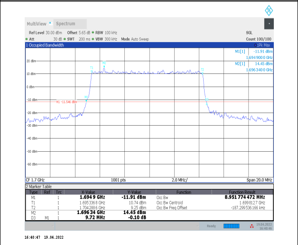
1-N70--15-10-L-1-DFT-QPSK-Outer_Full-50@0-Ant2 -8.952-9.720<=10-PASS
