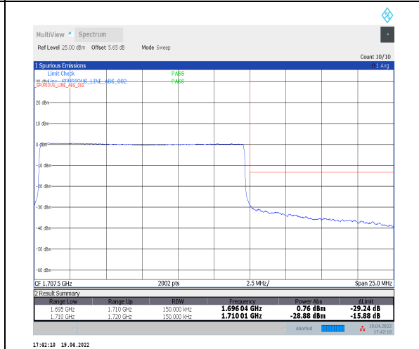
1-N70--15-15-H-6-CP-QPSK-Outer_Full-79@0-Ant2-seegraph-PASS-see graph
