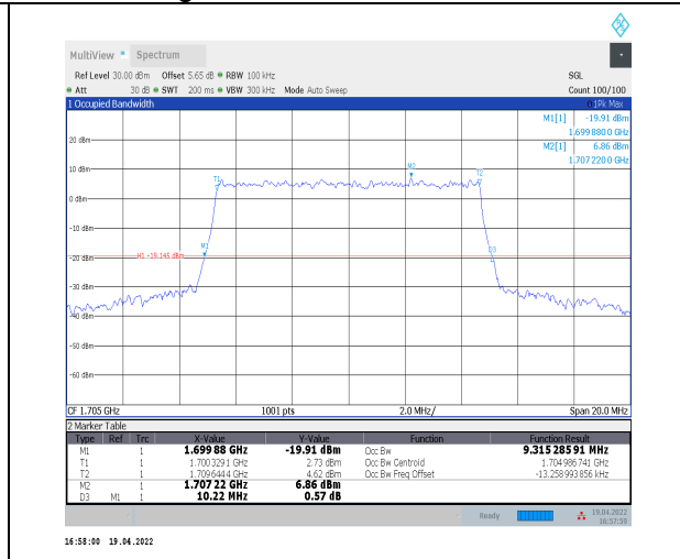
1-N70--15-10-H-9-CP-256QAM-Outer_Full-52@0-An t2-9.315-10.220-≤10-PASS
