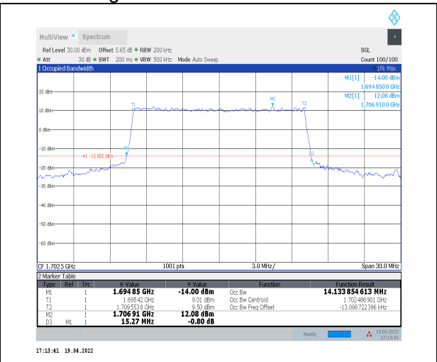
1-N70--15-15-H-6-CP-QPSK-Outer_Full-79@0-Ant2- 14.134-15.270≤15-PASS
