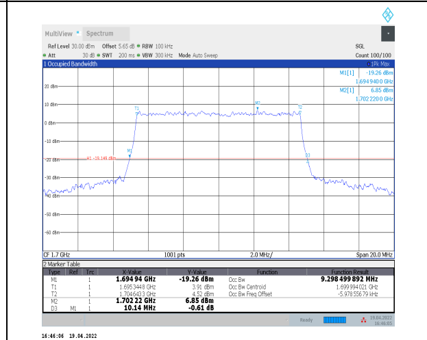
1-N70--15-10-L-9-CP-256QAM-Outer_Full-52@0-An 12-9.298-10.140≤10-PASS
