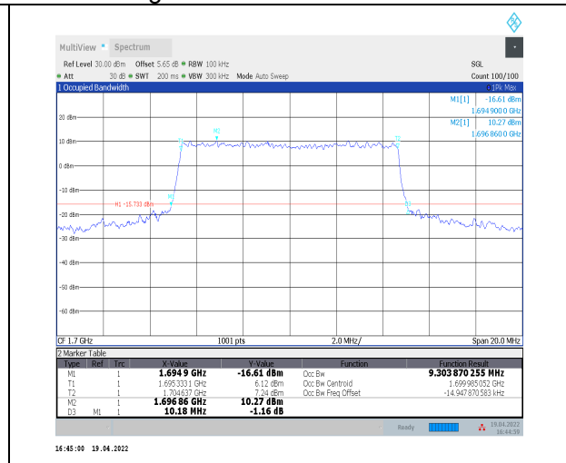
1-N70--15-10-L-7-CP-16QAM-Outer_Full-52@0-Ant 2-9.304-10.180≤10-PASS
