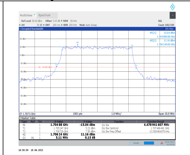
1-N70--15-5-H-4-DFT-64QAM-Outer_Full-25@0-Ant 2-4.479-5.110-<math>\leq</math>5-PASS
