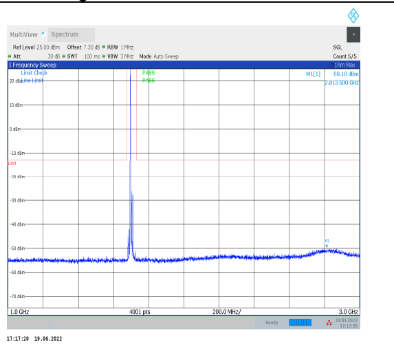
1-N70--15-15-H-1-DFT-PI2BPSK-Inner_1RB_Left-1 @1-1000-3000-Ant2--50.10--13-PASS
