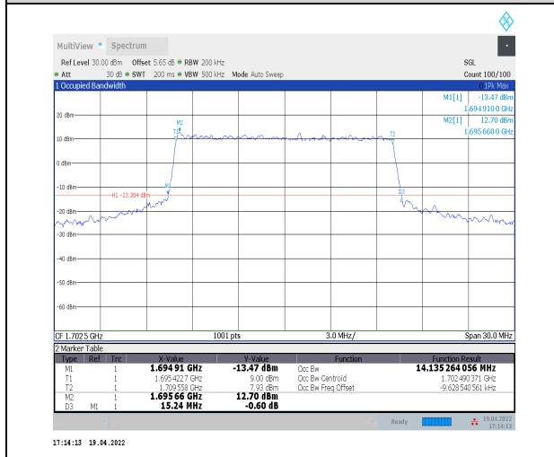
1-N70--15-15-H-7-CP-16QAM-Outer_Full-79@0-Ant 2-14.135-15.240≤15-PASS
