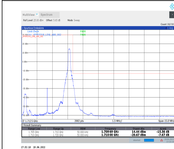
1-N70--15-5-H-5-CP-QPSK-Edge_1RB_Right-1@24-Ant2-seegraph-PASS-see graph
