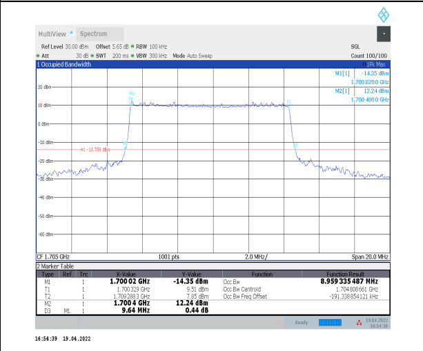
1-N70--15-10-H-3-DFT-16QAM-Outer_Full-50@0-Ant t2-8.959-9.640-<=10-PASS
