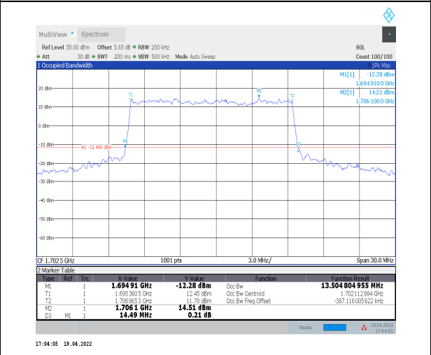
1-N70--15-15-M-1-DFT-QPSK-Outer_Full-75@0-Ant 2-13.505-14.490≤15-PASS
