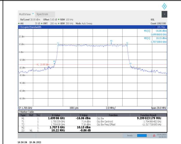
1-N70--15-10-H-7-CP-16QAM-Outer_Full-52@0-Ant 2-9.299-10.220-≤10-PASS
