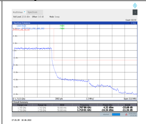
1-N70--15-5-H-3-DFT-PI2BPSK-Outer_Full-25@0-Ant2-seegraph-PASS-see graph
