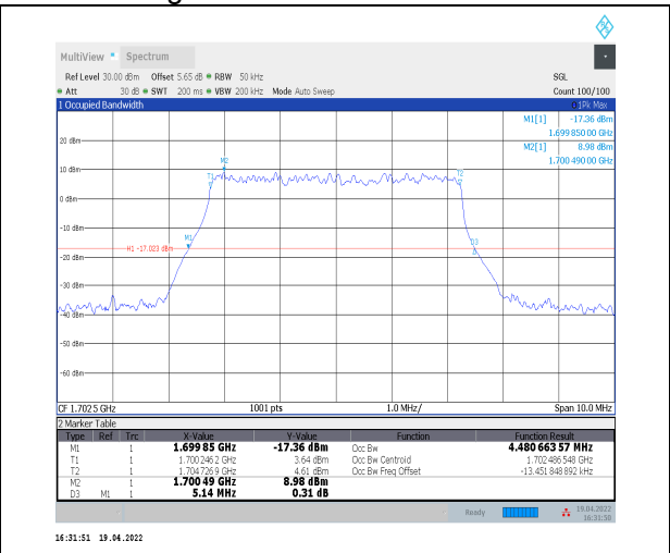
1-N70--15-5-M-5-DFT-256QAM-Outer_Full-25@0-A nt2-4.481-5.140-<math>\leq 5</math>-PASS
