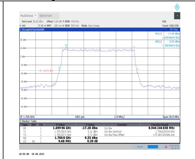
1-N70--15-10-H-5-DFT-256QAM-Outer_Full-50@0-Ant t2-8.946-9.680-≤10-PASS
