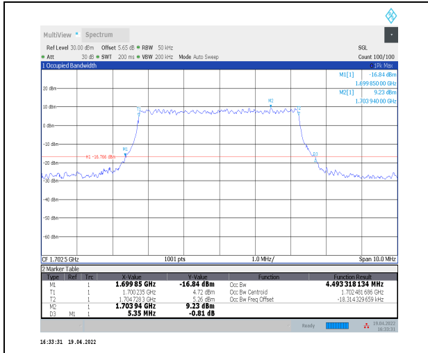
1-N70--15-5-M-8-CP-64QAM-Outer_Full-25@0-Ant2 -4.493-5.350-≤5-PASS
