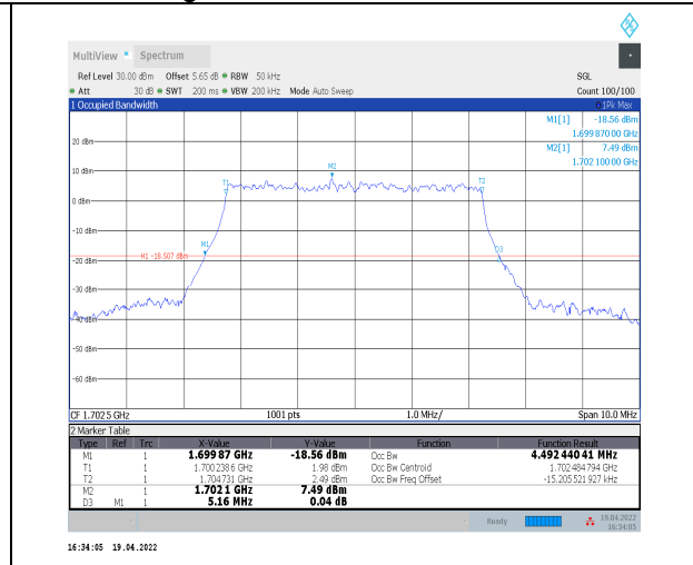
1-N70--15-5-M-9-CP-256QAM-Outer_Full-25@0-Ant 2-4.492-5.160-≤5-PASS
