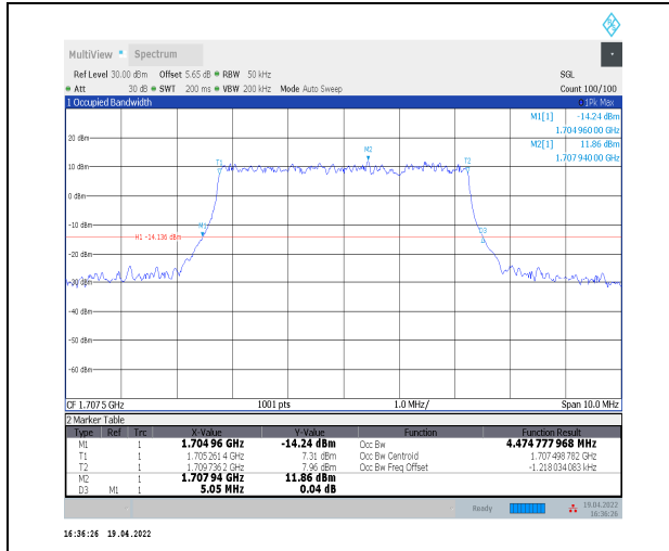
1-N70--15-5-H-3-DFT-16QAM-Outer_Full-25@0-Ant 2-4.475-5.050-<math>\leq</math>5-PASS
