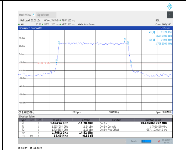
1-N70--15-15-L-2-DFT-PI2BPSK-Outer_Full-75@0-A nt2-13.425-14.490-≤15-PASS
