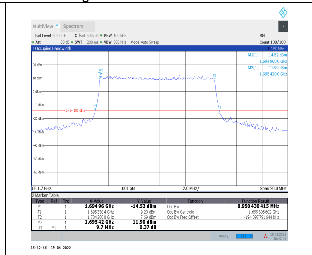
1-N70--15-10-L-3-DFT-16QAM-Outer_Full-50@0-An t2-8.95-9.700-<=10-PASS
