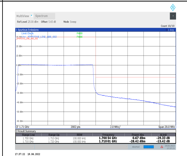
1-N70--15-10-H-6-CP-QPSK-Outer_Full-52@0-An t2-seegraph-PASS-see graph
