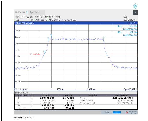
1-N70--15-5-L-5-DFT-25QAM-Outer_Full-25@0-Ant 2-4.481-5.090-<math>\leq 5</math>-PASS
