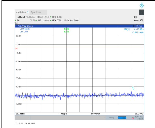
1-N70--15-15-M-1-DFT-PI2BPSK-Inner_1RB_Left-1 @1-0.15-30-Ant2--84.23--33-PASS
