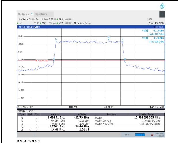
1-N70--15-15-L-1-DFT-QPSK-Outer_Full-75@0-Ant2 -13.505-14.460-≤15-PASS
