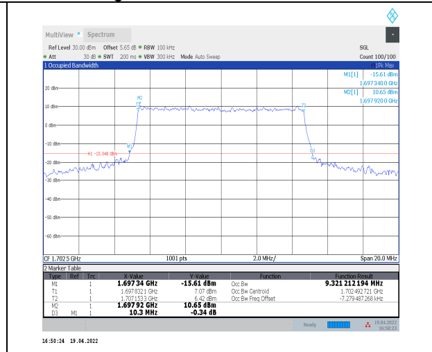
1-N70--15-10-M-6-CP-QPSK-Outer_Full-52@0-Ant2 -9.321-10.300-≤10-PASS
