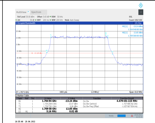
1-N70--15-5-H-2-DFT-PI2BPSK-Outer_Full-25@0-Ant2- 4.479-5.160-≤5-PASS
