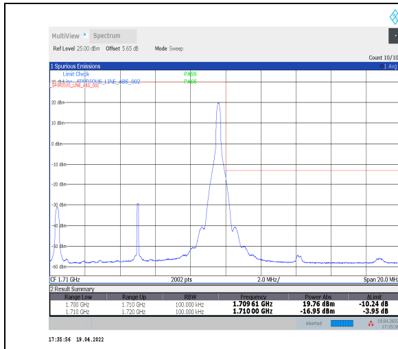
1-N70--15-10-H-2-DFT-PI2BPSK-Edge_1RB_Right-1 @51-Ant2-seegraph-PASS-see graph
