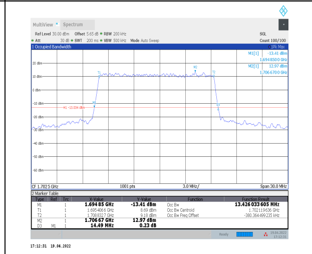
1-N70--15-15-H-4-DFT-64QAM-Outer_Full-75@0-An t2-13.426-14.490≤15-PASS
