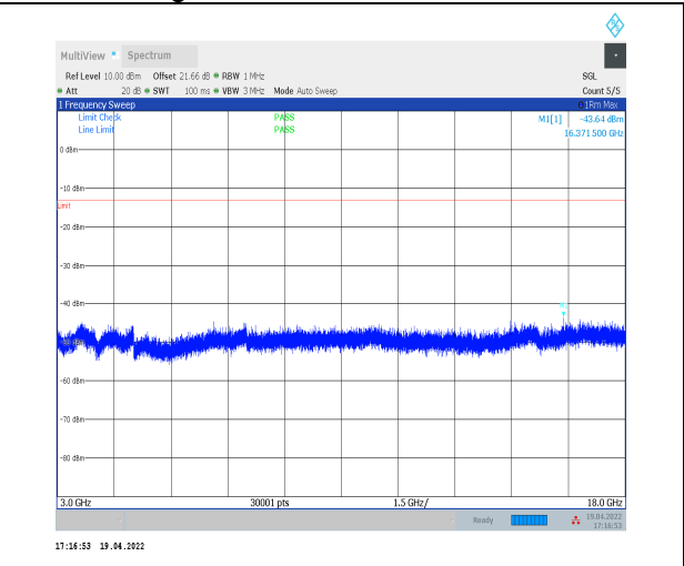
1-N70--15-15-M-1-DFT-PI2BPSK-Inner_1RB_Left-1 @1-3000-18000-Ant2--43.64--13-PASS
