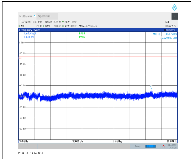
1-N70--15-15-L-1-DFT-PI2BPSK-Inner_1RB_Left-1 @1-3000-18000-Ant2--44.17--13-PASS
