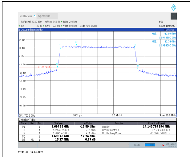
1-N70--15-15-M-6-CP-QPSK-Outer_Full-79@0-Ant2- 14.144-15.270-≤15-PASS
