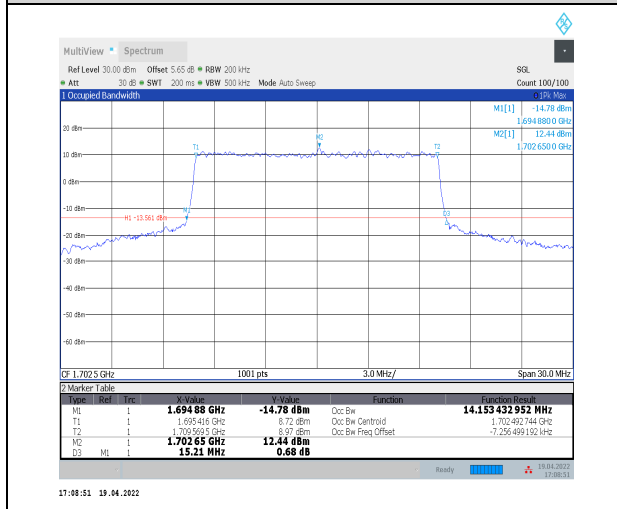
1-N70--15-15-M-8-CP-64QAM-Outer_Full-79@0-Ant 2-14.153-15.210-≤15-PASS
