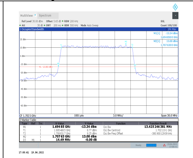
1-N70--15-15-L-4-DFT-64QAM-Outer_Full-75@0-An t2-13.425-14.490-≤15-PASS
