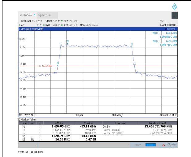
1-N70--15-15-H-3-DFT-16QAM-Outer_Full-75@0-An t2-13.456-14.550≤15-PASS
