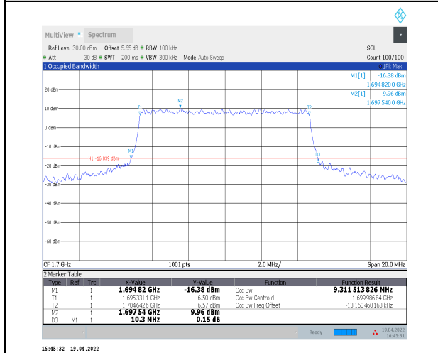
1-N70--15-10-L-8-CP-64QAM-Outer_Full-52@0-Ant2 -9.312-10.300≤10-PASS
