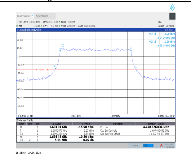
1-N70--15-5-L-6-CP-QPSK-Outer_Full-25@0-Ant2-4 .478-5.110-<math>\leq 5</math>-PASS
