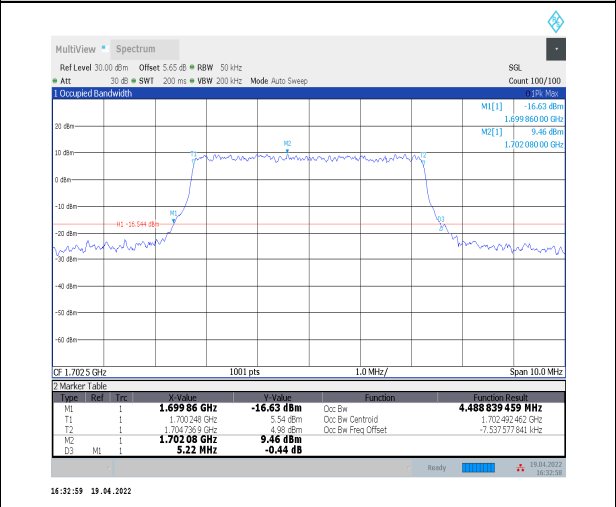
1-N70--15-5-M-7-CP-16QAM-Outer_Full-25@0-Ant2 -4.489-5.220-<math>\leq 5</math>-PASS
