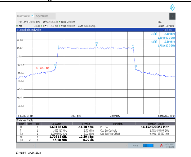
1-N70--15-15-L-8-CP-64QAM-Outer_Full-79@0-Ant 2-14.152-15.180≤15-PASS
