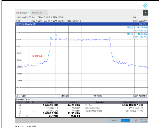
1-N70--15-10-L-4-DFT-64QAM-Outer_Full-50@0-Ant 2-8.942-9.700-<=10-PASS
