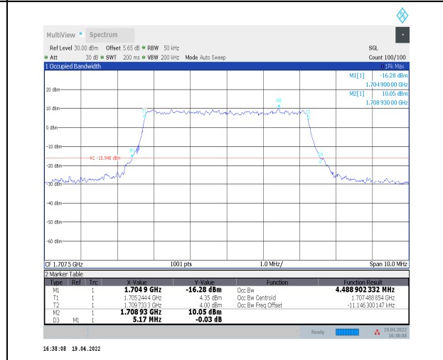
1-N70--15-5-H-6-CP-QPSK-Outer_Full-25@0-Ant2-4 .489-5.170-<math>\leq</math>5-PASS
