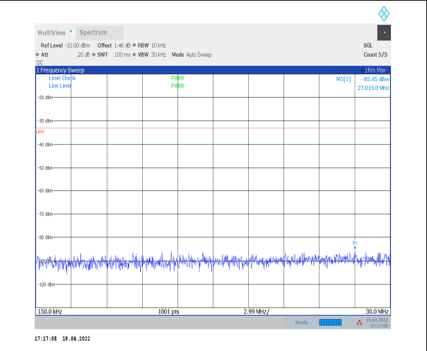
1-N70--15-15-H-1-DFT-PI2BPSK-Inner_1RB_Left-1 @1-0.15-30-Ant2--85.45--33-PASS
