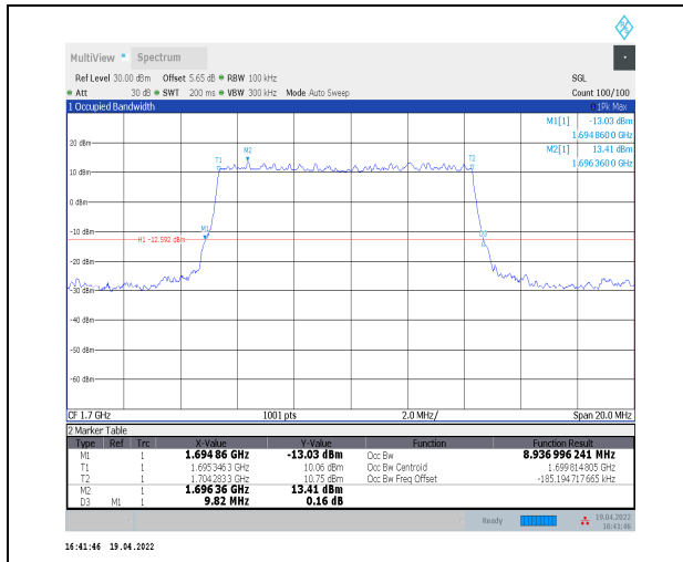
1-N70--15-10-L-2-DFT-PI2BPSK-Outer_Full-50@0-A nt2-8.937-9.820-<=10-PASS
