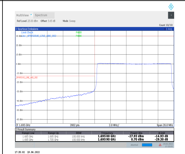
1-N70--15-10-L-6-CP-QPSK-Outer_Full-52@0-Ant 2-seegraph-PASS-see graph
