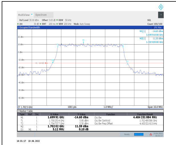
1-N70--15-5-M-4-DFT-64QAM-Outer_Full-25@0-Ant 2-4.484-5.120-<math>\leq 5</math>-PASS
