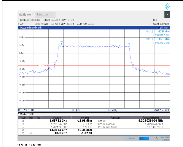
1-N70--15-10-M-7-CP-16QAM-Outer_Full-52@0-Ant 2-9.305-10.300-≤10-PASS
