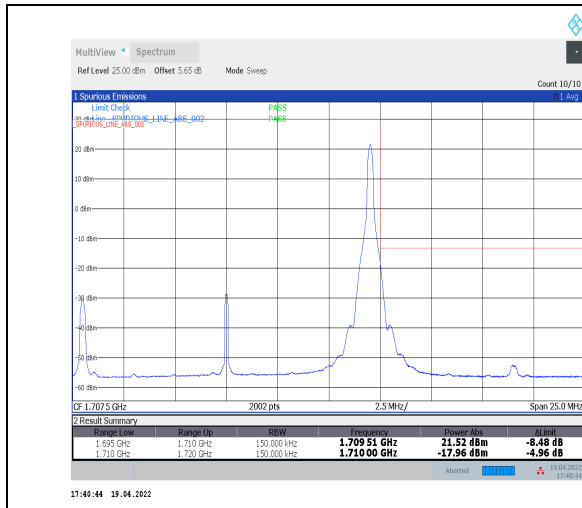
1-N70--15-15-H-2-DFT-PI2BPSK-Edge_1RB_Right-1 @78-Ant2-seegraph-PASS-see graph
