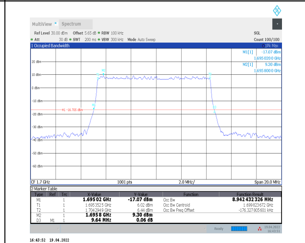
1-N70--15-10-L-5-DFT-256QAM-Outer_Full-50@0-A nt2-8.942-9.640-<=10-PASS
