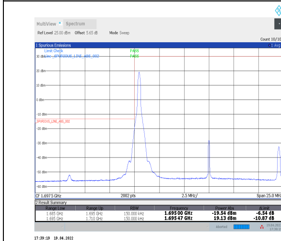
1-N70--15-15-L-4-CP-QPSK-Edge_1RB_Left-1@0-Ant 2-seegraph-PASS-see graph
