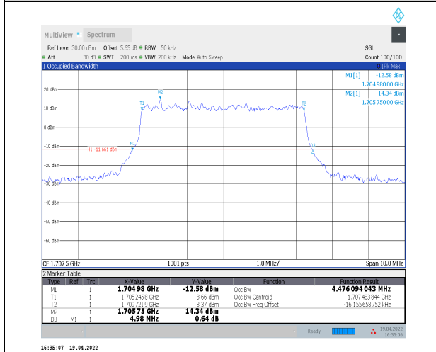
1-N70--15-5-H-1-DFT-QPSK-Outer_Full-25@0-Ant2- 4.476-4.980-≤5-PASS
