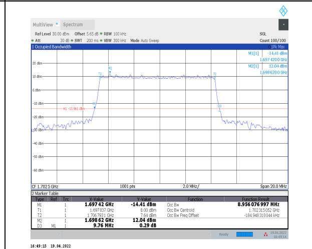
1-N70--15-10-M-4-DFT-64QAM-Outer_Full-50@0-A nt2-8.956-9.760≤10-PASS
