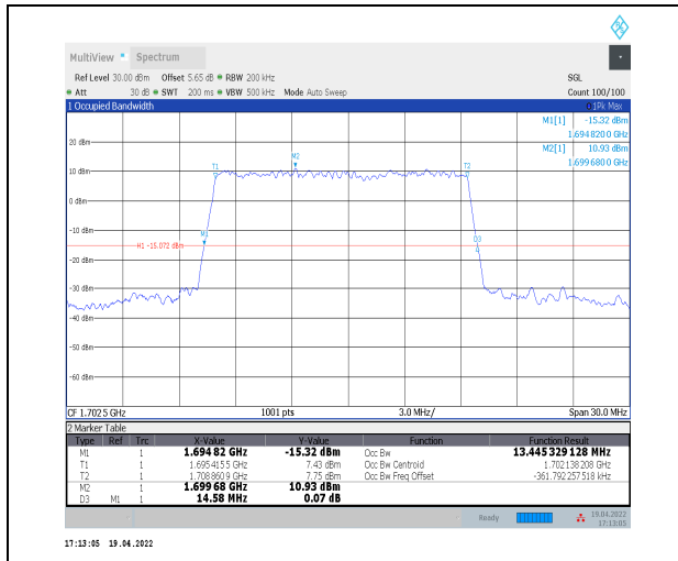
1-N70--15-15-H-5-DFT-256QAM-Outer_Full-75@0-A nt2-13.445-14.580≤15-PASS
