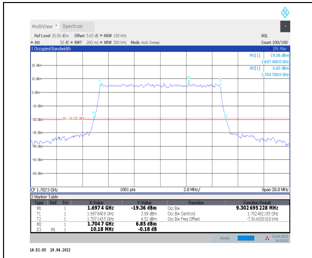
1-N70--15-10-M-9-CP-256QAM-Outer_Full-52@0-An t2-9.303-10.180-<=10-PASS
