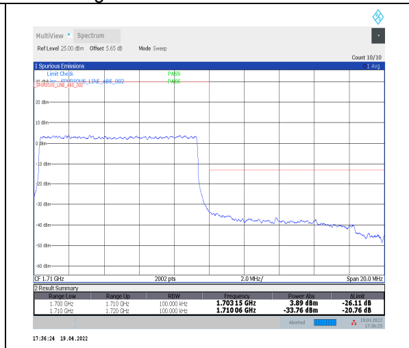
1-N70--15-10-H-3-DFT-PI2BPSK-Outer_Full-50@ 0-Ant2-seegraph-PASS-see graph
