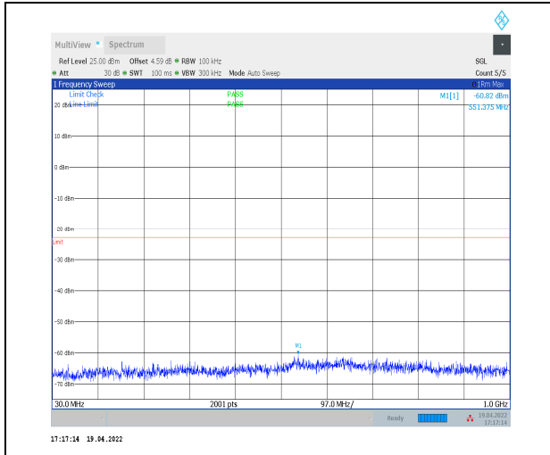
1-N70--15-15-H-1-DFT-PI2BPSK-Inner_1RB_Left-1 @1-30-1000-Ant2--60.82--23-PASS
