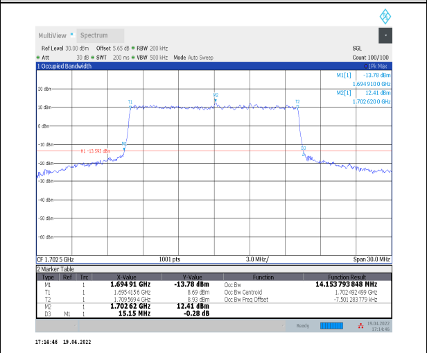
1-N70--15-15-H-8-CP-64QAM-Outer_Full-79@0-Ant 2-14.154-15.150≤15-PASS
