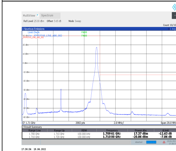
1-N70--15-10-H-5-CP-QPSK-Edge_1RB_Right-1@51- Ant2-seegraph-PASS-see graph
