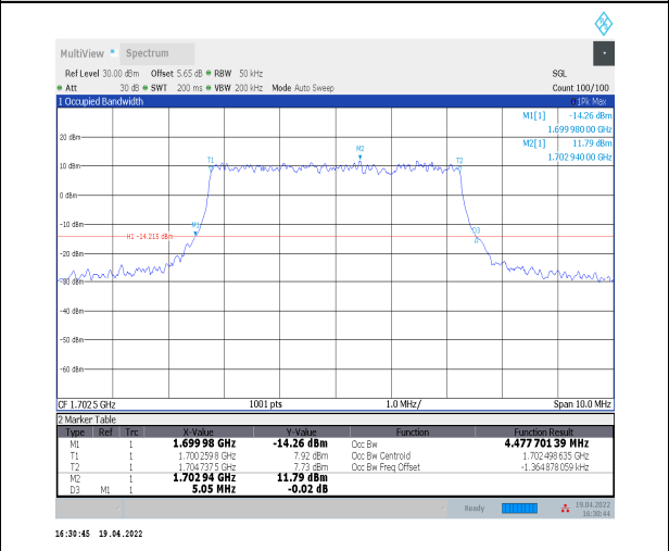
1-N70--15-5-M-3-DFT-16QAM-Outer_Full-25@0-Ant 2-4.478-5.050-≤5-PASS
