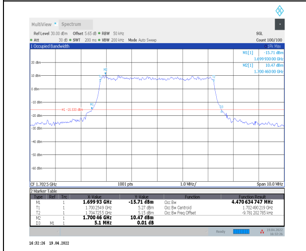
1-N70--15-5-M-6-CP-QPSK-Outer_Full-25@0-Ant2-4 .471-5.100-<math>\leq 5</math>-PASS
