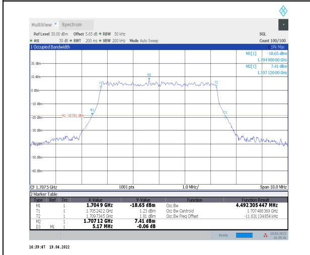
1-N70--15-5-H-9-CP-256QAM-Outer_Full-25@0-Ant 2-4.492-5.170<=5-PASS
