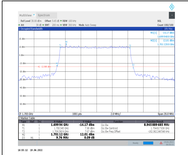
1-N70--15-10-H-4-DFT-64QAM-Outer_Full-50@0-Ant t2-8.946-9.760-≤10-PASS
