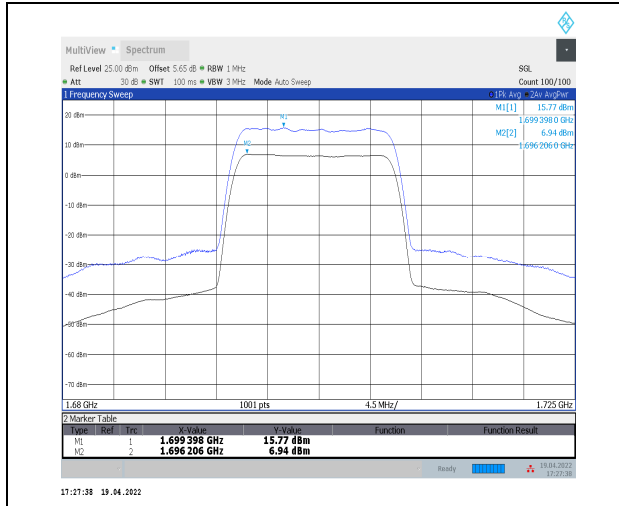
1-N70--15-15-H-1-DFT-256QAM-Outer_Full-75@0-A nt2-8.83-100%-0.00-8.83-PASS-≤13
