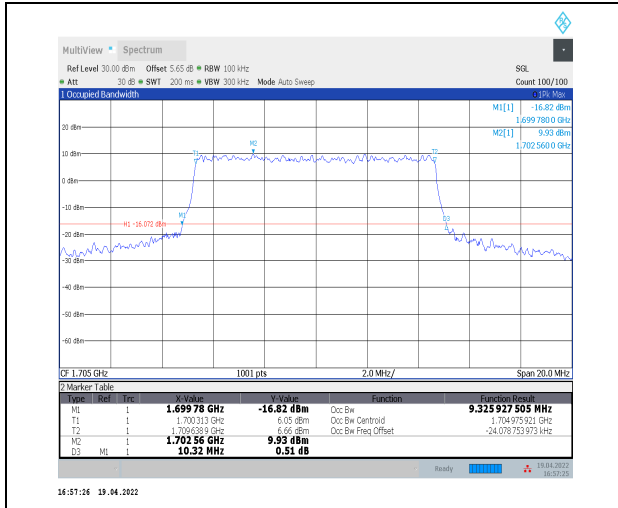
1-N70--15-10-H-8-CP-64QAM-Outer_Full-52@0-Ant 2-9.326-10.320-≤10-PASS
