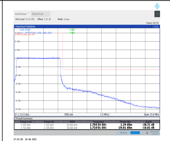
1-N70--15-5-H-6-CP-QPSK-Outer_Full-25@0-Ant2-seegraph-PASS-see graph
