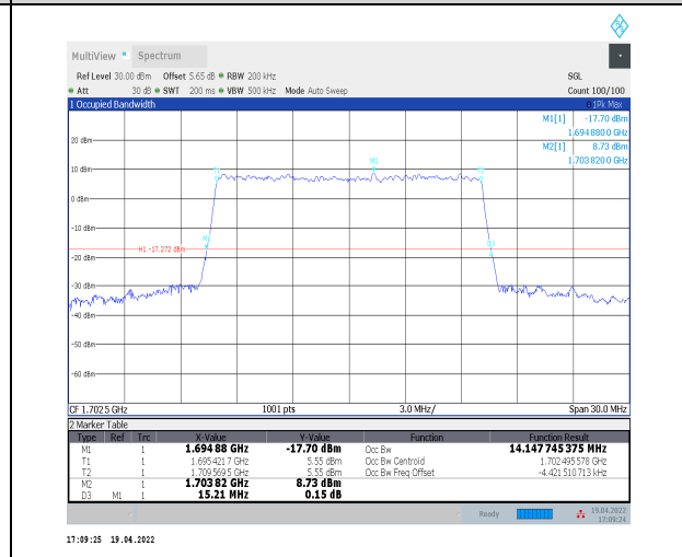
1-N70--15-15-M-9-CP-256QAM-Outer_Full-79@0-A nt2-14.148-15.210-≤15-PASS
