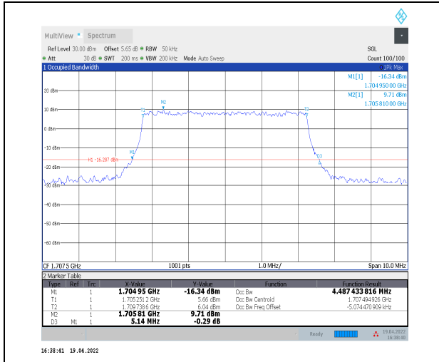
1-N70--15-5-H-7-CP-16QAM-Outer_Full-25@0-Ant2- 4.487-5.140<=5-PASS
