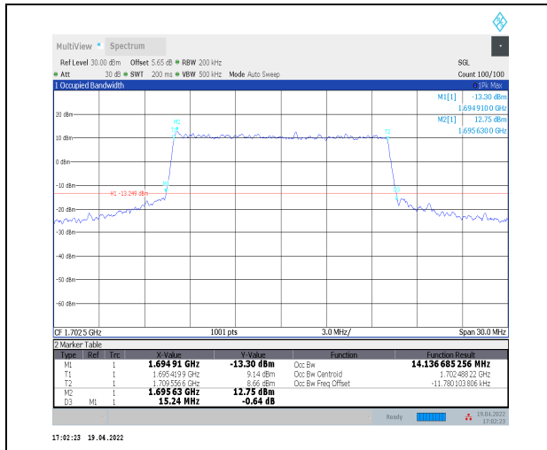
1-N70--15-15-L-7-CP-16QAM-Outer_Full-79@0-Ant2 -14.137-15.240≤15-PASS
