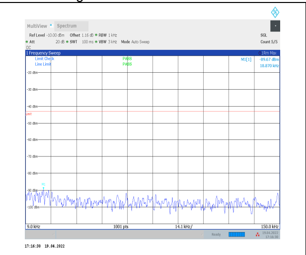
1-N70--15-15-M-1-DFT-PI2BPSK-Inner_1RB_Left-1 @1-0.009-0.15-Ant2--89.67--43-PASS
