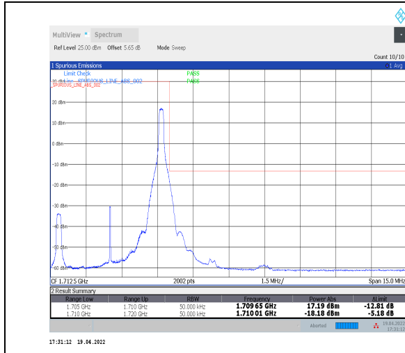
1-N70--15-5-H-2-DFT-PI2BPSK-Edge_1RB_Right-1@24-Ant2-seegraph-PASS-see graph
