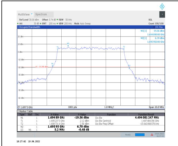
1-N70--15-5-L-9-CP-256QAM-Outer_Full-25@0-Ant2 -4.494-5.200-≤5-PASS
