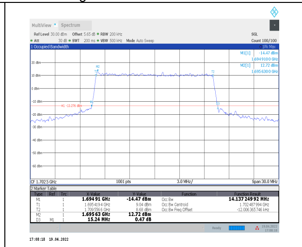
1-N70--15-15-M-7-CP-16QAM-Outer_Full-79@0-Ant 2-14.137-15.240-≤15-PASS
