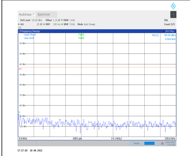
1-N70--15-15-H-1-DFT-PI2BPSK-Inner_1RB_Left-1 @1-0.009-0.15-Ant2--89.58--43-PASS
