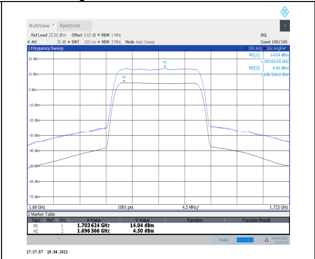
1-N70--15-15-H-2-CP-256QAM-Outer_Full-79@0-A nt2-9.54-100%-0.00-9.54-PASS-≤13
