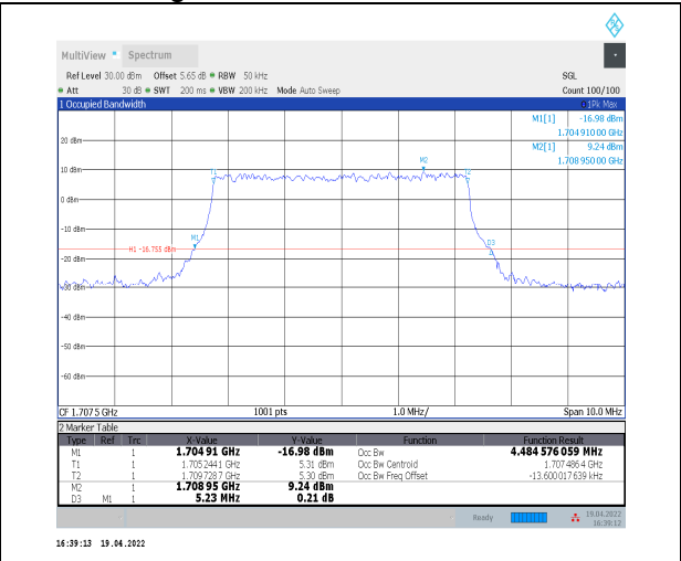
1-N70--15-5-H-8-CP-64QAM-Outer_Full-25@0-Ant2 -4.485-5.230<=5-PASS
