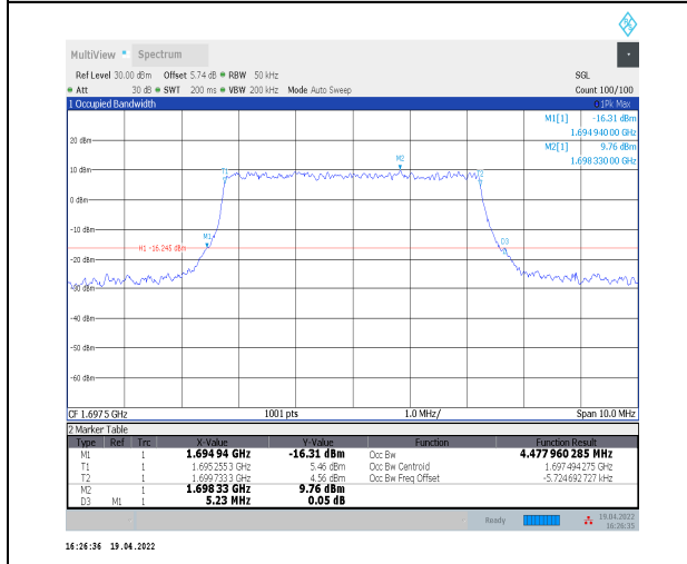
1-N70--15-5-L-7-CP-16QAM-Outer_Full-25@0-Ant2- 4.478-5.230-<math>\leq 5</math>-PASS
