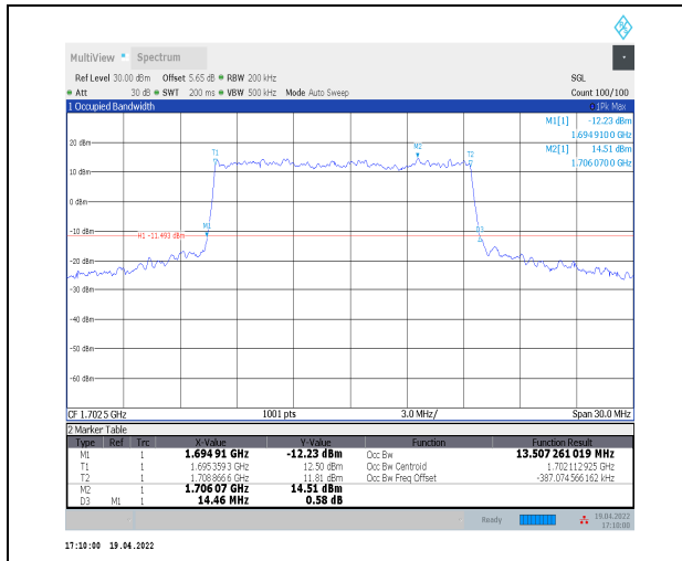
1-N70--15-15-H-1-DFT-QPSK-Outer_Full-75@0-Ant 2-13.507-14.460≤15-PASS
