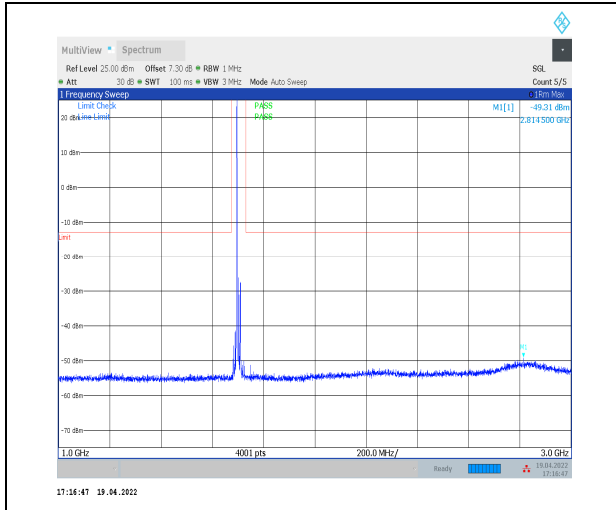
1-N70--15-15-M-1-DFT-PI2BPSK-Inner_1RB_Left-1 @1-1000-3000-Ant2--49.31--13-PASS
