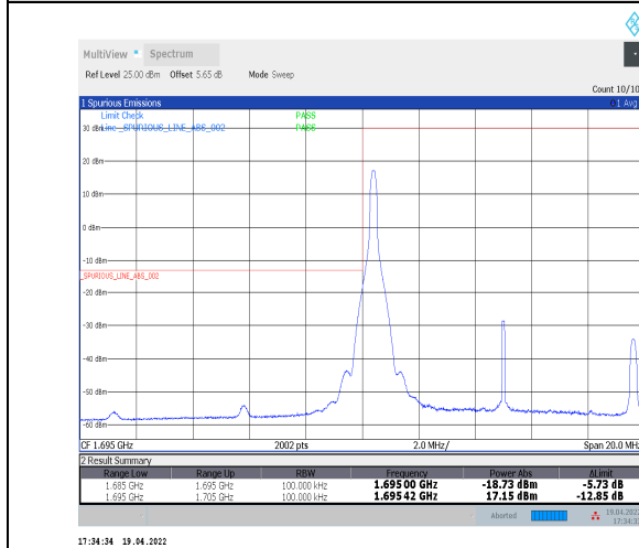
1-N70--15-10-L-4-CP-QPSK-Edge_1RB_Left-1@0-Ant 2-seegraph-PASS-see graph
