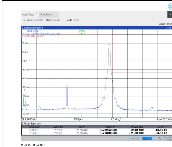
1-N70--15-15-H-5-CP-QPSK-Edge_1RB_Right-1@78-Ant2-seegraph-PASS-see graph
