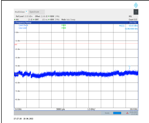
1-N70--15-15-H-1-DFT-PI2BPSK-Inner_1RB_Left-1 @1-3000-18000-Ant2--43.65--13-PASS
