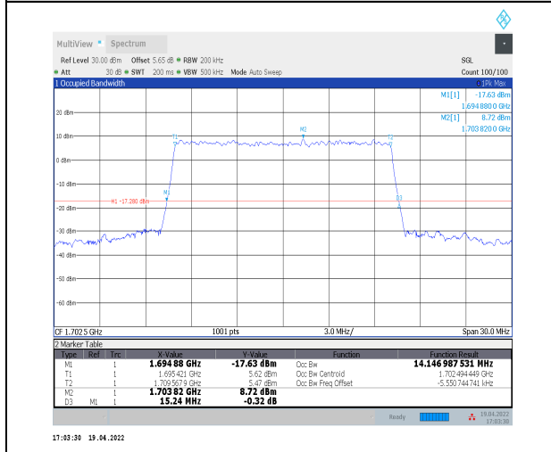
1-N70--15-15-L-9-CP-256QAM-Outer_Full-79@0-Ant 2-14.147-15.240≤15-PASS
