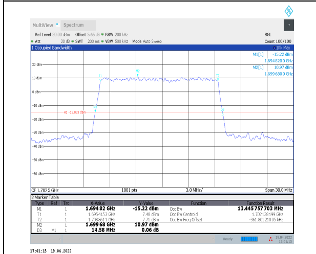
1-N70--15-15-L-5-DFT-256QAM-Outer_Full-75@0-A nt2-13.446-14.580-≤15-PASS
