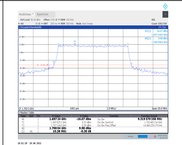
1-N70--15-10-M-8-CP-64QAM-Outer_Full-52@0-Ant 2-9.32-10.380-≤10-PASS
