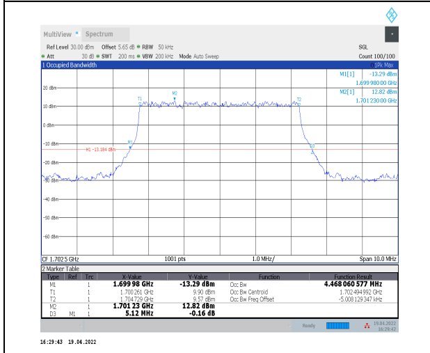
1-N70--15-5-M-2-DFT-PI2BPSK-Outer_Full-25@0-A nt2-4.468-5.120-≤5-PASS
