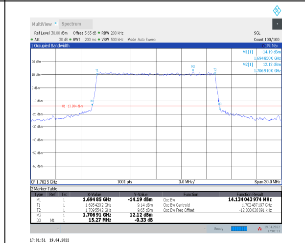
1-N70--15-15-L-6-CP-QPSK-Outer_Full-79@0-Ant2- 14.134-15.270-≤15-PASS
