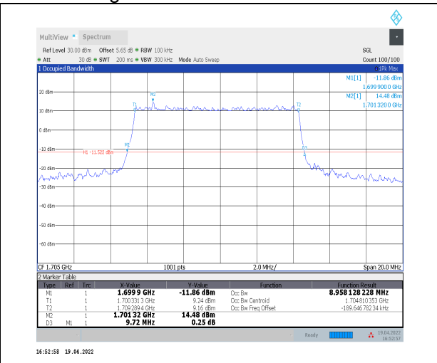
1-N70--15-10-H-1-DFT-QPSK-Outer_Full-50@0-Ant 2-8.958-9.720-<=10-PASS
