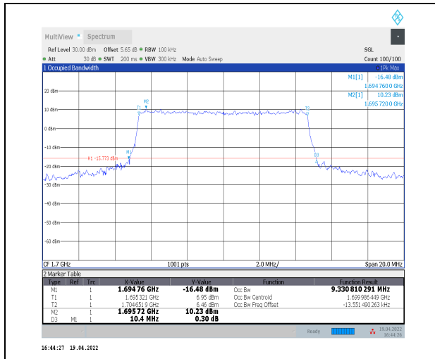
1-N70--15-10-L-6-CP-QPSK-Outer_Full-52@0-Ant2 9.331-10.400≤10-PASS
