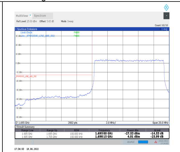
1-N70--15-10-L-3-DFT-PI2BPSK-Outer_Full-50@0 -Ant2-seegraph-PASS-see graph
