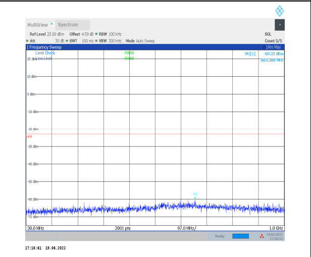
1-N70--15-15-M-1-DFT-PI2BPSK-Inner_1RB_Left-1 @1-30-1000-Ant2--60.33--23-PASS
