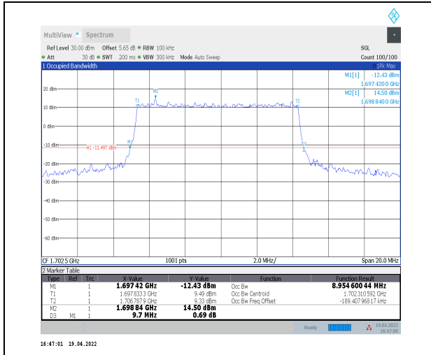
1-N70--15-10-M-1-DFT-QPSK-Outer_Full-50@0-Ant 2-8.955-9.700≤10-PASS
