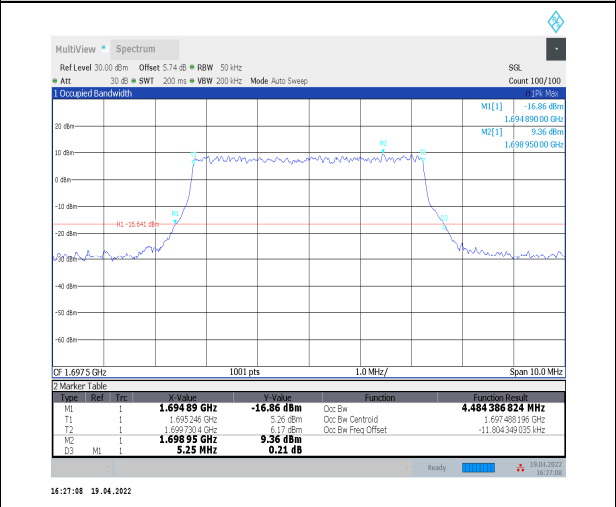
1-N70--15-5-L-8-CP-64QAM-Outer_Full-25@0-Ant2- 4.484-5.250-<math>\leq 5</math>-PASS
