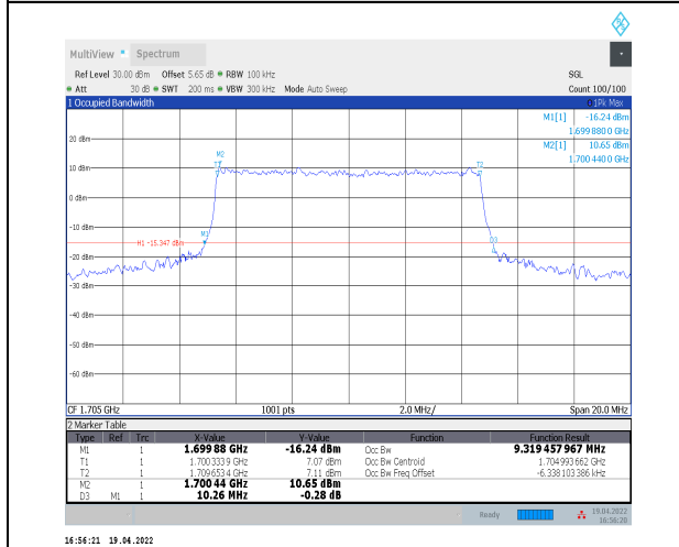
1-N70--15-10-H-6-CP-QPSK-Outer_Full-52@0-Ant2- 9.319-10.260-≤10-PASS
