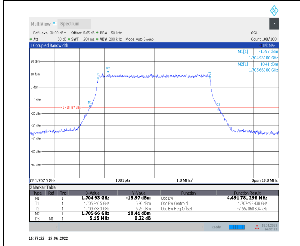
1-N70--15-5-H-5-DFT-256QAM-Outer_Full-25@0-Ant t2-4.492-5.150-<math>\leq</math>5-PASS
