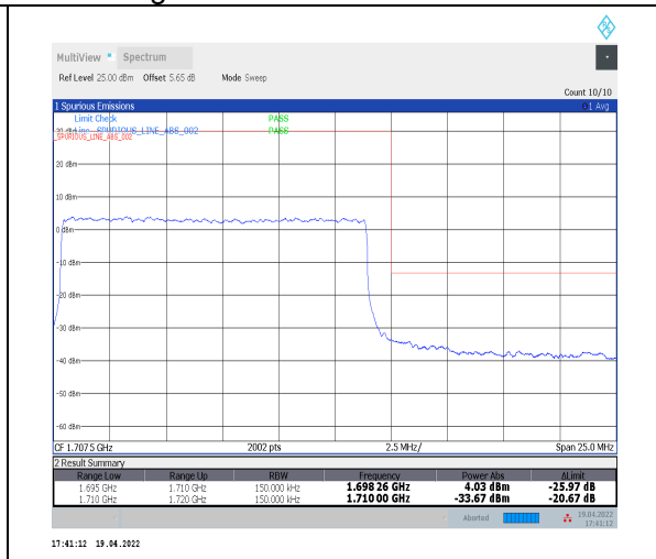
1-N70--15-15-H-3-DFT-PI2BPSK-Outer_Full-75@0-Ant2-seegraph-PASS-see graph
