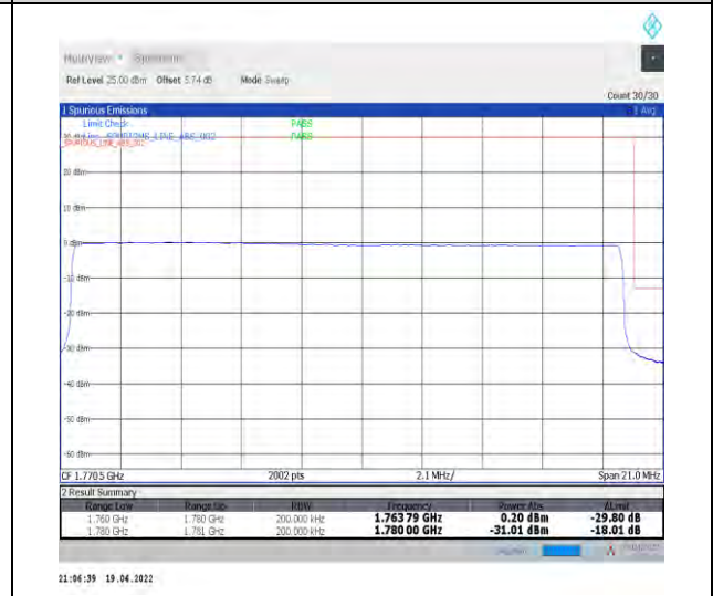
1-N66-PC3-15-20-H-6-CP-QPSK-Outer_Full-106@0-Ant0-seegraph-PASS-see graph
