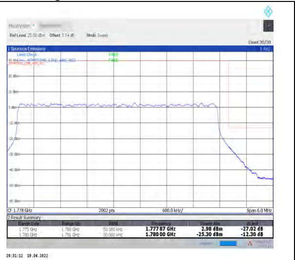
1-N66-PC3-15-5-H-3-DFT-PI2BPSK-Outer_Full-25@0-Ant0-seegraph-PASS-see graph
