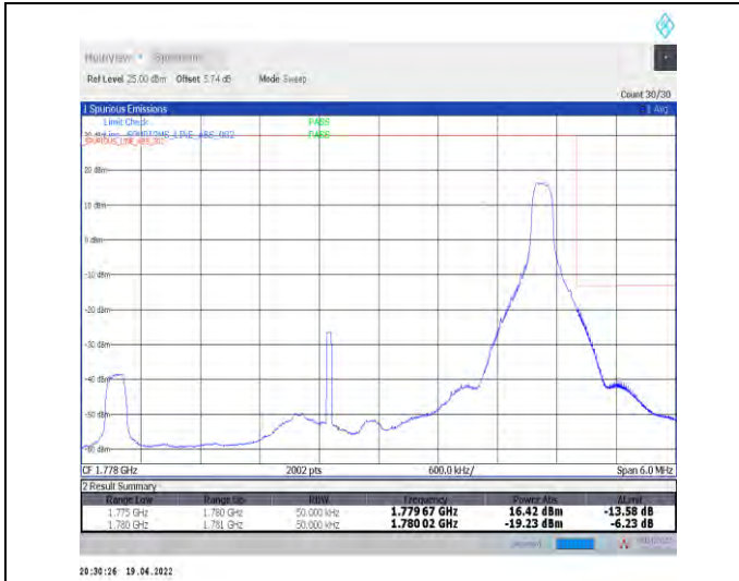
1-N66-PC3-15-5-H-2-DFT-PI2BPSK-Edge_1RB_Right-1@24-Ant0-seegraph-PASS-see graph
