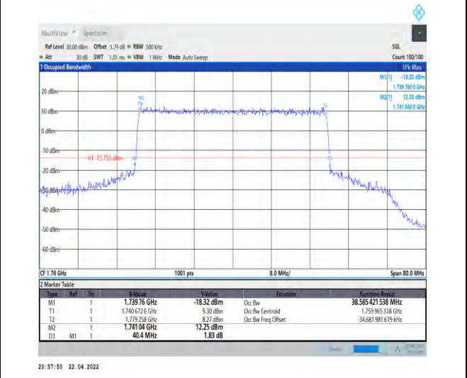
1-N66-PC3-15-40-H-7-CP-16QAM-Outer_Full-216@0 -Ant0-38.585-40.400-≤40-PASS
