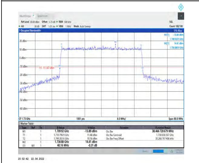
1-N66-PC3-15-40-L-4-DFT-64QAM-Outer_Full-216 @0-Ant0-38.467-40.160-≤40-PASS
