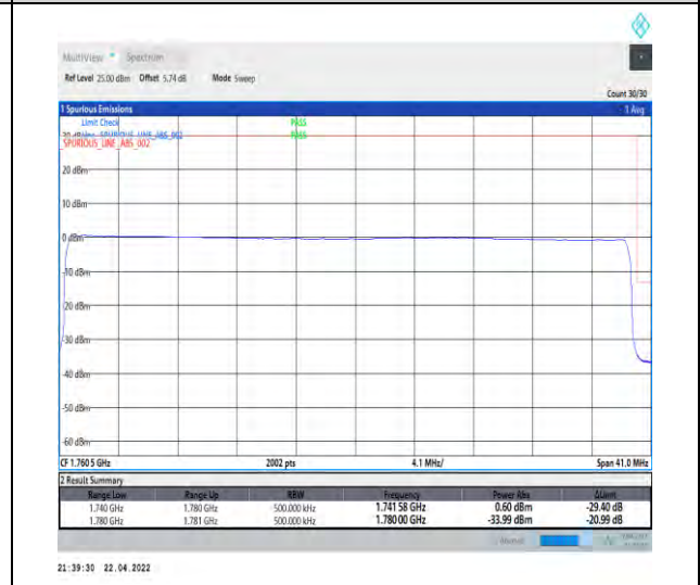
1-N66-PC3-15-40-H-6-CP-QPSK-Outer_Full-216@0-Ant0-seegraph-PASS-see graph
