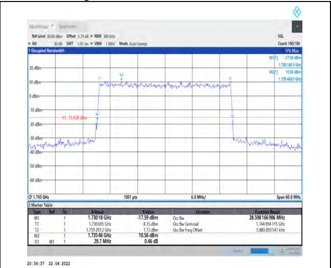
1-N66-PC3-15-30-M-5-DFT-256QAM-Outer_Full-160 @0-Ant0-28.598-29.700-≤30-PASS
