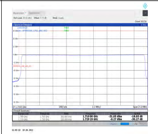
1-N66-PC3-15-20-L-6-CP-QPSK-Outer_Full-106@0-Ant0-seegraph-PASS-see graph
