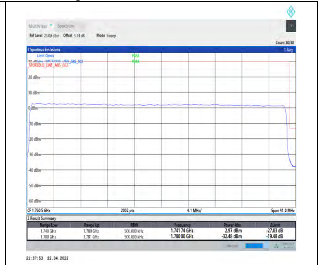
1-N66-PC3-15-40-H-3-DFT-PI2BPSK-Outer_Full-216@0-Ant0-seegraph-PASS-see graph
