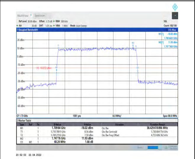
1-N66-PC3-15-40-L-5-DFT-256QAM-Outer_Full-216 @0-Ant0-38.43-40.240-≤40-PASS
