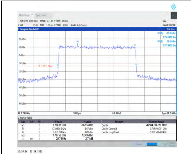
1-N66-PC3-15-30-M-4-DFT-64QAM-Outer_Full-160 @0-Ant0-28.584-29.700-≤30-PASS
