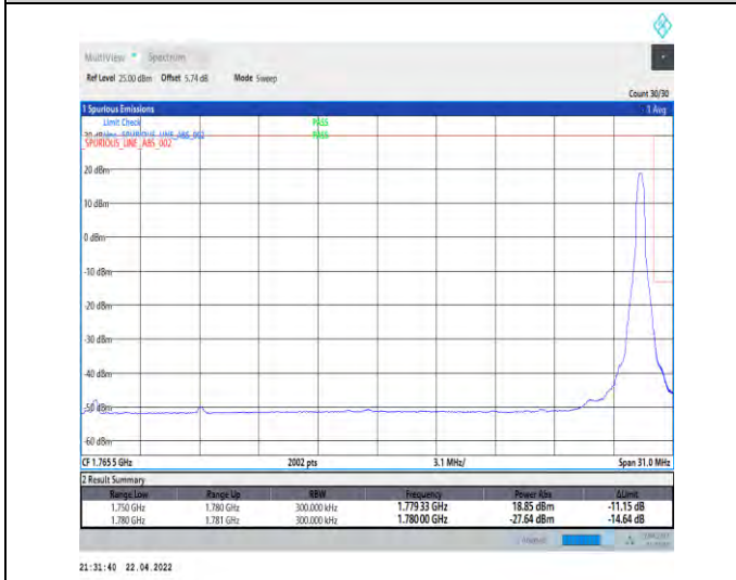
1-N66-PC3-15-30-H-5-CP-QPSK-Edge_1RB_Right-1 @159-Ant0-seegraph-PASS-see graph
