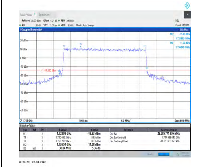
1-N66-PC3-15-30-M-6-CP-QPSK-Outer_Full-160@0 -Ant0-28.586-30.840-≤30-PASS
