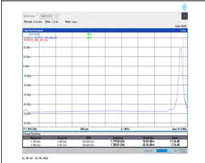
1-N66-PC3-15-40-H-5-CP-QPSK-Edge_1RB_Right-1@215-Ant0-seegraph-PASS-see graph
