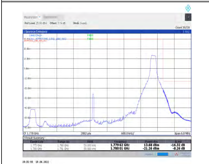
1-N66-PC3-15-5-H-5-CP-QPSK-Edge_1RB_Right-1@24-Ant0-seegraph-PASS-see graph
