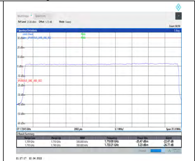
1-N66-PC3-15-30-L-3-DFT-PI2BPSK-Outer_Full-160@0-Ant0-seegraph-PASS-see graph
