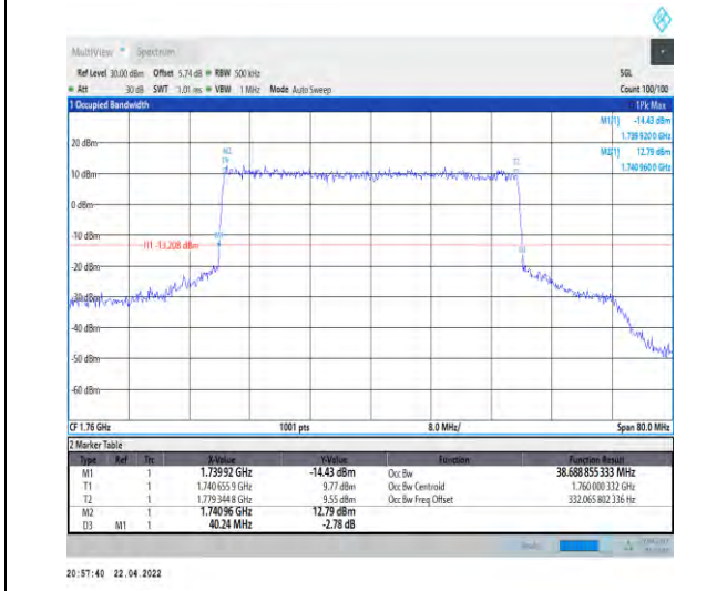
1-N66-PC3-15-40-H-6-CP-QPSK-Outer_Full-216@0 -Ant0-38.689-40.240-≤40-PASS
