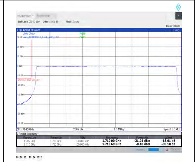
1-N66-PC3-15-10-L-6-CP-QPSK-Outer_Full-52@0-Ant0-seegraph-PASS-see graph
