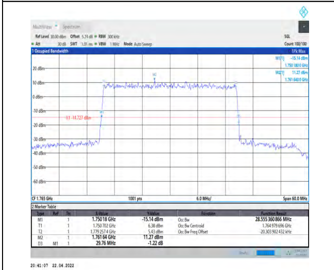
1-N66-PC3-15-30-H-5-DFT-256QAM-Outer_Full-160 @0-Ant0-28.555-29.760-≤30-PASS
