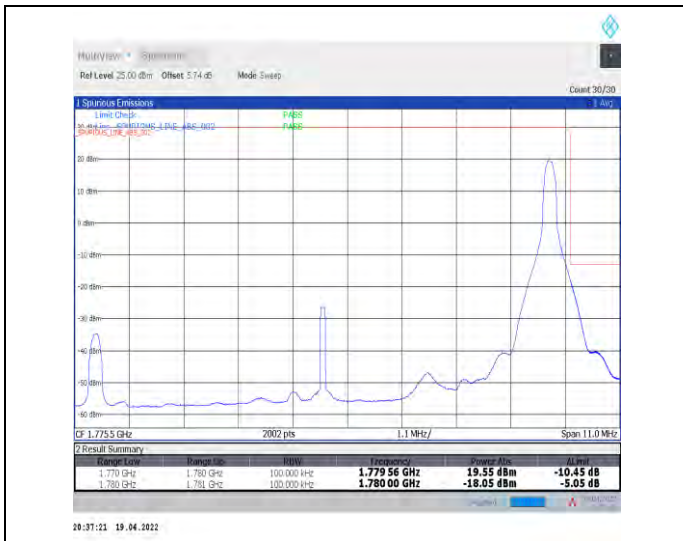
1-N66-PC3-15-10-H-2-DFT-PI2BPSK-Edge_1RB_Right-t-1@51-Ant0-seegraph-PASS-see graph
