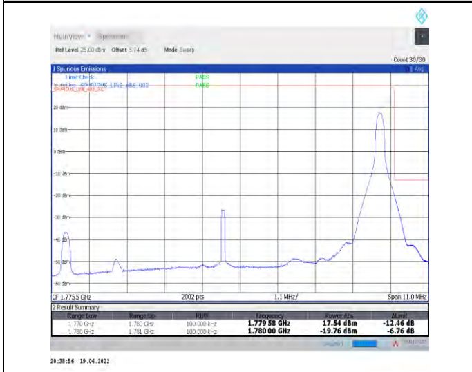
1-N66-PC3-15-10-H-5-CP-QPSK-Edge_1RB_Right-1@51-Ant0-seegraph-PASS-see graph
