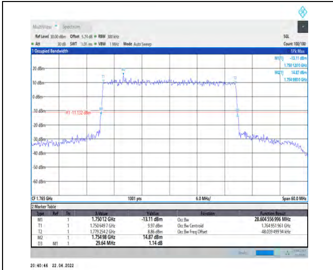
1-N66-PC3-15-30-H-3-DFT-16QAM-Outer_Full-160 @0-Ant0-28.605-29.640-≤30-PASS
