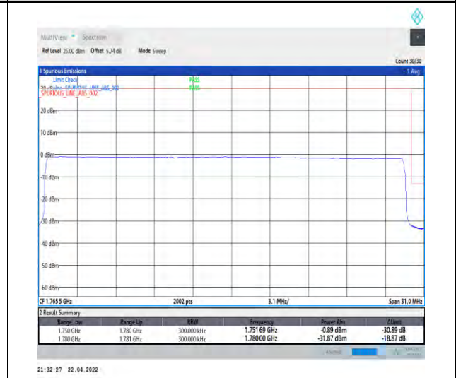
1-N66-PC3-15-30-H-6-CP-QPSK-Outer_Full-160 @0-Ant0-seegraph-PASS-see graph
