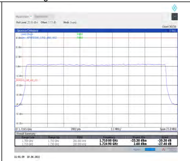
1-N66-PC3-15-20-L-3-DFT-PI2BPSK-Outer_Full-100@0-Ant0-seegraph-PASS-see graph
