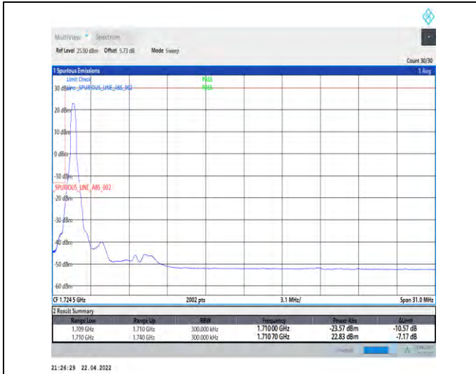
1-N66-PC3-15-30-L-1-DFT-PI2BPSK-Edge_1RB_Left-1@0-Ant0-seegraph-PASS-see graph
