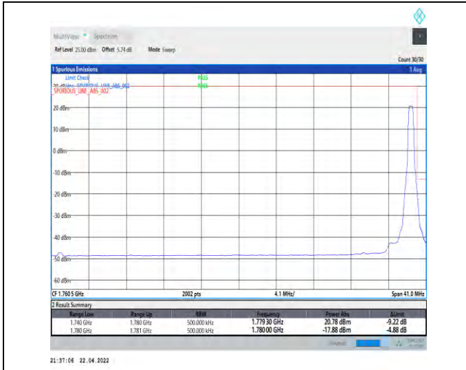
1-N66-PC3-15-40-H-2-DFT-PI2BPSK-Edge_1RB_Right-t-1@215-Ant0-seegraph-PASS-see graph
