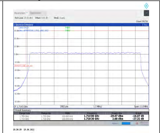
1-N66-PC3-15-10-L-3-DFT-PI2BPSK-Outer_Full-50@0-Ant0-seegraph-PASS-see graph
