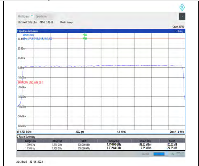
1-N66-PC3-15-40-L-3-DFT-PI2BPSK-Outer_Full-216@0-Ant0-seegraph-PASS-see graph
