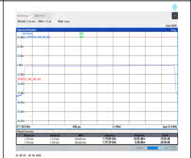
1-N66-PC3-15-30-L-6-CP-QPSK-Outer_Full-160@0-Ant0-seegraph-PASS-see graph
