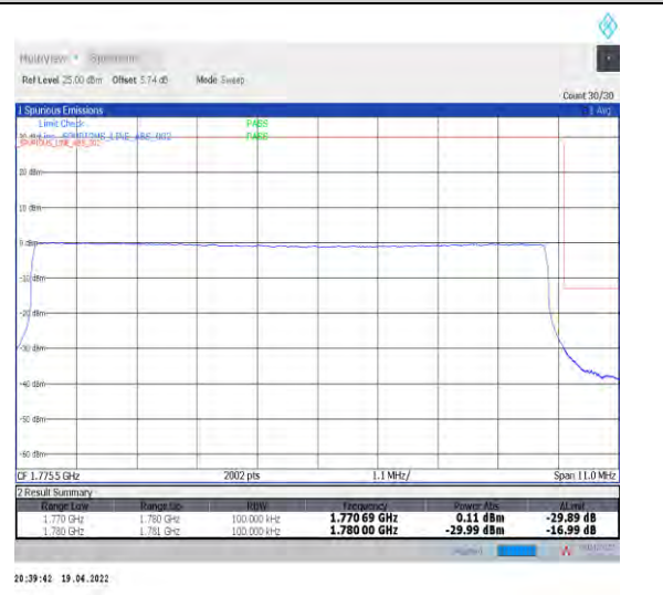
1-N66-PC3-15-10-H-6-CP-QPSK-Outer_Full-52@0-Ant0-seegraph-PASS-see graph
