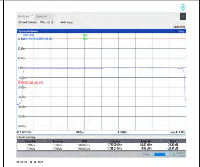
1-N66-PC3-15-40-L-6-CP-QPSK-Outer_Full-216@0-Ant0-seegraph-PASS-see graph
