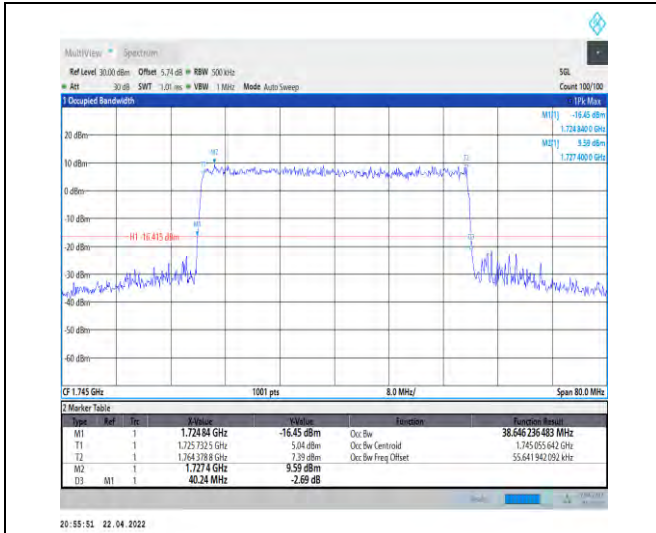
1-N66-PC3-15-40-M-9-CP-256QAM-Outer_Full-216 @0-Ant0-38.646-40.240-≤40-PASS
