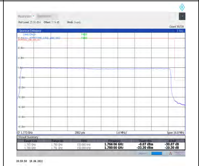
1-N66-PC3-15-15-H-6-CP-QPSK-Outer_Full-79@0-Ant0-seegraph-PASS-see graph
