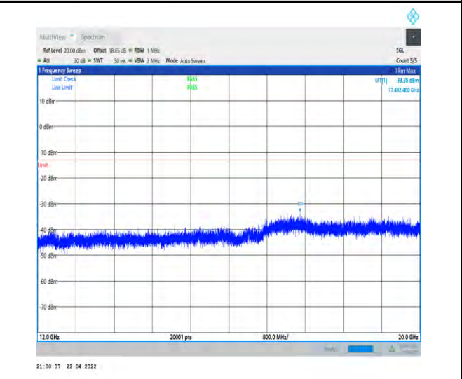
1-N66-PC3-15-40-M-1-DFT-PI2BPSK-Inner_1RB_Le ft-1@1-12000-20000-Ant0--33.38--13-PASS
