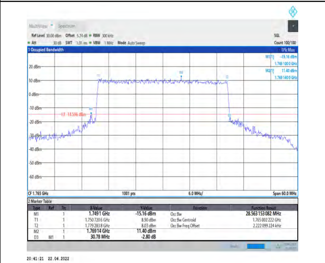
1-N66-PC3-15-30-H-6-CP-QPSK-Outer_Full-160 @0-Ant0-28.563-30.780-≤30-PASS
