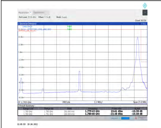
1-N66-PC3-15-20-H-5-CP-QPSK-Edge_1RB_Right-1@105-Ant0-seegraph-PASS-see graph
