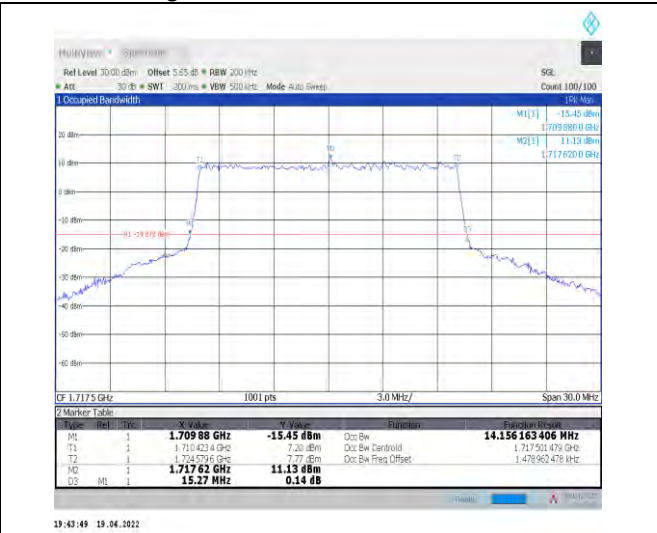
1-N66-PC3-15-15-L-8-CP-64QAM-Outer_Full-79@0-Ant0-14.156-15.270-≤15-PASS
