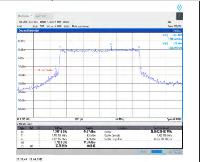
1-N66-PC3-15-30-L-6-CP-QPSK-Outer_Full-160@0-Ant0-28.568-30.780-≤30-PASS
