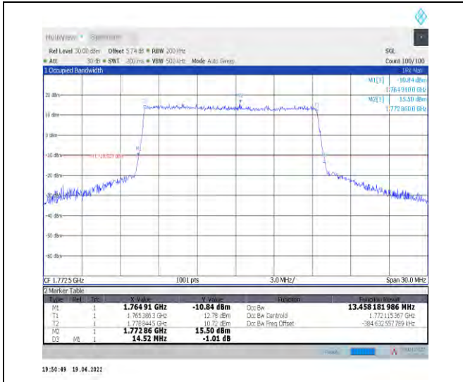
1-N66-PC3-15-15-H-1-DFT-QPSK-Outer_Full-75@0-Ant0-13.458-14.520-≤15-PASS
