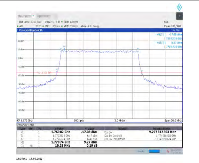
1-N66-PC3-15-10-H-7-CP-16QAM-Outer_Full-52@0 -Ant0-9.298-10.280-≤10-PASS
