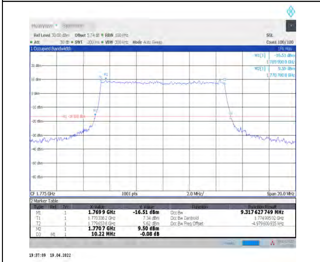
1-N66-PC3-15-10-H-6-CP-QPSK-Outer_Full-52@0- Ant0-9.318-10.220-≤10-PASS
