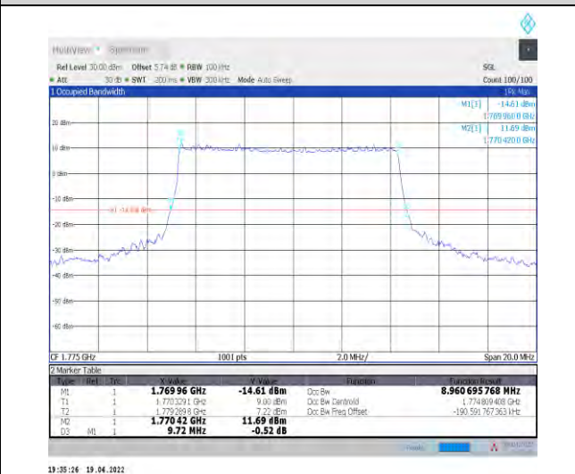
1-N66-PC3-15-10-H-3-DFT-16QAM-Outer_Full-50@ 0-Ant0-8.961-9.720-≤10-PASS
