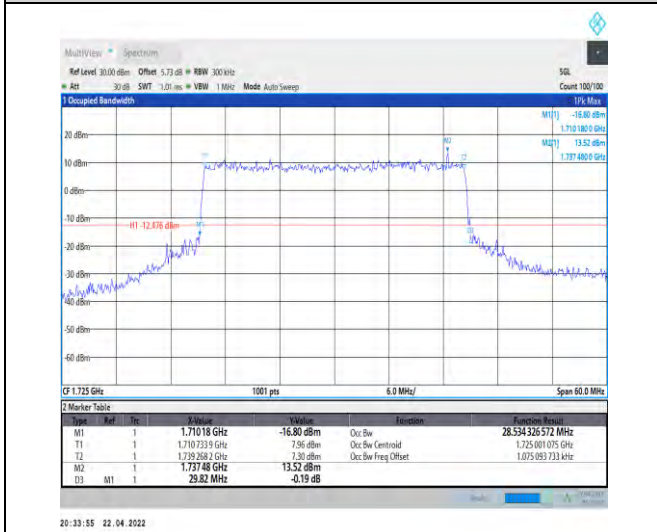
1-N66-PC3-15-30-L-7-CP-16QAM-Outer_Full-160@0-Ant0-28.534-29.820-≤30-PASS
