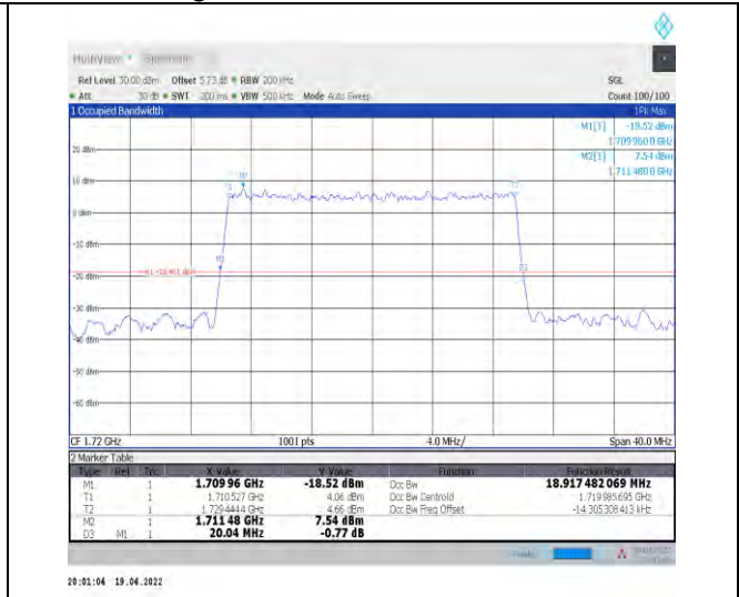
1-N66-PC3-15-20-L-9-CP-256QAM-Outer_Full-106 @0-Ant0-18.917-20.040-≤20-PASS
