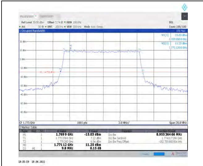
1-N66-PC3-15-10-H-4-DFT-64QAM-Outer_Full-50@ 0-Ant0-8.955-9.800-≤10-PASS
